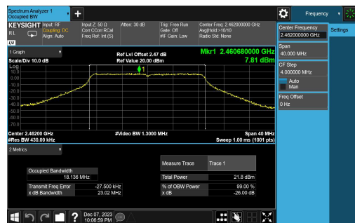
11N20MIMO-Ant2-2462
