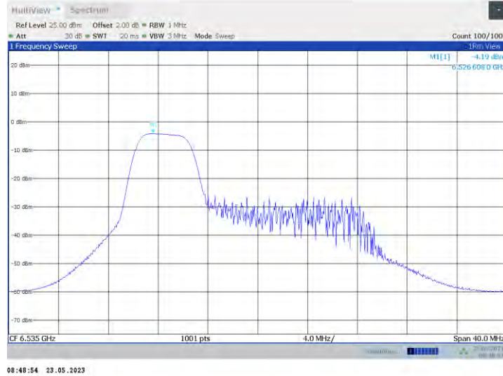
11ax20MIMO Ant1_6535_106Tone_RU53
