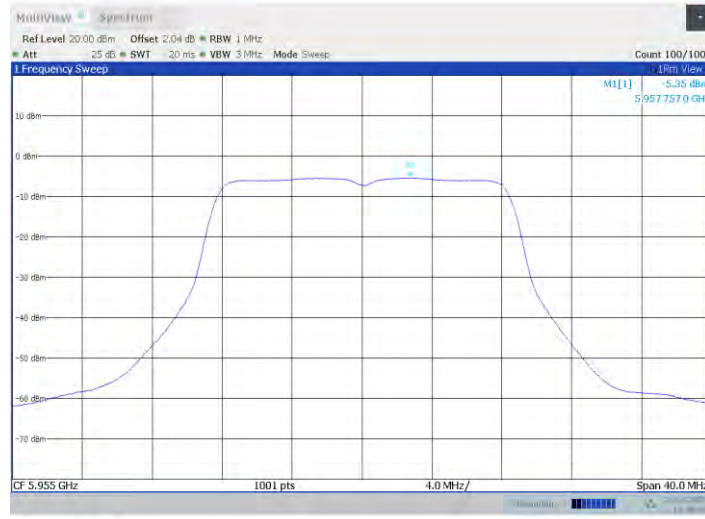
11a-CDD Ant1_5955
