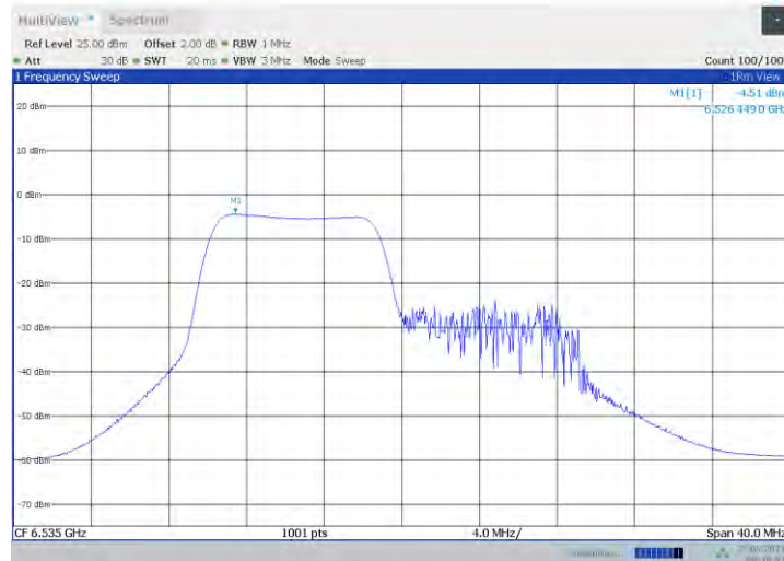
11ax20MIMO Ant1_6535_106Tone_RU53
