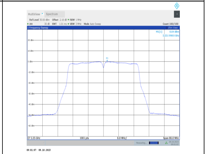
11n40SISO-Ant1-5550-PASS
