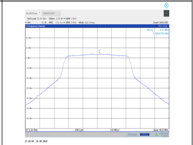
11n20SISO-Ant1-5320-PASS
