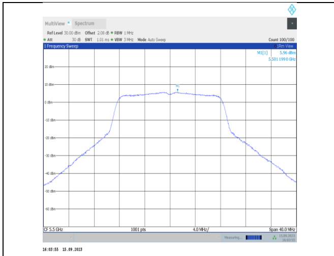
11a-Ant1-5500-PASS
