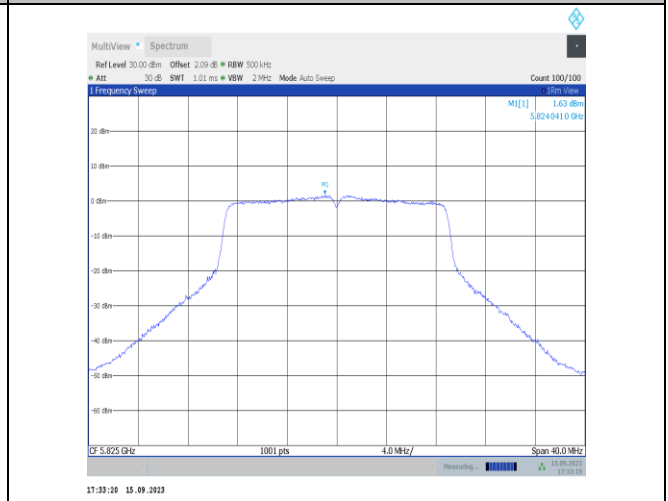
11n20SISO-Ant1-5825-PASS
