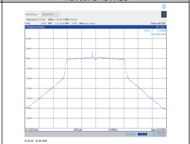
11a-Ant1-5825-PASS
