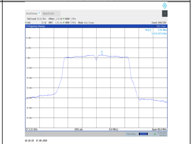
11n40SISO-Ant1-5310-PASS
