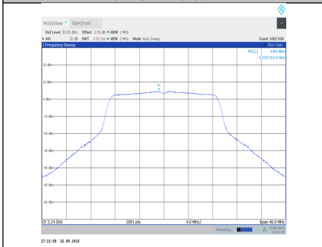
11n20SISO-Ant1-5240-PASS
