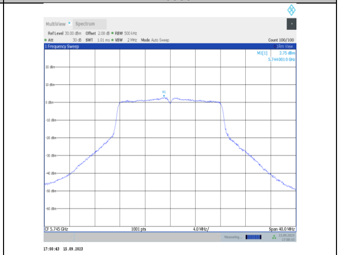
11a-Ant1-5745-PASS
