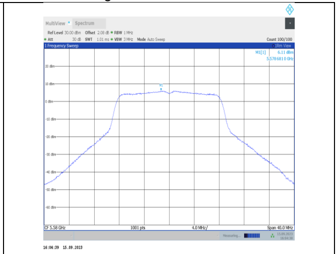
11a-Ant1-5580-PASS
