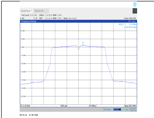
11n40SISO-Ant1-5190-PASS
