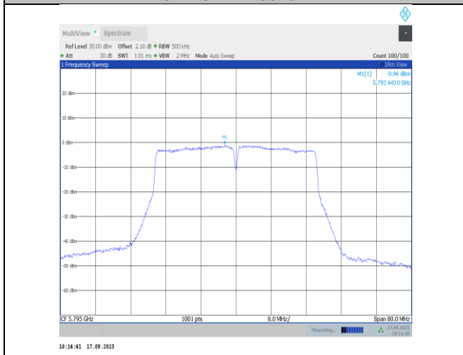
11n40SISO-Ant1-5795-PASS
