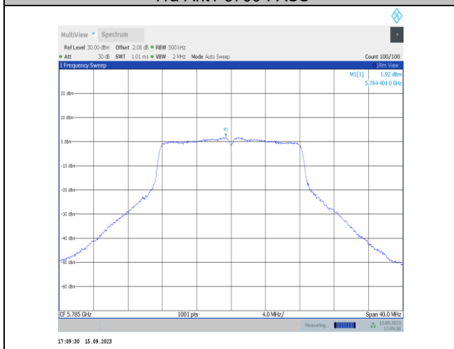
11a-Ant1-5785-PASS
