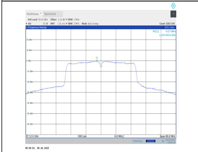
11n40SISO-Ant1-5510-PASS
