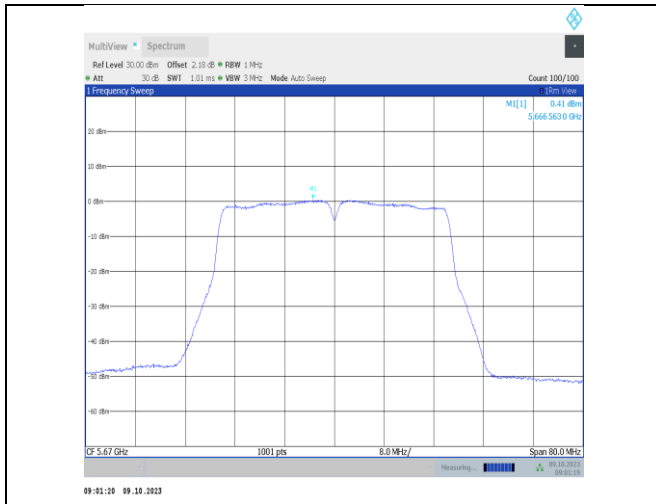
11n40SISO-Ant1-5670-PASS
