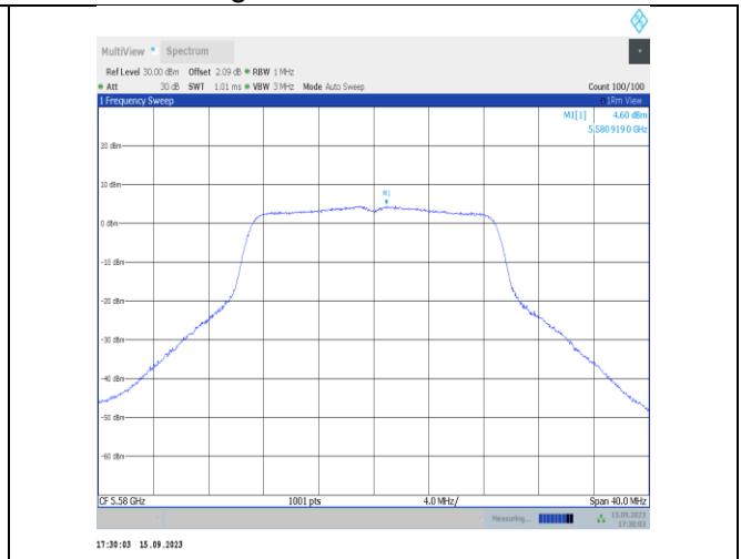
11n20SISO-Ant1-5580-PASS
