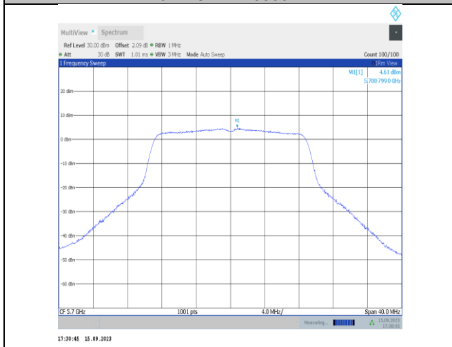
11n20SISO-Ant1-5700-PASS
