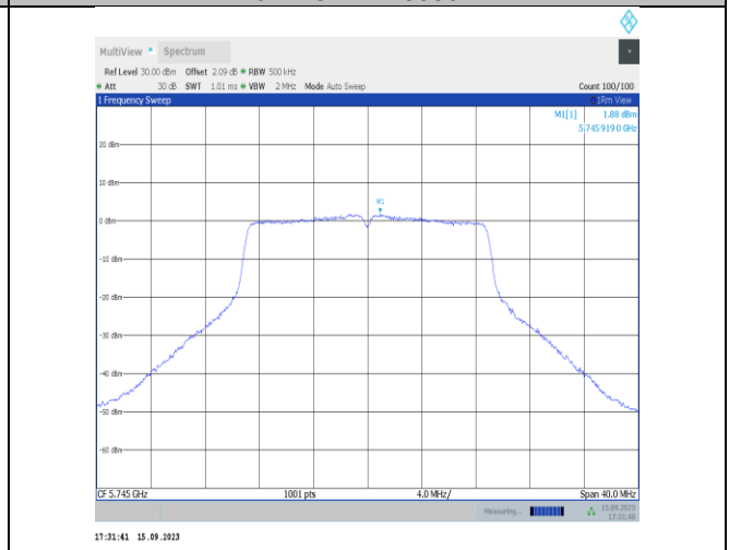
11n20SISO-Ant1-5745-PASS
