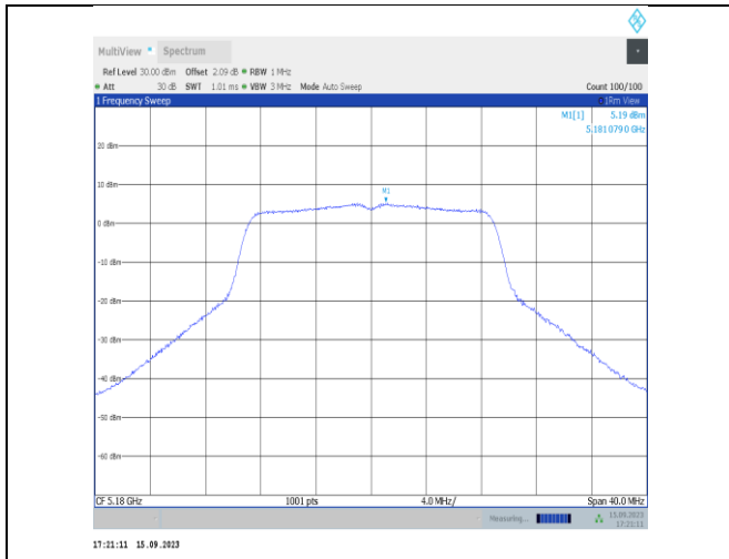
11n20SISO-Ant1-5180-PASS
