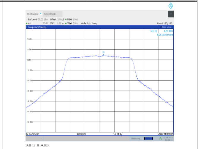
11n20SISO-Ant1-5260-PASS
