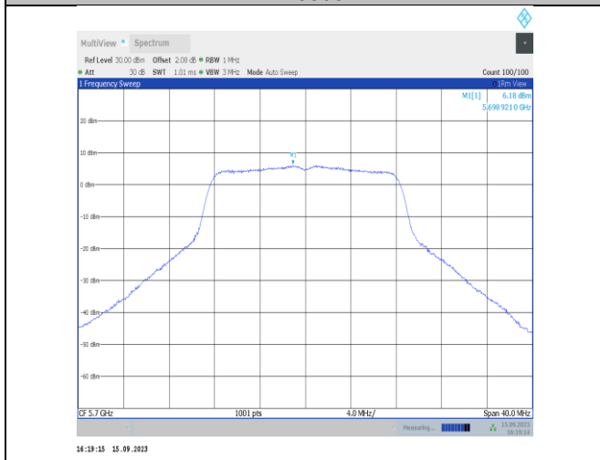
11a-Ant1-5700-PASS
