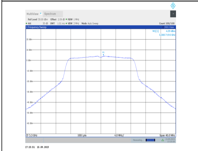
11n20SISO-Ant1-5300-PASS
