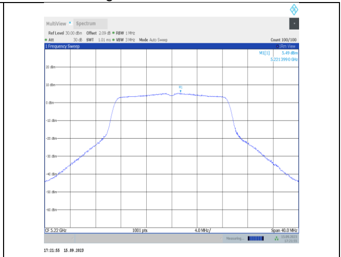
11n20SISO-Ant1-5220-PASS
