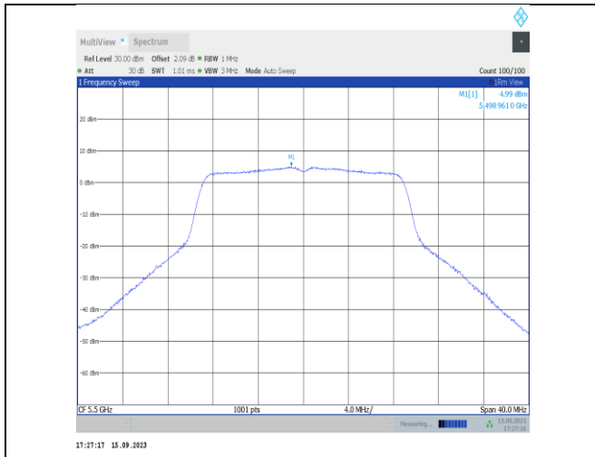
11n20SISO-Ant1-5500-PASS
