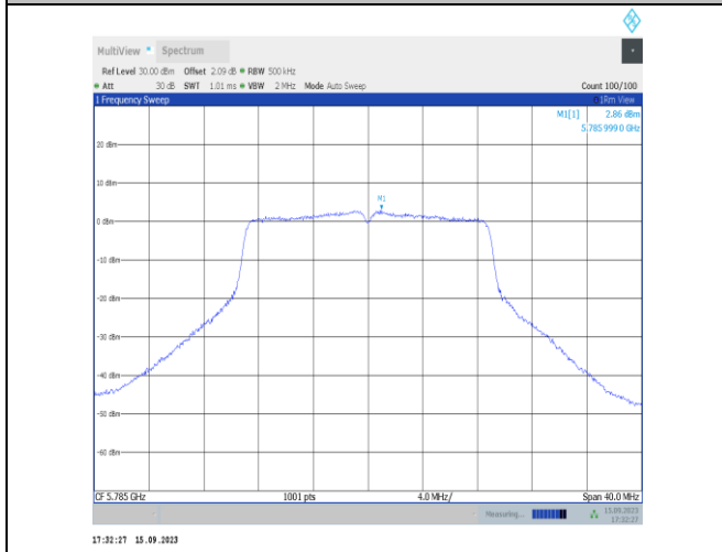
11n20SISO-Ant1-5785-PASS
