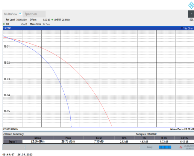
Band71-20MHz-QPSK-133322-100RB#0
