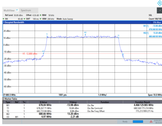
Band71-5MHz-16QAM-133297-25RB#0
