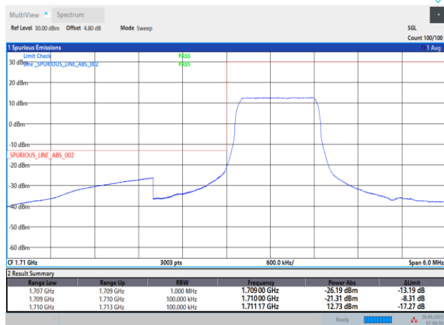
Band66-1.4MHz-QPSK-131979-6RB#0
