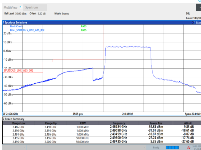
Band41-5MHz-QPSK-39675-25RB#0
