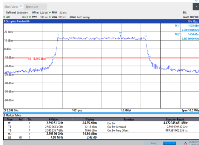
Band41-5MHz-16QAM-40620-25RB#0
