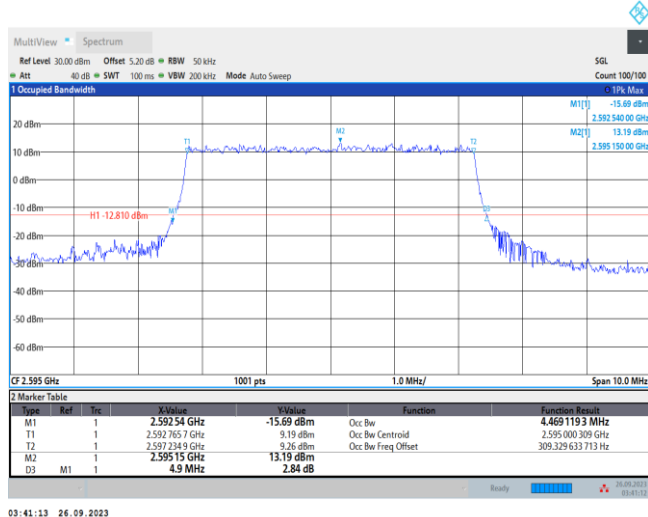
Band38-5MHz-16QAM-38000-25RB#0
