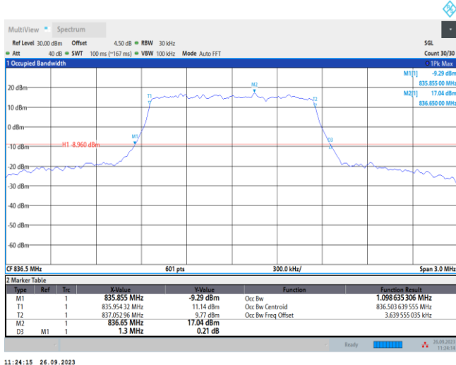
Band26-1.4MHz-16QAM-26915-6RB#0
