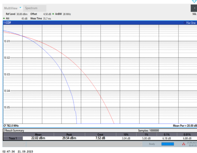
Band13-10MHz-16QAM-23230-50RB#0
