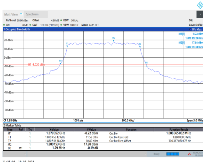
Band2-1.4MHz-16QAM-18900-6RB#0
