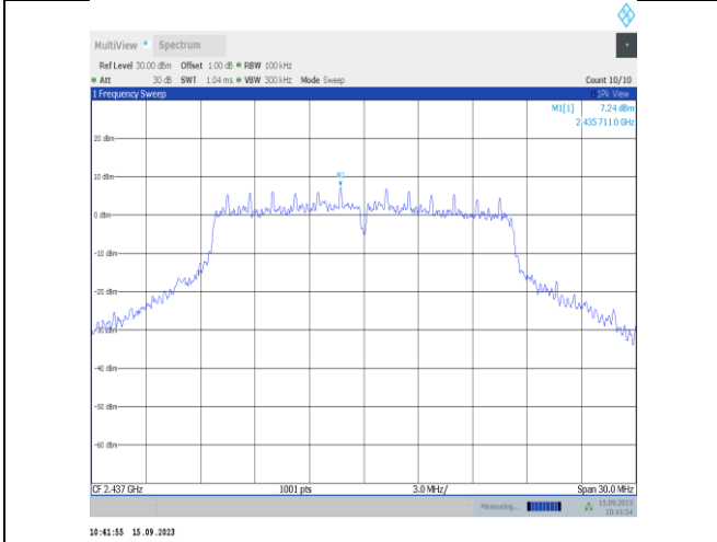
11g-Ant1-2437-0~Reference-PASS
