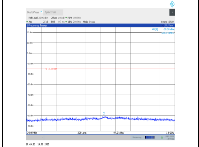
11n20SISO-Ant1-2412-30~1000-PASS
