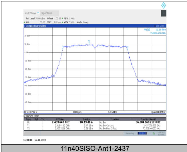
11n40SISO-Ant1-2437
