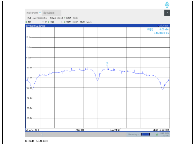
11b-Ant1-2437-PASS
