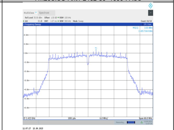
11n40SISO-Ant1-2422-0~Reference-PASS
