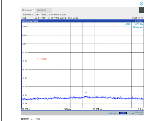
11n40SISO-Ant1-2437-30~1000-PASS
