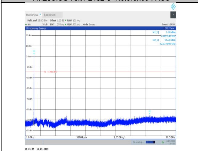
11n20SISO-Ant1-2462-1000~26500-PASS
