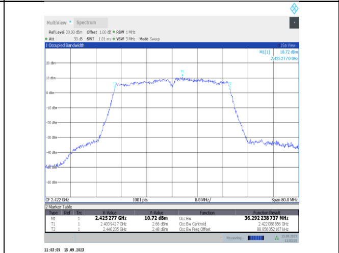
11n40SISO-Ant1-2422
