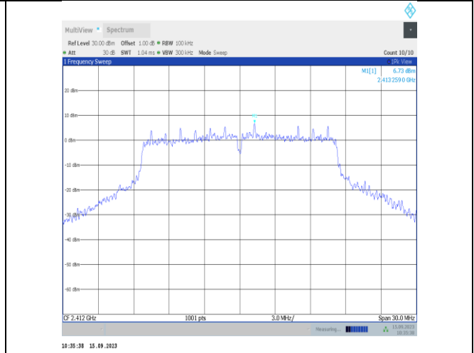
11g-Ant1-2412-0~Reference-PASS
