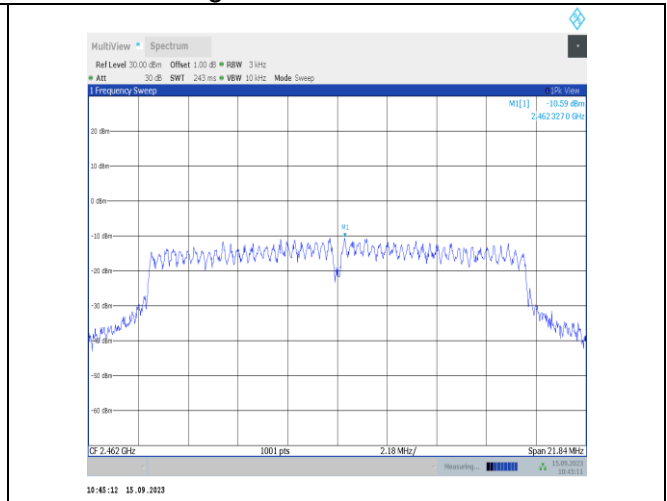
11g-Ant1-2462-PASS
