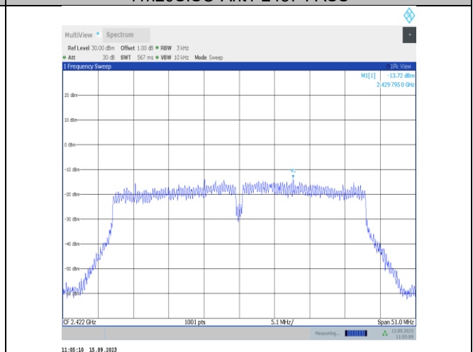
11n40SISO-Ant1-2422-PASS
