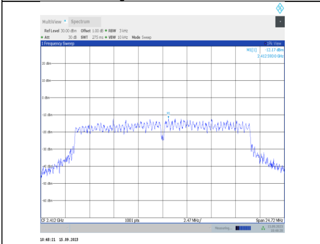
11n20SISO-Ant1-2412-PASS
