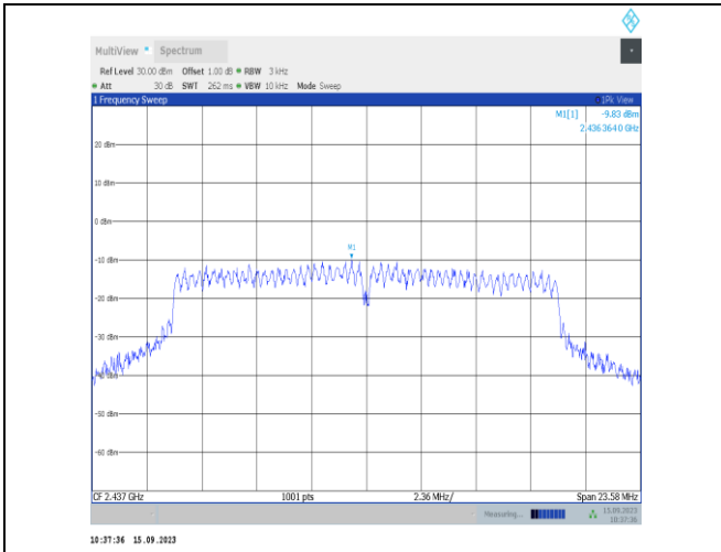
11g-Ant1-2437-PASS
