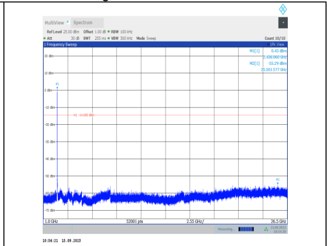
11n20SISO-Ant1-2437-1000~26500-PASS
