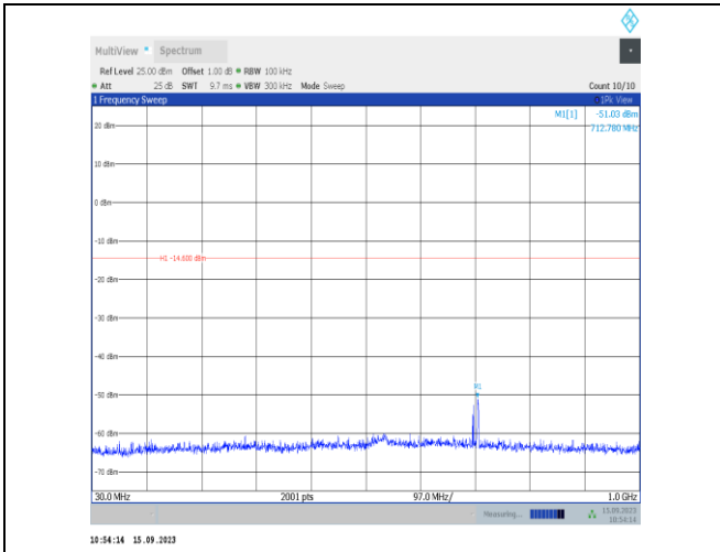
11n20SISO-Ant1-2437-30~1000-PASS
