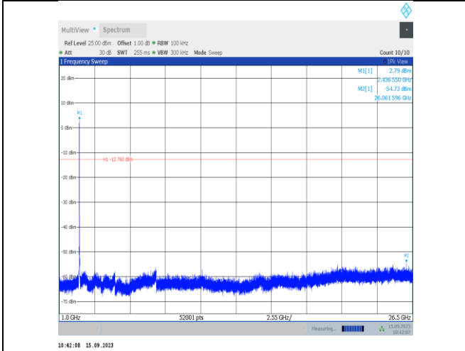
11g-Ant1-2437-1000~26500-PASS
