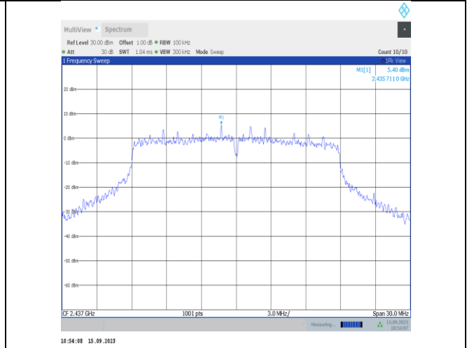
11n20SISO-Ant1-2437-0~Reference-PASS
