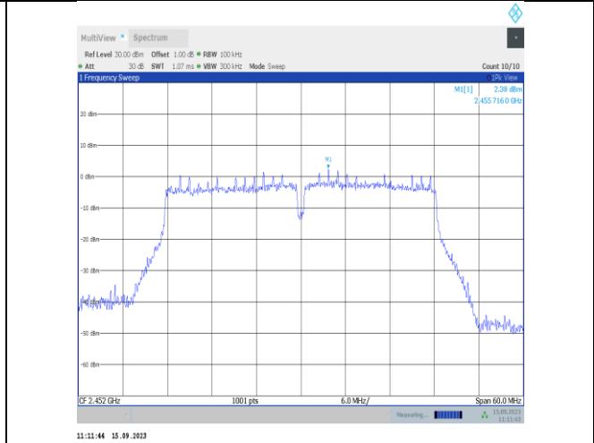
11n40SISO-Ant1-2452-0~Reference-PASS
