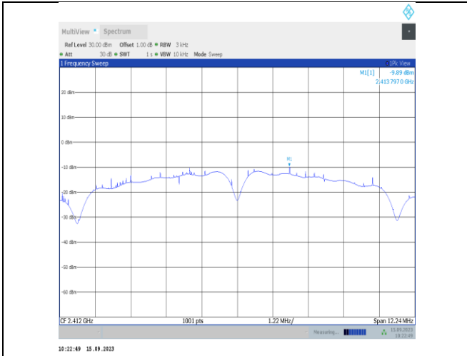
11b-Ant1-2412-PASS
