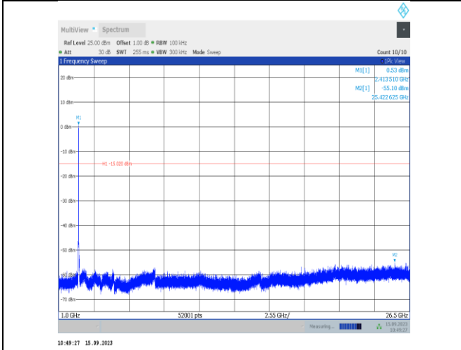
11n20SISO-Ant1-2412-1000~26500-PASS
