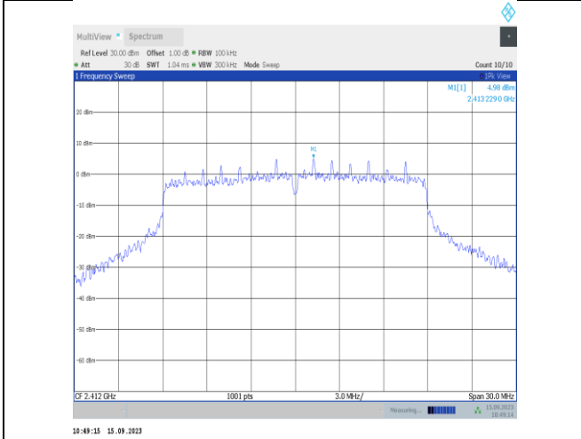
11n20SISO-Ant1-2412-0~Reference-PASS
