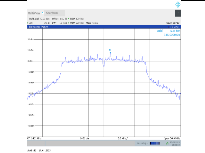
11g-Ant1-2462-0~Reference-PASS
