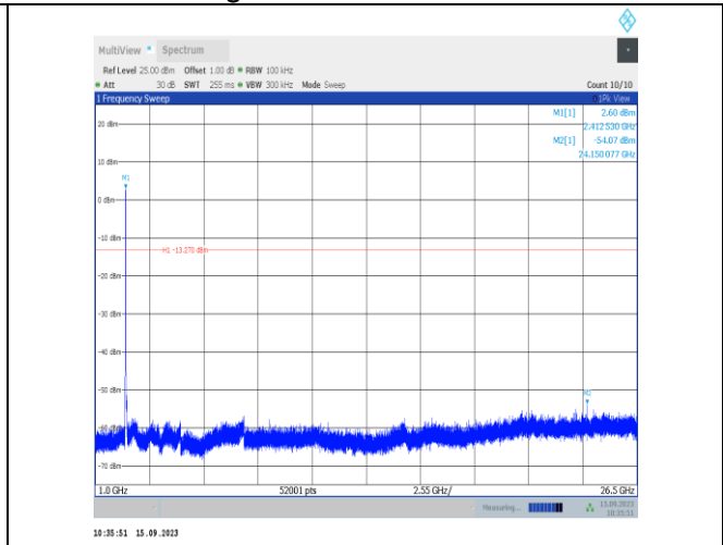
11g-Ant1-2412-1000~26500-PASS
