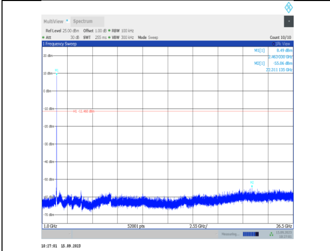
11b-Ant1-2462-1000~26500-PASS
