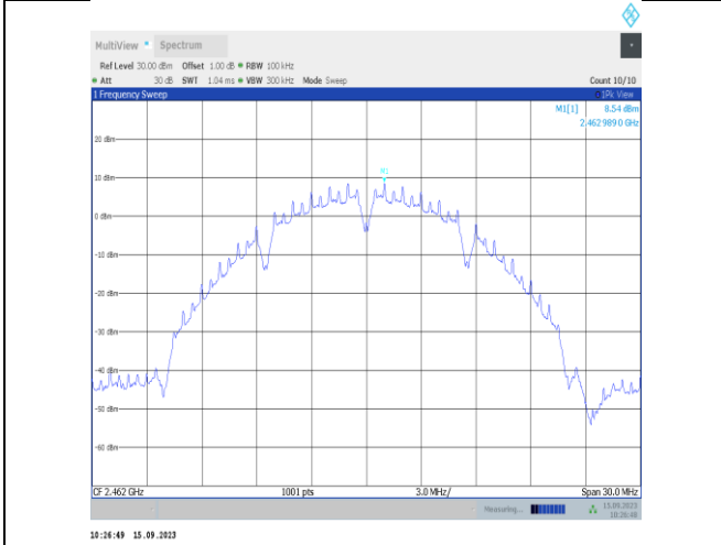
11b-Ant1-2462-0~Reference-PASS
