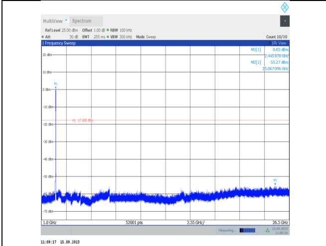
11n40SISO-Ant1-2437-1000~26500-PASS
