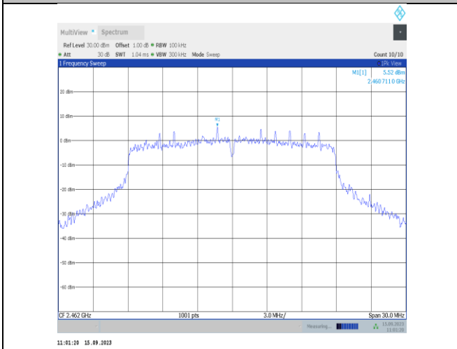
11n20SISO-Ant1-2462-0~Reference-PASS
