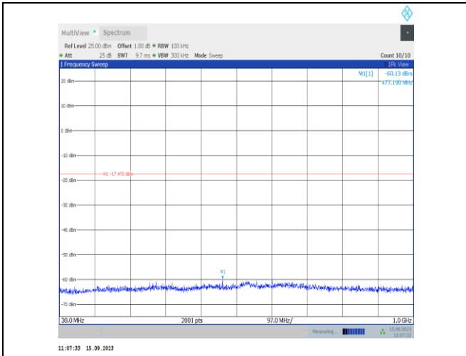
11n40SISO-Ant1-2422-30~1000-PASS
