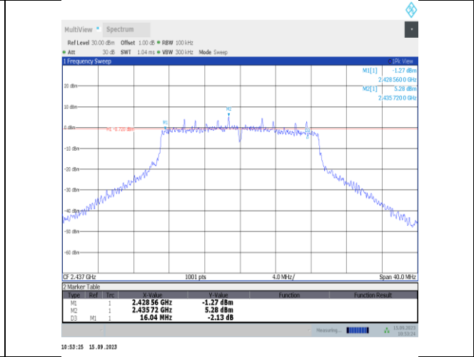
11n20SISO-Ant1-2437-PASS
