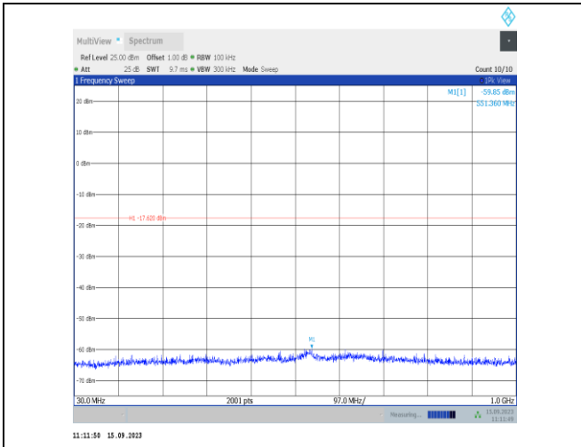
11n40SISO-Ant1-2452-30~1000-PASS
