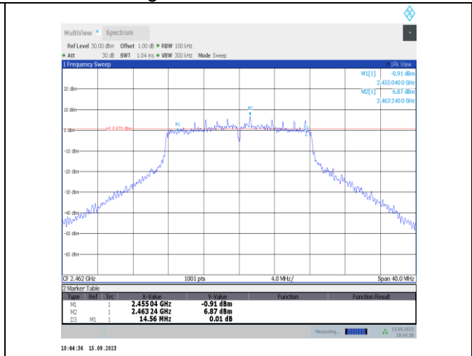
11g-Ant1-2462-PASS
