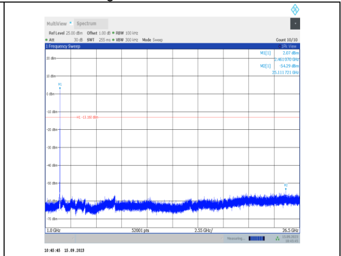
11g-Ant1-2462-1000~26500-PASS
