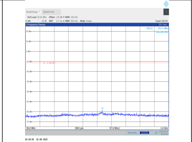
11b-Ant1-2462-30~1000-PASS
