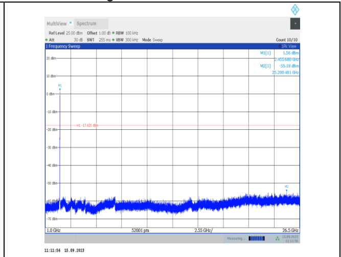
11n40SISO-Ant1-2452-1000~26500-PASS
