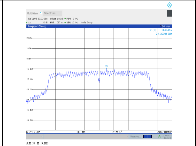
11g-Ant1-2412-PASS
