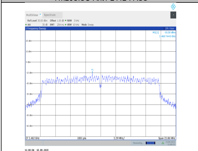
11n20SISO-Ant1-2462-PASS
