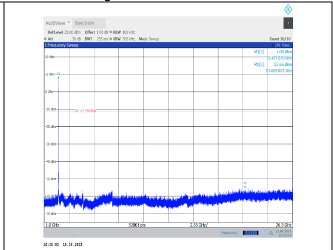
11b-Ant1-2437-1000~26500-PASS
