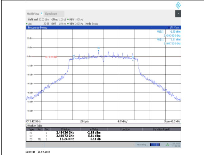
11n20SISO-Ant1-2462-PASS
