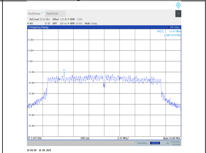
11n20SISO-Ant1-2437-PASS
