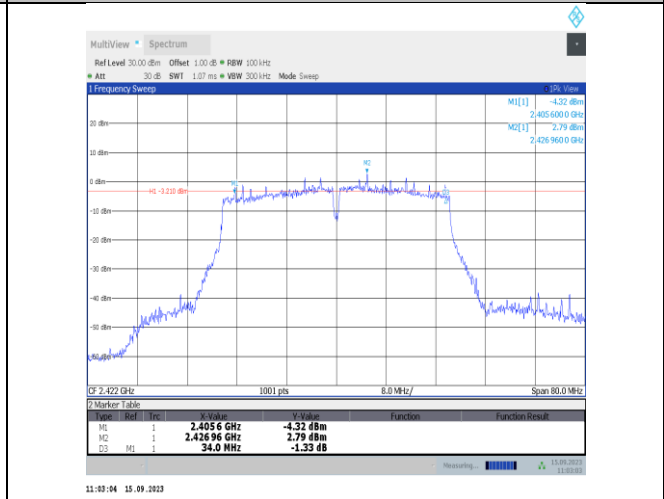
11n40SISO-Ant1-2422-PASS
