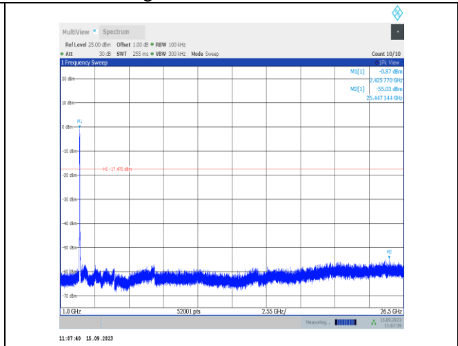
11n40SISO-Ant1-2422-1000~26500-PASS
