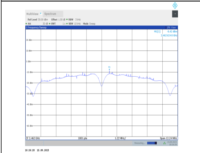
11b-Ant1-2462-PASS
