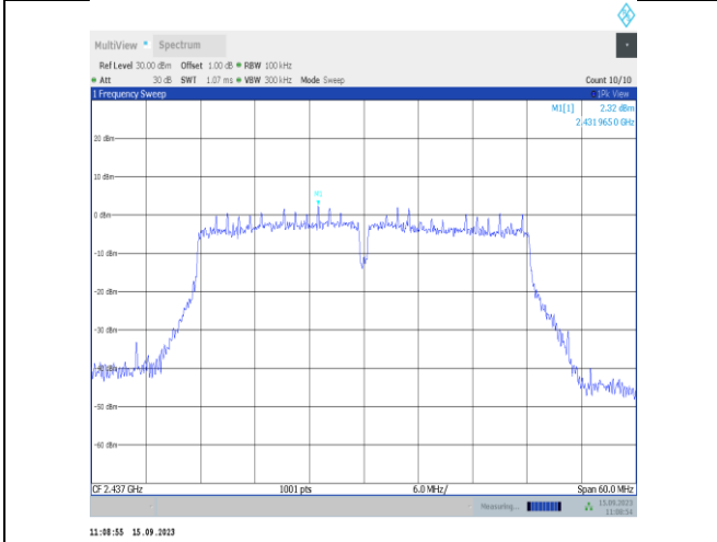
11n40SISO-Ant1-2437-0~Reference-PASS
