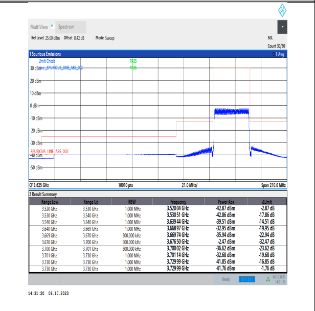
NTNV_N48_PC3_30_30_H_TID6_RID1#1
