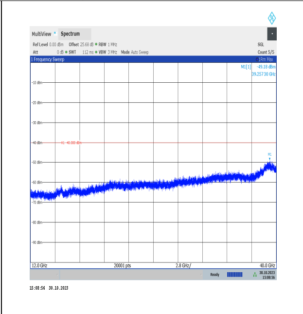
NTNV_N48_PC3_30_30_L_TID1_NS_01_12000_40000_#
