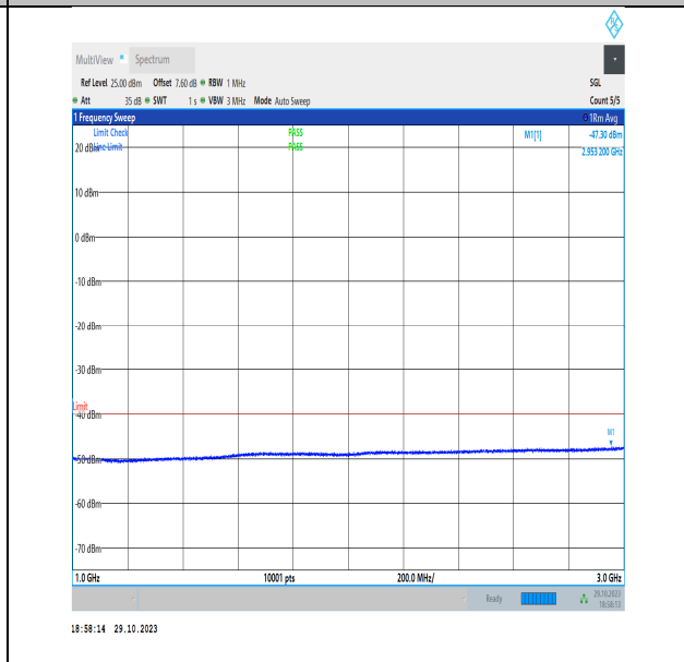
NTNV_N48_PC3_30_30_H_TID1_NS_01_1000_3000_#1
