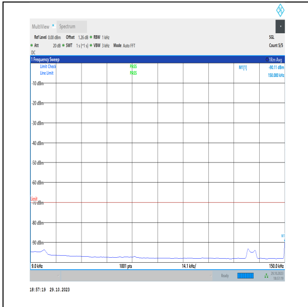
NTNV_N48_PC3_30_30_H_TID1_NS_01_0.009_0.15_#1
