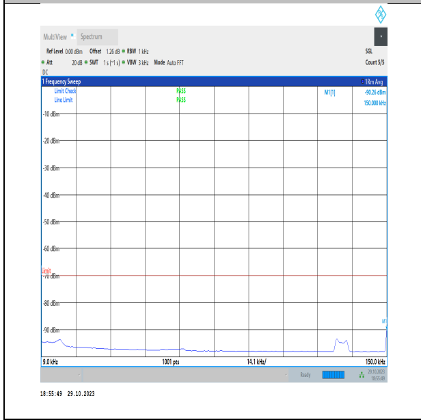
NTNV_N48_PC3_30_30_M_TID1_NS_01_0.009_0.15_#
