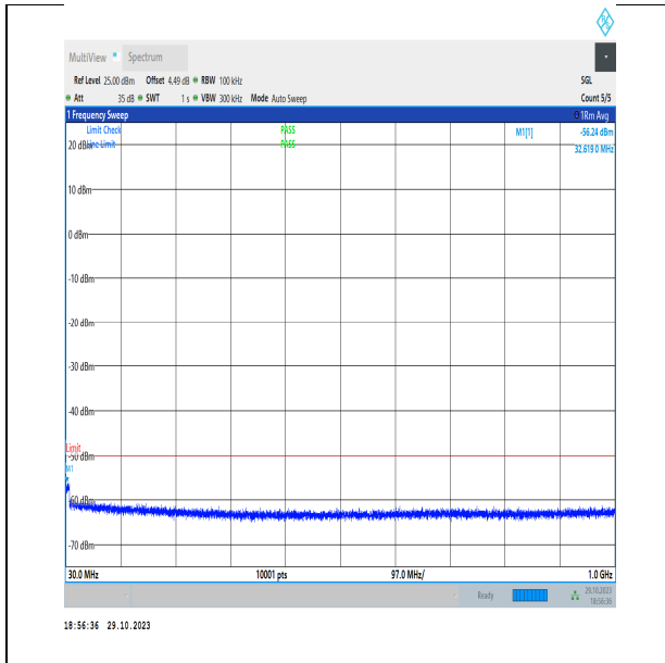
NTVN_N48_PC3_30_30_M_TID1_NS_01_30_1000_#1
