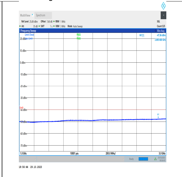
NTVN_N48_PC3_30_30_M_TID1_NS_01_1000_3000_#1
