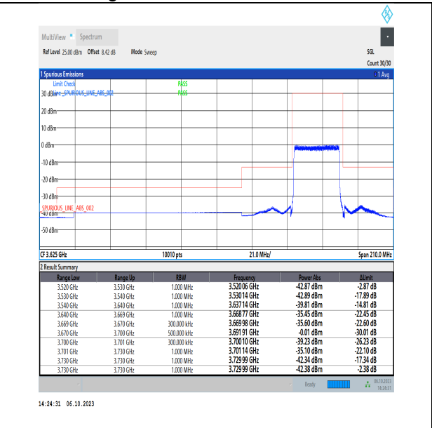
NTNV_N48_PC3_30_30_H_TID3_RID1#1
