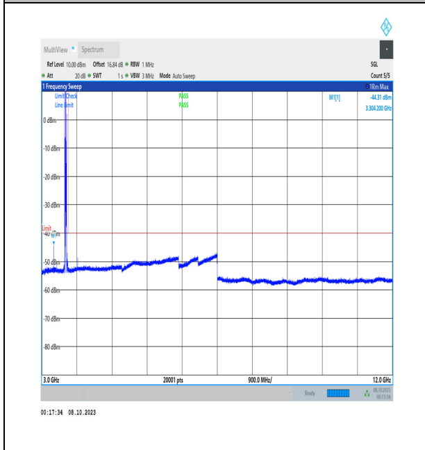
NTVN_N48_PC3_30_30_M_TID1_NS_01_3000_12000_#1
