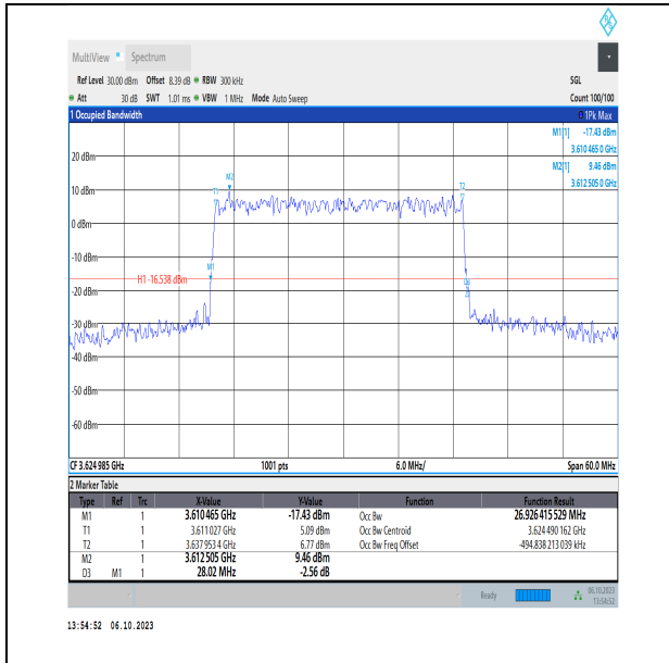
NTNV_N48_PC3_30_30_M_TID5_Ant2#1
