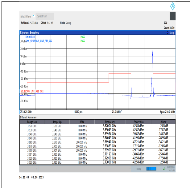
NTNV_N48_PC3_30_30_H_TID2_RID1#1
