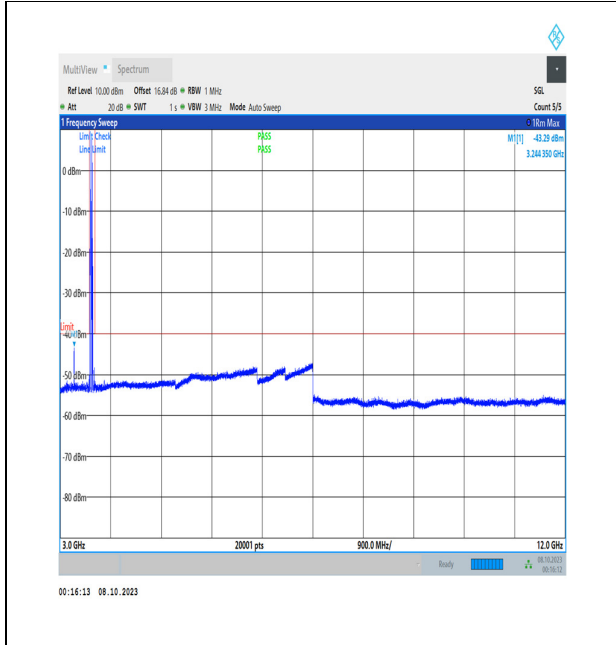
NTNV_N48_PC3_30_30_L_TID1_NS_01_3000_12000_#
