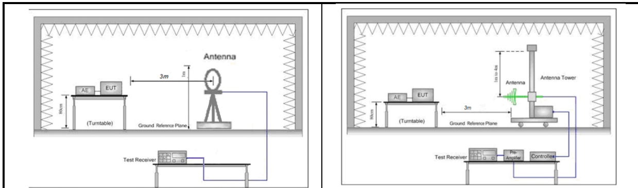
Figure 2. 30MHz to 1GHz
