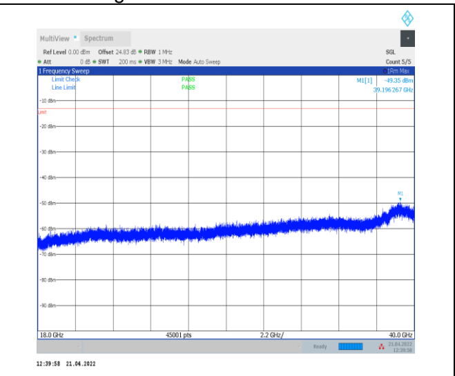
1-N78-3700-3800--30-100-H-1-DFT-PI2BPSK-Inner_ 1RB_Left-1 @ 1-18000-40000-Ant0--49.35--13-PASS
