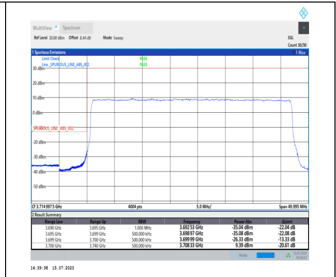
1-N78-3700-3800-PC1-30-40-L-3-DFT-PI2BPSK-Outer_Full-100@0-Ant0-1--PASS-see graph
