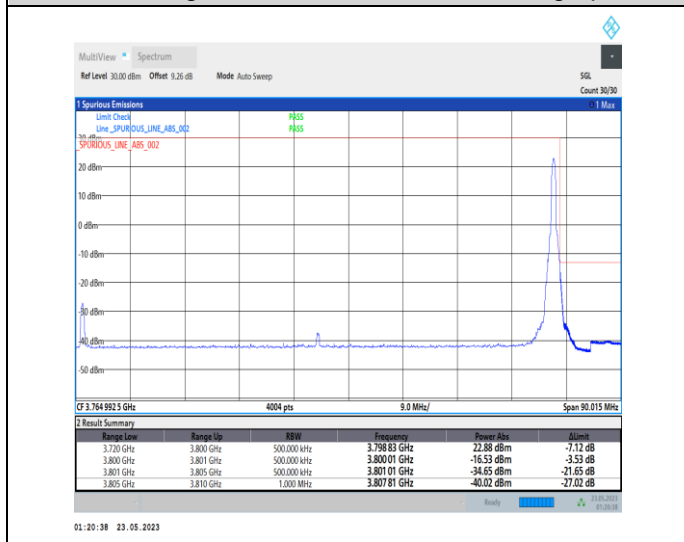
1-N78-3700-3800-PC1-30-80-H-5-CP-QPSK-Edge_1R B_Right-1@216-Ant0-1--PASS-see graph
