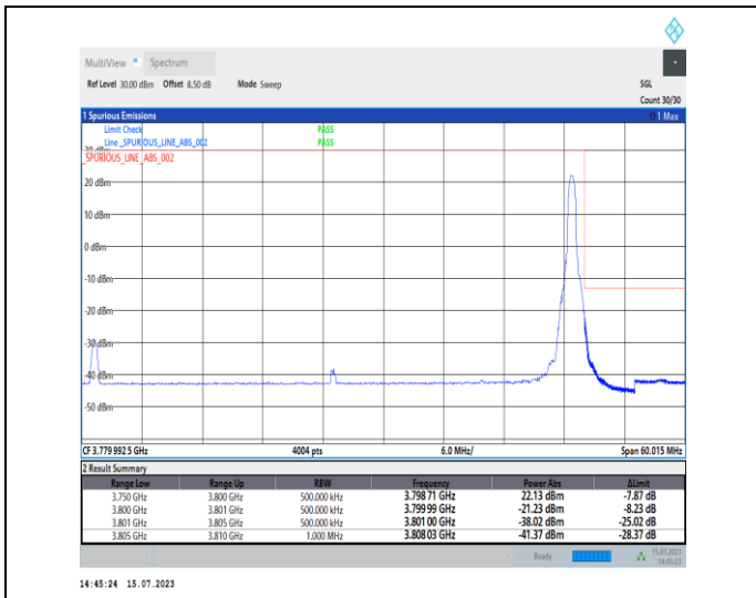
1-N78-3700-3800-PC1-30-50-H-2-DFT-PI2BPSK-Edge _1RB_Right-1@132-Ant0-1--PASS-see graph
