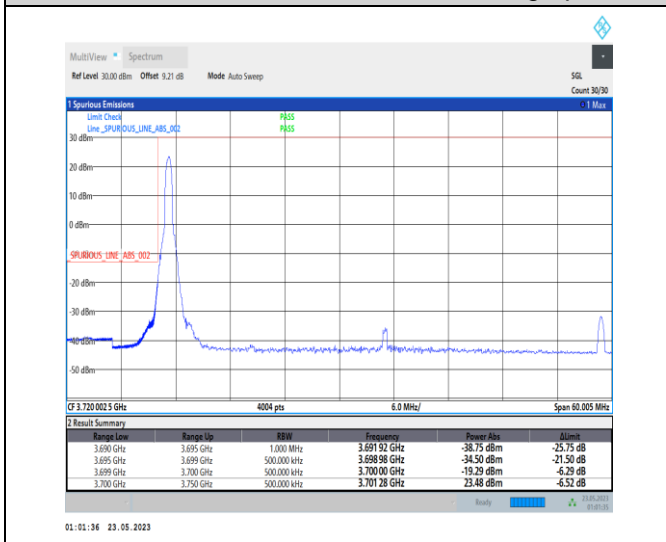
1-N78-3700-3800-PC1-30-50-L-4-CP-QPSK-Edge_1_RB_Left-1@0-Ant0-1--PASS-see graph
