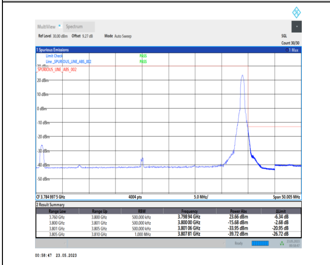
1-N78-3700-3800-PC1-30-40-H-5-CP-QPSK-Edge_1RB_Right-1@105-Ant0-1--PASS-see graph
