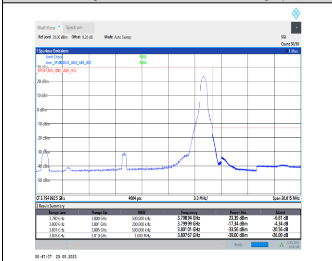
1-N78-3700-3800-PC1-30-20-H-5-CP-QPSK-Edge_1R B_Right-1@50-Ant0-1--PASS-see graph
