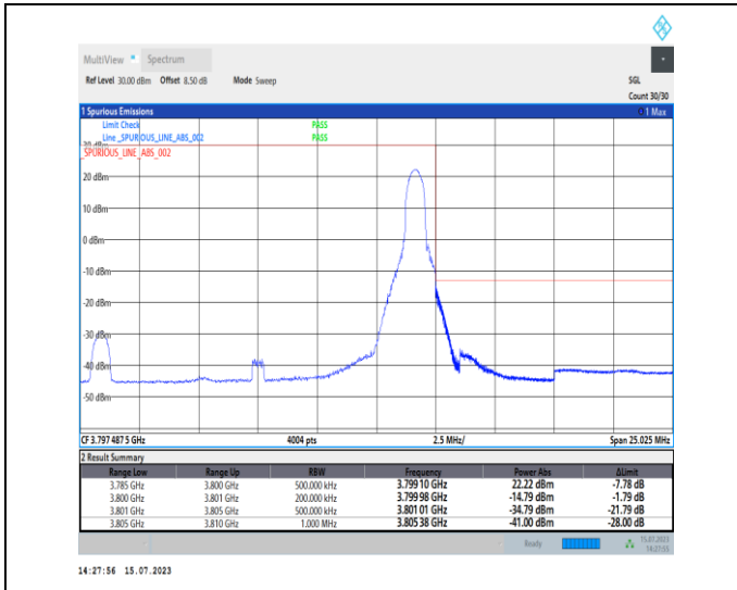
1-N78-3700-3800-PC1-30-15-H-2-DFT-PI2BPSK-Edge _1RB_Right-1@37-Ant0-1--PASS-see graph
