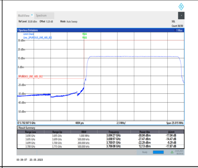
1-N78-3700-3800-PC1-30-15-L-6-CP-QPSK-Outer_Full-38@0-Ant0-1--PASS-see graph
