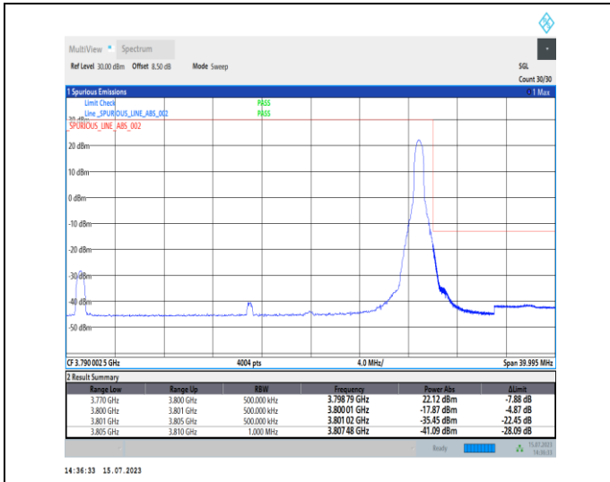
1-N78-3700-3800-PC1-30-30-H-2-DFT-PI2BPSK-Edge _1RB_Right-1@77-Ant0-1--PASS-see graph
