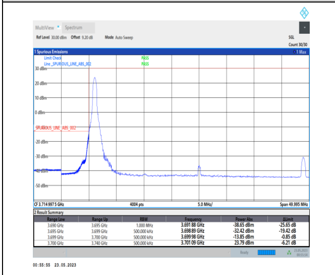
1-N78-3700-3800-PC1-30-40-L-4-CP-QPSK-Edge_1_RB_Left-1@0-Ant0-1--PASS-see graph
