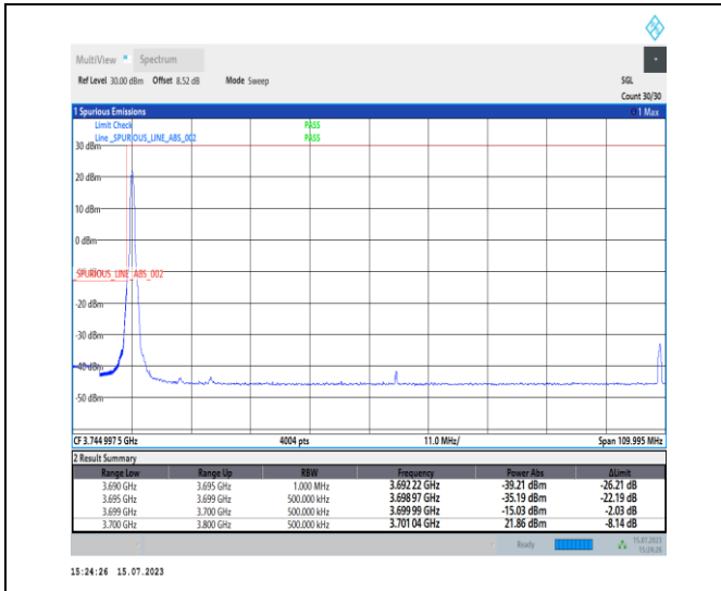
1-N78-3700-3800-PC1-30-100-L-1-DFT-PI2BPSK-Edge_1RB_Left-1@0-Ant0-1--PASS-see graph
