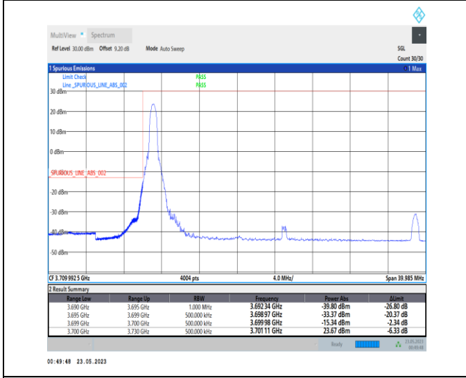
1-N78-3700-3800-PC1-30-30-L-4-CP-QPSK-Edge_1RB_Left-1@0-Ant0-1--PASS-see graph
