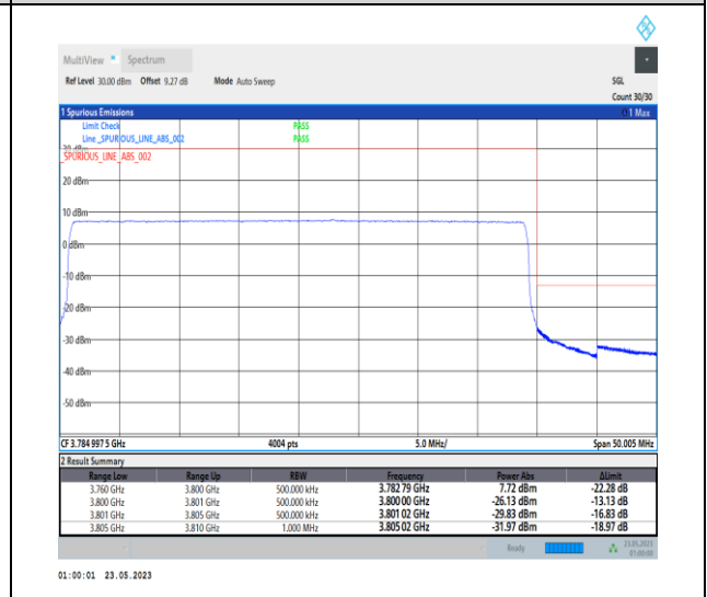
1-N78-3700-3800-PC1-30-40-H-6-CP-QPSK-Outer_Full-106@0-Ant0-1--PASS-see graph
