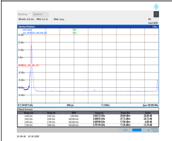
1-N78-3700-3800-PC1-30-100-L-4-CP-QPSK-Edge_1RB_Left-1@0-Ant0-1--PASS-see graph
