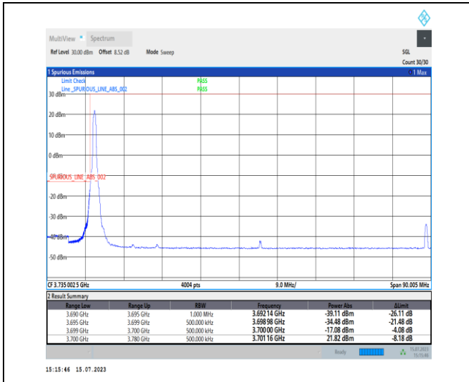
1-N78-3700-3800-PC1-30-80-L-1-DFT-PI2BPSK-Edge_1_RB_Left-1@0-Ant0-1--PASS-see graph
