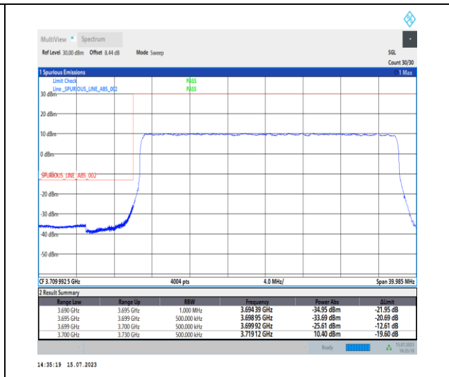
1-N78-3700-3800-PC1-30-30-L-3-DFT-PI2BPSK-Outer_Full-75@0-Ant0-1--PASS-see graph
