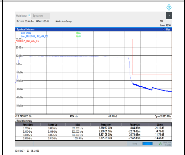
1-N78-3700-3800-PC1-30-30-H-6-CP-QPSK-Outer _Full-78@0-Ant0-1--PASS-see graph
