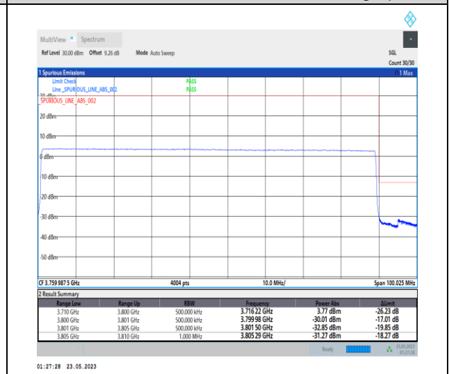
1-N78-3700-3800-PC1-30-90-H-6-CP-QPSK-Outer_Full-245@0-Ant0-1--PASS-see graph
