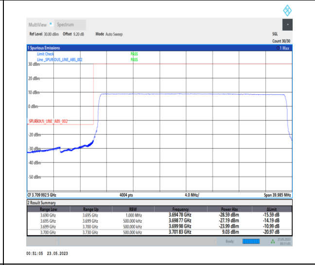
1-N78-3700-3800-PC1-30-30-L-6-CP-QPSK-Outer_Full-78@0-Ant0-1--PASS-see graph
