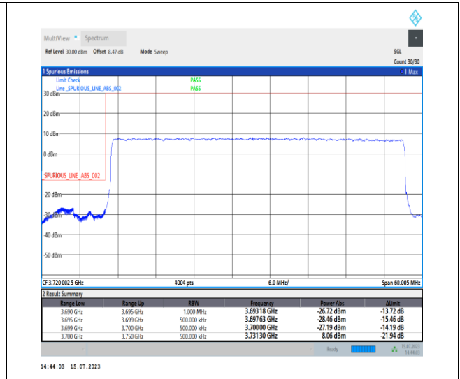
1-N78-3700-3800-PC1-30-50-L-3-DFT-PI2BPSK-Outer_Full-128@0-Ant0-1--PASS-see graph
