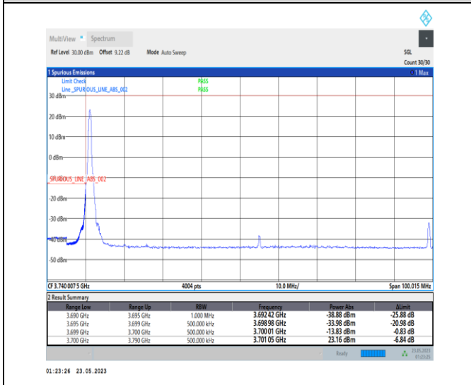
1-N78-3700-3800-PC1-30-90-L-4-CP-QPSK-Edge_1_RB_Left-1@0-Ant0-1--PASS-see graph
