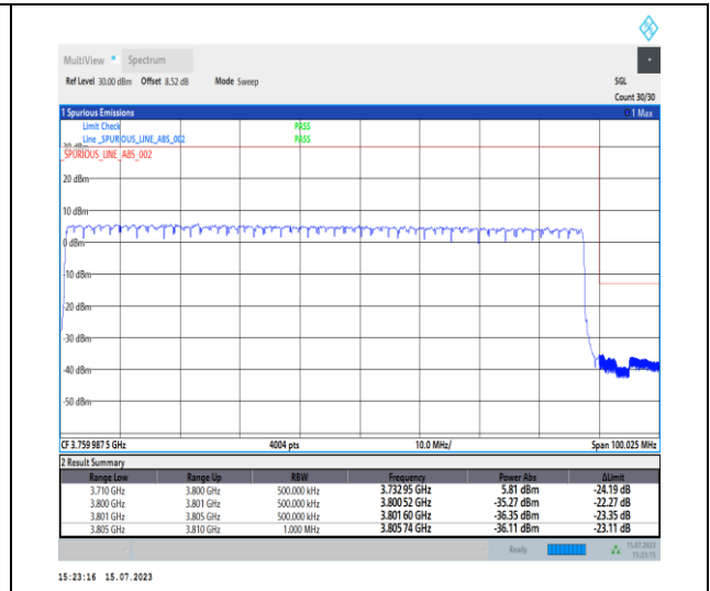
1-N78-3700-3800-PC1-30-90-H-3-DFT-PI2BPSK-Outer_Full-240@0-Ant0-1--PASS-see graph
