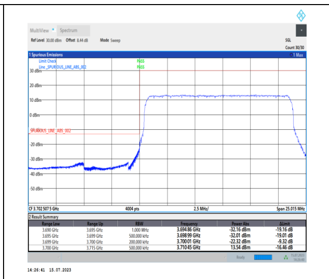
1-N78-3700-3800-PC1-30-15-L-3-DFT-PI2BPSK-Outer_Full-36@0-Ant0-1--PASS-see graph
