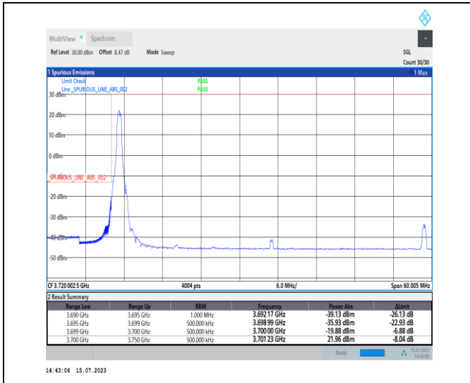
1-N78-3700-3800-PC1-30-50-L-1-DFT-PI2BPSK-Edge_1_RB_Left-1@0-Ant0-1--PASS-see graph
