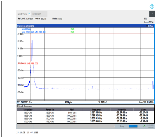
1-N78-3700-3800-PC1-30-90-L-1-DFT-PI2BPSK-Edge_1_RB_Left-1@0-Ant0-1--PASS-see graph
