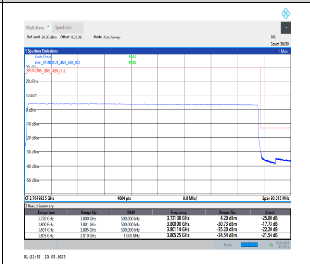
1-N78-3700-3800-PC1-30-80-H-6-CP-QPSK-Outer _Full-217@0-Ant0-1--PASS-see graph
