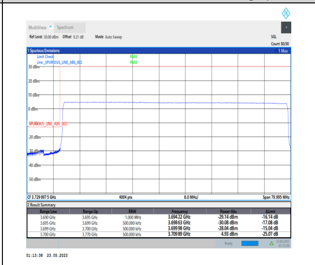
1-N78-3700-3800-PC1-30-70-L-6-CP-QPSK-Outer_Full-189@0-Ant0-1--PASS-see graph
