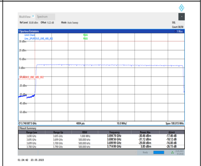
1-N78-3700-3800-PC1-30-90-L-6-CP-QPSK-Outer_Full-245@0-Ant0-1--PASS-see graph
