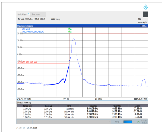
1-N78-3700-3800-PC1-30-15-L-1-DFT-PI2BPSK-Edge_e_1RB_Left-1@0-Ant0-1--PASS-see graph
