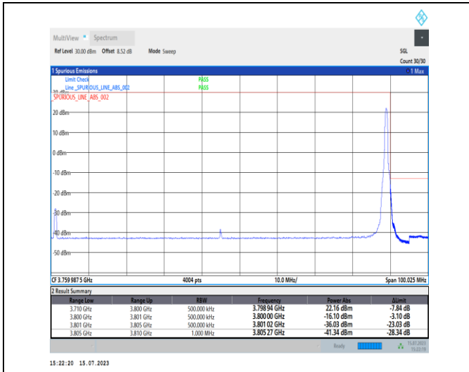
1-N78-3700-3800-PC1-30-90-H-2-DFT-PI2BPSK-Edge_1RB_Right-1@244-Ant0-1--PASS-see graph
