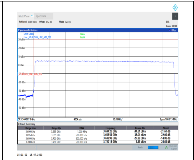
1-N78-3700-3800-PC1-30-90-L-3-DFT-PI2BPSK-Outer_Full-240@0-Ant0-1--PASS-see graph
