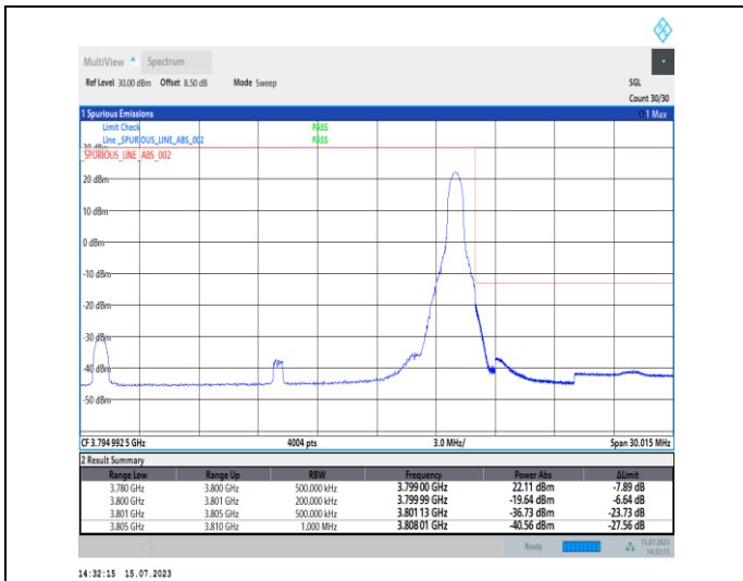
1-N78-3700-3800-PC1-30-20-H-2-DFT-PI2BPSK-Edge _1RB_Right-1@50-Ant0-1--PASS-see graph
