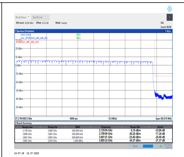
1-N78-3700-3800-PC1-30-80-H-3-DFT-PI2BPSK- Outer_Full-216@0-Ant0-1--PASS-see graph
