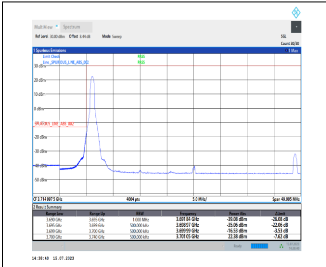
1-N78-3700-3800-PC1-30-40-L-1-DFT-PI2BPSK-Edge_1_RB_Left-1@0-Ant0-1--PASS-see graph
