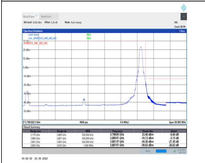
1-N78-3700-3800-PC1-30-30-H-5-CP-QPSK-Edge_1R B_Right-1@77-Ant0-1--PASS-see graph
