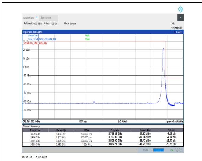
1-N78-3700-3800-PC1-30-80-H-2-DFT-PI2BPSK-Edge _1RB_Right-1@216-Ant0-1--PASS-see graph
