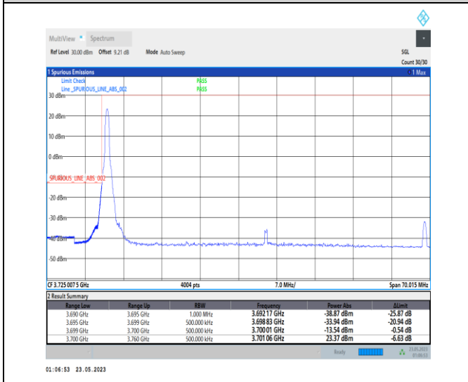
1-N78-3700-3800-PC1-30-60-L-4-CP-QPSK-Edge_1_RB_Left-1@0-Ant0-1--PASS-see graph
