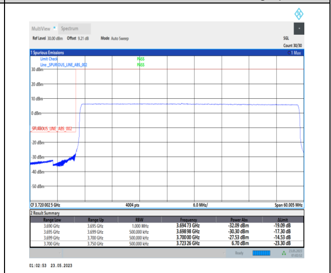
1-N78-3700-3800-PC1-30-50-L-6-CP-QPSK-Outer_Full-133@0-Ant0-1--PASS-see graph
