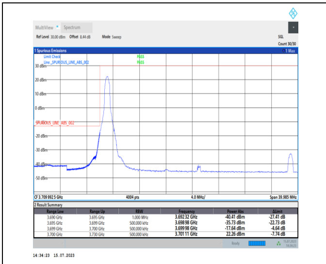
1-N78-3700-3800-PC1-30-30-L-1-DFT-PI2BPSK-Edge_1RB_Left-1@0-Ant0-1--PASS-see graph
