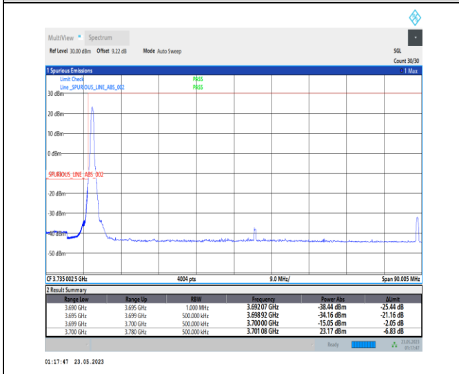
1-N78-3700-3800-PC1-30-80-L-4-CP-QPSK-Edge_1_RB_Left-1@0-Ant0-1--PASS-see graph
