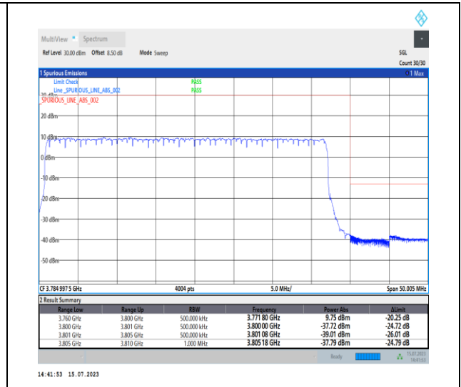
1-N78-3700-3800-PC1-30-40-H-3-DFT-PI2BPSK-Outer_Full-100@0-Ant0-1--PASS-see graph
