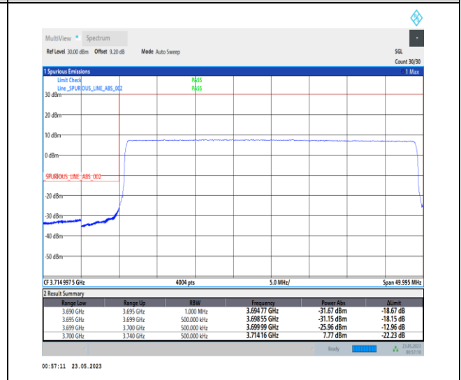
1-N78-3700-3800-PC1-30-40-L-6-CP-QPSK-Outer_Full-106@0-Ant0-1--PASS-see graph
