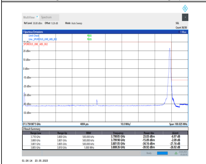
1-N78-3700-3800-PC1-30-90-H-5-CP-QPSK-Edge_1RB_Right-1@244-Ant0-1--PASS-see graph
