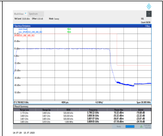
1-N78-3700-3800-PC1-30-30-H-3-DFT-PI2BPSK- Outer_Full-75@0-Ant0-1--PASS-see graph
