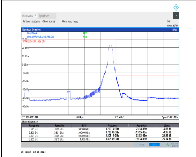
1-N78-3700-3800-PC1-30-15-H-5-CP-QPSK-Edge_1R B_Right-1@37-Ant0-1--PASS-see graph
