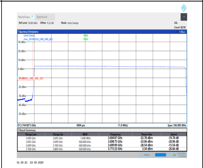
1-N78-3700-3800-PC1-30-100-L-6-CP-QPSK-Outer_Full-273@0-Ant0-1--PASS-see graph
