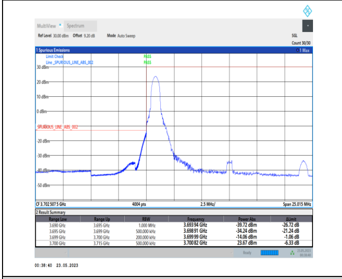
1-N78-3700-3800-PC1-30-15-L-4-CP-QPSK-Edge_1RB_Left-1@0-Ant0-1--PASS-see graph
