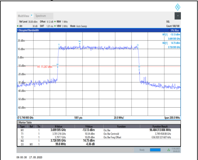
1-N78-3700-3800-PC1-30-100-L-4-DFT-64QAM-Out er_Full-270@0-Ant0-96.484-99.800-≤100-PASS
