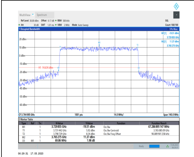
1-N78-3700-3800-PC1-30-70-H-8-CP-64QAM-Outer_Full-189@0-Ant0-67.287-69.860-≤70-PASS
