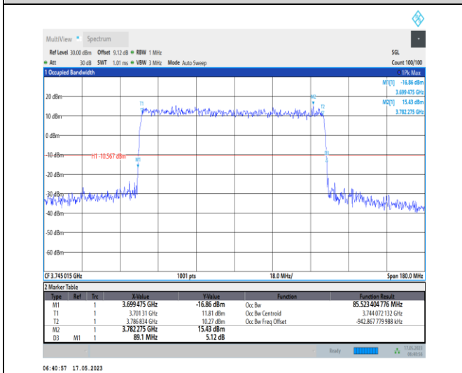
1-N78-3700-3800-PC1-30-90-L-4-DFT-64QAM-Out er_Full-240@0-Ant0-85.523-89.100-<=90-PASS
