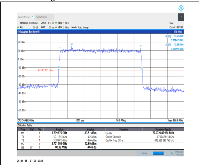
1-N78-3700-3800-PC1-30-80-M-5-DFT-256QAM-Outer_Full-216@0-Ant0-77.072-80.320-≤80-PASS
