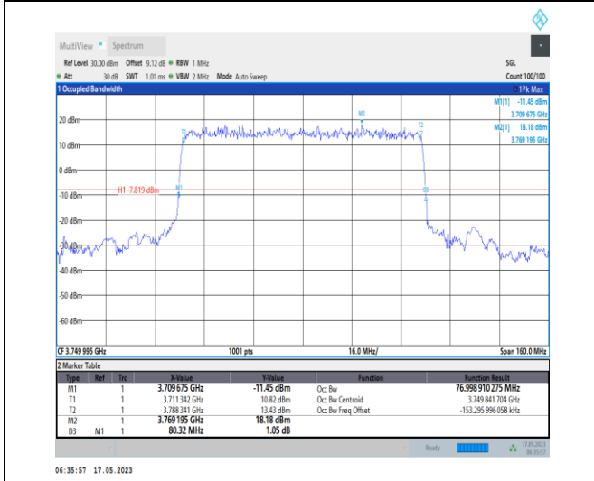
1-N78-3700-3800-PC1-30-80-M-2-DFT-PI2BPSK-Outer_Full-216@0-Ant0-76.999-80.320-≤80-PASS
