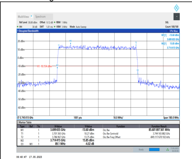
1-N78-3700-3800-PC1-30-90-L-3-DFT-16QAM-Out er_Full-240@0-Ant0-85.602-89.100-<=90-PASS
