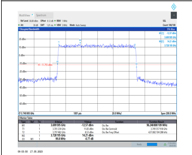
1-N78-3700-3800-PC1-30-100-M-4-DFT-64QAM-Out er_Full-270@0-Ant0-96.249-99.800-≤100-PASS
