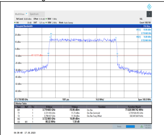
1-N78-3700-3800-PC1-30-80-H-4-DFT-64QAM-Outer_Full-216@0-Ant0-77.02-80.320-≤80-PASS
