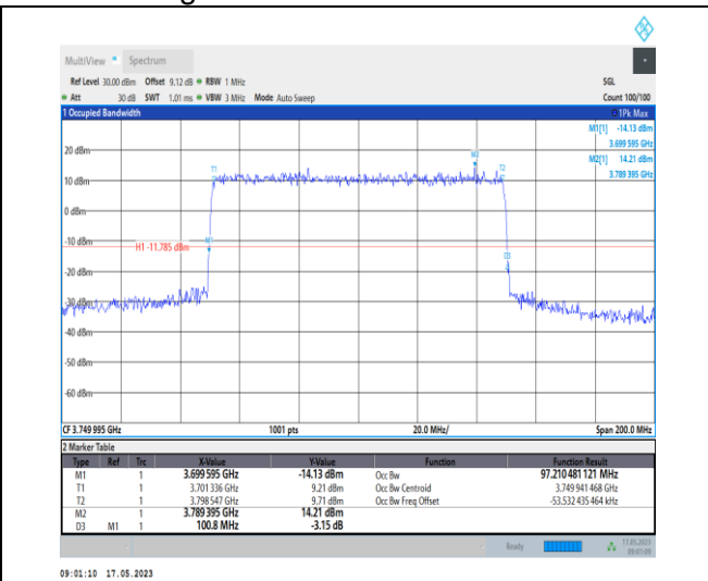
1-N78-3700-3800-PC1-30-100-L-8-CP-64QAM-Outer_Full-273@0-Ant0-97.21-100.800-≤100-PASS
