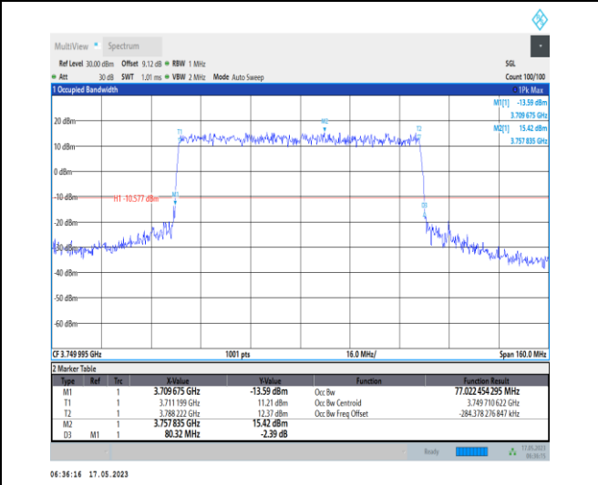
1-N78-3700-3800-PC1-30-80-M-3-DFT-16QAM-Outer_Full-216@0-Ant0-77.022-80.320-≤80-PASS
