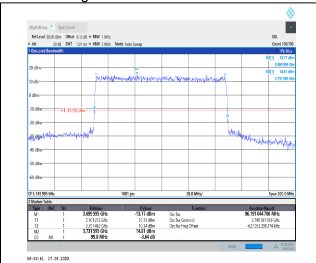
1-N78-3700-3800-PC1-30-100-M-3-DFT-16QAM-Out er_Full-270@0-Ant0-96.191-99.800-≤100-PASS
