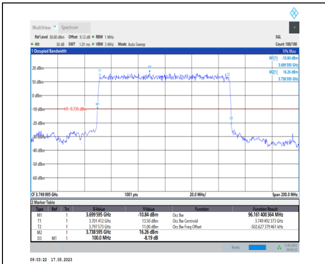
1-N78-3700-3800-PC1-30-100-M-2-DFT-PI2BPSK-Out uter_Full-270@0-Ant0-96.161-100.000-≤100-PASS
