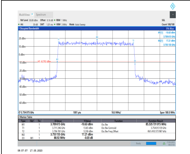
1-N78-3700-3800-PC1-30-90-H-2-DFT-PI2BPSK-Outer_Full-240@0-Ant0-85.536-88.920-≤90-PASS
