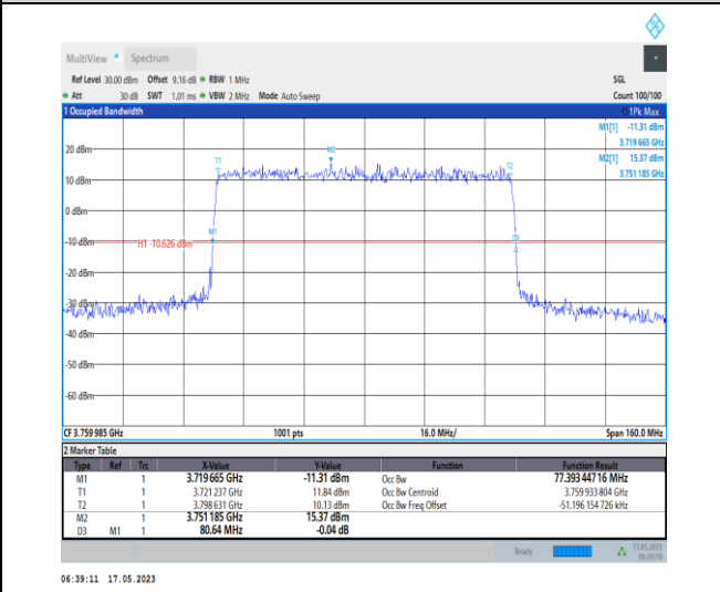
1-N78-3700-3800-PC1-30-80-H-6-CP-QPSK-Outer_Full-217@0-Ant0-77.393-80.640-≤80-PASS
