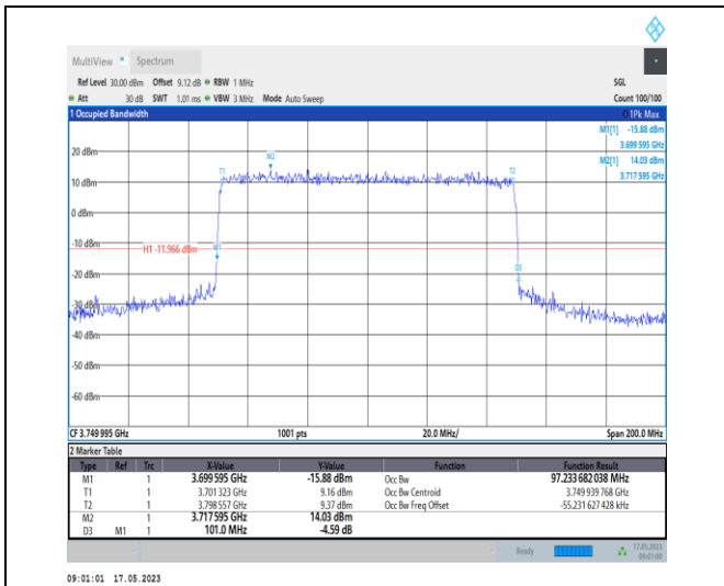
1-N78-3700-3800-PC1-30-100-L-7-CP-16QAM-Outer_Full-273@0-Ant0-97.234-101.000-≤100-PASS
