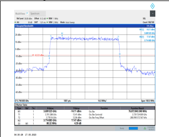
1-N78-3700-3800-PC1-30-80-L-2-DFT-PI2BPSK-Outer_Full-216@0-Ant0-76.873-80.320-≤80-PASS
