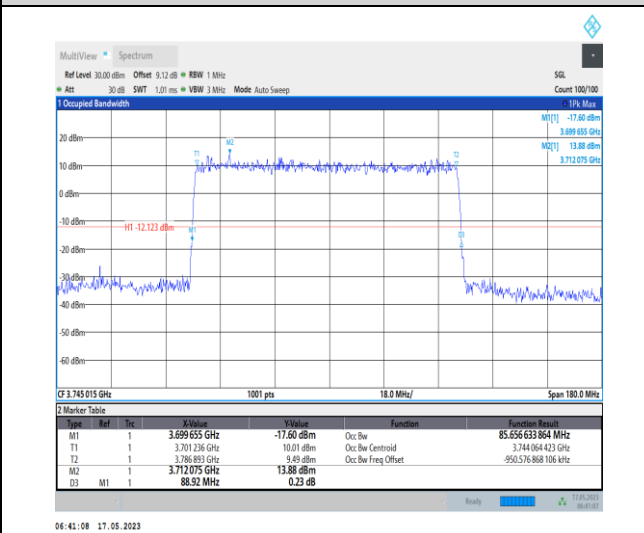
1-N78-3700-3800-PC1-30-90-L-5-DFT-256QAM-Out er_Full-240@0-Ant0-85.657-88.920-<=90-PASS
