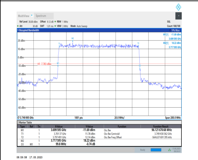
1-N78-3700-3800-PC1-30-100-L-2-DFT-PI2BPSK-Outer_Full-270@0-Ant0-96.122-99.800-≤100-PASS
