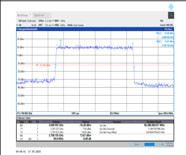
1-N78-3700-3800-PC1-30-100-M-5-DFT-256QAM-Out uter_Full-270@0-Ant0-96.288-99.800-≤100-PASS
