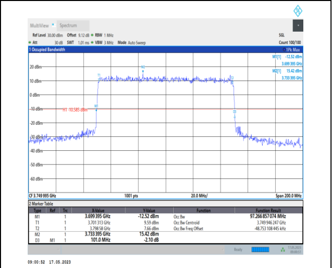
1-N78-3700-3800-PC1-30-100-L-6-CP-QPSK-Outer _Full-273@0-Ant0-97.267-101.000-≤100-PASS
