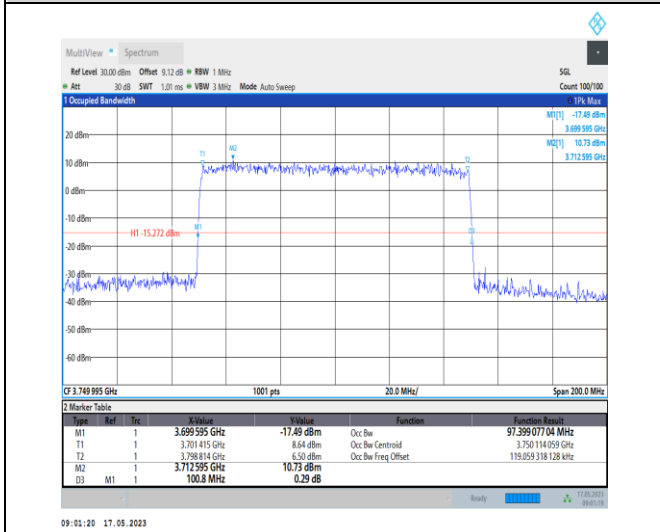
1-N78-3700-3800-PC1-30-100-L-9-CP-256QAM-Outer_Full-273@0-Ant0-97.399-100.800-≤100-PASS
