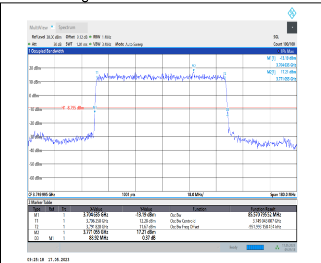
1-N78-3700-3800-PC1-30-90-M-2-DFT-PI2BPSK-Outer_Full-240@0-Ant0-85.571-88.920-≤90-PASS
