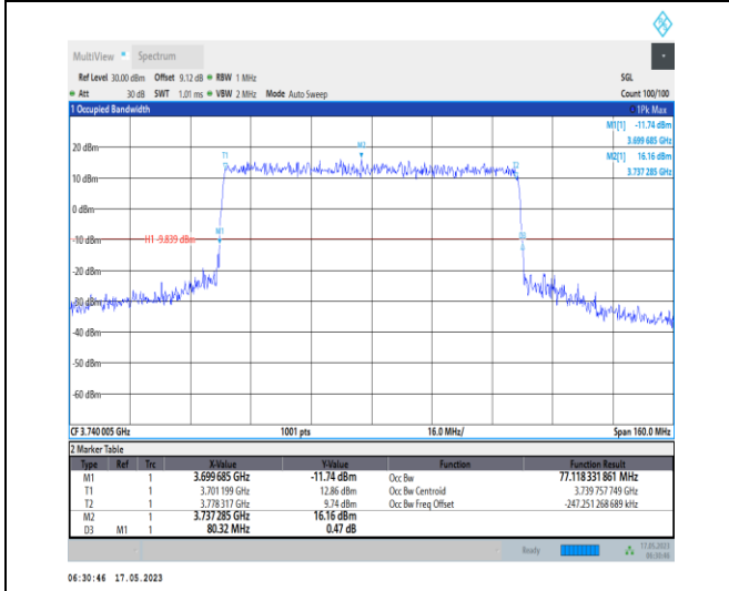
1-N78-3700-3800-PC1-30-80-L-3-DFT-16QAM-Outer_Full-216@0-Ant0-77.118-80.320-≤80-PASS
