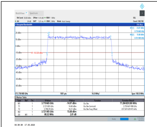
1-N78-3700-3800-PC1-30-80-H-3-DFT-16QAM-Outer_Full-216@0-Ant0-77.285-80.320-≤80-PASS
