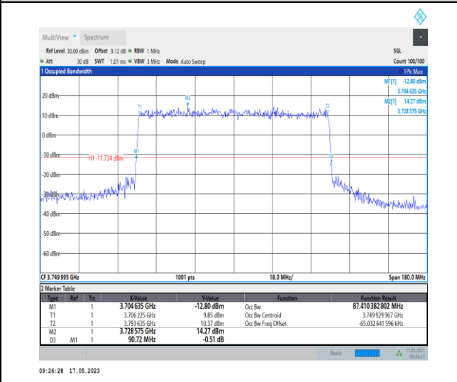
1-N78-3700-3800-PC1-30-90-M-8-CP-64QAM-Outer _Full-245@0-Ant0-87.41-90.720-<90-PASS
