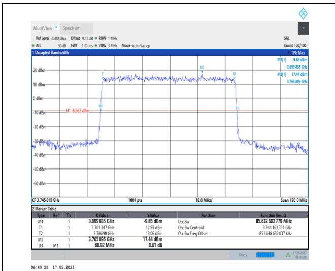
1-N78-3700-3800-PC1-30-90-L-2-DFT-PI2BPSK-Out er_Full-240@0-Ant0-85.633-88.920-<=90-PASS
