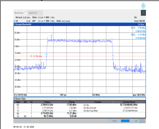
1-N78-3700-3800-PC1-30-90-H-9-CP-256QAM-Outer_Full-245@0-Ant0-87.716-90.720-≤90-PASS
