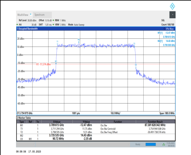
1-N78-3700-3800-PC1-30-90-H-7-CP-16QAM-Outer_Full-245@0-Ant0-87.302-90.720-≤90-PASS
