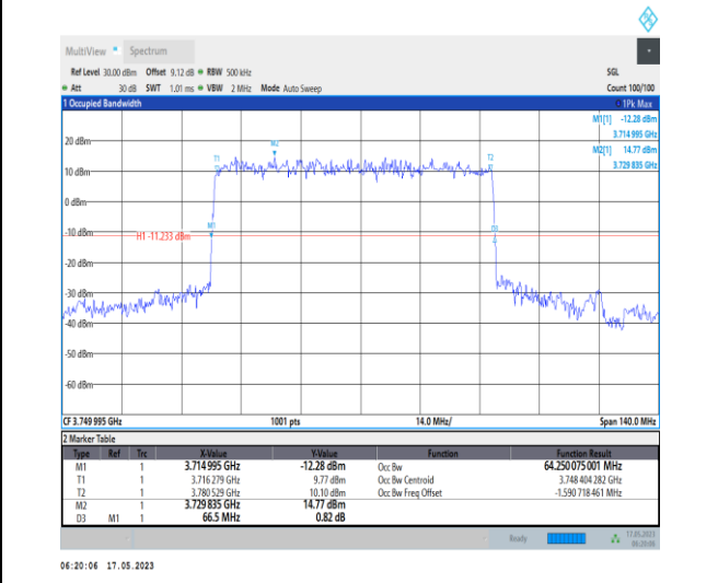
1-N78-3700-3800-PC1-30-70-M-2-DFT-PI2BPSK-Outer_Full-180@0-Ant0-64.25-66.500-≤70-PASS
