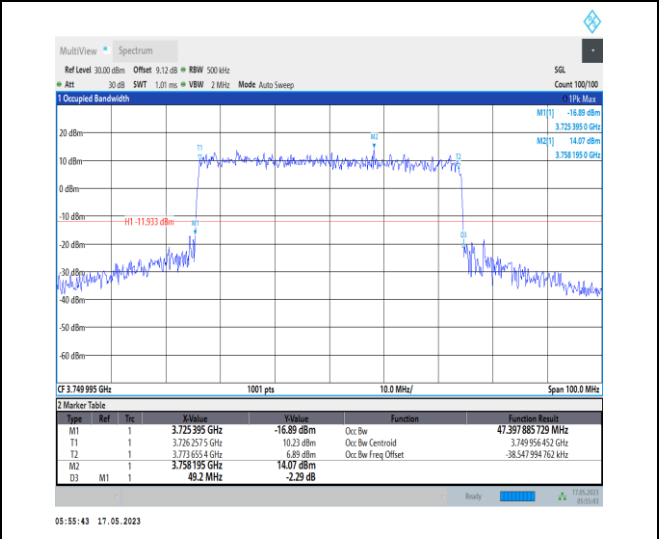
1-N78-3700-3800-PC1-30-50-M-8-CP-64QAM-Outer _Full-133@0-Ant0-47.398-49.200-≤50-PASS
