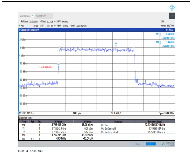
1-N78-3700-3800-PC1-30-50-M-9-CP-256QAM-Outer_Full-133@0-Ant0-47.435-49.300-≤50-PASS
