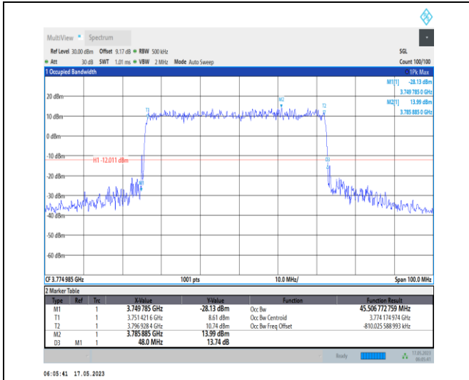
1-N78-3700-3800-PC1-30-50-H-4-DFT-64QAM-Outer_Full-128@0-Ant0-45.507-48.000-≤50-PASS
