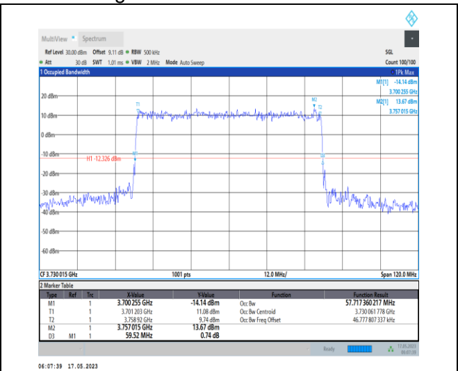
1-N78-3700-3800-PC1-30-60-L-4-DFT-64QAM-Outer_Full-162@0-Ant0-57.717-59.520-≤60-PASS
