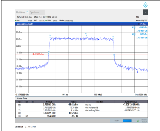
1-N78-3700-3800-PC1-30-50-M-7-CP-16QAM-Outer _Full-133@0-Ant0-47.503-49.500-≤50-PASS
