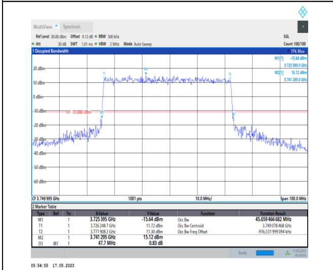
1-N78-3700-3800-PC1-30-50-M-3-DFT-16QAM-Outer_Full-128@0-Ant0-45.659-47.700-≤50-PASS
