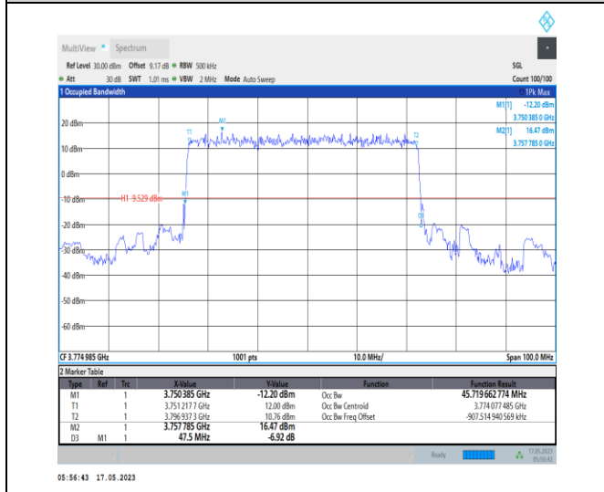
1-N78-3700-3800-PC1-30-50-H-2-DFT-PI2BPSK-Outer_Full-128@0-Ant0-45.72-47.500-≤50-PASS
