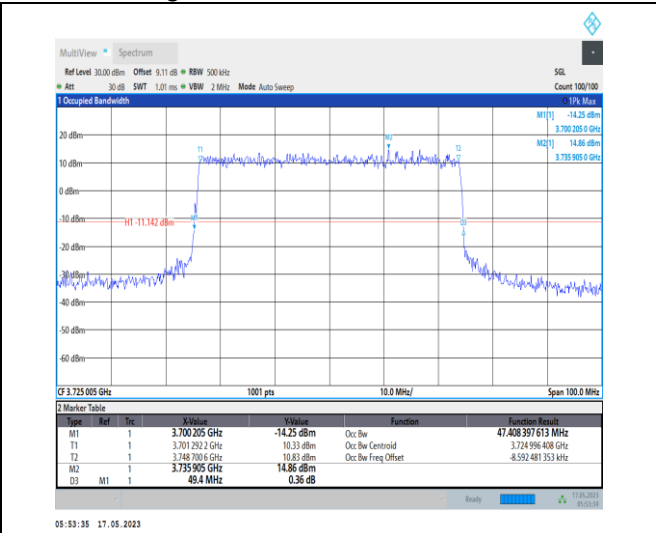
1-N78-3700-3800-PC1-30-50-L-7-CP-16QAM-Outer_Full-133@0-Ant0-47.408-49.400-≤50-PASS
