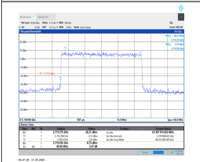
1-N78-3700-3800-PC1-30-70-M-9-CP-256QAM-Outer _Full-189@0-Ant0-67.302-69.440-≤70-PASS
