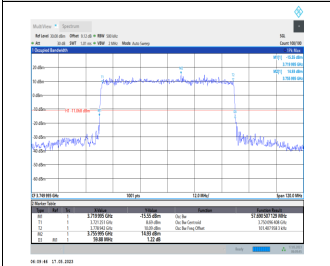
1-N78-3700-3800-PC1-30-60-M-4-DFT-64QAM-Outer_Full-162@0-Ant0-57.691-59.880-≤60-PASS
