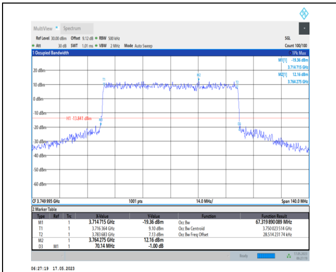
1-N78-3700-3800-PC1-30-70-M-7-CP-16QAM-Outer _Full-189@0-Ant0-67.32-70.140-≤70-PASS
