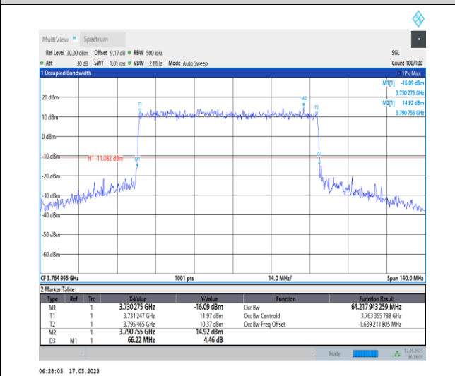
1-N78-3700-3800-PC1-30-70-H-1-DFT-QPSK-Outer _Full-180@0-Ant0-64.218-66.220-≤70-PASS
