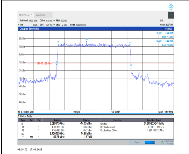
1-N78-3700-3800-PC1-30-70-L-2-DFT-PI2BPSK-Outer_Full-180@0-Ant0-64.306-66.780-≤70-PASS
