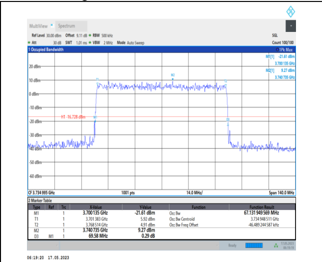
1-N78-3700-3800-PC1-30-70-L-9-CP-256QAM-Outer_Full-189@0-Ant0-67.132-69.580-≤70-PASS
