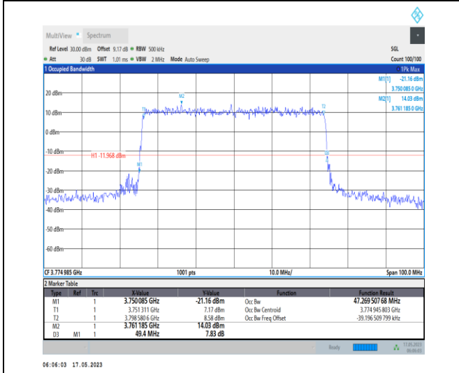
1-N78-3700-3800-PC1-30-50-H-6-CP-QPSK-Outer_Full-133@0-Ant0-47.27-49.400-≤50-PASS
