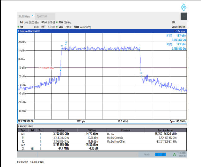
1-N78-3700-3800-PC1-30-50-H-3-DFT-16QAM-Outer_Full-128@0-Ant0-45.75-47.700-≤50-PASS
