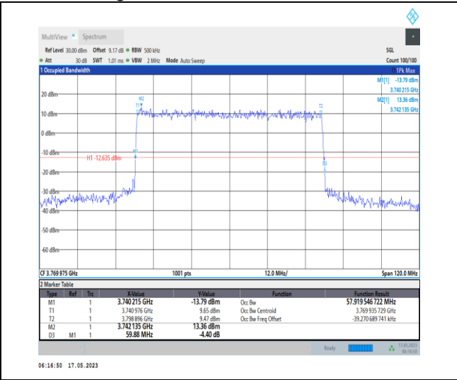
1-N78-3700-3800-PC1-30-60-H-6-CP-QPSK-Outer_Full-162@0-Ant0-57.92-59.880-≤60-PASS
