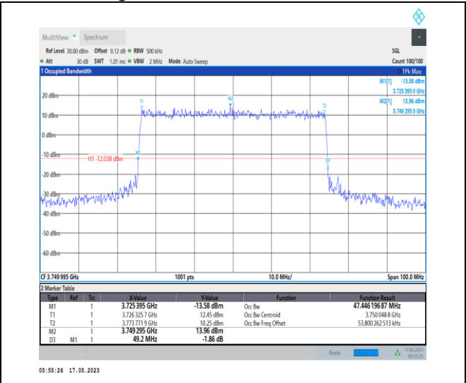
1-N78-3700-3800-PC1-30-50-M-6-CP-QPSK-Outer _Full-133@0-Ant0-47.446-49.200-≤50-PASS
