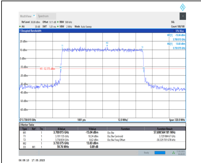
1-N78-3700-3800-PC1-30-60-L-7-CP-16QAM-Outer_Full-162@0-Ant0-57.699-59.760-≤60-PASS
