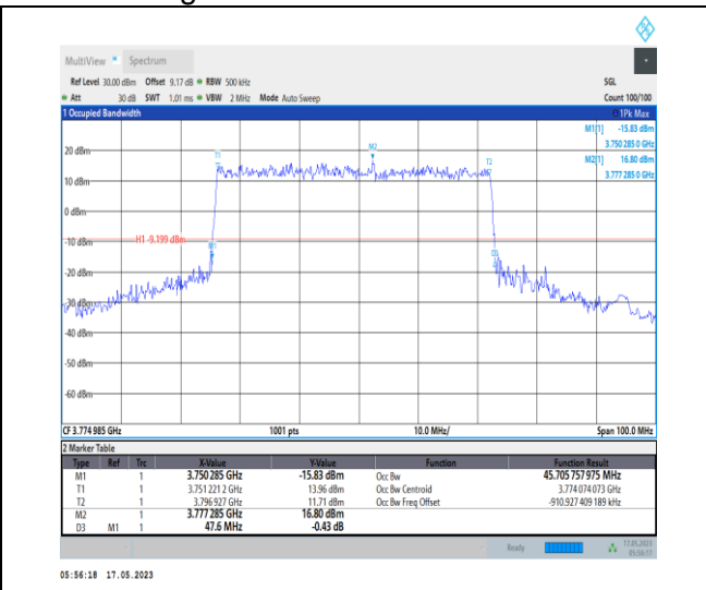
1-N78-3700-3800-PC1-30-50-H-1-DFT-QPSK-Outer_Full-128@0-Ant0-45.706-47.600-≤50-PASS
