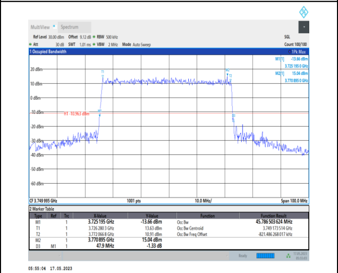
1-N78-3700-3800-PC1-30-50-M-4-DFT-64QAM-Outer_Full-128@0-Ant0-45.787-47.900-≤50-PASS
