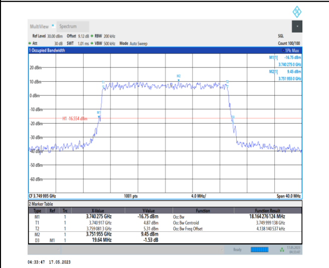
1-N78-3700-3800-PC1-30-20-M-9-CP-256QAM-Outer_Full-51 @ 0-Ant0-18.164-19.640-≤20-PASS
