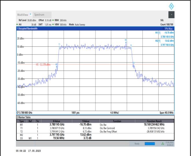
1-N78-3700-3800-PC1-30-20-H-8-CP-64QAM-Outer _Full-51@0-Ant0-18.169-19.560-≤20-PASS
