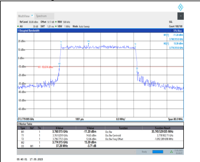
1-N78-3700-3800-PC1-30-40-H-4-DFT-64QAM-Outer_Full-100@0-Ant0-35.746-37.280-≤40-PASS
