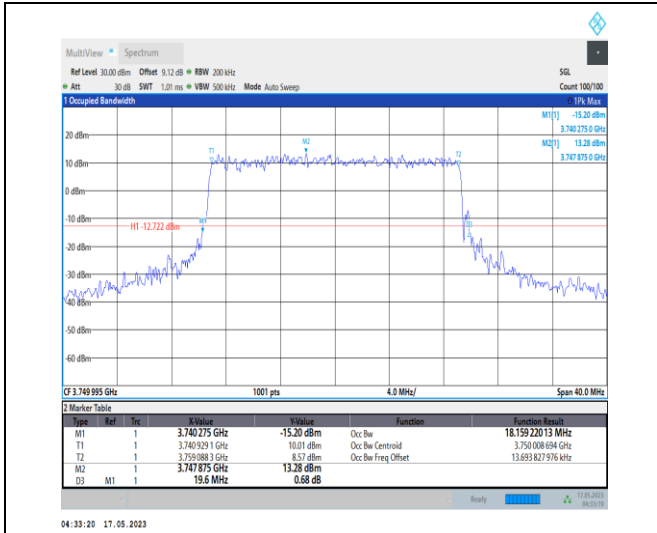
1-N78-3700-3800-PC1-30-20-M-6-CP-QPSK-Outer_Full-51 @ 0-Ant0-18.159-19.600-≤20-PASS
