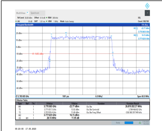
1-N78-3700-3800-PC1-30-30-H-2-DFT-PI2BPSK-Outer_Full-75@0-Ant0-26.819-28.140-≤30-PASS
