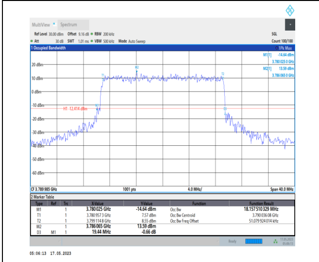
1-N78-3700-3800-PC1-30-20-H-7-CP-16QAM-Outer _Full-51@0-Ant0-18.158-19.440-≤20-PASS
