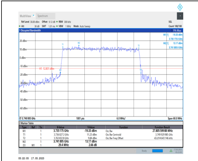
1-N78-3700-3800-PC1-30-30-M-7-CP-16QAM-Outer _Full-78@0-Ant0-27.806-29.400-≤30-PASS
