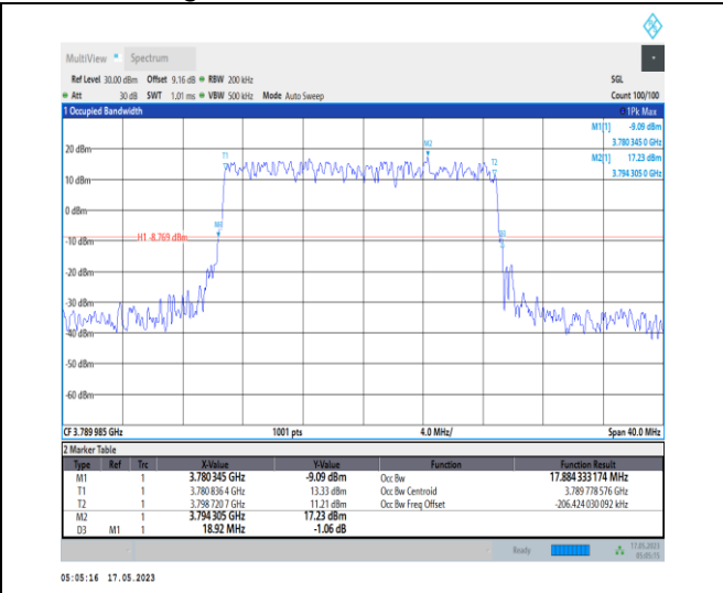
1-N78-3700-3800-PC1-30-20-H-2-DFT-PI2BPSK-Outer_Full-50@0-Ant0-17.884-18.920-≤20-PASS
