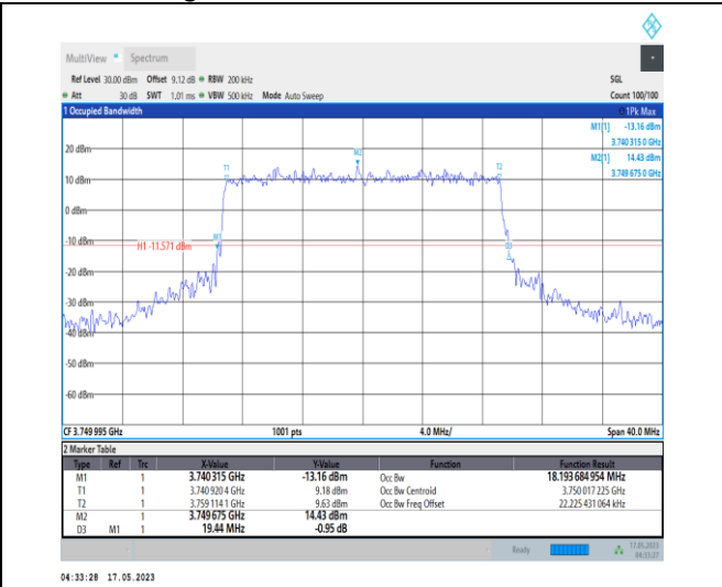
1-N78-3700-3800-PC1-30-20-M-7-CP-16QAM-Outer_Full-51 @ 0-Ant0-18.194-19.440-≤20-PASS
