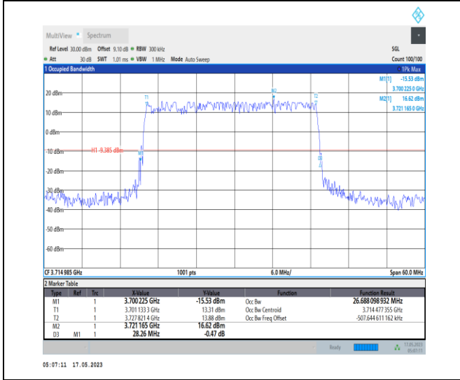
1-N78-3700-3800-PC1-30-30-L-2-DFT-PI2BPSK-Outer_Full-75@0-Ant0-26.688-28.260-≤30-PASS
