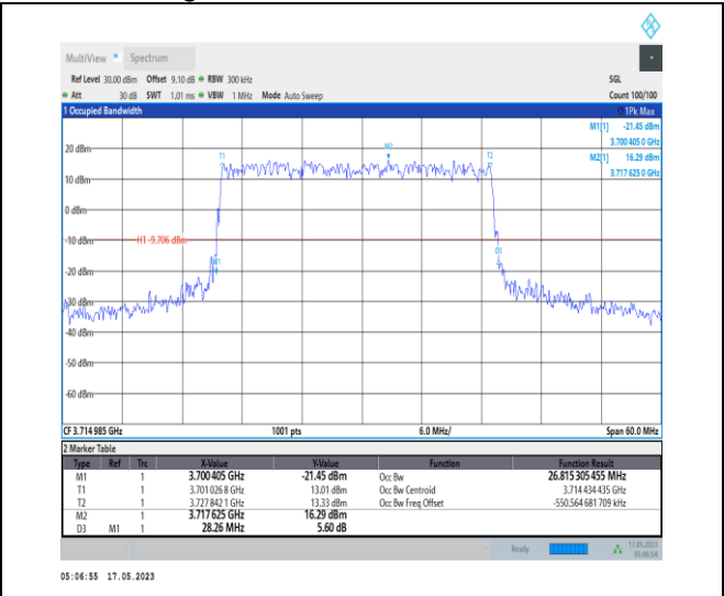
1-N78-3700-3800-PC1-30-30-L-1-DFT-QPSK-Outer_Full-75@0-Ant0-26.815-28.260-≤30-PASS
