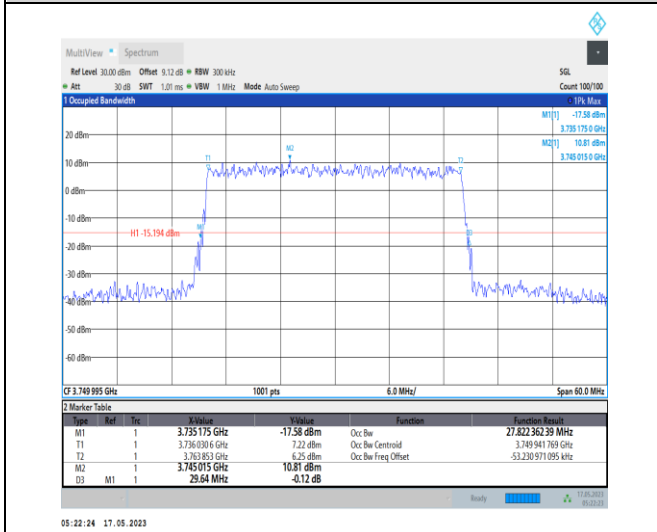
1-N78-3700-3800-PC1-30-30-M-9-CP-256QAM-Outer _Full-78@0-Ant0-27.822-29.640-≤30-PASS
