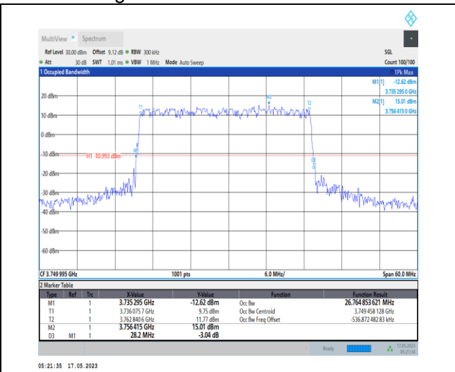
1-N78-3700-3800-PC1-30-30-M-4-DFT-64QAM-Outer_Full-75@0-Ant0-26.765-28.200-≤30-PASS
