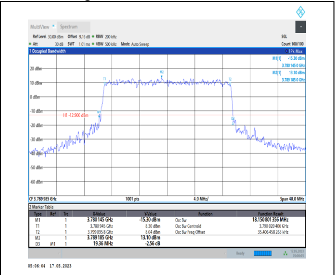
1-N78-3700-3800-PC1-30-20-H-6-CP-QPSK-Outer Full-51@0-Ant0-18.151-19.360-≤20-PASS
