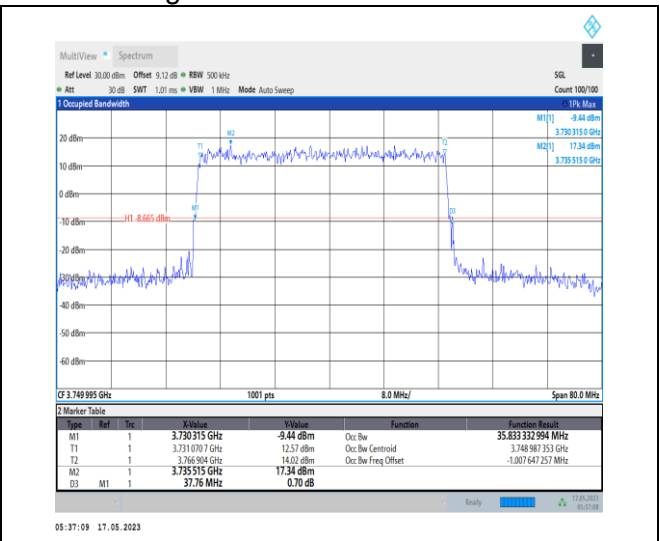
1-N78-3700-3800-PC1-30-40-M-1-DFT-QPSK-Outer_Full-100@0-Ant0-35.833-37.760-≤40-PASS
