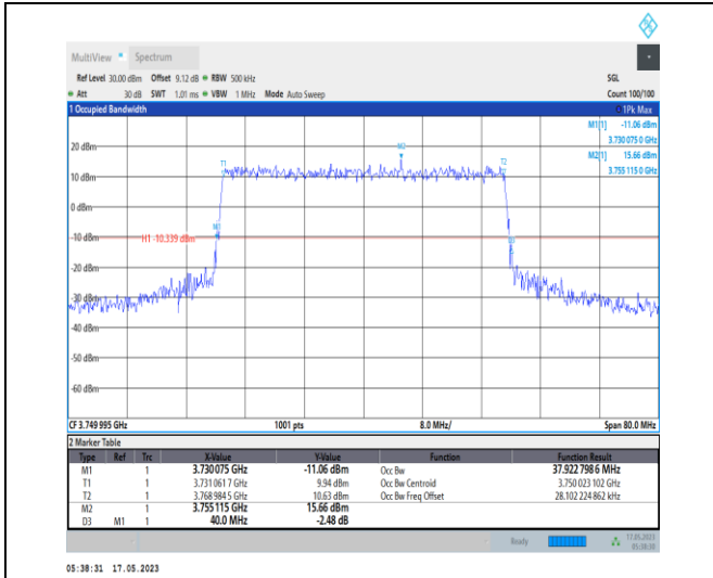
1-N78-3700-3800-PC1-30-40-M-8-CP-64QAM-Outer_Full-106@0-Ant0-37.923-40.000-≤40-PASS
