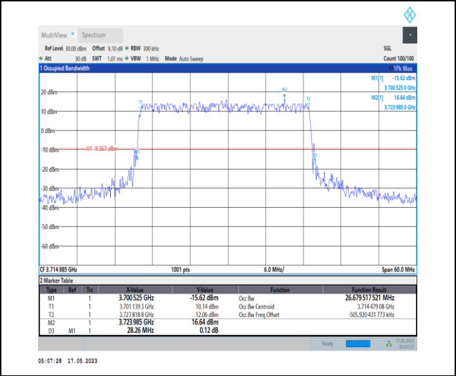
1-N78-3700-3800-PC1-30-30-L-3-DFT-16QAM-Outer_Full-75@0-Ant0-26.68-28.260-≤30-PASS
