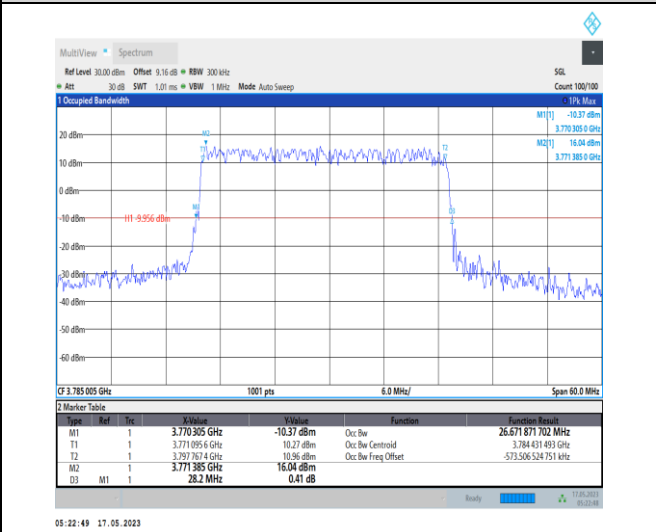
1-N78-3700-3800-PC1-30-30-H-1-DFT-QPSK-Outer _Full-75@0-Ant0-26.672-28.200-≤30-PASS
