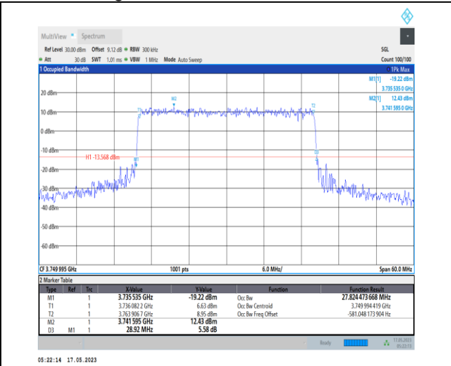
1-N78-3700-3800-PC1-30-30-M-8-CP-64QAM-Outer _Full-78@0-Ant0-27.824-28.920-≤30-PASS
