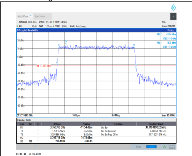
1-N78-3700-3800-PC1-30-40-H-8-CP-64QAM-Outer_Full-106@0-Ant0-37.719-39.600-≤40-PASS
