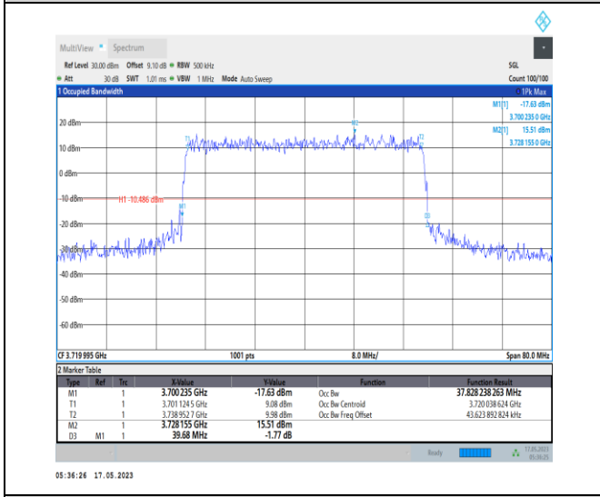
1-N78-3700-3800-PC1-30-40-L-7-CP-16QAM-Outer_Full-106@0-Ant0-37.828-39.680-≤40-PASS
