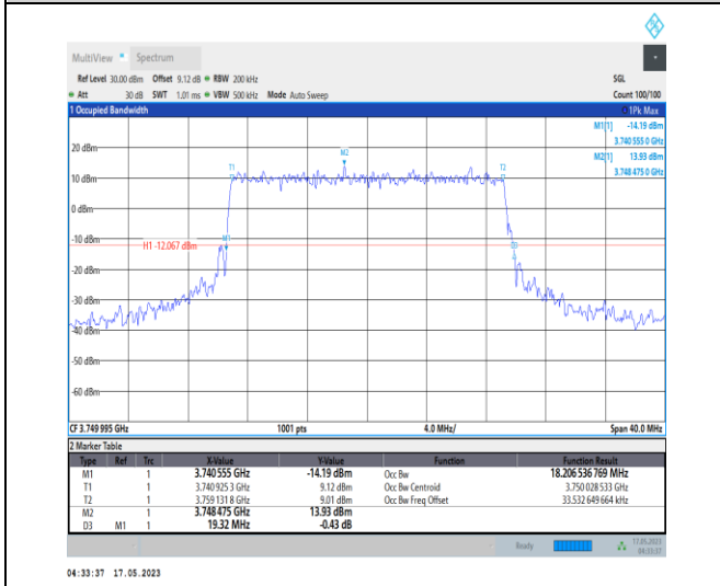
1-N78-3700-3800-PC1-30-20-M-8-CP-64QAM-Outer_Full-51 @ 0-Ant0-18.207-19.320-≤20-PASS
