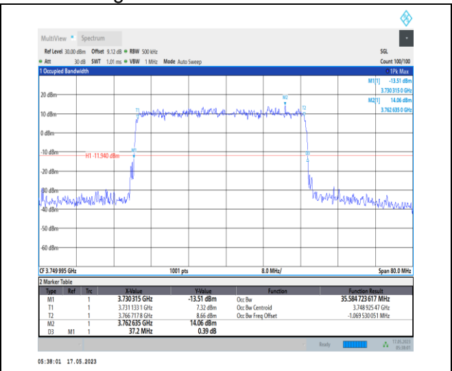
1-N78-3700-3800-PC1-30-40-M-5-DFT-256QAM-Outer_Full-100@0-Ant0-35.585-37.200-≤40-PASS
