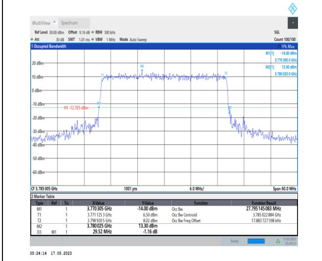
1-N78-3700-3800-PC1-30-30-H-8-CP-64QAM-Outer_Full-78@0-Ant0-27.795-29.520-≤30-PASS
