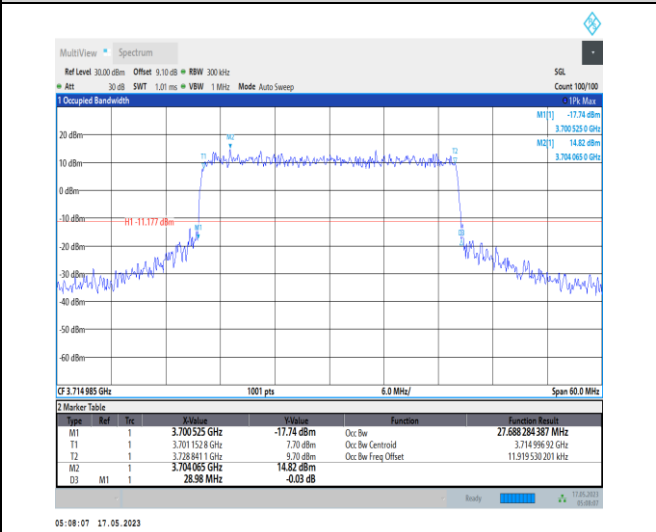
1-N78-3700-3800-PC1-30-30-L-7-CP-16QAM-Outer_Full-78@0-Ant0-27.688-28.980-≤30-PASS
