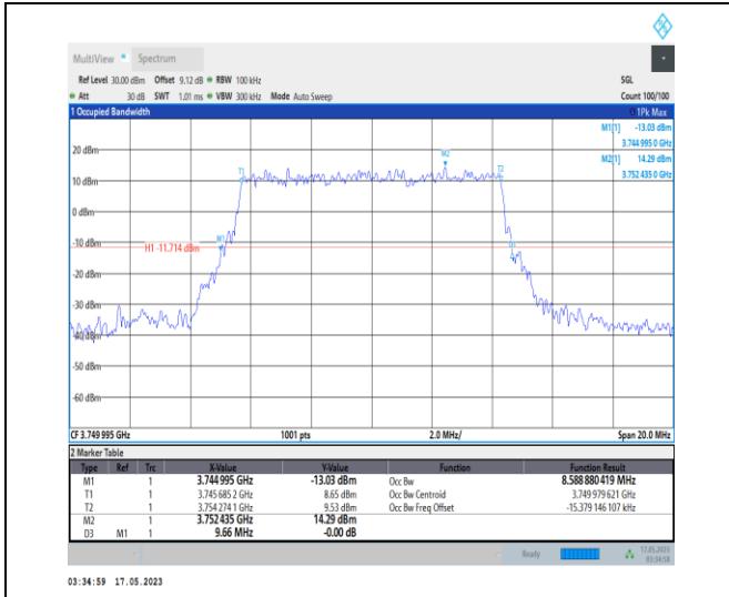
1-N78-3700-3800-PC1-30-10-M-4-DFT-64QAM-Outer_Full-24@0-Ant0-8.589-9.660-≤10-PASS
