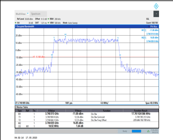
1-N78-3700-3800-PC1-30-20-M-1-DFT-QPSK-Outer_Full-50@0-Ant0-17.762-18.920-≤20-PASS
