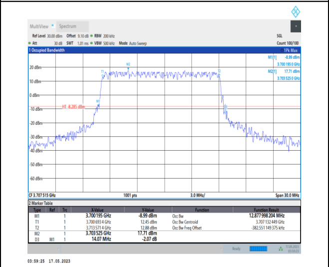
1-N78-3700-3800-PC1-30-15-L-1-DFT-QPSK-Outer Full-36@0-Ant0-12.878-14.070-≤15-PASS
