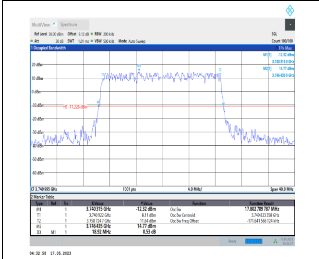
1-N78-3700-3800-PC1-30-20-M-4-DFT-64QAM-Outer_Full-50@0-Ant0-17.803-18.920-≤20-PASS
