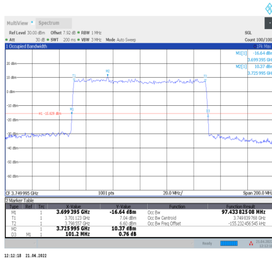
1-N78-3700-3800--30-100-M-9-CP-256QAM-Outer_Full -273@0-Ant0-97.434-101.200-≤100-PASS
