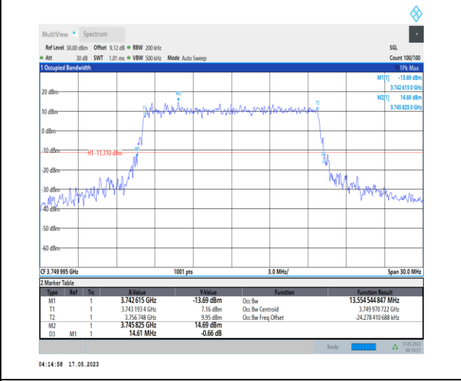
1-N78-3700-3800-PC1-30-15-M-8-CP-64QAM-Outer _Full-38@0-Ant0-13.555-14.610-≤15-PASS
