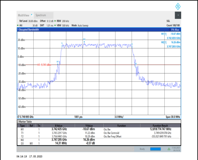
1-N78-3700-3800-PC1-30-15-M-4-DFT-64QAM-Outer_Full-36@0-Ant0-12.819-14.310-≤15-PASS
