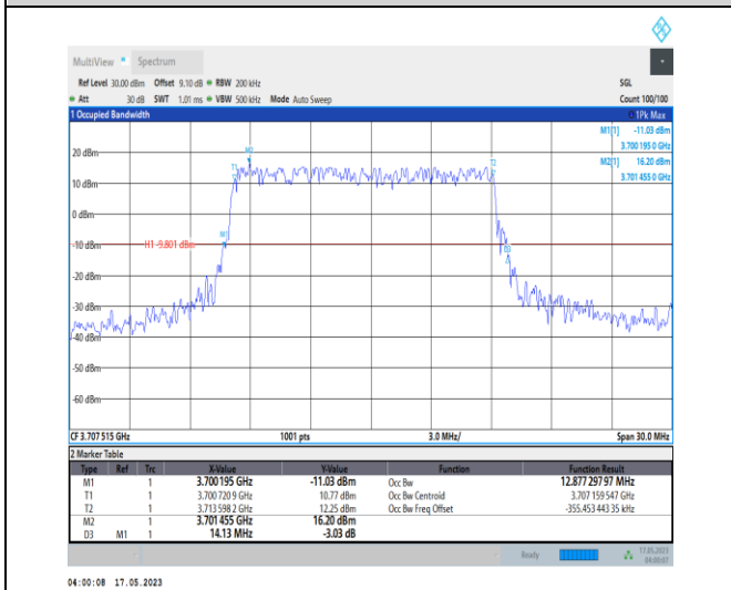
1-N78-3700-3800-PC1-30-15-L-4-DFT-64QAM-Out er_Full-36@0-Ant0-12.877-14.130-≤15-PASS
