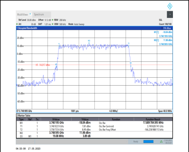
1-N78-3700-3800-PC1-30-20-M-5-DFT-256QAM-Outer_Full-50@0-Ant0-17.81-19.080-≤20-PASS
