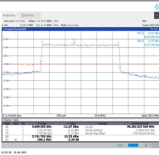
1-N78-3700-3800--30-100-H-1-DFT-QPSK-Outer_Full-270@0-Ant0-96.361-100.200-≤100-PASS
