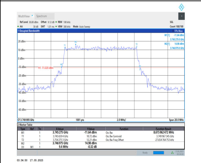
1-N78-3700-3800-PC1-30-10-M-3-DFT-16QAM-Outer_Full-24@0-Ant0-8.616-9.400-≤10-PASS
