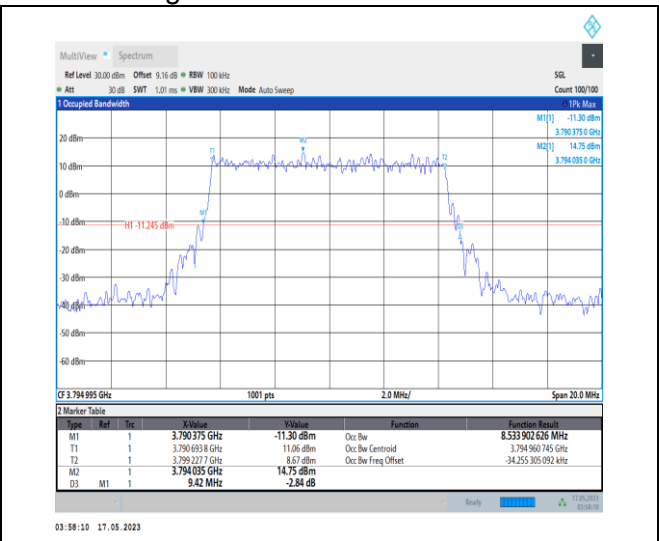
1-N78-3700-3800-PC1-30-10-H-4-DFT-64QAM-Outer_Full-24@0-Ant0-8.534-9.420-≤10-PASS
