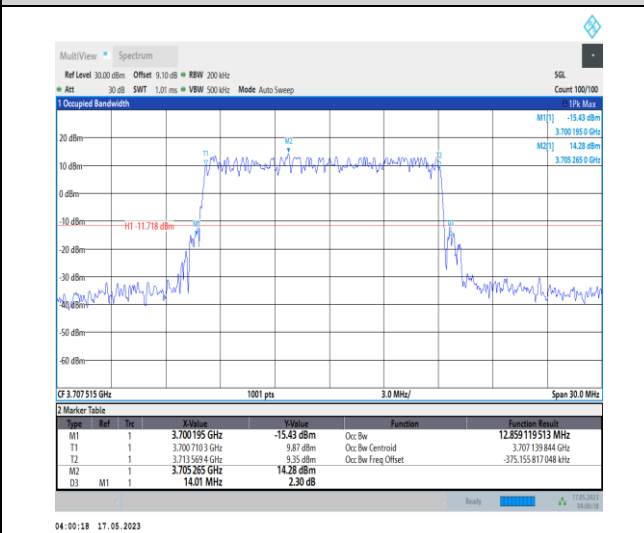
1-N78-3700-3800-PC1-30-15-L-5-DFT-256QAM-Out er_Full-36@0-Ant0-12.859-14.010-≤15-PASS
