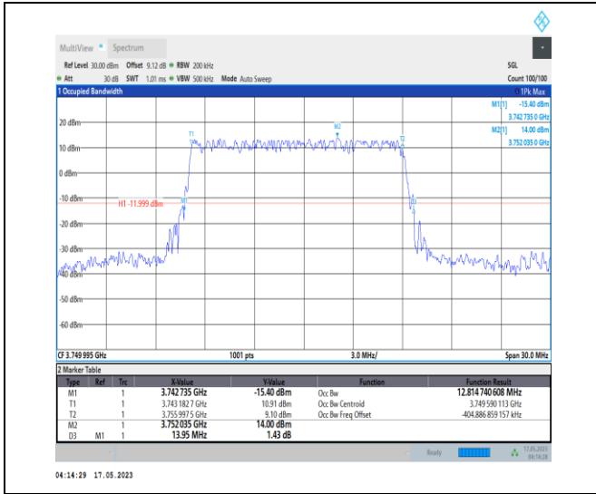
1-N78-3700-3800-PC1-30-15-M-5-DFT-256QAM-Out _Full-36@0-Ant0-12.815-13.950-≤15-PASS
