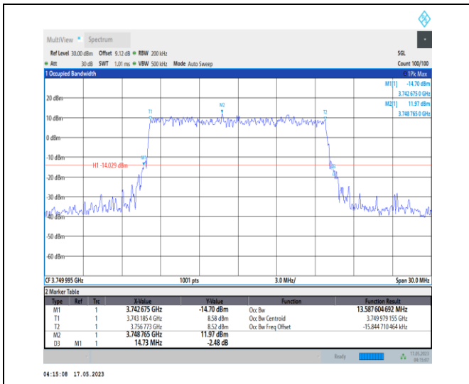
1-N78-3700-3800-PC1-30-15-M-9-CP-256QAM-Outer_Full-38@0-Ant0-13.588-14.730-≤15-PASS
