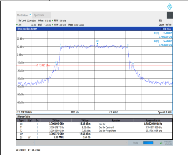
1-N78-3700-3800-PC1-30-10-L-6-CP-QPSK-Outer Full-24@0-Ant0-8.586-9.880-≤10-PASS
