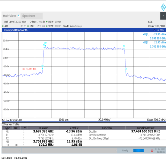
1-N78-3700-3800--30-100-M-6-CP-QPSK-Outer_Full -273@0-Ant0-97.485-101.200-≤100-PASS
