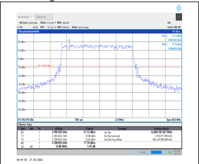
1-N78-3700-3800-PC1-30-15-H-1-DFT-QPSK-Outer_Full-36@0-Ant0-12.843-13.860-≤15-PASS
