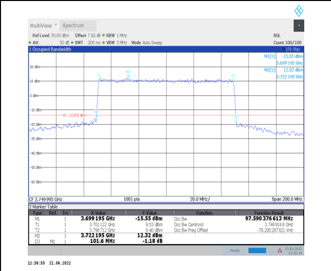
1-N78-3700-3800--30-100-H-8-CP-64QAM-Outer_Full-273@0-Ant0-97.59-101.600-≤100-PASS
