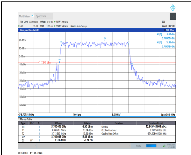
1-N78-3700-3800-PC1-30-15-L-2-DFT-PI2BPSK-Out er_Full-36@0-Ant0-12.845-13.860-≤15-PASS
