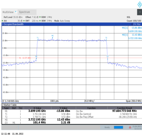
1-N78-3700-3800--30-100-M-8-CP-64QAM-Outer_Full -273@0-Ant0-97.605-101.400-≤100-PASS
