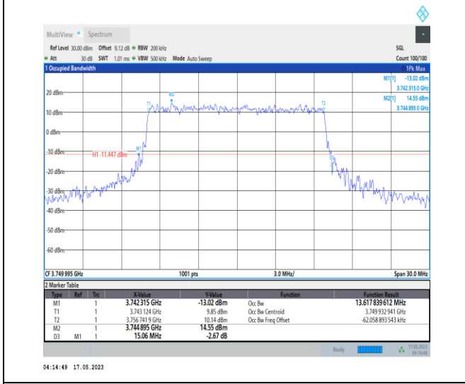
1-N78-3700-3800-PC1-30-15-M-7-CP-16QAM-Outer _Full-38@0-Ant0-13.618-15.060-≤15-PASS
