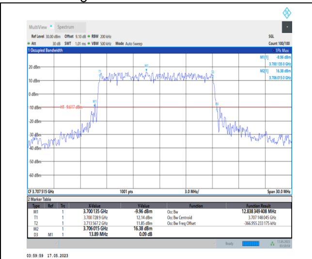
1-N78-3700-3800-PC1-30-15-L-3-DFT-16QAM-Out er_Full-36@0-Ant0-12.838-13.890-≤15-PASS
