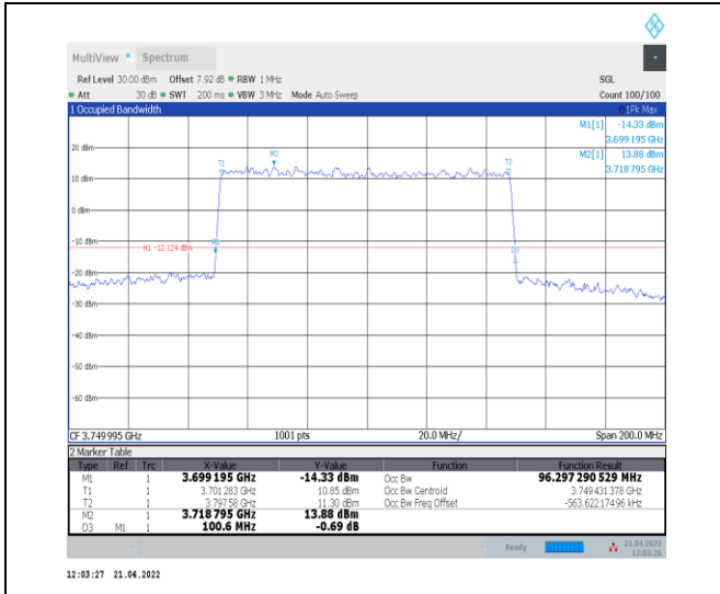
1-N78-3700-3800--30-100-L-3-DFT-16QAM-Outer_F ull-270@0-Ant0-96.297-100.600-≤100-PASS
