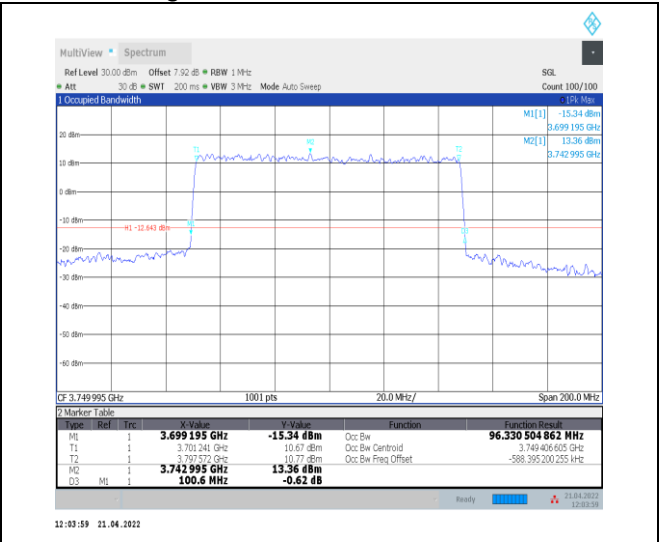
1-N78-3700-3800--30-100-L-4-DFT-64QAM-Outer_F ull-270@0-Ant0-96.331-100.600-≤100-PASS
