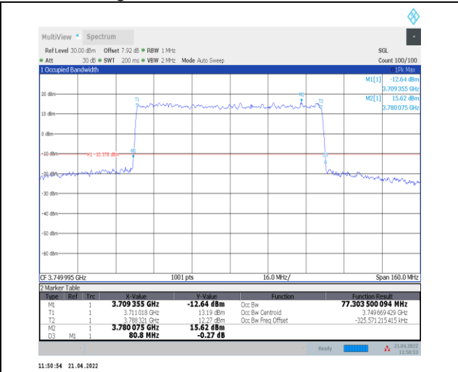
1-N78-3700-3800--30-80-M-1-DFT-QPSK-Outer_Full-216@0-Ant0-77.304-80.800≤80-PASS
