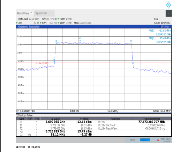
1-N78-3700-3800--30-80-L-8-CP-64QAM-Outer_Full-217@0-Ant0-77.473-81.120-≤80-PASS
