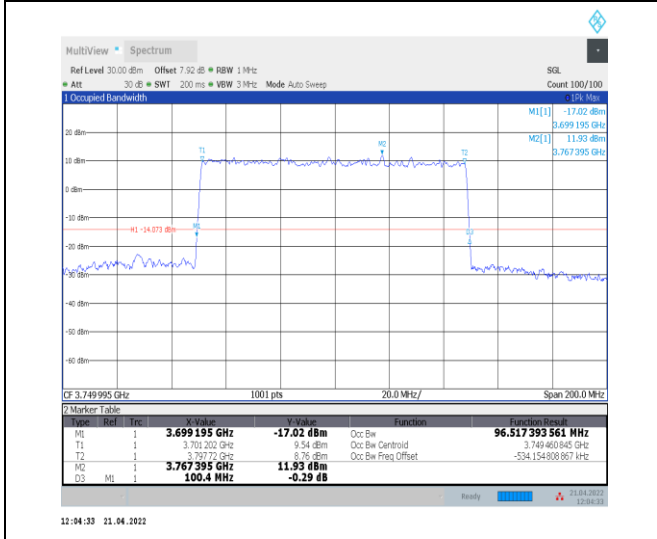
1-N78-3700-3800--30-100-L-5-DFT-256QAM-Outer_F ull-270@0-Ant0-96.517-100.400-≤100-PASS
