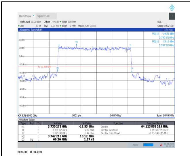
1-N78-3700-3800--30-70-H-2-DFT-PI2BPSK-Outer_Fu Full-180@0-Ant0-64.124-66.360-≤70-PASS
