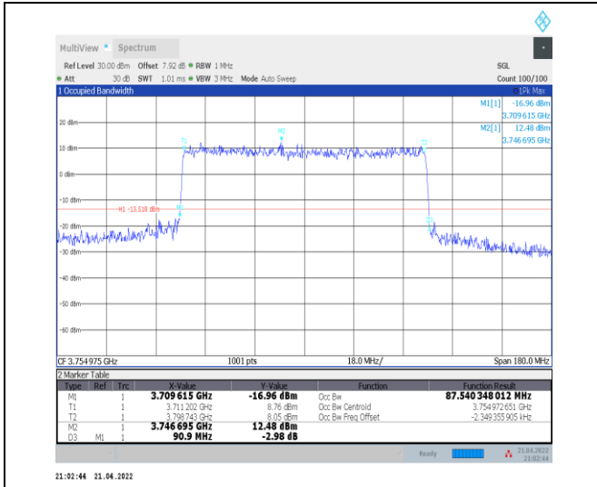
1-N78-3700-3800--30-90-H-8-CP-64QAM-Outer_Full -245@0-Ant0-87.54-90.900-<=90-PASS
