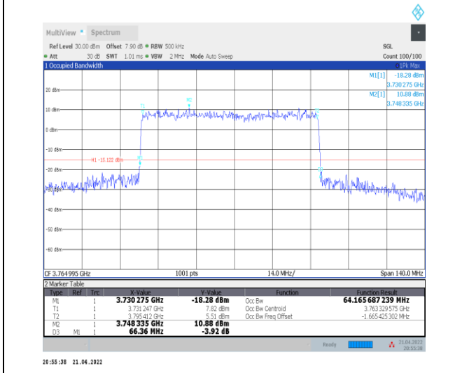
1-N78-3700-3800--30-70-H-4-DFT-64QAM-Outer_Fu II-180@0-Ant0-64.166-66.360-≤70-PASS
