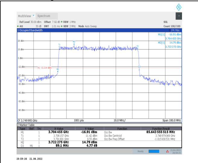
1-N78-3700-3800--30-90-M-2-DFT-PI2BPSK-Outer_Full -240@0-Ant0-85.644-89.100-≤90-PASS
