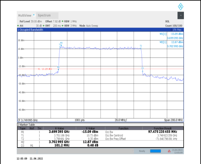
1-N78-3700-3800--30-100-L-6-CP-QPSK-Outer_F ull-273@0-Ant0-97.475-101.200-≤100-PASS
