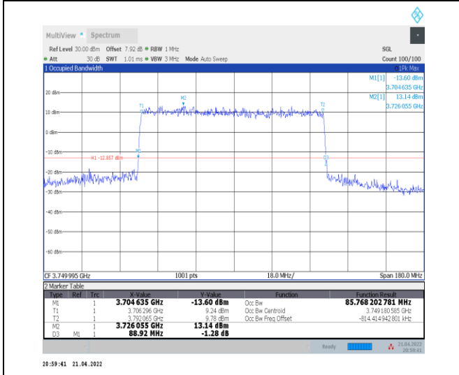
1-N78-3700-3800--30-90-M-3-DFT-16QAM-Outer_Full -240@0-Ant0-85.768-88.920-≤90-PASS
