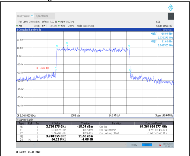
1-N78-3700-3800--30-70-H-3-DFT-16QAM-Outer_Fu II-180@0-Ant0-64.365-66.220-≤70-PASS
