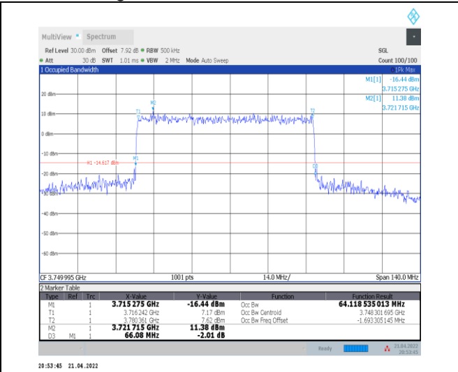
1-N78-3700-3800--30-70-M-4-DFT-64QAM-Outer_Full-180@0-Ant0-64.119-66.080-≤70-PASS
