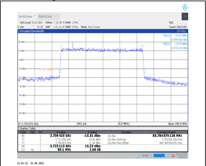
1-N78-3700-3800--30-90-H-1-DFT-QPSK-Outer_Full-240@0-Ant0-85.785-89.100-≤90-PASS
