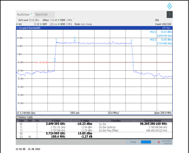
1-N78-3700-3800--30-100-L-2-DFT-PI2BPSK-Outer_Full Full-270@0-Ant0-96.395-100.400-<=100-PASS
