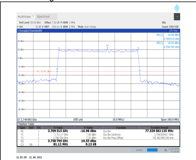
1-N78-3700-3800--30-80-M-9-CP-256QAM-Outer_Full-217@0-Ant0-77.54-81.120-<math>\leq</math>80-PASS
