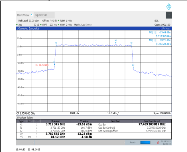
1-N78-3700-3800--30-80-H-8-CP-64QAM-Outer_Full -217@0-Ant0-77.489-81.120-≤80-PASS
