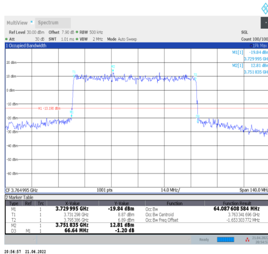
1-N78-3700-3800--30-70-H-1-DFT-QPSK-Outer_Full -180@0-Ant0-64.088-66.640-≤70-PASS
