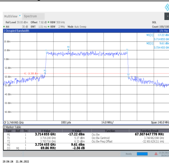
1-N78-3700-3800--30-70-M-8-CP-64QAM-Outer_Ful I-189@0-Ant0-67.508-69.860-≤70-PASS
