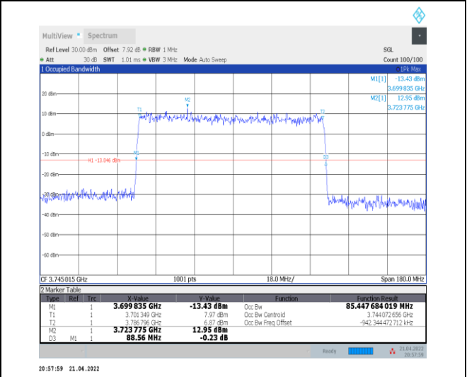
1-N78-3700-3800--30-90-L-5-DFT-256QAM-Outer_F ull-240@0-Ant0-85.448-88.560-<math>\leq 90</math>-PASS
