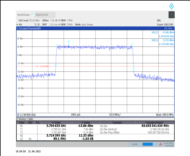
1-N78-3700-3800--30-90-M-4-DFT-64QAM-Outer_Full -240@0-Ant0-85.656-89.100-≤90-PASS
