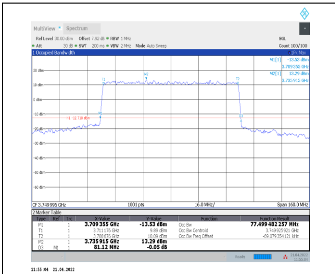
1-N78-3700-3800--30-80-M-8-CP-64QAM-Outer_Full -217@0-Ant0-77.499-81.120-<math>\leq</math>80-PASS
