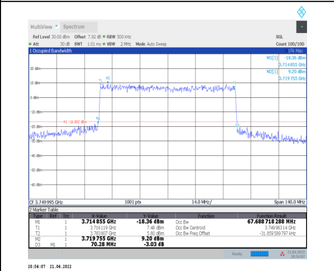
1-N78-3700-3800--30-70-M-6-CP-QPSK-Outer_Full-189@0-Ant0-67.689-70.280-≤70-PASS
