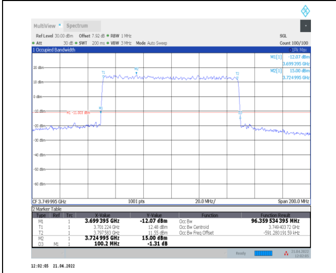
1-N78-3700-3800--30-100-L-1-DFT-QPSK-Outer_Full I-270@0-Ant0-96.36-100.200-<=100-PASS
