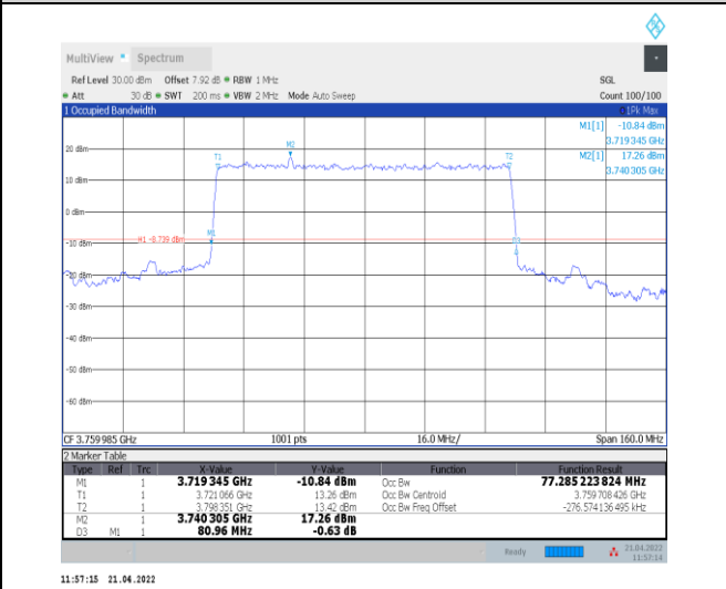
1-N78-3700-3800--30-80-H-2-DFT-PI2BPSK-Outer_Full-216@0-Ant0-77.285-80.960-<math>\leq</math>80-PASS
