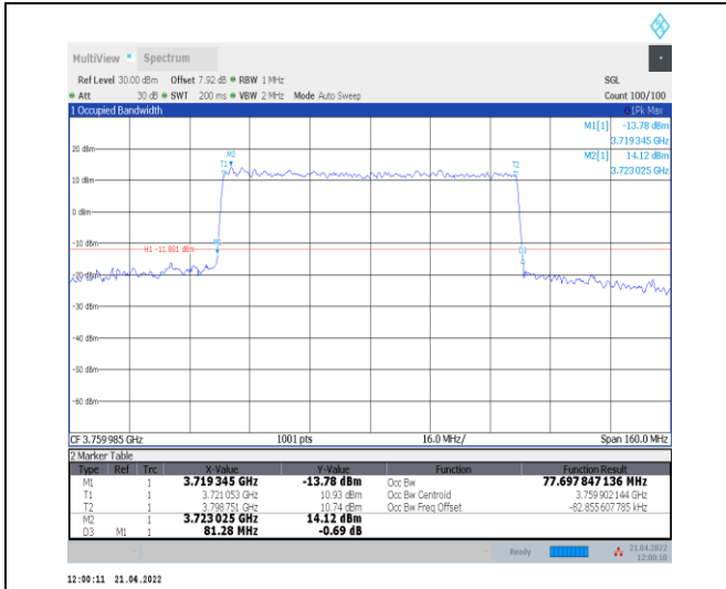
1-N78-3700-3800--30-80-H-7-CP-16QAM-Outer_Full -217@0-Ant0-77.698-81.280-≤80-PASS
