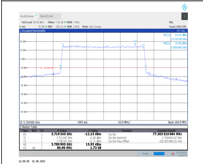
1-N78-3700-3800--30-80-H-1-DFT-QPSK-Outer_Full -216@0-Ant0-77.304-80.960-<math>\leq</math>80-PASS
