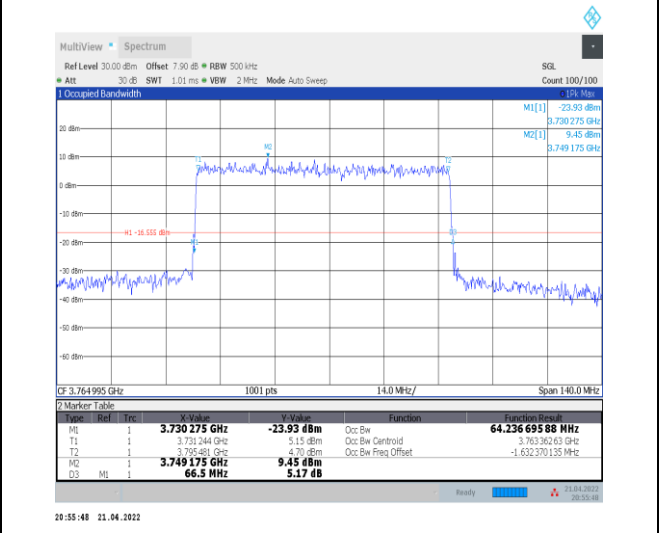
1-N78-3700-3800--30-70-H-5-DFT-256QAM-Outer_Fu Full-180@0-Ant0-64.237-66.500-≤70-PASS
