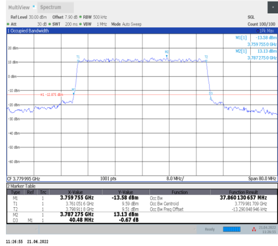
1-N78-3700-3800--30-40-H-8-CP-64QAM-Outer_Full -106@0-Ant0-37.86-40.480-≤40-PASS
