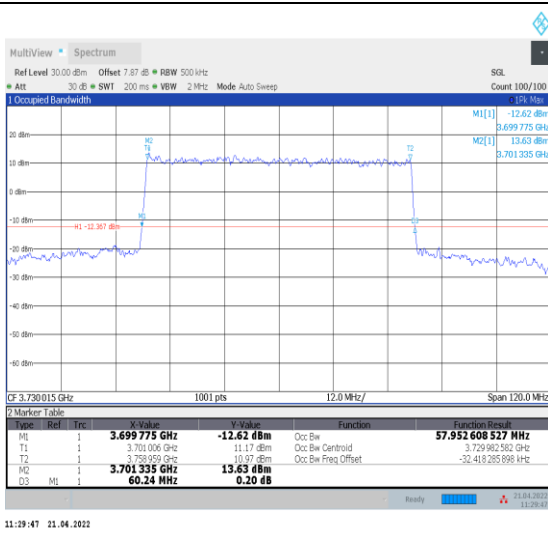
1-N78-3700-3800--30-60-L-3-DFT-16QAM-Outer_Ful I-162@0-Ant0-57.953-60.240-≤60-PASS
