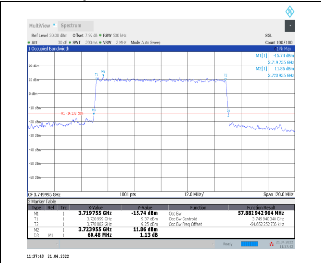
1-N78-3700-3800--30-60-M-7-CP-16QAM-Outer_Full-162@0-Ant0-57.883-60.480-≤60-PASS
