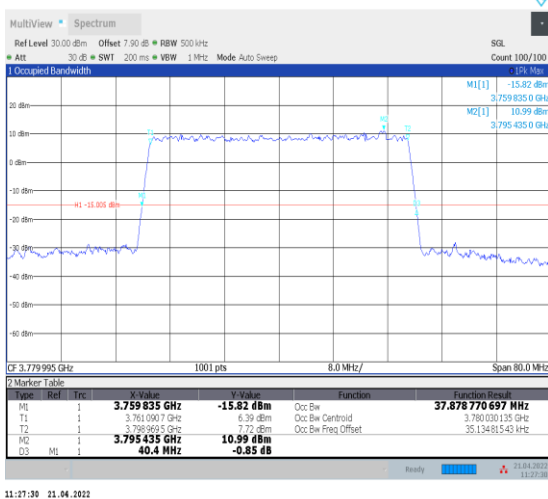
1-N78-3700-3800--30-40-H-9-CP-256QAM-Outer_Fu ll-106@0-Ant0-37.879-40.400-≤40-PASS
