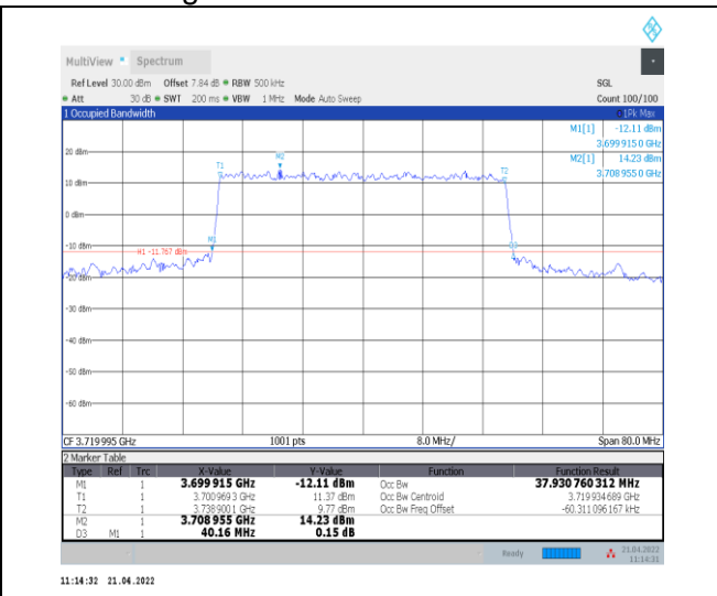
1-N78-3700-3800--30-40-L-6-CP-QPSK-Outer_Full-106@0-Ant0-37.931-40.160-≤40-PASS
