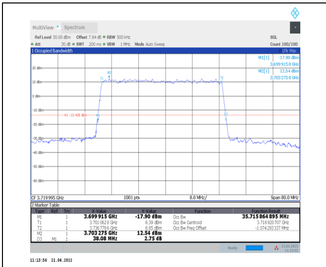
1-N78-3700-3800--30-40-L-5-DFT-256QAM-Outer_Full-100@0-Ant0-35.716-38.080-≤40-PASS
