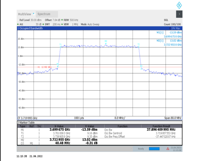
1-N78-3700-3800--30-40-L-8-CP-64QAM-Outer_Full-106@0-Ant0-37.896-40.480-≤40-PASS
