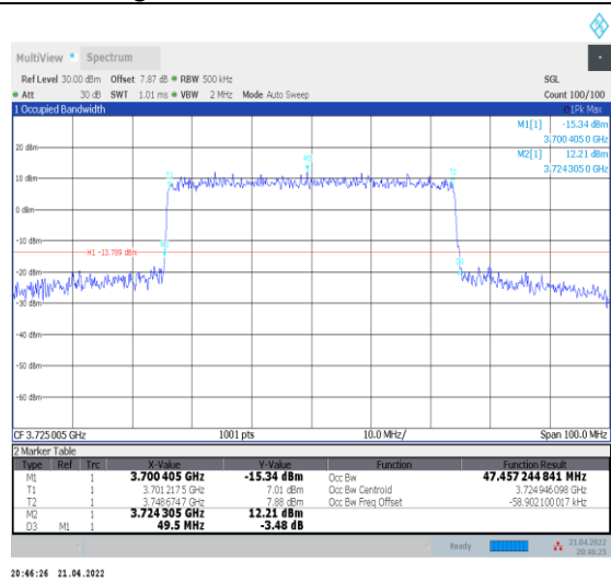
1-N78-3700-3800--30-50-L-7-CP-16QAM-Outer_Full -133@0-Ant0-47.457-49.500≤50-PASS
