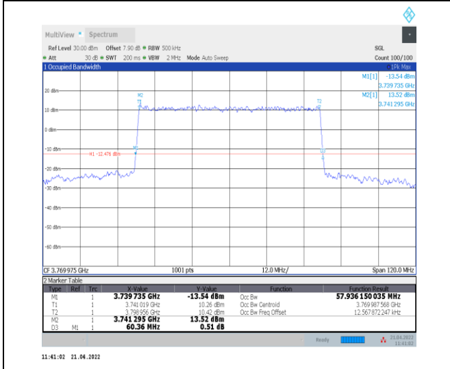
1-N78-3700-3800--30-60-H-3-DFT-16QAM-Outer_Fu ll-162@0-Ant0-57.936-60.360-≤60-PASS
