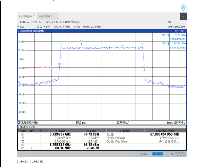
1-N78-3700-3800--30-60-H-2-DFT-PI2BPSK-Outer_Full Full-162@0-Ant0-57.887-60.360-≤60-PASS
