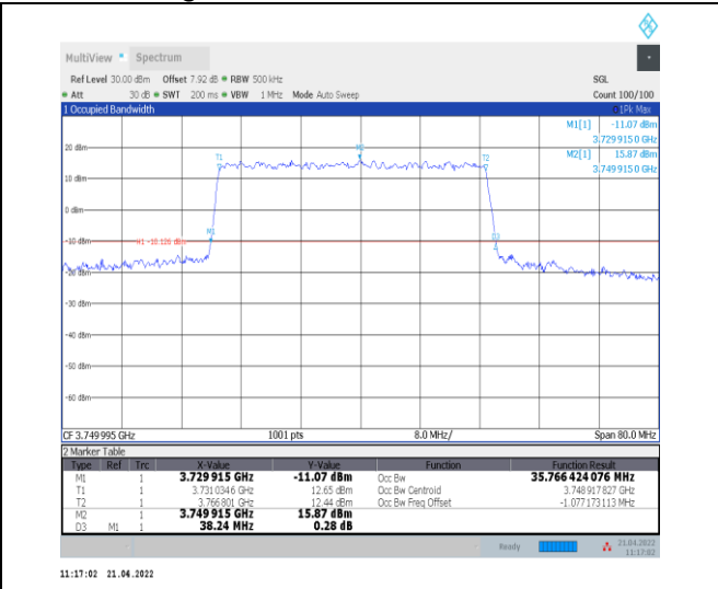
1-N78-3700-3800--30-40-M-1-DFT-QPSK-Outer_Full -100@0-Ant0-35.766-38.240-≤40-PASS
