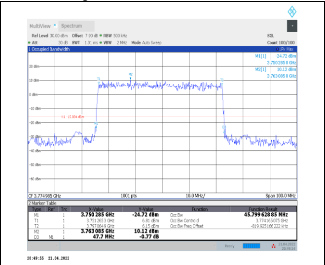
1-N78-3700-3800--30-50-H-5-DFT-256QAM-Outer_Full-128@0-Ant0-45.8-47.700-≤50-PASS
