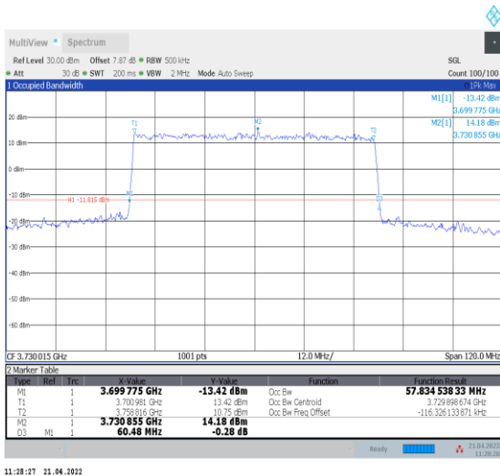
1-N78-3700-3800--30-60-L-1-DFT-QPSK-Outer_Full-162@0-Ant0-57.835-60.480-≤60-PASS
