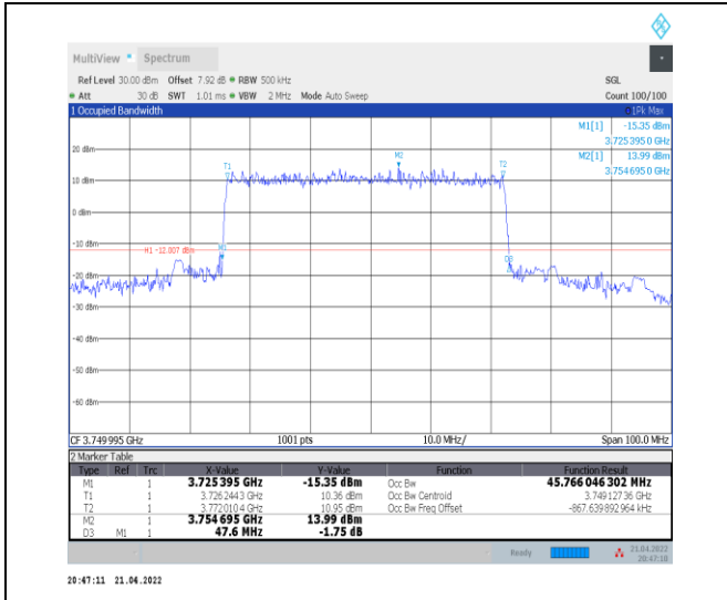
1-N78-3700-3800--30-50-M-1-DFT-QPSK-Outer_Full -128@0-Ant0-45.766-47.600-≤50-PASS
