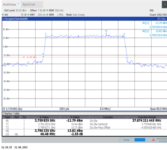
1-N78-3700-3800--30-40-H-7-CP-16QAM-Outer_Full -106@0-Ant0-37.874-40.480-≤40-PASS
