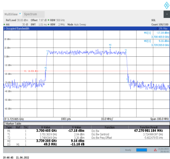
1-N78-3700-3800--30-50-L-9-CP-256QAM-Outer_Fu ll-133@0-Ant0-47.271-49.300≤50-PASS
