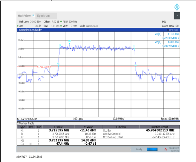
1-N78-3700-3800--30-50-M-2-DFT-PI2BPSK-Outer_Full -128@0-Ant0-45.704-47.400-≤50-PASS
