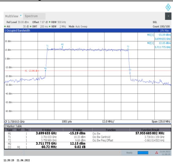
1-N78-3700-3800--30-60-L-4-DFT-64QAM-Outer_Fu II-162@0-Ant0-57.956-60.720-≤60-PASS
