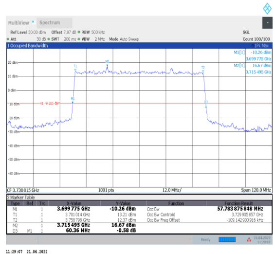
1-N78-3700-3800--30-60-L-2-DFT-PI2BPSK-Outer_Full-162@0-Ant0-57.784-60.360-≤60-PASS
