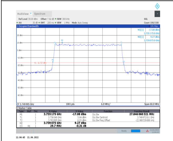
1-N78-3700-3800--30-30-M-9-CP-256QAM-Outer_F ull-78@0-Ant0-27.846-29.700-≤30-PASS
