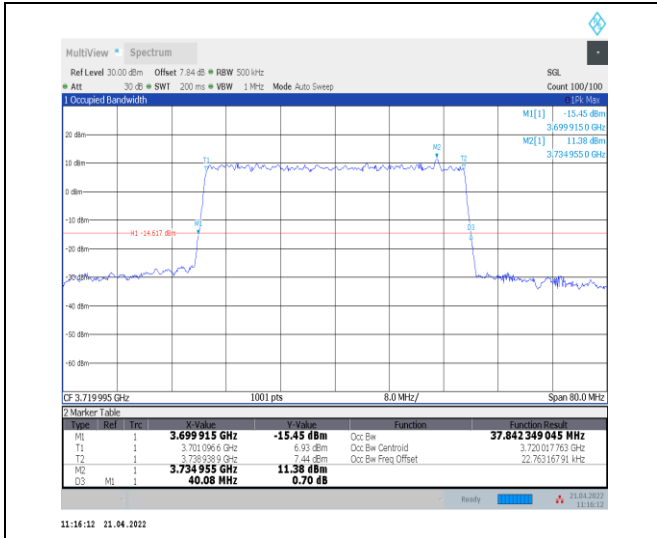
1-N78-3700-3800--30-40-L-9-CP-256QAM-Outer_Fu II-106@0-Ant0-37.842-40.080-≤40-PASS
