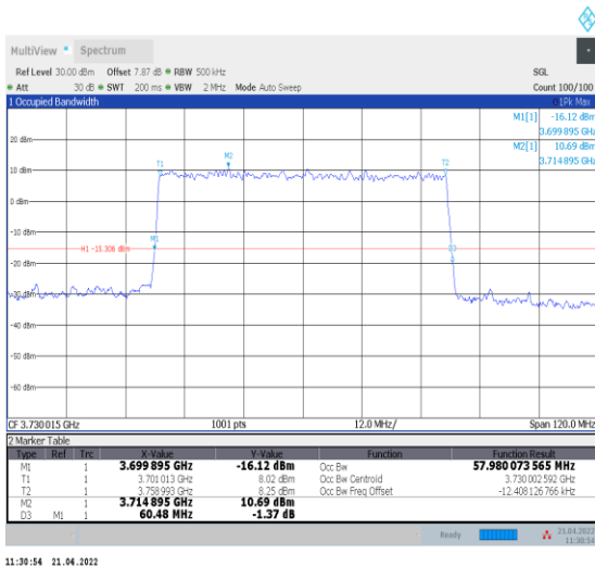
1-N78-3700-3800--30-60-L-5-DFT-256QAM-Outer_F ull-162@0-Ant0-57.98-60.480-≤60-PASS
