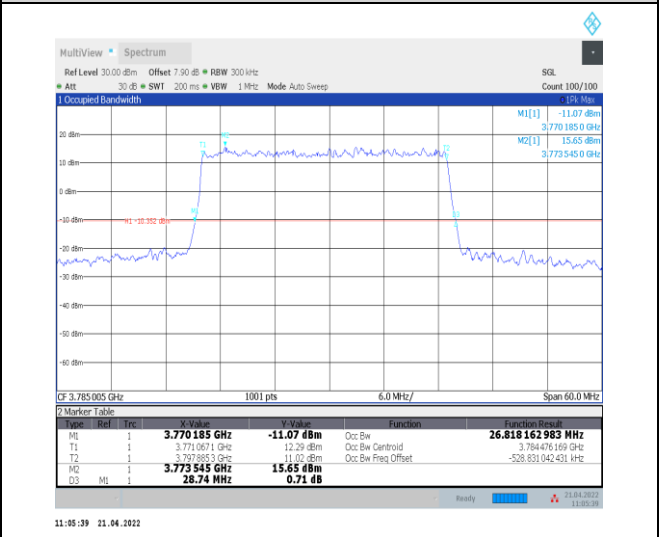
1-N78-3700-3800--30-30-H-1-DFT-QPSK-Outer_Full -75@0-Ant0-26.818-28.740-≤30-PASS
