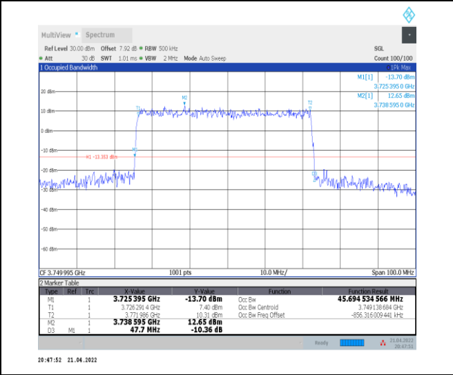
1-N78-3700-3800--30-50-M-4-DFT-64QAM-Outer_Full -128@0-Ant0-45.695-47.700-≤50-PASS
