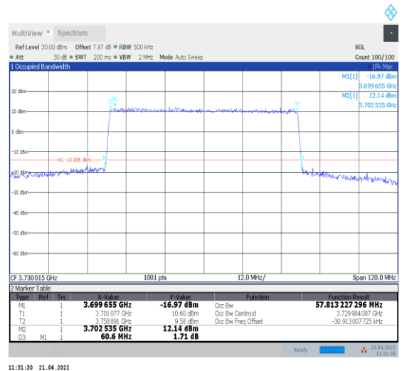
1-N78-3700-3800--30-60-L-6-CP-QPSK-Outer_Full- 162@0-Ant0-57.813-60.600-≤60-PASS
