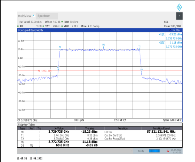
1-N78-3700-3800--30-60-H-8-CP-64QAM-Outer_Full-162@0-Ant0-57.821-60.600-≤60-PASS
