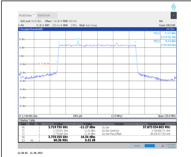
1-N78-3700-3800--30-60-M-2-DFT-PI2BPSK-Outer_Full-162@0-Ant0-57.874-60.360-≤60-PASS
