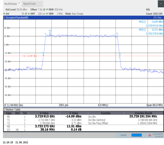
1-N78-3700-3800--30-40-M-5-DFT-256QAM-Outer_Full-100@0-Ant0-35.739-38.160-≤40-PASS
