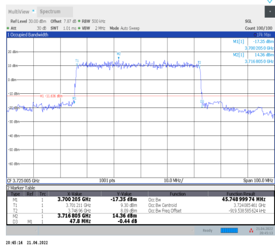
1-N78-3700-3800--30-50-L-1-DFT-QPSK-Outer_Full- 128@0-Ant0-45.749-47.800-≤50-PASS
