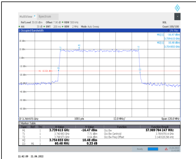
1-N78-3700-3800--30-60-H-5-DFT-256QAM-Outer_Full-162@0-Ant0-57.99-60.480-≤60-PASS
