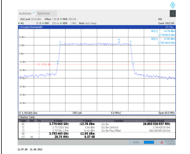
1-N78-3700-3800--30-30-H-4-DFT-64QAM-Outer_Fu II-75@0-Ant0-26.806-28.740-≤30-PASS
