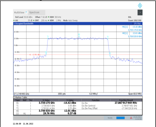
1-N78-3700-3800--30-30-M-8-CP-64QAM-Outer_Ful I-78@0-Ant0-27.868-29.760-≤30-PASS
