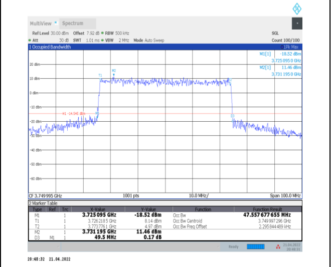
1-N78-3700-3800--30-50-M-8-CP-64QAM-Outer_Full-133@0-Ant0-47.558-49.500-<math>\leq 50</math>-PASS
