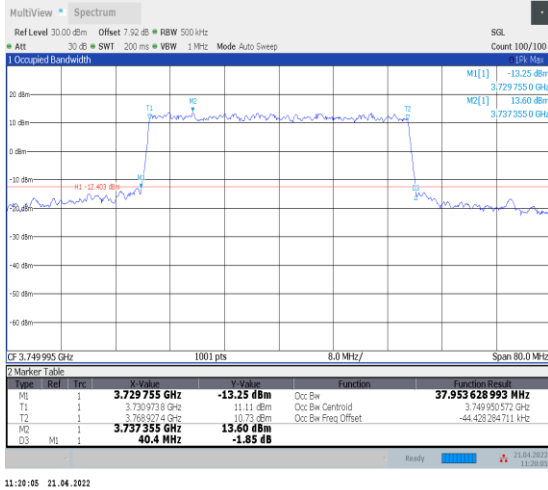
1-N78-3700-3800--30-40-M-6-CP-QPSK-Outer_Full-106@0-Ant0-37.954-40.400-≤40-PASS
