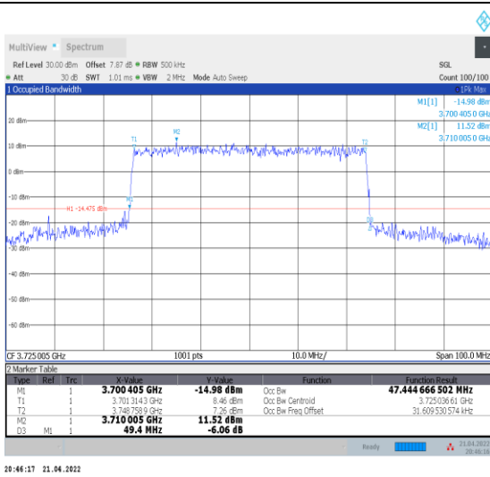
1-N78-3700-3800--30-50-L-6-CP-QPSK-Outer_Full-1 33@0-Ant0-47.445-49.400≤50-PASS
