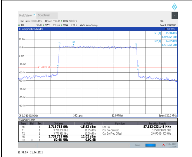
1-N78-3700-3800--30-60-M-4-DFT-64QAM-Outer_Full-162@0-Ant0-57.933-60.480-≤60-PASS
