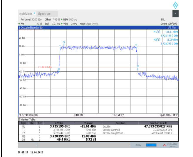
1-N78-3700-3800--30-50-M-7-CP-16QAM-Outer_Full-133@0-Ant0-47.393-49.400-<math>\leq 50</math>-PASS
