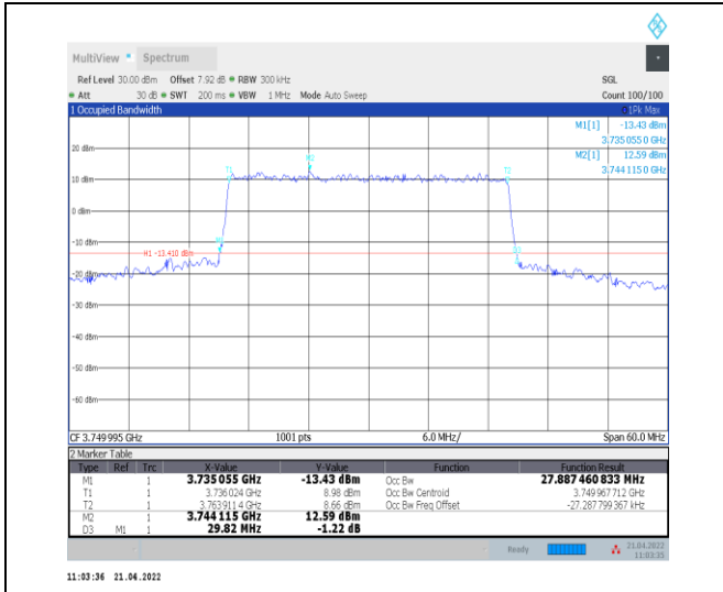
1-N78-3700-3800--30-30-M-7-CP-16QAM-Outer_Full -78@0-Ant0-27.887-29.820-≤30-PASS
