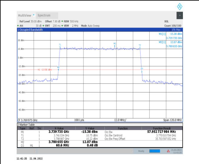
1-N78-3700-3800--30-60-H-4-DFT-64QAM-Outer_Fu ll-162@0-Ant0-57.953-60.600-≤60-PASS
