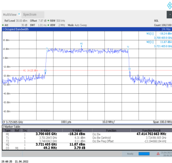
1-N78-3700-3800--30-50-L-8-CP-64QAM-Outer_Full -133@0-Ant0-47.415-49.200≤50-PASS
