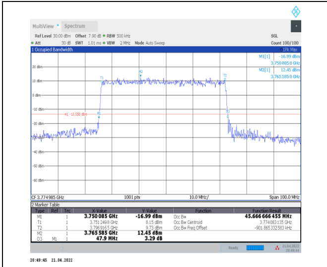
1-N78-3700-3800--30-50-H-4-DFT-64QAM-Outer_Fu II-128@0-Ant0-45.667-47.900-≤50-PASS
