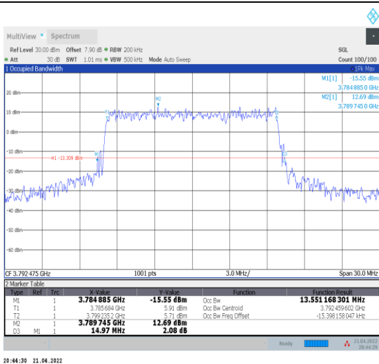
1-N78-3700-3800--30-15-H-8-CP-64QAM-Outer_Full -38@0-Ant0-13.551-14.970-≤15-PASS
