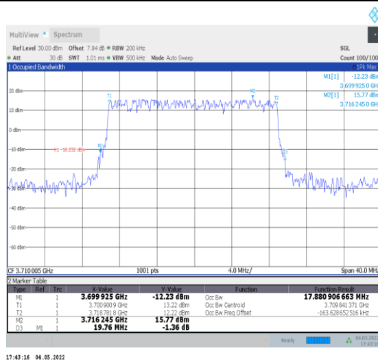
1-N78-3700-3800--30-20-L-2-DFT-PI2BPSK-Outer_Full Full-50@0-Ant0-17.881-19.760-≤20-PASS
