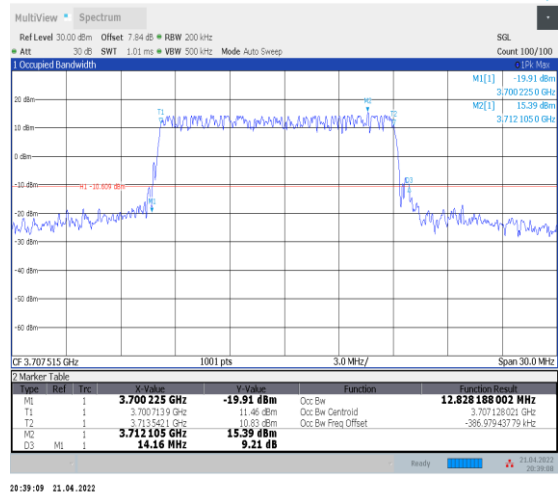
1-N78-3700-3800--30-15-L-1-DFT-QPSK-Outer_Full- 36@0-Ant0-12.828-14.160≤15-PASS
