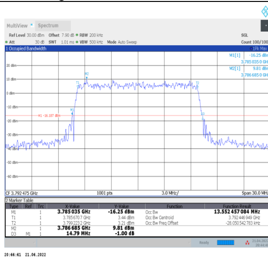
1-N78-3700-3800--30-15-H-9-CP-256QAM-Outer_Full ull-38@0-Ant0-13.552-14.790-≤15-PASS
