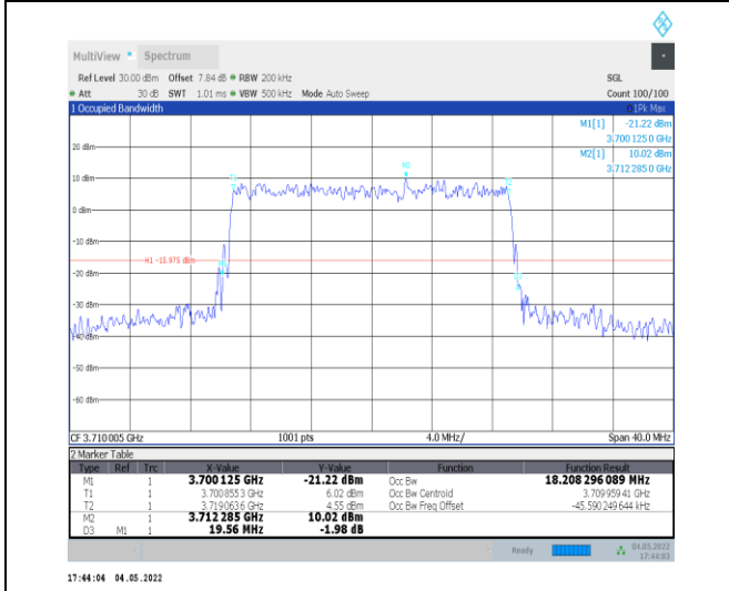
1-N78-3700-3800--30-20-L-9-CP-256QAM-Outer_Fu II-51 @0-Ant0-18.208-19.560-<=20-PASS
