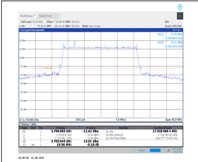
1-N78-3700-3800--30-20-L-3-DFT-16QAM-Outer_Ful I-50@0-Ant0-17.928-19.560-<math>\leq 20</math>-PASS
