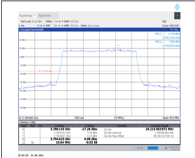
1-N78-3700-3800--30-20-H-9-CP-256QAM-Outer_Fu II-51 @0-Ant0-18.216-19.640-≤20-PASS
