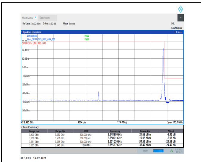
1-N78-3450-3550-PC1-30-70-H-2-DFT-PI2BPSK-Edge_1RB_Right-1@188-Ant0-1--PASS-see graph
