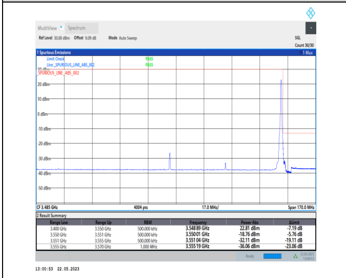
1-N78-3450-3550-PC1-30-70-H-5-CP-QPSK-Edge_1RB_Right-1@188-Ant0-1--PASS-see graph
