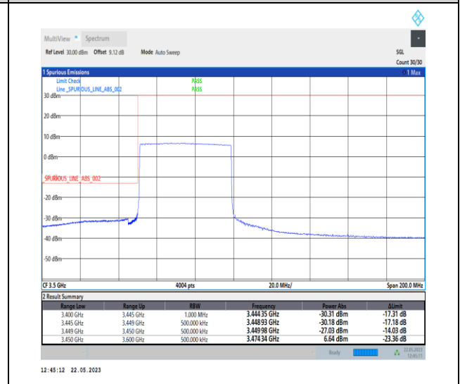
1-N78-3450-3550-PC1-30-50-L-6-CP-QPSK-Outer_Full-133@0-Ant0-1--PASS-see graph
