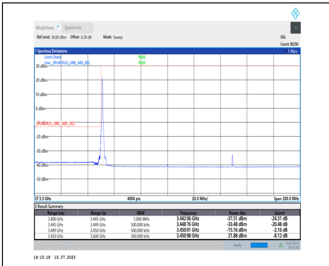
1-N78-3450-3550-PC1-30-100-L-1-DFT-PI2BPSK-Edge_e_1RB_Left-1@0-Ant0-1--PASS-see graph
