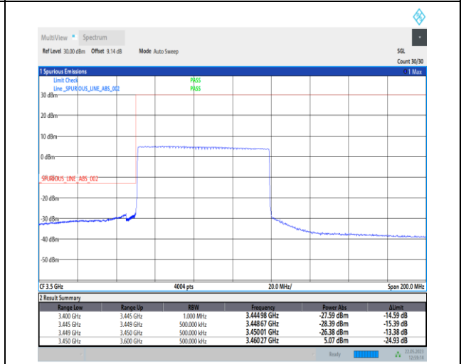
1-N78-3450-3550-PC1-30-70-L-3-DFT-PI2BPSK-Outer_Full-180@0-Ant0-1--PASS-see graph
