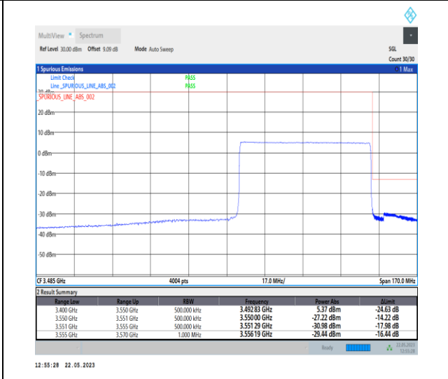
1-N78-3450-3550-PC1-30-60-H-6-CP-QPSK-Outer_Full-162@0-Ant0-1--PASS-see graph
