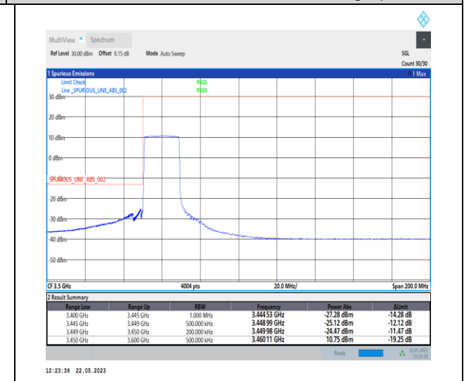
1-N78-3450-3550-PC1-30-20-L-6-CP-QPSK-Outer_Full-51@0-Ant0-1--PASS-see graph
