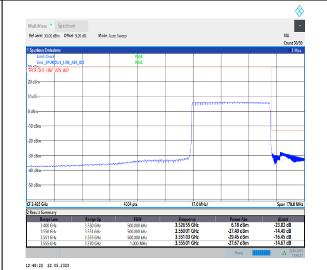
1-N78-3450-3550-PC1-30-50-H-6-CP-QPSK-Outer_Full-133@0-Ant0-1--PASS-see graph
