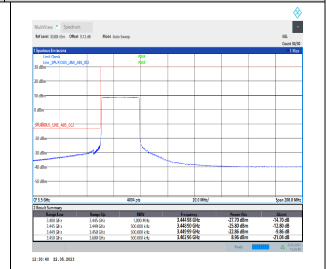
1-N78-3450-3550-PC1-30-30-L-6-CP-QPSK-Outer_Full-78@0-Ant0-1--PASS-see graph
