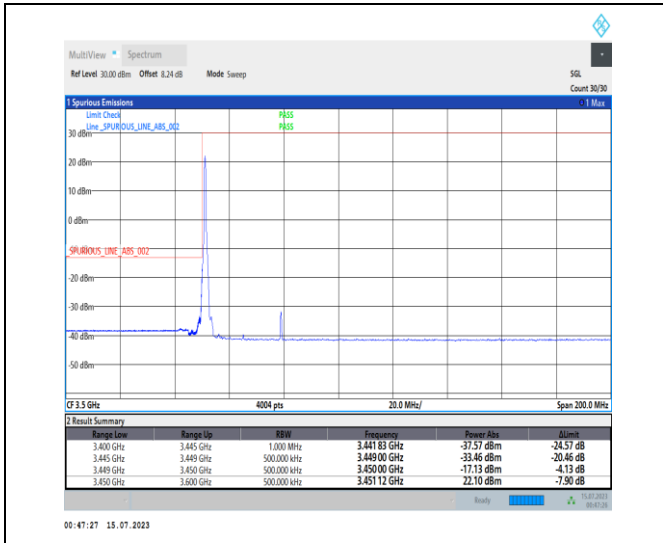
1-N78-3450-3550-PC1-30-30-L-1-DFT-PI2BPSK-Edge_e_1RB_Left-1@0-Ant0-1--PASS-see graph
