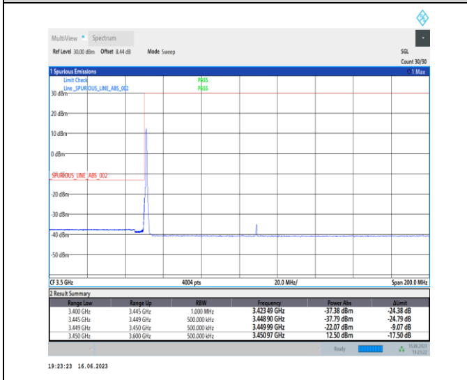
1-N78-3450-3550-PC1-30-60-L-4-CP-QPSK-Edge_1RB_Left-1@0-Ant0-1--PASS-see graph
