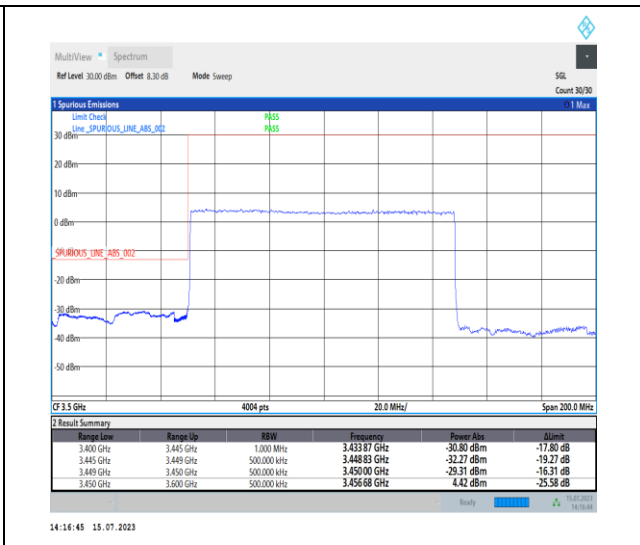
1-N78-3450-3550-PC1-30-100-L-3-DFT-PI2BPSK-Outer_Full-270@0-Ant0-1--PASS-see graph
