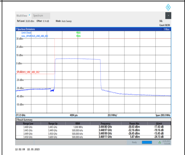
1-N78-3450-3550-PC1-30-60-L-6-CP-QPSK-Outer_Full-162@0-Ant0-1--PASS-see graph
