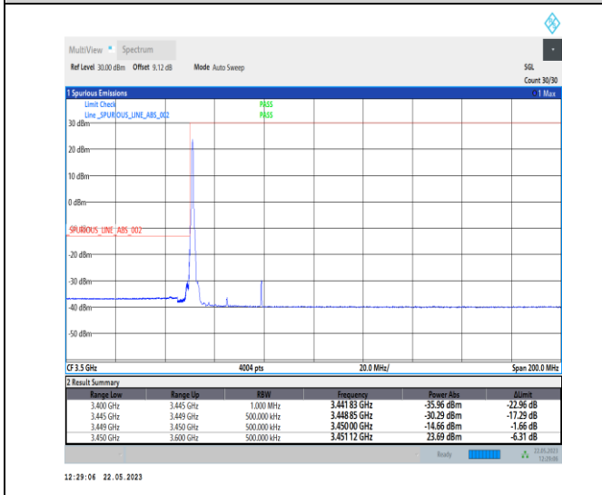
1-N78-3450-3550-PC1-30-30-L-4-CP-QPSK-Edge_1R_B_Left-1@0-Ant0-1--PASS-see graph
