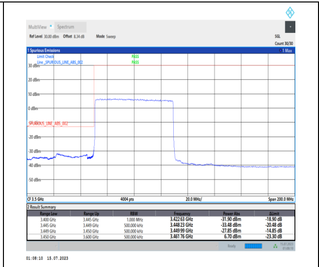
1-N78-3450-3550-PC1-30-60-L-3-DFT-PI2BPSK-Outer_Full-162@0-Ant0-1--PASS-see graph
