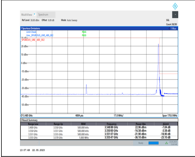
1-N78-3450-3550-PC1-30-80-H-5-CP-QPSK-Edge_1RB_Right-1@216-Ant0-1--PASS-see graph
