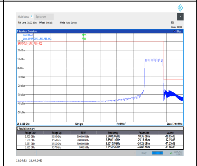
1-N78-3450-3550-PC1-30-20-H-6-CP-QPSK-Outer_Full-51@0-Ant0-1--PASS-see graph
