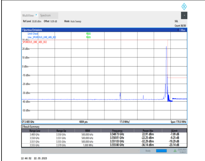
1-N78-3450-3550-PC1-30-50-H-5-CP-QPSK-Edge_1RB_Right-1@132-Ant0-1--PASS-see graph
