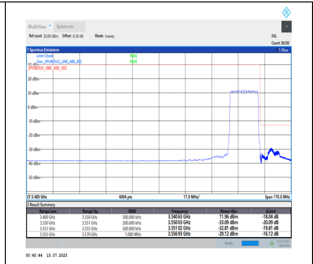
1-N78-3450-3550-PC1-30-20-H-3-DFT-PI2BPSK-Outer_Full-50@0-Ant0-1--PASS-see graph
