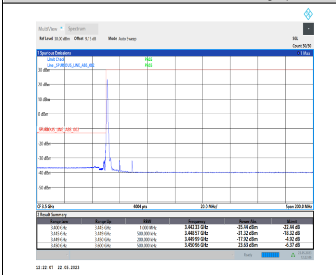
1-N78-3450-3550-PC1-30-20-L-4-CP-QPSK-Edge_1_RB_Left-1@0-Ant0-1--PASS-see graph
