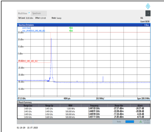
1-N78-3450-3550-PC1-30-80-L-1-DFT-PI2BPSK-Edge_1RB_Left-1@0-Ant0-1--PASS-see graph
