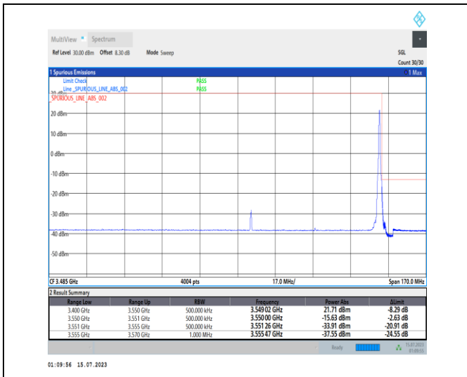
1-N78-3450-3550-PC1-30-60-H-2-DFT-PI2BPSK-Edge_e_1RB_Right-1@161-Ant0-1--PASS-see graph
