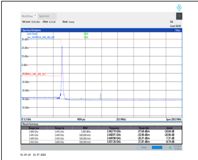
1-N78-3450-3550-PC1-30-50-L-1-DFT-PI2BPSK-Edge_1RB_Left-1@0-Ant0-1--PASS-see graph
