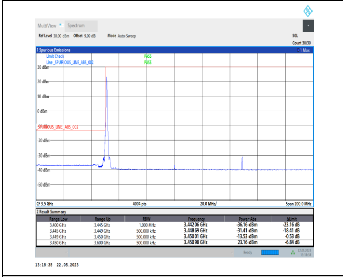
1-N78-3450-3550-PC1-30-100-L-4-CP-QPSK-Edge_1RB_Left-1@0-Ant0-1--PASS-see graph
