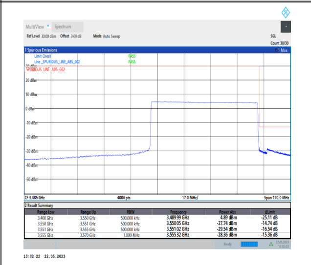
1-N78-3450-3550-PC1-30-70-H-6-CP-QPSK-Outer_Full-189@0-Ant0-1--PASS-see graph
