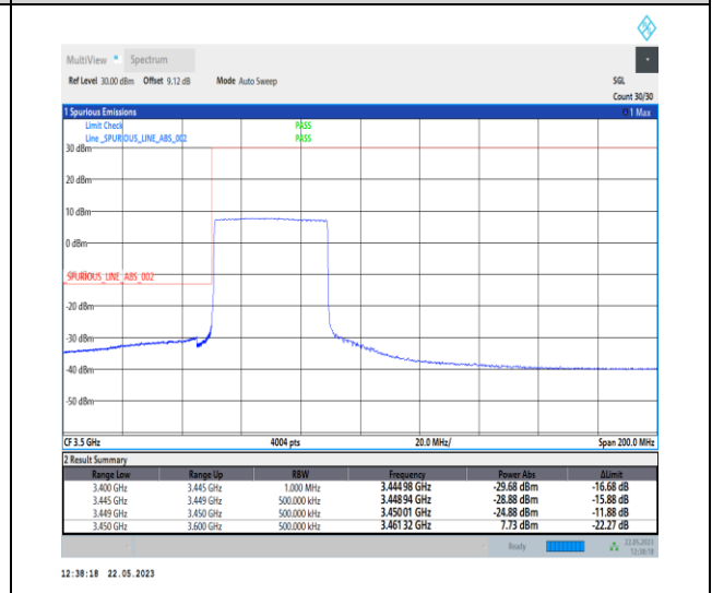
1-N78-3450-3550-PC1-30-40-L-6-CP-QPSK-Outer_Full-106@0-Ant0-1--PASS-see graph
