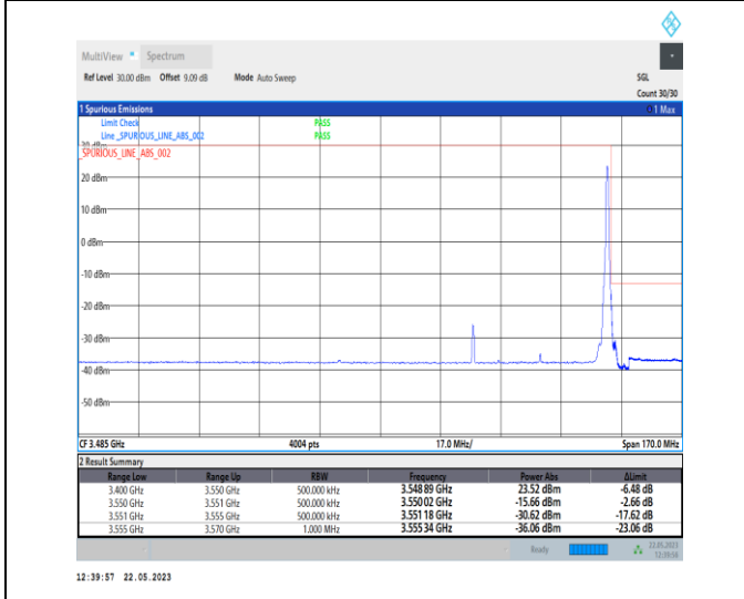
1-N78-3450-3550-PC1-30-40-H-5-CP-QPSK-Edge_1RB_Right-1@105-Ant0-1--PASS-see graph
