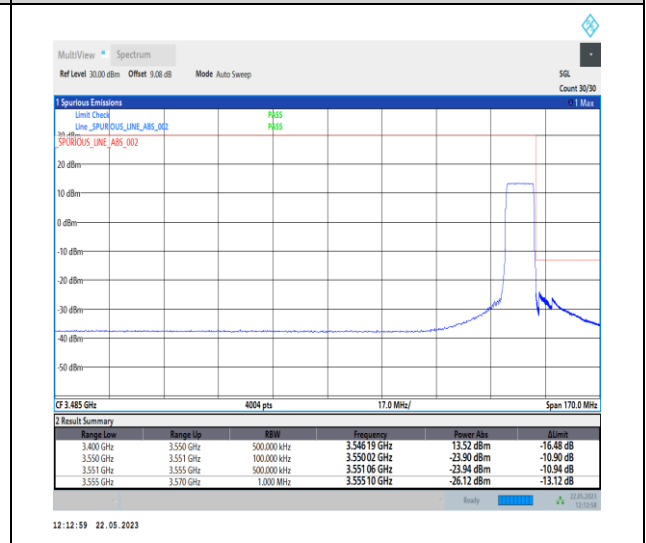
1-N78-3450-3550-PC1-30-10-H-6-CP-QPSK-Outer _Full-24@0-Ant0-1--PASS-see graph
