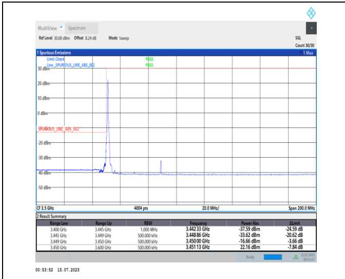
1-N78-3450-3550-PC1-30-40-L-1-DFT-PI2BPSK-Edge_1RB_Left-1@0-Ant0-1--PASS-see graph
