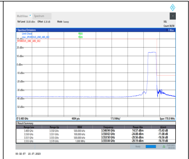
1-N78-3450-3550-PC1-30-10-H-3-DFT-PI2BPSK- Outer_Full-24@0-Ant0-1--PASS-see graph
