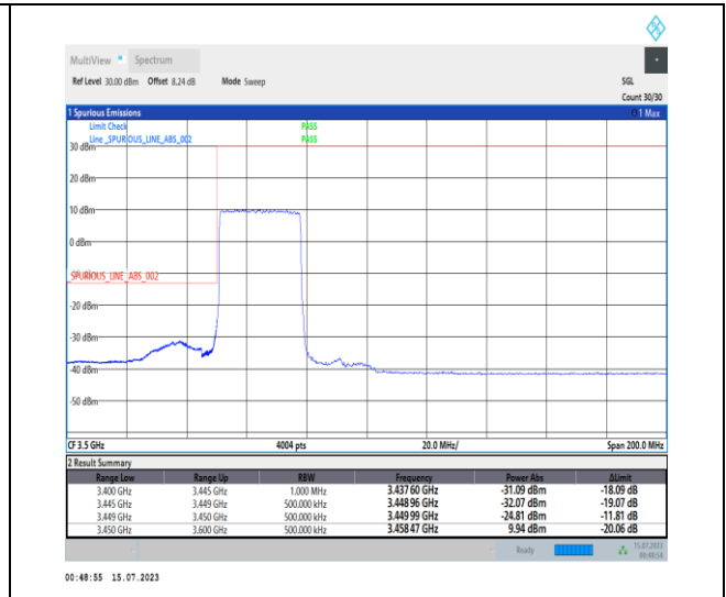
1-N78-3450-3550-PC1-30-30-L-3-DFT-PI2BPSK-Outer_Full-75@0-Ant0-1--PASS-see graph
