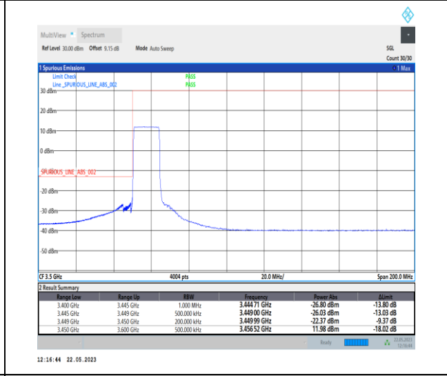
1-N78-3450-3550-PC1-30-15-L-6-CP-QPSK-Outer_Full-38@0-Ant0-1--PASS-see graph
