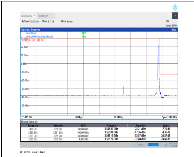
1-N78-3450-3550-PC1-30-40-H-2-DFT-PI2BPSK-Edge_1RB_Right-1@105-Ant0-1--PASS-see graph
