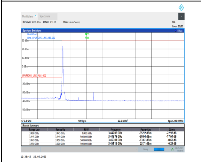
1-N78-3450-3550-PC1-30-40-L-4-CP-QPSK-Edge_1RB_Left-1@0-Ant0-1--PASS-see graph
