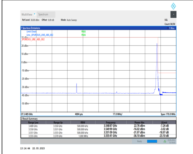
1-N78-3450-3550-PC1-30-90-H-5-CP-QPSK-Edge_1RB_Right-1@244-Ant0-1--PASS-see graph
