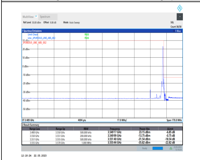
1-N78-3450-3550-PC1-30-15-H-5-CP-QPSK-Edge_1RB_Right-1@37-Ant0-1--PASS-see graph
