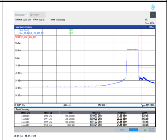
1-N78-3450-3550-PC1-30-15-H-6-CP-QPSK-Outer_Full-38@0-Ant0-1--PASS-see graph
