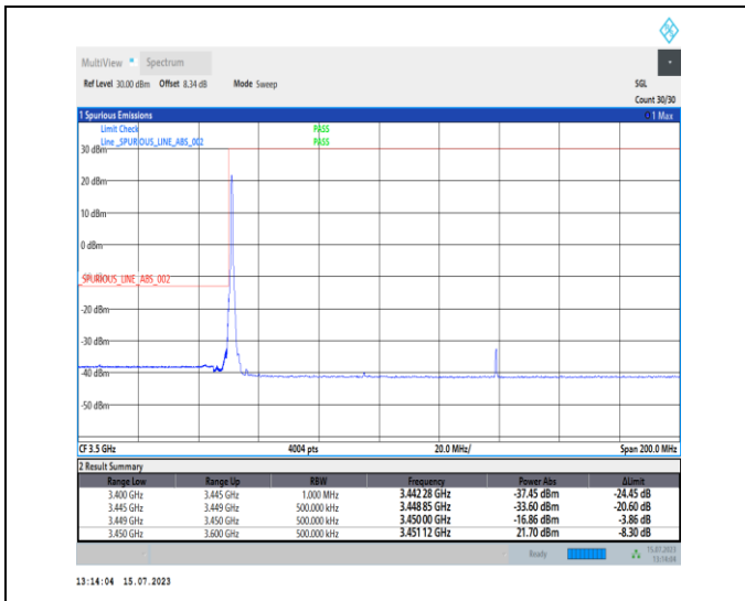
1-N78-3450-3550-PC1-30-90-L-1-DFT-PI2BPSK-Edge_1RB_Left-1@0-Ant0-1--PASS-see graph
