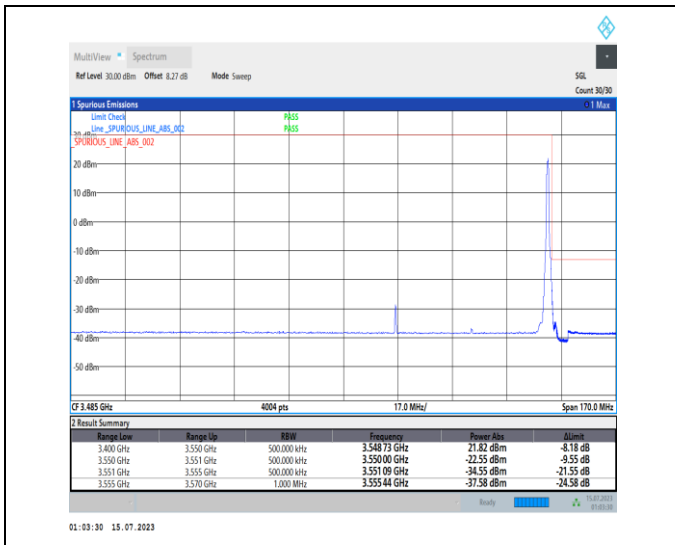
1-N78-3450-3550-PC1-30-50-H-2-DFT-PI2BPSK-Edge_1RB_Right-1@132-Ant0-1--PASS-see graph
