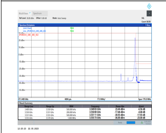
1-N78-3450-3550-PC1-30-20-H-5-CP-QPSK-Edge_1RB_Right-1@50-Ant0-1--PASS-see graph
