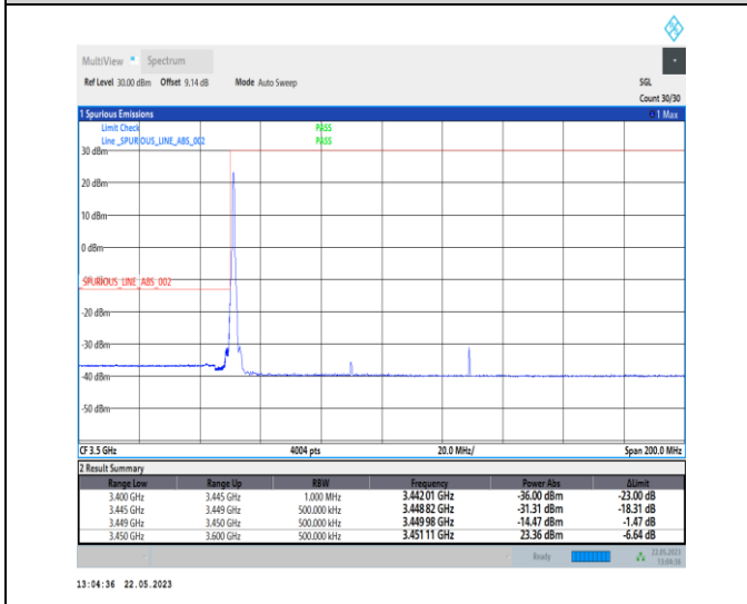
1-N78-3450-3550-PC1-30-80-L-4-CP-QPSK-Edge_1RB_Left-1@0-Ant0-1--PASS-see graph
