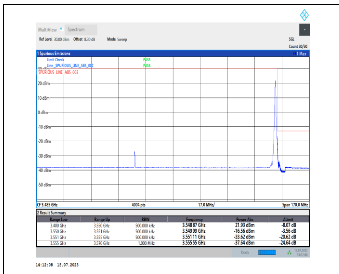
1-N78-3450-3550-PC1-30-90-H-2-DFT-PI2BPSK-Edge_1RB_Right-1@244-Ant0-1--PASS-see graph
