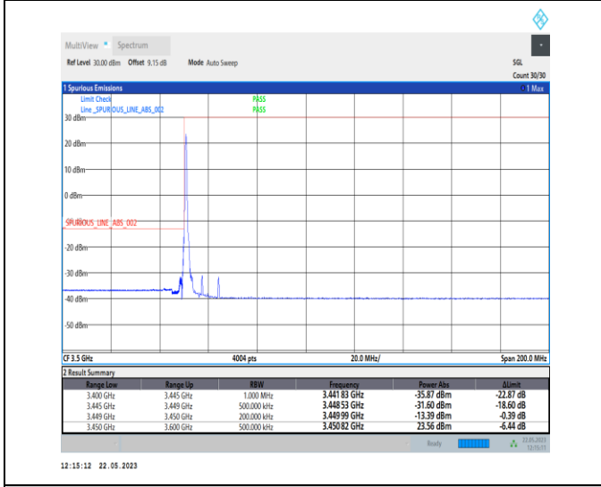
1-N78-3450-3550-PC1-30-15-L-4-CP-QPSK-Edge_1RB_Left-1@0-Ant0-1--PASS-see graph
