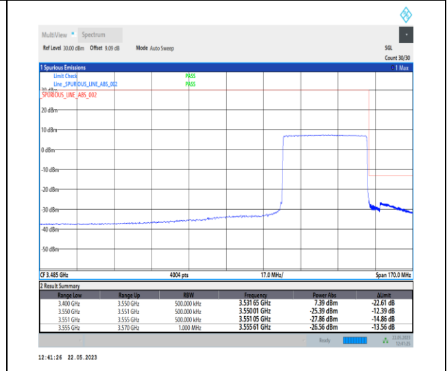
1-N78-3450-3550-PC1-30-40-H-6-CP-QPSK-Outer_Full-106@0-Ant0-1--PASS-see graph
