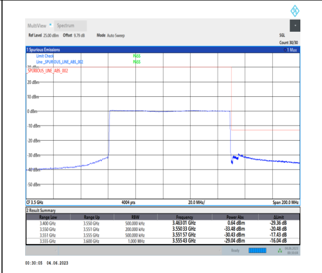
1-N78-3450-3550-PC1-30-90-H-6-CP-QPSK-Outer_Full-245@0-Ant0-1--PASS-see graph
