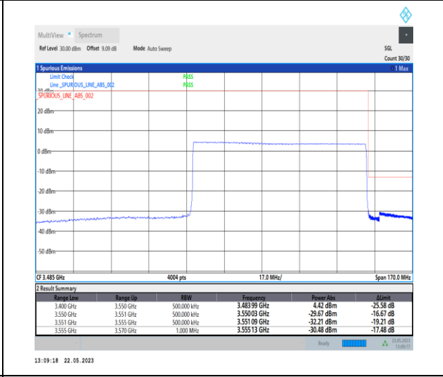
1-N78-3450-3550-PC1-30-80-H-6-CP-QPSK-Outer_Full-217@0-Ant0-1--PASS-see graph
