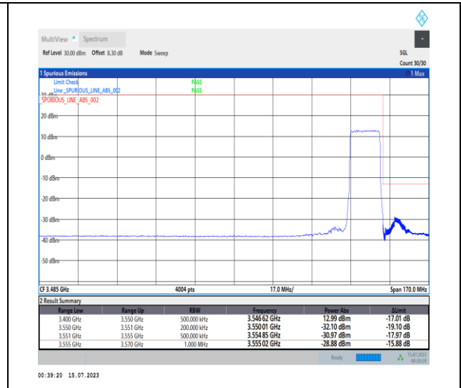
1-N78-3450-3550-PC1-30-15-H-3-DFT-PI2BPSK-Outer_Full-36@0-Ant0-1--PASS-see graph
