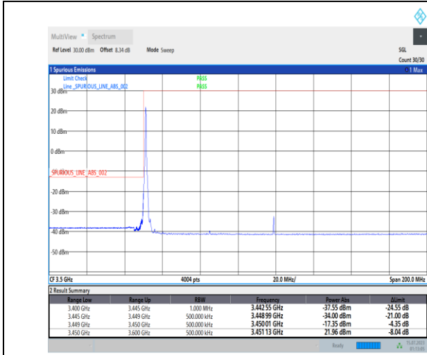
1-N78-3450-3550-PC1-30-70-L-1-DFT-PI2BPSK-Edge_1RB_Left-1@0-Ant0-1--PASS-see graph
