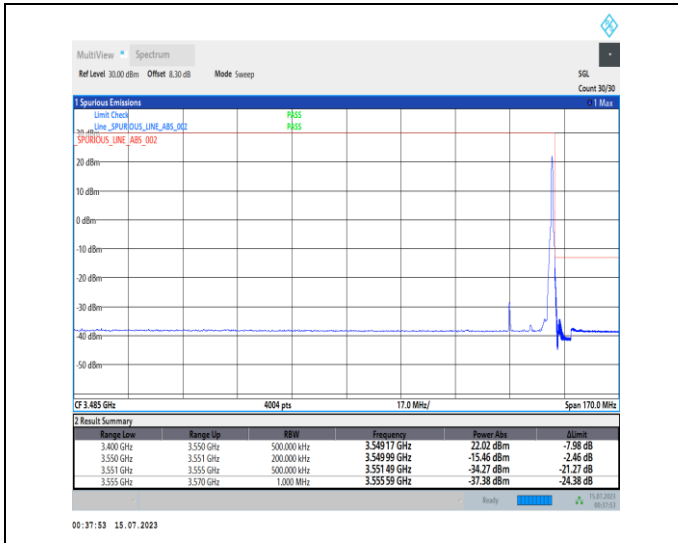
1-N78-3450-3550-PC1-30-15-H-2-DFT-PI2BPSK-Edge_1RB_Right-1@37-Ant0-1--PASS-see graph
