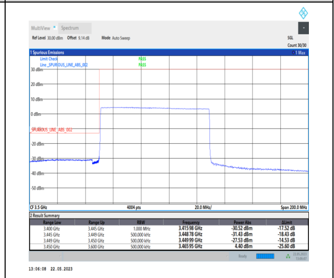
1-N78-3450-3550-PC1-30-80-L-6-CP-QPSK-Outer_Full-217@0-Ant0-1--PASS-see graph
