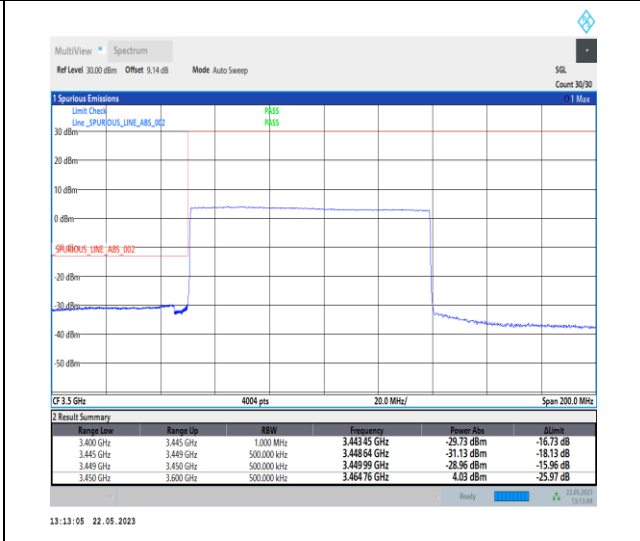
1-N78-3450-3550-PC1-30-90-L-6-CP-QPSK-Outer_Full-245@0-Ant0-1--PASS-see graph
