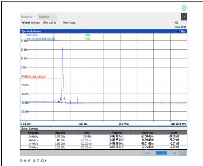
1-N78-3450-3550-PC1-30-20-L-1-DFT-PI2BPSK-Edge_1_RB_Left-1@0-Ant0-1--PASS-see graph
