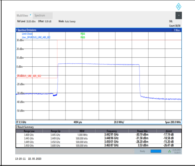
1-N78-3450-3550-PC1-30-100-L-6-CP-QPSK-Outer_Full-273@0-Ant0-1--PASS-see graph
