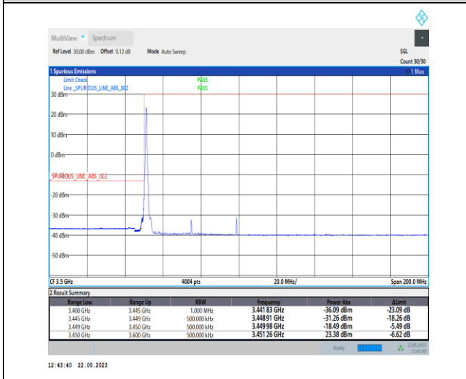
1-N78-3450-3550-PC1-30-50-L-4-CP-QPSK-Edge_1RB_Left-1@0-Ant0-1--PASS-see graph
