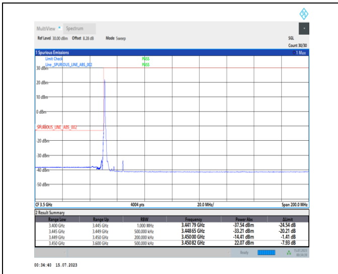
1-N78-3450-3550-PC1-30-15-L-1-DFT-PI2BPSK-Edge_e_1RB_Left-1@0-Ant0-1--PASS-see graph
