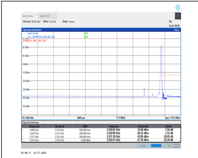
1-N78-3450-3550-PC1-30-20-H-2-DFT-PI2BPSK-Edge_1RB_Right-1@50-Ant0-1--PASS-see graph
