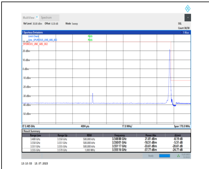
1-N78-3450-3550-PC1-30-80-H-2-DFT-PI2BPSK-Edge_1RB_Right-1@216-Ant0-1--PASS-see graph
