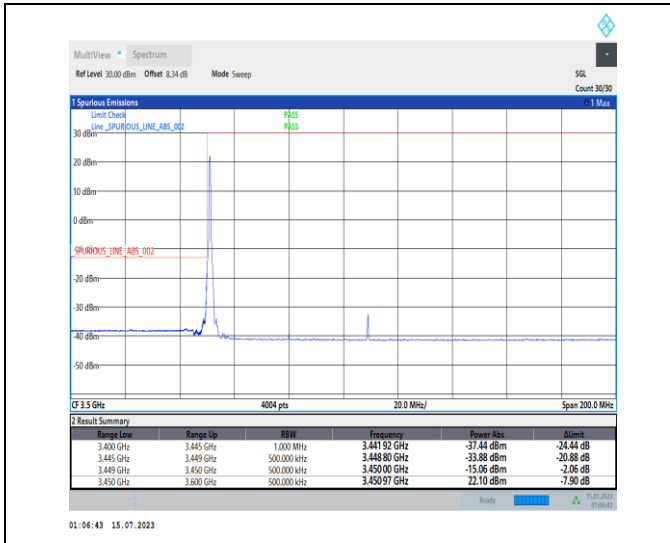
1-N78-3450-3550-PC1-30-60-L-1-DFT-PI2BPSK-Edge_1RB_Left-1@0-Ant0-1--PASS-see graph
