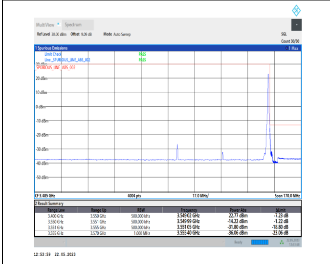
1-N78-3450-3550-PC1-30-60-H-5-CP-QPSK-Edge_1RB_Right-1@161-Ant0-1--PASS-see graph
