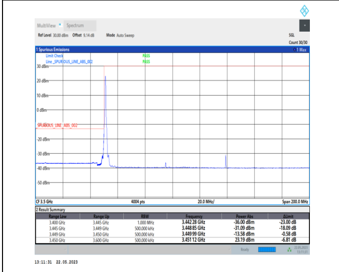
1-N78-3450-3550-PC1-30-90-L-4-CP-QPSK-Edge_1RB_Left-1@0-Ant0-1--PASS-see graph
