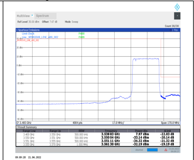
1-N78-3450-3550--30-30-H-3-DFT-PI2BPSK-Outer_Full-75@0-Ant0-PASS-see graph
