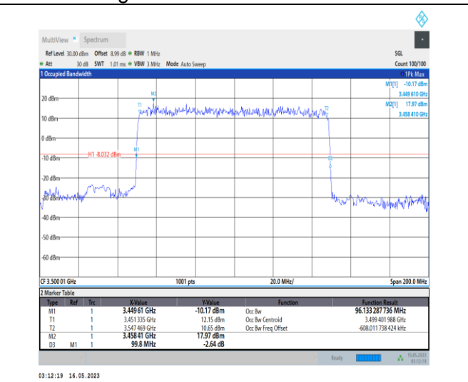
1-N78-3450-3550-PC1-30-100-H-2-DFT-PI2BPSK-Outer_Full-270@0-Ant0-96.133-99.800-≤100-PASS
