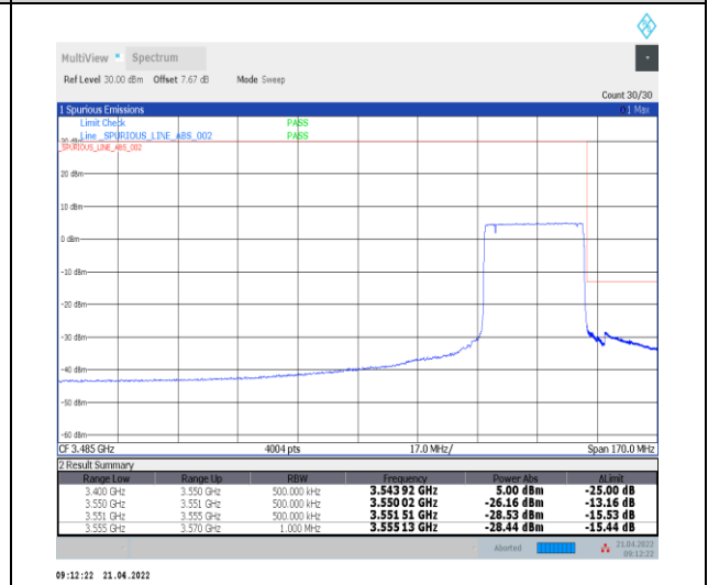
1-N78-3450-3550--30-30-H-6-CP-QPSK-Outer_Fu ll-78@0-Ant0-PASS-see graph
