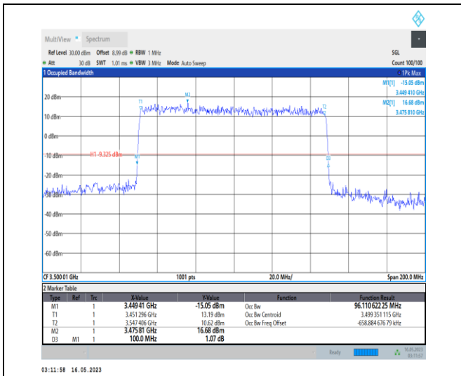
1-N78-3450-3550-PC1-30-100-H-1-DFT-QPSK-Outer_Full-270@0-Ant0-96.111-100.000-≤100-PASS
