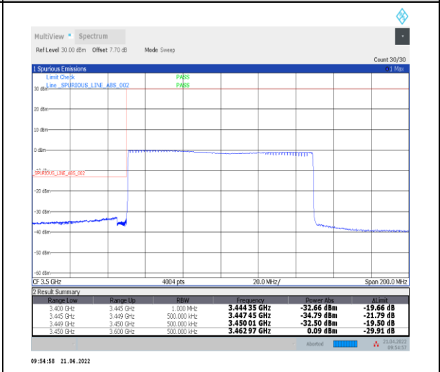
1-N78-3450-3550--30-100-L-6-CP-QPSK-Outer_F ull-273@0-Ant0-PASS-see graph
