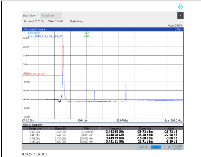
1-N78-3450-3550--30-80-L-1-DFT-PI2BPSK-Edge_1R_B_Left-1@0-Ant0-PASS-see graph
