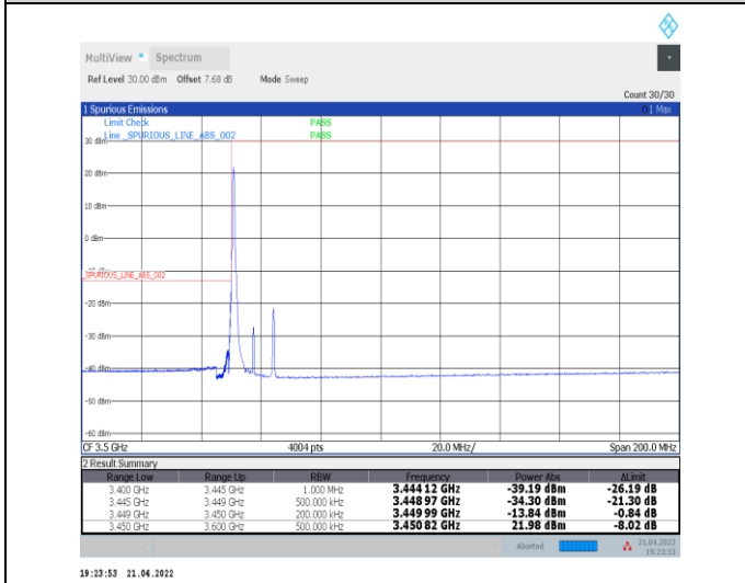
1-N78-3450-3550--30-15-L-4-CP-QPSK-Edge_1RB_L_eff-1@0-Ant0-PASS-see graph
