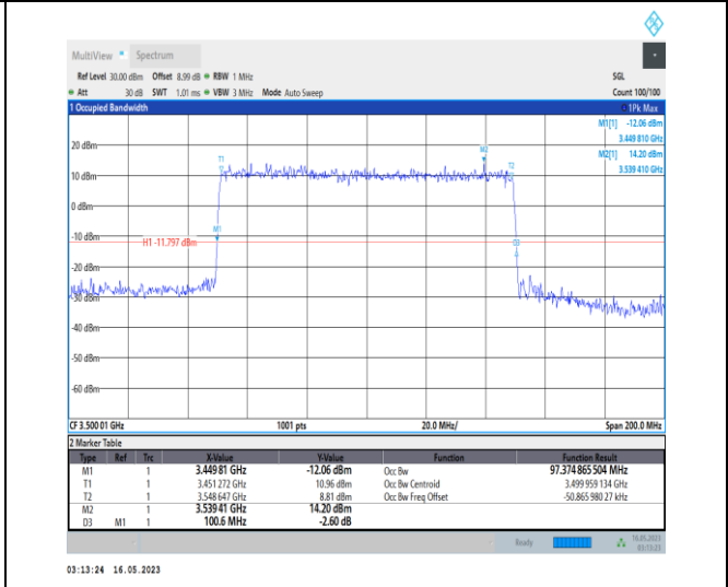
1-N78-3450-3550-PC1-30-100-H-8-CP-64QAM-Outer_Full-273@0-Ant0-97.375-100.600-≤100-PASS
