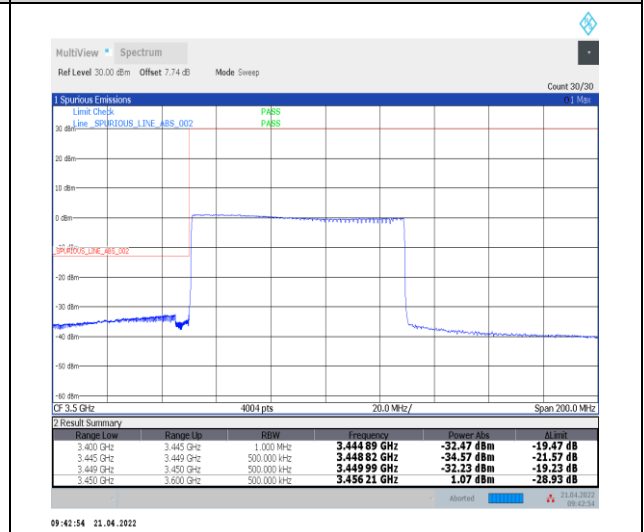
1-N78-3450-3550--30-80-L-6-CP-QPSK-Outer_Ful I-217@0-Ant0-PASS-see graph
