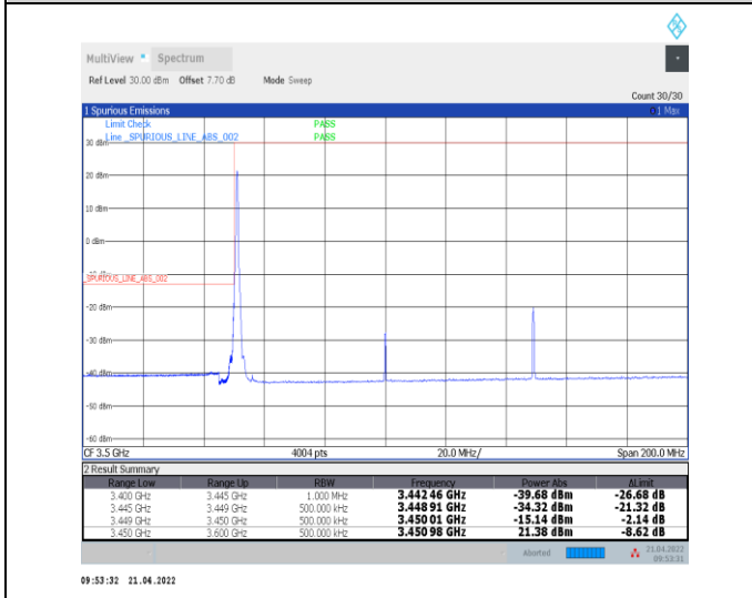
1-N78-3450-3550--30-100-L-4-CP-QPSK-Edge_1RB_Left-1@0-Ant0-PASS-see graph
