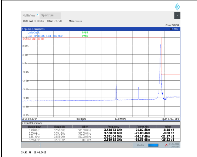
1-N78-3450-3550--30-50-H-5-CP-QPSK-Edge_1RB_Right-1@132-Ant0-PASS-see graph
