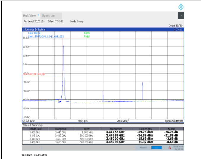
1-N78-3450-3550--30-100-L-1-DFT-PI2BPSK-Edge_1 RB_Left-1@0-Ant0-PASS-see graph
