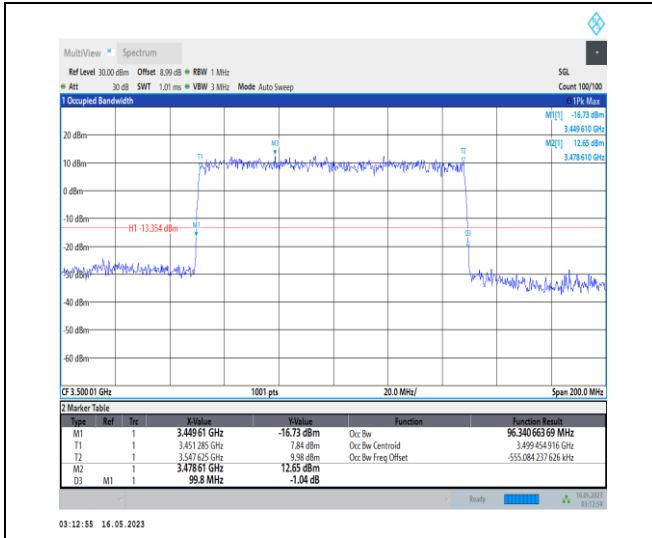
1-N78-3450-3550-PC1-30-100-H-5-DFT-256QAM-Outer_Full-270@0-Ant0-96.341-99.800-≤100-PASS
