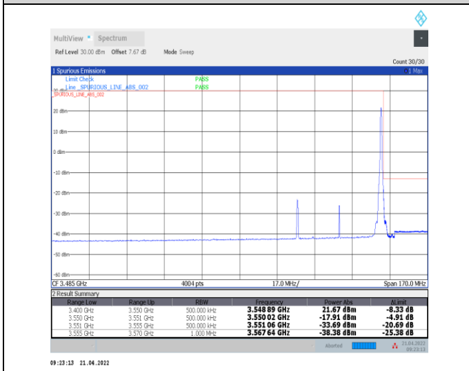
1-N78-3450-3550--30-40-H-5-CP-QPSK-Edge_1RB_Right-1@105-Ant0-PASS-see graph
