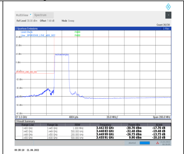
1-N78-3450-3550--30-20-L-3-DFT-PI2BPSK-Outer_Full-50@0-Ant0-PASS-see graph
