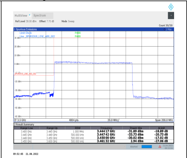
1-N78-3450-3550--30-100-L-3-DFT-PI2BPSK-Out er_Full-270@0-Ant0-PASS-see graph
