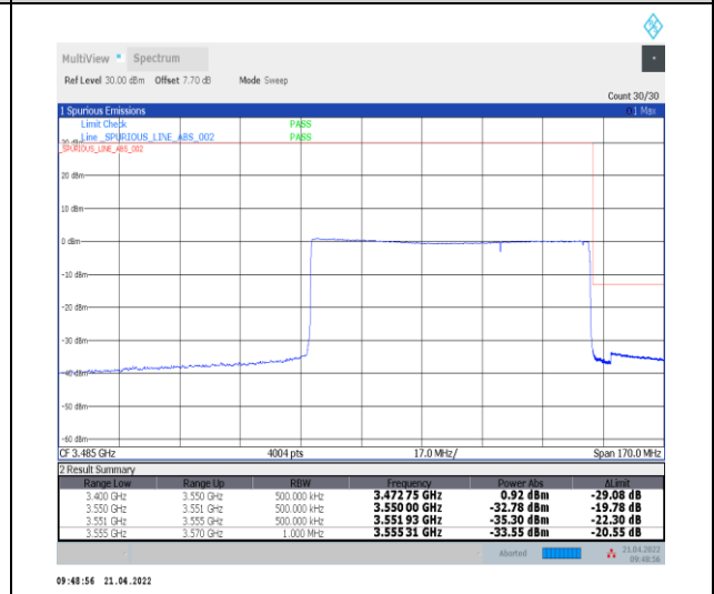
1-N78-3450-3550--30-80-H-6-CP-QPSK-Outer_Full-217@0-Ant0-PASS-see graph
