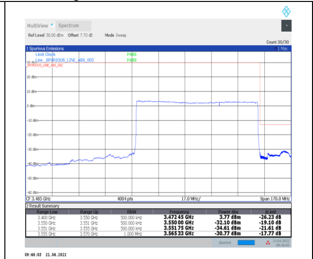
1-N78-3450-3550--30-80-H-3-DFT-PI2BPSK-Outer_Full-216@0-Ant0-PASS-see graph
