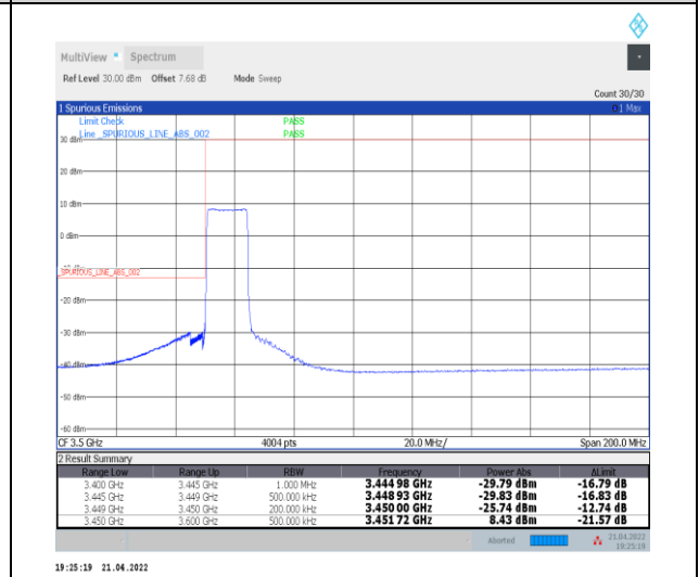
1-N78-3450-3550--30-15-L-6-CP-QPSK-Outer_Ful l-38@0-Ant0-PASS-see graph
