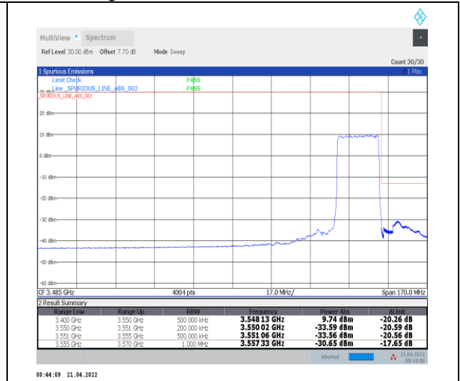
1-N78-3450-3550--30-20-H-3-DFT-PI2BPSK-Outer_Full-50@0-Ant0-PASS-see graph
