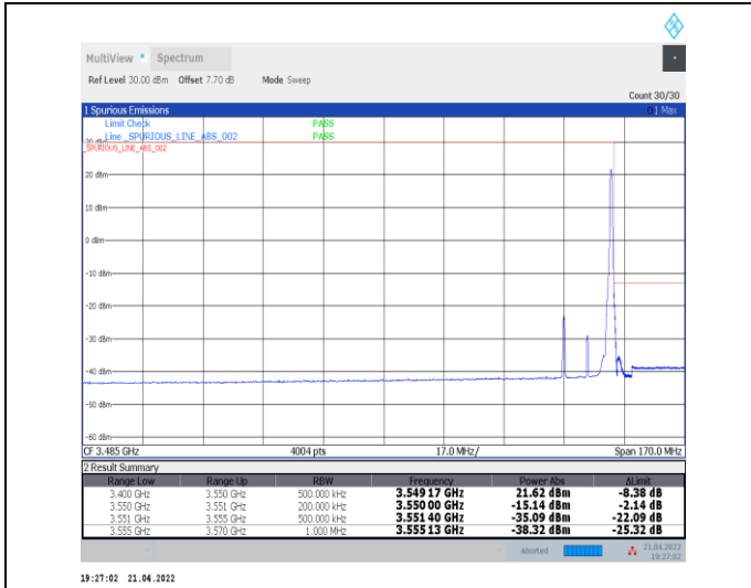
1-N78-3450-3550--30-15-H-2-DFT-PI2BPSK-Edge_1R_B_Right-1@37-Ant0-PASS-see graph
