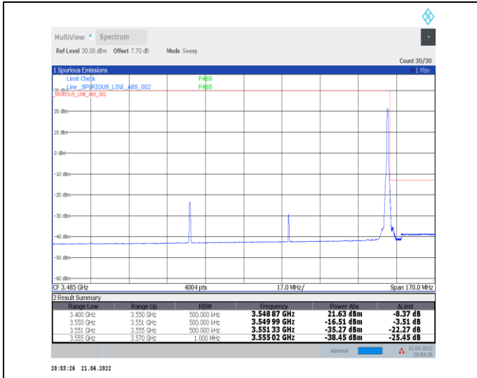
1-N78-3450-3550--30-90-H-2-DFT-PI2BPSK-Edge_1R_B_Right-1@244-Ant0-PASS-see graph
