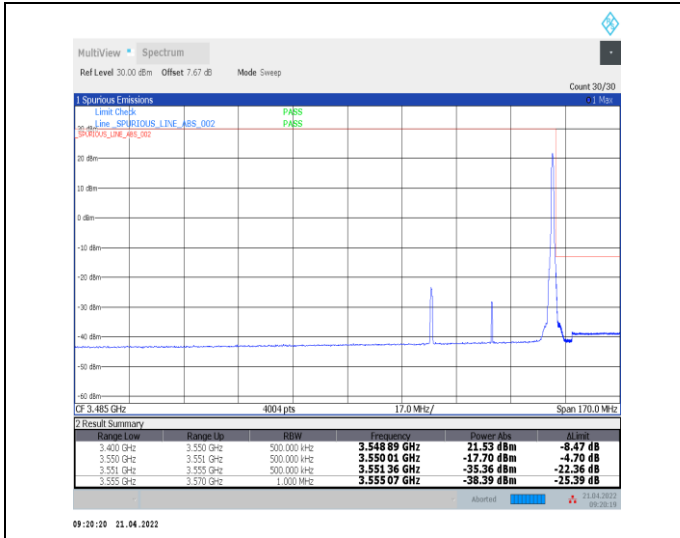
1-N78-3450-3550--30-40-H-2-DFT-PI2BPSK-Edge_1R_B_Right-1@105-Ant0-PASS-see graph
