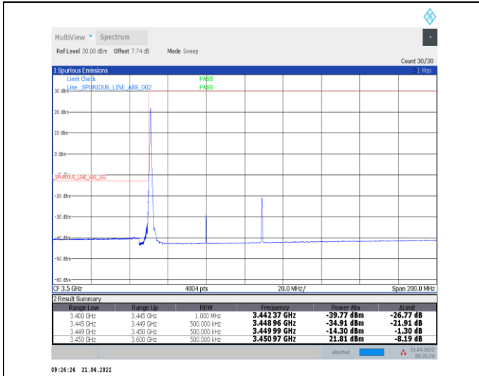
1-N78-3450-3550--30-60-L-1-DFT-PI2BPSK-Edge_1R_B_Left-1@0-Ant0-PASS-see graph
