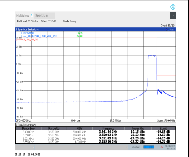
1-N78-3450-3550--30-10-H-6-CP-QPSK-Outer_Fu ll-24@0-Ant0-PASS-see graph
