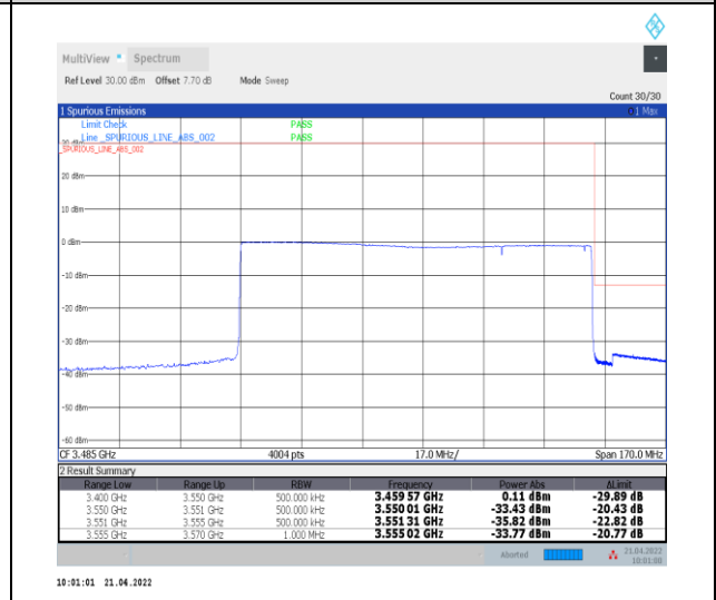
1-N78-3450-3550--30-100-H-6-CP-QPSK-Outer_F ull-273@0-Ant0-PASS-see graph
