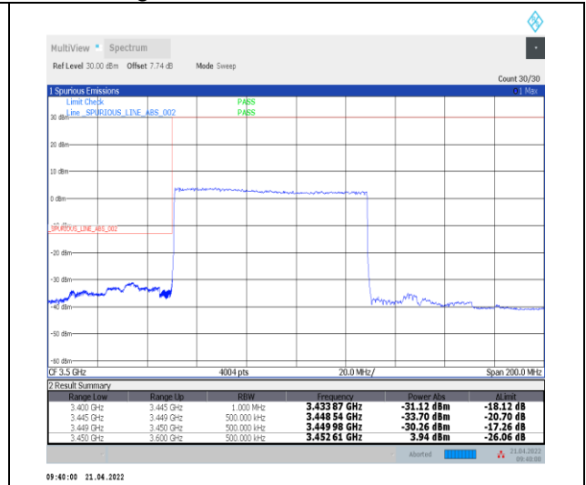
1-N78-3450-3550--30-80-L-3-DFT-PI2BPSK-Outer_Full-216@0-Ant0-PASS-see graph
