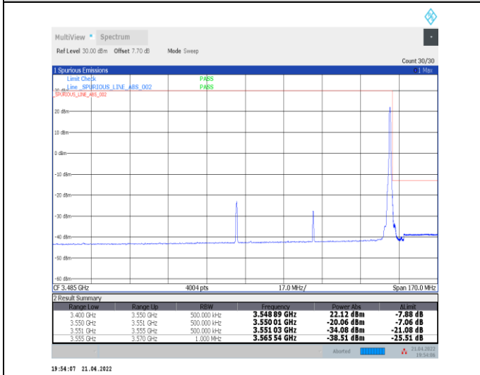
1-N78-3450-3550--30-70-H-5-CP-QPSK-Edge_1RB_Right-1@188-Ant0-PASS-see graph
