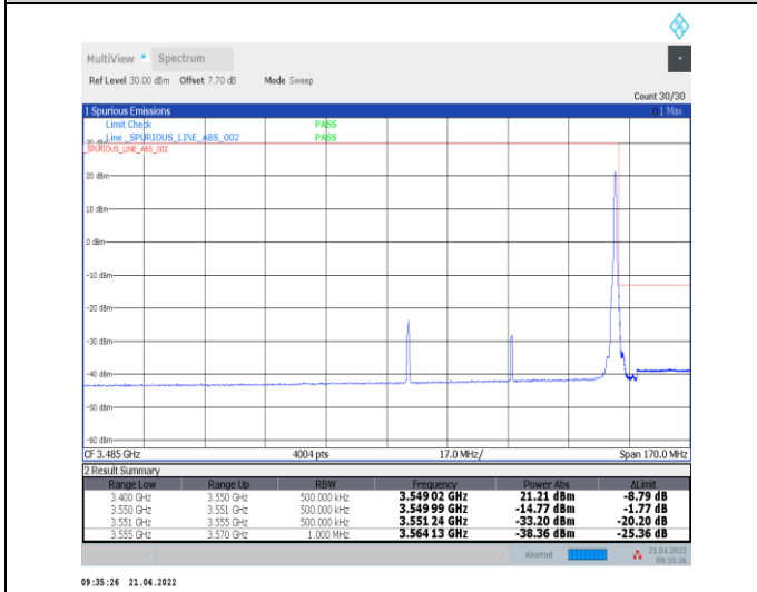
1-N78-3450-3550--30-60-H-5-CP-QPSK-Edge_1RB_R ight-1@161-Ant0-PASS-see graph
