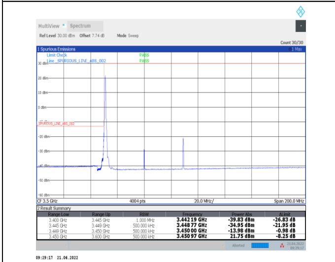
1-N78-3450-3550--30-60-L-4-CP-QPSK-Edge_1RB_L_eff-1@0-Ant0-PASS-see graph
