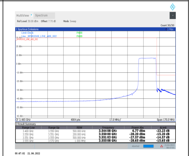
1-N78-3450-3550--30-20-H-6-CP-QPSK-Outer_Fu ll-51@0-Ant0-PASS-see graph
