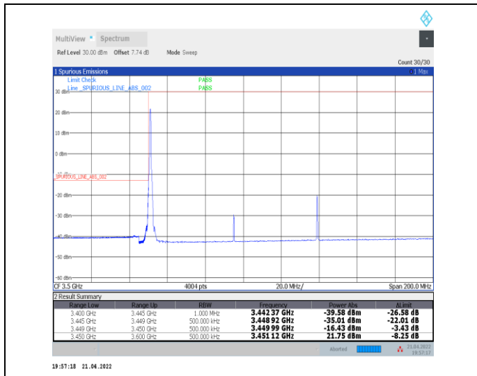
1-N78-3450-3550--30-90-L-1-DFT-PI2BPSK-Edge_1R_B_Left-1@0-Ant0-PASS-see graph
