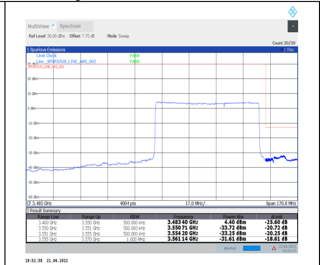
1-N78-3450-3550--30-70-H-3-DFT-PI2BPSK-Outer_Full-180@0-Ant0-PASS-see graph
