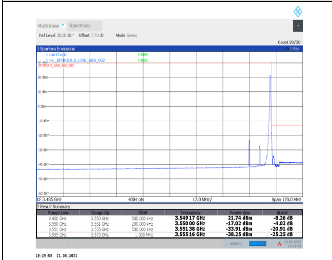
1-N78-3450-3550--30-15-H-5-CP-QPSK-Edge_1RB_R ight-1@37-Ant0-PASS-see graph
