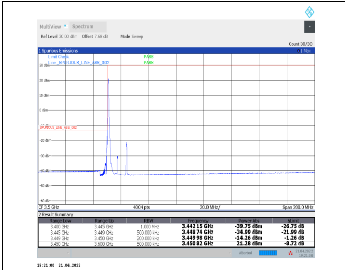
1-N78-3450-3550--30-15-L-1-DFT-PI2BPSK-Edge_1R_B_Left-1@0-Ant0-PASS-see graph
