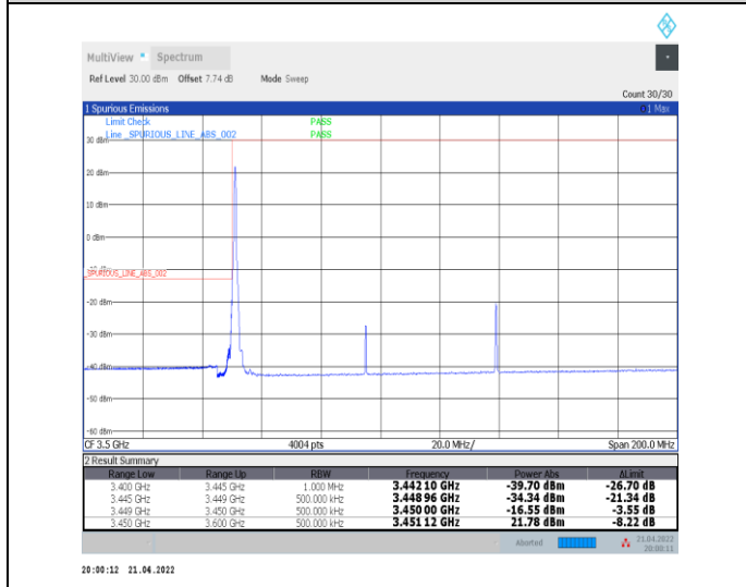
1-N78-3450-3550--30-90-L-4-CP-QPSK-Edge_1RB_L_eff-1@0-Ant0-PASS-see graph
