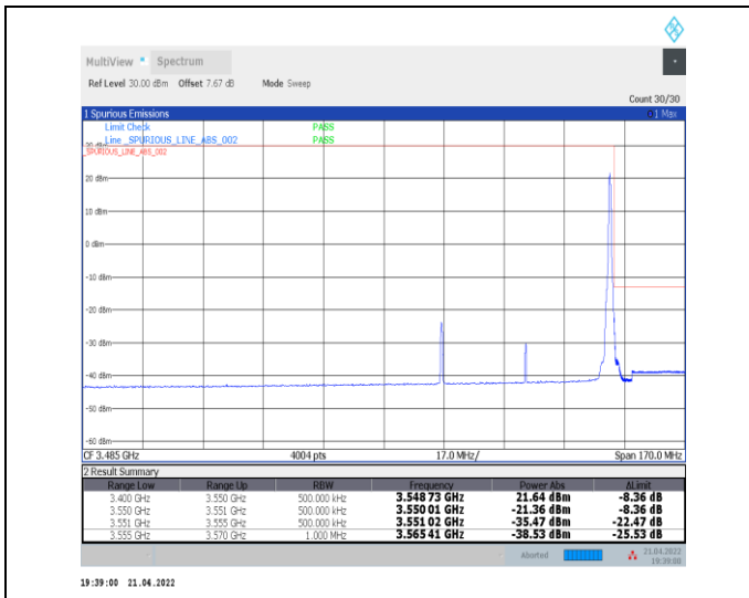
1-N78-3450-3550--30-50-H-2-DFT-PI2BPSK-Edge_1R_B_Right-1@132-Ant0-PASS-see graph
