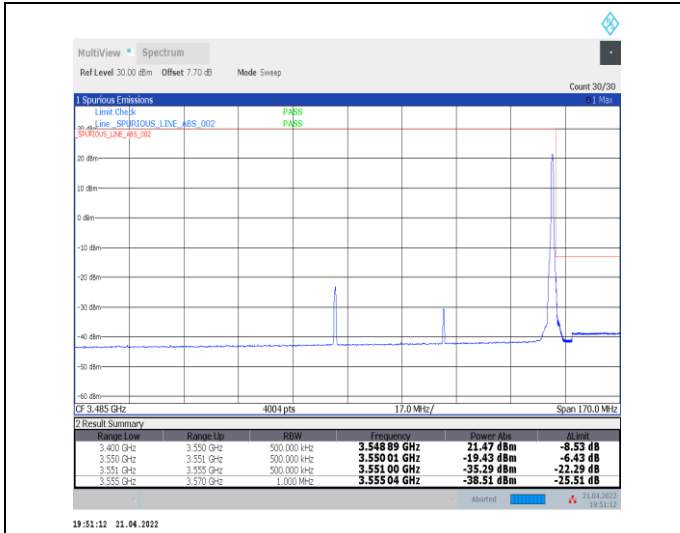
1-N78-3450-3550--30-70-H-2-DFT-PI2BPSK-Edge_1R_B_Right-1@188-Ant0-PASS-see graph
