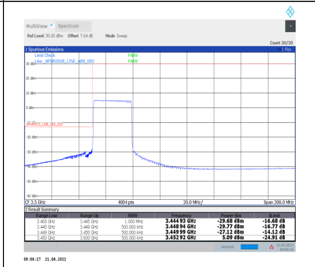
1-N78-3450-3550--30-30-L-6-CP-QPSK-Outer_Ful l-78@0-Ant0-PASS-see graph
