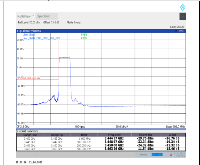
1-N78-3450-3550--30-15-L-3-DFT-PI2BPSK-Outer_Full-36@0-Ant0-PASS-see graph
