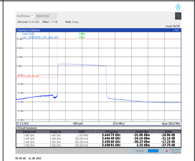
1-N78-3450-3550--30-60-L-6-CP-QPSK-Outer_Ful I-162@0-Ant0-PASS-see graph
