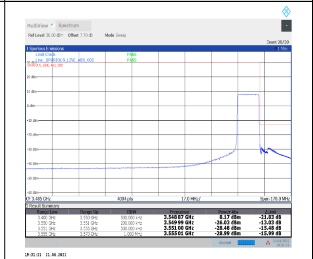
1-N78-3450-3550--30-15-H-6-CP-QPSK-Outer_Fu ll-38@0-Ant0-PASS-see graph
