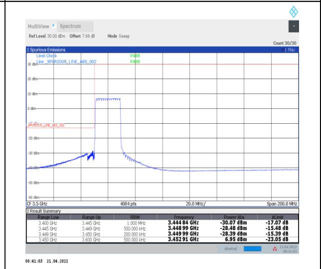
1-N78-3450-3550--30-20-L-6-CP-QPSK-Outer_Ful I-51@0-Ant0-PASS-see graph
