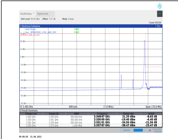
1-N78-3450-3550--30-30-H-2-DFT-PI2BPSK-Edge_1R_B_Right-1@77-Ant0-PASS-see graph
