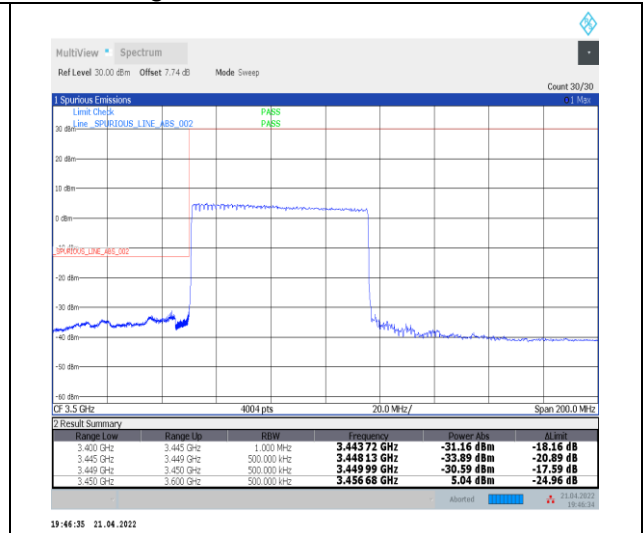
1-N78-3450-3550--30-70-L-3-DFT-PI2BPSK-Outer_Full-180@0-Ant0-PASS-see graph
