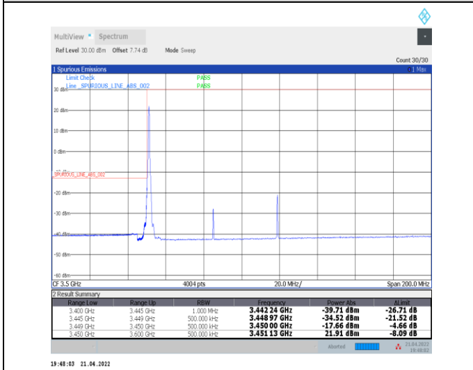
1-N78-3450-3550--30-70-L-4-CP-QPSK-Edge_1RB_L_eff-1@0-Ant0-PASS-see graph
