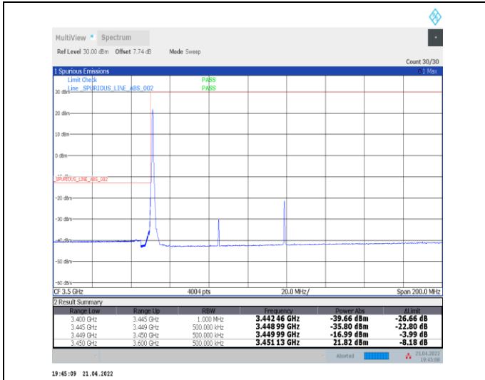
1-N78-3450-3550--30-70-L-1-DFT-PI2BPSK-Edge_1R_B_Left-1@0-Ant0-PASS-see graph
