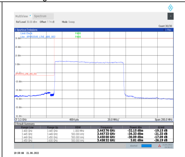
1-N78-3450-3550--30-90-L-3-DFT-PI2BPSK-Outer_Full-240@0-Ant0-PASS-see graph
