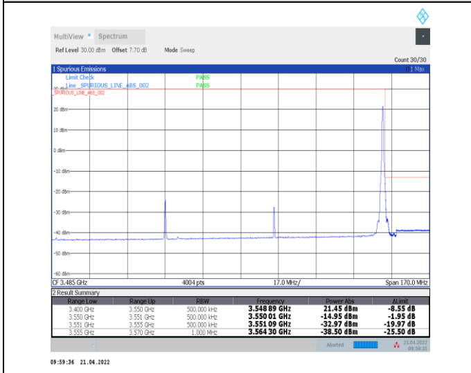
1-N78-3450-3550--30-100-H-5-CP-QPSK-Edge_1RB_Right-1@272-Ant0-PASS-see graph
