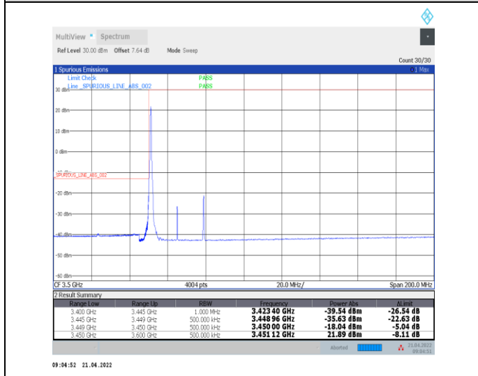
1-N78-3450-3550--30-30-L-4-CP-QPSK-Edge_1RB_L_eft-1@0-Ant0-PASS-see graph
