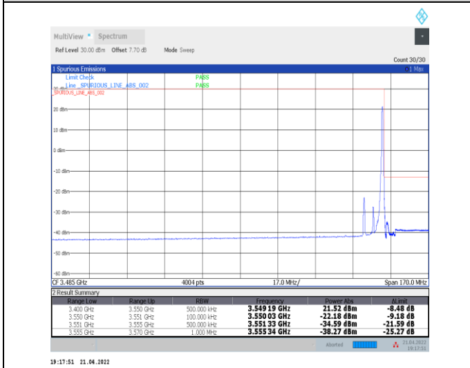
1-N78-3450-3550--30-10-H-5-CP-QPSK-Edge_1RB_R ight-1@23-Ant0-PASS-see graph
