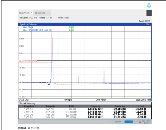
1-N78-3450-3550--30-80-L-4-CP-QPSK-Edge_1RB_L_eff-1@0-Ant0-PASS-see graph
