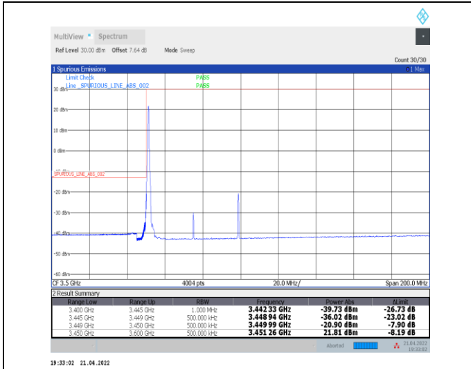
1-N78-3450-3550--30-50-L-1-DFT-PI2BPSK-Edge_1R_B_Left-1@0-Ant0-PASS-see graph
