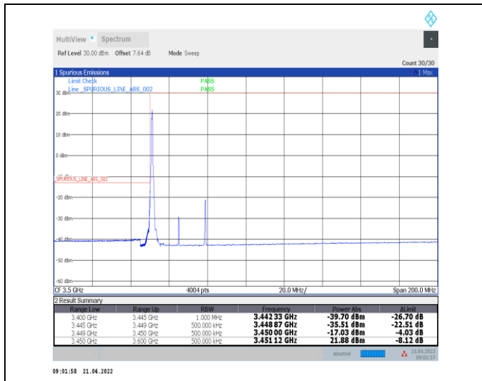
1-N78-3450-3550--30-30-L-1-DFT-PI2BPSK-Edge_1R_B_Left-1@0-Ant0-PASS-see graph
