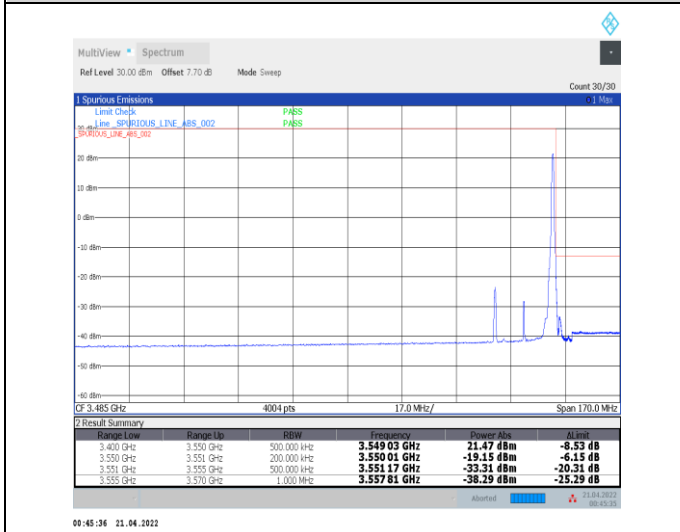
1-N78-3450-3550--30-20-H-5-CP-QPSK-Edge_1RB_R ight-1@50-Ant0-PASS-see graph
