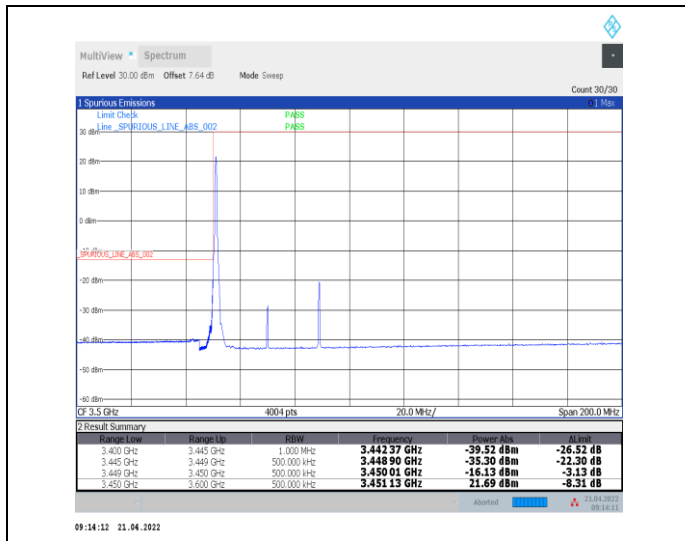
1-N78-3450-3550--30-40-L-1-DFT-PI2BPSK-Edge_1R_B_Left-1@0-Ant0-PASS-see graph
