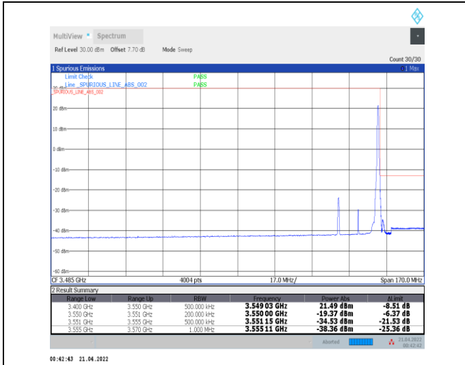
1-N78-3450-3550--30-20-H-2-DFT-PI2BPSK-Edge_1R_B_Right-1@50-Ant0-PASS-see graph
