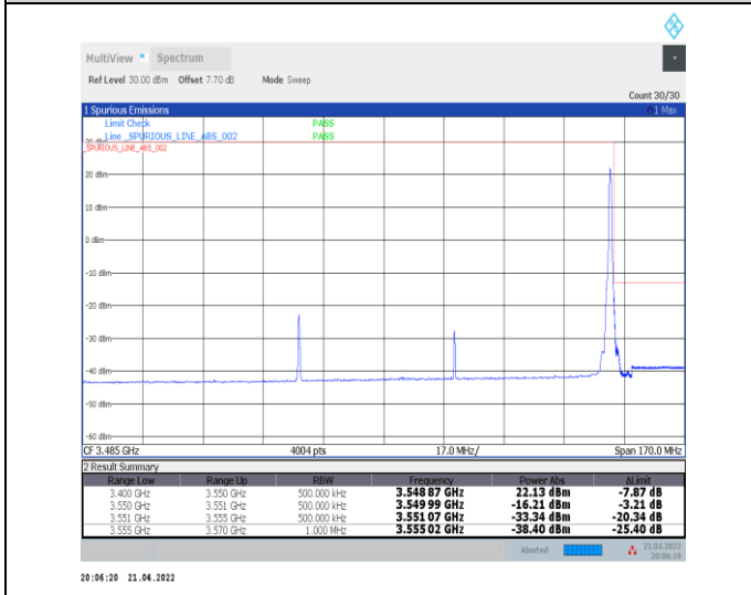
1-N78-3450-3550--30-90-H-5-CP-QPSK-Edge_1RB_R ight-1@244-Ant0-PASS-see graph
