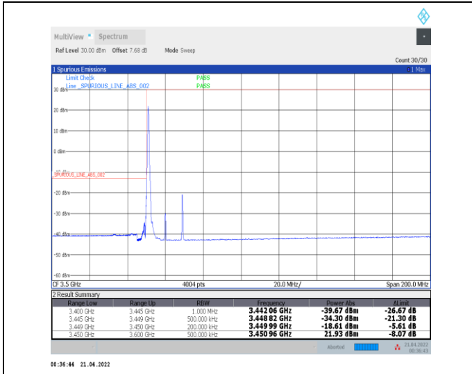
1-N78-3450-3550--30-20-L-1-DFT-PI2BPSK-Edge_1R_B_Left-1@0-Ant0-PASS-see graph
