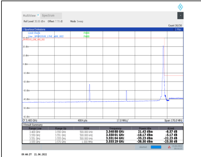
1-N78-3450-3550--30-80-H-2-DFT-PI2BPSK-Edge_1R_B_Right-1@216-Ant0-PASS-see graph
