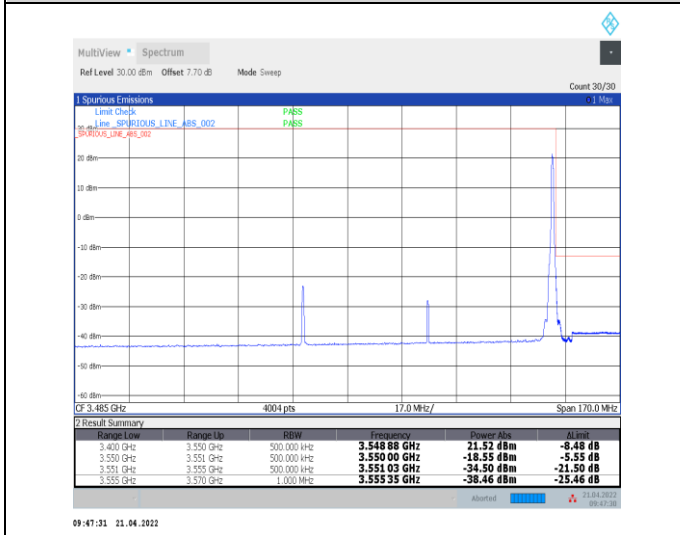
1-N78-3450-3550--30-80-H-5-CP-QPSK-Edge_1RB_Right-1@216-Ant0-PASS-see graph
