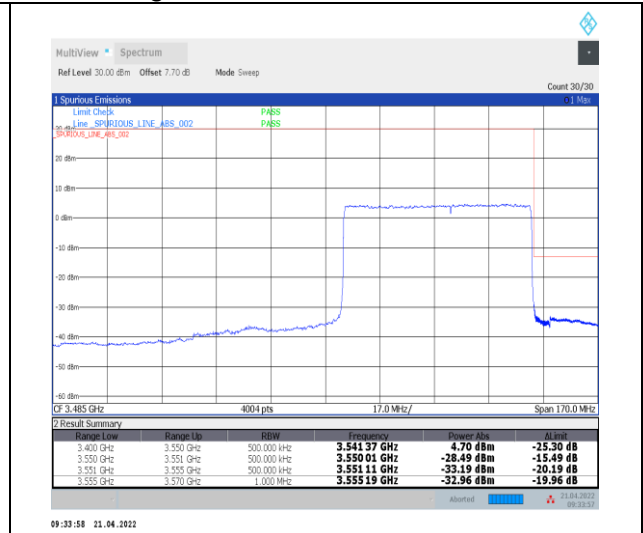
1-N78-3450-3550--30-60-H-3-DFT-PI2BPSK-Outer_Full-162@0-Ant0-PASS-see graph
