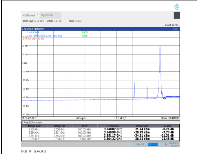
1-N78-3450-3550--30-30-H-5-CP-QPSK-Edge_1RB_R ight-1@77-Ant0-PASS-see graph
