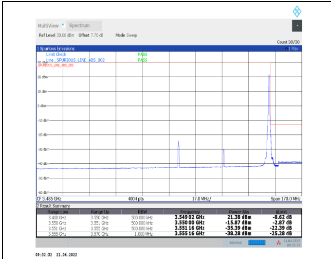
1-N78-3450-3550--30-60-H-2-DFT-PI2BPSK-Edge_1R_B_Right-1@161-Ant0-PASS-see graph
