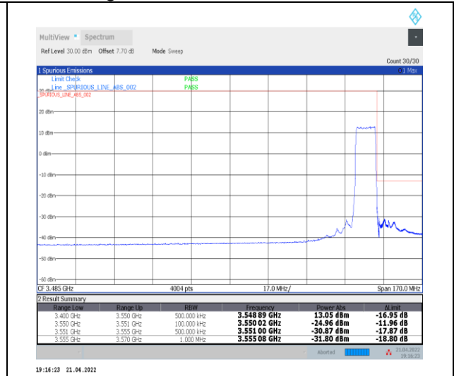
1-N78-3450-3550--30-10-H-3-DFT-PI2BPSK-Outer_Full-24@0-Ant0-PASS-see graph
