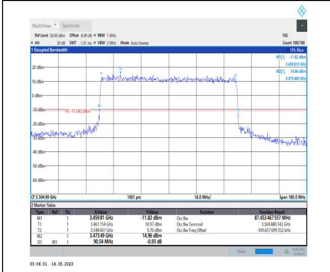
1-N78-3450-3550-PC1-30-90-H-6-CP-QPSK-Outer_Full-245@0-Ant0-87.453-90.540-≤90-PASS
