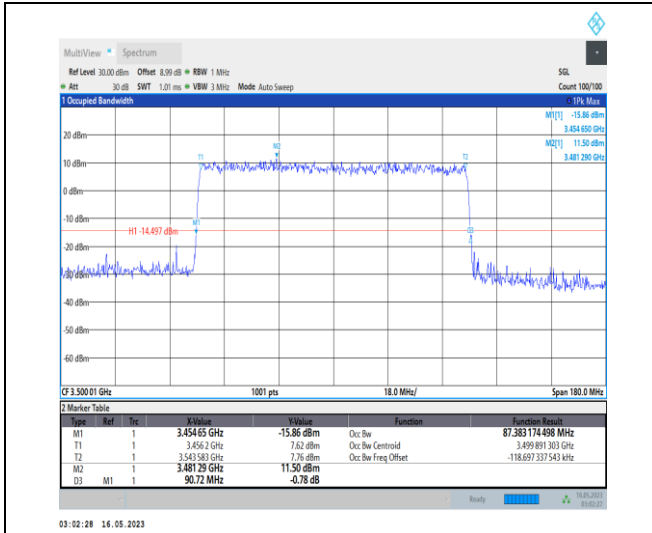
1-N78-3450-3550-PC1-30-90-M-9-CP-256QAM-Out er_Full-245@0-Ant0-87.383-90.720-≤90-PASS
