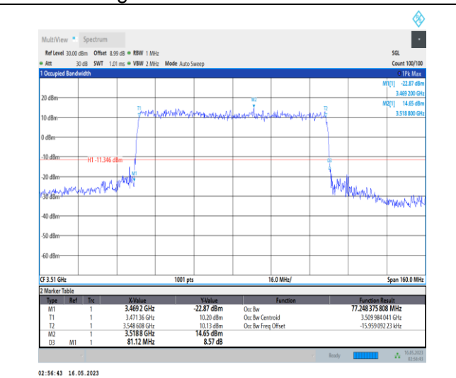
1-N78-3450-3550-PC1-30-80-H-8-CP-64QAM-Outer _Full-217@0-Ant0-77.248-81.120-≤80-PASS
