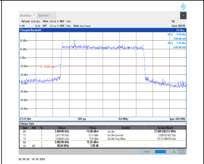
1-N78-3450-3550-PC1-30-80-H-6-CP-QPSK-Outer_Full-217@0-Ant0-77.47-80.640-≤80-PASS
