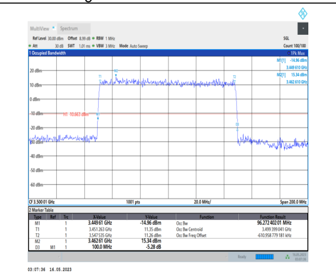
1-N78-3450-3550-PC1-30-100-L-4-DFT-64QAM-Out er_Full-270@0-Ant0-96.272-100.000-≤100-PASS
