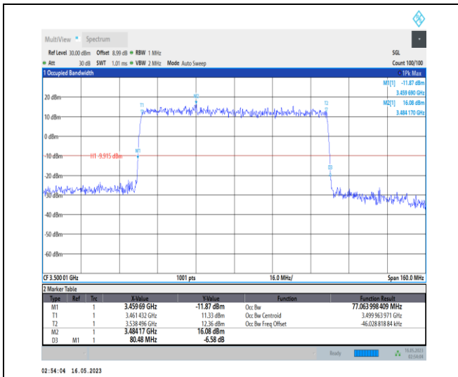
1-N78-3450-3550-PC1-30-80-M-4-DFT-64QAM-Out_er_Full-216@0-Ant0-77.064-80.480-≤80-PASS
