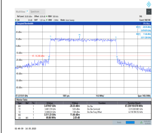
1-N78-3450-3550-PC1-30-70-H-8-CP-64QAM-Outer_Full-189@0-Ant0-67.259-69.860-≤70-PASS
