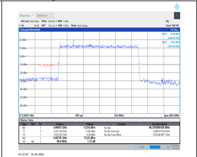
1-N78-3450-3550-PC1-30-100-M-3-DFT-16QAM-Outer_Full-270@0-Ant0-96.378-99.800-≤100-PASS
