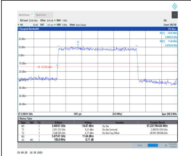
1-N78-3450-3550-PC1-30-100-L-9-CP-256QAM-Outer_Full-273@0-Ant0-97.236-100.800-≤100-PASS
