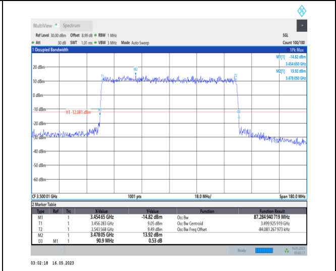
1-N78-3450-3550-PC1-30-90-M-8-CP-64QAM-Outer_Full-245@0-Ant0-87.285-90.900-≤90-PASS
