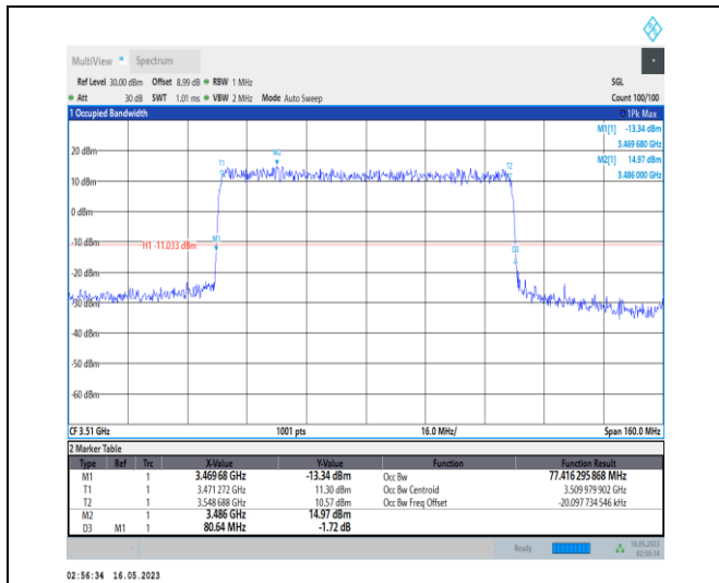
1-N78-3450-3550-PC1-30-80-H-7-CP-16QAM-Outer _Full-217@0-Ant0-77.416-80.640-≤80-PASS
