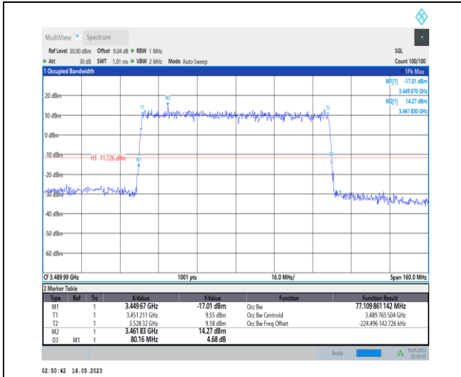
1-N78-3450-3550-PC1-30-80-L-5-DFT-256QAM-Out_er_Full-216@0-Ant0-77.11-80.160-<math>\leq 80</math>-PASS
