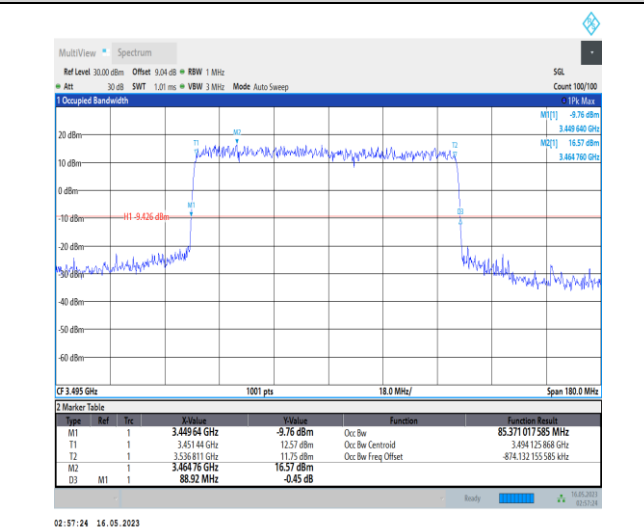
1-N78-3450-3550-PC1-30-90-L-1-DFT-QPSK-Outer Full-240@0-Ant0-85.371-88.920-≤90-PASS
