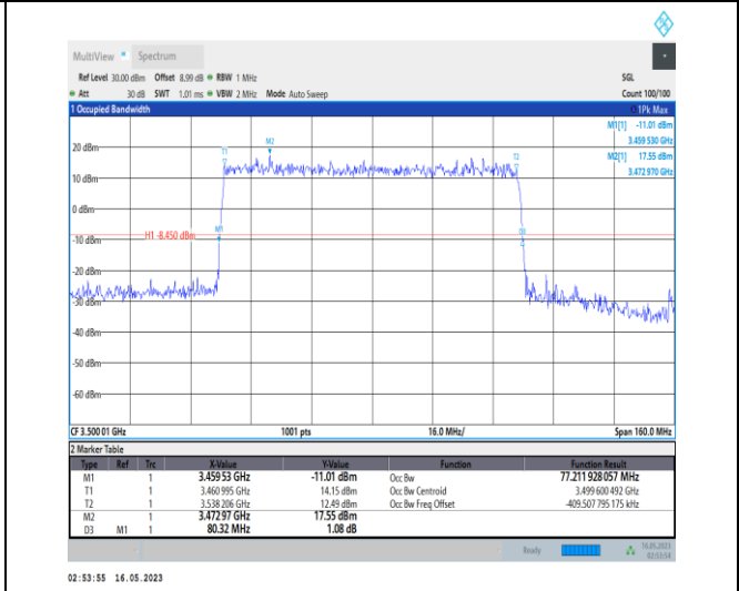
1-N78-3450-3550-PC1-30-80-M-3-DFT-16QAM-Outer_Full-216@0-Ant0-77.212-80.320-≤80-PASS
