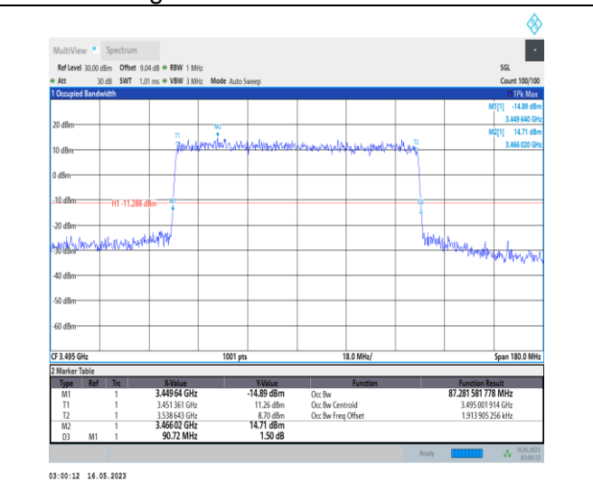
1-N78-3450-3550-PC1-30-90-L-7-CP-16QAM-Outer_Full-245@0-Ant0-87.282-90.720-<math>\leq 90</math>-PASS
