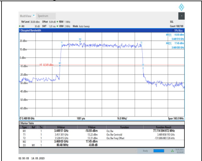
1-N78-3450-3550-PC1-30-80-L-2-DFT-PI2BPSK-Out_er_Full-216@0-Ant0-77.115-80.480-≤80-PASS
