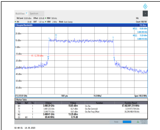
1-N78-3450-3550-PC1-30-70-H-6-CP-QPSK-Outer_Full-189@0-Ant0-67.483-69.440-≤70-PASS
