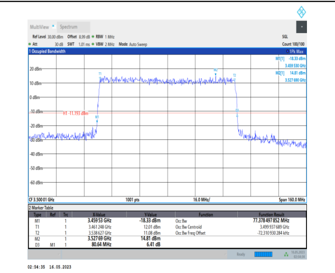
1-N78-3450-3550-PC1-30-80-M-7-CP-16QAM-Outer_Full-217@0-Ant0-77.378-80.640-≤80-PASS
