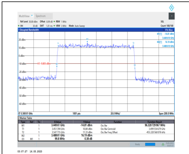
1-N78-3450-3550-PC1-30-100-L-3-DFT-16QAM-Out er_Full-270@0-Ant0-96.321-99.800-≤100-PASS
