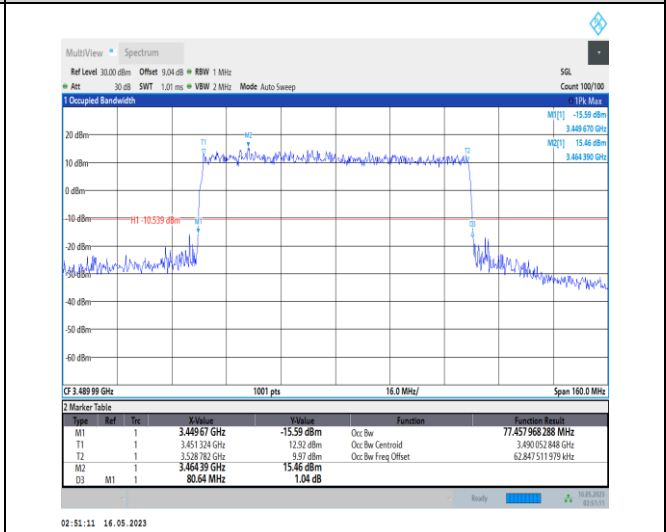
1-N78-3450-3550-PC1-30-80-L-8-CP-64QAM-Outer_Full-217@0-Ant0-77.458-80.640-<math>\leq 80</math>-PASS
