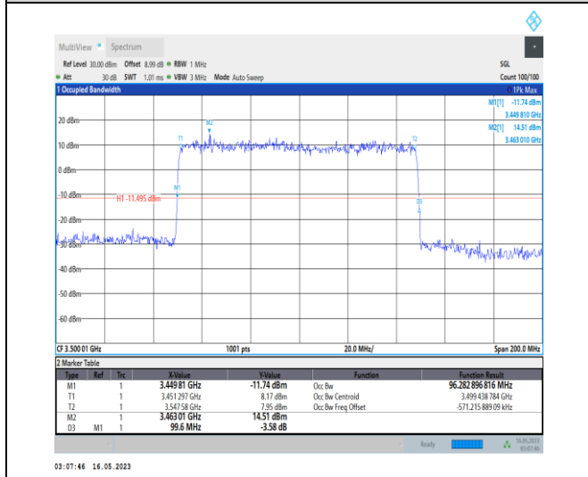
1-N78-3450-3550-PC1-30-100-L-5-DFT-256QAM-Out er_Full-270@0-Ant0-96.283-99.600-≤100-PASS
