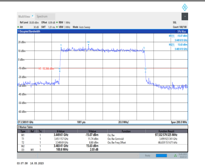
1-N78-3450-3550-PC1-30-100-L-6-CP-QPSK-Outer Full-273@0-Ant0-97.533-100.800-≤100-PASS
