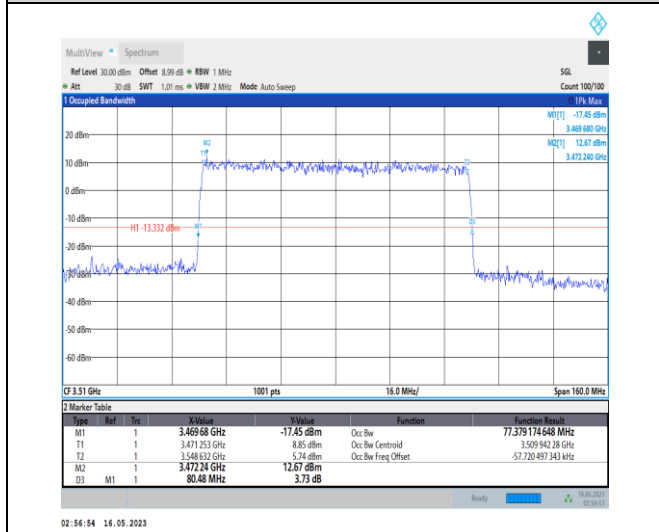
1-N78-3450-3550-PC1-30-80-H-9-CP-256QAM-Outer _Full-217@0-Ant0-77.379-80.480-≤80-PASS
