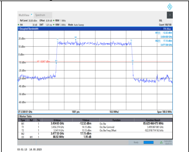
1-N78-3450-3550-PC1-30-90-M-2-DFT-PI2BPSK-Outer_Full-240@0-Ant0-85.625-88.920-≤90-PASS
