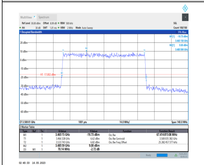
1-N78-3450-3550-PC1-30-70-M-9-CP-256QAM-Outer_Full-189@0-Ant0-67.415-70.140-≤70-PASS
