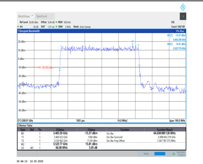
1-N78-3450-3550-PC1-30-70-M-2-DFT-PI2BPSK-Outer _Full-180@0-Ant0-64.039-66.080-≤70-PASS
