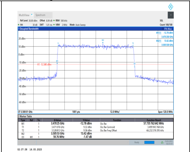
1-N78-3450-3550-PC1-30-60-M-7-CP-16QAM-Outer_Full-162@0-Ant0-57.736-59.760-≤60-PASS
