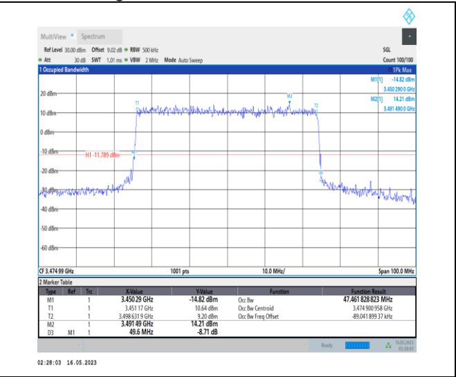
1-N78-3450-3550-PC1-30-50-L-7-CP-16QAM-Outer_Full-133@0-Ant0-47.462-49.600-≤50-PASS
