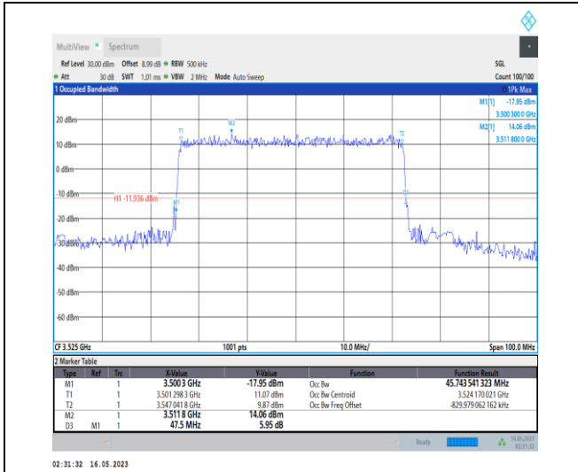
1-N78-3450-3550-PC1-30-50-H-4-DFT-64QAM-Outer_Full-128@0-Ant0-45.744-47.500-≤50-PASS
