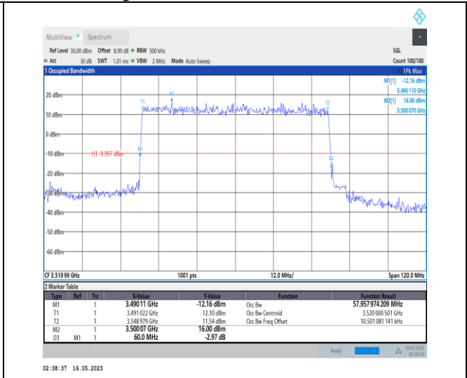
1-N78-3450-3550-PC1-30-60-H-2-DFT-PI2BPSK-Outer_Full-162@0-Ant0-57.958-60.000-≤60-PASS
