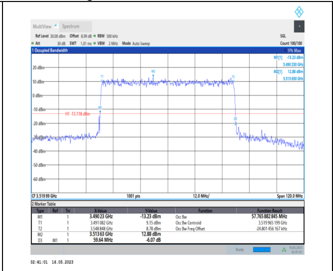
1-N78-3450-3550-PC1-30-60-H-6-CP-QPSK-Outer Full-162@0-Ant0-57.766-59.640-≤60-PASS
