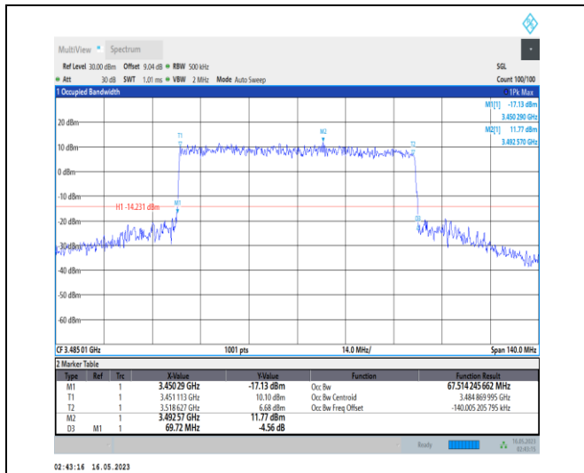
1-N78-3450-3550-PC1-30-70-L-8-CP-64QAM-Outer _Full-189@0-Ant0-67.514-69.720-≤70-PASS
