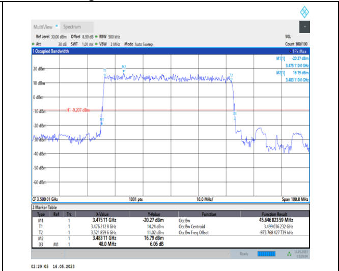
1-N78-3450-3550-PC1-30-50-M-2-DFT-PI2BPSK-Outer_Full-128@0-Ant0-45.647-48.000-≤50-PASS
