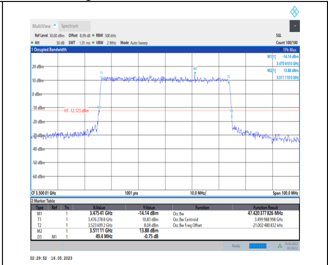
1-N78-3450-3550-PC1-30-50-M-6-CP-QPSK-Outer_Full-133@0-Ant0-47.42-49.400-≤50-PASS
