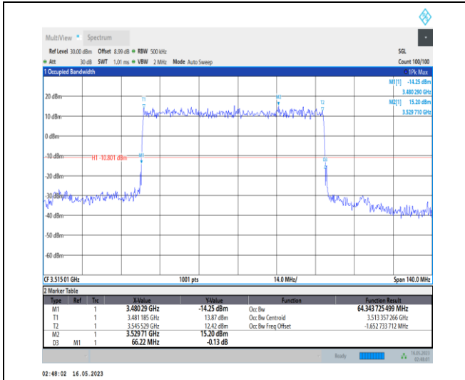
1-N78-3450-3550-PC1-30-70-H-2-DFT-PI2BPSK-Outer_Full-180@0-Ant0-64.344-66.220-≤70-PASS
