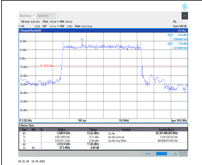
1-N78-3450-3550-PC1-30-50-H-2-DFT-PI2BPSK-Outer _Full-128@0-Ant0-45.761-47.500-≤50-PASS
