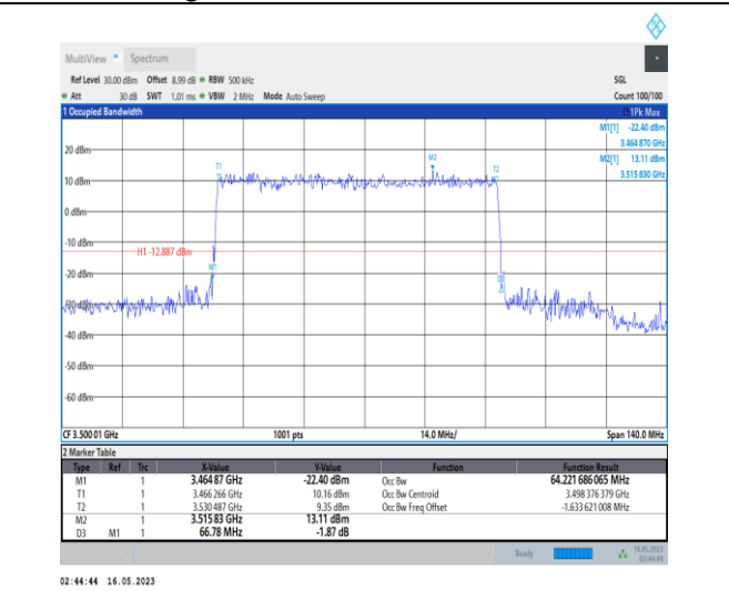
1-N78-3450-3550-PC1-30-70-M-4-DFT-64QAM-Out_r_Full-180@0-Ant0-64.222-66.780-≤70-PASS
