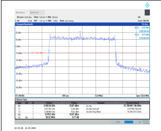
1-N78-3450-3550-PC1-30-60-L-1-DFT-QPSK-Outer_Full-162@0-Ant0-57.79-59.520-<math>\leq 60</math>-PASS
