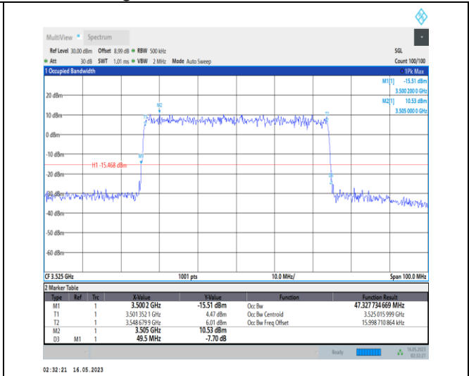
1-N78-3450-3550-PC1-30-50-H-9-CP-256QAM-Outer_Full-133@0-Ant0-47.328-49.500-<math>\leq 50</math>-PASS
