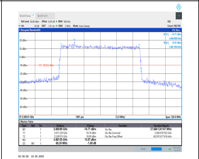
1-N78-3450-3550-PC1-30-60-M-1-DFT-QPSK-Outer_Full-162@0-Ant0-57.684-60.240-≤60-PASS
