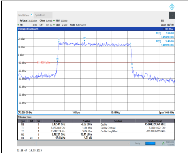
1-N78-3450-3550-PC1-30-50-M-1-DFT-QPSK-Outer_Full-128@0-Ant0-45.604-47.400-≤50-PASS
