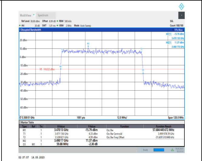
1-N78-3450-3550-PC1-30-60-M-9-CP-256QAM-Outer_Full-162@0-Ant0-57.684-59.880-≤60-PASS
