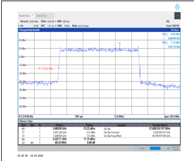
1-N78-3450-3550-PC1-30-60-H-5-DFT-256QAM-Out er_Full-162@0-Ant0-57.609-60.240-≤60-PASS
