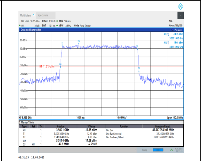
1-N78-3450-3550-PC1-30-50-H-3-DFT-16QAM-Outer _Full-128@0-Ant0-45.548-47.800-≤50-PASS
