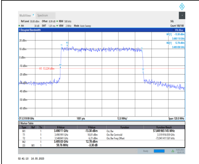
1-N78-3450-3550-PC1-30-60-H-7-CP-16QAM-Outer _Full-162@0-Ant0-57.85-59.760-≤60-PASS
