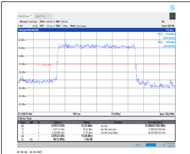
1-N78-3450-3550-PC1-30-60-M-2-DFT-PI2BPSK-Outer_Full-162@0-Ant0-57.699-60.120-≤60-PASS
