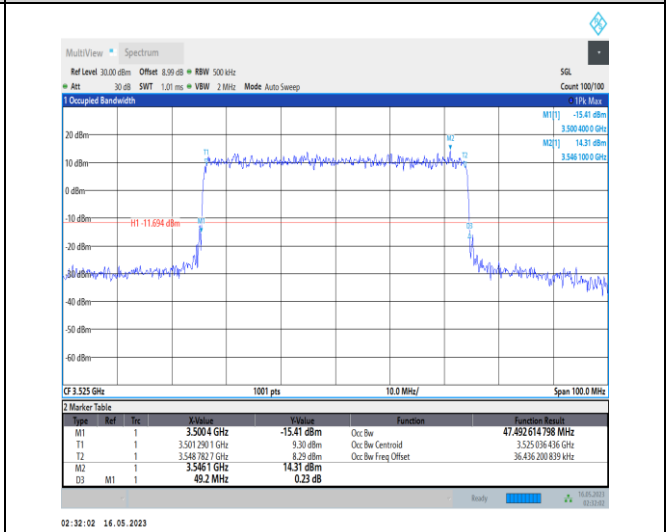
1-N78-3450-3550-PC1-30-50-H-7-CP-16QAM-Outer_Full-133@0-Ant0-47.493-49.200-≤50-PASS
