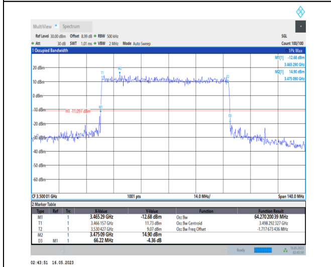
1-N78-3450-3550-PC1-30-70-M-1-DFT-QPSK-Outer _Full-180@0-Ant0-64.27-66.220-≤70-PASS
