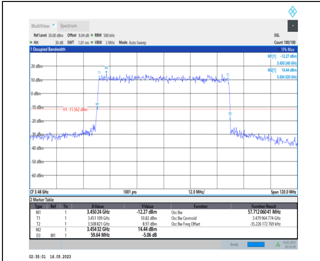
1-N78-3450-3550-PC1-30-60-L-3-DFT-16QAM-Outer_Full-162@0-Ant0-57.712-59.640-≤60-PASS
