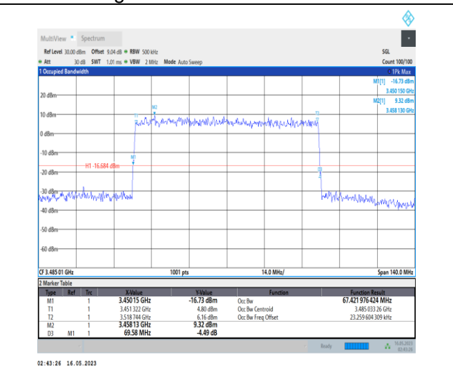
1-N78-3450-3550-PC1-30-70-L-9-CP-256QAM-Outer _Full-189@0-Ant0-67.422-69.580-≤70-PASS
