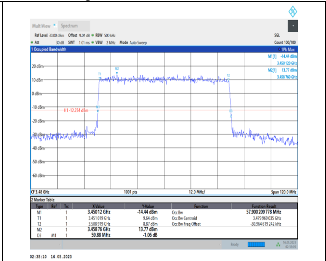
1-N78-3450-3550-PC1-30-60-L-4-DFT-64QAM-Outer_Full-162@0-Ant0-57.9-59.880-≤60-PASS
