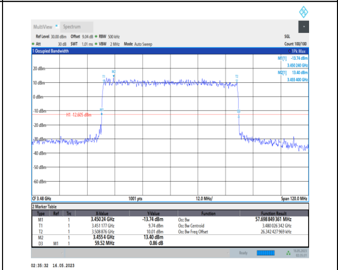
1-N78-3450-3550-PC1-30-60-L-6-CP-QPSK-Outer_Full-162@0-Ant0-57.699-59.520-≤60-PASS
