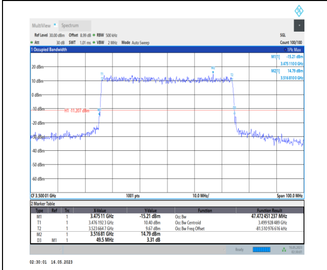
1-N78-3450-3550-PC1-30-50-M-7-CP-16QAM-Outer_Full-133@0-Ant0-47.472-49.500-≤50-PASS
