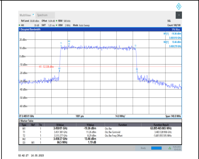
1-N78-3450-3550-PC1-30-70-L-3-DFT-16QAM-Outer_Full-180@0-Ant0-63.895-66.500-≤70-PASS
