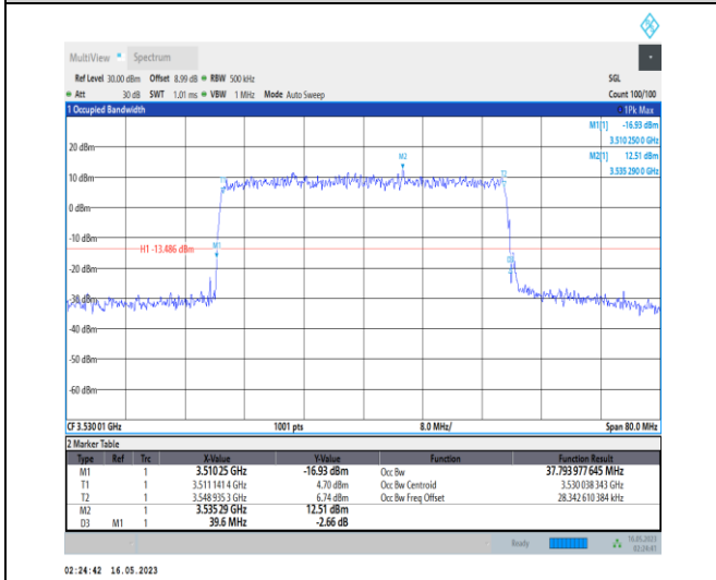
1-N78-3450-3550-PC1-30-40-H-9-CP-256QAM-Outer _Full-106@0-Ant0-37.794-39.600-≤40-PASS
