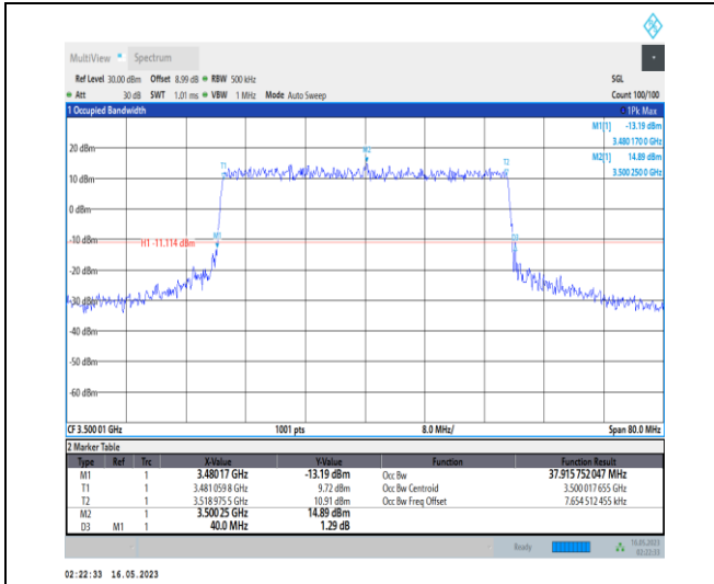
1-N78-3450-3550-PC1-30-40-M-8-CP-64QAM-Outer_Full-106@0-Ant0-37.916-40.000-≤40-PASS
