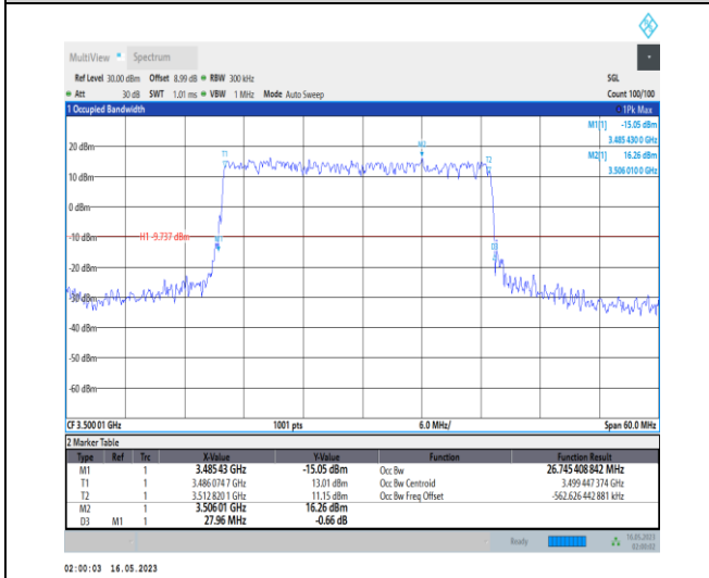
1-N78-3450-3550-PC1-30-30-M-1-DFT-QPSK-Outer _Full-75@0-Ant0-26.745-27.960-≤30-PASS
