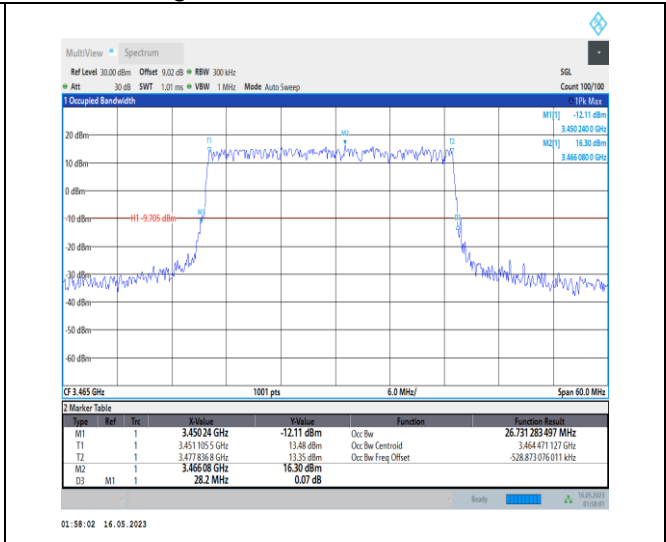
1-N78-3450-3550-PC1-30-30-L-1-DFT-QPSK-Outer_Full-75@0-Ant0-26.731-28.200-≤30-PASS
