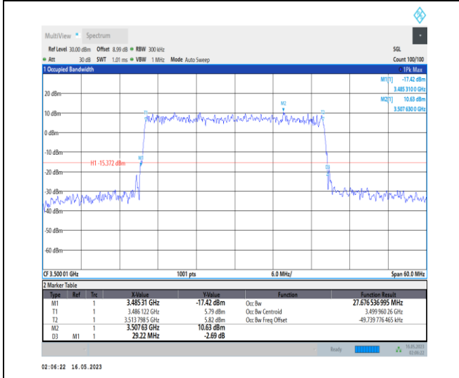
1-N78-3450-3550-PC1-30-30-M-9-CP-256QAM-Outer_Full-78@0-Ant0-27.677-29.220-≤30-PASS
