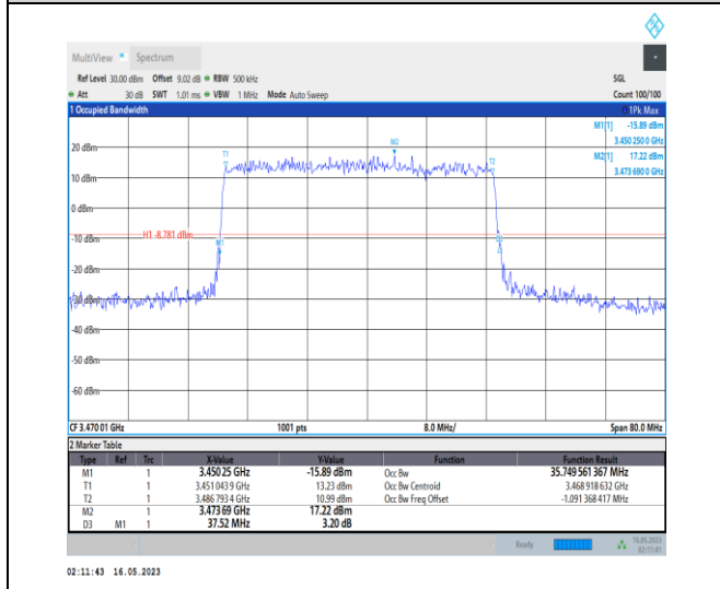
1-N78-3450-3550-PC1-30-40-L-3-DFT-16QAM-Outer_Full-100@0-Ant0-35.75-37.520-≤40-PASS
