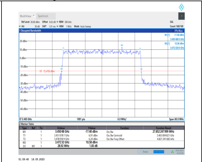
1-N78-3450-3550-PC1-30-30-L-9-CP-256QAM-Outer _Full-78@0-Ant0-27.852-28.920-≤30-PASS
