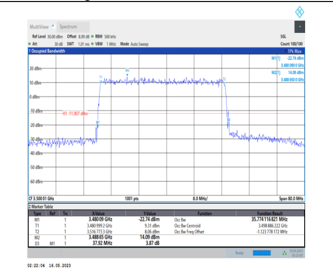
1-N78-3450-3550-PC1-30-40-M-5-DFT-256QAM-Out er_Full-100@0-Ant0-35.774-37.920-≤40-PASS
