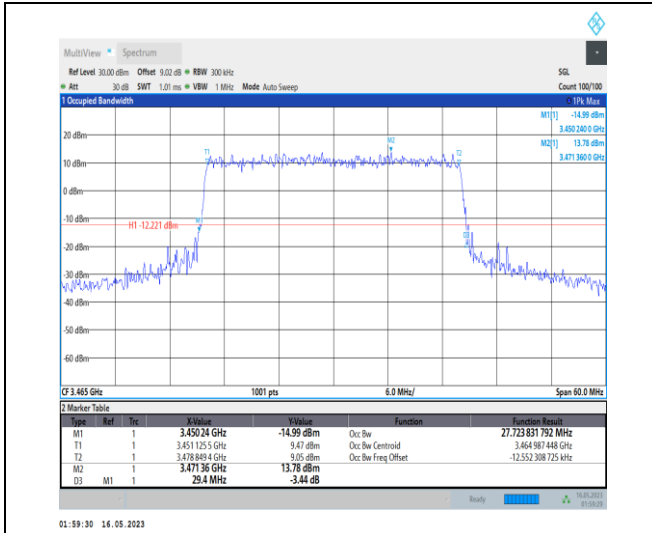
1-N78-3450-3550-PC1-30-30-L-8-CP-64QAM-Outer _Full-78@0-Ant0-27.724-29.400-≤30-PASS
