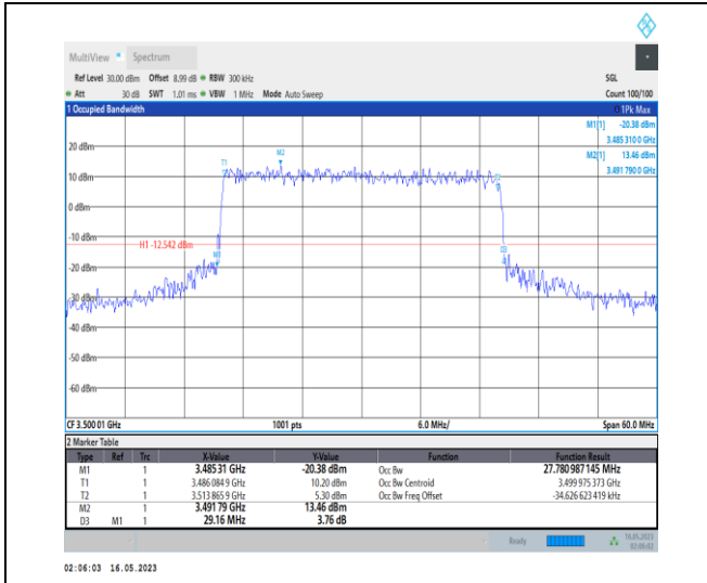
1-N78-3450-3550-PC1-30-30-M-7-CP-16QAM-Outer_Full-78@0-Ant0-27.781-29.160-≤30-PASS
