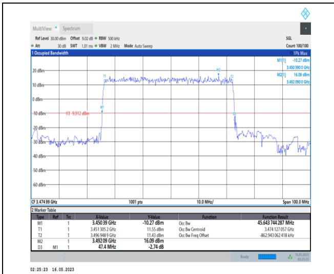
1-N78-3450-3550-PC1-30-50-L-2-DFT-PI2BPSK-Out er_Full-128@0-Ant0-45.644-47.400-≤50-PASS
