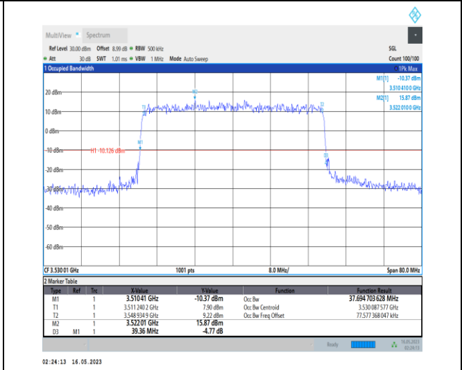
1-N78-3450-3550-PC1-30-40-H-6-CP-QPSK-Outer_Full-106@0-Ant0-37.695-39.360-≤40-PASS
