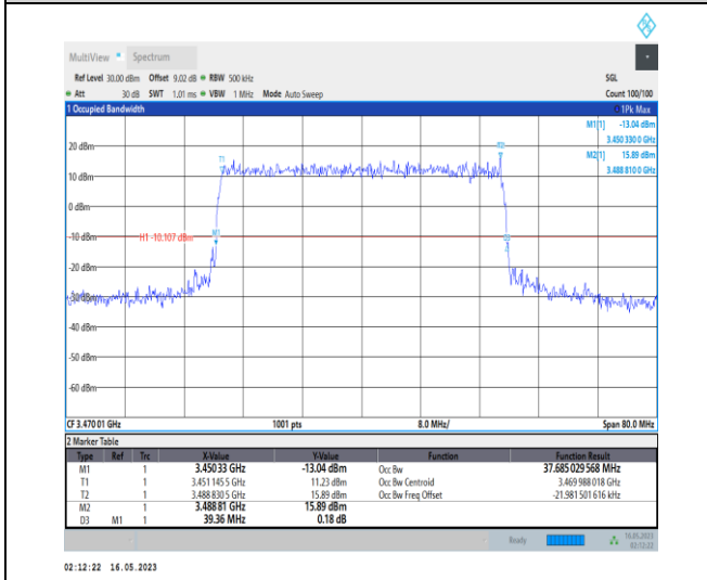
1-N78-3450-3550-PC1-30-40-L-7-CP-16QAM-Outer_Full-106@0-Ant0-37.685-39.360-≤40-PASS
