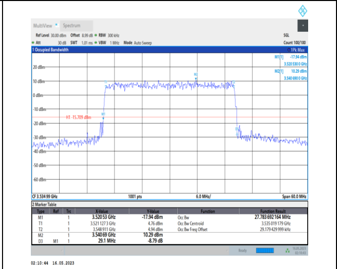
1-N78-3450-3550-PC1-30-30-H-9-CP-256QAM-Outer_Full-78@0-Ant0-27.784-29.100-≤30-PASS
