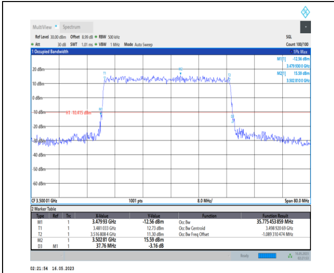
1-N78-3450-3550-PC1-30-40-M-4-DFT-64QAM-Out er_Full-100@0-Ant0-35.775-37.760-≤40-PASS
