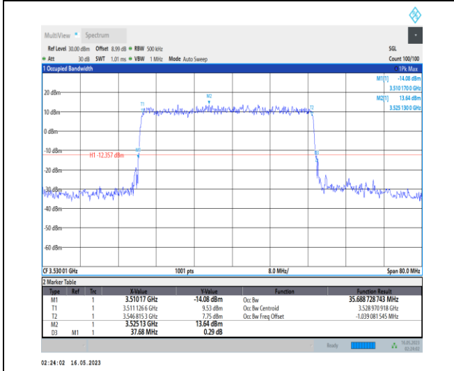
1-N78-3450-3550-PC1-30-40-H-5-DFT-256QAM-Outer_Full-100@0-Ant0-35.689-37.680-≤40-PASS
