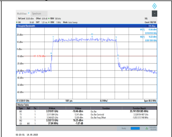
1-N78-3450-3550-PC1-30-40-H-4-DFT-64QAM-Outer_Full-100@0-Ant0-35.741-37.840-≤40-PASS
