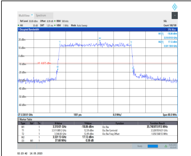
1-N78-3450-3550-PC1-30-40-H-3-DFT-16QAM-Outer_Full-100@0-Ant0-35.741-37.680-≤40-PASS
