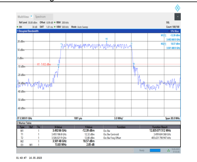
1-N78-3450-3550-PC1-30-15-M-2-DFT-PI2BPSK-Outer_Full-36@0-Ant0-12.835-13.830-≤15-PASS
