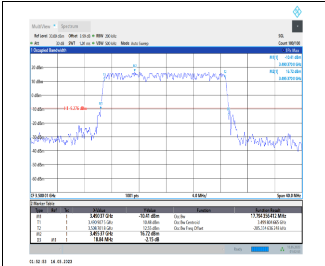
1-N78-3450-3550-PC1-30-20-M-2-DFT-PI2BPSK-Outer_Full-50@0-Ant0-17.794-18.840-≤20-PASS
