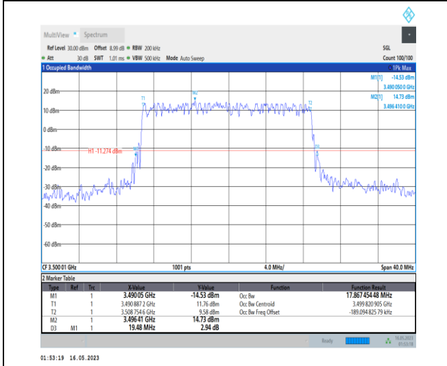
1-N78-3450-3550-PC1-30-20-M-4-DFT-64QAM-Outer_Full-50@0-Ant0-17.867-19.480-≤20-PASS
