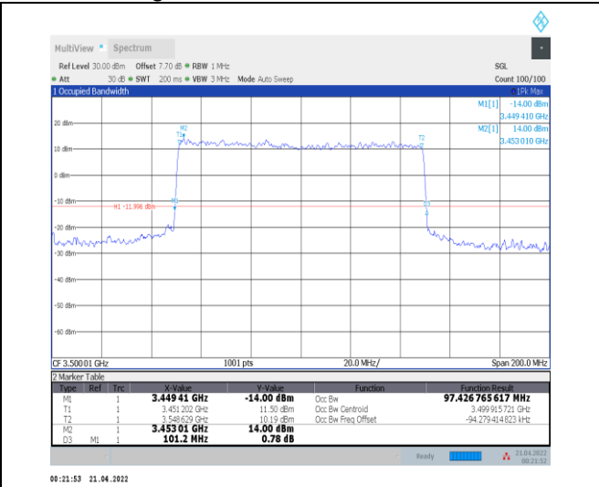
1-N78-3450-3550--30-100-H-6-CP-QPSK-Outer_Full-273@0-Ant0-97.427-101.200-≤100-PASS
