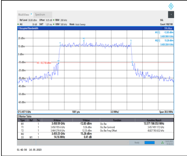
1-N78-3450-3550-PC1-30-15-L-8-CP-64QAM-Outer _Full-38@0-Ant0-13.571-14.160-≤15-PASS
