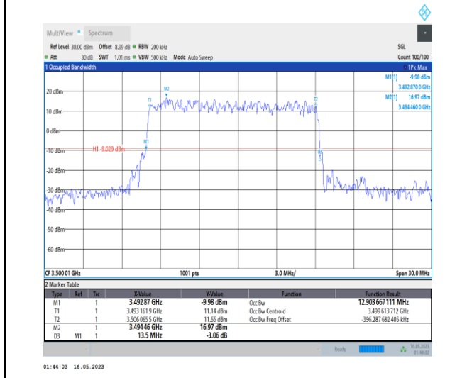
1-N78-3450-3550-PC1-30-15-M-3-DFT-16QAM-Outer_Full-36@0-Ant0-12.904-13.500-≤15-PASS
