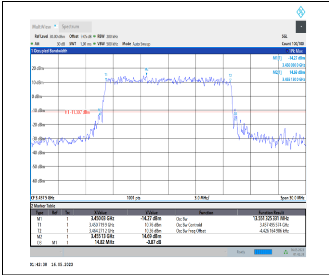
1-N78-3450-3550-PC1-30-15-L-6-CP-QPSK-Outer _Full-38@0-Ant0-13.551-14.820-≤15-PASS
