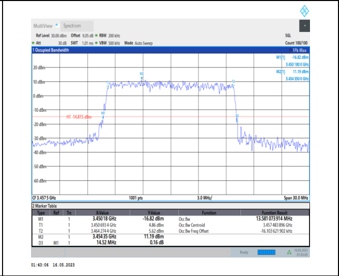
1-N78-3450-3550-PC1-30-15-L-9-CP-256QAM-Outer _Full-38@0-Ant0-13.581-14.520-≤15-PASS
