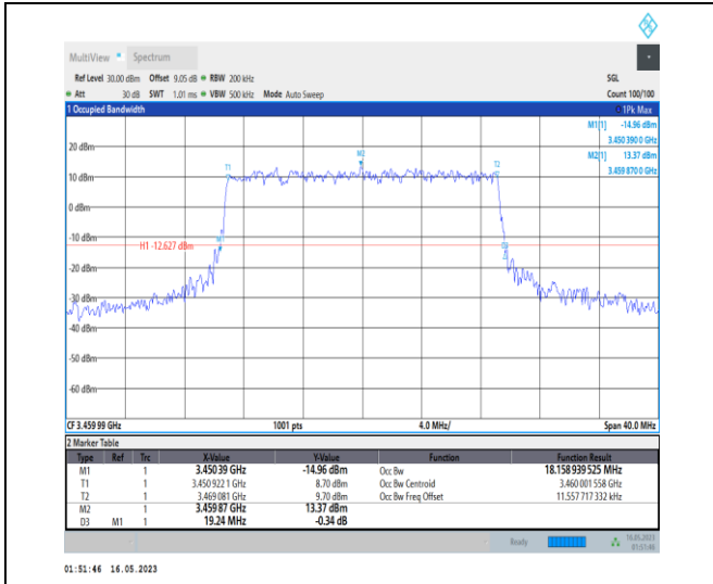
1-N78-3450-3550-PC1-30-20-L-7-CP-16QAM-Outer_Full-51@0-Ant0-18.159-19.240-≤20-PASS
