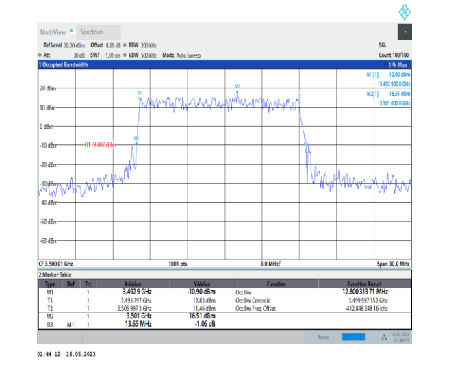
1-N78-3450-3550-PC1-30-15-M-4-DFT-64QAM-Outer_Full-36@0-Ant0-12.8-13.650-≤15-PASS
