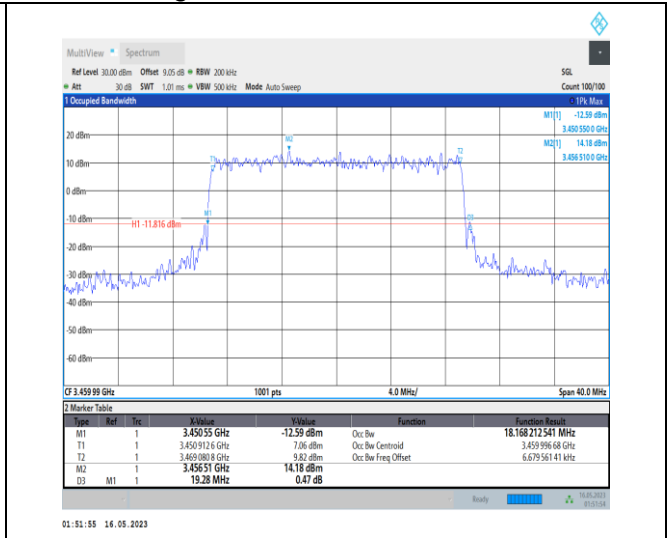
1-N78-3450-3550-PC1-30-20-L-8-CP-64QAM-Outer_Full-51@0-Ant0-18.168-19.280-≤20-PASS
