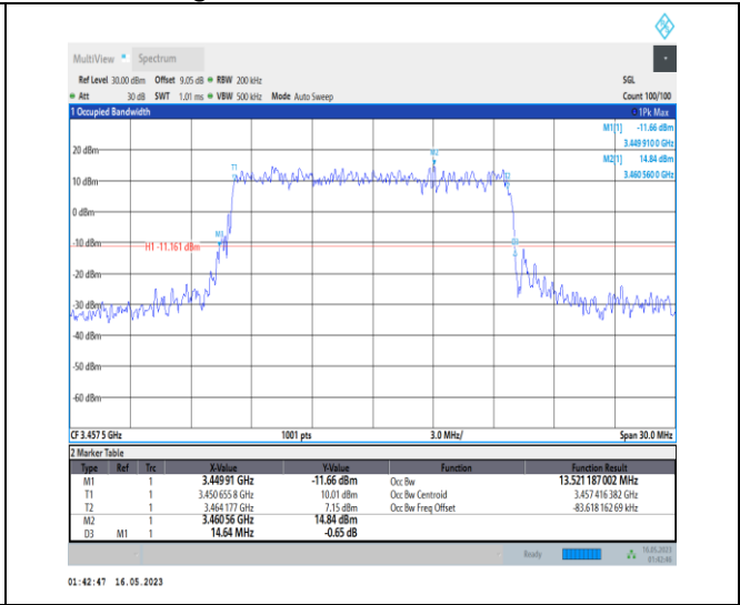
1-N78-3450-3550-PC1-30-15-L-7-CP-16QAM-Outer _Full-38@0-Ant0-13.521-14.640-≤15-PASS
