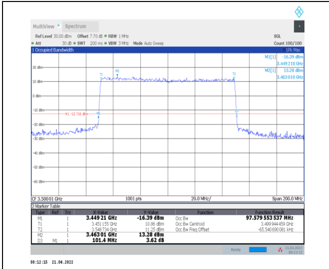
1-N78-3450-3550--30-100-L-7-CP-16QAM-Outer_Fu II-273@0-Ant0-97.58-101.400-≤100-PASS
