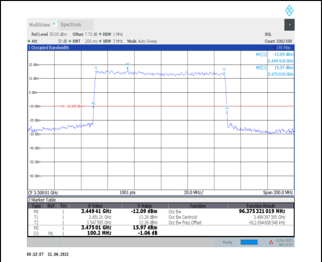
1-N78-3450-3550--30-100-M-1-DFT-QPSK-Outer_Fu ull-270@0-Ant0-96.375-100.200-≤100-PASS
