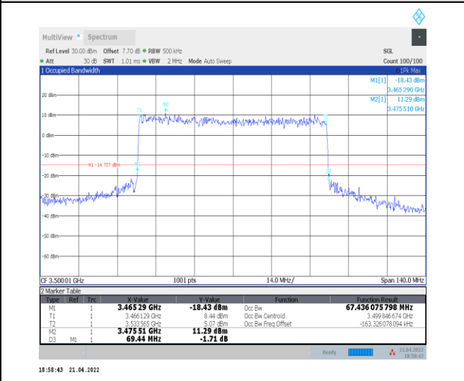
1-N78-3450-3550--30-70-M-6-CP-QPSK-Outer_Full-189@0-Ant0-67.436-69.440-≤70-PASS
