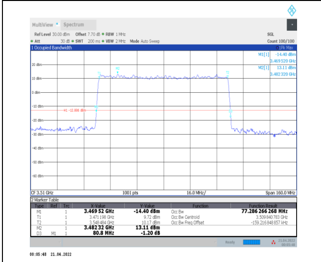
1-N78-3450-3550--30-80-H-5-DFT-256QAM-Outer_F ull-216@0-Ant0-77.286-80.800-<=80-PASS
