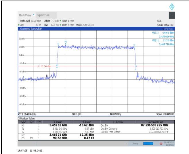
1-N78-3450-3550--30-90-H-8-CP-64QAM-Outer_Full -245@0-Ant0-87.537-90.720-≤90-PASS
