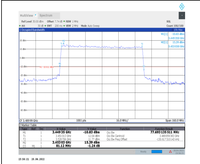
1-N78-3450-3550--30-80-L-7-CP-16QAM-Outer_Full-217@0-Ant0-77.693-81.120-<math>\leq 80</math>-PASS
