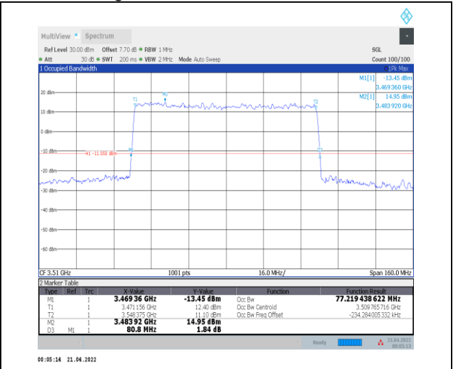
1-N78-3450-3550--30-80-H-4-DFT-64QAM-Outer_Fu II-216@0-Ant0-77.219-80.800-<=80-PASS
