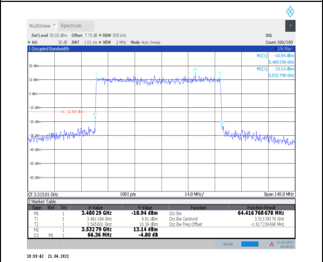
1-N78-3450-3550--30-70-H-1-DFT-QPSK-Outer_Full -180@0-Ant0-64.417-66.360-≤70-PASS
