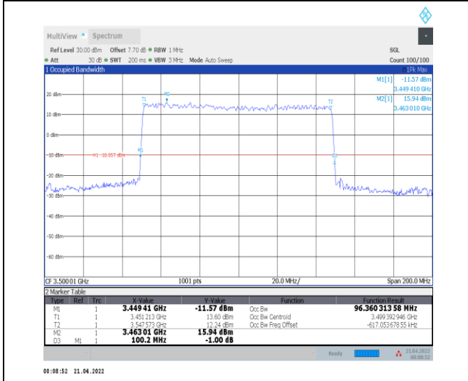
1-N78-3450-3550--30-100-L-1-DFT-QPSK-Outer_Full I-270@0-Ant0-96.36-100.200-≤100-PASS
