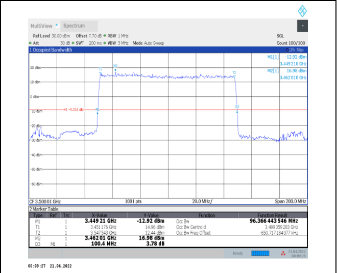
1-N78-3450-3550--30-100-L-2-DFT-P12BPSK-Outer_Full Full-270@0-Ant0-96.366-100.400-≤100-PASS
