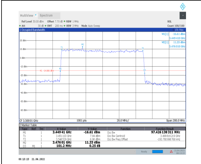
1-N78-3450-3550--30-100-L-9-CP-256QAM-Outer_Fu ull-273@0-Ant0-97.426-101.200-≤100-PASS
