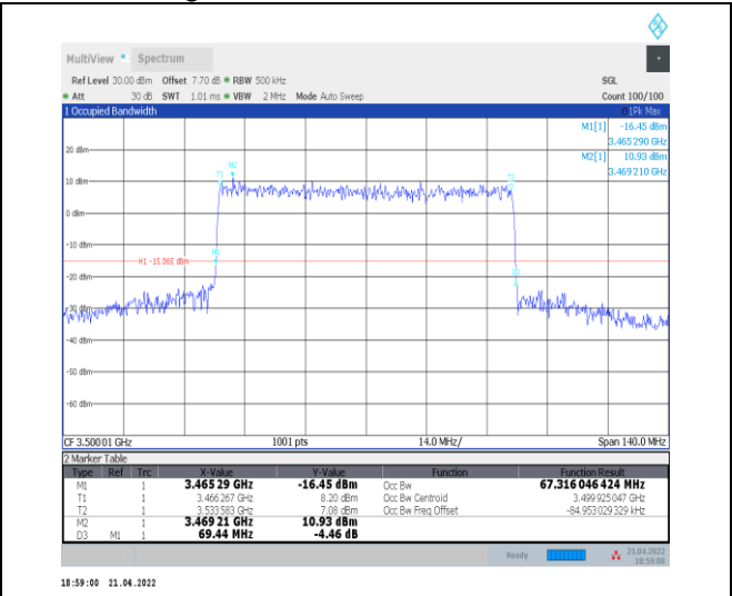
1-N78-3450-3550--30-70-M-8-CP-64QAM-Outer_Ful I-189@0-Ant0-67.316-69.440-≤70-PASS
