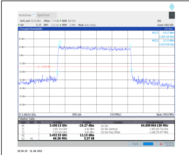
1-N78-3450-3550--30-70-L-4-DFT-64QAM-Outer_Full-180@0-Ant0-64.1-66.360-≤70-PASS
