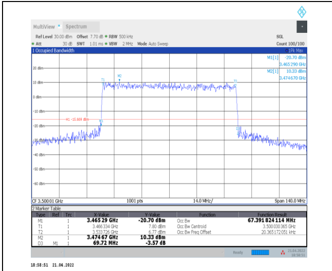
1-N78-3450-3550--30-70-M-7-CP-16QAM-Outer_Full -189@0-Ant0-67.392-69.720-≤70-PASS
