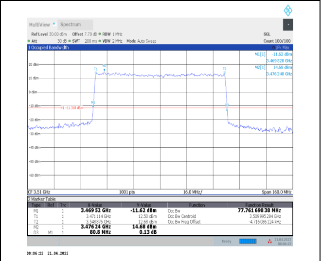
1-N78-3450-3550--30-80-H-6-CP-QPSK-Outer_Full- 217@0-Ant0-77.762-80.800-<=80-PASS
