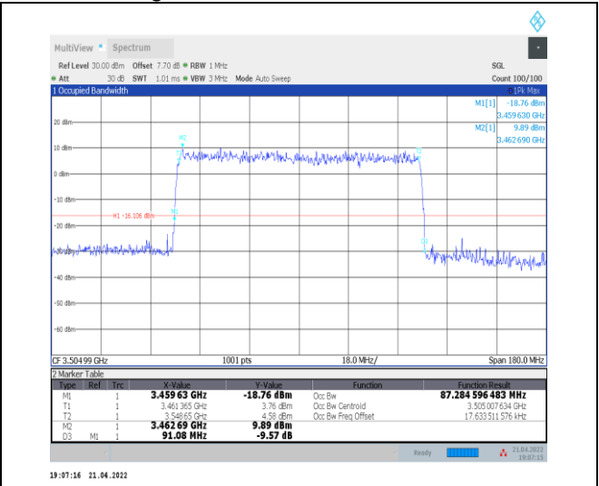
1-N78-3450-3550--30-90-H-9-CP-256QAM-Outer_Full -245@0-Ant0-87.285-91.080-≤90-PASS
