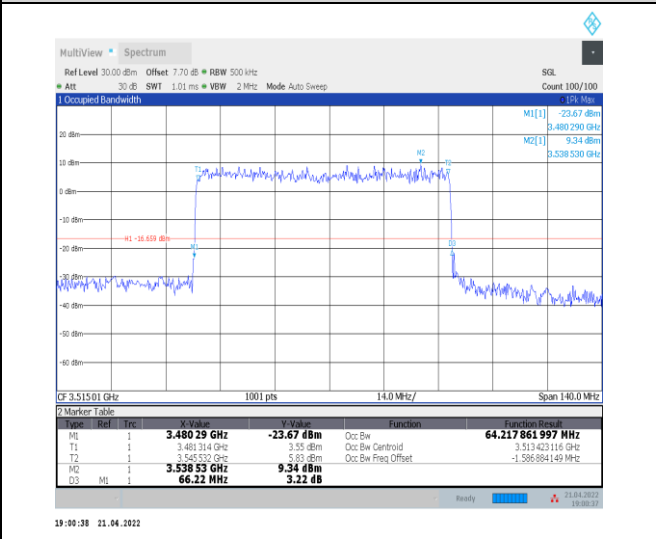
1-N78-3450-3550--30-70-H-5-DFT-256QAM-Outer_F ull-180@0-Ant0-64.218-66.220-≤70-PASS
