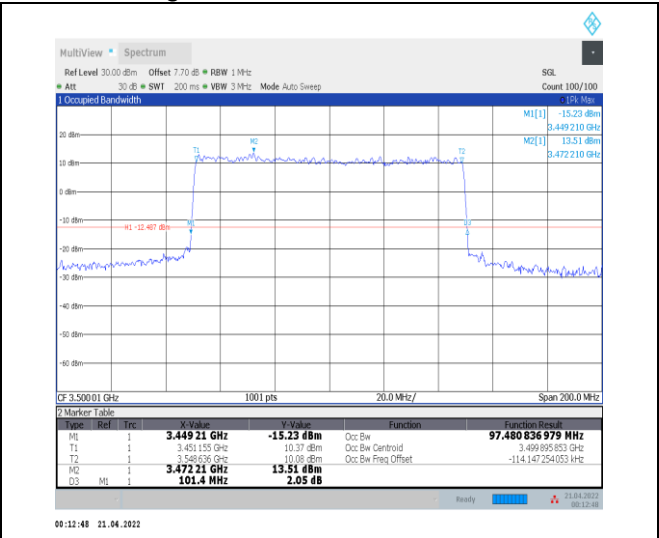
1-N78-3450-3550--30-100-L-8-CP-64QAM-Outer_Fu II-273@0-Ant0-97.481-101.400-≤100-PASS
