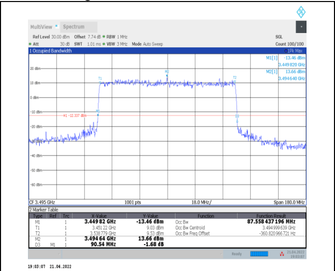
1-N78-3450-3550--30-90-L-7-CP-16QAM-Outer_Full -245@0-Ant0-87.558-90.540≤90-PASS
