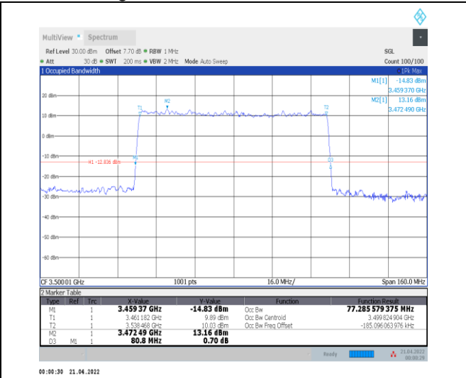
1-N78-3450-3550--30-80-M-5-DFT-256QAM-Outer_Full-216@0-Ant0-77.286-80.800-<math>\leq 80</math>-PASS
