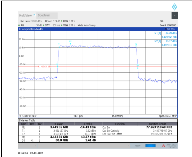
1-N78-3450-3550--30-80-L-5-DFT-256QAM-Outer_Full-216@0-Ant0-77.263-80.800-<math>\leq 80</math>-PASS
