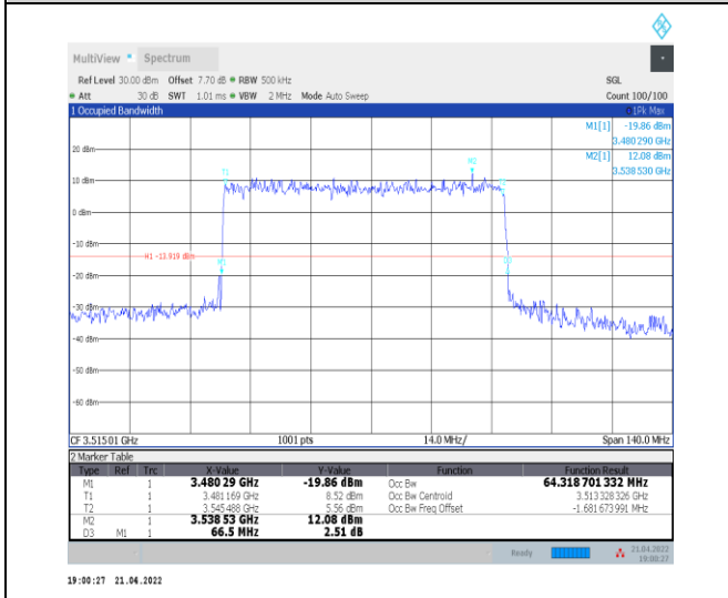
1-N78-3450-3550--30-70-H-4-DFT-64QAM-Outer_Fu ll-180@0-Ant0-64.319-66.500-≤70-PASS
