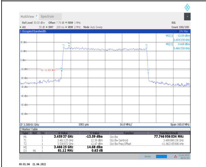
1-N78-3450-3550--30-80-M-6-CP-QPSK-Outer_Full-217@0-Ant0-77.747-81.120-<math>\leq 80</math>-PASS
