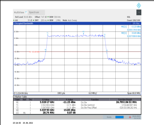
1-N78-3450-3550--30-30-H-1-DFT-QPSK-Outer_Full -75@0-Ant0-26.795-28.740-≤30-PASS
