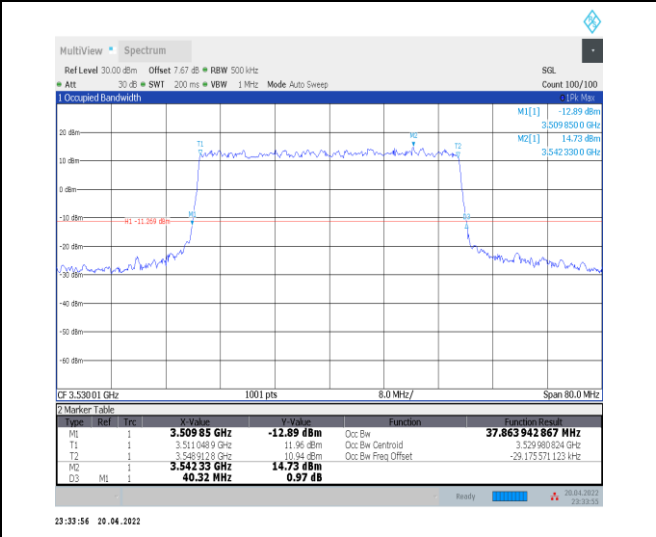
1-N78-3450-3550--30-40-H-6-CP-QPSK-Outer_Full-106@0-Ant0-37.864-40.320-≤40-PASS
