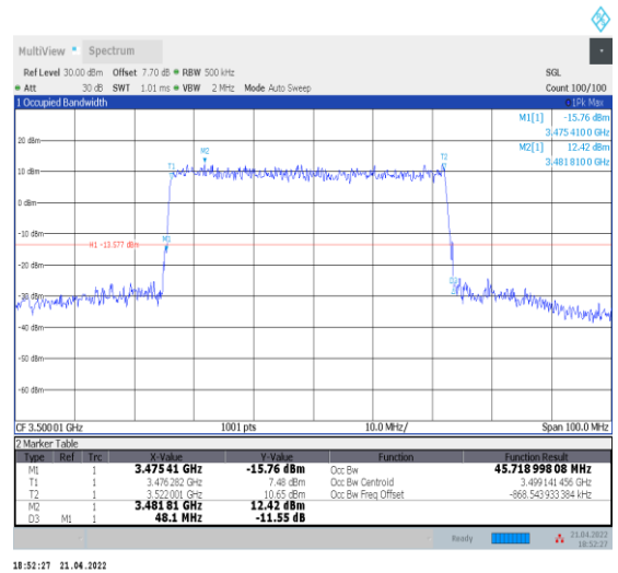
1-N78-3450-3550--30-50-M-4-DFT-64QAM-Outer_Full Full-128@0-Ant0-45.719-48.100-≤50-PASS
