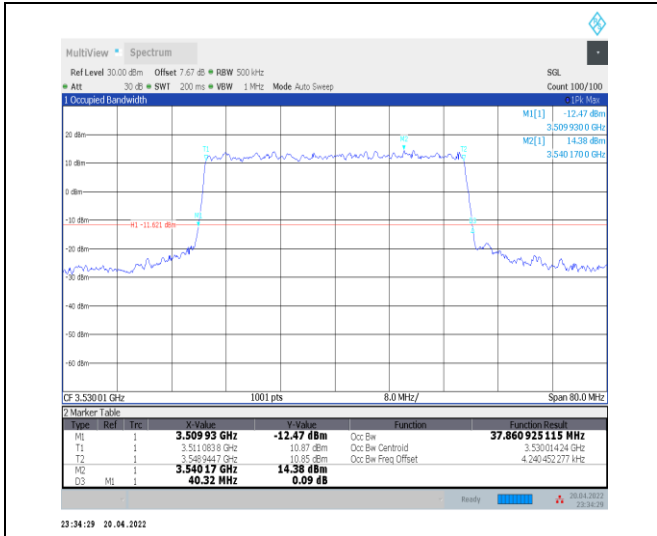
1-N78-3450-3550--30-40-H-7-CP-16QAM-Outer_Full -106@0-Ant0-37.861-40.320-≤40-PASS
