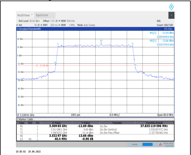
1-N78-3450-3550--30-40-H-8-CP-64QAM-Outer_Full -106@0-Ant0-37.835-40.400-≤40-PASS
