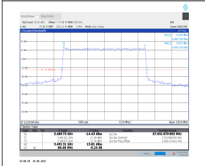
1-N78-3450-3550--30-60-H-3-DFT-16QAM-Outer_Fu ll-162@0-Ant0-57.952-60.480-≤60-PASS
