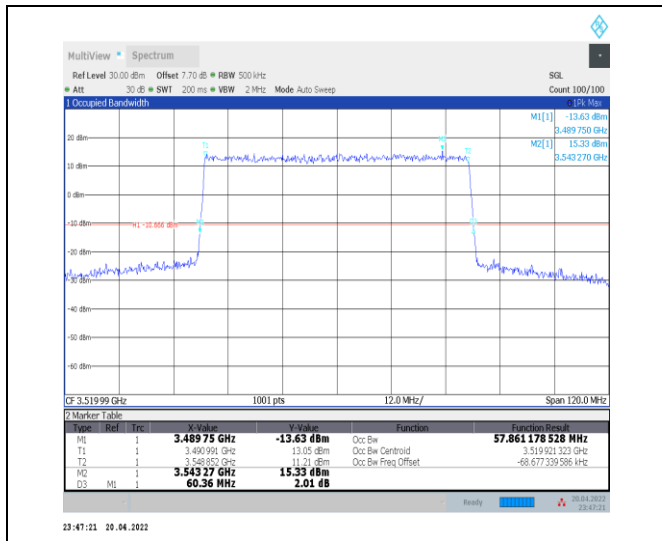
1-N78-3450-3550--30-60-H-1-DFT-QPSK-Outer_Full -162@0-Ant0-57.861-60.360-≤60-PASS
