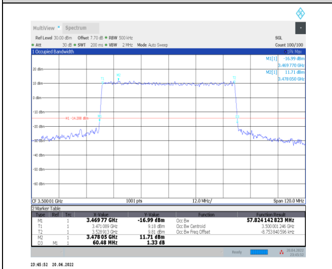
1-N78-3450-3550--30-60-M-8-CP-64QAM-Outer_Full-162@0-Ant0-57.824-60.480-<=60-PASS
