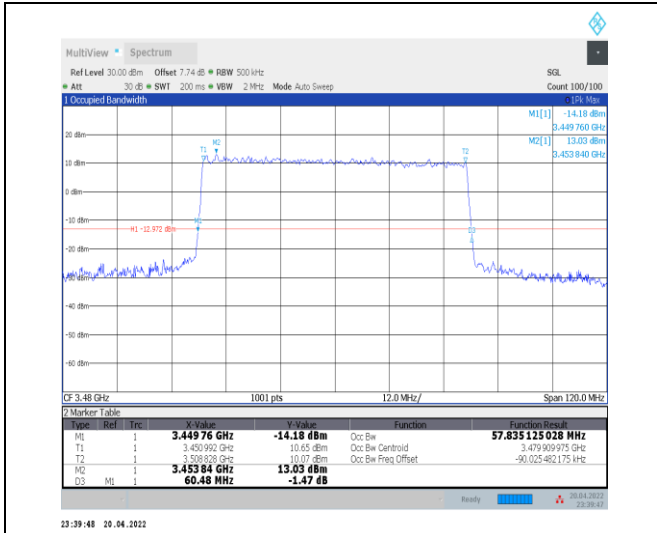
1-N78-3450-3550--30-60-L-7-CP-16QAM-Outer_Full -162@0-Ant0-57.835-60.480-≤60-PASS
