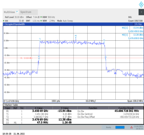
1-N78-3450-3550--30-50-L-5-DFT-256QAM-Outer_F ull-128@0-Ant0-45.687-47.500-≤50-PASS
