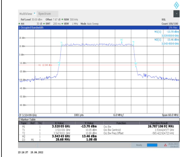
1-N78-3450-3550--30-30-H-4-DFT-64QAM-Outer_Fu II-75@0-Ant0-26.787-28.680-≤30-PASS
