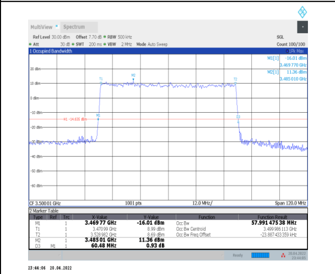
1-N78-3450-3550--30-60-M-5-DFT-256QAM-Outer_Full-162@0-Ant0-57.991-60.480-≤60-PASS
