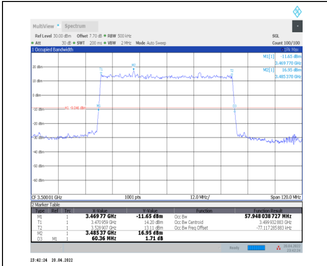
1-N78-3450-3550--30-60-M-2-DFT-PI2BPSK-Outer_Full-162@0-Ant0-57.948-60.360-≤60-PASS
