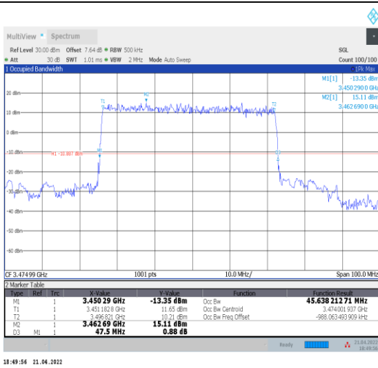
1-N78-3450-3550--30-50-L-2-DFT-PI2BPSK-Outer_F ull-128@0-Ant0-45.638-47.500-≤50-PASS
