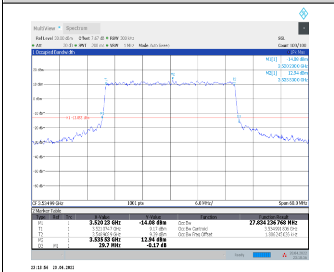
1-N78-3450-3550--30-30-H-8-CP-64QAM-Outer_Full-78@0-Ant0-27.834-29.700-≤30-PASS
