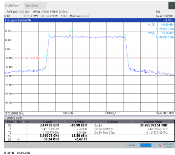
1-N78-3450-3550--30-40-M-3-DFT-16QAM-Outer_Full-100@0-Ant0-35.761-38.240-≤40-PASS
