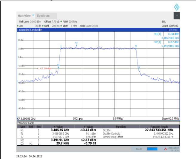
1-N78-3450-3550--30-30-M-8-CP-64QAM-Outer_Ful I-78@0-Ant0-27.844-29.700-≤30-PASS
