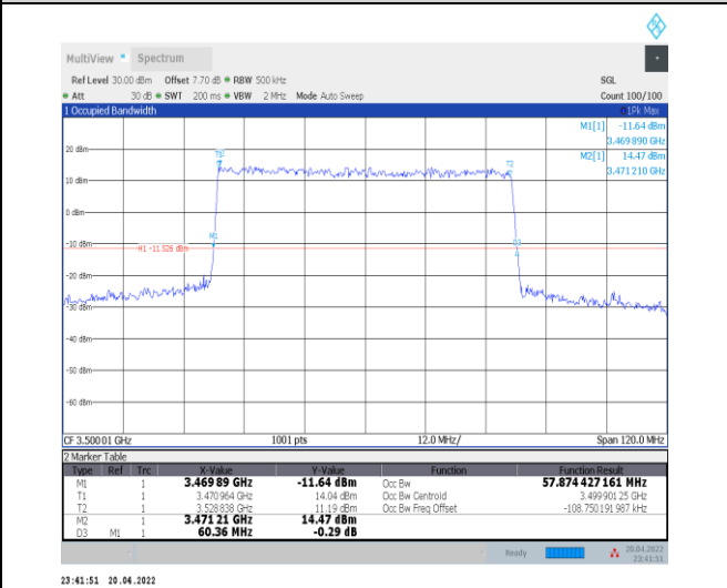
1-N78-3450-3550--30-60-M-1-DFT-QPSK-Outer_Full -162@0-Ant0-57.874-60.360-≤60-PASS
