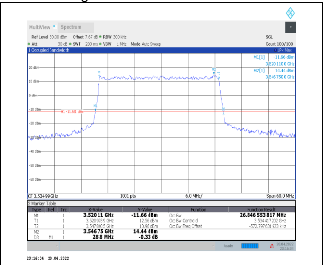
1-N78-3450-3550--30-30-H-3-DFT-16QAM-Outer_Fu II-75@0-Ant0-26.847-28.800-≤30-PASS
