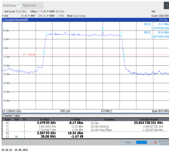
1-N78-3450-3550--30-40-M-2-DFT-PI2BPSK-Outer_Full-100@0-Ant0-35.835-38.080-≤40-PASS
