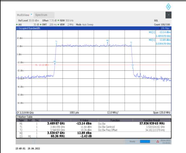
1-N78-3450-3550--30-60-H-4-DFT-64QAM-Outer_Fu ll-162@0-Ant0-57.937-60.360-≤60-PASS
