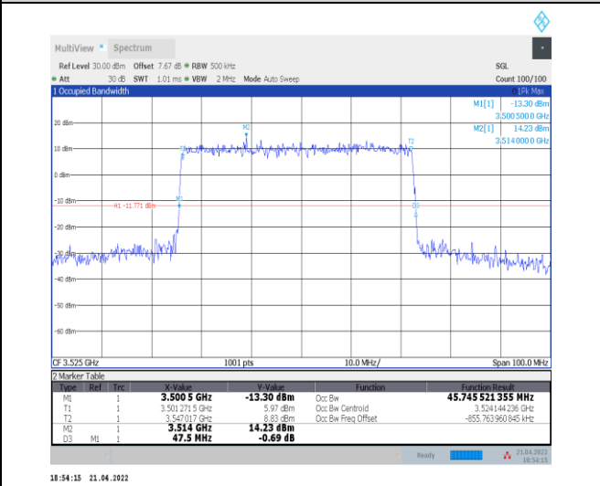
1-N78-3450-3550--30-50-H-3-DFT-16QAM-Outer_Full-128@0-Ant0-45.746-47.500-≤50-PASS
