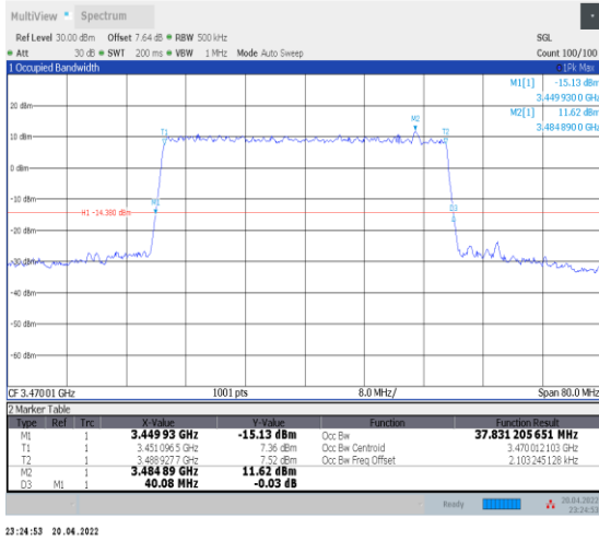
1-N78-3450-3550--30-40-L-9-CP-256QAM-Outer_Fu II-106@0-Ant0-37.831-40.080-≤40-PASS
