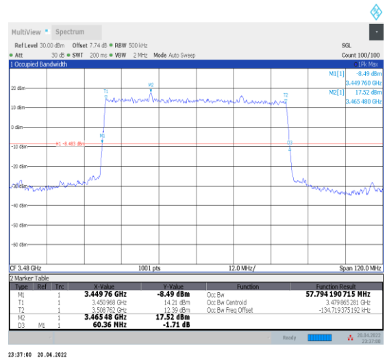
1-N78-3450-3550--30-60-L-2-DFT-PI2BPSK-Outer_Full-162@0-Ant0-57.794-60.360-≤60-PASS
