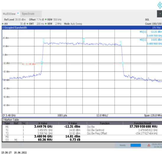
1-N78-3450-3550--30-60-L-1-DFT-QPSK-Outer_Full-162@0-Ant0-57.79-60.360-≤60-PASS
