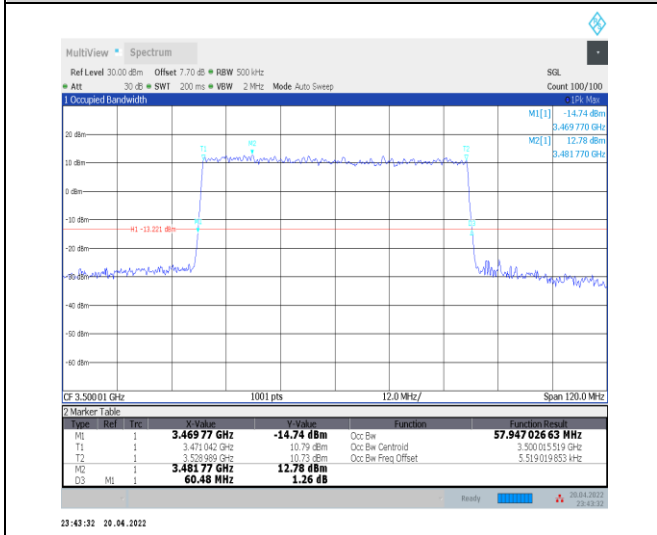
1-N78-3450-3550--30-60-M-4-DFT-64QAM-Outer_Full-162@0-Ant0-57.947-60.480-≤60-PASS
