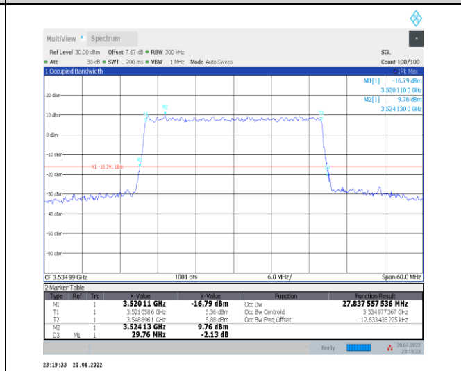
1-N78-3450-3550--30-30-H-9-CP-256QAM-Outer_Full-78@0-Ant0-27.838-29.760-≤30-PASS
