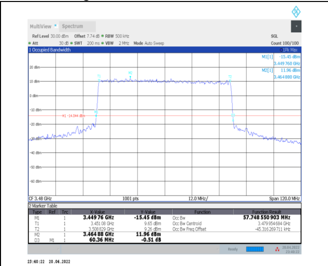
1-N78-3450-3550--30-60-L-8-CP-64QAM-Outer_Full -162@0-Ant0-57.749-60.360-≤60-PASS
