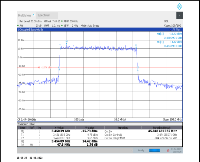
1-N78-3450-3550--30-50-L-1-DFT-QPSK-Outer_Full- 128@0-Ant0-45.848-47.600-≤50-PASS
