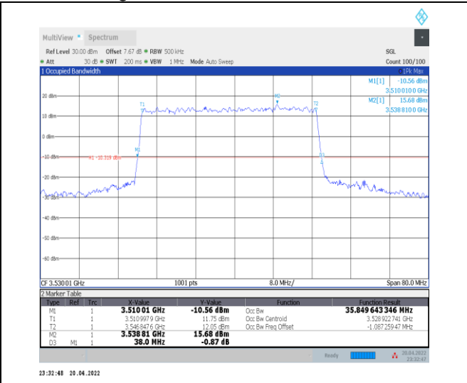
1-N78-3450-3550--30-40-H-4-DFT-64QAM-Outer_Fu II-100@0-Ant0-35.85-38.000-≤40-PASS
