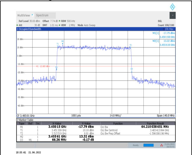
1-N78-3450-3550--30-70-L-1-DFT-QPSK-Outer_Full-180@0-Ant0-64.21-66.360-≤70-PASS
