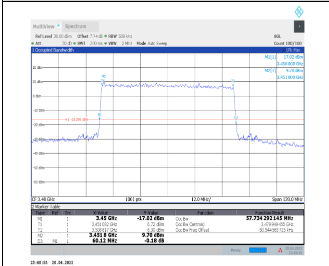
1-N78-3450-3550--30-60-L-9-CP-256QAM-Outer_Fu ll-162@0-Ant0-57.734-60.120-≤60-PASS
