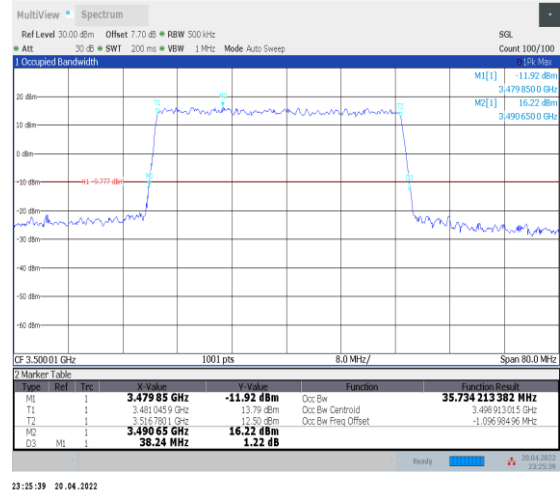
1-N78-3450-3550--30-40-M-1-DFT-QPSK-Outer_Full -100@0-Ant0-35.734-38.240-≤40-PASS
