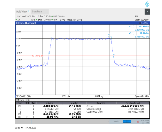
1-N78-3450-3550--30-30-M-5-DFT-256QAM-Outer_Full-75@0-Ant0-26.827-28.980-≤30-PASS
