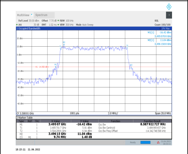
1-N78-3450-3550--30-10-M-7-CP-16QAM-Outer_Full-24@0-Ant0-8.588-9.740-<=10-PASS
