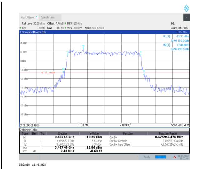
1-N78-3450-3550--30-10-M-4-DFT-64QAM-Outer_F ull-24@0-Ant0-8.576-9.480-<=10-PASS
