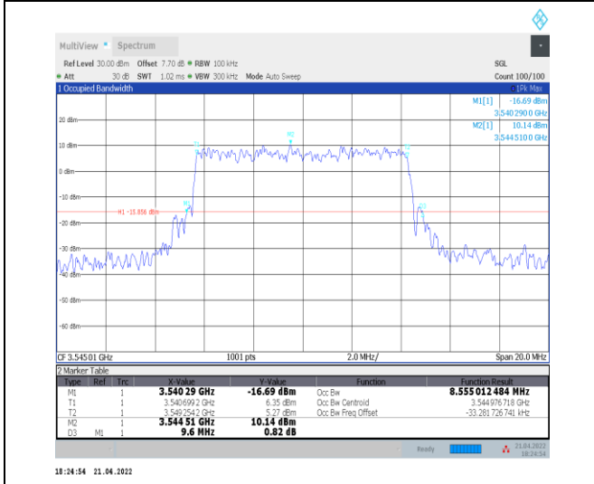
1-N78-3450-3550--30-10-H-5-DFT-256QAM-Outer_Full-24@0-Ant0-8.555-9.600-≤10-PASS
