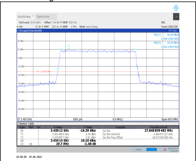
1-N78-3450-3550--30-30-L-9-CP-256QAM-Outer_Fu II-78@0-Ant0-27.849-29.700-<30-PASS
