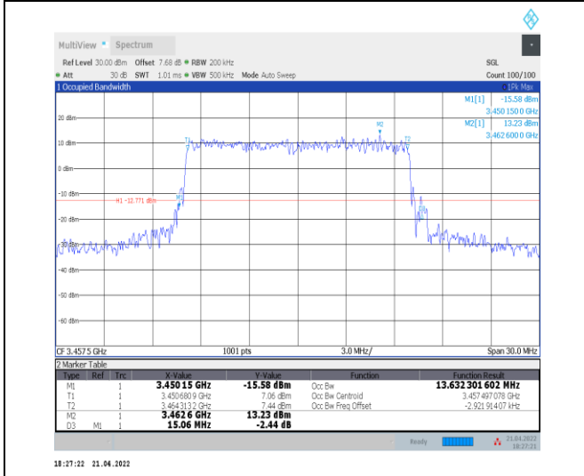
1-N78-3450-3550--30-15-L-8-CP-64QAM-Outer_Full -38@0-Ant0-13.632-15.060-≤15-PASS
