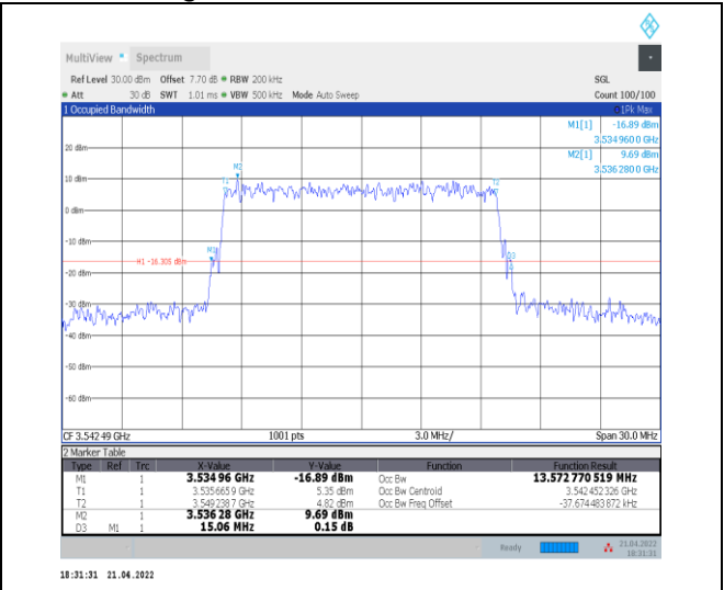
1-N78-3450-3550--30-15-H-9-CP-256QAM-Outer_Full -38@0-Ant0-13.573-15.060-≤15-PASS
