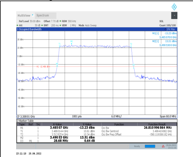
1-N78-3450-3550--30-30-M-4-DFT-64QAM-Outer_Full-75@0-Ant0-26.811-28.680-≤30-PASS
