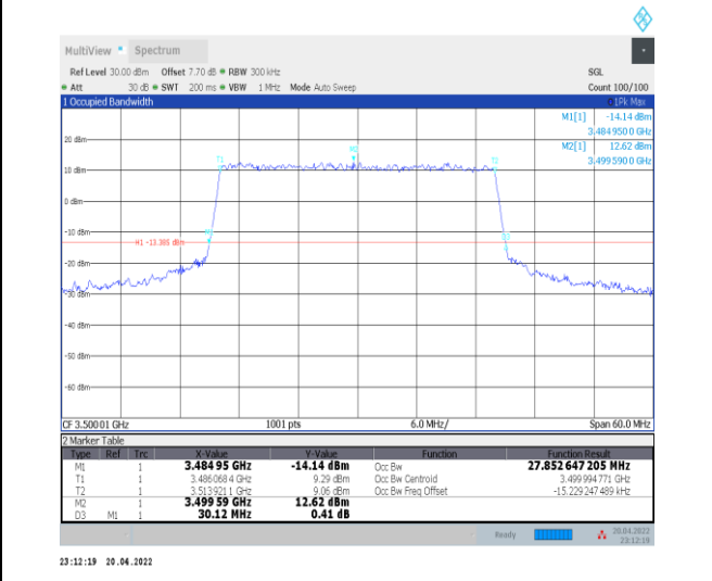
1-N78-3450-3550--30-30-M-6-CP-QPSK-Outer_Full-78@0-Ant0-27.853-30.120-≤30-PASS
