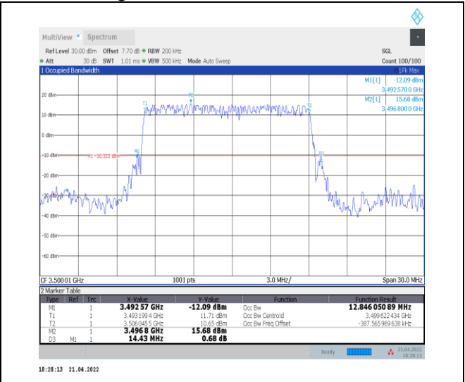
1-N78-3450-3550--30-15-M-2-DFT-PI2BPSK-Outer_Full Full-36@0-Ant0-12.846-14.430-≤15-PASS
