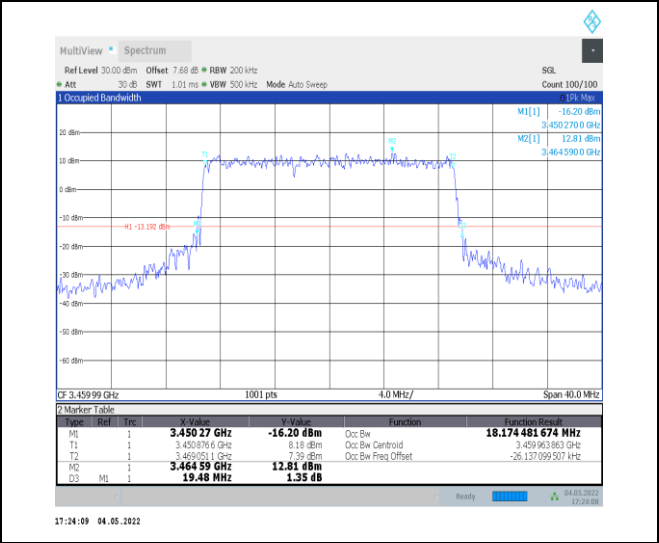
1-N78-3450-3550--30-20-L-6-CP-QPSK-Outer_Full-51@0-Ant0-18.174-19.480-<=20-PASS
