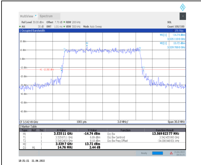
1-N78-3450-3550--30-15-H-8-CP-64QAM-Outer_Full -38@0-Ant0-13.57-14.760-≤15-PASS
