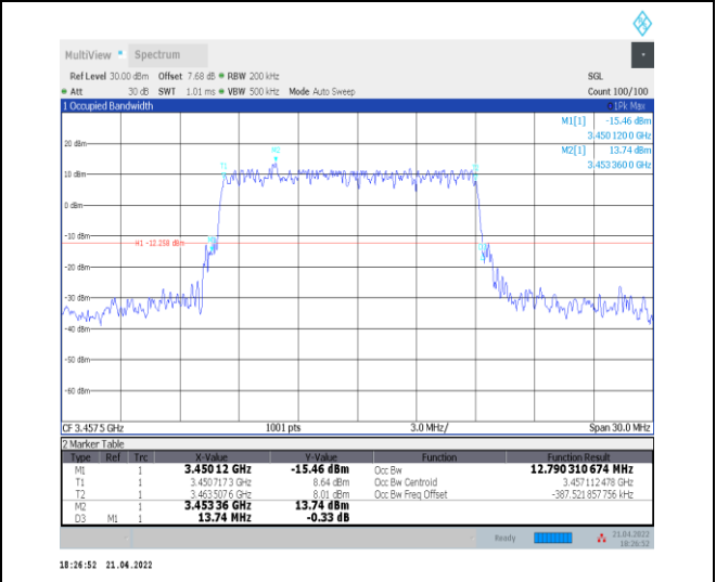
1-N78-3450-3550--30-15-L-5-DFT-256QAM-Outer_Full-36@0-Ant0-12.79-13.740-≤15-PASS
