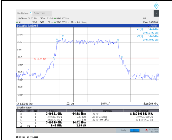
1-N78-3450-3550--30-10-M-2-DFT-PI2BPSK-Outer_Full-24@0-Ant0-8.58-9.480-≤10-PASS
