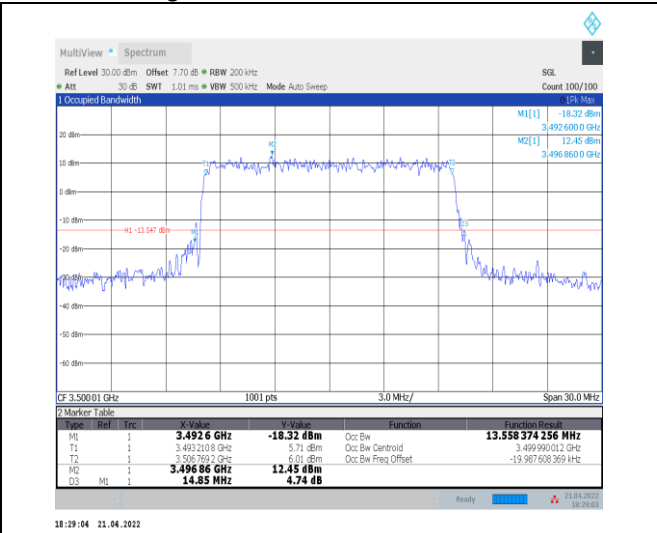
1-N78-3450-3550--30-15-M-6-CP-QPSK-Outer_Full-38@0-Ant0-13.558-14.850-≤15-PASS
