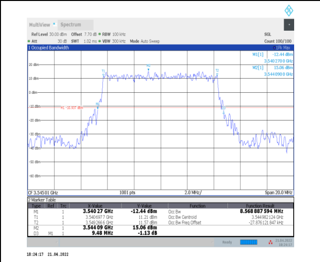
1-N78-3450-3550--30-10-H-2-DFT-PI2BPSK-Outer_ Full-24@0-Ant0-8.569-9.480-≤10-PASS
