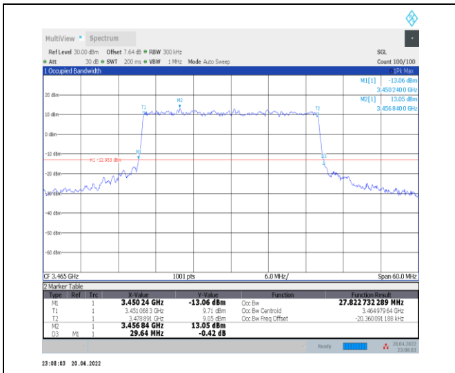
1-N78-3450-3550--30-30-L-8-CP-64QAM-Outer_Full -78@0-Ant0-27.823-29.640-<30-PASS
