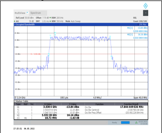
1-N78-3450-3550--30-20-H-2-DFT-PI2BPSK-Outer_Full Full-50@0-Ant0-17.844-18.720-≤20-PASS
