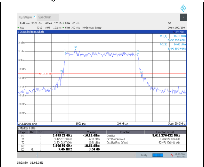
1-N78-3450-3550--30-10-M-5-DFT-256QAM-Outer_ Full-24@0-Ant0-8.611-9.460-<=10-PASS
