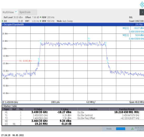
1-N78-3450-3550--30-20-L-9-CP-256QAM-Outer_Fu II-51 @ 0-Ant0-18.218-19.240-≤20-PASS
