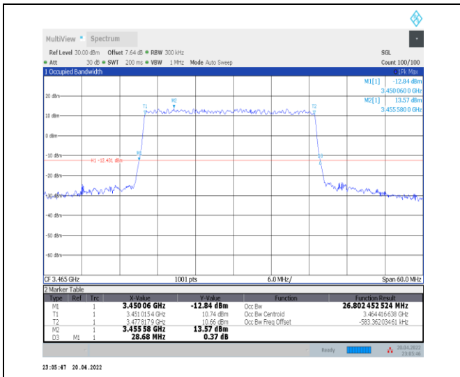
1-N78-3450-3550--30-30-L-4-DFT-64QAM-Outer_Full I-75@0-Ant0-26.802-28.680-≤30-PASS
