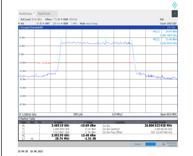
1-N78-3450-3550--30-30-M-1-DFT-QPSK-Outer_Full -75@0-Ant0-26.807-28.740-<30-PASS
