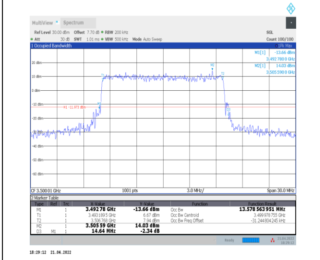
1-N78-3450-3550--30-15-M-7-CP-16QAM-Outer_Full-38@0-Ant0-13.579-14.640-≤15-PASS
