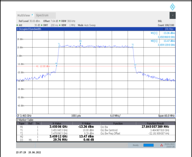
1-N78-3450-3550--30-30-L-7-CP-16QAM-Outer_Full -78@0-Ant0-27.845-29.760-≤30-PASS
