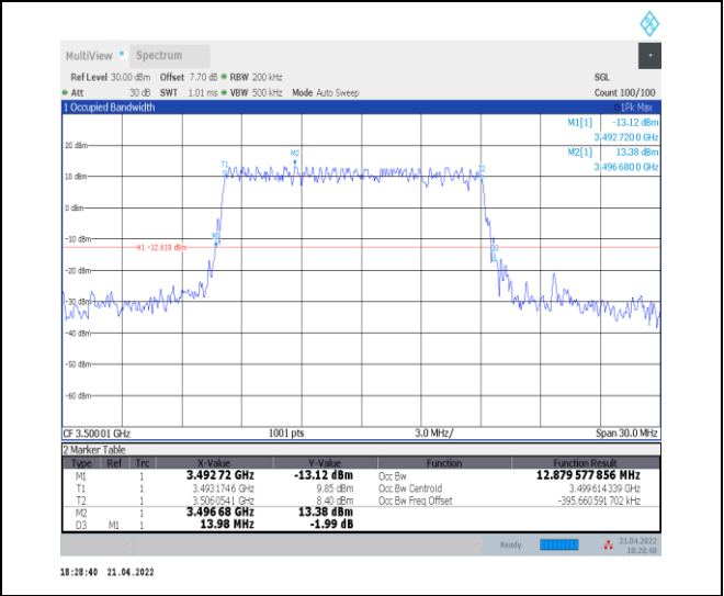
1-N78-3450-3550--30-15-M-4-DFT-64QAM-Outer_Full ull-36@0-Ant0-12.88-13.980-≤15-PASS
