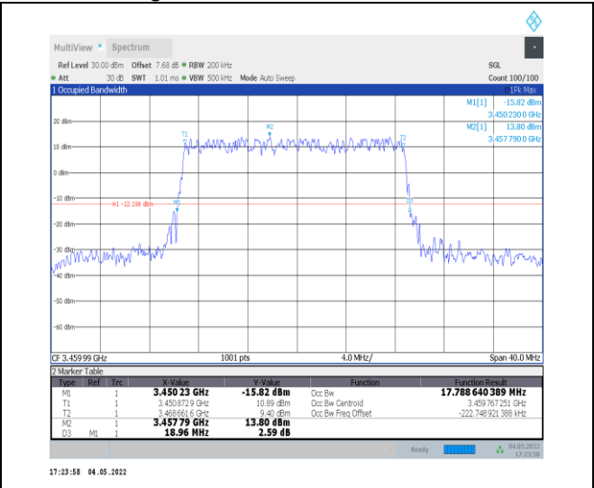
1-N78-3450-3550--30-20-L-4-DFT-64QAM-Outer_Fu II-50@0-Ant0-17.789-18.960-<=20-PASS
