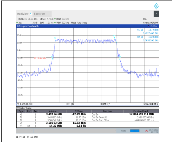
1-N78-3450-3550--30-15-M-1-DFT-QPSK-Outer_Full -36@0-Ant0-12.885-14.220-≤15-PASS
