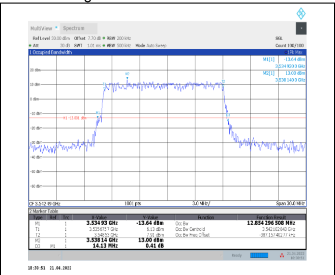
1-N78-3450-3550--30-15-H-5-DFT-256QAM-Outer_F ull-36@0-Ant0-12.854-14.130-≤15-PASS
