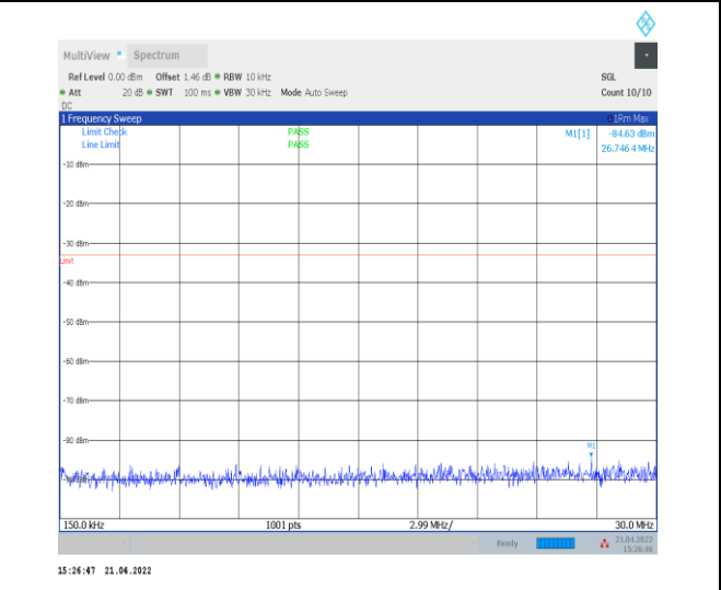
1-N77-3700-3980--30-100-M-1-DFT-PI2BPSK-Inner_1RB_Left-1 @ 1-0.15-30-Ant0--84.63--33-PASS
