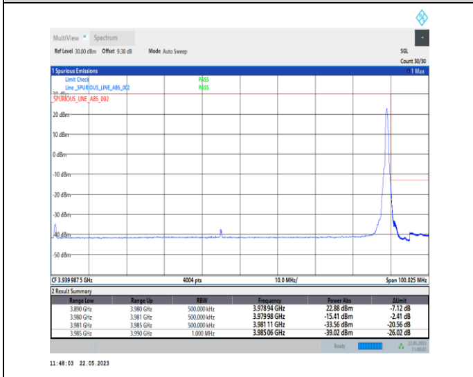
1-N77-3700-3980-PC1-30-90-H-5-CP-QPSK-Edge_1R B_Right-1@244-Ant0-1--PASS-see graph
