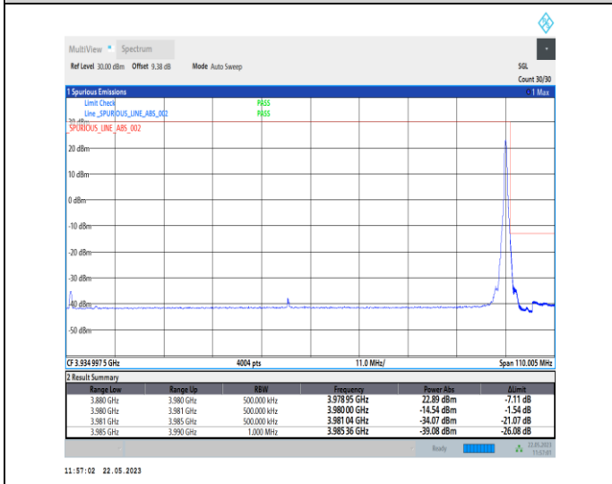
1-N77-3700-3980-PC1-30-100-H-5-CP-QPSK-Edge_1RB_Right-1@272-Ant0-1--PASS-see graph
