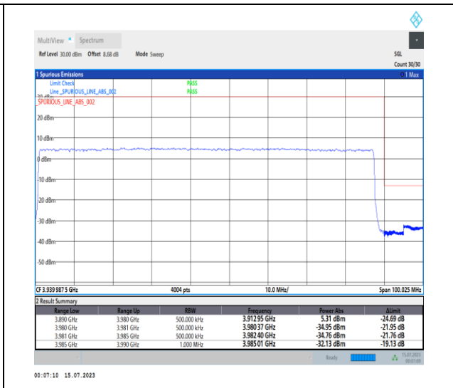
1-N77-3700-3980-PC1-30-90-H-3-DFT-PI2BPSK- Outer_Full-240@0-Ant0-1--PASS-see graph
