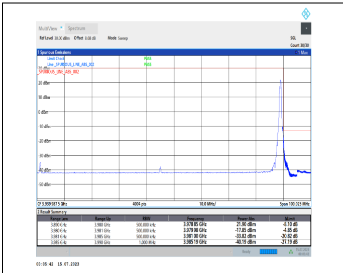
1-N77-3700-3980-PC1-30-90-H-2-DFT-PI2BPSK-Edge _1RB_Right-1@244-Ant0-1--PASS-see graph
