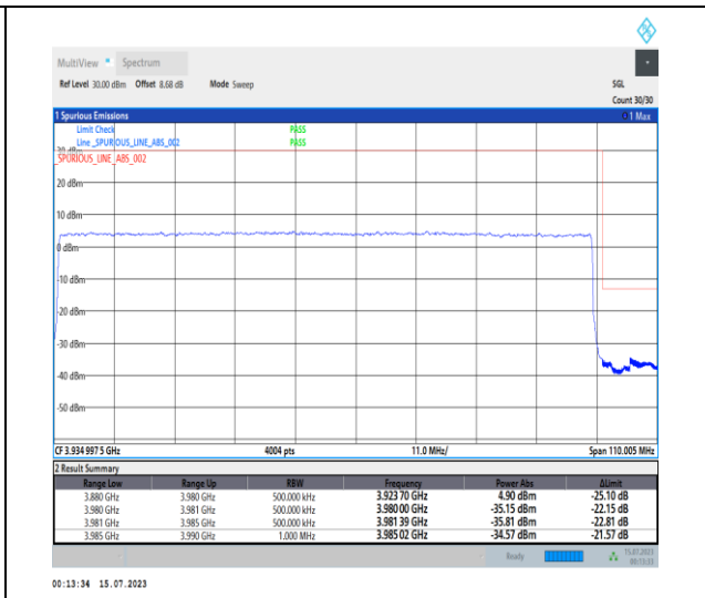
1-N77-3700-3980-PC1-30-100-H-3-DFT-PI2BPSK-Outer_Full-270@0-Ant0-1--PASS-see graph
