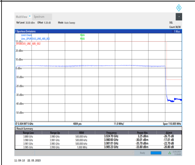
1-N77-3700-3980-PC1-30-100-H-6-CP-QPSK-Outer_Full-273@0-Ant0-1--PASS-see graph
