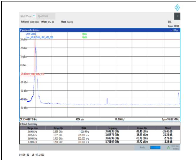
1-N77-3700-3980-PC1-30-100-L-1-DFT-PI2BPSK-Edge_1RB_Left-1@0-Ant0-1--PASS-see graph
