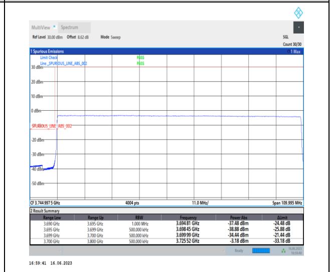
1-N77-3700-3980-PC1-30-100-L-6-CP-QPSK-Outer_Full-273@0-Ant0-1--PASS-see graph
