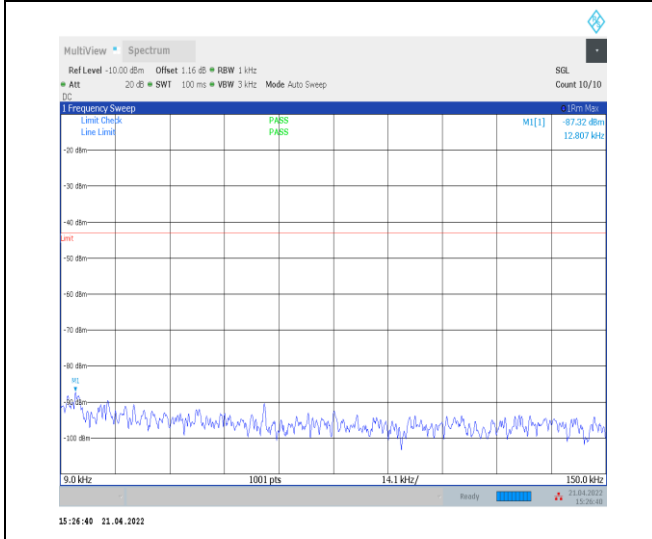
1-N77-3700-3980--30-100-M-1-DFT-PI2BPSK-Inner_1RB_Left-1 @ 1-0.009-0.15-Ant0--87.32--43-PASS
