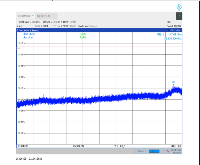
1-N77-3700-3980--30-100-L-1-DFT-PI2BPSK-Inner_1RB_Left-1 @ 1-18000-40000-Ant0--47.61--13-PASS
