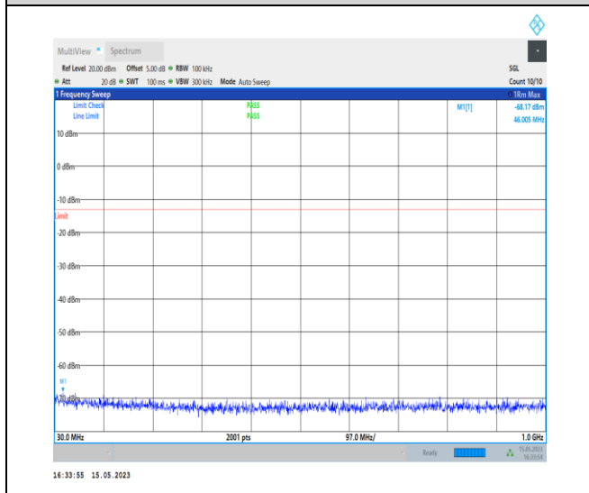
1-N77-3700-3980-PC1-30-100-H-1-DFT-PI2BPSK-I nner_1RB_Left-1@1-30-1000-Ant0-46.01--68.17--1 3-PASS
