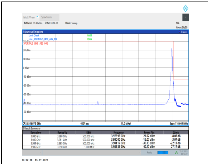
1-N77-3700-3980-PC1-30-100-H-2-DFT-PI2BPSK-Edge_e_1RB_Right-1@272-Ant0-1--PASS-see graph
