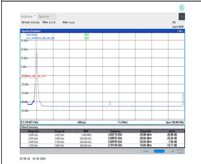
1-N77-3700-3980-PC1-30-100-L-4-CP-QPSK-Edge_1RB_Left-1@0-Ant0-1--PASS-see graph
