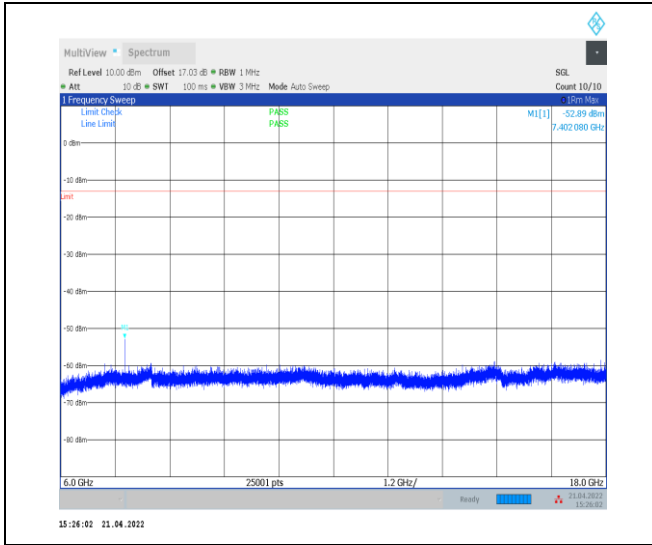
1-N77-3700-3980--30-100-L-1-DFT-PI2BPSK-Inner_1RB_Left-1 @ 1-6000-18000-Ant0--52.89--13-PASS
