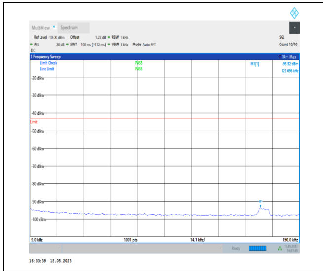
1-N77-3700-3980-PC1-30-100-H-1-DFT-PI2BPSK- Inner_1RB_Left-1@1-0.009-0.15-Ant0-0.13--93.52-- 43-PASS
