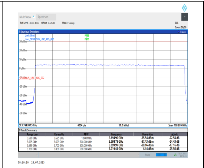
1-N77-3700-3980-PC1-30-100-L-3-DFT-PI2BPSK-Outer_Full-270@0-Ant0-1--PASS-see graph
