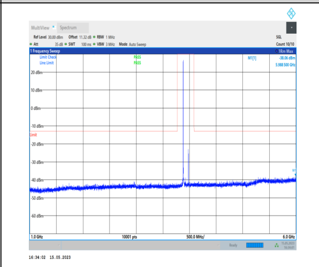
1-N77-3700-3980-PC1-30-100-H-1-DFT-PI2BPSK-In ner_1RB_Left-1@1-1000-6000-Ant0-5988.50--38.06- -13-PASS
