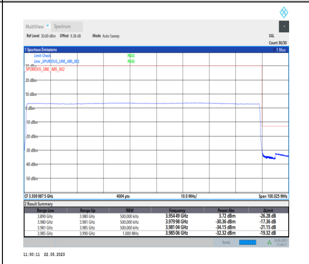
1-N77-3700-3980-PC1-30-90-H-6-CP-QPSK-Outer _Full-245@0-Ant0-1--PASS-see graph
