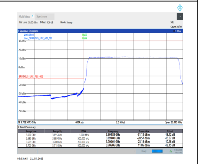
1-N77-3700-3980-PC1-30-15-L-6-CP-QPSK-Outer_Full-38@0-Ant0-1--PASS-see graph
