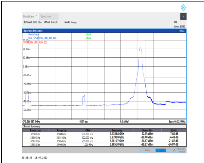
1-N77-3700-3980-PC1-30-30-H-2-DFT-PI2BPSK-Edge _1RB_Right-1@77-Ant0-1--PASS-see graph
