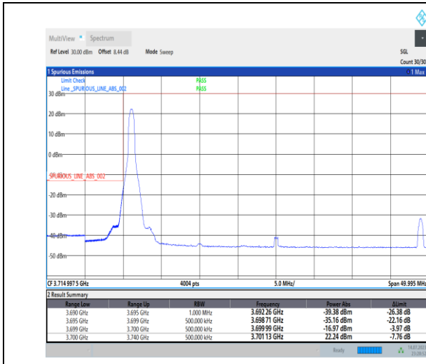
1-N77-3700-3980-PC1-30-40-L-1-DFT-PI2BPSK-Edge_1_RB_Left-1@0-Ant0-1--PASS-see graph
