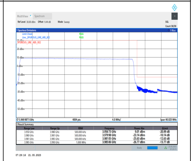
1-N77-3700-3980-PC1-30-30-H-6-CP-QPSK-Outer _Full-78@0-Ant0-1--PASS-see graph
