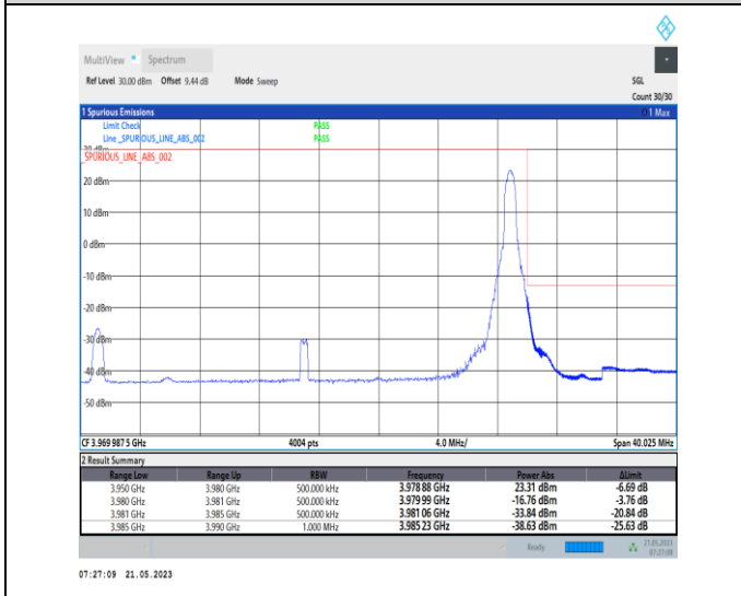
1-N77-3700-3980-PC1-30-30-H-5-CP-QPSK-Edge_1R B_Right-1@77-Ant0-1--PASS-see graph
