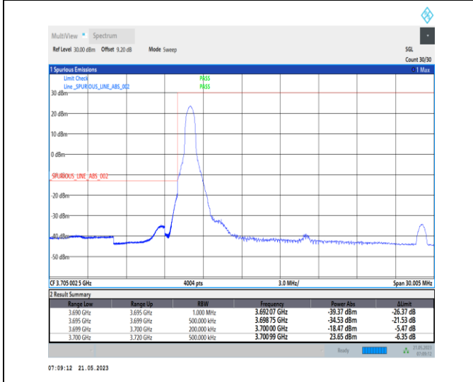
1-N77-3700-3980-PC1-30-20-L-4-CP-QPSK-Edge_1RB_Left-1@0-Ant0-1--PASS-see graph
