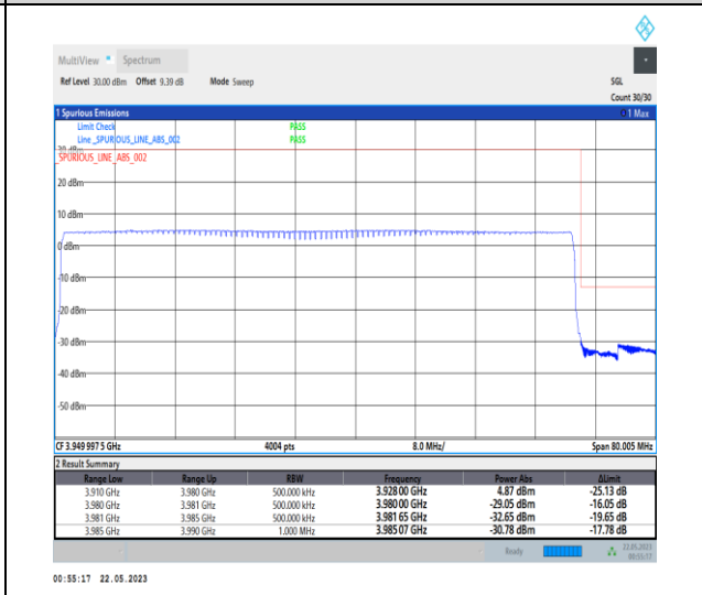
1-N77-3700-3980-PC1-30-70-H-6-CP-QPSK-Outer _Full-189@0-Ant0-1--PASS-see graph
