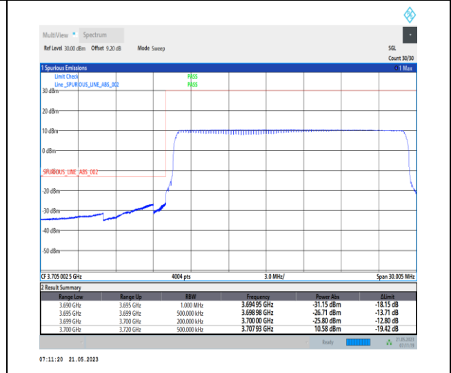
1-N77-3700-3980-PC1-30-20-L-6-CP-QPSK-Outer_Full-51@0-Ant0-1--PASS-see graph
