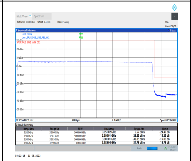
1-N77-3700-3980-PC1-30-60-H-6-CP-QPSK-Outer _Full-162@0-Ant0-1--PASS-see graph
