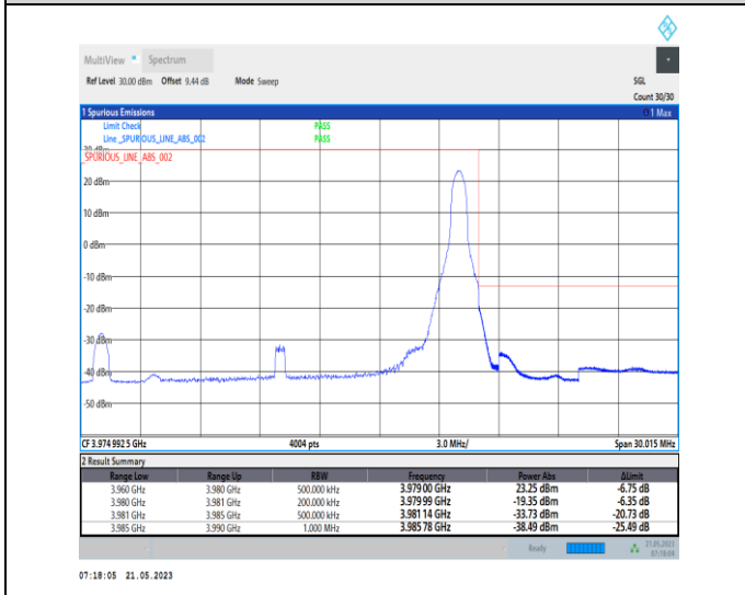
1-N77-3700-3980-PC1-30-20-H-5-CP-QPSK-Edge_1RB_Right-1@50-Ant0-1--PASS-see graph
