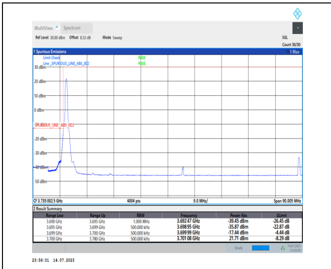
1-N77-3700-3980-PC1-30-80-L-1-DFT-PI2BPSK-Edge_1_RB_Left-1@0-Ant0-1--PASS-see graph
