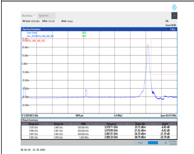
1-N77-3700-3980-PC1-30-50-H-5-CP-QPSK-Edge_1R B_Right-1@132-Ant0-1--PASS-see graph
