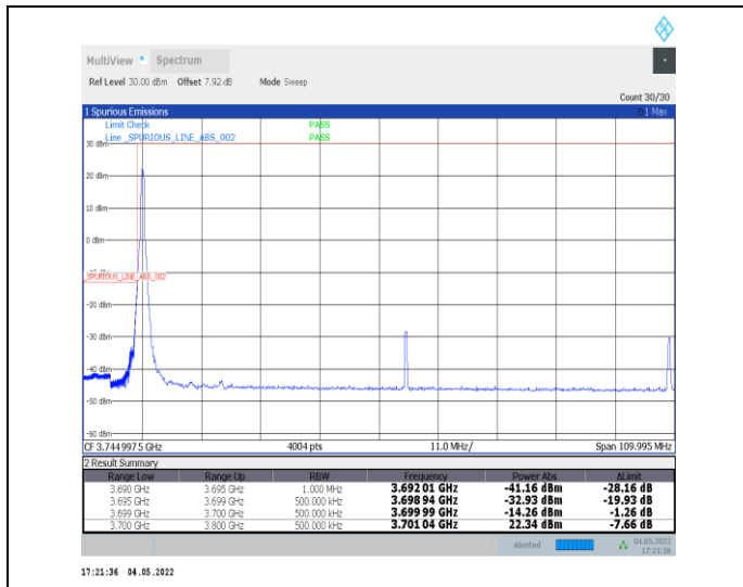
1-N77-3700-3980--30-100-L-1-DFT-PI2BPSK-Edge_1 RB_Left-1@0-Ant0-PASS-see graph
