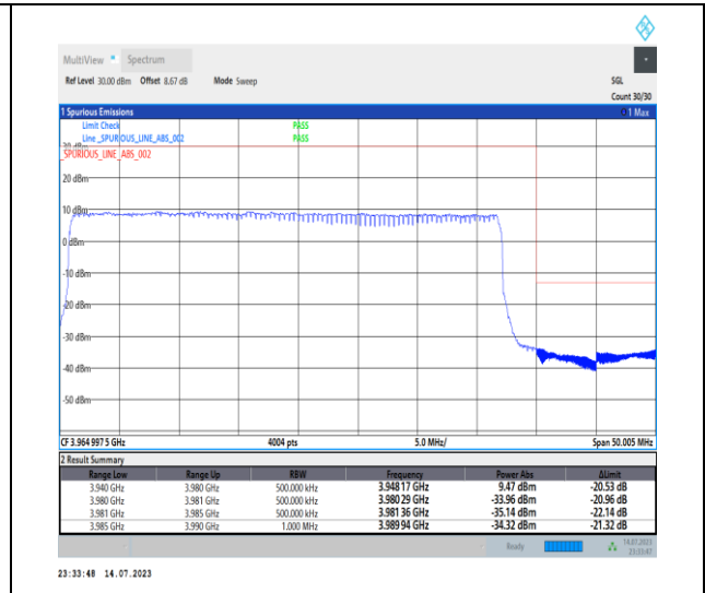
1-N77-3700-3980-PC1-30-40-H-3-DFT-PI2BPSK-Outer_Full-100@0-Ant0-1--PASS-see graph
