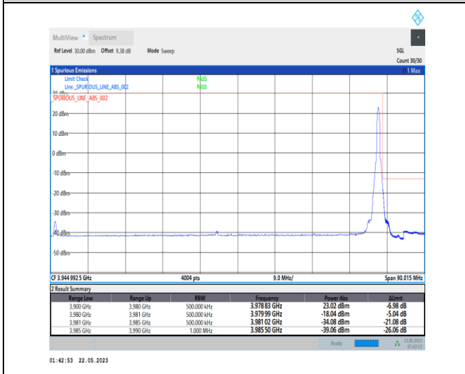
1-N77-3700-3980-PC1-30-80-H-5-CP-QPSK-Edge_1R B_Right-1@216-Ant0-1--PASS-see graph
