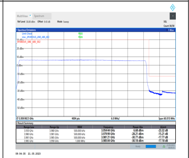
1-N77-3700-3980-PC1-30-50-H-6-CP-QPSK-Outer _Full-133@0-Ant0-1--PASS-see graph
