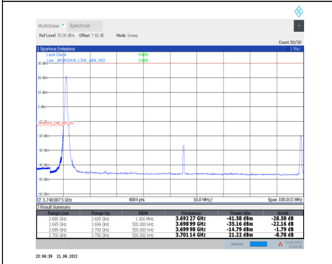
1-N77-3700-3980--30-90-L-4-CP-QPSK-Edge_1RB_L_eff-1@0-Ant0-PASS-see graph
