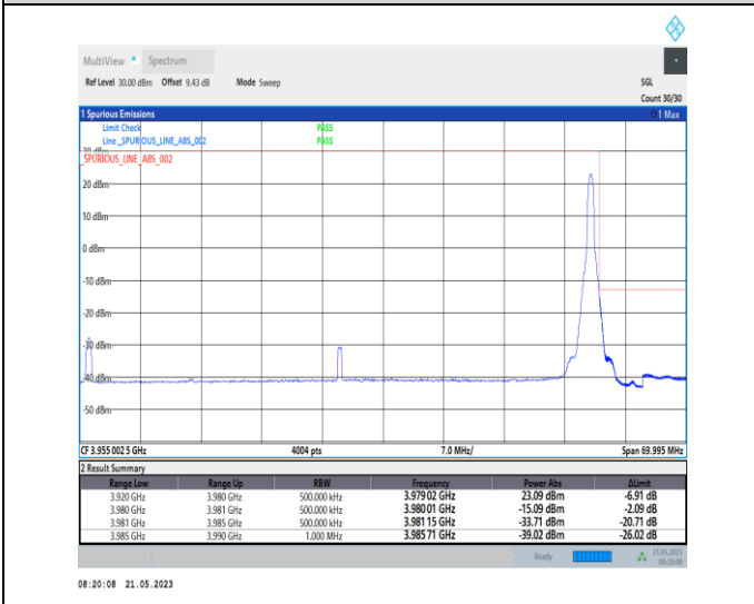
1-N77-3700-3980-PC1-30-60-H-5-CP-QPSK-Edge_1R B_Right-1@161-Ant0-1--PASS-see graph
