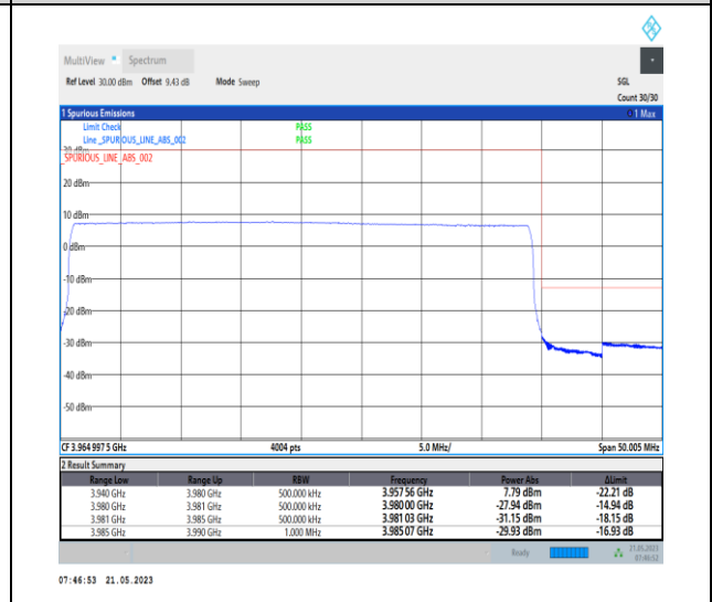
1-N77-3700-3980-PC1-30-40-H-6-CP-QPSK-Outer_Full-106@0-Ant0-1--PASS-see graph
