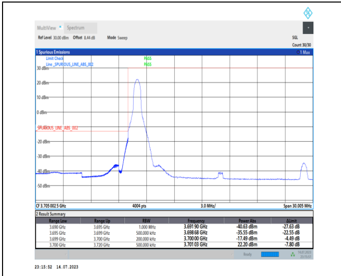
1-N77-3700-3980-PC1-30-20-L-1-DFT-PI2BPSK-Edge_e_1RB_Left-1@0-Ant0-1--PASS-see graph
