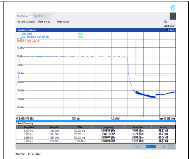
1-N77-3700-3980-PC1-30-30-H-3-DFT-PI2BPSK- Outer_Full-75@0-Ant0-1--PASS-see graph
