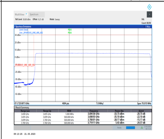
1-N77-3700-3980-PC1-30-60-L-6-CP-QPSK-Outer_Full-162@0-Ant0-1--PASS-see graph
