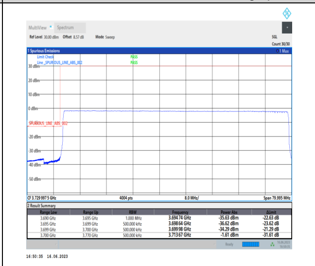
1-N77-3700-3980-PC1-30-70-L-6-CP-QPSK-Outer_Full-189@0-Ant0-1--PASS-see graph
