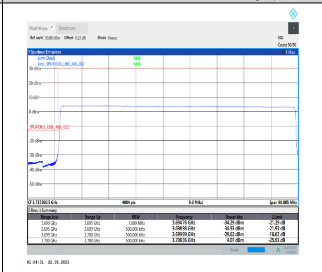
1-N77-3700-3980-PC1-30-80-L-6-CP-QPSK-Outer_Full-217@0-Ant0-1--PASS-see graph
