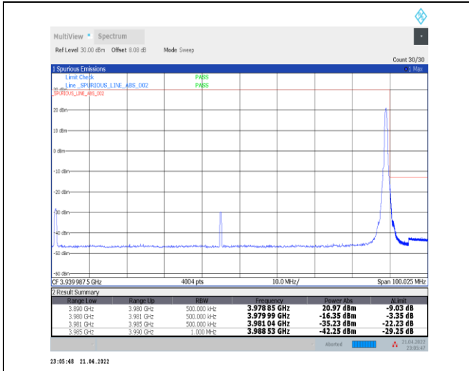
1-N77-3700-3980--30-90-H-2-DFT-PI2BPSK-Edge_1R_B_Right-1@244-Ant0-PASS-see graph
