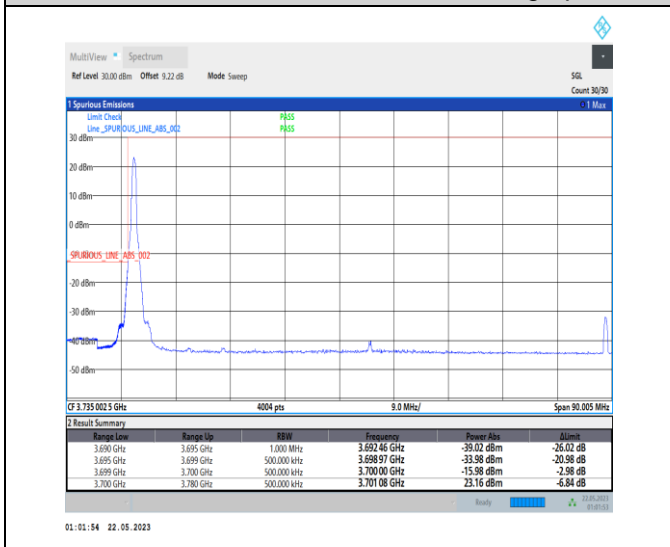
1-N77-3700-3980-PC1-30-80-L-4-CP-QPSK-Edge_1_RB_Left-1@0-Ant0-1--PASS-see graph
