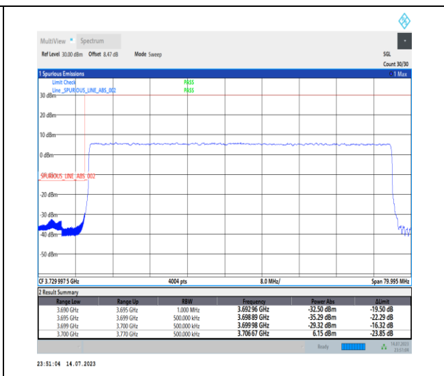
1-N77-3700-3980-PC1-30-70-L-3-DFT-PI2BPSK-Outer_Full-180@0-Ant0-1--PASS-see graph
