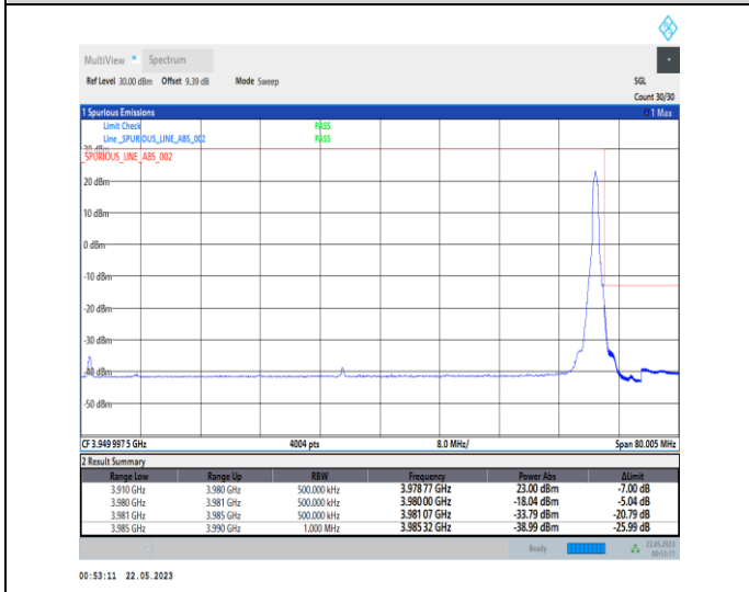
1-N77-3700-3980-PC1-30-70-H-5-CP-QPSK-Edge_1R B_Right-1@188-Ant0-1--PASS-see graph
