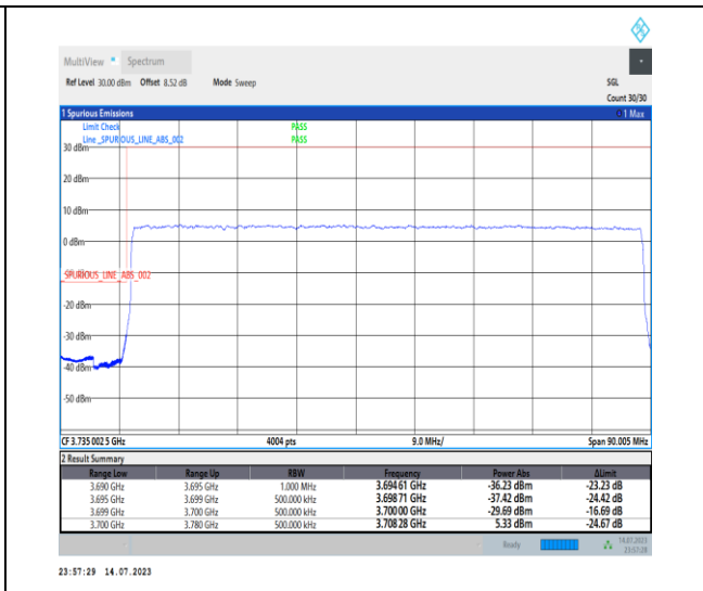
1-N77-3700-3980-PC1-30-80-L-3-DFT-PI2BPSK-Outer_Full-216@0-Ant0-1--PASS-see graph
