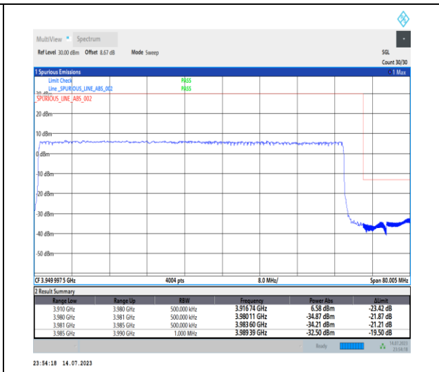
1-N77-3700-3980-PC1-30-70-H-3-DFT-PI2BPSK- Outer_Full-180@0-Ant0-1--PASS-see graph
