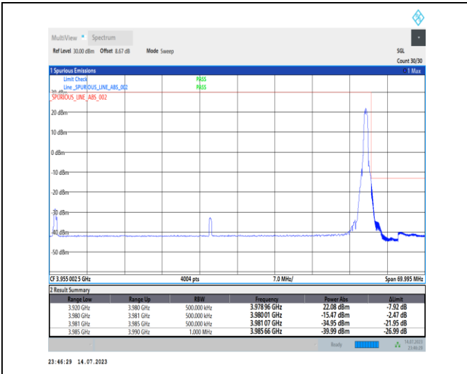
1-N77-3700-3980-PC1-30-60-H-2-DFT-PI2BPSK-Edge _1RB_Right-1@161-Ant0-1--PASS-see graph
