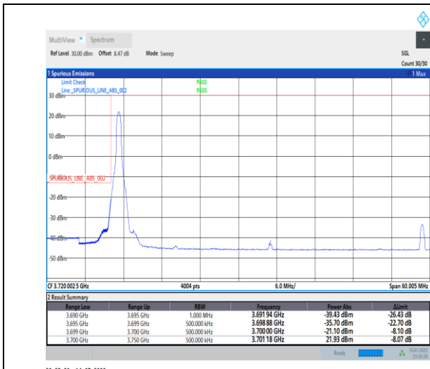
1-N77-3700-3980-PC1-30-50-L-1-DFT-PI2BPSK-Edge_1_RB_Left-1@0-Ant0-1--PASS-see graph
