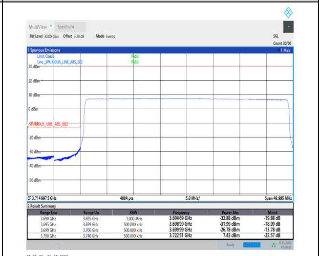
1-N77-3700-3980-PC1-30-40-L-6-CP-QPSK-Outer_Full-106@0-Ant0-1--PASS-see graph
