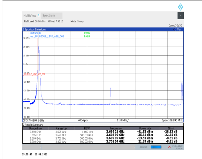
1-N77-3700-3980--30-100-L-4-CP-QPSK-Edge_1RB_Left-1@0-Ant0-PASS-see graph
