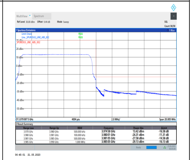
1-N77-3700-3980-PC1-30-10-H-6-CP-QPSK-Outer _Full-24@0-Ant0-1--PASS-see graph
