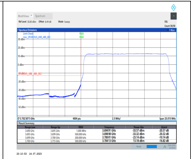
1-N77-3700-3980-PC1-30-15-L-3-DFT-PI2BPSK-Outer_Full-36@0-Ant0-1--PASS-see graph
