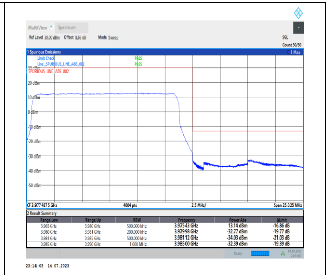
1-N77-3700-3980-PC1-30-15-H-3-DFT-PI2BPSK-Outer_Full-36@0-Ant0-1--PASS-see graph
