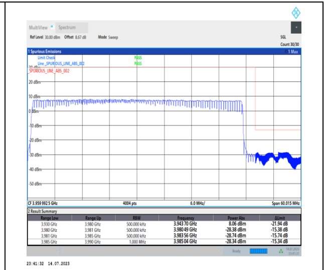
1-N77-3700-3980-PC1-30-50-H-3-DFT-PI2BPSK- Outer_Full-128@0-Ant0-1--PASS-see graph
