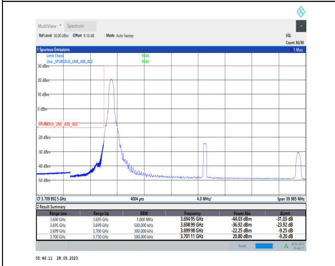
1-N77-3700-3980-PC1-30-30-L-4-CP-QPSK-Edge_1RB_Left-1@0-Ant0-1--PASS-see graph
