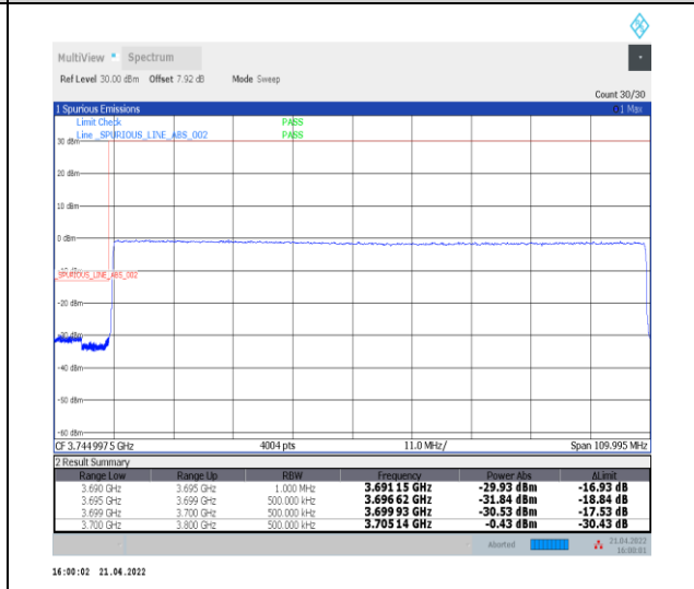
1-N77-3700-3980--30-100-L-6-CP-QPSK-Outer_F ull-273@0-Ant0-PASS-see graph
