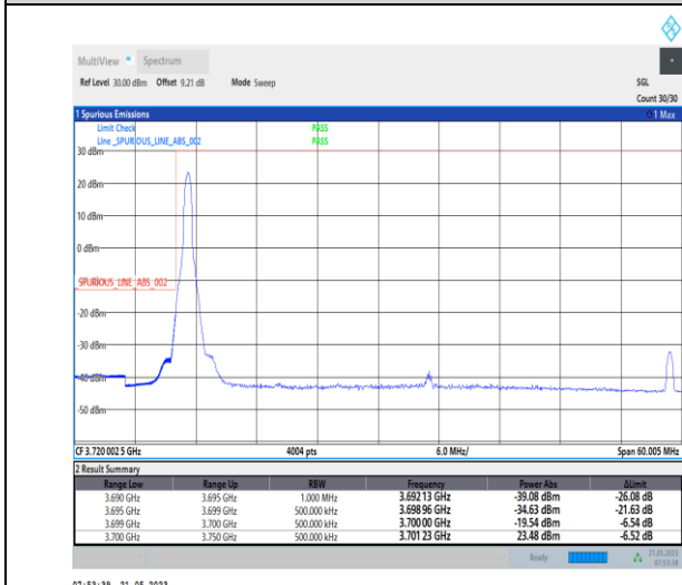
1-N77-3700-3980-PC1-30-50-L-4-CP-QPSK-Edge_1_RB_Left-1@0-Ant0-1--PASS-see graph
