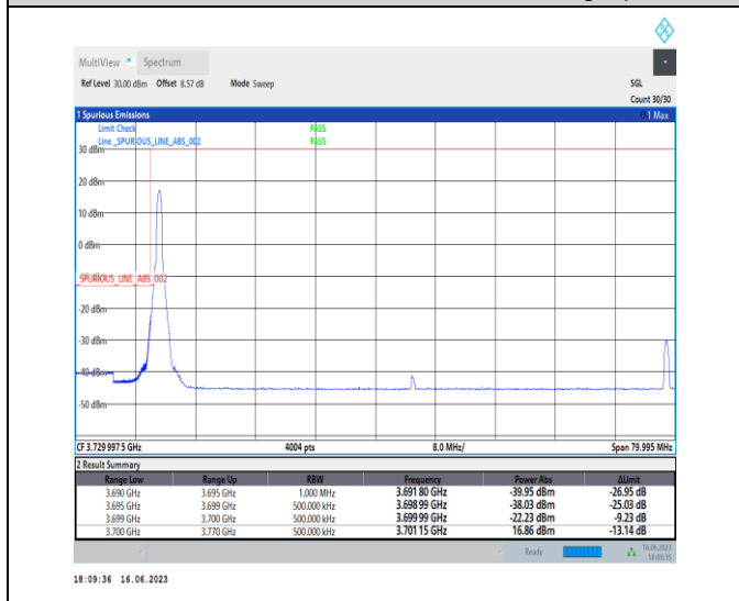
1-N77-3700-3980-PC1-30-70-L-4-CP-QPSK-Edge_1_RB_Left-1@0-Ant0-1--PASS-see graph
