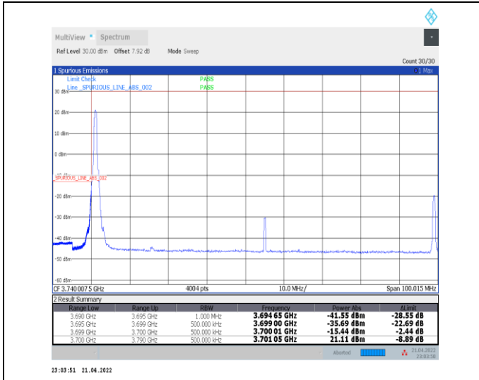
1-N77-3700-3980--30-90-L-1-DFT-PI2BPSK-Edge_1R_B_Left-1@0-Ant0-PASS-see graph
