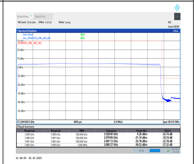
1-N77-3700-3980-PC1-30-80-H-6-CP-QPSK-Outer _Full-217@0-Ant0-1--PASS-see graph
