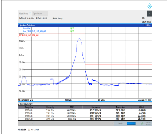
1-N77-3700-3980-PC1-30-10-H-5-CP-QPSK-Edge_1R B_Right-1@23-Ant0-1--PASS-see graph
