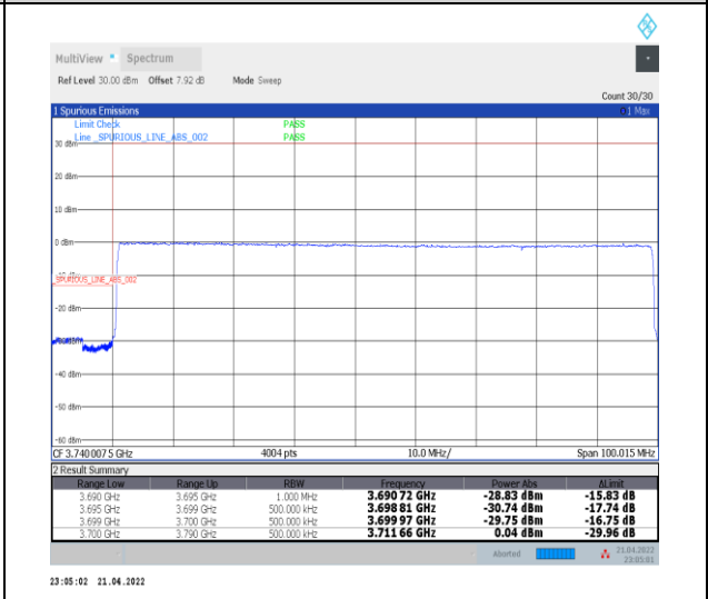
1-N77-3700-3980--30-90-L-6-CP-QPSK-Outer_FulI-245@0-Ant0-PASS-see graph
