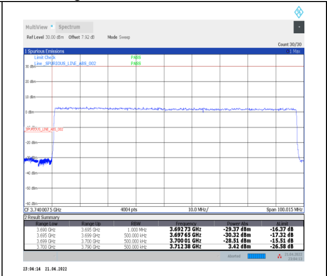
1-N77-3700-3980--30-90-L-3-DFT-PI2BPSK-Outer_Full-240@0-Ant0-PASS-see graph
