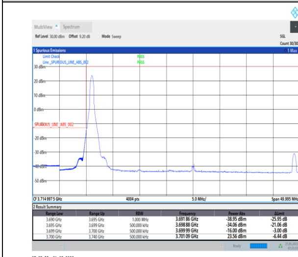
1-N77-3700-3980-PC1-30-40-L-4-CP-QPSK-Edge_1_RB_Left-1@0-Ant0-1--PASS-see graph
