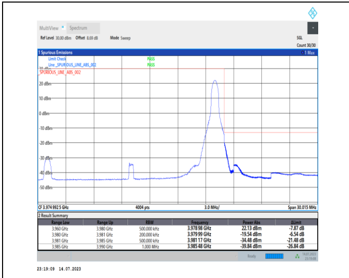
1-N77-3700-3980-PC1-30-20-H-2-DFT-PI2BPSK-Edge_1RB_Right-1@50-Ant0-1--PASS-see graph
