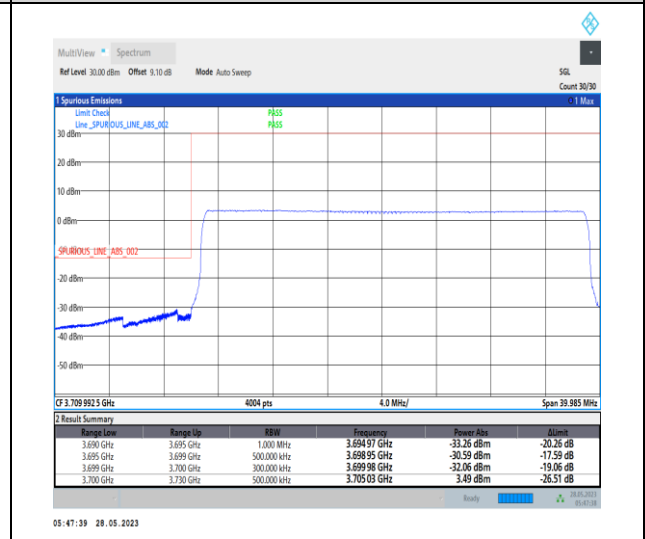
1-N77-3700-3980-PC1-30-30-L-6-CP-QPSK-Outer_Full-78@0-Ant0-1--PASS-see graph
