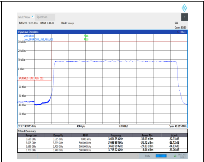
1-N77-3700-3980-PC1-30-40-L-3-DFT-PI2BPSK-Outer_Full-100@0-Ant0-1--PASS-see graph
