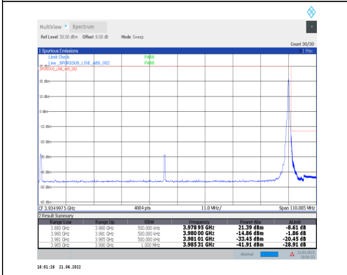
1-N77-3700-3980--30-100-H-5-CP-QPSK-Edge_1RB_Right-1@272-Ant0-PASS-see graph
