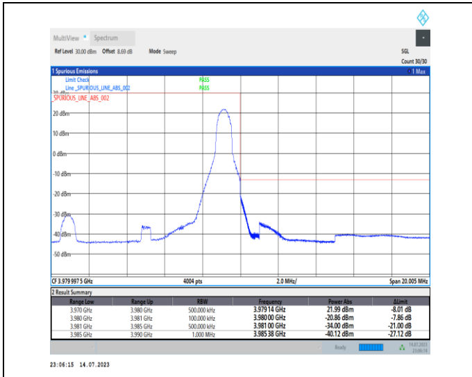
1-N77-3700-3980-PC1-30-10-H-2-DFT-PI2BPSK-Edge _1RB_Right-1@23-Ant0-1--PASS-see graph
