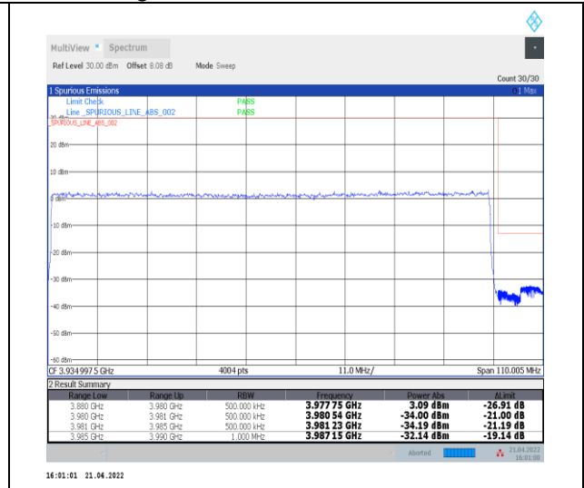
1-N77-3700-3980--30-100-H-3-DFT-PI2BPSK-Outer_Full-270@0-Ant0-PASS-see graph
