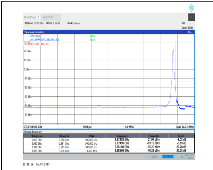
1-N77-3700-3980-PC1-30-80-H-2-DFT-PI2BPSK-Edge _1RB_Right-1@216-Ant0-1--PASS-see graph
