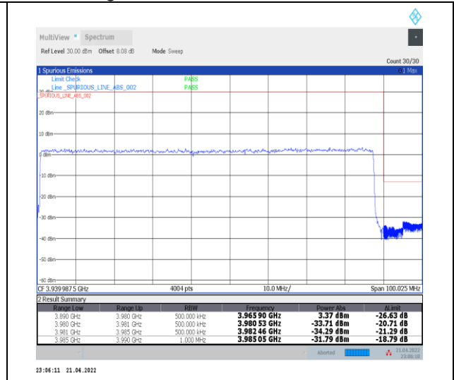
1-N77-3700-3980--30-90-H-3-DFT-PI2BPSK-Outer_Full-240@0-Ant0-PASS-see graph
