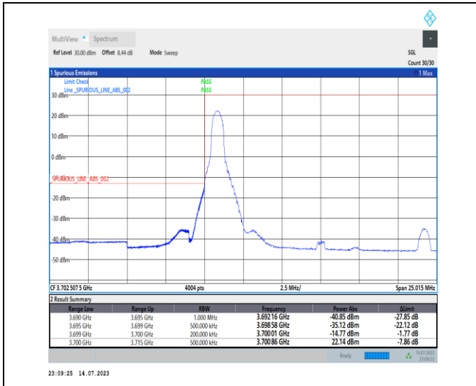
1-N77-3700-3980-PC1-30-15-L-1-DFT-PI2BPSK-Edge_1RB_Left-1@0-Ant0-1--PASS-see graph
