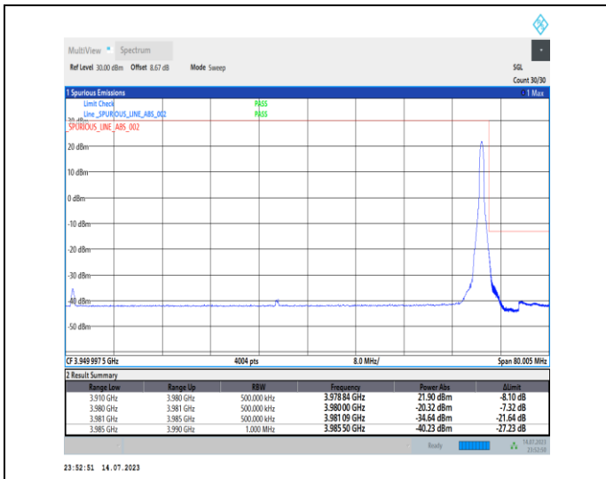
1-N77-3700-3980-PC1-30-70-H-2-DFT-PI2BPSK-Edge _1RB_Right-1@188-Ant0-1--PASS-see graph
