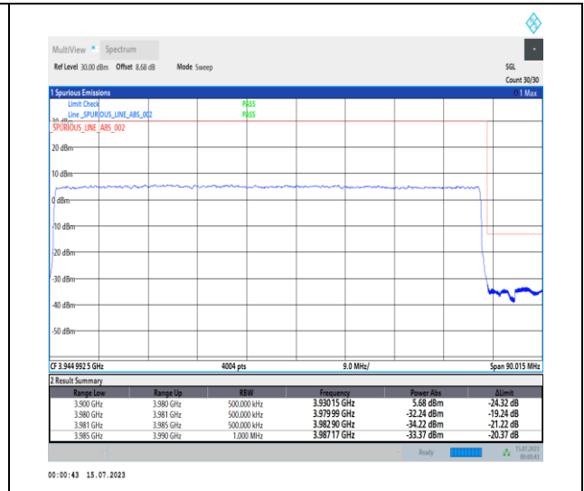
1-N77-3700-3980-PC1-30-80-H-3-DFT-PI2BPSK- Outer_Full-216@0-Ant0-1--PASS-see graph
