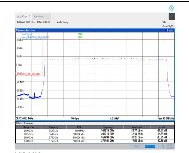
1-N77-3700-3980-PC1-30-50-L-3-DFT-PI2BPSK-Outer_Full-128@0-Ant0-1--PASS-see graph
