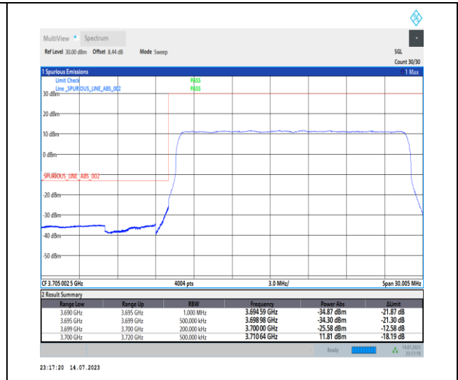
1-N77-3700-3980-PC1-30-20-L-3-DFT-PI2BPSK-Outer_Full-50@0-Ant0-1--PASS-see graph
