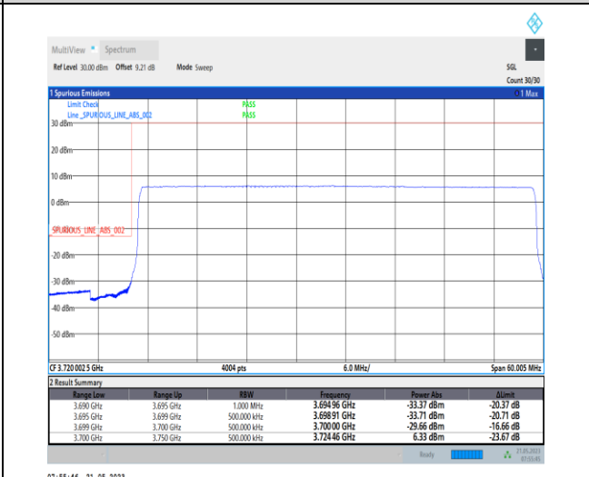
1-N77-3700-3980-PC1-30-50-L-6-CP-QPSK-Outer_Full-133@0-Ant0-1--PASS-see graph
