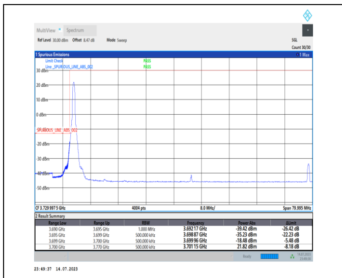
1-N77-3700-3980-PC1-30-70-L-1-DFT-PI2BPSK-Edge_1_RB_Left-1@0-Ant0-1--PASS-see graph
