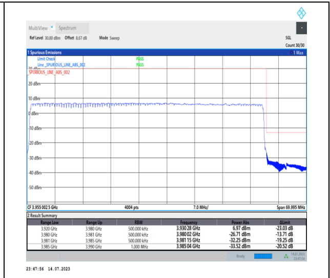
1-N77-3700-3980-PC1-30-60-H-3-DFT-PI2BPSK- Outer_Full-162@0-Ant0-1--PASS-see graph
