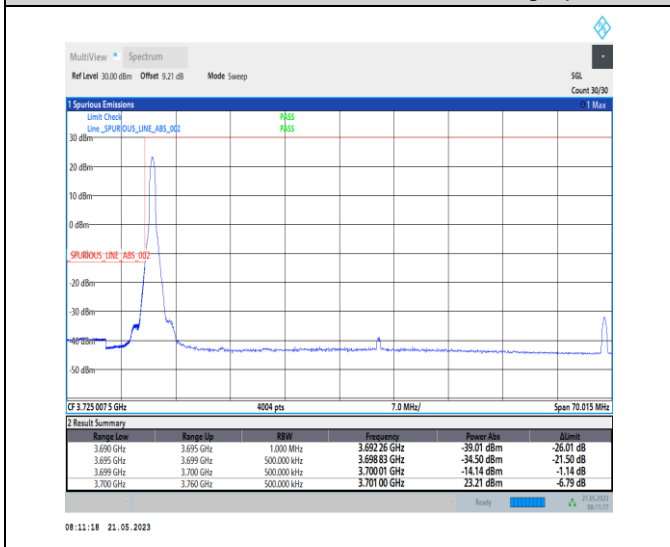
1-N77-3700-3980-PC1-30-60-L-4-CP-QPSK-Edge_1_RB_Left-1@0-Ant0-1--PASS-see graph
