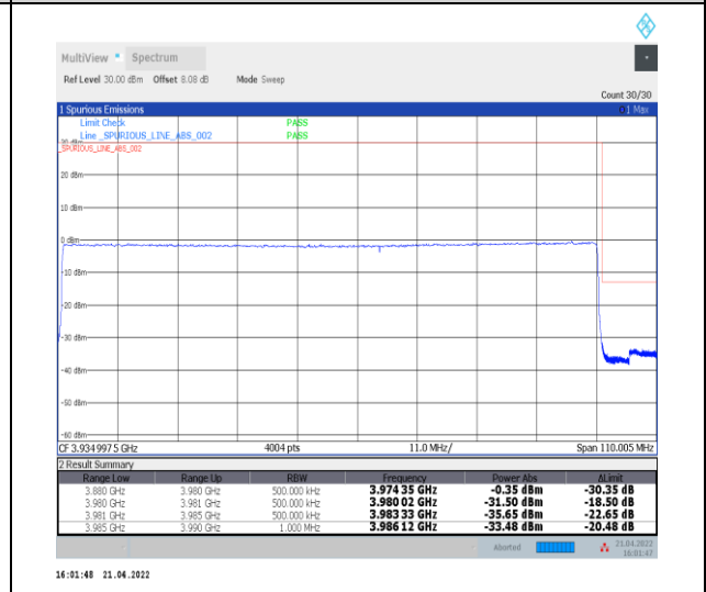
1-N77-3700-3980--30-100-H-6-CP-QPSK-Outer_Full-273@0-Ant0-PASS-see graph
