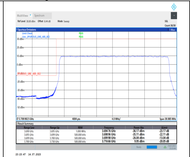
1-N77-3700-3980-PC1-30-30-L-3-DFT-PI2BPSK-Outer_Full-75@0-Ant0-1--PASS-see graph
