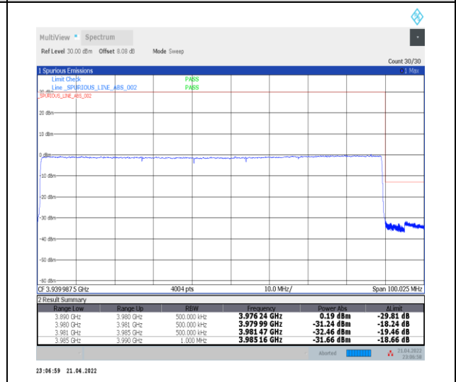
1-N77-3700-3980--30-90-H-6-CP-QPSK-Outer_Full-245@0-Ant0-PASS-see graph
