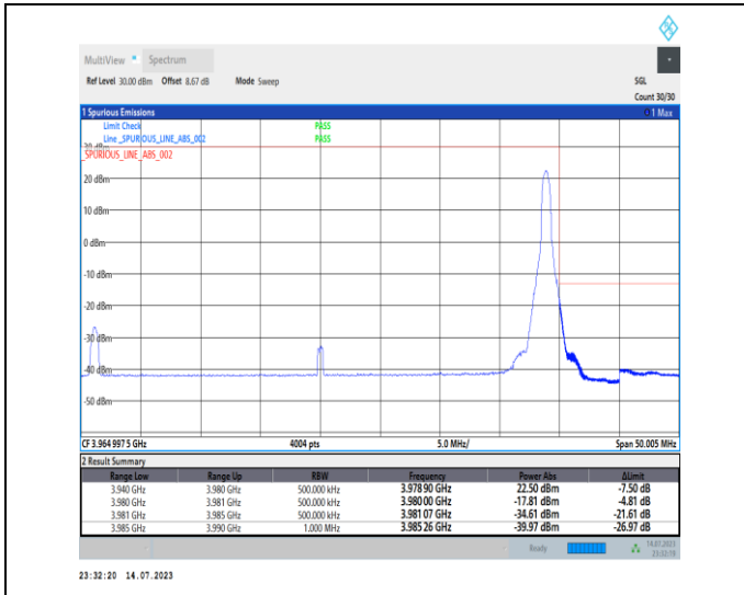
1-N77-3700-3980-PC1-30-40-H-2-DFT-PI2BPSK-Edge _1RB_Right-1@105-Ant0-1--PASS-see graph
