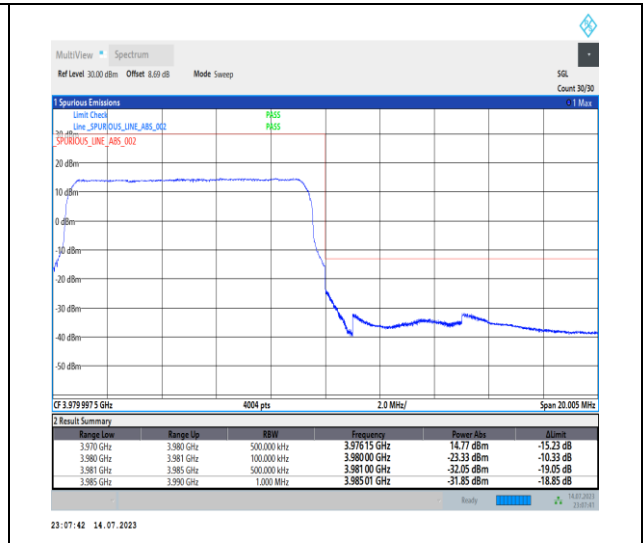
1-N77-3700-3980-PC1-30-10-H-3-DFT-PI2BPSK- Outer_Full-24@0-Ant0-1--PASS-see graph
