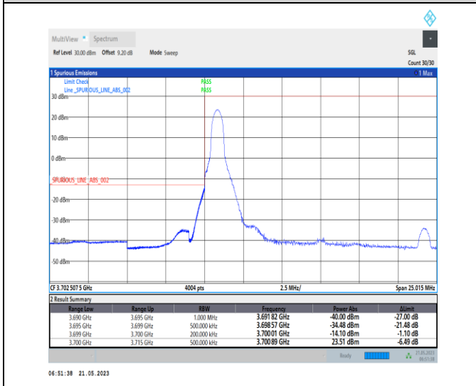
1-N77-3700-3980-PC1-30-15-L-4-CP-QPSK-Edge_1RB_Left-1@0-Ant0-1--PASS-see graph
