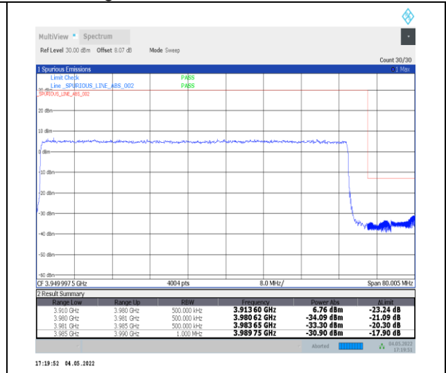
1-N77-3700-3980--30-70-H-3-DFT-PI2BPSK-Outer_Full-180@0-Ant0-PASS-see graph
