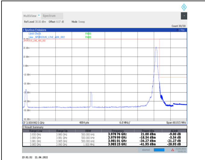
1-N77-3700-3980--30-50-H-2-DFT-PI2BPSK-Edge_1R_B_Right-1@132-Ant0-PASS-see graph
