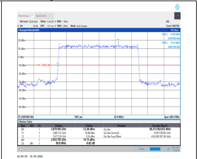
1-N77-3700-3980-PC1-30-100-H-2-DFT-PI2BPSK-Outer_Full-270@0-Ant0-96.313-99.800-≤100-PASS
