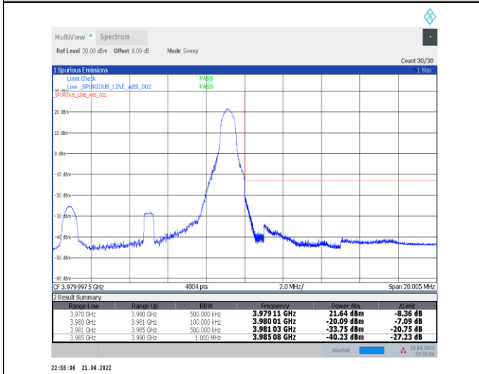
1-N77-3700-3980--30-10-H-5-CP-QPSK-Edge_1RB_Right-1@23-Ant0-PASS-see graph
