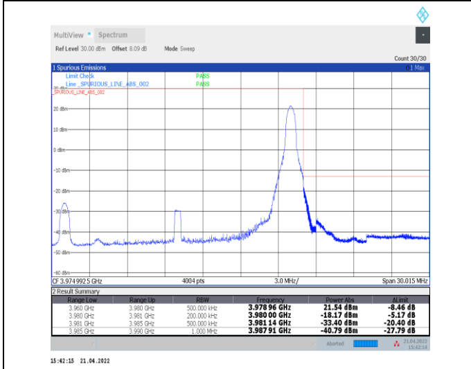
1-N77-3700-3980--30-20-H-5-CP-QPSK-Edge_1RB_Right-1@50-Ant0-PASS-see graph
