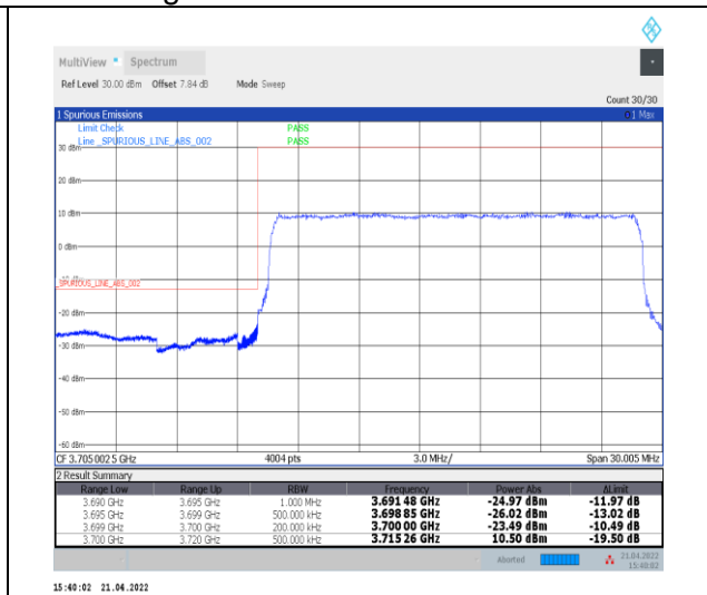
1-N77-3700-3980--30-20-L-3-DFT-PI2BPSK-Outer_Full-50@0-Ant0-PASS-see graph
