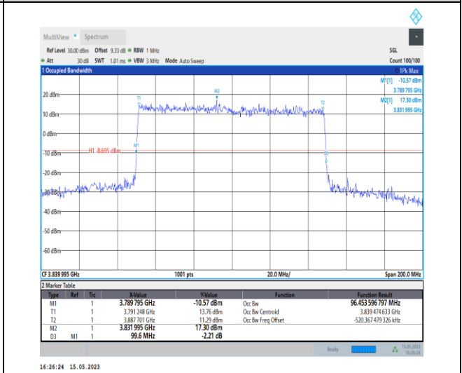
1-N77-3700-3980-PC1-30-100-M-1-DFT-QPSK-Outer_Full-270@0-Ant0-96.454-99.600-≤100-PASS
