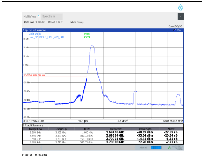
1-N77-3700-3980--30-15-L-1-DFT-PI2BPSK-Edge_1R_B_Left-1@0-Ant0-PASS-see graph
