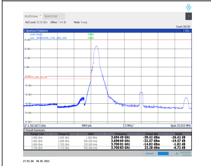
1-N77-3700-3980--30-15-L-4-CP-QPSK-Edge_1RB_L_eff-1@0-Ant0-PASS-see graph
