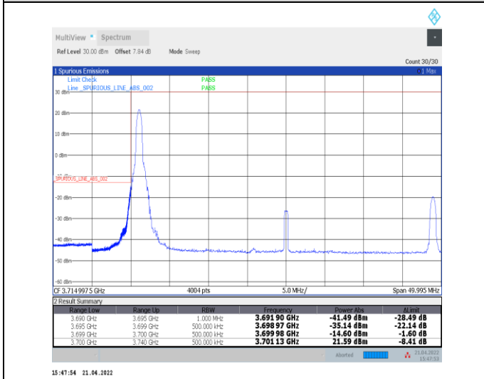
1-N77-3700-3980--30-40-L-4-CP-QPSK-Edge_1RB_L_eff-1@0-Ant0-PASS-see graph
