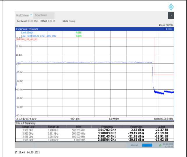
1-N77-3700-3980--30-70-H-6-CP-QPSK-Outer_Full-189@0-Ant0-PASS-see graph
