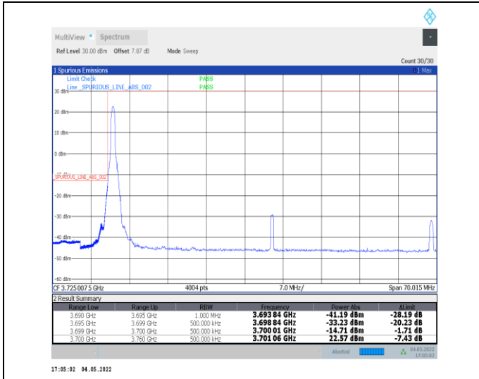
1-N77-3700-3980--30-60-L-1-DFT-PI2BPSK-Edge_1R_B_Left-1@0-Ant0-PASS-see graph
