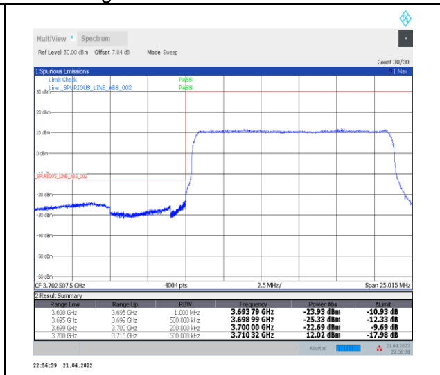
1-N77-3700-3980--30-15-L-3-DFT-PI2BPSK-Outer_Full-36@0-Ant0-PASS-see graph
