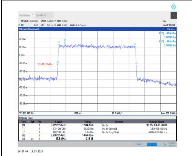
1-N77-3700-3980-PC1-30-100-M-4-DFT-64QAM-Outer_Full-270@0-Ant0-96.283-99.800-≤100-PASS
