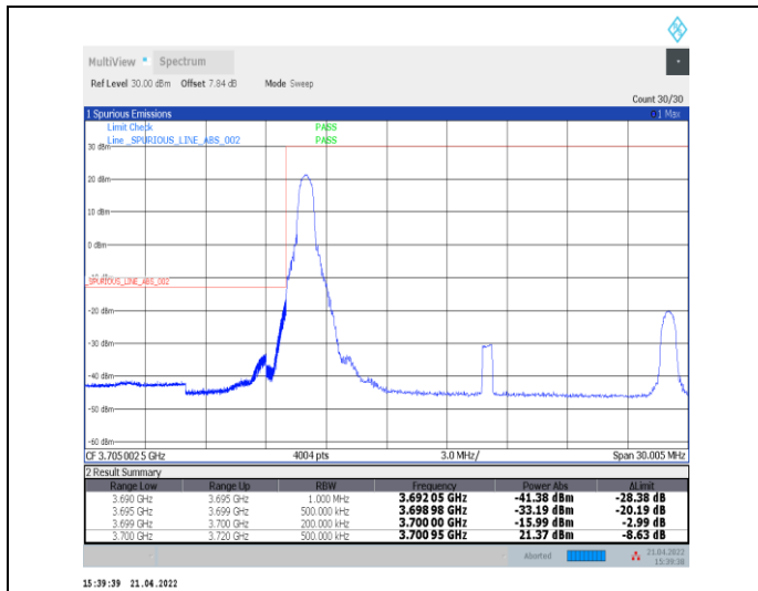
1-N77-3700-3980--30-20-L-1-DFT-PI2BPSK-Edge_1R_B_Left-1@0-Ant0-PASS-see graph
