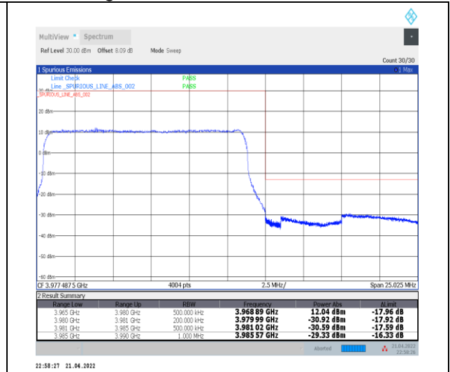
1-N77-3700-3980--30-15-H-3-DFT-PI2BPSK-Outer_Full-36@0-Ant0-PASS-see graph
