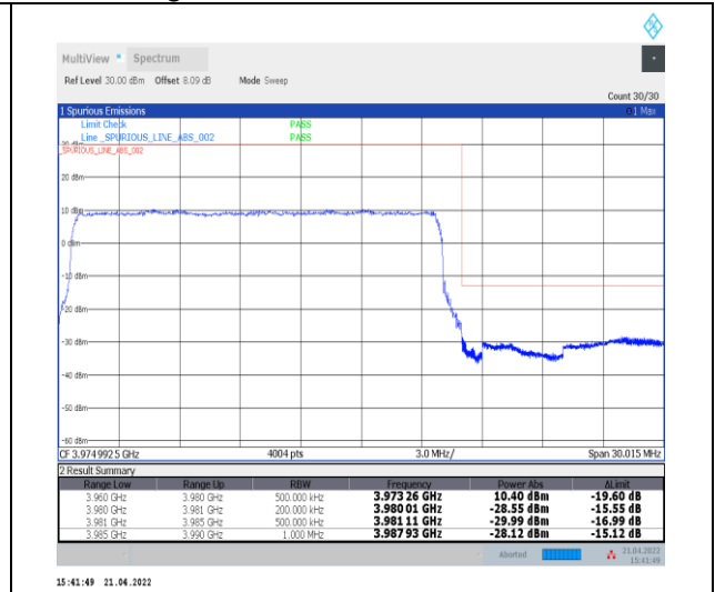
1-N77-3700-3980--30-20-H-3-DFT-PI2BPSK-Outer_Full-50@0-Ant0-PASS-see graph
