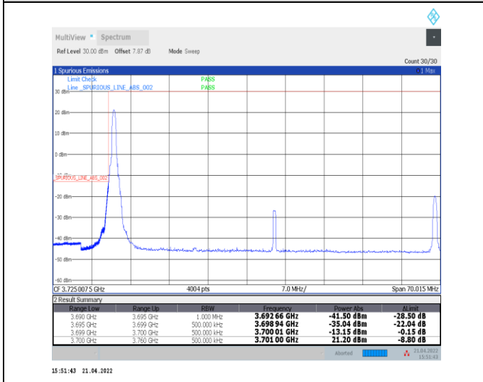
1-N77-3700-3980--30-60-L-4-CP-QPSK-Edge_1RB_L_eff-1@0-Ant0-PASS-see graph
