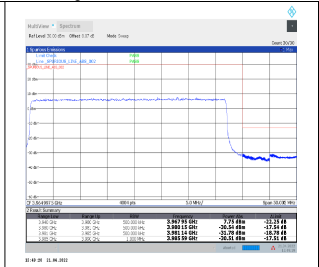
1-N77-3700-3980--30-40-H-3-DFT-PI2BPSK-Outer_Full-100@0-Ant0-PASS-see graph
