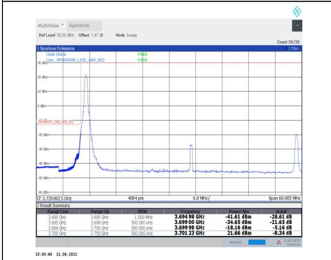
1-N77-3700-3980--30-50-L-4-CP-QPSK-Edge_1RB_L_eff-1@0-Ant0-PASS-see graph
