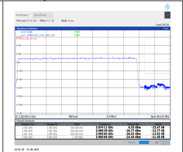
1-N77-3700-3980--30-50-H-3-DFT-PI2BPSK-Outer_Full-128@0-Ant0-PASS-see graph
