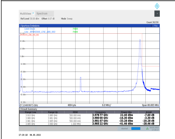
1-N77-3700-3980--30-70-H-5-CP-QPSK-Edge_1RB_Right-1@188-Ant0-PASS-see graph
