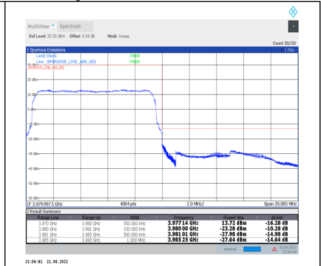
1-N77-3700-3980--30-10-H-3-DFT-PI2BPSK-Outer_Full-24@0-Ant0-PASS-see graph
