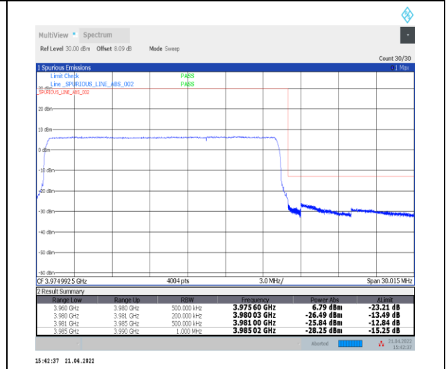
1-N77-3700-3980--30-20-H-6-CP-QPSK-Outer_Full-51@0-Ant0-PASS-see graph
