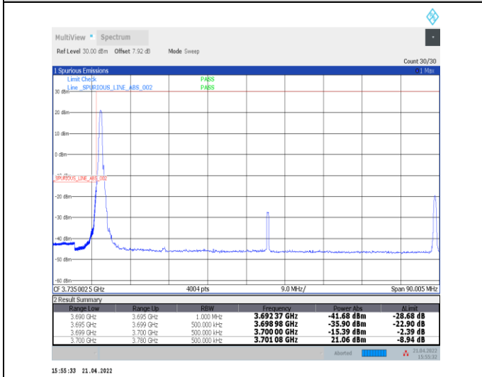
1-N77-3700-3980--30-80-L-4-CP-QPSK-Edge_1RB_L_eff-1@0-Ant0-PASS-see graph
