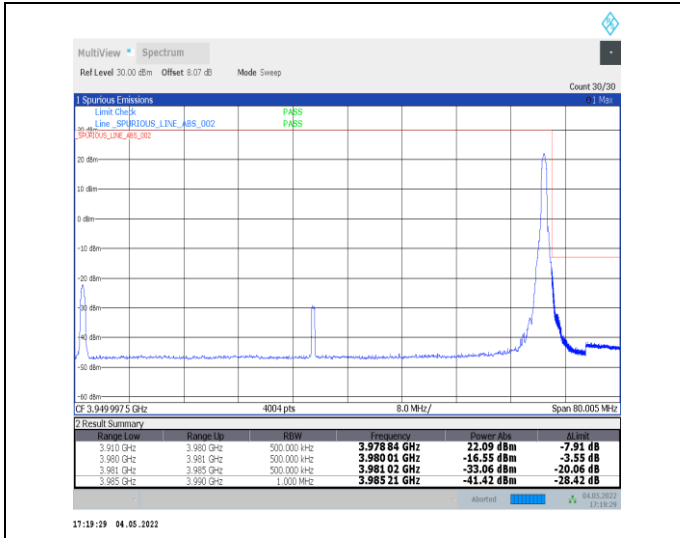
1-N77-3700-3980--30-70-H-2-DFT-PI2BPSK-Edge_1R_B_Right-1@188-Ant0-PASS-see graph
