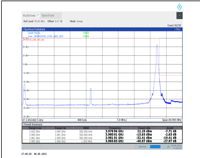
1-N77-3700-3980--30-60-H-2-DFT-PI2BPSK-Edge_1R_B_Right-1@161-Ant0-PASS-see graph
