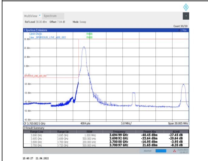
1-N77-3700-3980--30-20-L-4-CP-QPSK-Edge_1RB_L_eft-1@0-Ant0-PASS-see graph
