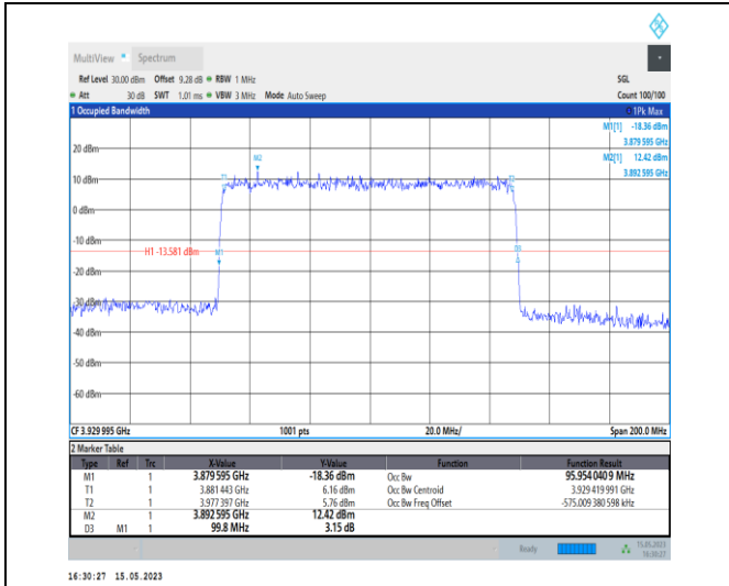
1-N77-3700-3980-PC1-30-100-H-5-DFT-256QAM-Outer_Full-270@0-Ant0-95.954-99.800-≤100-PASS
