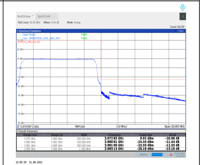
1-N77-3700-3980--30-10-H-6-CP-QPSK-Outer_Full-24@0-Ant0-PASS-see graph
