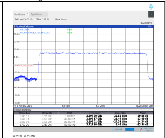
1-N77-3700-3980--30-50-L-3-DFT-PI2BPSK-Outer_Full-128@0-Ant0-PASS-see graph
