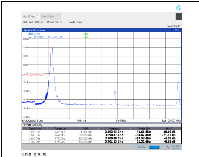
1-N77-3700-3980--30-50-L-1-DFT-PI2BPSK-Edge_1R_B_Left-1@0-Ant0-PASS-see graph
