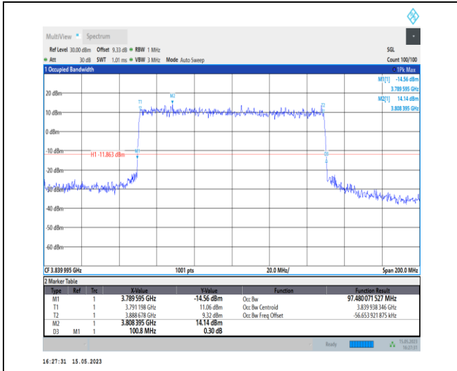
1-N77-3700-3980-PC1-30-100-M-6-CP-QPSK-Outer_Full-273@0-Ant0-97.48-100.800-≤100-PASS
