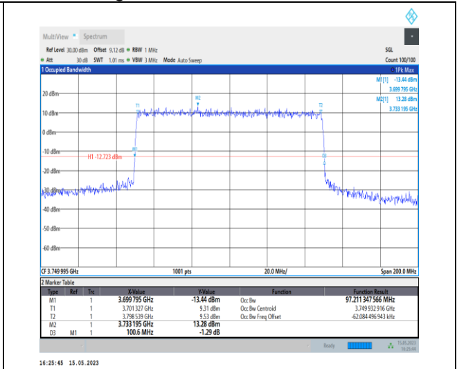
1-N77-3700-3980-PC1-30-100-L-8-CP-64QAM-Outer_Full-273@0-Ant0-97.211-100.600-≤100-PASS
