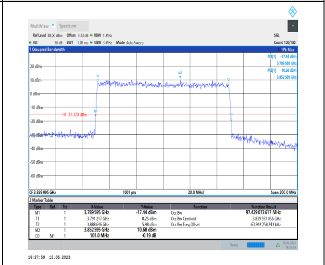
1-N77-3700-3980-PC1-30-100-M-9-CP-256QAM-Outer_Full-273@0-Ant0-97.429-101.000-≤100-PASS
