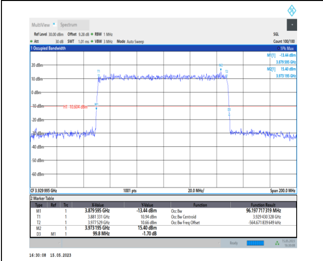
1-N77-3700-3980-PC1-30-100-H-3-DFT-16QAM-Outer_Full-270@0-Ant0-96.198-99.800-≤100-PASS
