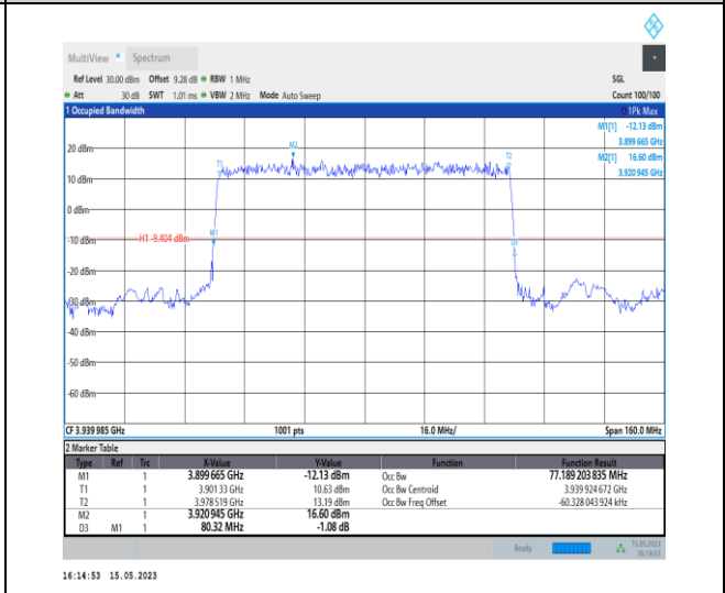
1-N77-3700-3980-PC1-30-80-H-2-DFT-PI2BPSK-Outer_Full-216@0-Ant0-77.189-80.320-≤80-PASS
