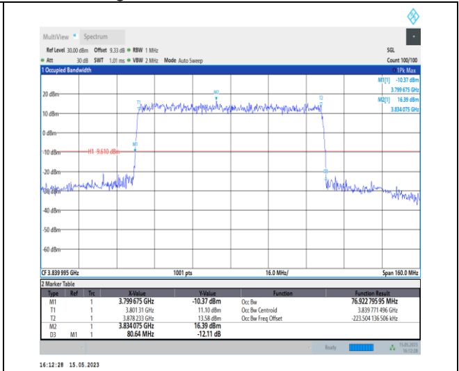
1-N77-3700-3980-PC1-30-80-M-1-DFT-QPSK-Outer_Full-216@0-Ant0-76.923-80.640-≤80-PASS
