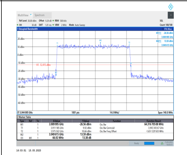
1-N77-3700-3980-PC1-30-70-H-1-DFT-QPSK-Outer _Full-180@0-Ant0-64.317-66.920-≤70-PASS
