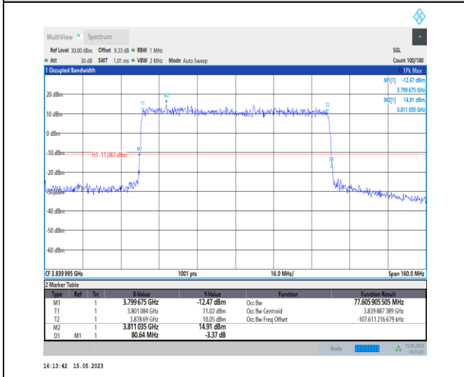
1-N77-3700-3980-PC1-30-80-M-6-CP-QPSK-Outer_Full-217@0-Ant0-77.606-80.640-≤80-PASS
