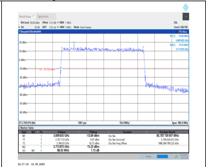
1-N77-3700-3980-PC1-30-90-L-3-DFT-16QAM-Out er_Full-240@0-Ant0-85.788-88.920-≤90-PASS
