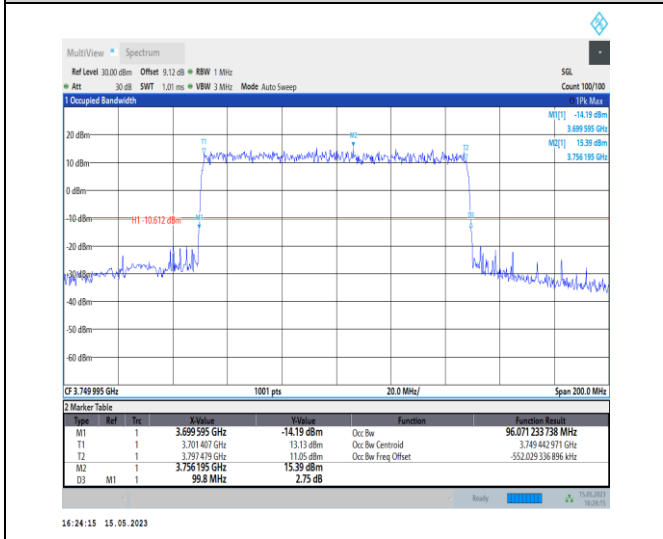
1-N77-3700-3980-PC1-30-100-L-1-DFT-QPSK-Outer_Full-270@0-Ant0-96.071-99.800-≤100-PASS
