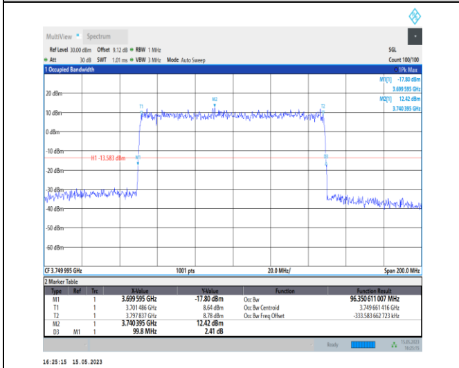
1-N77-3700-3980-PC1-30-100-L-5-DFT-256QAM-Out er_Full-270@0-Ant0-96.351-99.800-≤100-PASS
