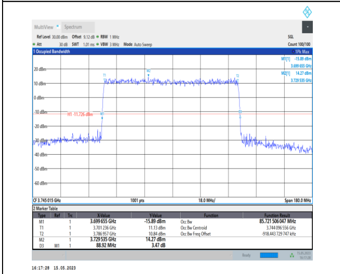
1-N77-3700-3980-PC1-30-90-L-4-DFT-64QAM-Out er_Full-240@0-Ant0-85.722-88.920-≤90-PASS
