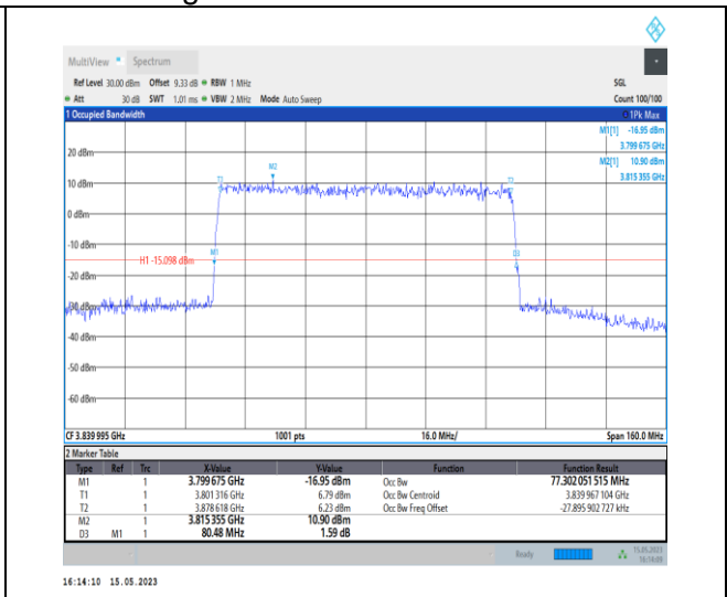
1-N77-3700-3980-PC1-30-80-M-9-CP-256QAM-Outer_Full-217@0-Ant0-77.302-80.480-≤80-PASS
