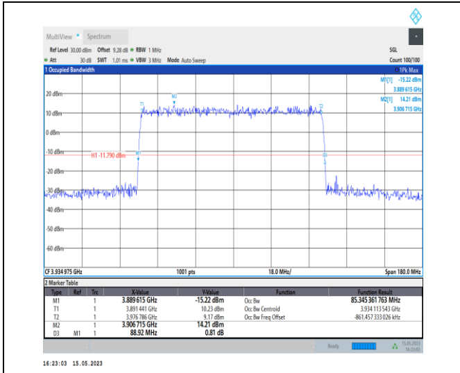
1-N77-3700-3980-PC1-30-90-H-4-DFT-64QAM-Outer_Full-240@0-Ant0-85.345-88.920-≤90-PASS
