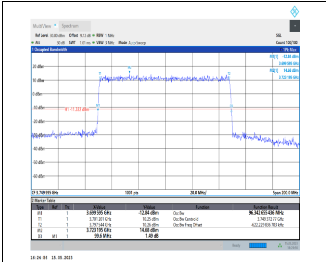
1-N77-3700-3980-PC1-30-100-L-3-DFT-16QAM-Out er_Full-270@0-Ant0-96.343-99.600-≤100-PASS
