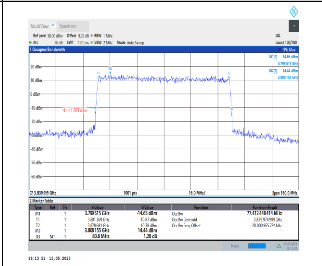
1-N77-3700-3980-PC1-30-80-M-7-CP-16QAM-Outer_Full-217@0-Ant0-77.412-80.800-≤80-PASS
