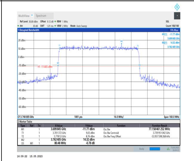
1-N77-3700-3980-PC1-30-80-L-8-CP-64QAM-Outer_Full-217@0-Ant0-77.158-80.480-≤80-PASS
