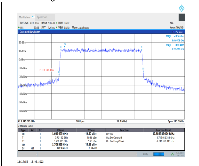
1-N77-3700-3980-PC1-30-90-L-7-CP-16QAM-Outer_Full-245@0-Ant0-87.385-90.900-≤90-PASS
