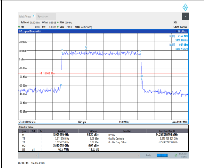
1-N77-3700-3980-PC1-30-70-H-5-DFT-256QAM-Out er_Full-180@0-Ant0-64.259-66.500-≤70-PASS
