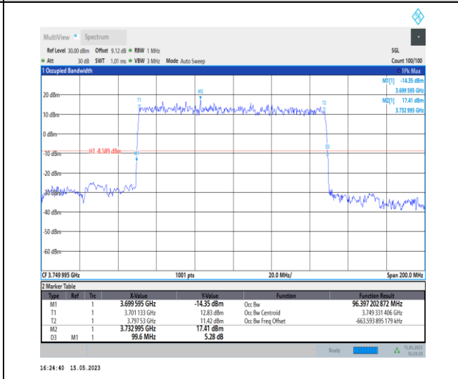
1-N77-3700-3980-PC1-30-100-L-2-DFT-PI2BPSK-Outer_Full-270@0-Ant0-96.397-99.600-≤100-PASS
