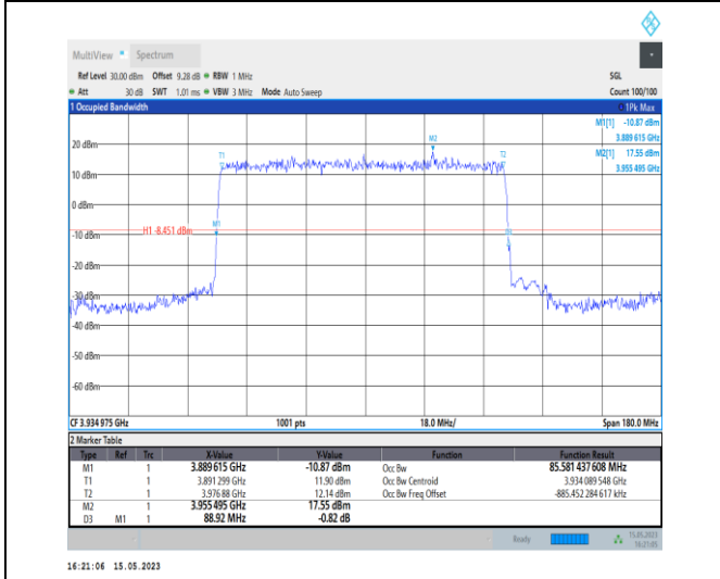
1-N77-3700-3980-PC1-30-90-H-2-DFT-PI2BPSK-Outer_Full-240@0-Ant0-85.581-88.920-≤90-PASS
