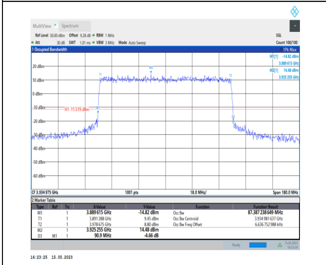
1-N77-3700-3980-PC1-30-90-H-6-CP-QPSK-Outer_Full-245@0-Ant0-87.387-90.900-≤90-PASS
