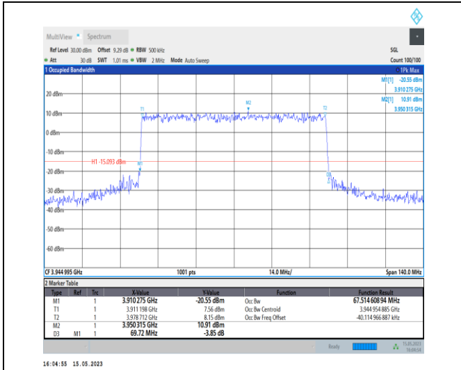
1-N77-3700-3980-PC1-30-70-H-6-CP-QPSK-Outer_Full-189@0-Ant0-67.515-69.720-≤70-PASS
