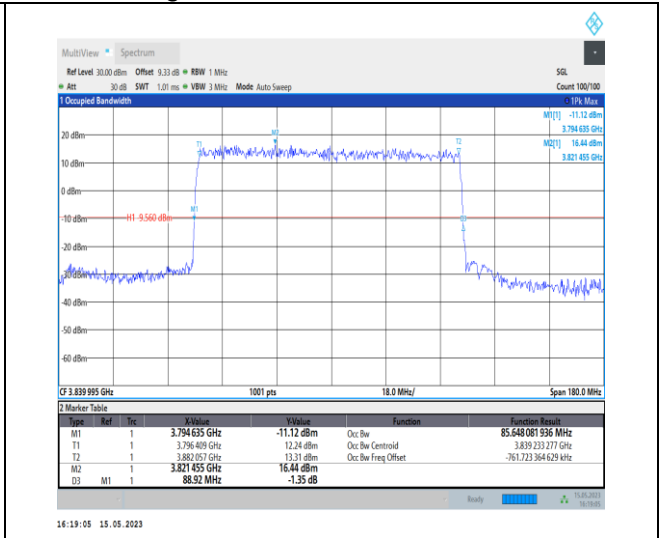
1-N77-3700-3980-PC1-30-90-M-2-DFT-PI2BPSK-Outer_Full-240@0-Ant0-85.648-88.920-≤90-PASS
