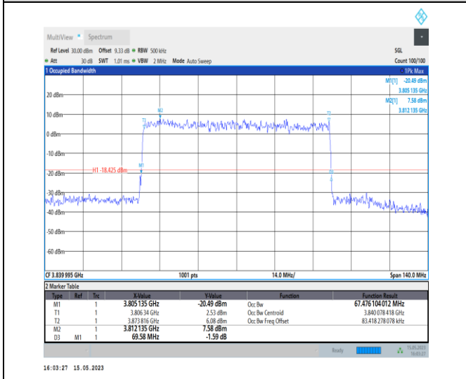
1-N77-3700-3980-PC1-30-70-M-9-CP-256QAM-Outer _Full-189@0-Ant0-67.476-69.580-≤70-PASS
