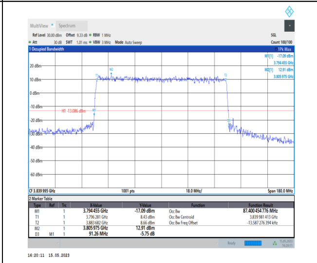
1-N77-3700-3980-PC1-30-90-M-8-CP-64QAM-Outer_Full-245@0-Ant0-87.4-91.260-≤90-PASS
