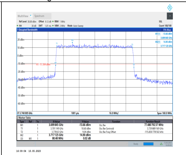
1-N77-3700-3980-PC1-30-80-L-6-CP-QPSK-Outer_Full-217@0-Ant0-77.481-80.480-≤80-PASS
