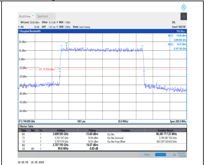
1-N77-3700-3980-PC1-30-100-L-4-DFT-64QAM-Out er_Full-270@0-Ant0-96.382-99.800-≤100-PASS
