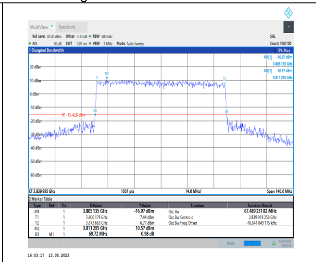
1-N77-3700-3980-PC1-30-70-M-8-CP-64QAM-Outer _Full-189@0-Ant0-67.489-69.720-≤70-PASS
