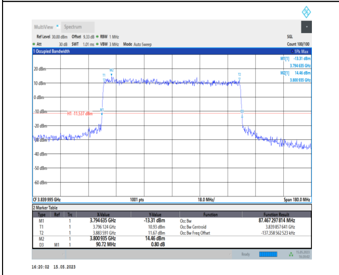
1-N77-3700-3980-PC1-30-90-M-7-CP-16QAM-Outer_Full-245@0-Ant0-87.467-90.720-≤90-PASS
