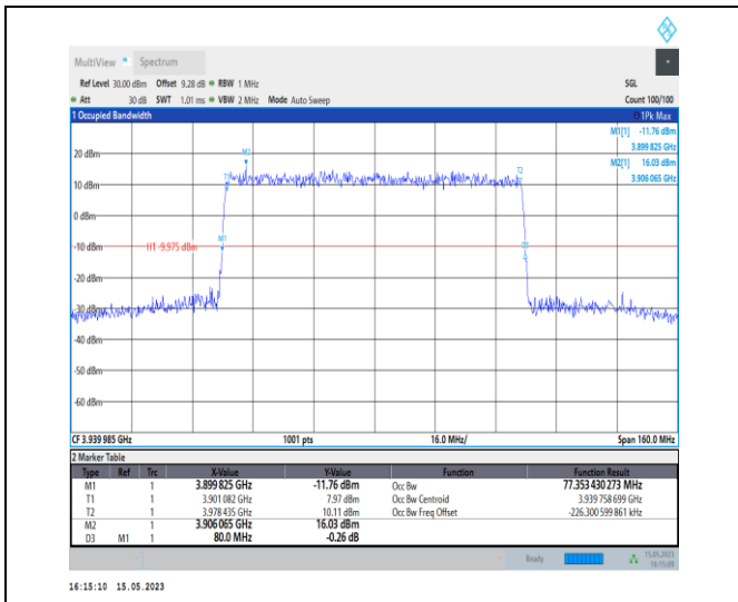
1-N77-3700-3980-PC1-30-80-H-3-DFT-16QAM-Outer_Full-216@0-Ant0-77.353-80.000-≤80-PASS
