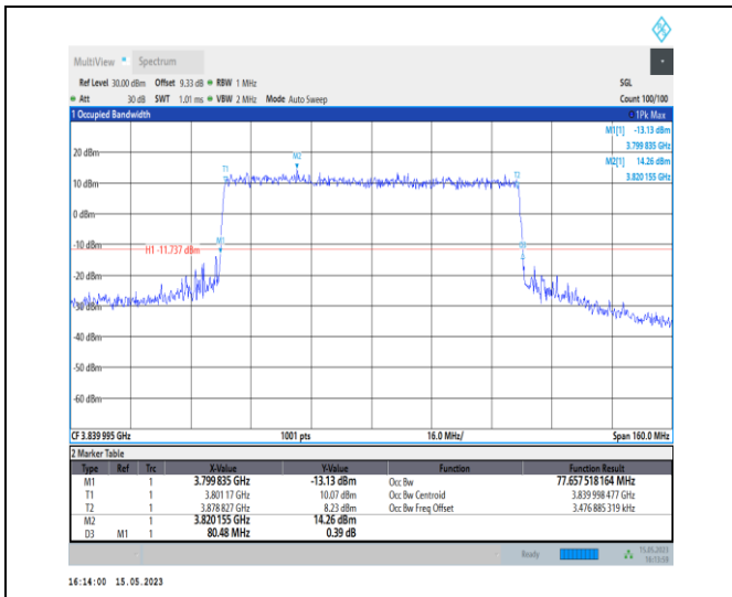
1-N77-3700-3980-PC1-30-80-M-8-CP-64QAM-Outer_Full-217@0-Ant0-77.658-80.480-≤80-PASS
