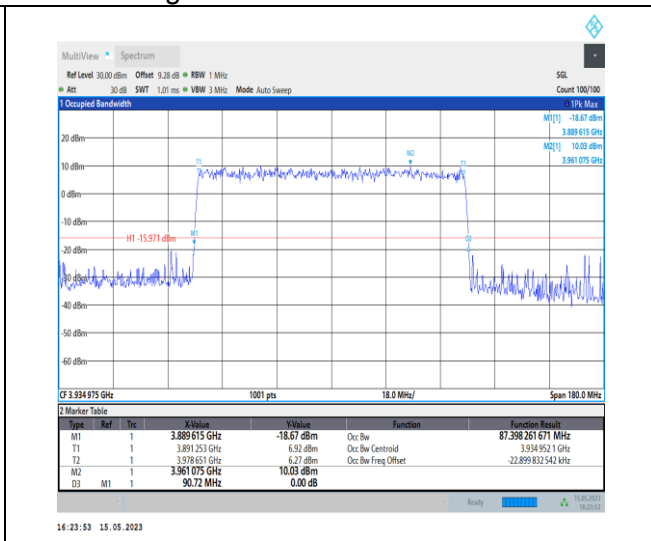
1-N77-3700-3980-PC1-30-90-H-9-CP-256QAM-Outer_Full-245@0-Ant0-87.398-90.720-≤90-PASS
