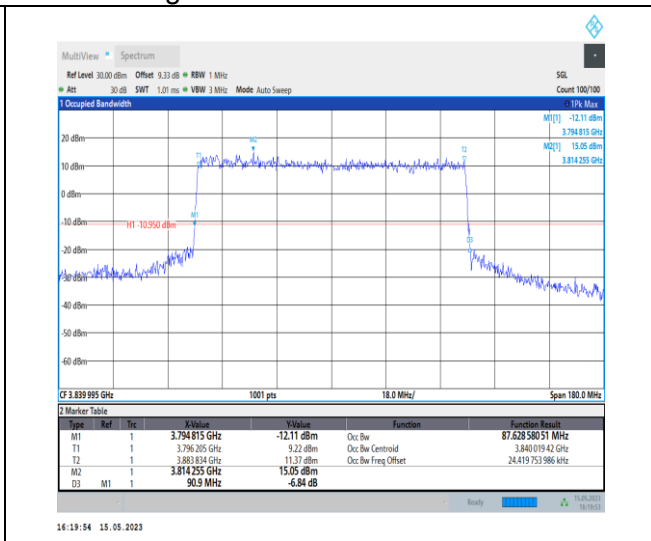
1-N77-3700-3980-PC1-30-90-M-6-CP-QPSK-Outer_Full-245@0-Ant0-87.629-90.900-≤90-PASS
