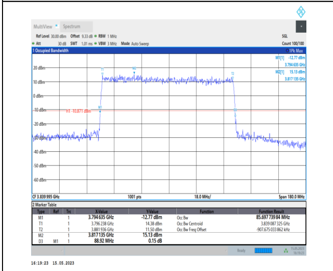
1-N77-3700-3980-PC1-30-90-M-3-DFT-16QAM-Outer_Full-240@0-Ant0-85.698-88.920-≤90-PASS
