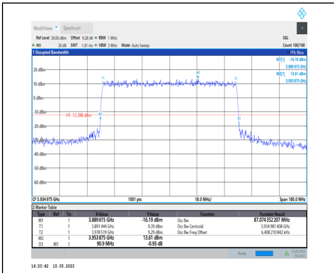
1-N77-3700-3980-PC1-30-90-H-8-CP-64QAM-Outer_Full-245@0-Ant0-87.074-90.900-≤90-PASS
