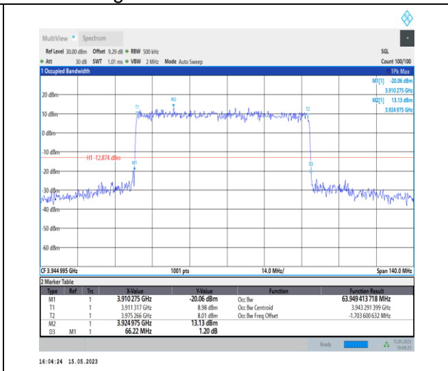
1-N77-3700-3980-PC1-30-70-H-3-DFT-16QAM-Out er_Full-180@0-Ant0-63.949-66.220-≤70-PASS
