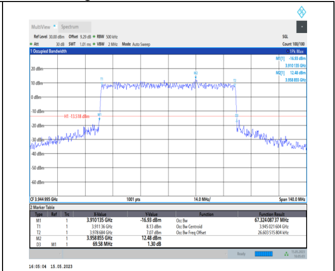
1-N77-3700-3980-PC1-30-70-H-7-CP-16QAM-Outer_Full-189@0-Ant0-67.324-69.580-≤70-PASS
