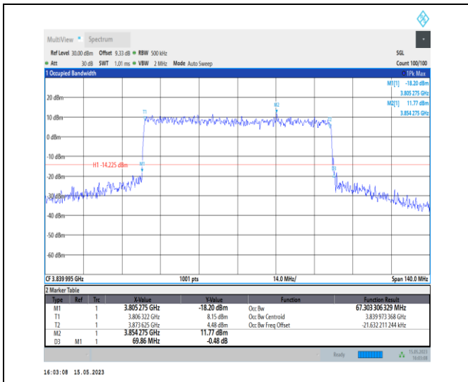
1-N77-3700-3980-PC1-30-70-M-7-CP-16QAM-Outer _Full-189@0-Ant0-67.303-69.860-≤70-PASS
