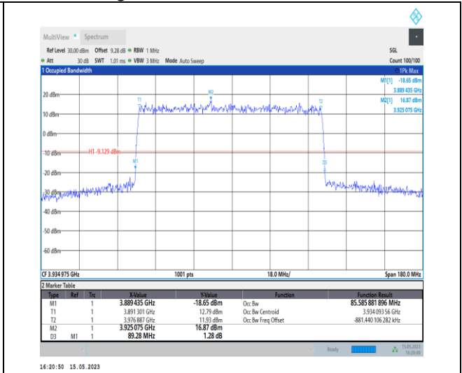
1-N77-3700-3980-PC1-30-90-H-1-DFT-QPSK-Outer_Full-240@0-Ant0-85.586-89.280-≤90-PASS
