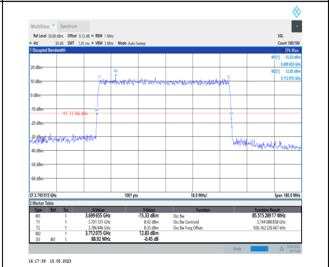
1-N77-3700-3980-PC1-30-90-L-5-DFT-256QAM-Out er_Full-240@0-Ant0-85.515-88.920-≤90-PASS
