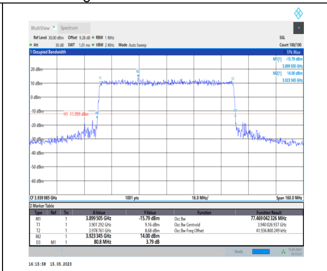
1-N77-3700-3980-PC1-30-80-H-8-CP-64QAM-Outer_Full-217@0-Ant0-77.469-80.800-≤80-PASS
