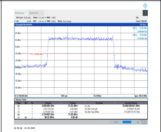
1-N77-3700-3980-PC1-30-80-L-4-DFT-64QAM-Outer_Full-216@0-Ant0-76.907-80.320-≤80-PASS
