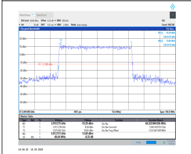
1-N77-3700-3980-PC1-30-70-H-4-DFT-64QAM-Out er_Full-180@0-Ant0-64.324-66.640-≤70-PASS
