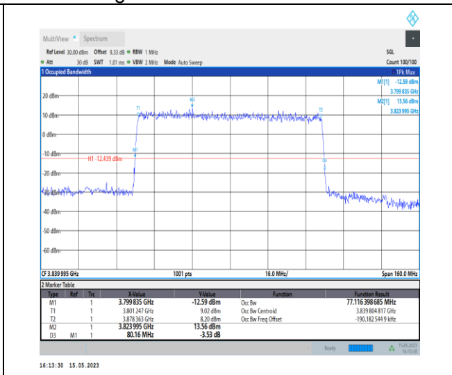
1-N77-3700-3980-PC1-30-80-M-5-DFT-256QAM-Outer_Full-216@0-Ant0-77.116-80.160-≤80-PASS
