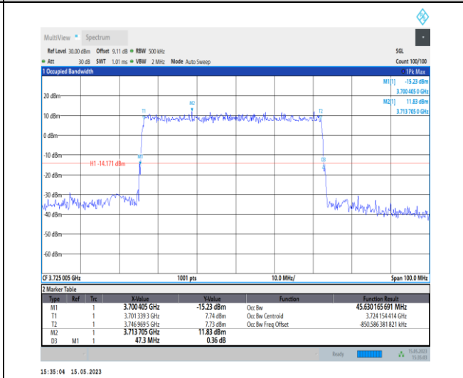
1-N77-3700-3980-PC1-30-50-L-5-DFT-256QAM-Out er_Full-128@0-Ant0-45.63-47.300-<math>\leq 50</math>-PASS
