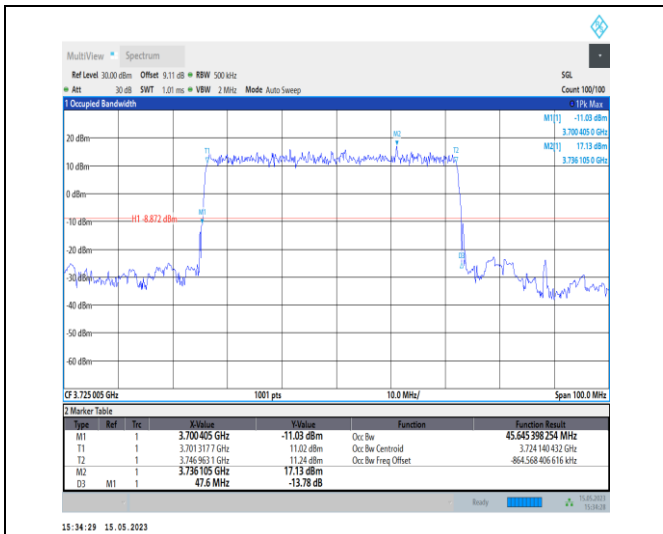
1-N77-3700-3980-PC1-30-50-L-2-DFT-PI2BPSK-Out er_Full-128@0-Ant0-45.645-47.600-<math>\leq 50</math>-PASS
