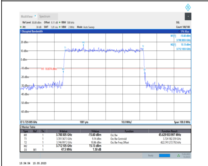
1-N77-3700-3980-PC1-30-50-L-4-DFT-64QAM-Out er_Full-128@0-Ant0-45.63-47.500-<math>\leq 50</math>-PASS
