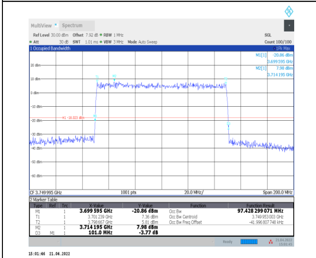
1-N77-3700-3980--30-100-L-9-CP-256QAM-Outer_F ull-273@0-Ant0-97.428-101.000-≤100-PASS
