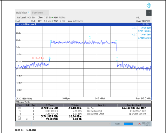
1-N77-3700-3980--30-70-L-7-CP-16QAM-Outer_Full-189@0-Ant0-67.341-69.580-<math>\leq</math>70-PASS
