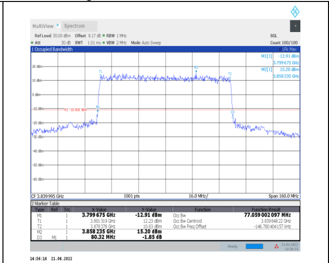
1-N77-3700-3980--30-80-M-1-DFT-QPSK-Outer_Full -216@0-Ant0-77.059-80.320-<=80-PASS
