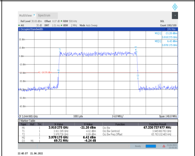
1-N77-3700-3980--30-70-H-9-CP-256QAM-Outer_Fu ll-189@0-Ant0-67.331-69.720-<=70-PASS
