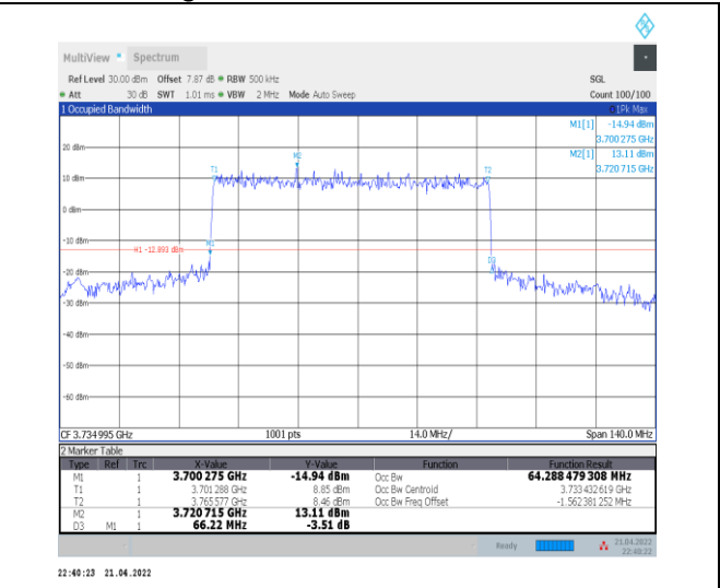
1-N77-3700-3980--30-70-L-1-DFT-QPSK-Outer_Full-180@0-Ant0-64.288-66.220-≤70-PASS
