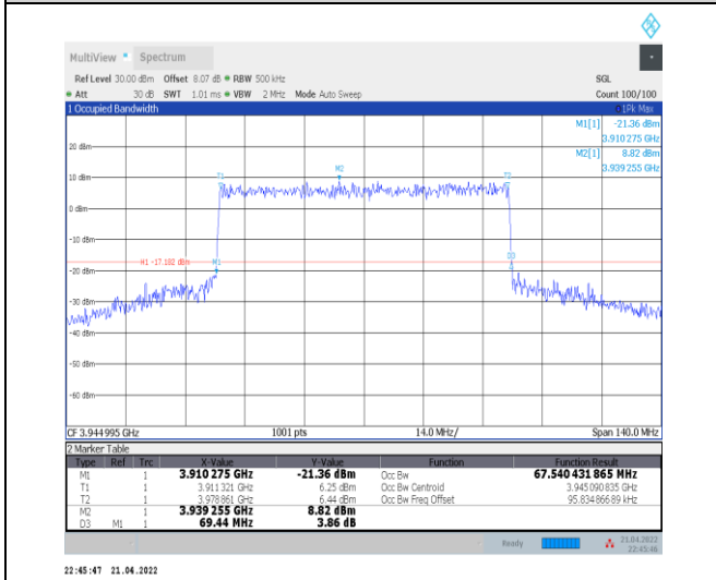
1-N77-3700-3980--30-70-H-8-CP-64QAM-Outer_Full-189@0-Ant0-67.54-69.440-<=70-PASS
