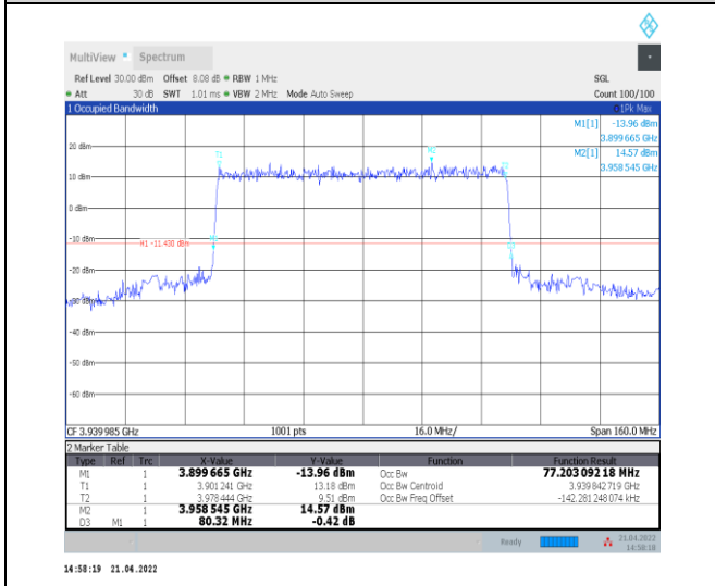
1-N77-3700-3980--30-80-H-1-DFT-QPSK-Outer_Full-I-216@0-Ant0-77.203-80.320-<math>\leq 80</math>-PASS
