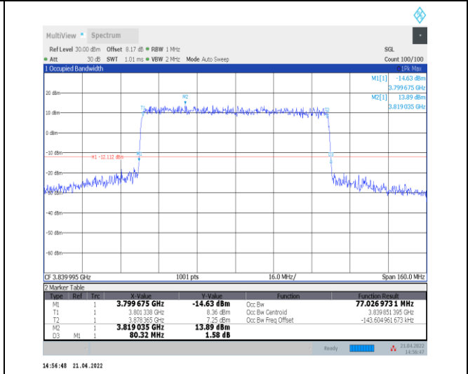
1-N77-3700-3980--30-80-M-3-DFT-16QAM-Outer_Full-216@0-Ant0-77.027-80.320-<=80-PASS
