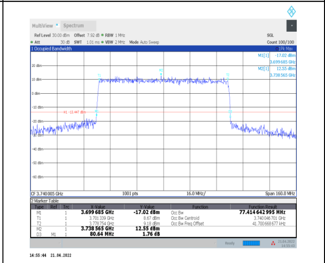
1-N77-3700-3980--30-80-L-8-CP-64QAM-Outer_Full-217@0-Ant0-77.415-80.640-<math>\leq 80</math>-PASS
