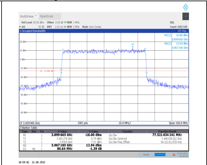
1-N77-3700-3980--30-80-H-8-CP-64QAM-Outer_Full -217@0-Ant0-77.522-80.640-<80-PASS
