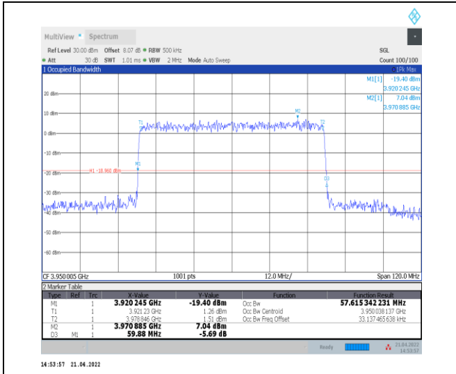
1-N77-3700-3980--30-60-H-9-CP-256QAM-Outer_Full-162@0-Ant0-57.615-59.880-≤60-PASS
