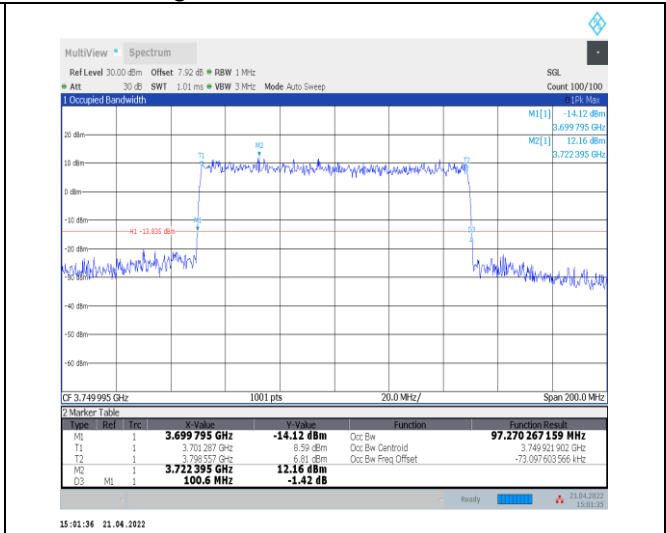
1-N77-3700-3980--30-100-L-8-CP-64QAM-Outer_Ful I-273@0-Ant0-97.27-100.600-≤100-PASS
