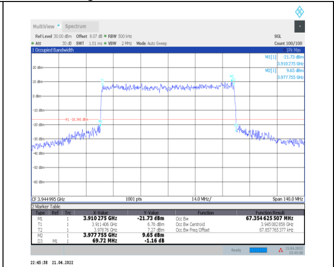
1-N77-3700-3980--30-70-H-7-CP-16QAM-Outer_Full-189@0-Ant0-67.355-69.720-<=70-PASS
