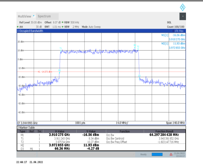
1-N77-3700-3980--30-70-H-1-DFT-QPSK-Outer_Full -180@0-Ant0-64.297-66.360-≤70-PASS
