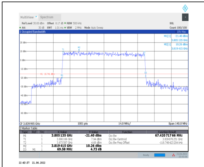
1-N77-3700-3980--30-70-M-7-CP-16QAM-Outer_Full I-189@0-Ant0-67.421-69.580-≤70-PASS
