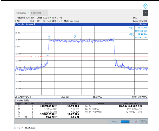
1-N77-3700-3980--30-90-H-8-CP-64QAM-Outer_Full -245@0-Ant0-87.548-90.900-<math>\leq</math>90-PASS
