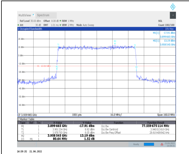
1-N77-3700-3980--30-80-H-7-CP-16QAM-Outer_Full -217@0-Ant0-77.56-80.640-<80-PASS
