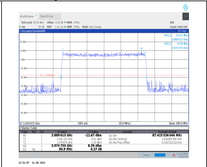
1-N77-3700-3980--30-90-H-9-CP-256QAM-Outer_Fu ll-245@0-Ant0-87.426-90.900-<math>\leq</math>90-PASS
