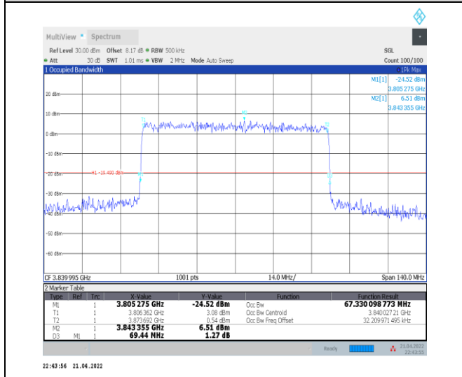
1-N77-3700-3980--30-70-M-9-CP-256QAM-Outer_Full ull-189@0-Ant0-67.33-69.440-≤70-PASS
