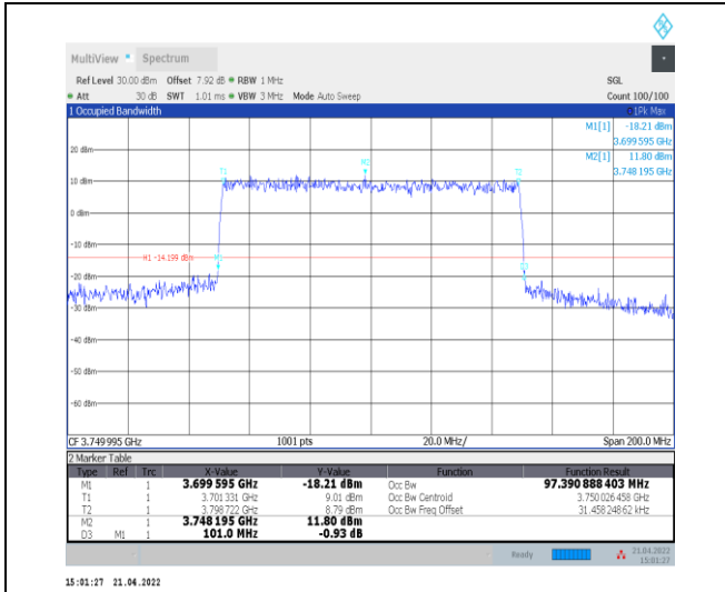
1-N77-3700-3980--30-100-L-7-CP-16QAM-Outer_Fu I1-273@0-Ant0-97.391-101.000-≤100-PASS
