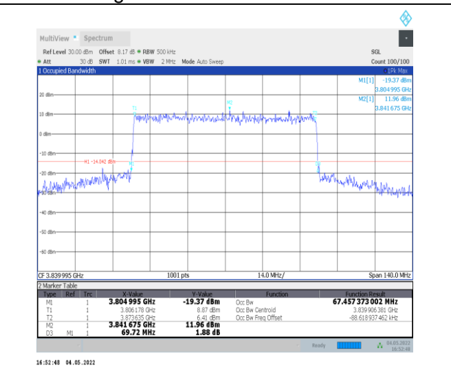
1-N77-3700-3980--30-70-M-8-CP-64QAM-Outer_Full -189@0-Ant0-67.457-69.720-≤70-PASS
