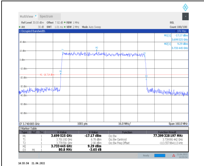
1-N77-3700-3980--30-80-L-9-CP-256QAM-Outer_Fu II-217@0-Ant0-77.399-80.800-<=80-PASS
