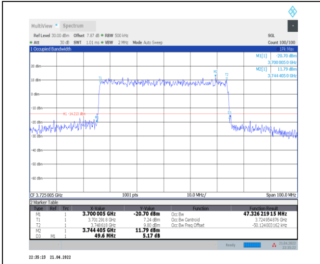
1-N77-3700-3980--30-50-L-6-CP-QPSK-Outer_Full-133@0-Ant0-47.326-49.600-<math>\leq 50</math>-PASS
