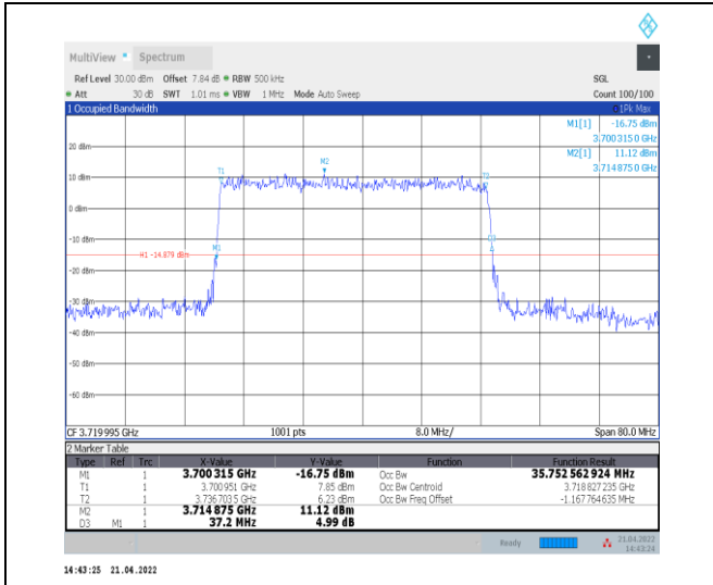
1-N77-3700-3980--30-40-L-5-DFT-256QAM-Outer_Full-100@0-Ant0-35.765-37.200-<=40-PASS
