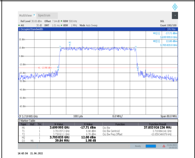
1-N77-3700-3980--30-40-L-8-CP-64QAM-Outer_Full-106@0-Ant0-37.849-39.840-<=40-PASS
