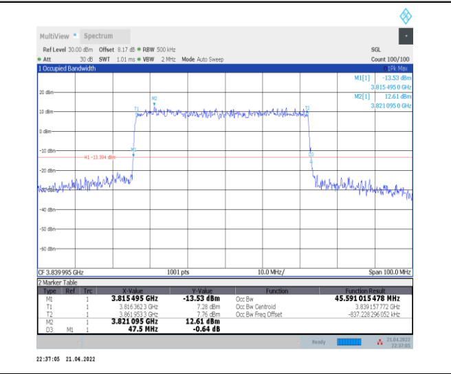
1-N77-3700-3980--30-50-M-4-DFT-64QAM-Outer_Full Full-128@0-Ant0-45.591-47.500-≤50-PASS
