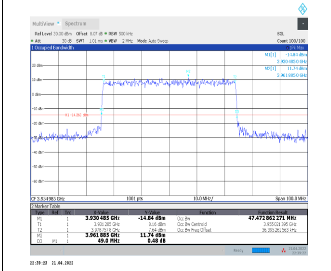
1-N77-3700-3980--30-50-H-6-CP-QPSK-Outer_Full-133@0-Ant0-47.473-49.000-≤50-PASS
