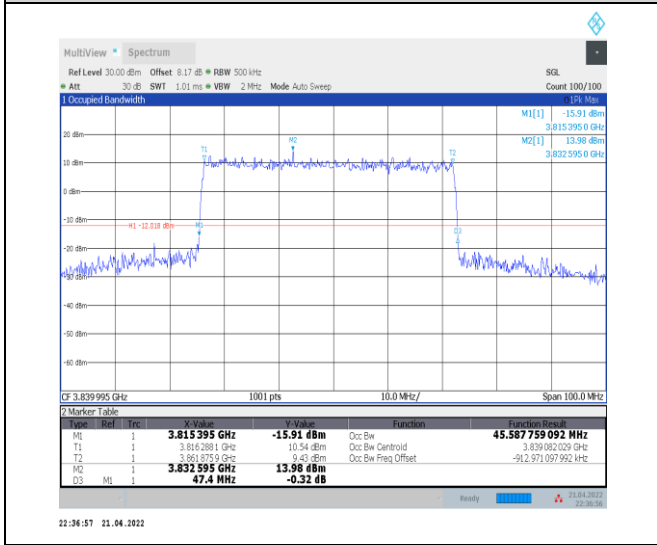
1-N77-3700-3980--30-50-M-3-DFT-16QAM-Outer_Full Full-128@0-Ant0-45.588-47.400-≤50-PASS
