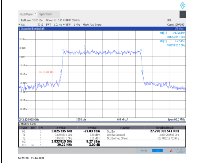
1-N77-3700-3980--30-30-M-9-CP-256QAM-Outer_Full ull-78@0-Ant0-27.798-29.220-≤30-PASS
