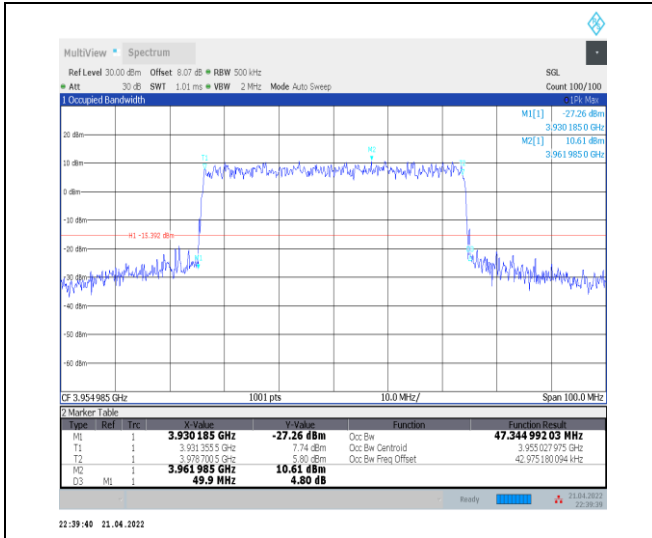
1-N77-3700-3980--30-50-H-8-CP-64QAM-Outer_Full -133@0-Ant0-47.345-49.900-≤50-PASS
