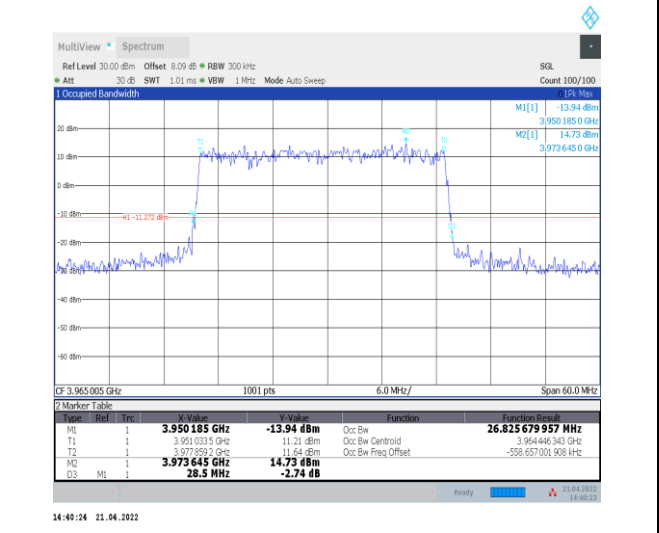
1-N77-3700-3980--30-30-H-1-DFT-QPSK-Outer_Full -75@0-Ant0-26.826-28.500-≤30-PASS
