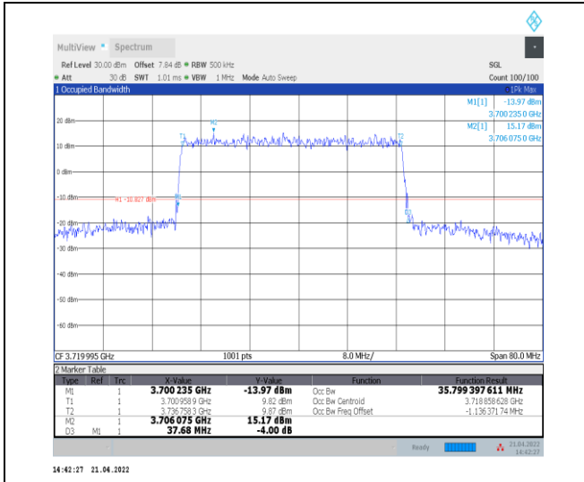
1-N77-3700-3980--30-40-L-1-DFT-QPSK-Outer_Full -100@0-Ant0-35.818-37.680-≤40-PASS
