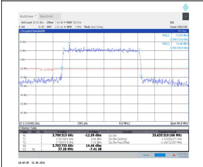
1-N77-3700-3980--30-40-L-3-DFT-16QAM-Outer_Full -100@0-Ant0-35.643-37.280-≤40-PASS
