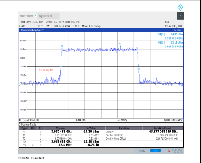
1-N77-3700-3980--30-50-H-3-DFT-16QAM-Outer_Full-128@0-Ant0-45.677-47.400-<=50-PASS
