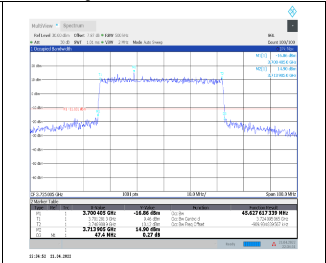
1-N77-3700-3980--30-50-L-3-DFT-16QAM-Outer_Full-128@0-Ant0-45.628-47.400-<math>\leq 50</math>-PASS
