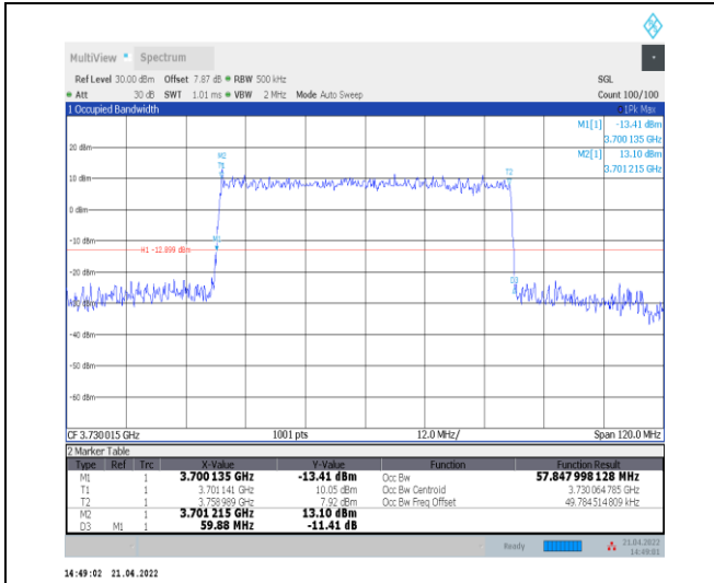
1-N77-3700-3980--30-60-L-3-DFT-16QAM-Outer_Fu II-162@0-Ant0-57.848-59.880-≤60-PASS
