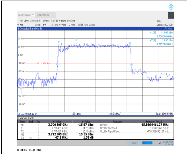
1-N77-3700-3980--30-50-L-2-DFT-PI2BPSK-Outer_Full-128@0-Ant0-45.567-47.500-<math>\leq 50</math>-PASS
