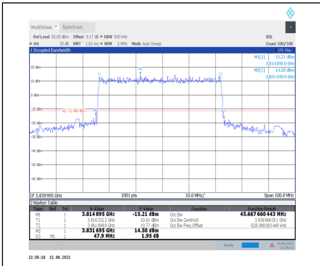
1-N77-3700-3980--30-50-M-1-DFT-QPSK-Outer_Full -128@0-Ant0-45.668-47.900-≤50-PASS
