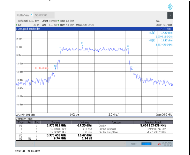
1-N77-3700-3980--30-10-H-8-CP-64QAM-Outer_Full -24@0-Ant0-8.604-9.760-≤10-PASS
