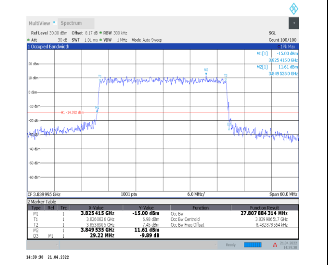
1-N77-3700-3980--30-30-M-6-CP-QPSK-Outer_Full-78@0-Ant0-27.809-29.220-≤30-PASS
