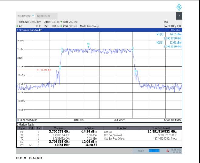
1-N77-3700-3980--30-15-L-5-DFT-256QAM-Outer_Full-36@0-Ant0-12.852-13.740-≤15-PASS
