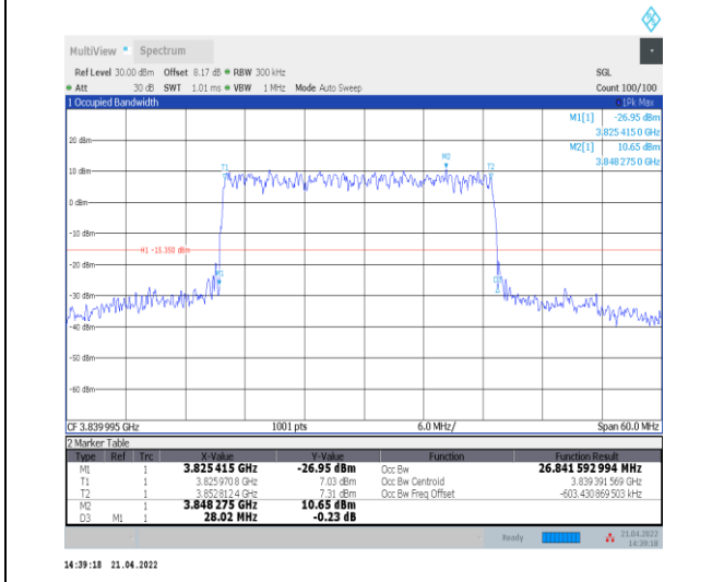
1-N77-3700-3980--30-30-M-5-DFT-256QAM-Outer_Full-75@0-Ant0-26.842-28.020-≤30-PASS
