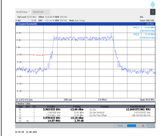
1-N77-3700-3980--30-15-H-2-DFT-PI2BPSK-Outer_Full-36@0-Ant0-12.84-14.070-≤15-PASS
