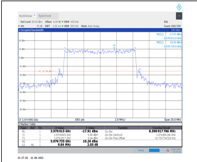
1-N77-3700-3980--30-10-H-7-CP-16QAM-Outer_Full -24@0-Ant0-8.599-9.840-≤10-PASS
