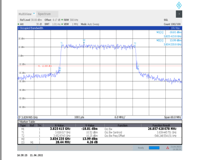
1-N77-3700-3980--30-30-M-1-DFT-QPSK-Outer_Full -75@0-Ant0-26.857-28.440-<30-PASS
