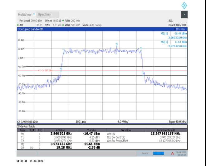
1-N77-3700-3980--30-20-H-8-CP-64QAM-Outer_Full-51@0-Ant0-18.248-19.280-<=20-PASS
