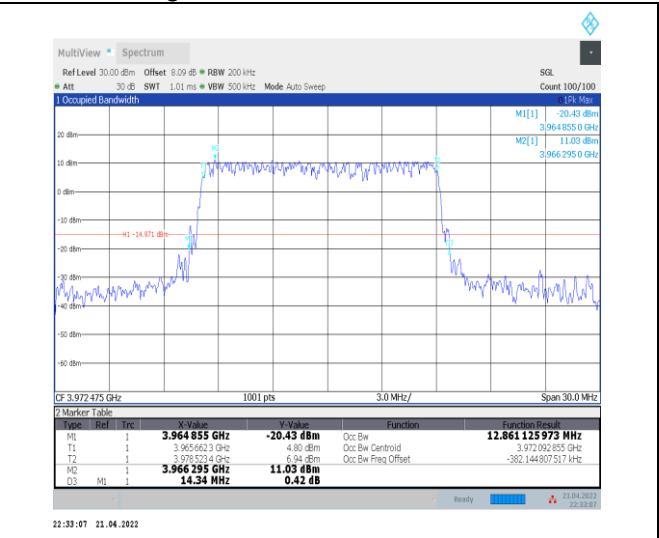
1-N77-3700-3980--30-15-H-5-DFT-256QAM-Outer_Full-36@0-Ant0-12.861-14.340-≤15-PASS
