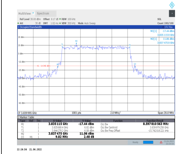
1-N77-3700-3980--30-10-M-6-CP-QPSK-Outer_Full-24@0-Ant0-8.598-9.820-≤10-PASS
