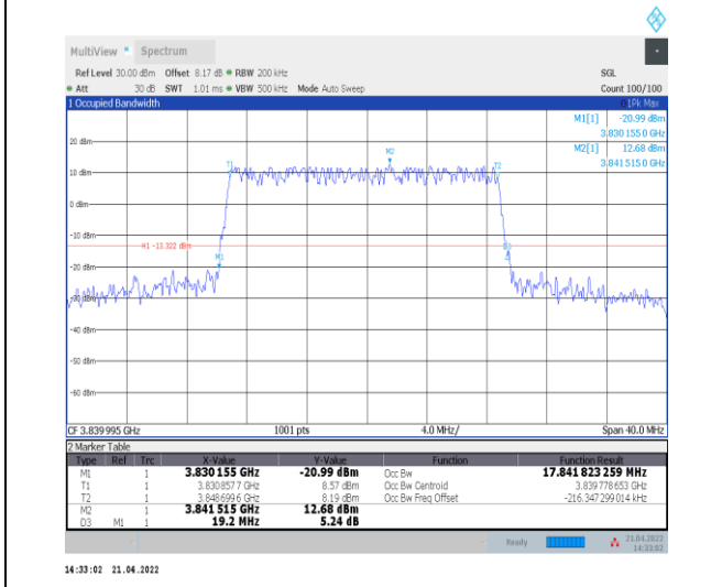
1-N77-3700-3980--30-20-M-4-DFT-64QAM-Outer_Full-50@0-Ant0-17.842-19.200-≤20-PASS
