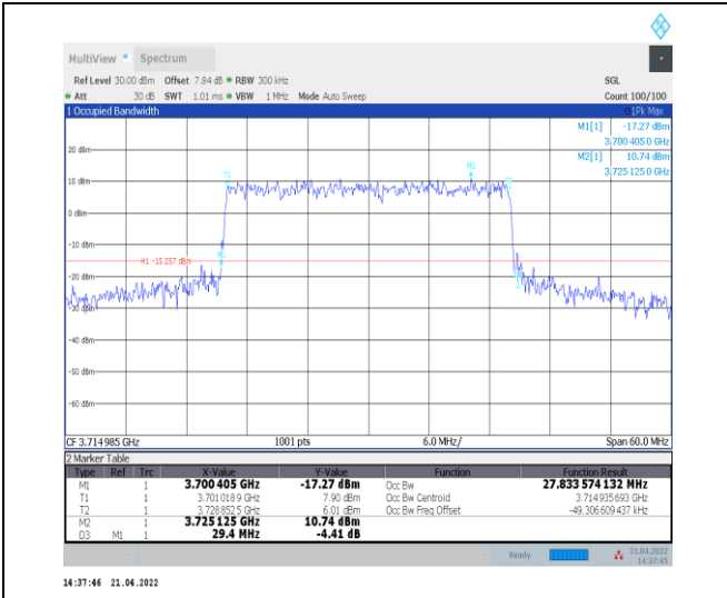
1-N77-3700-3980--30-30-L-8-CP-64QAM-Outer_Full -78@0-Ant0-27.833-29.400-<30-PASS
