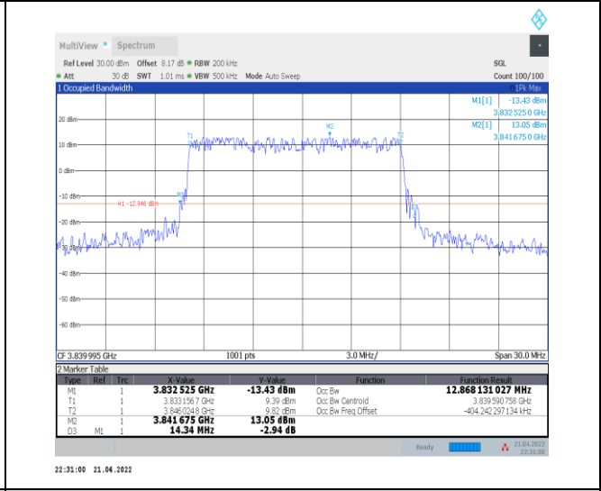
1-N77-3700-3980--30-15-M-4-DFT-64QAM-Outer_Full ll-36@0-Ant0-12.868-14.340≤15-PASS
