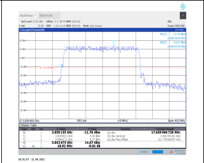
1-N77-3700-3980--30-20-M-1-DFT-QPSK-Outer_Full -50 @ 0-Ant0-17.66-18.920-≤20-PASS
