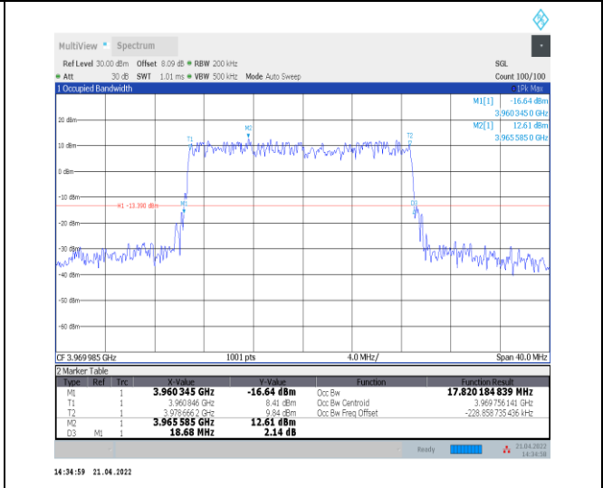
1-N77-3700-3980--30-20-H-4-DFT-64QAM-Outer_Full ll-50@0-Ant0-17.82-18.680-≤20-PASS
