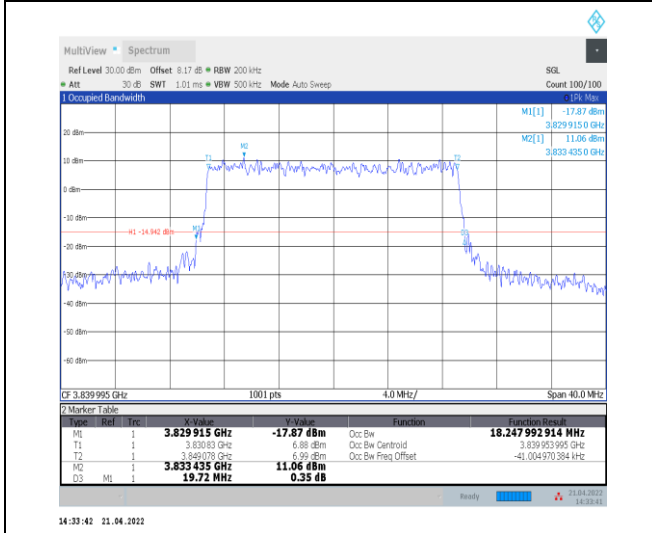
1-N77-3700-3980--30-20-M-8-CP-64QAM-Outer_Full-51@0-Ant0-18.248-19.720-≤20-PASS
