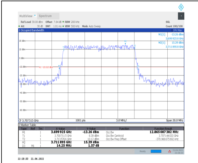
1-N77-3700-3980--30-15-L-2-DFT-PI2BPSK-Outer_Full-36@0-Ant0-12.865-14.250-≤15-PASS
