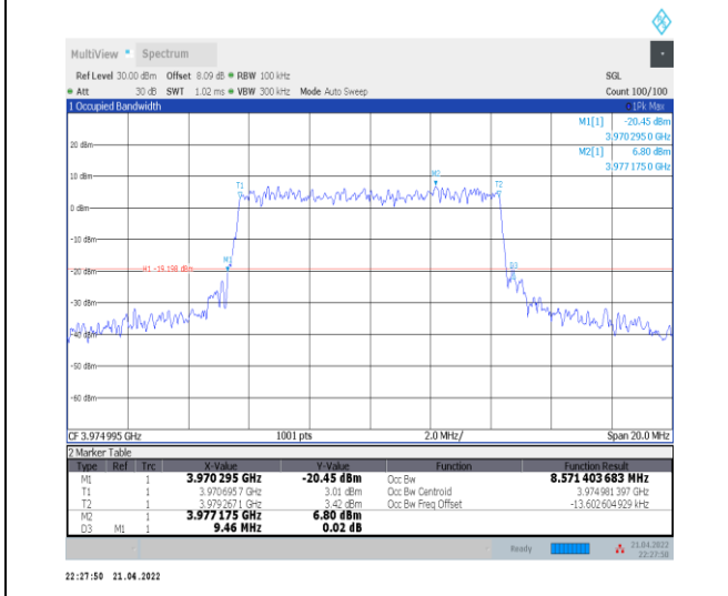
1-N77-3700-3980--30-10-H-9-CP-256QAM-Outer_F ull-24@0-Ant0-8.571-9.460-≤10-PASS
