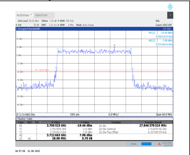
1-N77-3700-3980--30-30-L-9-CP-256QAM-Outer_Ful I-78@0-Ant0-27.852-28.980-<30-PASS
