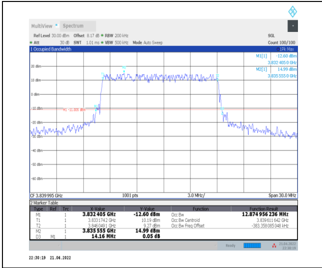
1-N77-3700-3980--30-15-M-1-DFT-QPSK-Outer_Full -36@0-Ant0-12.875-14.160≤15-PASS
