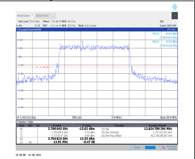
1-N77-3700-3980--30-15-L-3-DFT-16QAM-Outer_Full-36@0-Ant0-12.825-13.920-≤15-PASS
