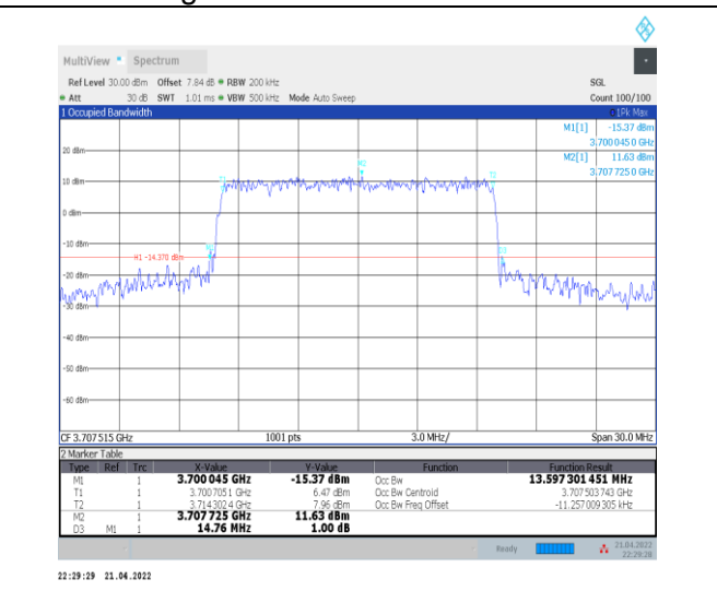
1-N77-3700-3980--30-15-L-7-CP-16QAM-Outer_Full-38@0-Ant0-13.597-14.760-≤15-PASS
