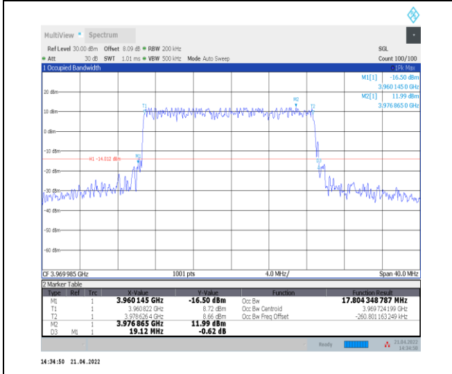
1-N77-3700-3980--30-20-H-3-DFT-16QAM-Outer_Full ull-50@0-Ant0-17.804-19.120-≤20-PASS
