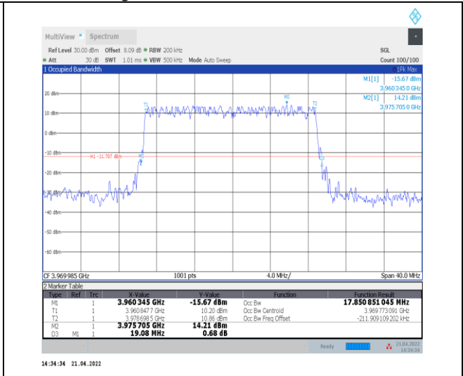
1-N77-3700-3980--30-20-H-2-DFT-PI2BPSK-Outer_Full Full-50@0-Ant0-17.851-19.080-≤20-PASS
