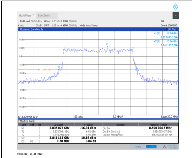
1-N77-3700-3980--30-10-M-8-CP-64QAM-Outer_Ful I-24@0-Ant0-8.591-9.780-≤10-PASS
