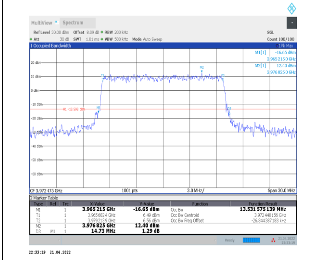
1-N77-3700-3980--30-15-H-6-CP-QPSK-Outer_Full-38@0-Ant0-13.532-14.730-≤15-PASS
