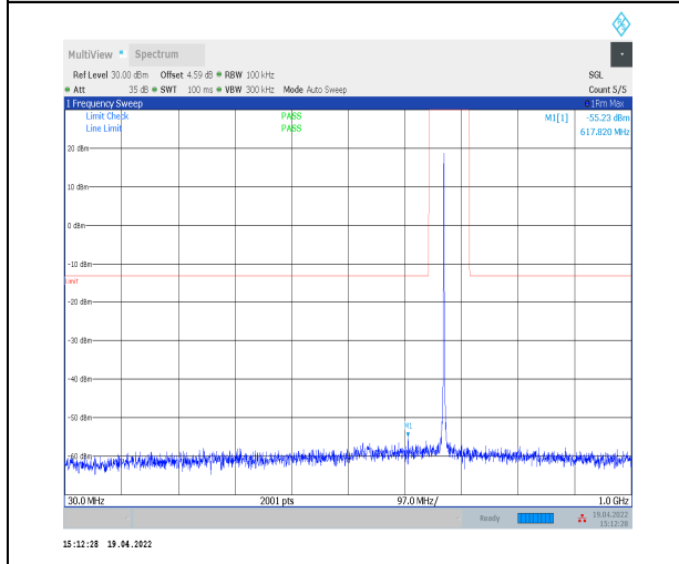
1-N71--15-20-H-1-DFT-PI2BPSK-Inner_1RB_Left-1 @1-30-1000-Ant0--55.23--13-PASS
