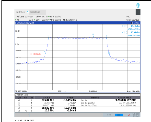
1-N71--15-10-M-7-CP-16QAM-Outer_Full-52@0-Ant 0-9.295-10.200-≤10-PASS
