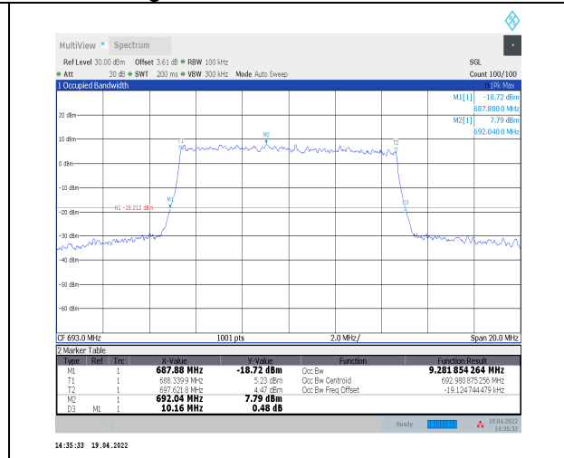
1-N71--15-10-H-9-CP-256QAM-Outer_Full-52@0-An 10-9.282-10.160-≤10-PASS
