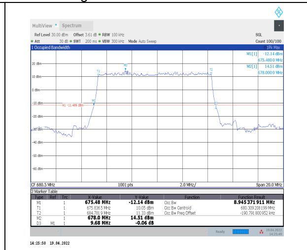
1-N71--15-10-M-2-DFT-PI2BPSK-Outer_Full-50@0-Ant 0-8.945-9.680≤10-PASS
