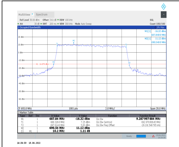
1-N71--15-10-H-8-CP-64QAM-Outer_Full-52@0-Ant 0-9.288-10.200-≤10-PASS
