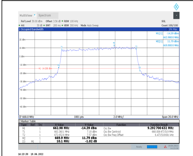
1-N71--15-10-L-8-CP-64QAM-Outer_Full-52@0-Ant0 -9.293-10.100-<=10-PASS
