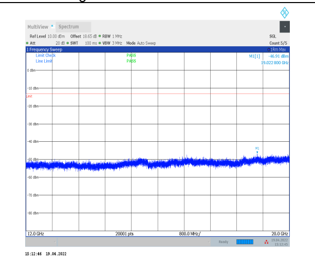
1-N71--15-20-H-1-DFT-PI2BPSK-Inner_1RB_Left-1 @1-12000-20000-Ant0--46.91--13-PASS
