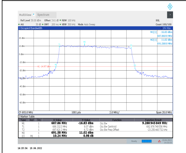
1-N71--15-10-H-6-CP-QPSK-Outer_Full-52@0-Ant0 9.289-10.240-≤10-PASS
