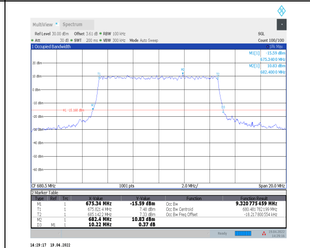
1-N71--15-10-M-8-CP-64QAM-Outer_Full-52@0-Ant 0-9.321-10.220-≤10-PASS
