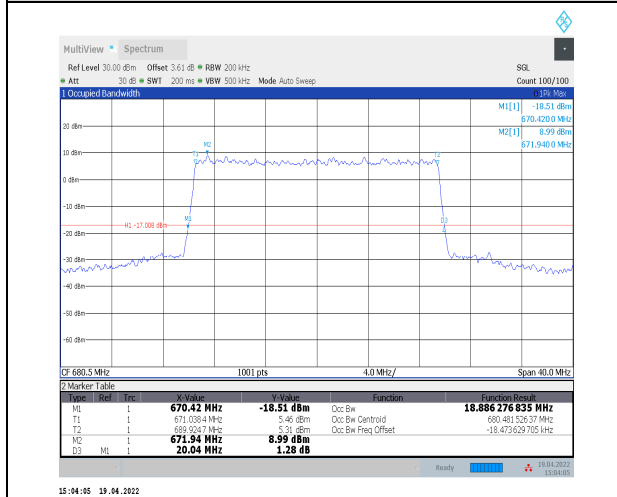
1-N71--15-20-M-9-CP-256QAM-Outer_Full-106@0-A nt0-18.886-20.040-<=20-PASS
