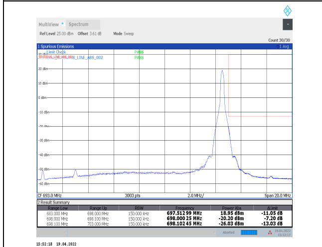
1-N71--15-15-H-5-CP-QPSK-Edge_1RB_Right-1@78-Ant0-PASS-see graph
