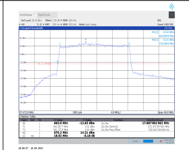
1-N71--15-20-L-3-DFT-16QAM-Outer_Full-100@0-Ant t0-17.808-18.920-<=20-PASS
