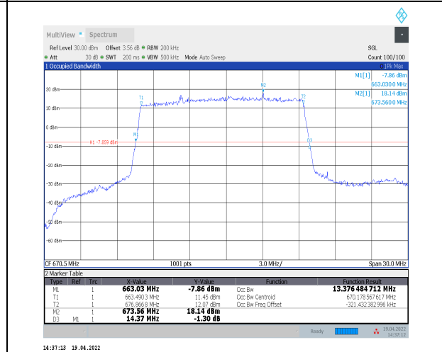
1-N71--15-15-L-2-DFT-PI2BPSK-Outer_Full-75@0-A n0-13.376-14.370-≤15-PASS
