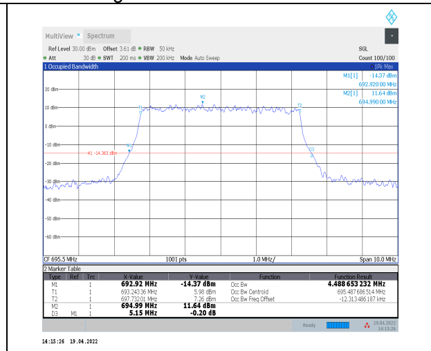
1-N71--15-5-H-4-DFT-64QAM-Outer_Full-25@0-Ant 0-4.489-5.150-≤5-PASS
