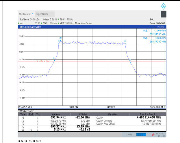
1-N71--15-5-H-2-DFT-PI2BPSK-Outer_Full-25@0-Ant0 4.487-5.130≤5-PASS
