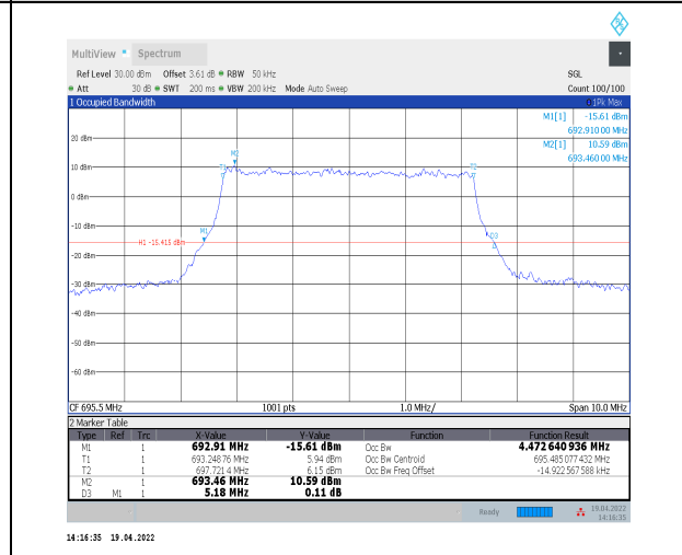
1-N71--15-5-H-6-CP-QPSK-Outer_Full-25@0-Ant0-4 .473-5.180-≤5-PASS
