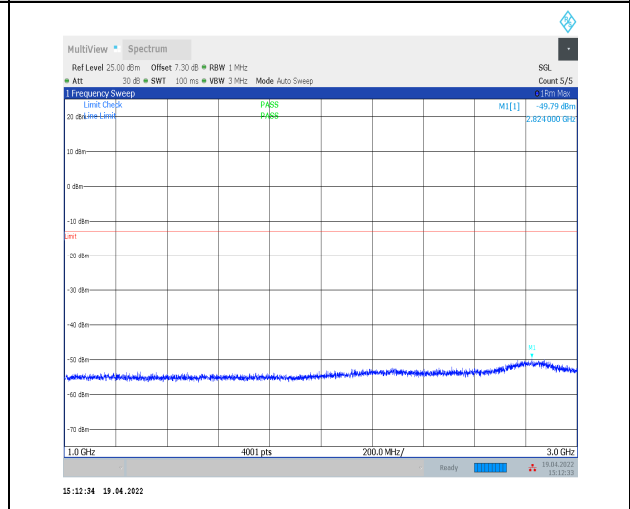
1-N71--15-20-H-1-DFT-PI2BPSK-Inner_1RB_Left-1 @1-1000-3000-Ant0--49.79--13-PASS
