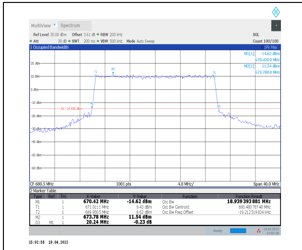
1-N71--15-20-M-7-CP-16QAM-Outer_Full-106@0-An t0-18.939-20.240-<=20-PASS
