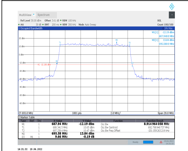
1-N71--15-10-H-2-DFT-PI2BPSK-Outer_Full-50@0-Ant Ant0-8.915-9.660-<=10-PASS
