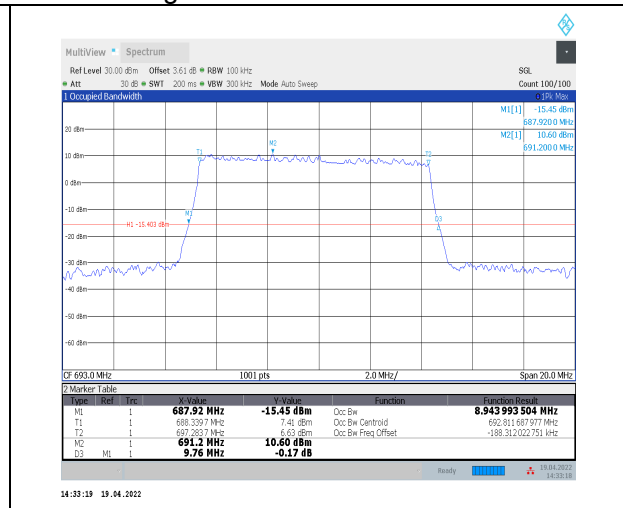
1-N71--15-10-H-5-DFT-256QAM-Outer_Full-50@0-Ant nt0-8.944-9.760-≤10-PASS
