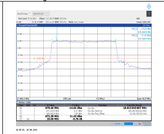
1-N71--15-20-M-8-CP-64QAM-Outer_Full-106@0-A nt0-18.915-20.080-<=20-PASS
