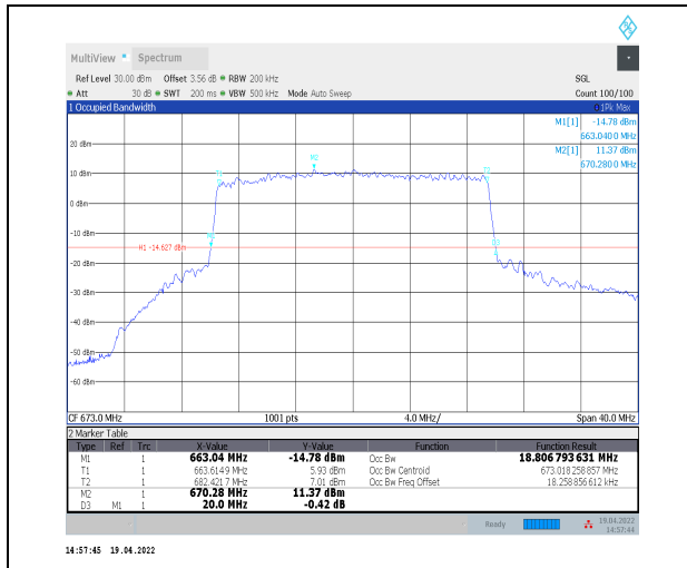
1-N71--15-20-L-8-CP-64QAM-Outer_Full-106@0-Ant 0-18.807-20.000-≤20-PASS
