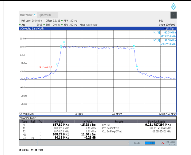
1-N71--15-10-H-7-CP-16QAM-Outer_Full-52@0-Ant 0-9.282-10.180-≤10-PASS
