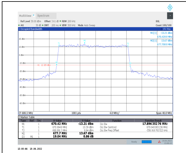
1-N71--15-20-M-3-DFT-16QAM-Outer_Full-100@0-A Ant0-17.896-19.040-≤20-PASS
