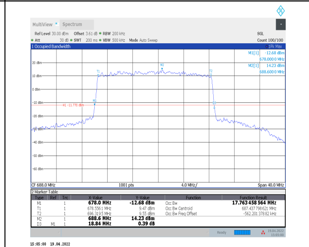
1-N71--15-20-H-1-DFT-QPSK-Outer_Full-100@0-An t0-17.763-18.840-<=20-PASS
