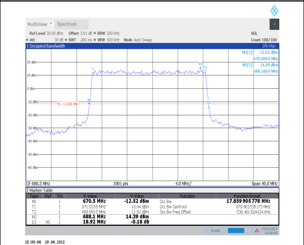
1-N71--15-20-M-2-DFT-PI2BPSK-Outer_Full-100@0-Ant -Ant0-17.86-18.920-≤20-PASS
