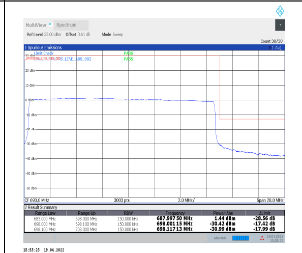
1-N71--15-15-H-6-CP-QPSK-Outer_Full-79@0-Ant0-PASS-see graph
