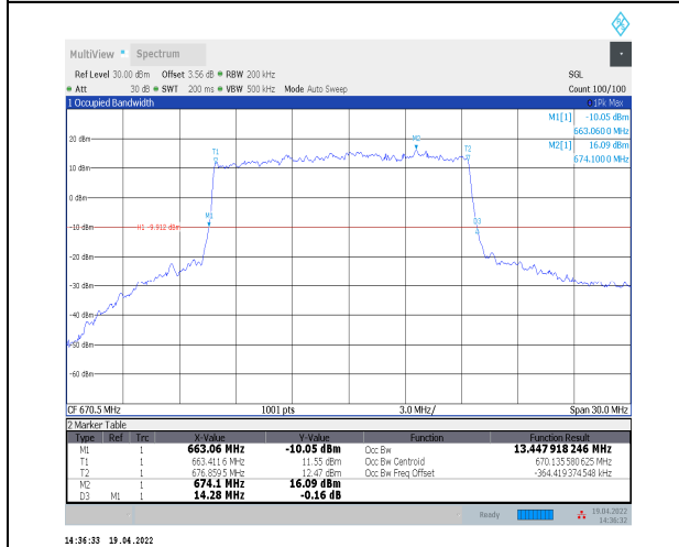
1-N71--15-15-L-1-DFT-QPSK-Outer_Full-75@0-Ant0 -13.448-14.280-≤15-PASS
