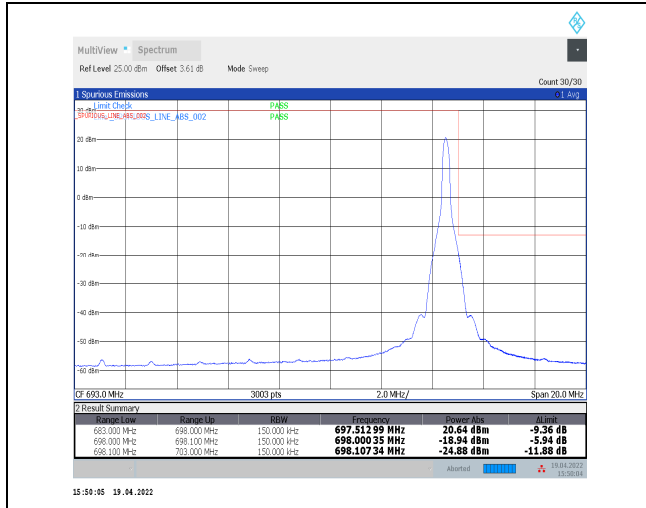
1-N71--15-15-H-2-DFT-PI2BPSK-Edge_1RB_Right-1@78-Ant0-PASS-see graph
