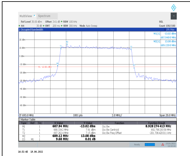
1-N71--15-10-H-4-DFT-64QAM-Outer_Full-50@0-Ant t0-8.928-9.680-≤10-PASS
