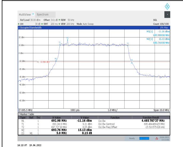
1-N71--15-5-H-1-DFT-QPSK-Outer_Full-25@0-Ant0 4.486-5.000≤5-PASS
