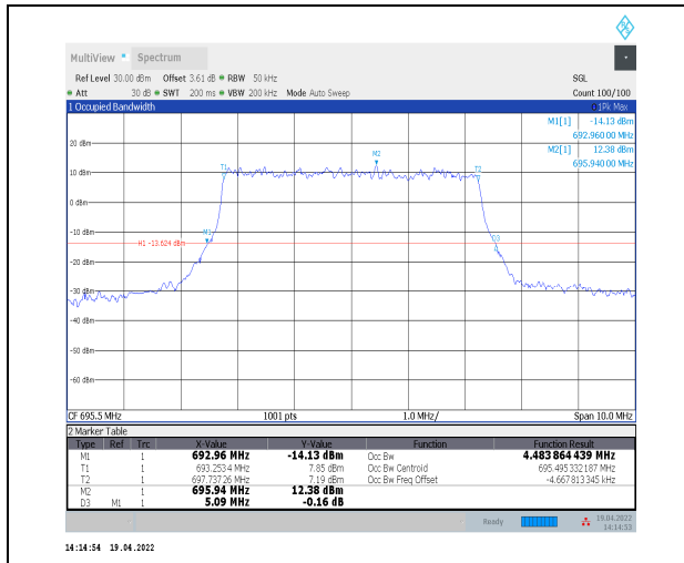
1-N71--15-5-H-3-DFT-16QAM-Outer_Full-25@0-Ant 0-4.484-5.090-≤5-PASS
