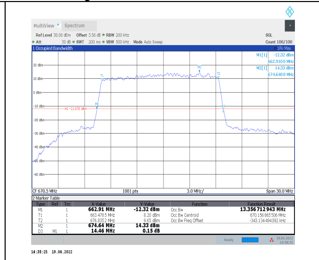
1-N71--15-15-L-4-DFT-64QAM-Outer_Full-75@0-An t0-13.357-14.460≤15-PASS
