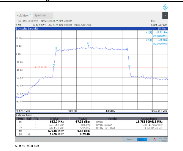
1-N71--15-20-L-9-CP-256QAM-Outer_Full-106@0-Ant nt0-18.786-19.920-≤20-PASS
