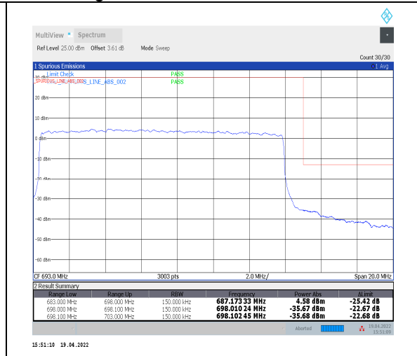
1-N71--15-15-H-3-DFT-PI2BPSK-Outer_Full-75@0-Ant0-PASS-see graph
