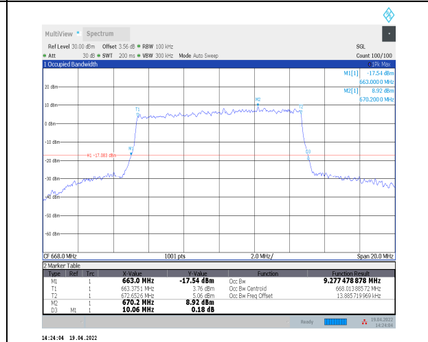
1-N71--15-10-L-9-CP-256QAM-Outer_Full-52@0-An 10-9.277-10.060-<=10-PASS
