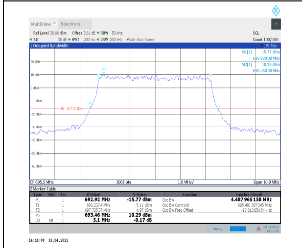
1-N71--15-5-H-5-DFT-256QAM-Outer_Full-25@0-Ant t0-4.488-5.100-≤5-PASS
