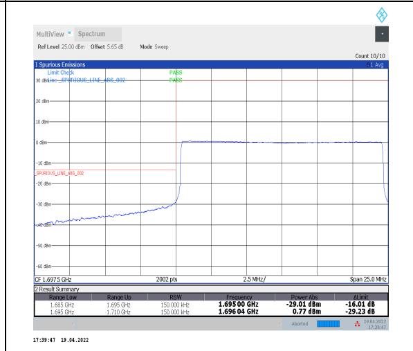
1-N70--15-15-L-6-CP-QPSK-Outer_Full-79@0-Ant 2-seegraph-PASS-see graph
