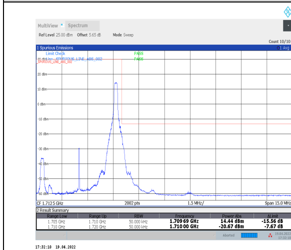
1-N70--15-5-H-5-CP-QPSK-Edge_1RB_Right-1@24-Ant2-seegraph-PASS-see graph
