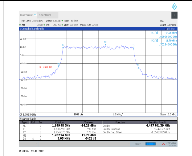
1-N70--15-5-M-3-DFT-16QAM-Outer_Full-25@0-Ant 2-4.478-5.050-≤5-PASS
