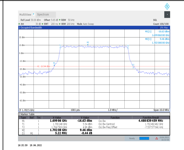
1-N70--15-5-M-7-CP-16QAM-Outer_Full-25@0-Ant2 -4.489-5.220-<math>\leq</math>5-PASS
