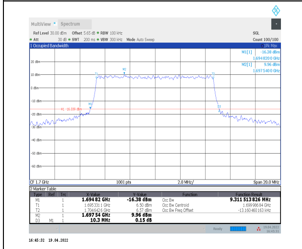
1-N70--15-10-L-8-CP-64QAM-Outer_Full-52@0-Ant2 -9.312-10.300≤10-PASS
