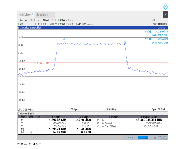
1-N70--15-15-L-3-DFT-16QAM-Outer_Full-75@0-Ant 2-13.46-14.550-≤15-PASS
