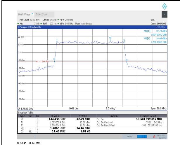
1-N70--15-15-L-1-DFT-QPSK-Outer_Full-75@0-Ant2 -13.505-14.460-<math>\leq 15</math>-PASS
