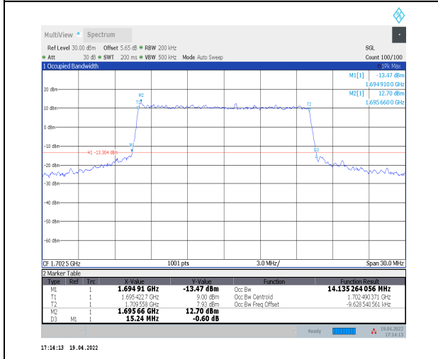
1-N70--15-15-H-7-CP-16QAM-Outer_Full-79@0-Ant 2-14.135-15.240≤15-PASS
