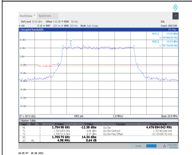
1-N70--15-5-H-1-DFT-QPSK-Outer_Full-25@0-Ant2- 4.476-4.980-≤5-PASS
