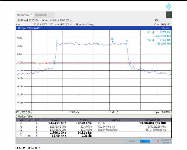
1-N70--15-15-M-1-DFT-QPSK-Outer_Full-75@0-Ant 2-13.505-14.490≤15-PASS
