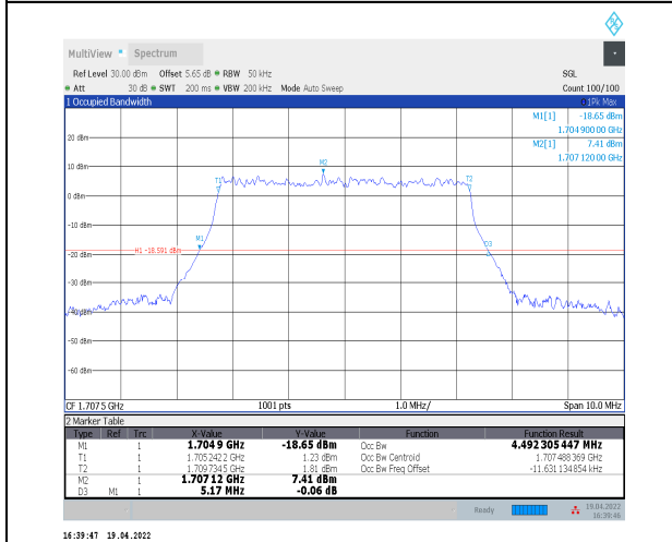
1-N70--15-5-H-9-CP-256QAM-Outer_Full-25@0-Ant 2-4.492-5.170≤5-PASS
