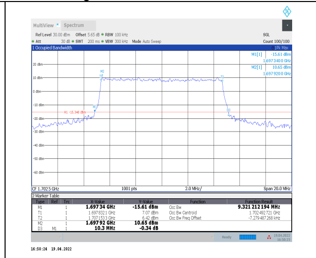
1-N70--15-10-M-6-CP-QPSK-Outer_Full-52@0-Ant2 -9.321-10.300-≤10-PASS
