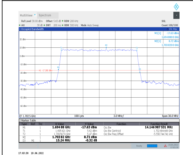
1-N70--15-15-L-9-CP-256QAM-Outer_Full-79@0-Ant 2-14.147-15.240≤15-PASS
