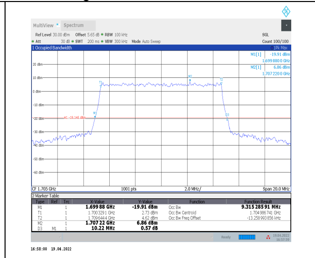
1-N70--15-10-H-9-CP-256QAM-Outer_Full-52@0-An t2-9.315-10.220-<math>\leq 10</math>-PASS
