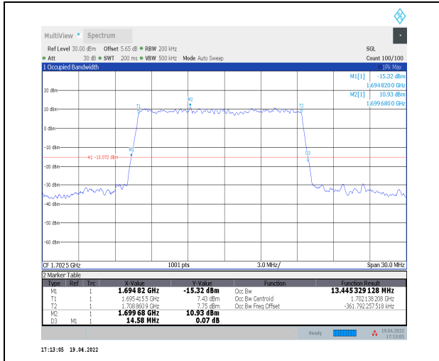
1-N70--15-15-H-5-DFT-256QAM-Outer_Full-75@0-A nt2-13.445-14.580≤15-PASS
