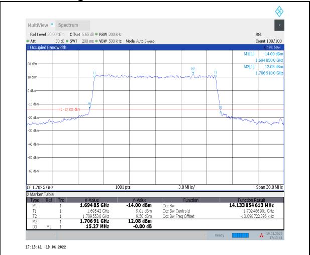
1-N70--15-15-H-6-CP-QPSK-Outer_Full-79@0-Ant2- 14.134-15.270≤15-PASS
