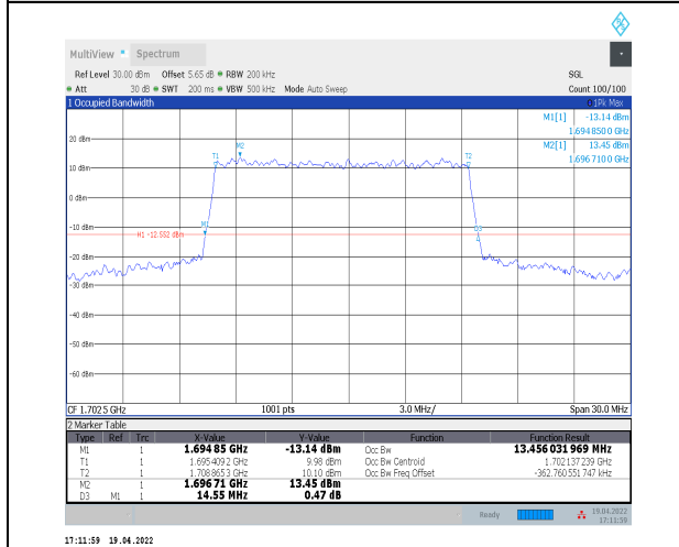
1-N70--15-15-H-3-DFT-16QAM-Outer_Full-75@0-An t2-13.456-14.550≤15-PASS
