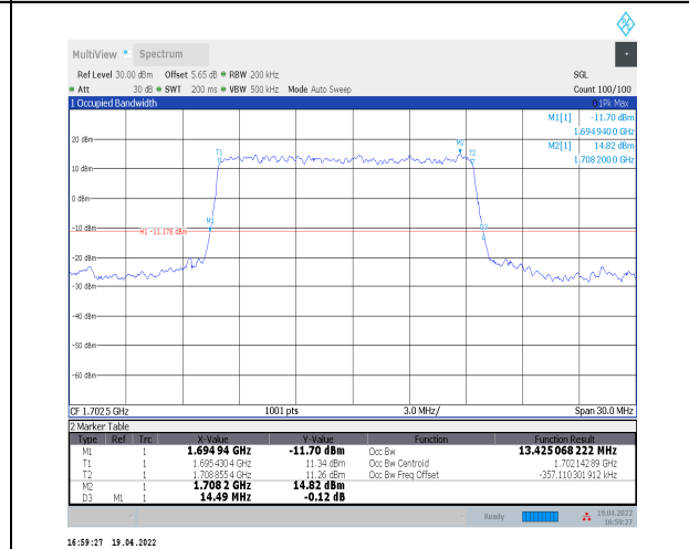
1-N70--15-15-L-2-DFT-PI2BPSK-Outer_Full-75@0-A nt2-13.425-14.490-<math>\leq 15</math>-PASS
