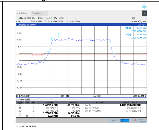
1-N70--15-5-M-1-DFT-QPSK-Outer_Full-25@0-Ant2 -4.487-5.030-≤5-PASS
