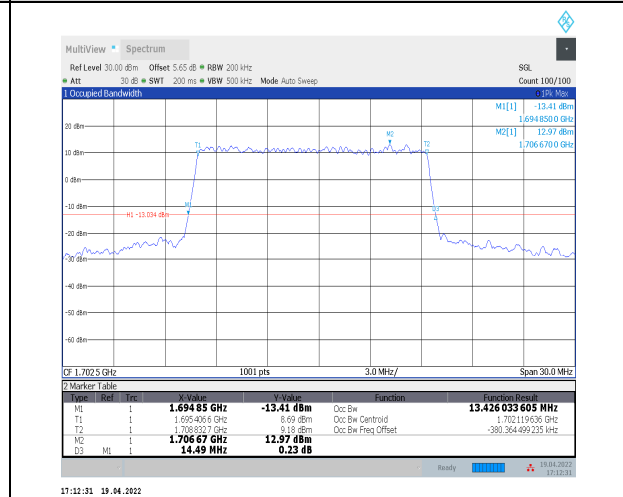
1-N70--15-15-H-4-DFT-64QAM-Outer_Full-75@0-An t2-13.426-14.490≤15-PASS
