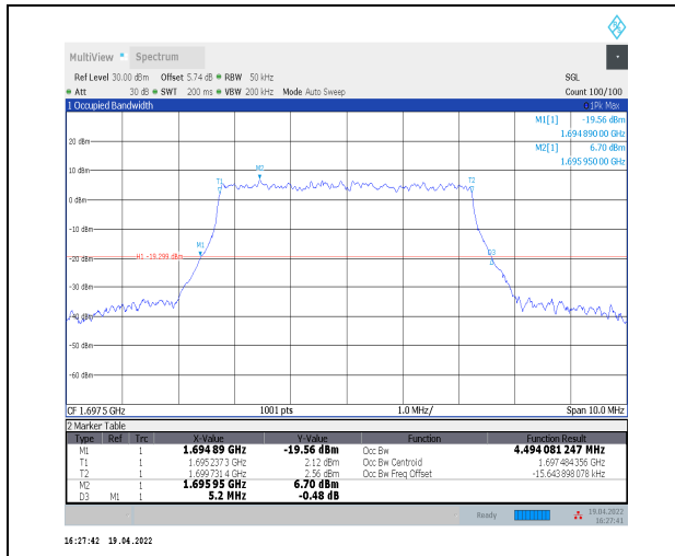
1-N70--15-5-L-9-CP-256QAM-Outer_Full-25@0-Ant2 -4.494-5.200-≤5-PASS
