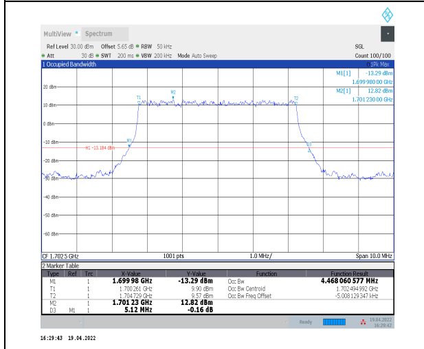
1-N70--15-5-M-2-DFT-PI2BPSK-Outer_Full-25@0-A nt2-4.468-5.120-≤5-PASS
