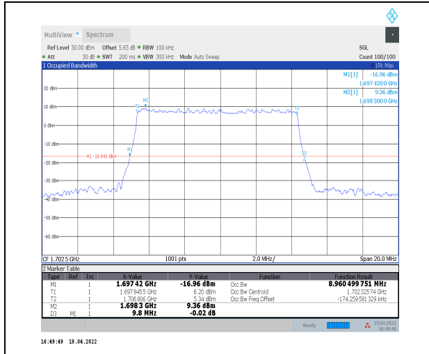
1-N70--15-10-M-5-DFT-256QAM-Outer_Full-50@0-A nt2-8.96-9.800-≤10-PASS
