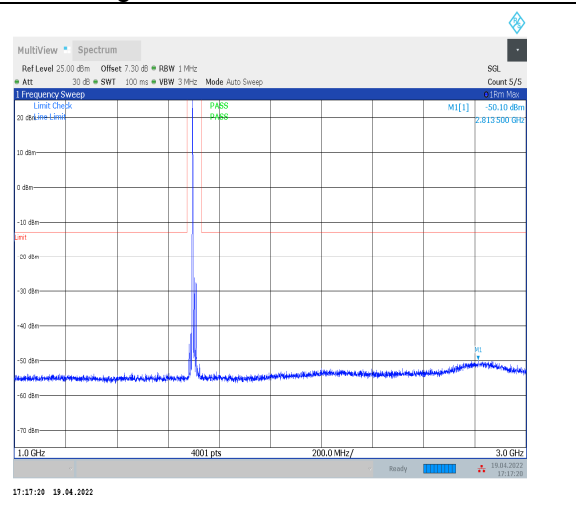
1-N70--15-15-H-1-DFT-PI2BPSK-Inner_1RB_Left-1 @1-1000-3000-Ant2--50.10--13-PASS
