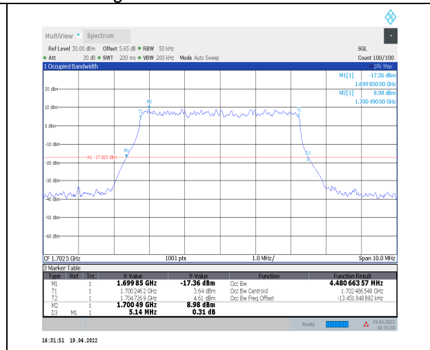
1-N70--15-5-M-5-DFT-256QAM-Outer_Full-25@0-A nt2-4.481-5.140-<math>\leq</math>5-PASS
