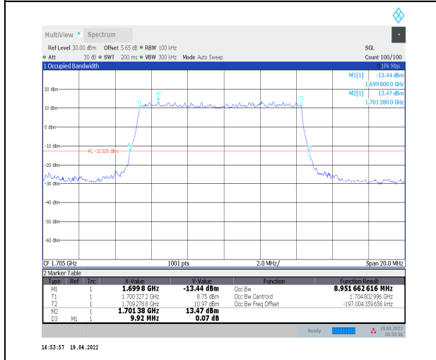
1-N70--15-10-H-2-DFT-PI2BPSK-Outer_Full-50@0-Ant Ant2-8.952-9.920-<=10-PASS
