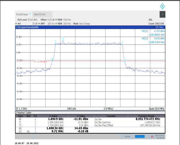
1-N70--15-10-L-1-DFT-QPSK-Outer_Full-50@0-Ant2 -8.952-9.720≤10-PASS
