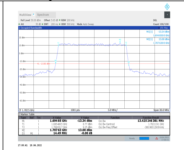
1-N70--15-15-L-4-DFT-64QAM-Outer_Full-75@0-An t2-13.425-14.490-≤15-PASS
