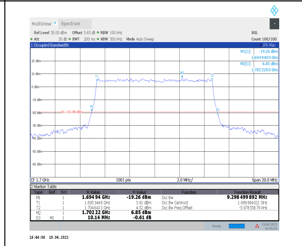
1-N70--15-10-L-9-CP-256QAM-Outer_Full-52@0-An 12-9.298-10.140≤10-PASS
