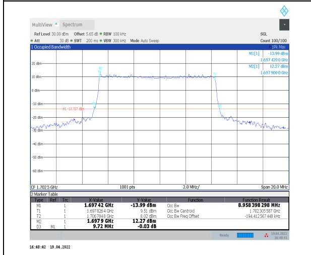
1-N70--15-10-M-3-DFT-16QAM-Outer_Full-50@0-Ant t2-8.958-9.720≤10-PASS
