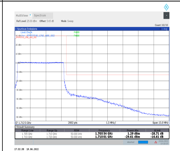
1-N70--15-5-H-6-CP-QPSK-Outer_Full-25@0-Ant2-seegraph-PASS-see graph
