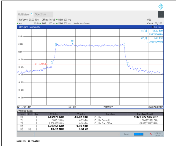
1-N70--15-10-H-8-CP-64QAM-Outer_Full-52@0-Ant 2-9.326-10.320-<math>\leq 10</math>-PASS
