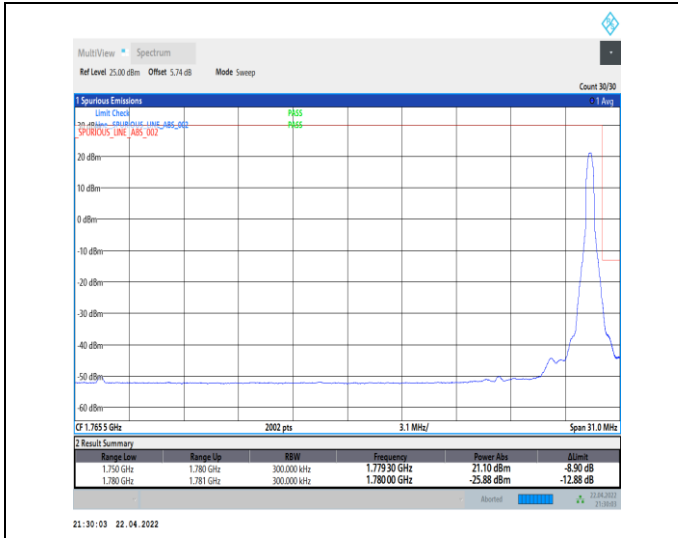
1-N66-PC3-15-30-H-2-DFT-PI2BPSK-Edge_1RB_Right-t-1@159-Ant0-seegraph-PASS-see graph
