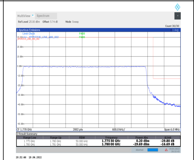
1-N66-PC3-15-5-H-6-CP-QPSK-Outer_Full-25@0-Ant0-seegraph-PASS-see graph
