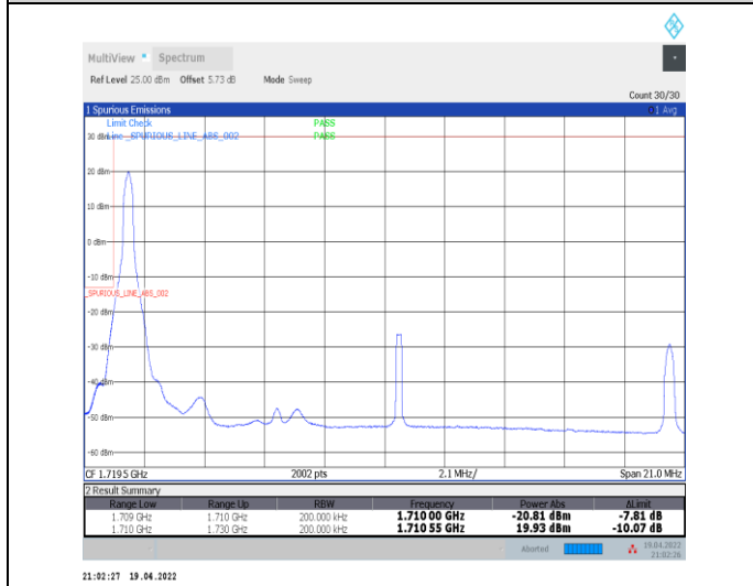
1-N66-PC3-15-20-L-4-CP-QPSK-Edge_1RB_Left-1@0-Ant0-seegraph-PASS-see graph
