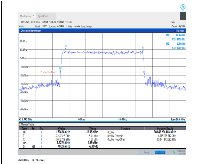
1-N66-PC3-15-40-M-9-CP-256QAM-Outer_Full-216 @ 0-Ant0-38.646-40.240-≤40-PASS
