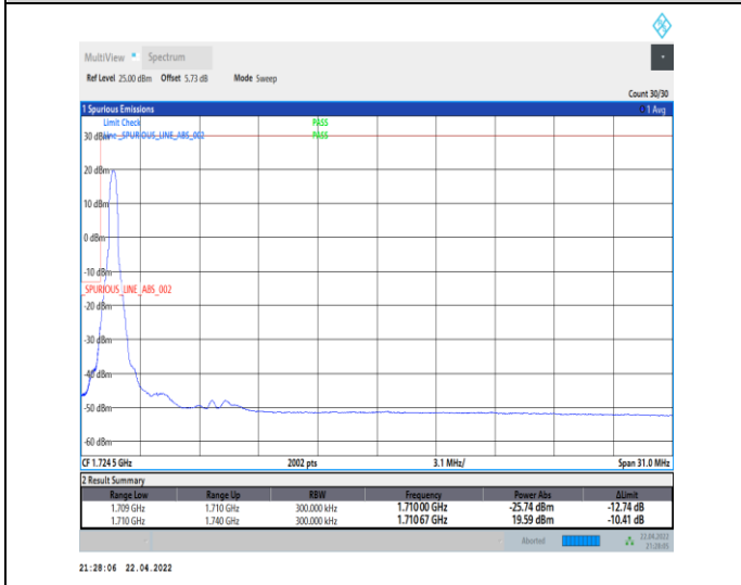
1-N66-PC3-15-30-L-4-CP-QPSK-Edge_1RB_Left-1@0-Ant0-seegraph-PASS-see graph
