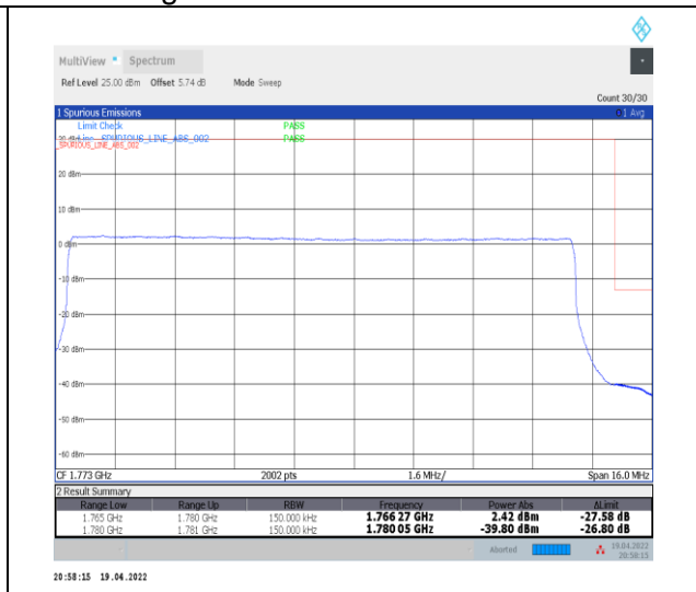
1-N66-PC3-15-15-H-3-DFT-PI2BPSK-Outer_Full-75@0-Ant0-seegraph-PASS-see graph
