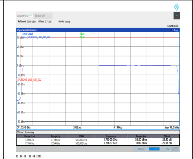
1-N66-PC3-15-40-L-6-CP-QPSK-Outer_Full-216@0-Ant0-seegraph-PASS-see graph
