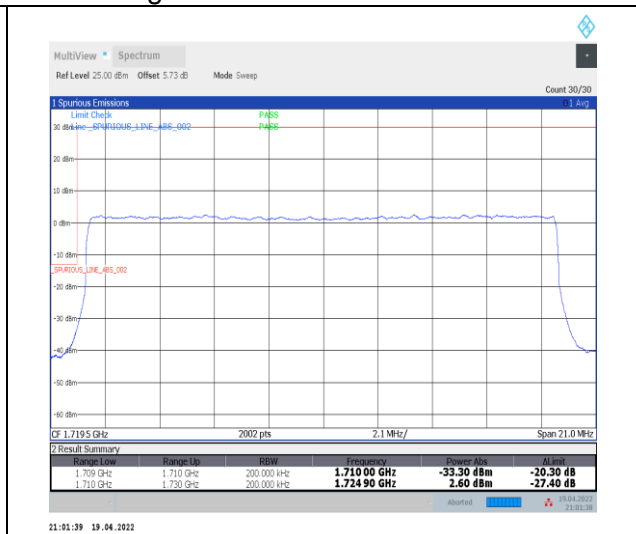
1-N66-PC3-15-20-L-3-DFT-PI2BPSK-Outer_Full-100@0-Ant0-seegraph-PASS-see graph
