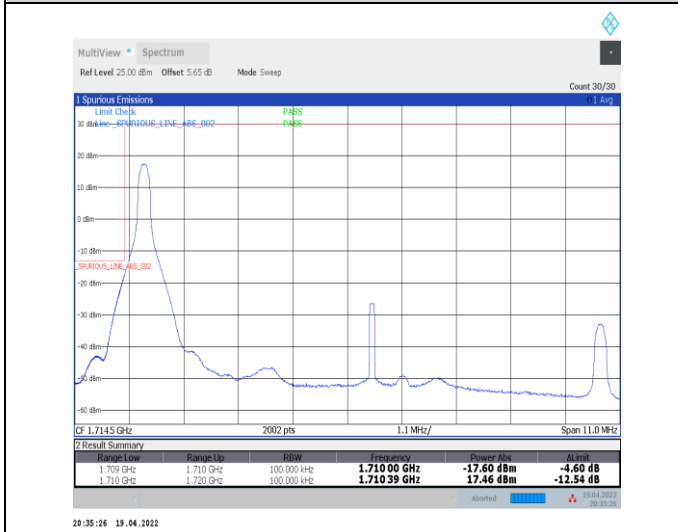
1-N66-PC3-15-10-L-4-CP-QPSK-Edge_1RB_Left-1@0-Ant0-seegraph-PASS-see graph
