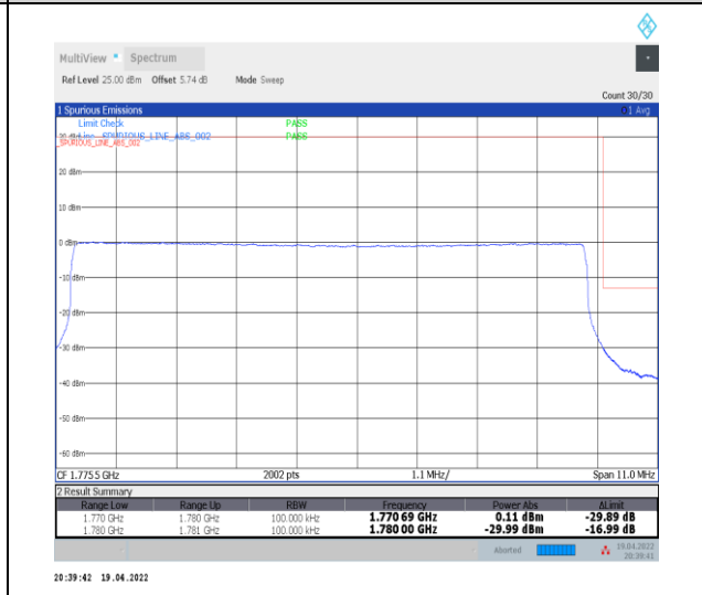
1-N66-PC3-15-10-H-6-CP-QPSK-Outer_Full-52@0-Ant0-seegraph-PASS-see graph
