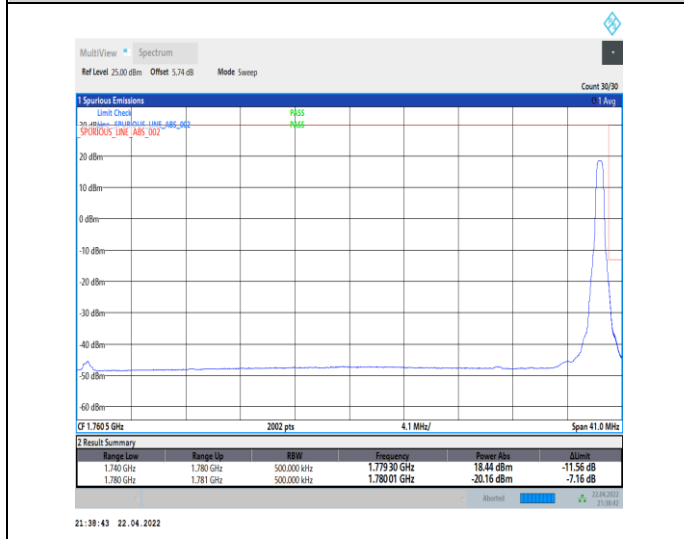
1-N66-PC3-15-40-H-5-CP-QPSK-Edge_1RB_Right-1@215-Ant0-seegraph-PASS-see graph
