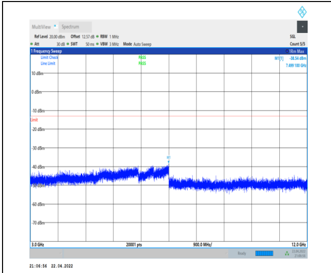
1-N66-PC3-15-40-H-1-DFT-PI2BPSK-Inner_1RB_Le ft-1@1-3000-12000-Ant0--38.54--13-PASS
