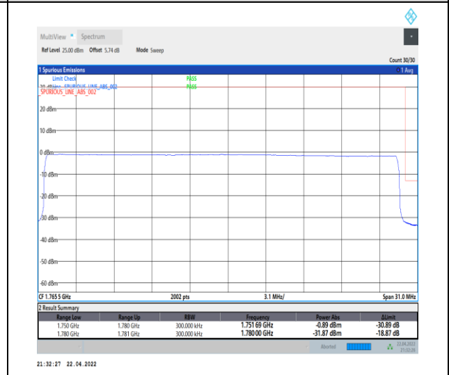
1-N66-PC3-15-30-H-6-CP-QPSK-Outer_Full-160@0-Ant0-seegraph-PASS-see graph
