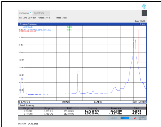
1-N66-PC3-15-15-H-2-DFT-PI2BPSK-Edge_1RB_Right-t-1@78-Ant0-seegraph-PASS-see graph
