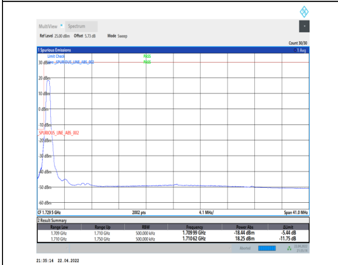
1-N66-PC3-15-40-L-4-CP-QPSK-Edge_1RB_Left-1@0-Ant0-seegraph-PASS-see graph
