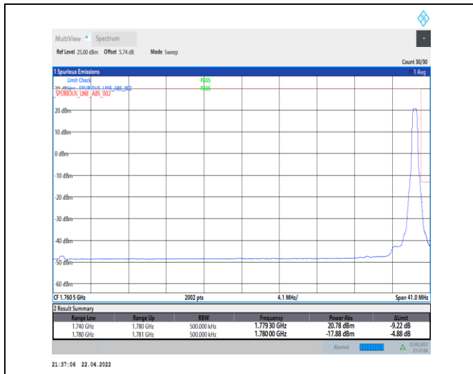
1-N66-PC3-15-40-H-2-DFT-PI2BPSK-Edge_1RB_Right-t-1@215-Ant0-seegraph-PASS-see graph
