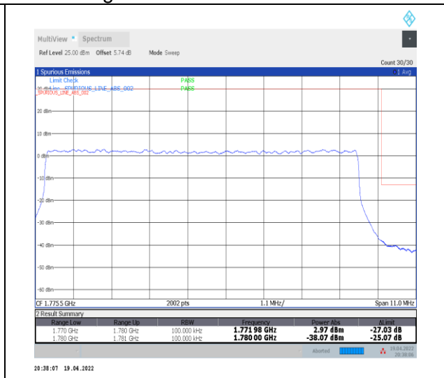
1-N66-PC3-15-10-H-3-DFT-PI2BPSK-Outer_Full-50@0-Ant0-seegraph-PASS-see graph
