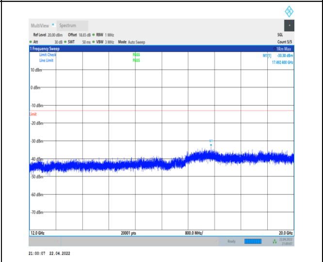
1-N66-PC3-15-40-M-1-DFT-PI2BPSK-Inner_1RB_Le ft-1@1-12000-20000-Ant0--33.38--13-PASS
