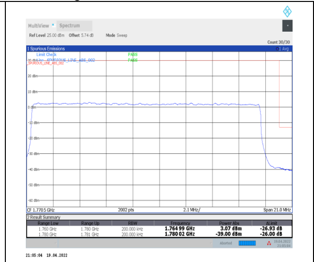
1-N66-PC3-15-20-H-3-DFT-PI2BPSK-Outer_Full-100@0-Ant0-seegraph-PASS-see graph
