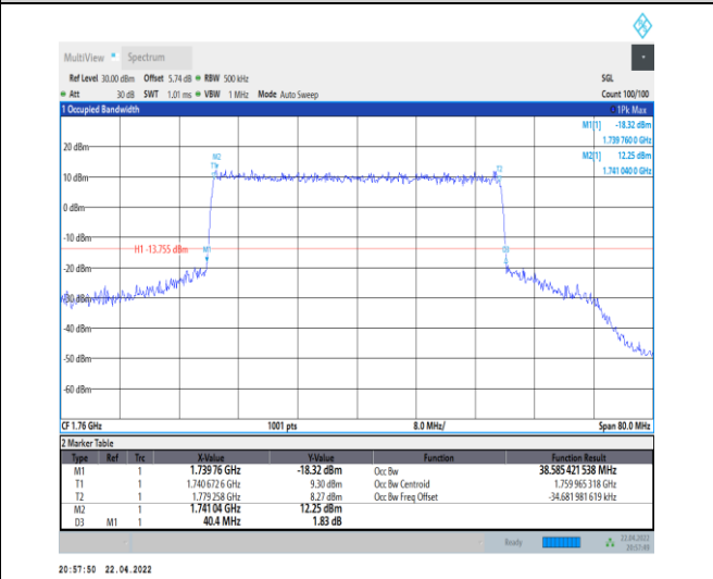
1-N66-PC3-15-40-H-7-CP-16QAM-Outer_Full-216 @ 0-Ant0-38.585-40.400-≤40-PASS
