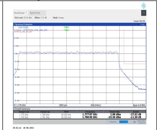
1-N66-PC3-15-5-H-3-DFT-PI2BPSK-Outer_Full-25@0-Ant0-seegraph-PASS-see graph
