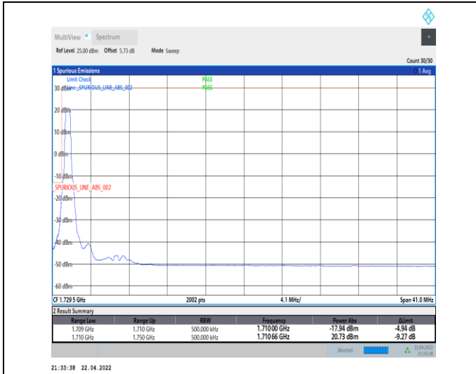
1-N66-PC3-15-40-L-1-DFT-PI2BPSK-Edge_1RB_Left-1@0-Ant0-seegraph-PASS-see graph
