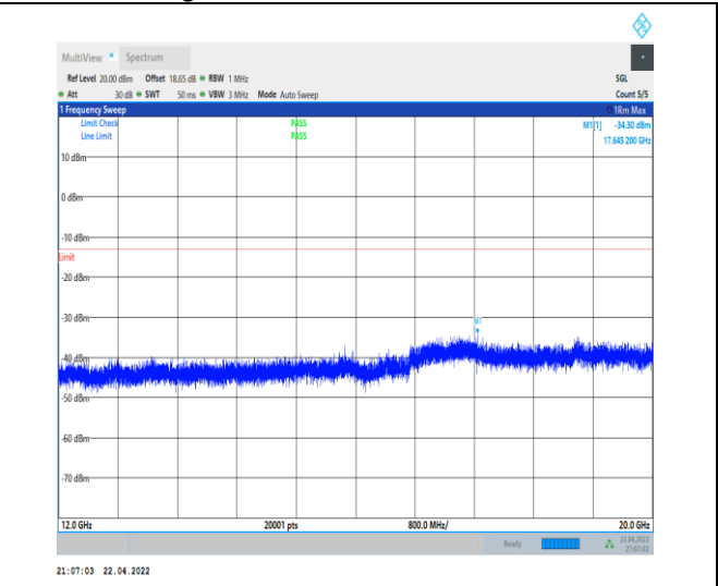
1-N66-PC3-15-40-H-1-DFT-PI2BPSK-Inner_1RB_Lef t-1@1-12000-20000-Ant0--34.30--13-PASS
