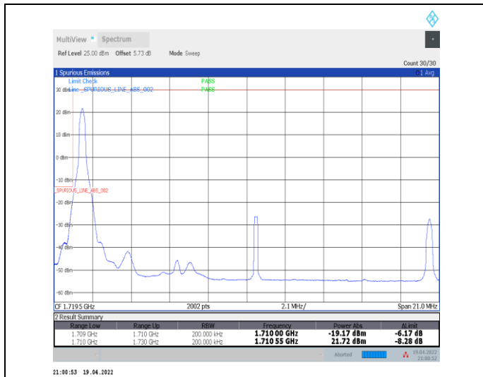
1-N66-PC3-15-20-L-1-DFT-PI2BPSK-Edge_1RB_Left-1@0-Ant0-seegraph-PASS-see graph
