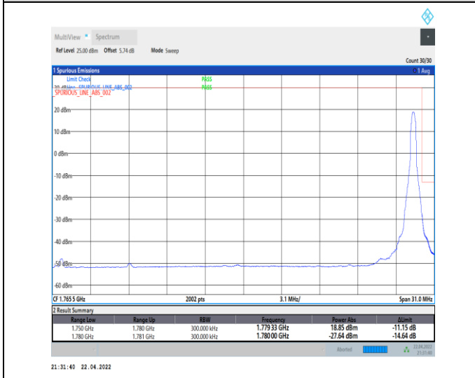
1-N66-PC3-15-30-H-5-CP-QPSK-Edge_1RB_Right-1@159-Ant0-seegraph-PASS-see graph
