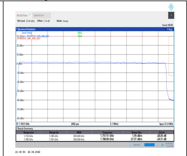
1-N66-PC3-15-30-H-3-DFT-PI2BPSK-Outer_Full-160@0-Ant0-seegraph-PASS-see graph
