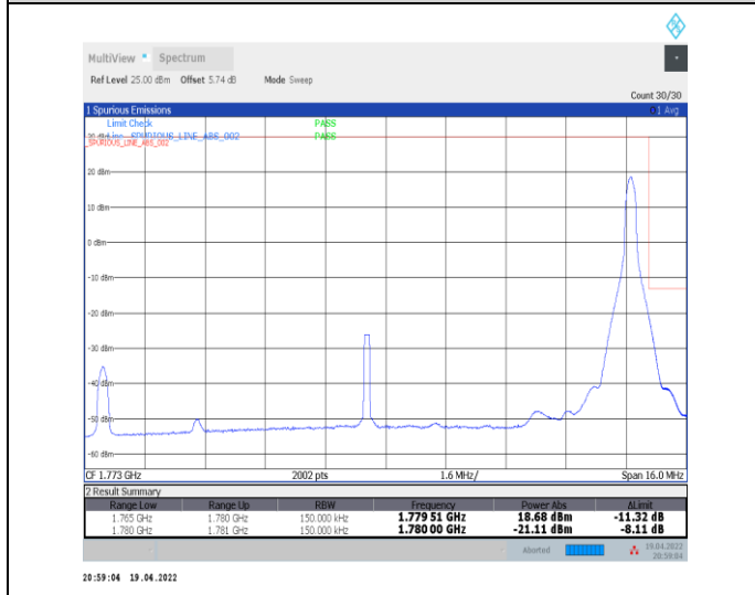
1-N66-PC3-15-15-H-5-CP-QPSK-Edge_1RB_Right-1@78-Ant0-seegraph-PASS-see graph
