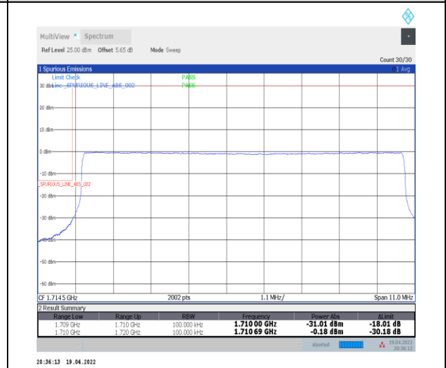
1-N66-PC3-15-10-L-6-CP-QPSK-Outer_Full-52@0-Ant0-seegraph-PASS-see graph
