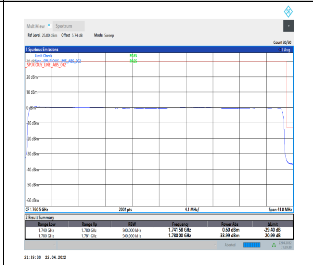
1-N66-PC3-15-40-H-6-CP-QPSK-Outer_Full-216@0-Ant0-seegraph-PASS-see graph
