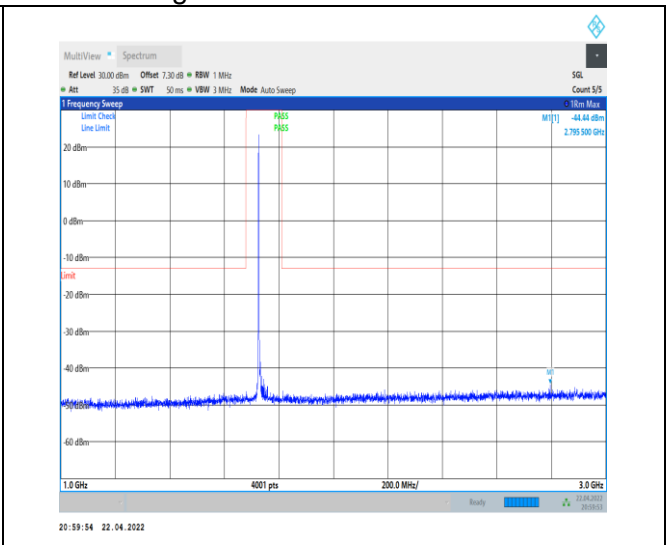
1-N66-PC3-15-40-M-1-DFT-PI2BPSK-Inner_1RB_Le ft-1@1-1000-3000-Ant0--44.44--13-PASS
