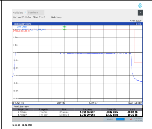
1-N66-PC3-15-15-H-6-CP-QPSK-Outer_Full-79@0-Ant0-seegraph-PASS-see graph
