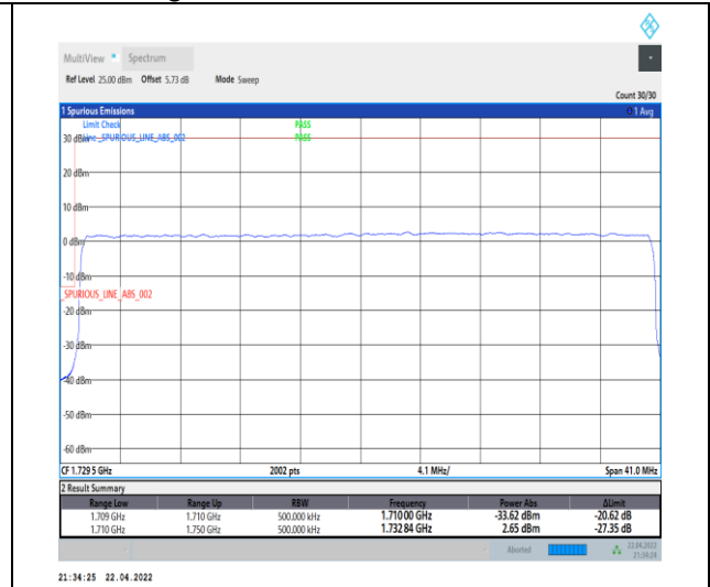
1-N66-PC3-15-40-L-3-DFT-PI2BPSK-Outer_Full-216@0-Ant0-seegraph-PASS-see graph
