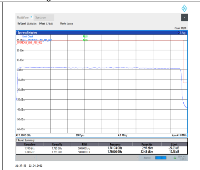
1-N66-PC3-15-40-H-3-DFT-PI2BPSK-Outer_Full-216@0-Ant0-seegraph-PASS-see graph
