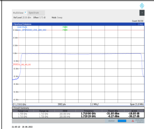
1-N66-PC3-15-20-L-6-CP-QPSK-Outer_Full-106@0-Ant0-seegraph-PASS-see graph
