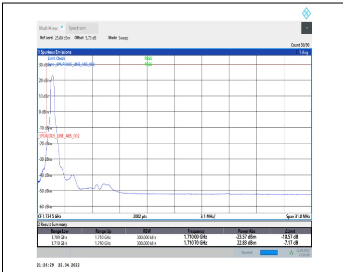
1-N66-PC3-15-30-L-1-DFT-PI2BPSK-Edge_1RB_Left-1@0-Ant0-seegraph-PASS-see graph
