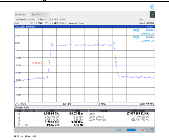
1-N66-PC3-15-20-L-5-DFT-256QAM-Outer_Full-100 @0-Ant0-17.907-19.040-≤20-PASS
