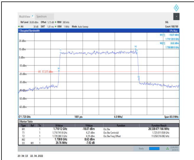
1-N66-PC3-15-30-L-9-CP-256QAM-Outer_Full-160 @0-Ant0-28.538-29.760-≤30-PASS
