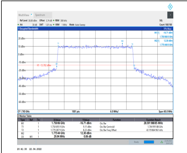
1-N66-PC3-15-30-H-7-CP-16QAM-Outer_Full-160@ 0-Ant0-28.592-29.940-≤30-PASS
