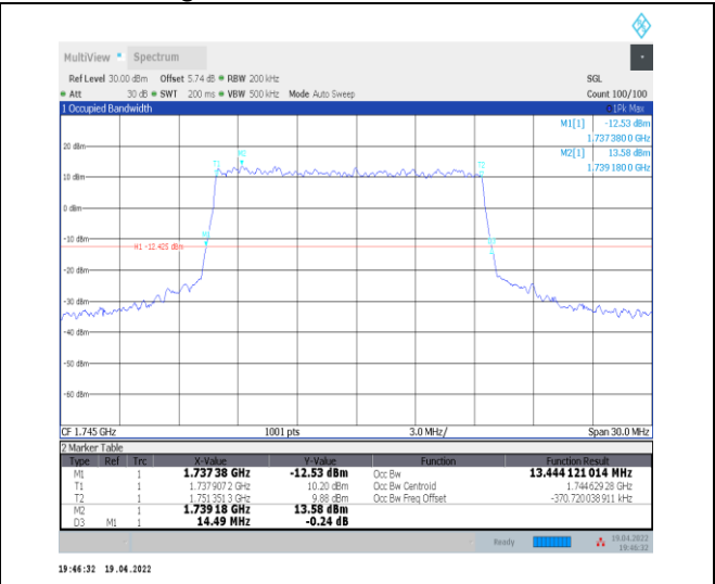
1-N66-PC3-15-15-M-3-DFT-16QAM-Outer_Full-75 @ 0-Ant0-13.444-14.490-≤15-PASS
