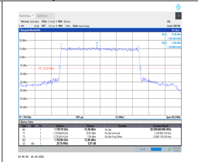
1-N66-PC3-15-30-H-4-DFT-64QAM-Outer_Full-160 @ 0-Ant0-28.599-29.760-≤30-PASS
