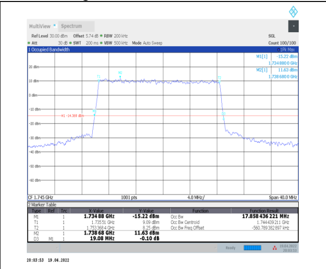
1-N66-PC3-15-20-M-4-DFT-64QAM-Outer_Full-100 @ 0-Ant0-17.858-19.080-≤20-PASS
