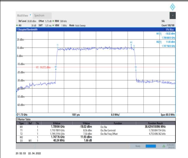
1-N66-PC3-15-40-L-5-DFT-256QAM-Outer_Full-216 @ 0-Ant0-38.43-40.240-≤40-PASS
