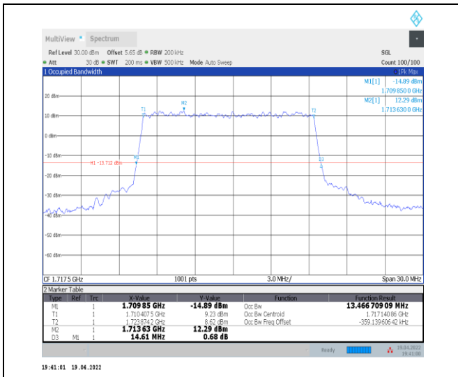
1-N66-PC3-15-15-L-3-DFT-16QAM-Outer_Full-75@ 0-Ant0-13.467-14.610-≤15-PASS
