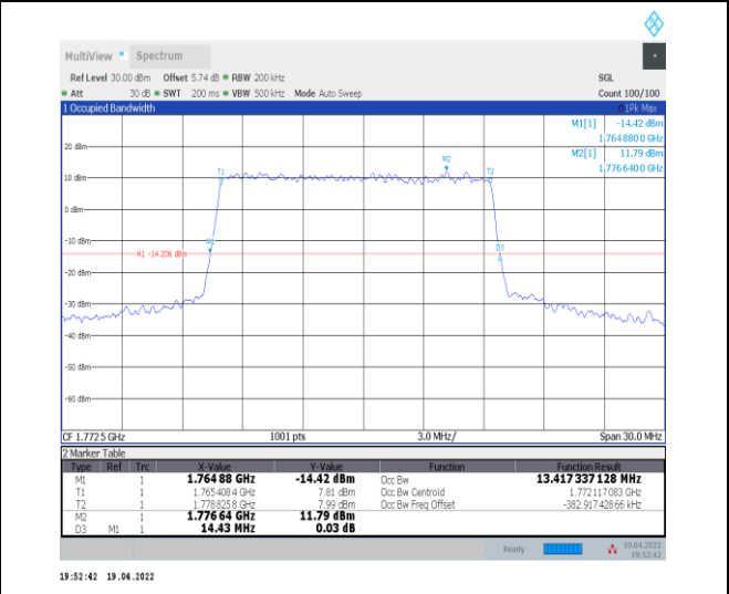
1-N66-PC3-15-15-H-4-DFT-64QAM-Outer_Full-75@ 0-Ant0-13.417-14.430-≤15-PASS
