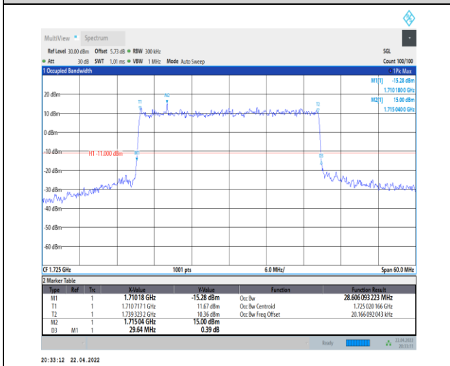
1-N66-PC3-15-30-L-3-DFT-16QAM-Outer_Full-160 @0-Ant0-28.606-29.640-≤30-PASS
