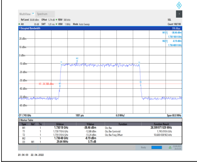
1-N66-PC3-15-30-M-2-DFT-PI2BPSK-Outer_Full-160 @0-Ant0-28.6-29.640-≤30-PASS
