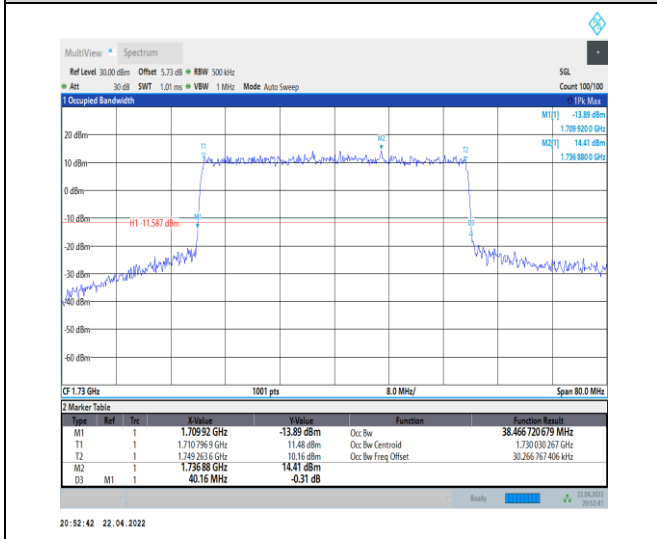
1-N66-PC3-15-40-L-4-DFT-64QAM-Outer_Full-216 @ 0-Ant0-38.467-40.160-≤40-PASS
