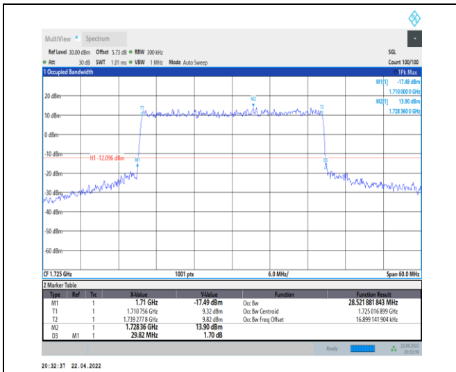
1-N66-PC3-15-30-L-1-DFT-QPSK-Outer_Full-160@ 0-Ant0-28.522-29.820-≤30-PASS
