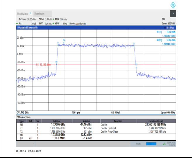
1-N66-PC3-15-30-M-3-DFT-16QAM-Outer_Full-160 @0-Ant0-28.555-30.000-≤30-PASS
