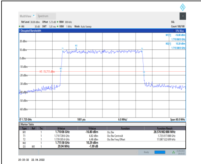
1-N66-PC3-15-30-L-5-DFT-256QAM-Outer_Full-160 @ 0-Ant0-28.577-29.940-≤30-PASS
