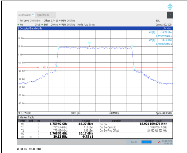
1-N66-PC3-15-20-H-6-CP-QPSK-Outer_Full-106@0 -Ant0-18.921-20.120-≤20-PASS
