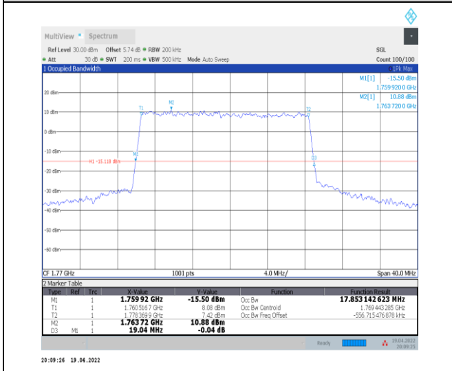
1-N66-PC3-15-20-H-4-DFT-64QAM-Outer_Full-100 @0-Ant0-17.853-19.040-≤20-PASS
