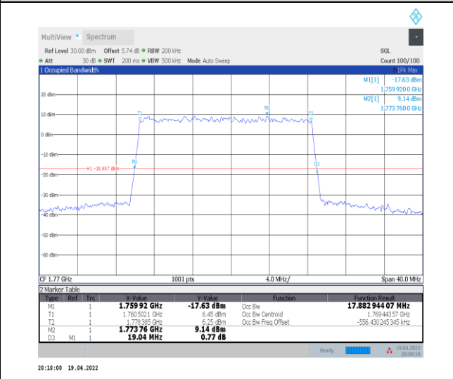
1-N66-PC3-15-20-H-5-DFT-256QAM-Outer_Full-100 @0-Ant0-17.883-19.040-≤20-PASS
