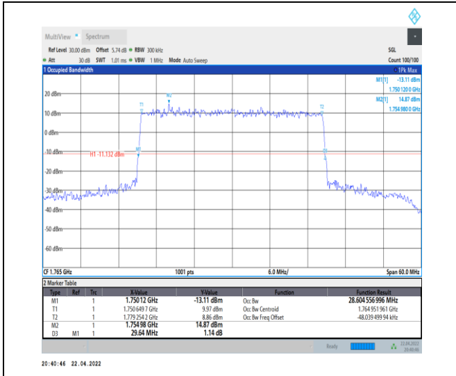
1-N66-PC3-15-30-H-3-DFT-16QAM-Outer_Full-160 @ 0-Ant0-28.605-29.640-≤30-PASS
