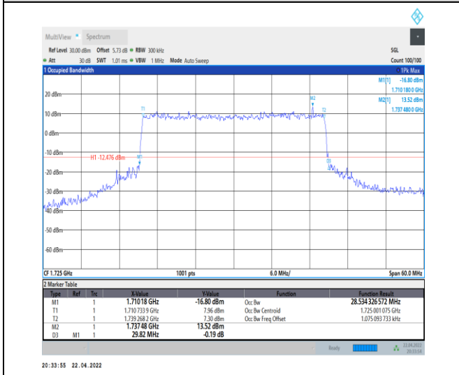
1-N66-PC3-15-30-L-7-CP-16QAM-Outer_Full-160 @ 0-Ant0-28.534-29.820-≤30-PASS
