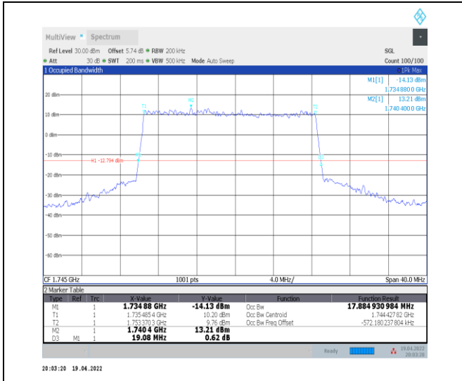
1-N66-PC3-15-20-M-3-DFT-16QAM-Outer_Full-100 @ 0-Ant0-17.885-19.080-≤20-PASS
