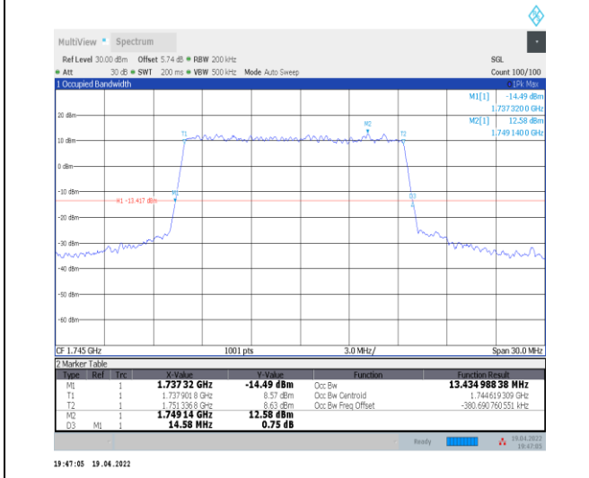
1-N66-PC3-15-15-M-4-DFT-64QAM-Outer_Full-75 @ 0-Ant0-13.435-14.580-≤15-PASS
