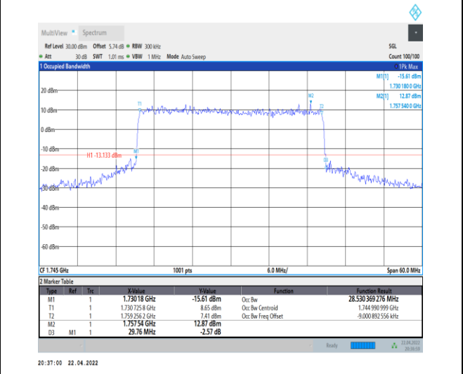
1-N66-PC3-15-30-M-7-CP-16QAM-Outer_Full-160 @ 0-Ant0-28.53-29.760-≤30-PASS
