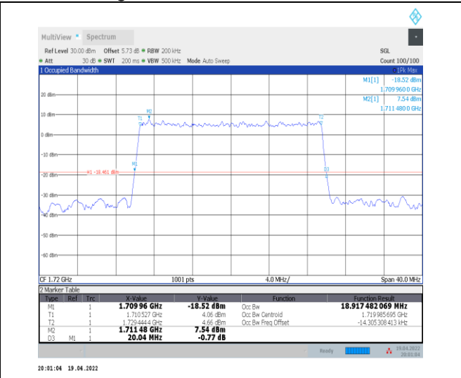
1-N66-PC3-15-20-L-9-CP-256QAM-Outer_Full-106 @0-Ant0-18.917-20.040-≤20-PASS
