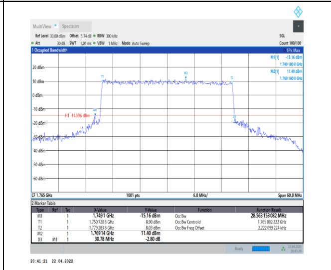
1-N66-PC3-15-30-H-6-CP-QPSK-Outer_Full-160 @ 0-Ant0-28.563-30.780-≤30-PASS
