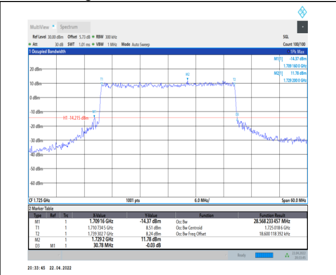
1-N66-PC3-15-30-L-6-CP-QPSK-Outer_Full-160 @ 0-Ant0-28.568-30.780-≤30-PASS
