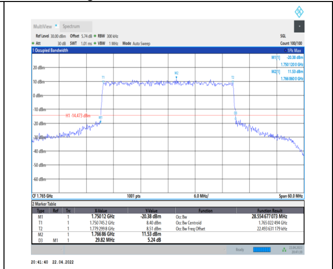
1-N66-PC3-15-30-H-8-CP-64QAM-Outer_Full-160@ 0-Ant0-28.555-29.820-≤30-PASS
