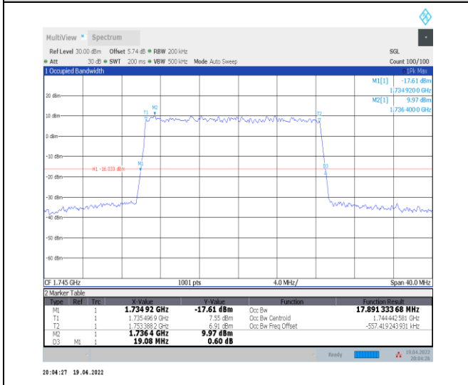
1-N66-PC3-15-20-M-5-DFT-256QAM-Outer_Full-100 @ 0-Ant0-17.891-19.080-≤20-PASS
