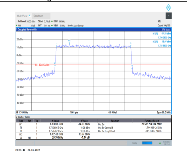
1-N66-PC3-15-30-M-1-DFT-QPSK-Outer_Full-160 @0-Ant0-28.586-29.760-≤30-PASS
