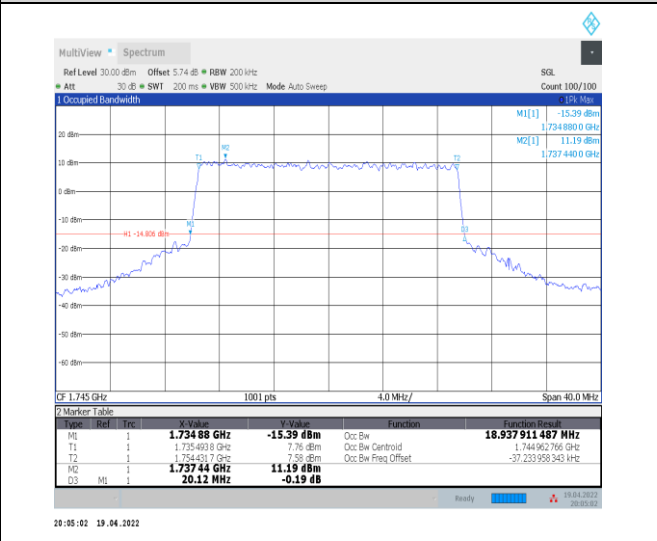
1-N66-PC3-15-20-M-6-CP-QPSK-Outer_Full-106 @ 0-Ant0-18.938-20.120-≤20-PASS
