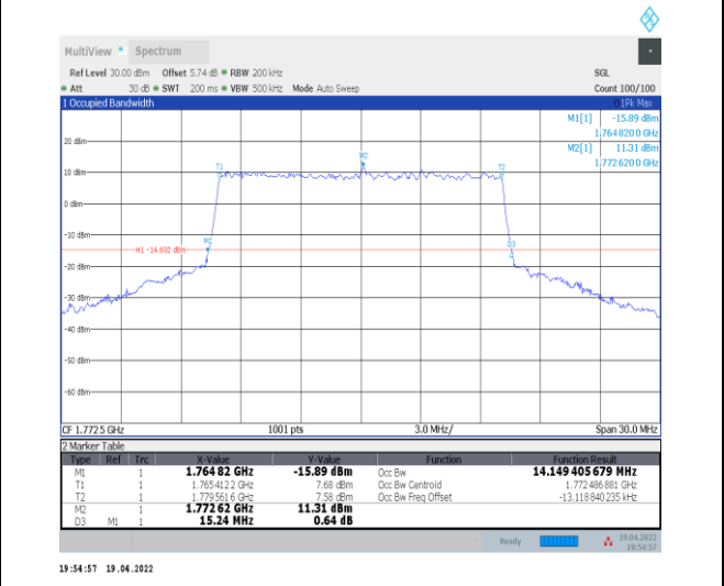
1-N66-PC3-15-15-H-8-CP-64QAM-Outer_Full-79@0 -Ant0-14.149-15.240-≤15-PASS
