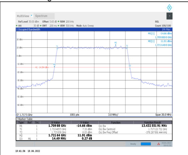
1-N66-PC3-15-15-L-4-DFT-64QAM-Outer_Full-75@ 0-Ant0-13.433-14.490-≤15-PASS
