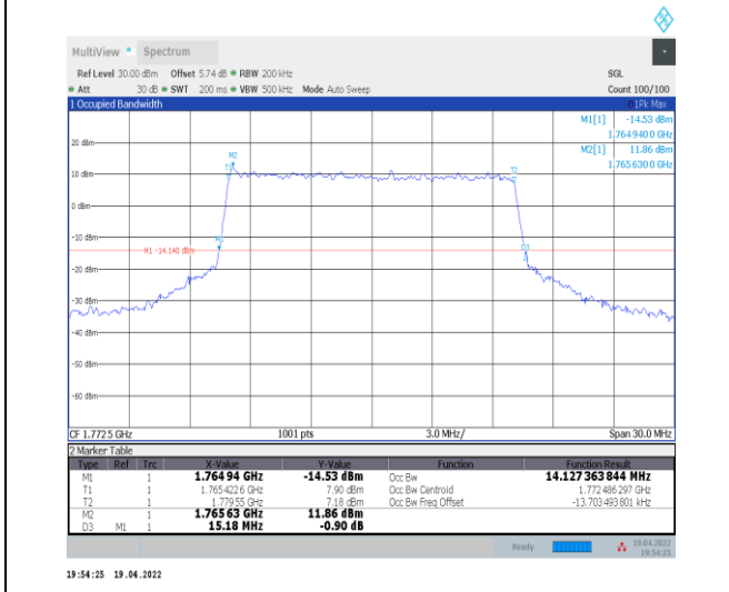
1-N66-PC3-15-15-H-7-CP-16QAM-Outer_Full-79@0 -Ant0-14.127-15.180-≤15-PASS
