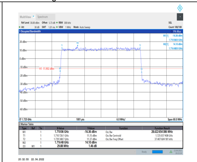
1-N66-PC3-15-30-L-2-DFT-PI2BPSK-Outer_Full-160 @0-Ant0-28.623-29.880-≤30-PASS
