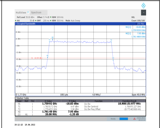
1-N66-PC3-15-20-H-9-CP-256QAM-Outer_Full-106@0 -Ant0-18.908-20.080-≤20-PASS
