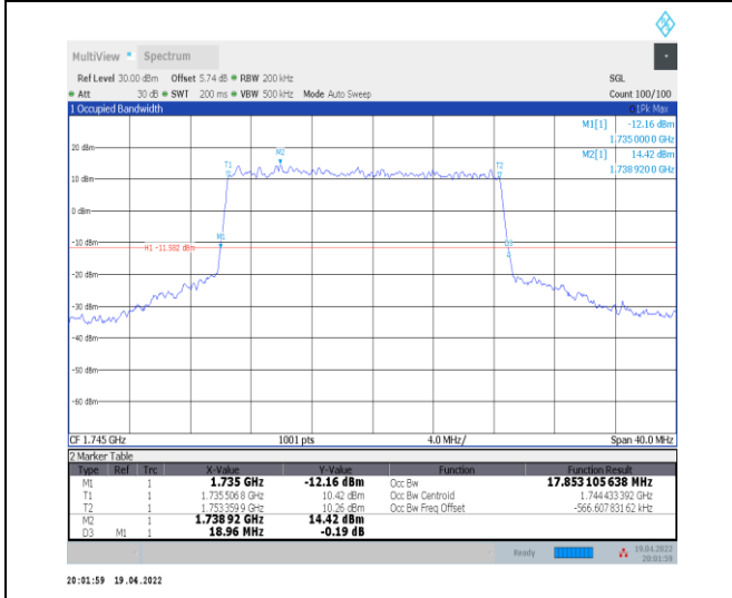
1-N66-PC3-15-20-M-1-DFT-QPSK-Outer_Full-100@ 0-Ant0-17.853-18.960-≤20-PASS
