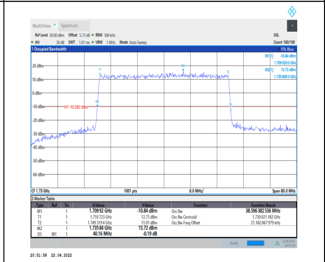
1-N66-PC3-15-40-L-1-DFT-QPSK-Outer_Full-216@0 -Ant0-38.596-40.160-≤40-PASS
