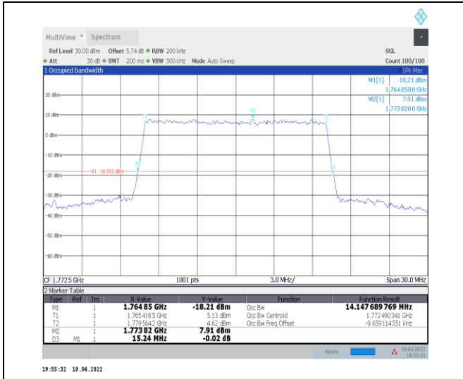
1-N66-PC3-15-15-H-9-CP-256QAM-Outer_Full-79@ 0-Ant0-14.148-15.240-≤15-PASS
