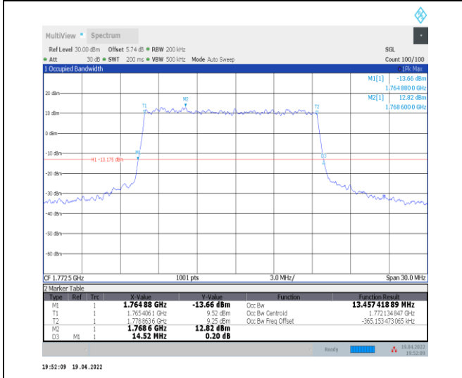
1-N66-PC3-15-15-H-3-DFT-16QAM-Outer_Full-75@ 0-Ant0-13.457-14.520-≤15-PASS
