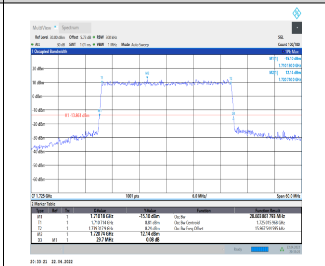
1-N66-PC3-15-30-L-4-DFT-64QAM-Outer_Full-160 @0-Ant0-28.604-29.700-≤30-PASS
