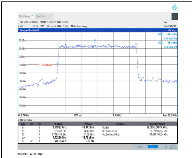
1-N66-PC3-15-40-L-2-DFT-PI2BPSK-Outer_Full-216 @ 0-Ant0-38.506-40.160-≤40-PASS
