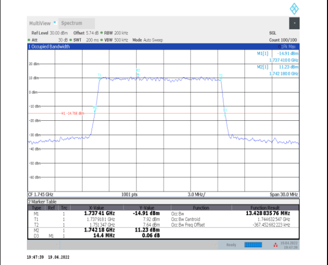
1-N66-PC3-15-15-M-5-DFT-256QAM-Outer_Full-75 @ 0-Ant0-13.429-14.400-≤15-PASS
