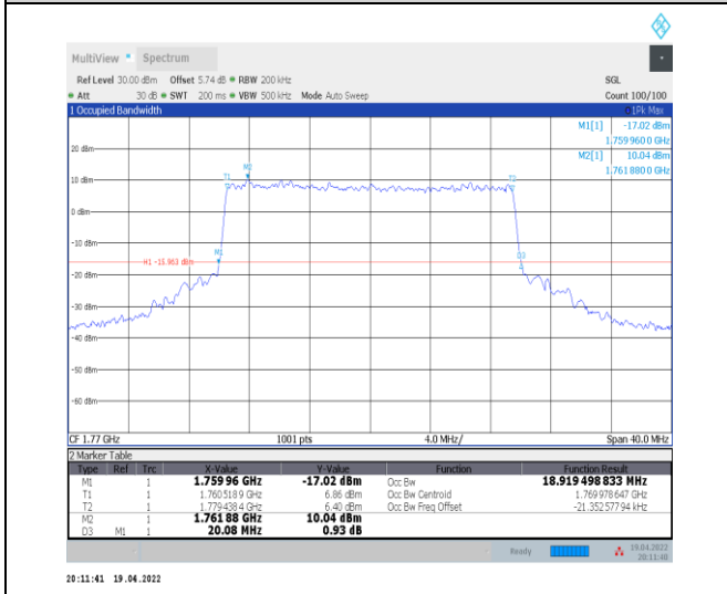
1-N66-PC3-15-20-H-8-CP-64QAM-Outer_Full-106@0 -Ant0-18.919-20.080-≤20-PASS
