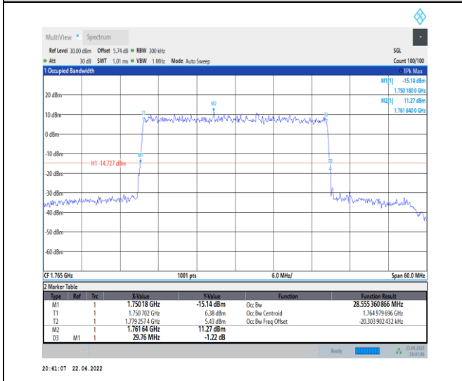
1-N66-PC3-15-30-H-5-DFT-256QAM-Outer_Full-160 @ 0-Ant0-28.555-29.760-≤30-PASS
