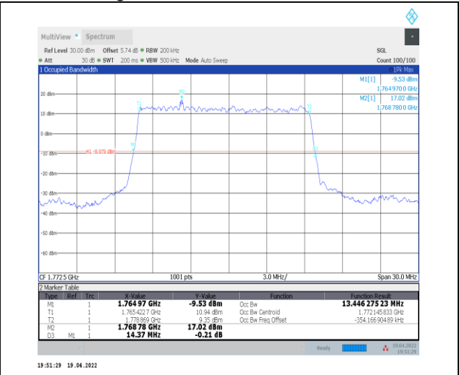
1-N66-PC3-15-15-H-2-DFT-PI2BPSK-Outer_Full-75 @0-Ant0-13.446-14.370-≤15-PASS
