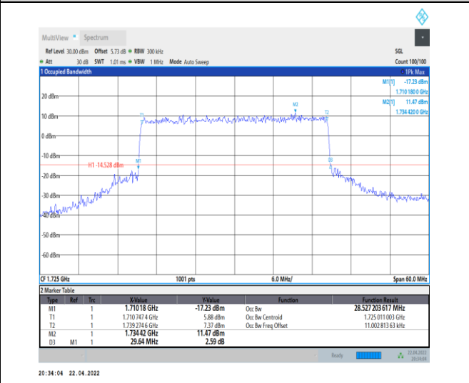
1-N66-PC3-15-30-L-8-CP-64QAM-Outer_Full-160 @ 0-Ant0-28.527-29.640-≤30-PASS
