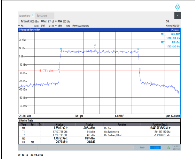
1-N66-PC3-15-30-H-9-CP-256QAM-Outer_Full-160 @0-Ant0-28.444-29.760-≤30-PASS
