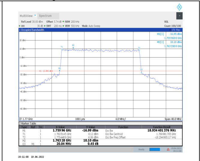
1-N66-PC3-15-20-H-7-CP-16QAM-Outer_Full-106@0 -Ant0-18.934-20.040-≤20-PASS
