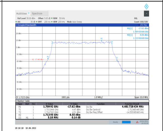
1-N66-PC3-15-5-L-8-CP-64QAM-Outer_Full-25@0-Ant0-4.482-5.180-≤5-PASS
