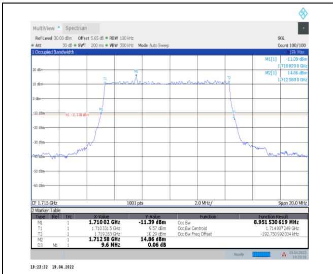
1-N66-PC3-15-10-L-2-DFT-PI2BPSK-Outer_Full-50 @ 0-Ant0-8.952-9.600-≤10-PASS
