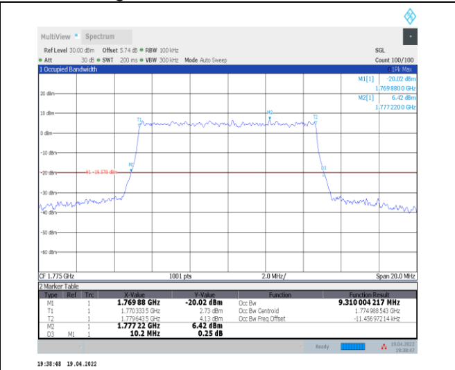
1-N66-PC3-15-10-H-9-CP-256QAM-Outer_Full-52@ 0-Ant0-9.31-10.200-<=10-PASS
