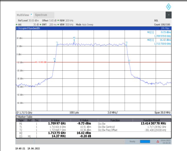
1-N66-PC3-15-15-L-2-DFT-PI2BPSK-Outer_Full-75 @0-Ant0-13.414-14.370-<=15-PASS
