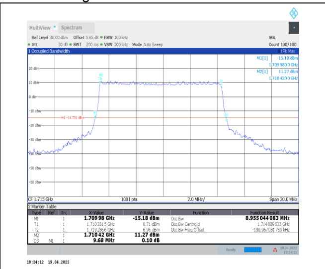
1-N66-PC3-15-10-L-3-DFT-16QAM-Outer_Full-50 @ 0-Ant0-8.955-9.680-≤10-PASS
