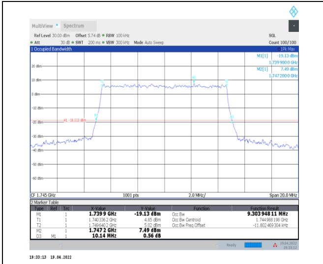
1-N66-PC3-15-10-M-9-CP-256QAM-Outer_Full-52@0-Ant0-9.304-10.140-≤10-PASS
