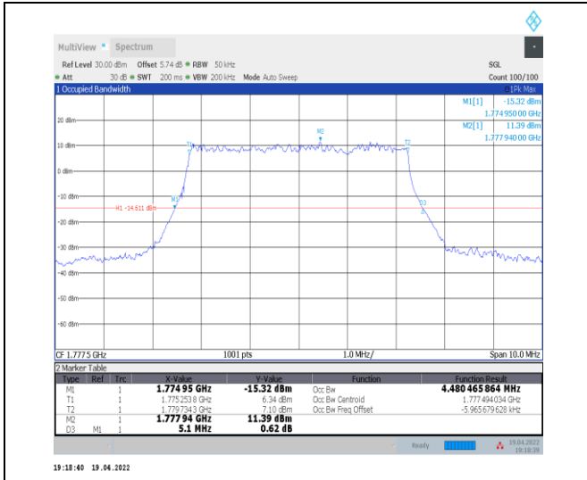
1-N66-PC3-15-5-H-3-DFT-16QAM-Outer_Full-25@0 -Ant0-4.48-5.100-≤5-PASS
