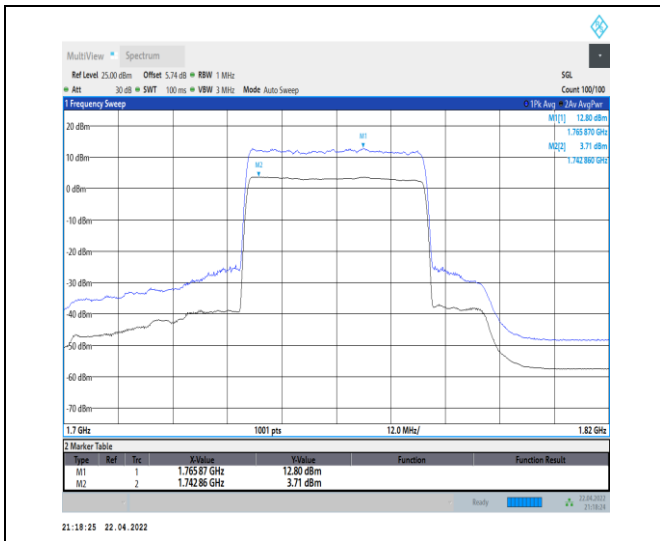
1-N66-PC3-15-40-H-1-DFT-256QAM-Outer_Full-216 @0-Ant0-9.09-100%-0.00-9.09-PASS-≤13
