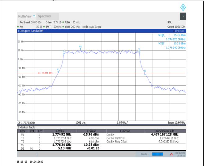
1-N66-PC3-15-5-H-4-DFT-64QAM-Outer_Full-25@0- Ant0-4.474-5.130-≤5-PASS
