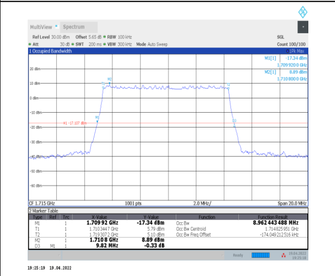
1-N66-PC3-15-10-L-5-DFT-256QAM-Outer_Full-50 @ 0-Ant0-8.962-9.820-≤10-PASS
