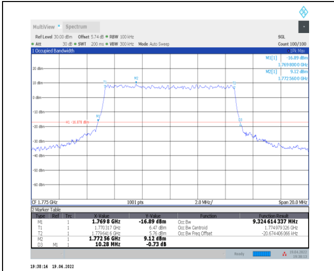
1-N66-PC3-15-10-H-8-CP-64QAM-Outer_Full-52@0 -Ant0-9.325-10.280-<=10-PASS
