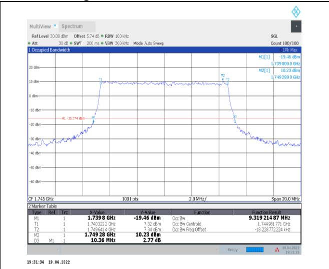
1-N66-PC3-15-10-M-6-CP-QPSK-Outer_Full-52 @ 0-Ant0-9.319-10.360-≤10-PASS
