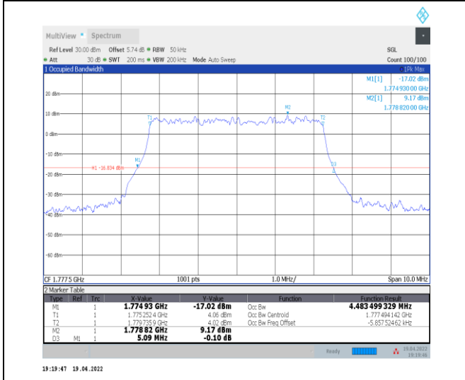
1-N66-PC3-15-5-H-5-DFT-256QAM-Outer_Full-25@ 0-Ant0-4.483-5.090-≤5-PASS
