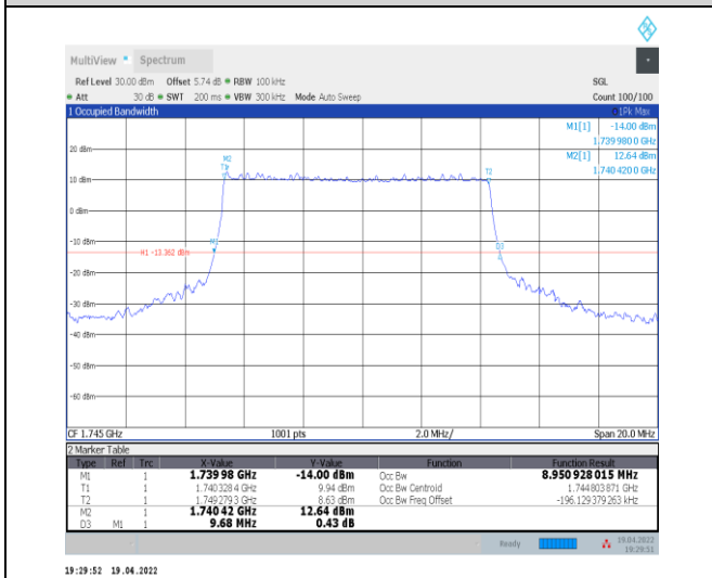
1-N66-PC3-15-10-M-3-DFT-16QAM-Outer_Full-50@0-Ant0-8.951-9.680-≤10-PASS
