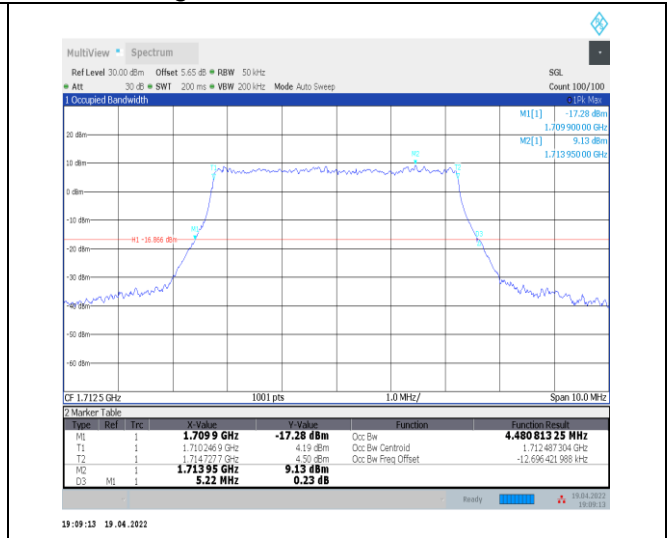
1-N66-PC3-15-5-L-6-CP-QPSK-Outer_Full-25@0-An t0-4.481-5.220-≤5-PASS
