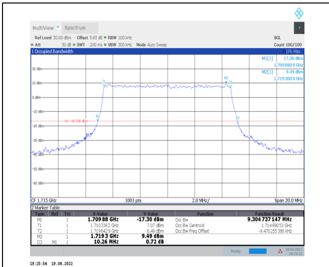
1-N66-PC3-15-10-L-6-CP-QPSK-Outer_Full-52@0-Ant0-9.305-10.260-≤10-PASS
