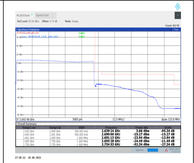
1-N41--30-60-H-6-CP-QPSK-Outer_Full-162@0-A nt0-PASS-see graph
