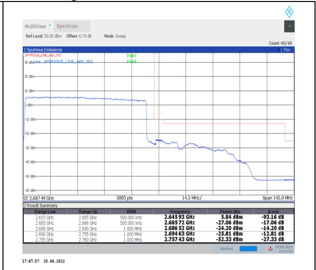
1-N41--30-70-H-3-DFT-PI2BPSK-Outer_Full-180@0-Ant0-PASS-see graph
