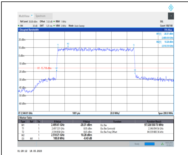
1-N41-PC1-30-100-L-9-CP-256QAM-Outer_Full-273 @ 0-Ant0-97.527-100.800-≤100-PASS
