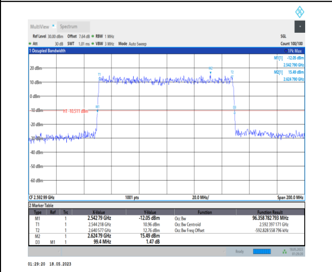
1-N41-PC1-30-100-M-3-DFT-16QAM-Outer_Full-270 @ 0-Ant0-96.359-99.400-≤100-PASS
