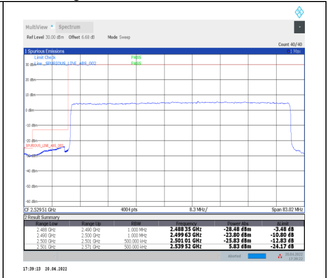
1-N41--30-70-L-3-DFT-PI2BPSK-Outer_Full-180@0-Ant0-PASS-see graph
