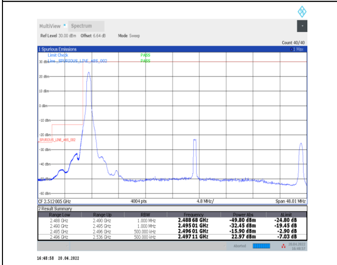
1-N41--30-40-L-4-CP-QPSK-Edge_1RB_Left-1@0-Ant0-PASS-see graph
