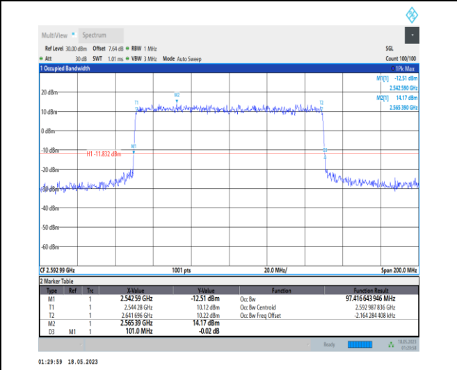
1-N41-PC1-30-100-M-7-CP-16QAM-Outer_Full-273 @0-Ant0-97.417-101.000-≤100-PASS
