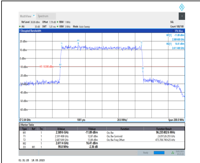
1-N41-PC1-30-100-H-3-DFT-16QAM-Outer_Full-270 @0-Ant0-96.236-99.800-≤100-PASS
