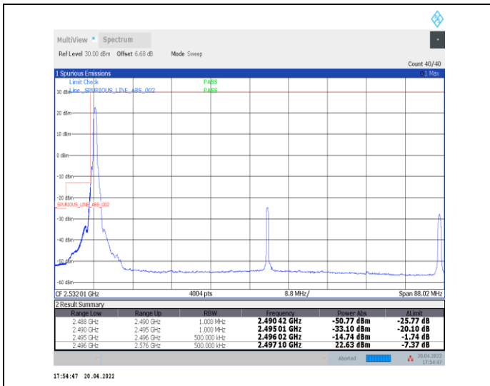
1-N41--30-80-L-1-DFT-PI2BPSK-Edge_1RB_Left-1@0-Ant0-PASS-see graph
