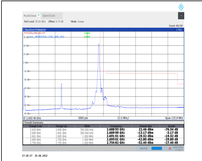
1-N41--30-60-H-2-DFT-PI2BPSK-Edge_1RB_Right-1@ 161-Ant0-PASS-see graph
