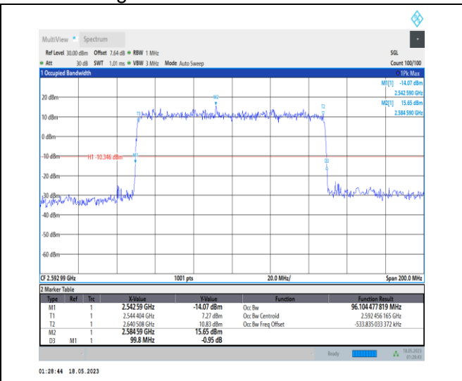
1-N41-PC1-30-100-M-1-DFT-QPSK-Outer_Full-270 @ 0-Ant0-96.104-99.800-≤100-PASS
