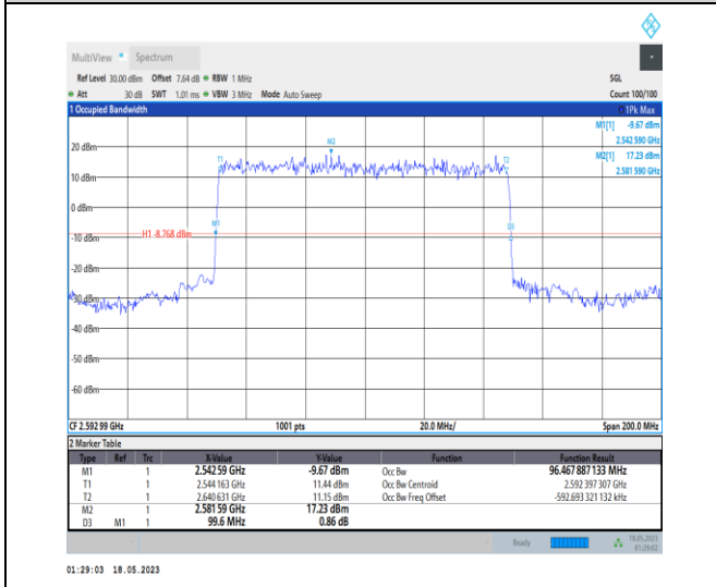
1-N41-PC1-30-100-M-2-DFT-PI2BPSK-Outer_Full-270 @ 0-Ant0-96.468-99.600-≤100-PASS
