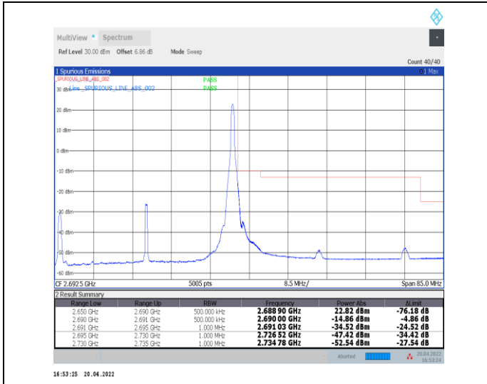
1-N41--30-40-H-2-DFT-PI2BPSK-Edge_1RB_Right-1@105-Ant0-PASS-see graph
