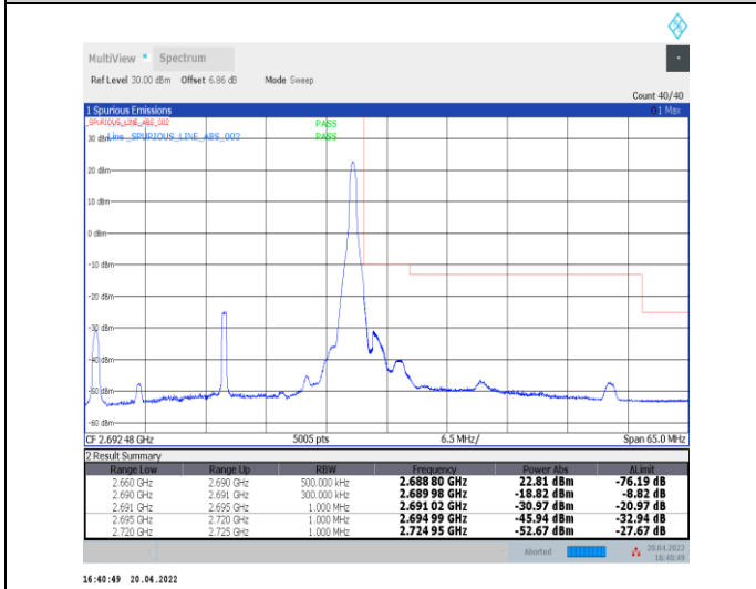
1-N41--30-30-H-5-CP-QPSK-Edge_1RB_Right-1@77-Ant0-PASS-see graph
