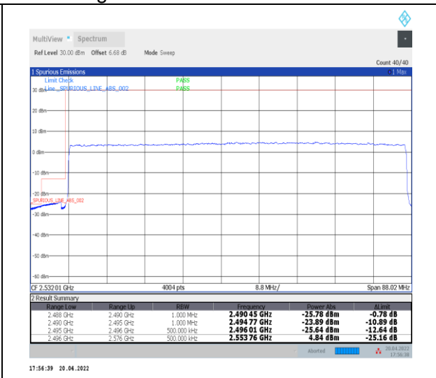
1-N41--30-80-L-3-DFT-PI2BPSK-Outer_Full-216@0-Ant0-PASS-see graph
