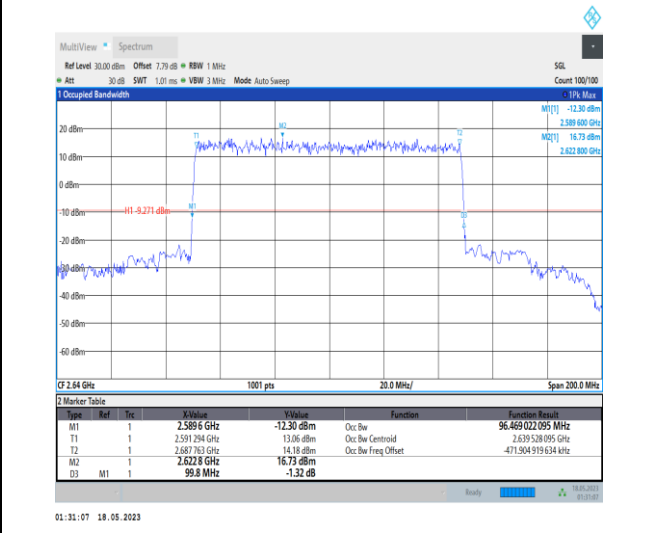
1-N41-PC1-30-100-H-2-DFT-PI2BPSK-Outer_Full-270 @0-Ant0-96.469-99.800-≤100-PASS
