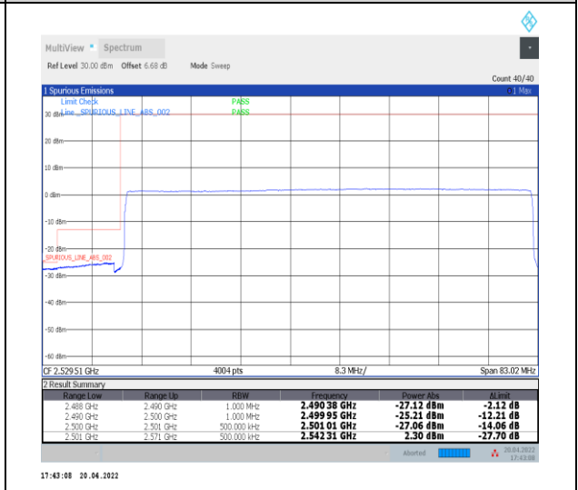
1-N41--30-70-L-6-CP-QPSK-Outer_Full-189@0-Ant0-PASS-see graph
