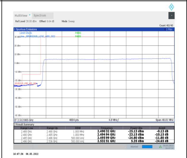
1-N41--30-40-L-6-CP-QPSK-Outer_Full-106@0-Ant0-PASS-see graph
