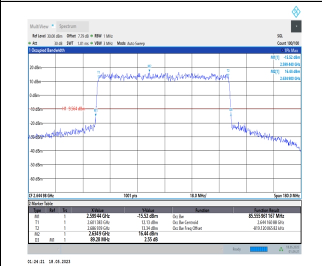
1-N41-PC1-30-90-H-1-DFT-QPSK-Outer_Full-240@ 0-Ant0-85.556-89.280-≤90-PASS
