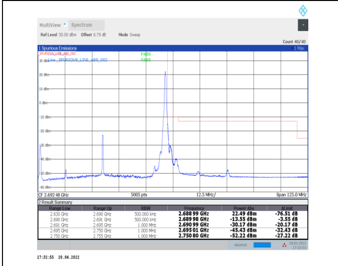
1-N41--30-60-H-5-CP-QPSK-Edge_1RB_Right-1@161 -Ant0-PASS-see graph
