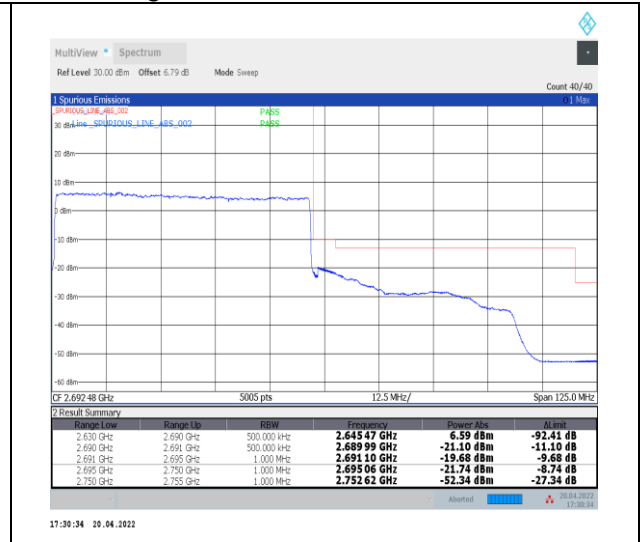
1-N41--30-60-H-3-DFT-PI2BPSK-Outer_Full-162 @0-Ant0-PASS-see graph
