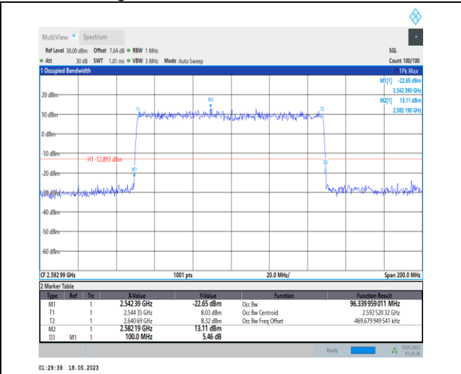
1-N41-PC1-30-100-M-5-DFT-256QAM-Outer_Full-270 @0-Ant0-96.34-100.000-≤100-PASS
