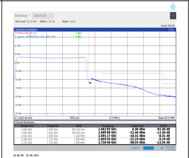
1-N41--30-30-H-6-CP-QPSK-Outer_Full-78@0-Ant0-PASS-see graph
