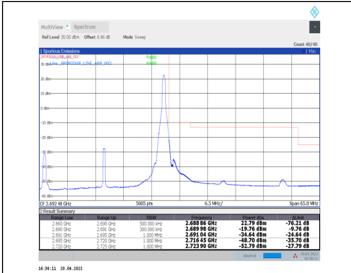
1-N41--30-30-H-2-DFT-PI2BPSK-Edge_1RB_Right-1@77-Ant0-PASS-see graph
