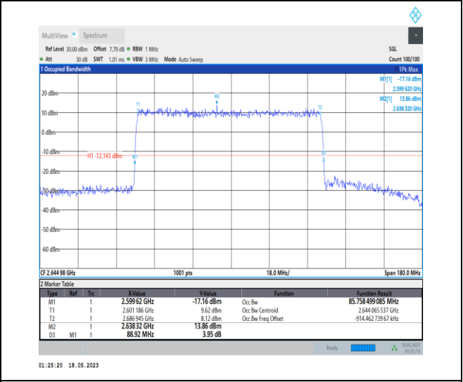
1-N41-PC1-30-90-H-5-DFT-256QAM-Outer_Full-240 @ 0-Ant0-85.758-88.920-≤90-PASS
