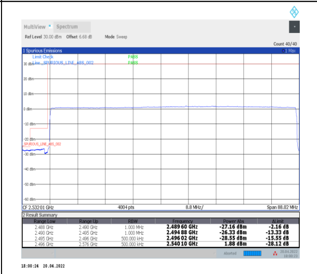
1-N41--30-80-L-6-CP-QPSK-Outer_Full-217@0-Ant0-PASS-see graph
