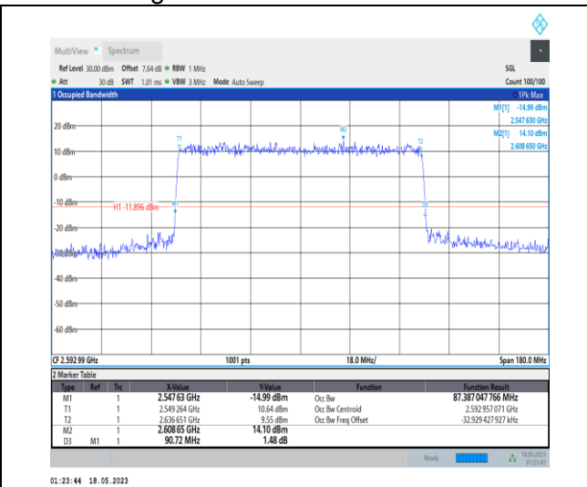
1-N41-PC1-30-90-M-8-CP-64QAM-Outer_Full-245@ 0-Ant0-87.387-90.720-≤90-PASS
