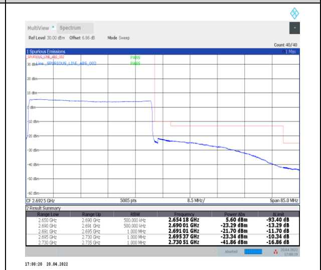
1-N41--30-40-H-6-CP-QPSK-Outer_Full-106@0-Ant0-PASS-see graph
