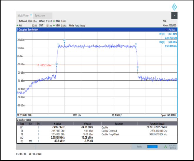
1-N41-PC1-30-80-L-6-CP-QPSK-Outer_Full-217 @ 0-Ant0-77.294-80.800-≤80-PASS
