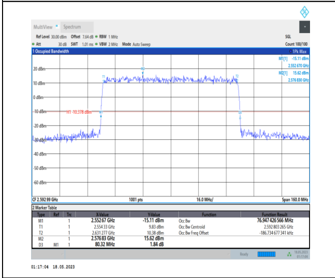
1-N41-PC1-30-80-M-4-DFT-64QAM-Outer_Full-216 @0-Ant0-76.947-80.320-≤80-PASS
