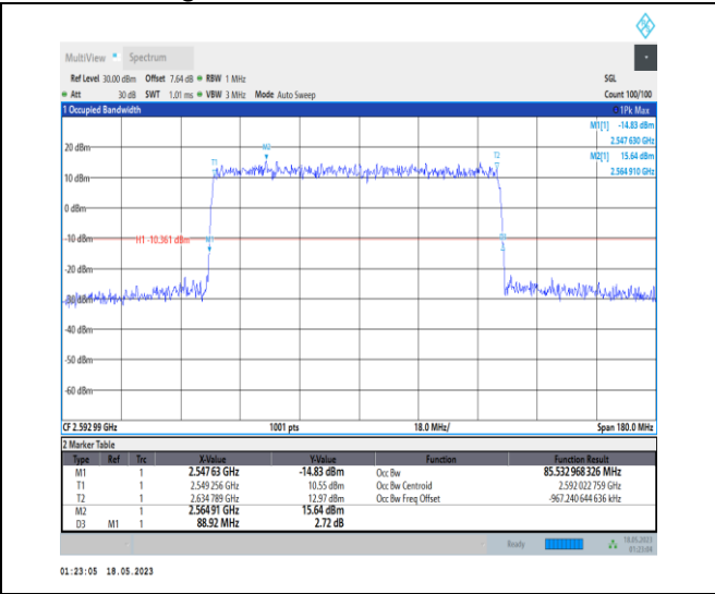
1-N41-PC1-30-90-M-4-DFT-64QAM-Outer_Full-240 @ 0-Ant0-85.533-88.920-≤90-PASS
