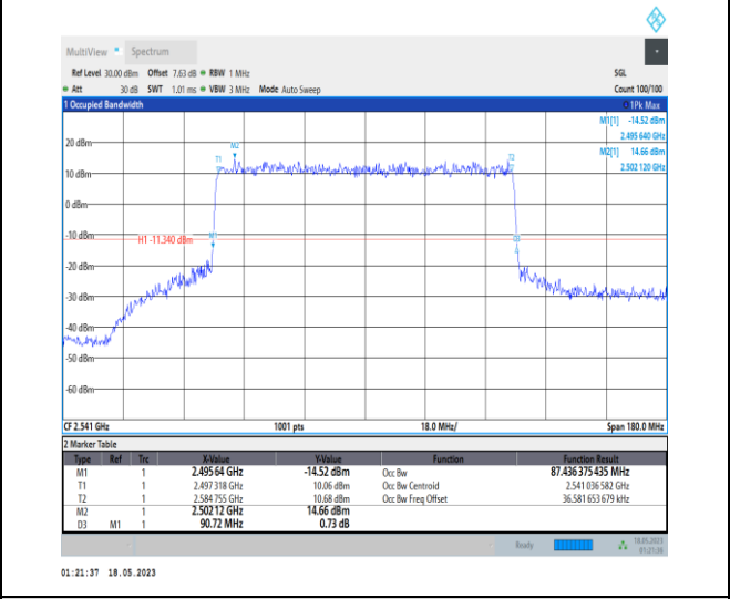
1-N41-PC1-30-90-L-7-CP-16QAM-Outer_Full-245 @ 0-Ant0-87.436-90.720-≤90-PASS
