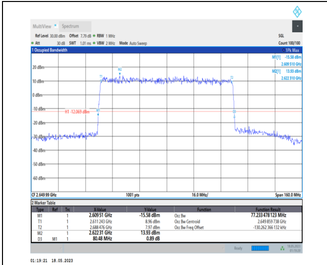
1-N41-PC1-30-80-H-5-DFT-256QAM-Outer_Full-216 @ 0-Ant0-77.233-80.480-≤80-PASS
