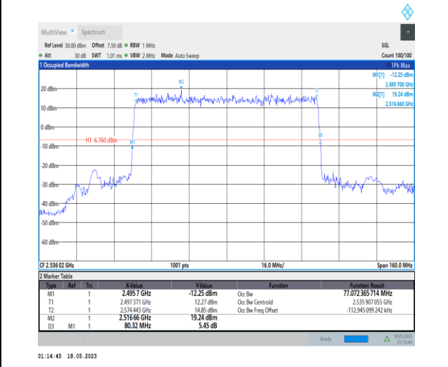
1-N41-PC1-30-80-L-2-DFT-PI2BPSK-Outer_Full-216 @0-Ant0-77.072-80.320-<=80-PASS
