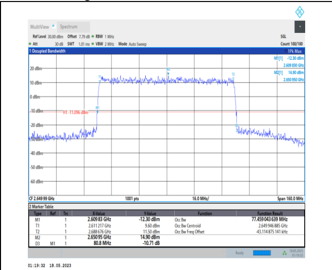
1-N41-PC1-30-80-H-6-CP-QPSK-Outer_Full-217 @ 0-Ant0-77.459-80.800-≤80-PASS
