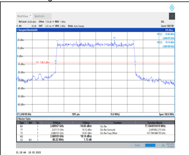
1-N41-PC1-30-80-H-2-DFT-PI2BPSK-Outer_Full-216@0-Ant0-77.105-80.320-≤80-PASS
