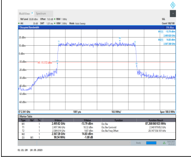
1-N41-PC1-30-90-L-6-CP-QPSK-Outer_Full-245 @ 0-Ant0-87.268-90.540-≤90-PASS
