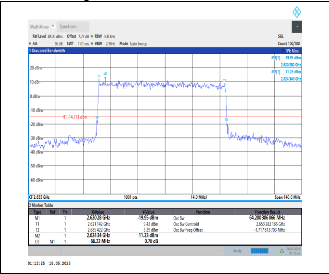
1-N41-PC1-30-70-H-5-DFT-256QAM-Outer_Full-180 @ 0-Ant0-64.28-66.220-≤70-PASS
