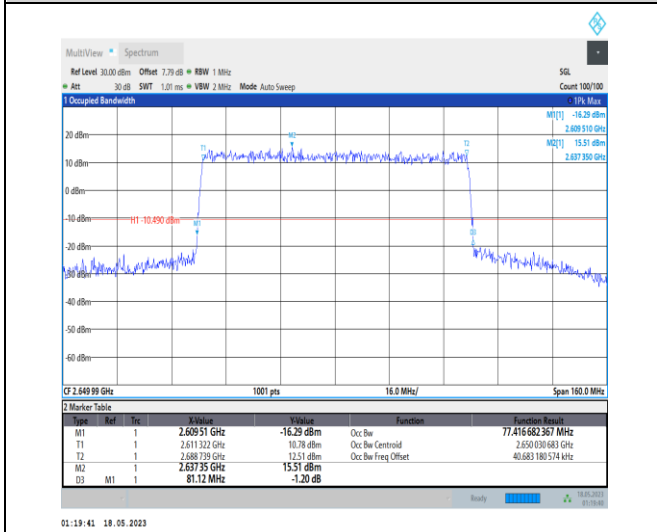
1-N41-PC1-30-80-H-7-CP-16QAM-Outer_Full-217 @ 0-Ant0-77.417-81.120-≤80-PASS
