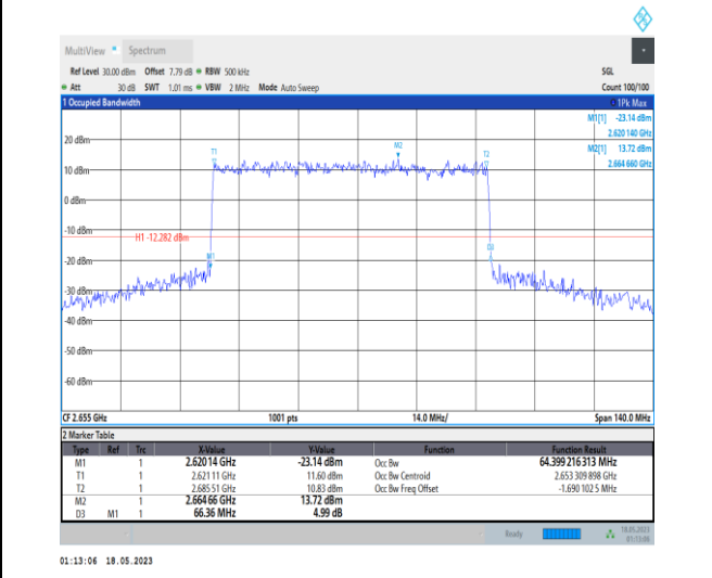
1-N41-PC1-30-70-H-3-DFT-16QAM-Outer_Full-180 @ 0-Ant0-64.399-66.360-≤70-PASS
