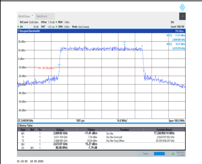
1-N41-PC1-30-80-H-8-CP-64QAM-Outer_Full-217 @ 0-Ant0-77.331-80.480-≤80-PASS
