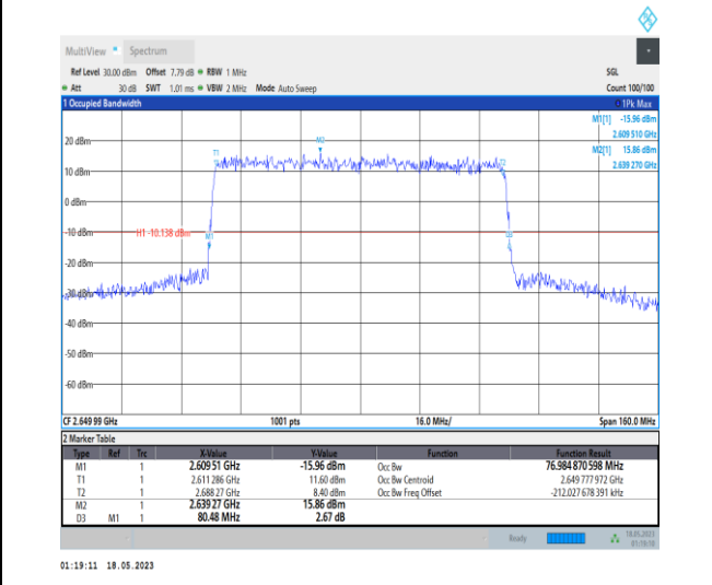
1-N41-PC1-30-80-H-4-DFT-64QAM-Outer_Full-216@0-Ant0-76.985-80.480-≤80-PASS
