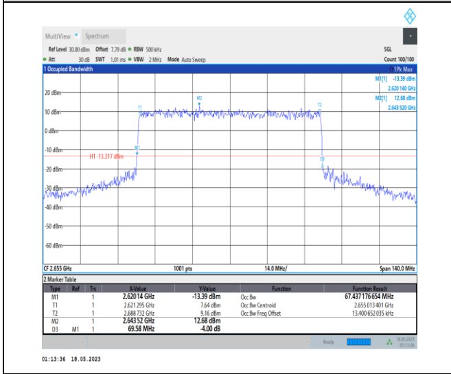
1-N41-PC1-30-70-H-6-CP-QPSK-Outer_Full-189@ 0-Ant0-67.437-69.580-≤70-PASS
