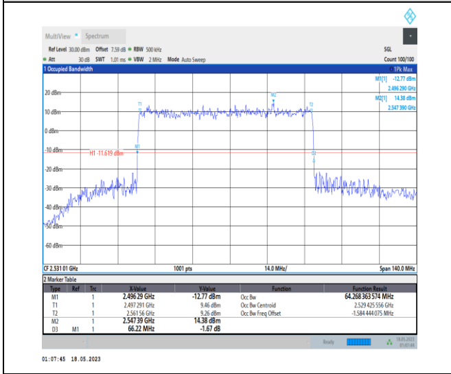
1-N41-PC1-30-70-L-4-DFT-64QAM-Outer_Full-180 @ 0-Ant0-64.268-66.220-≤70-PASS
