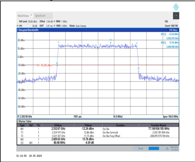
1-N41-PC1-30-80-M-3-DFT-16QAM-Outer_Full-216 @0-Ant0-77.17-80.480-≤80-PASS
