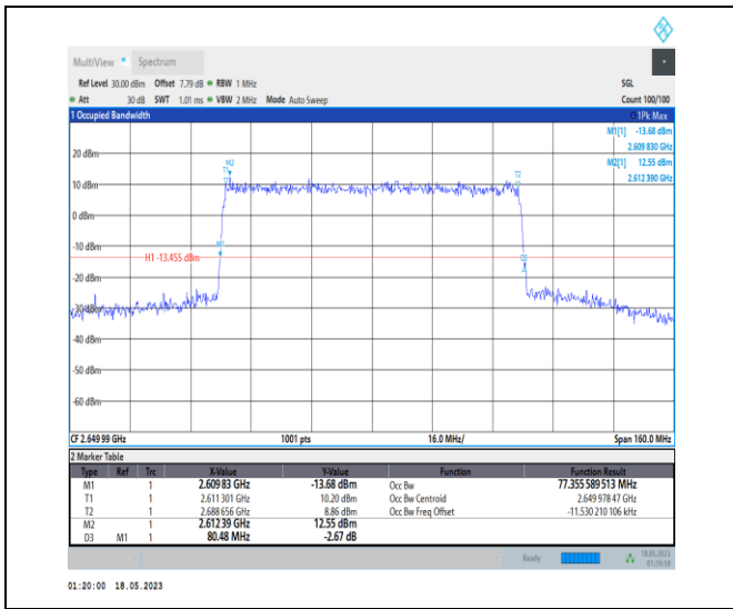
1-N41-PC1-30-80-H-9-CP-256QAM-Outer_Full-217 @ 0-Ant0-77.356-80.480-≤80-PASS
