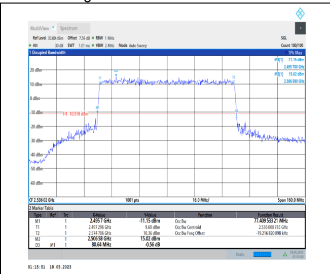
1-N41-PC1-30-80-L-8-CP-64QAM-Outer_Full-217@ 0-Ant0-77.41-80.640-≤80-PASS
