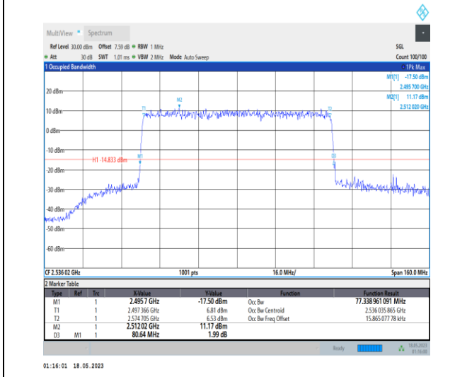
1-N41-PC1-30-80-L-9-CP-256QAM-Outer_Full-217 @0-Ant0-77.339-80.640-≤80-PASS
