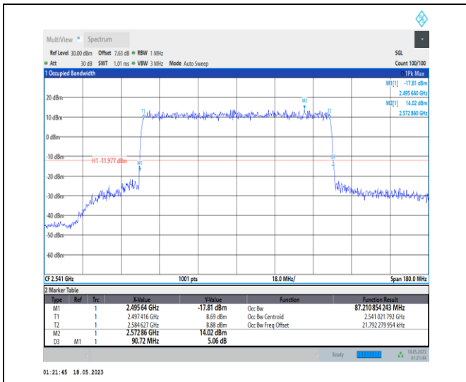
1-N41-PC1-30-90-L-8-CP-64QAM-Outer_Full-245@ 0-Ant0-87.211-90.720-≤90-PASS
