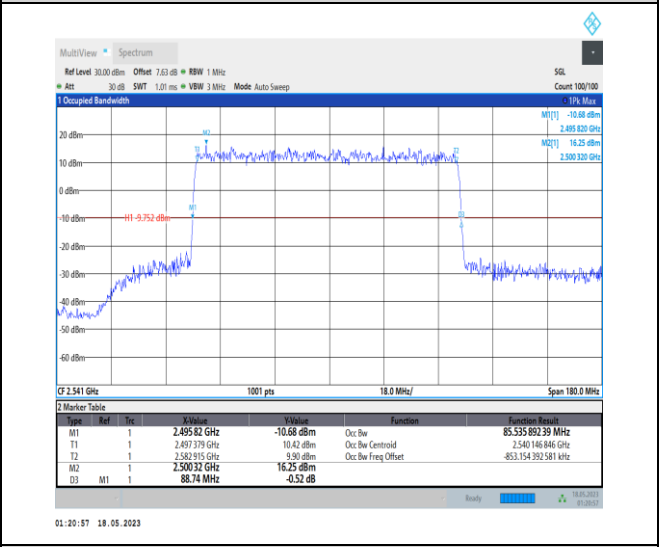
1-N41-PC1-30-90-L-3-DFT-16QAM-Outer_Full-240 @ 0-Ant0-85.536-88.740-≤90-PASS
