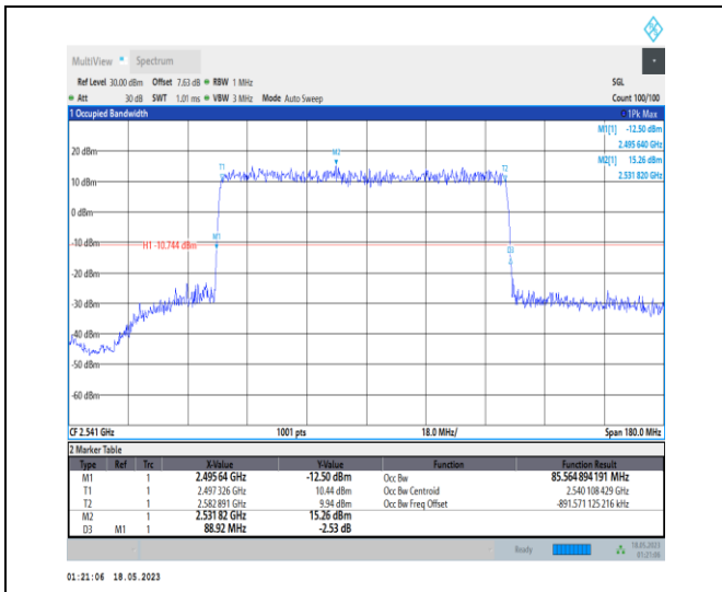
1-N41-PC1-30-90-L-4-DFT-64QAM-Outer_Full-240 @ 0-Ant0-85.565-88.920-≤90-PASS
