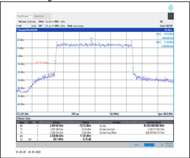
1-N41-PC1-30-90-L-1-DFT-QPSK-Outer_Full-240 @ 0-Ant0-85.565-89.100-≤90-PASS
