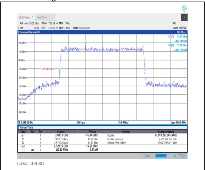
1-N41-PC1-30-80-L-4-DFT-64QAM-Outer_Full-216 @ 0-Ant0-77.011-80.320-≤80-PASS
