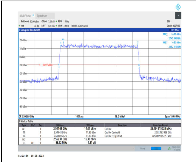
1-N41-PC1-30-90-M-3-DFT-16QAM-Outer_Full-240 @ 0-Ant0-85.465-88.920-≤90-PASS
