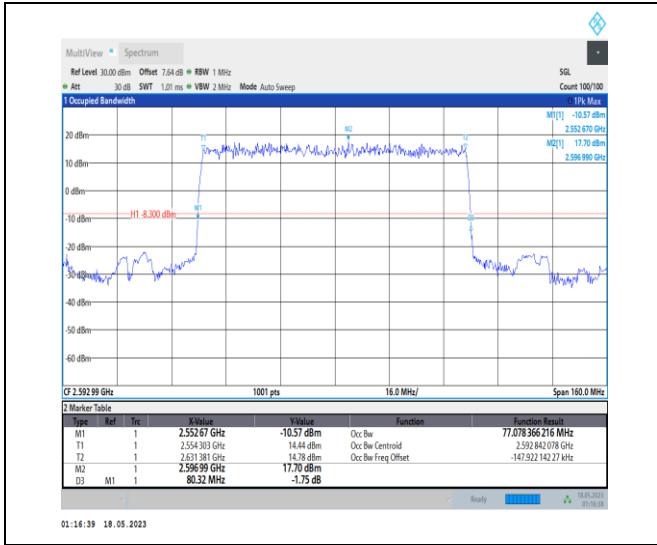
1-N41-PC1-30-80-M-2-DFT-PI2BPSK-Outer_Full-21 @0-Ant0-77.078-80.320-≤80-PASS
