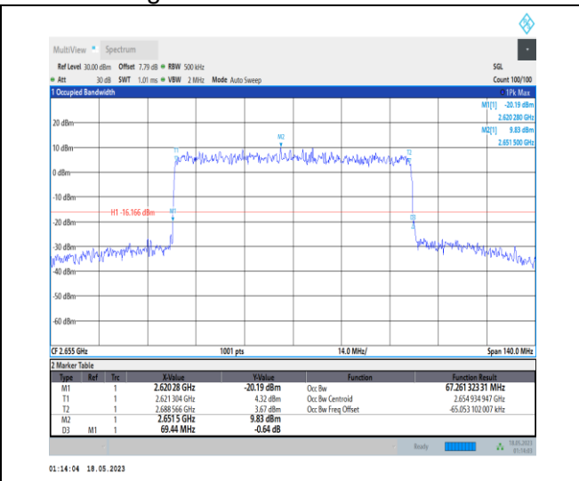
1-N41-PC1-30-70-H-9-CP-256QAM-Outer_Full-189 @0-Ant0-67.261-69.440-<=70-PASS
