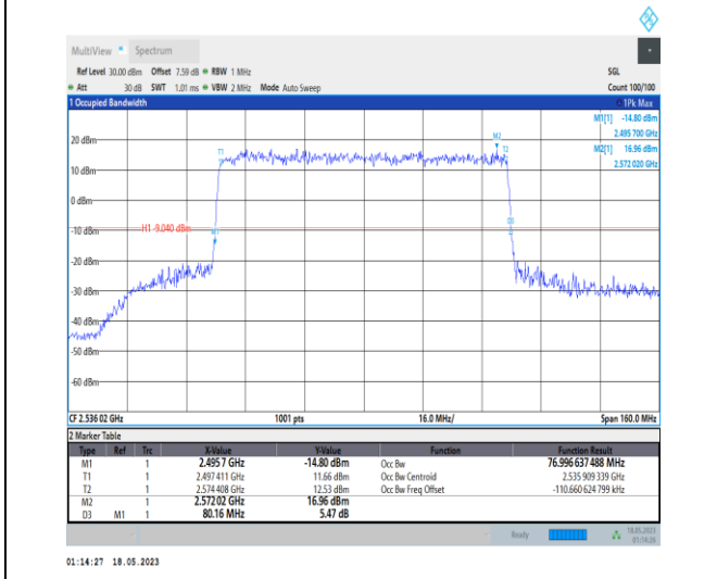
1-N41-PC1-30-80-L-1-DFT-QPSK-Outer_Full-216@0 -Ant0-76.997-80.160-<=80-PASS
