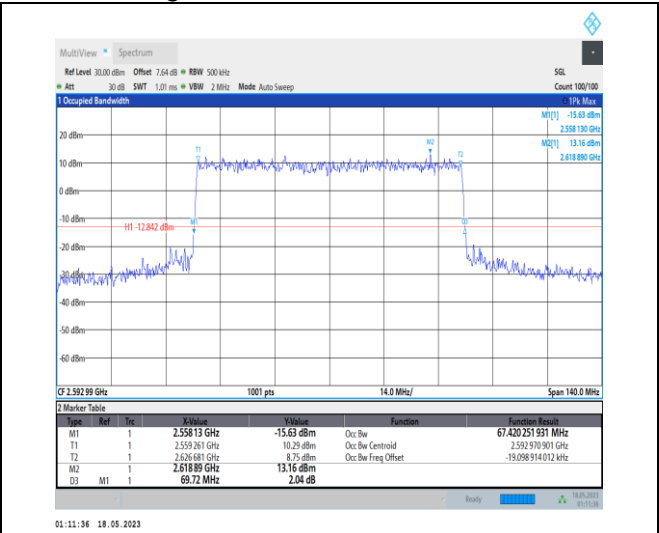
1-N41-PC1-30-70-M-6-CP-QPSK-Outer_Full-189@ 0-Ant0-67.42-69.720-<=70-PASS
