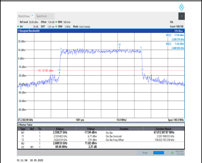
1-N41-PC1-30-70-M-8-CP-64QAM-Outer_Full-189@ 0-Ant0-67.012-69.440-<=70-PASS
