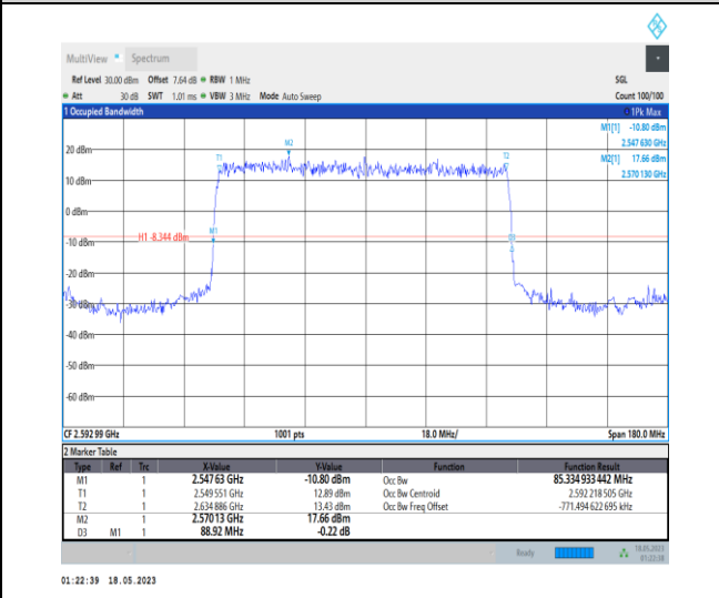
1-N41-PC1-30-90-M-2-DFT-PI2BPSK-Outer_Full-24 0@0-Ant0-85.335-88.920-≤90-PASS
