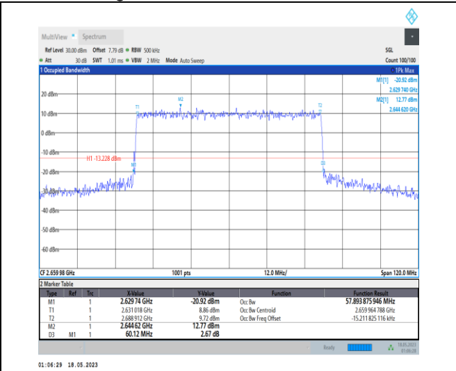
1-N41-PC1-30-60-H-8-CP-64QAM-Outer_Full-162@ 0-Ant0-57.894-60.120-≤60-PASS
