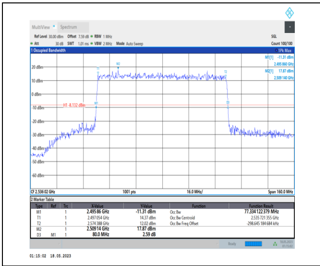
1-N41-PC1-30-80-L-3-DFT-16QAM-Outer_Full-216 @ 0-Ant0-77.334-80.000-≤80-PASS
