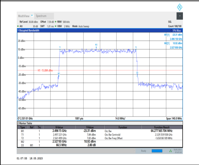
1-N41-PC1-30-70-L-5-DFT-256QAM-Outer_Full-180 @ 0-Ant0-64.278-66.500-≤70-PASS
