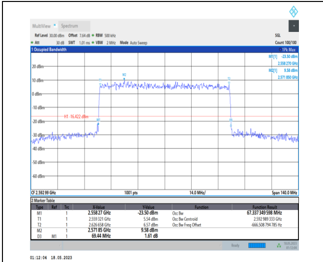
1-N41-PC1-30-70-M-9-CP-256QAM-Outer_Full-189 @ 0-Ant0-67.337-69.440-≤70-PASS
