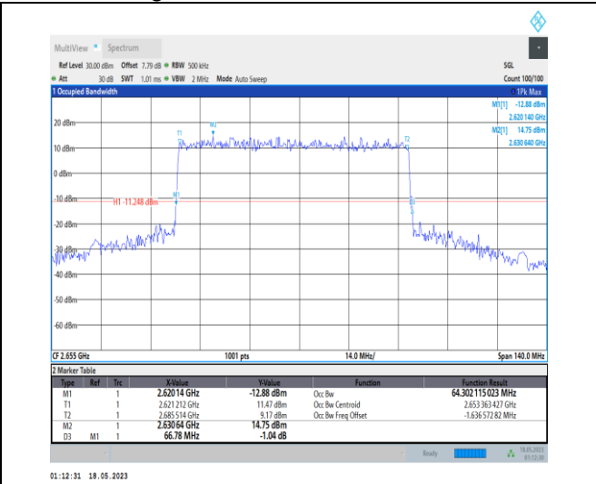
1-N41-PC1-30-70-H-1-DFT-QPSK-Outer_Full-180 @ 0-Ant0-64.302-66.780-≤70-PASS
