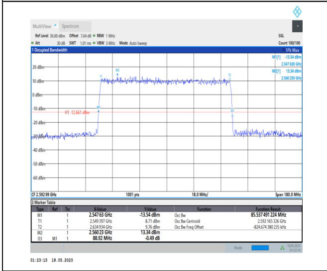
1-N41-PC1-30-90-M-5-DFT-256QAM-Outer_Full-240 @ 0-Ant0-85.537-88.920-≤90-PASS
