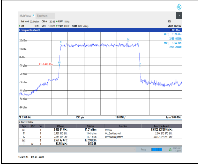
1-N41-PC1-30-90-L-2-DFT-PI2BPSK-Outer_Full-240 @ 0-Ant0-85.803-88.920-≤90-PASS
