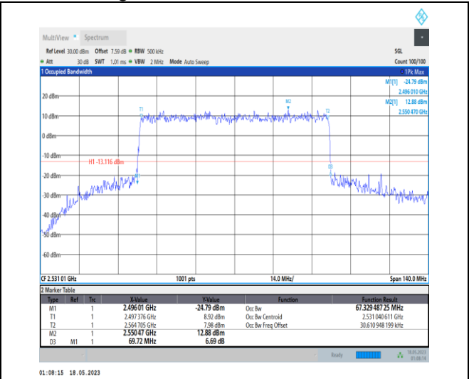
1-N41-PC1-30-70-L-7-CP-16QAM-Outer_Full-189@0-Ant0-67.329-69.720-≤70-PASS
