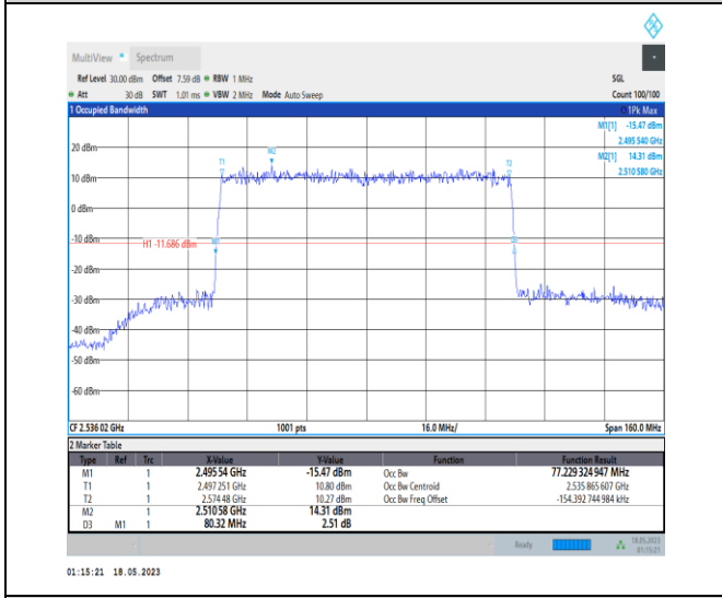
1-N41-PC1-30-80-L-5-DFT-256QAM-Outer_Full-216 @ 0-Ant0-77.229-80.320-≤80-PASS
