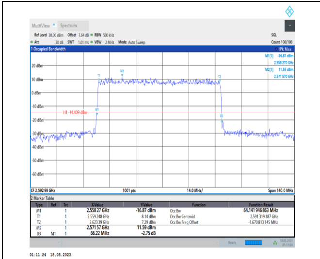
1-N41-PC1-30-70-M-5-DFT-256QAM-Outer_Full-180 @ 0-Ant0-64.142-66.220-<=70-PASS
