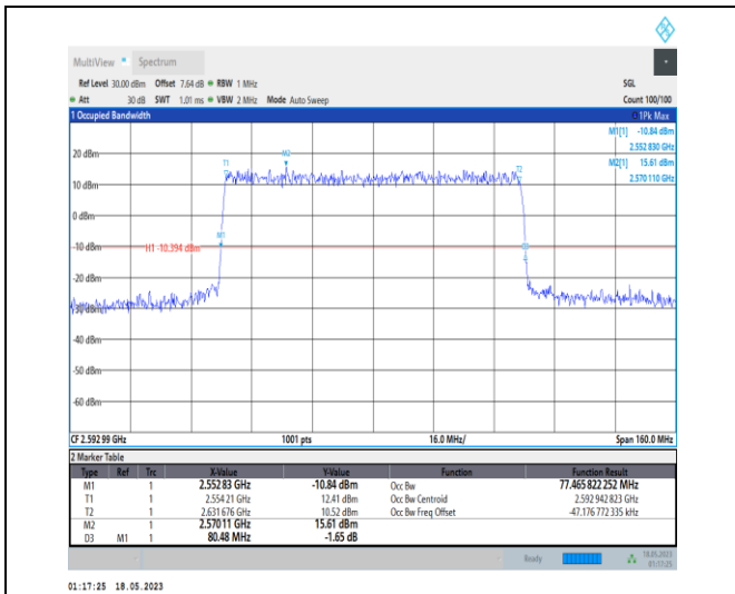
1-N41-PC1-30-80-M-6-CP-QPSK-Outer_Full-217@0 -Ant0-77.466-80.480-≤80-PASS
