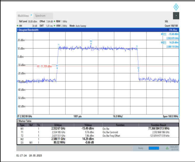
1-N41-PC1-30-80-M-5-DFT-256QAM-Outer_Full-216 @0-Ant0-77.367-80.320-≤80-PASS
