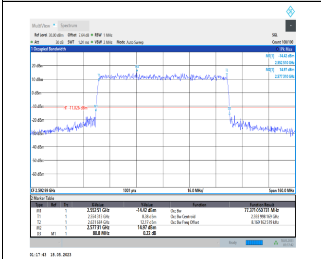
1-N41-PC1-30-80-M-8-CP-64QAM-Outer_Full-217@0 -Ant0-77.371-80.800-≤80-PASS
