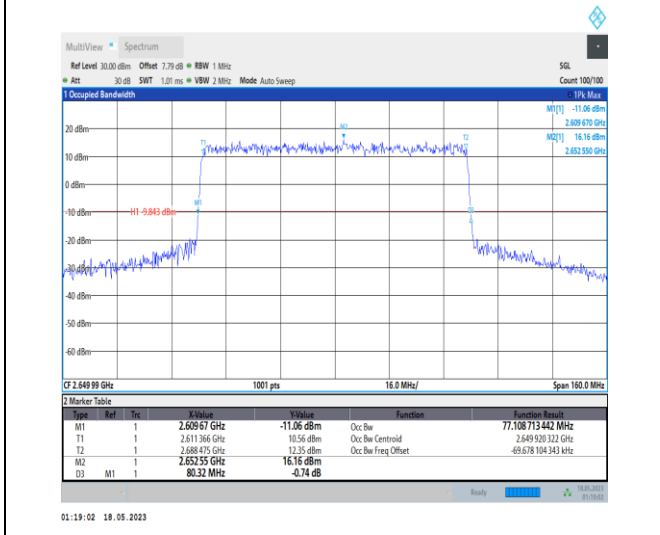
1-N41-PC1-30-80-H-3-DFT-16QAM-Outer_Full-216@0-Ant0-77.109-80.320-≤80-PASS
