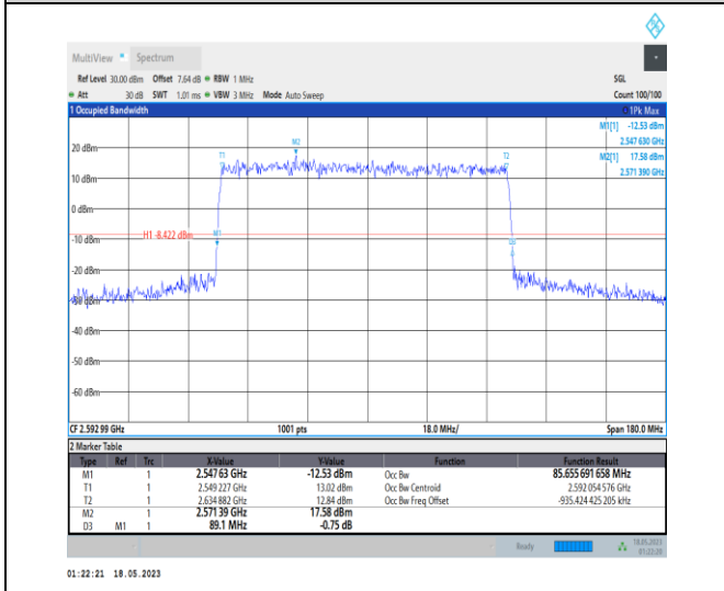
1-N41-PC1-30-90-M-1-DFT-QPSK-Outer_Full-240@ 0-Ant0-85.656-89.100-≤90-PASS
