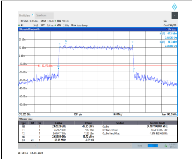
1-N41-PC1-30-70-H-4-DFT-64QAM-Outer_Full-180 @ 0-Ant0-64.187-66.360-≤70-PASS
