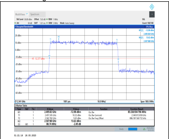
1-N41-PC1-30-90-L-5-DFT-256QAM-Outer_Full-240 @ 0-Ant0-85.537-88.740-≤90-PASS
