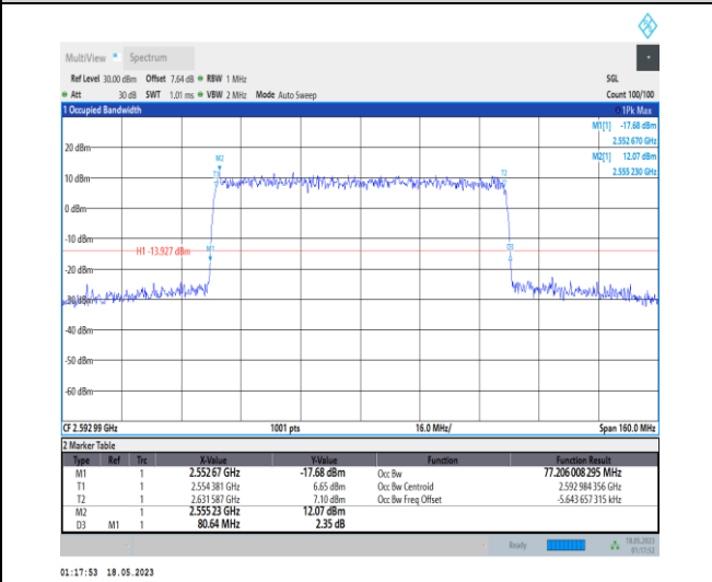
1-N41-PC1-30-80-M-9-CP-256QAM-Outer_Full-217@0 -Ant0-77.206-80.640-≤80-PASS
