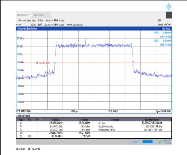
1-N41-PC1-30-90-M-6-CP-QPSK-Outer_Full-245 @ 0-Ant0-87.255-90.720-≤90-PASS
