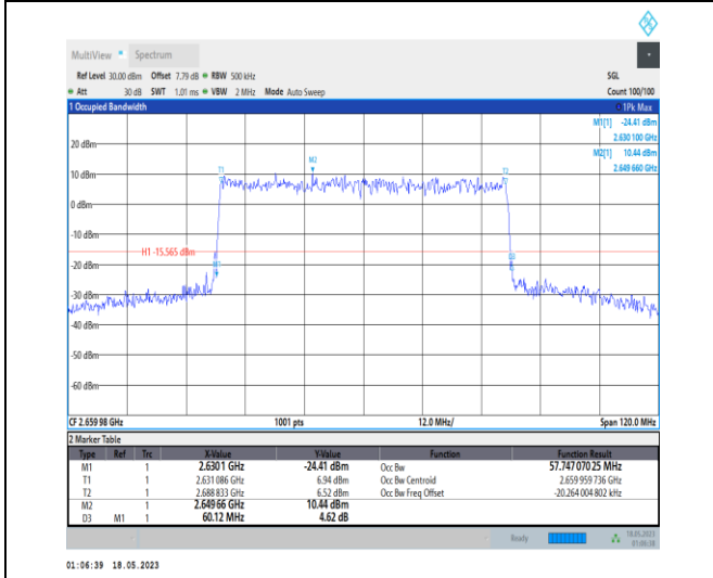
1-N41-PC1-30-60-H-9-CP-256QAM-Outer_Full-162 @0-Ant0-57.747-60.120-≤60-PASS
