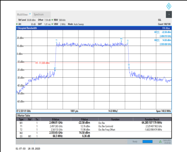
1-N41-PC1-30-70-L-1-DFT-QPSK-Outer_Full-180@ 0-Ant0-64.285-66.500-≤70-PASS
