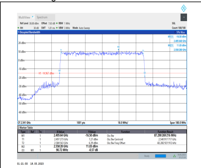
1-N41-PC1-30-90-L-9-CP-256QAM-Outer_Full-245 @0-Ant0-87.29-90.720-≤90-PASS
