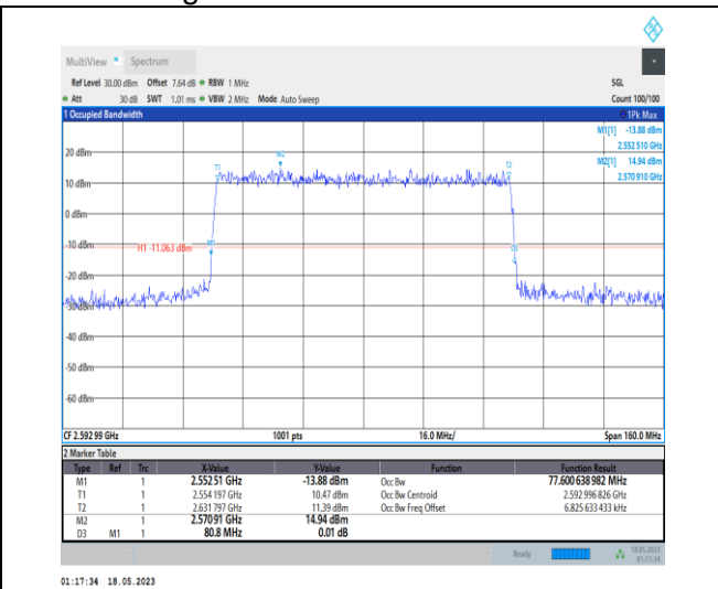
1-N41-PC1-30-80-M-7-CP-16QAM-Outer_Full-217@0 -Ant0-77.601-80.800-≤80-PASS
