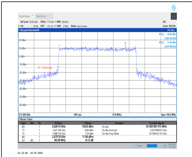
1-N41-PC1-30-70-H-8-CP-64QAM-Outer_Full-189@ 0-Ant0-67.492-69.580-<=70-PASS
