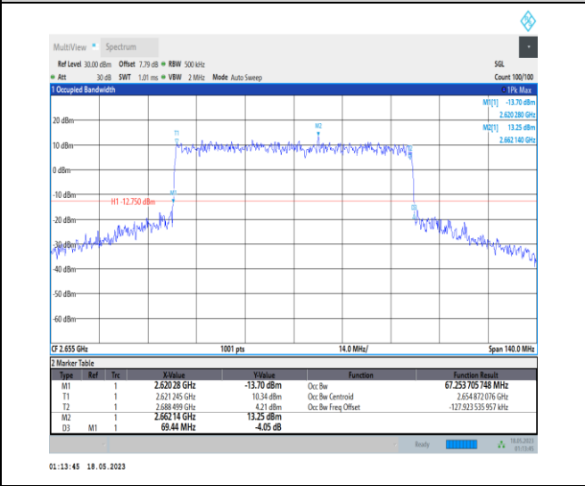
1-N41-PC1-30-70-H-7-CP-16QAM-Outer_Full-189@ 0-Ant0-67.254-69.440-≤70-PASS
