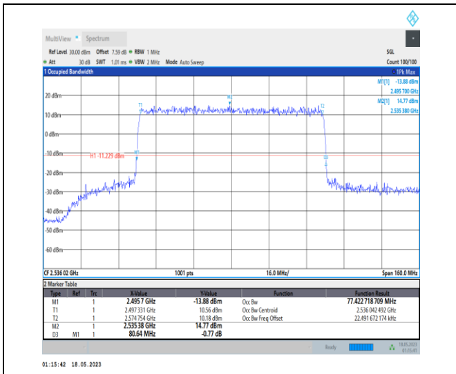
1-N41-PC1-30-80-L-7-CP-16QAM-Outer_Full-217@ 0-Ant0-77.423-80.640-≤80-PASS
