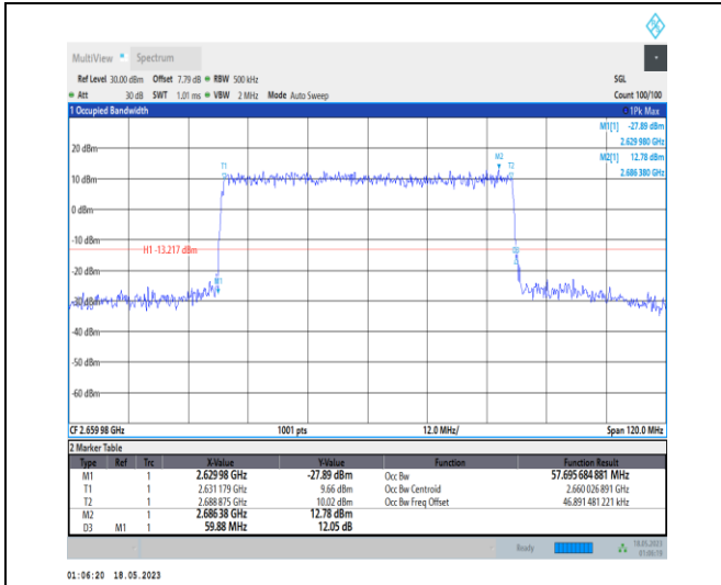
1-N41-PC1-30-60-H-7-CP-16QAM-Outer_Full-162@ 0-Ant0-57.696-59.880-≤60-PASS
