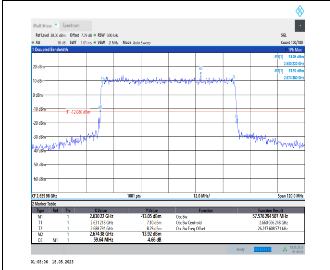
1-N41-PC1-30-60-H-1-DFT-QPSK-Outer_Full-162@ 0-Ant0-57.576-59.640-≤60-PASS
