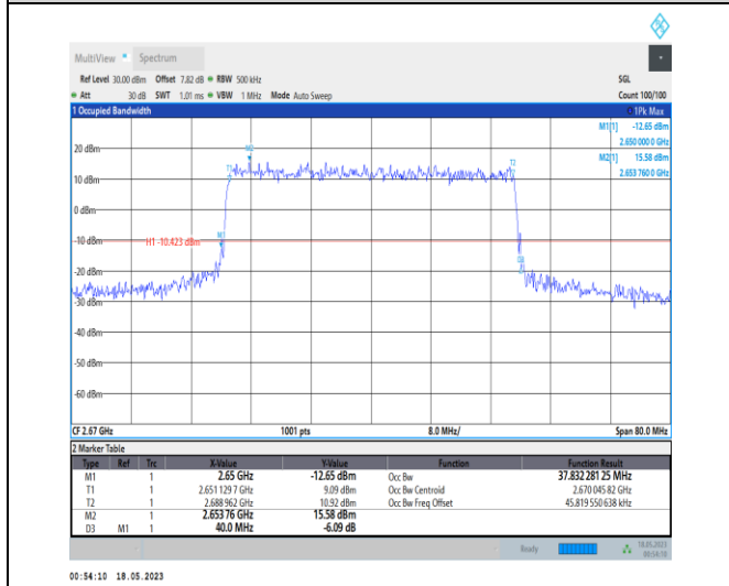
1-N41-PC1-30-40-H-7-CP-16QAM-Outer_Full-106 @ 0-Ant0-37.832-40.000-≤40-PASS
