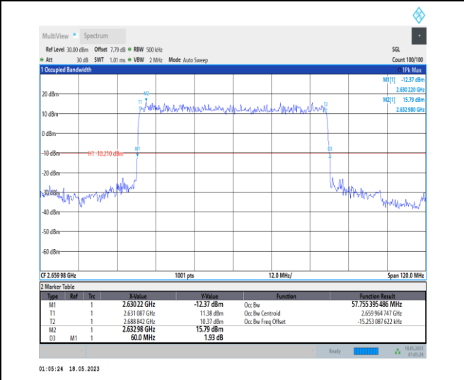
1-N41-PC1-30-60-H-2-DFT-PI2BPSK-Outer_Full-16 2@0-Ant0-57.755-60.000-≤60-PASS
