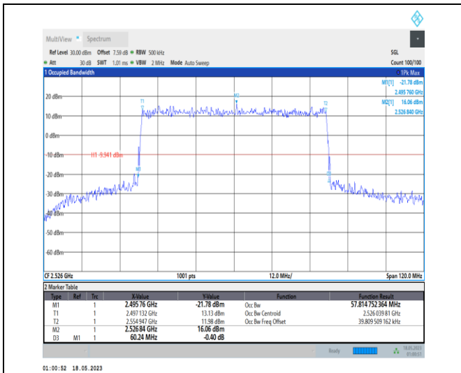
1-N41-PC1-30-60-L-1-DFT-QPSK-Outer_Full-162@0 -Ant0-57.815-60.240-≤60-PASS
