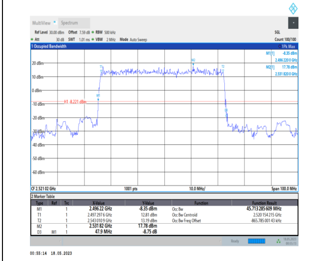
1-N41-PC1-30-50-L-2-DFT-PI2BPSK-Outer_Full-128 @ 0-Ant0-45.713-47.900-≤50-PASS
