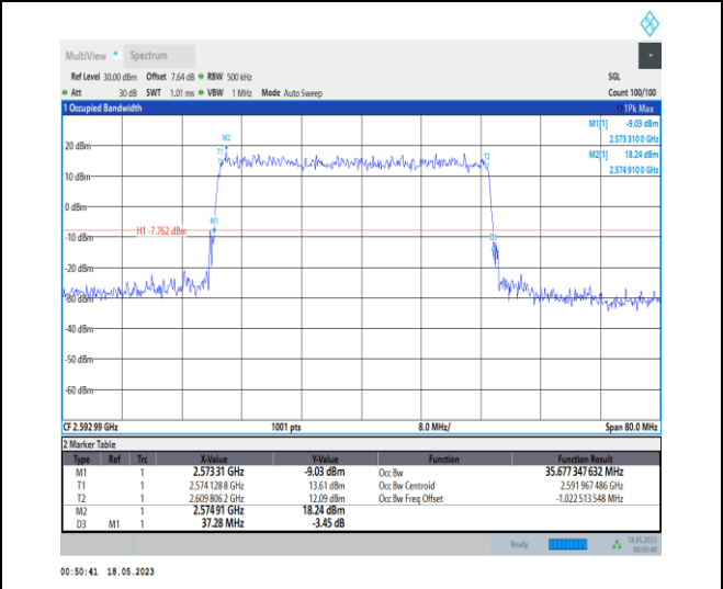
1-N41-PC1-30-40-M-1-DFT-QPSK-Outer_Full-100@ 0-Ant0-35.677-37.280-≤40-PASS
