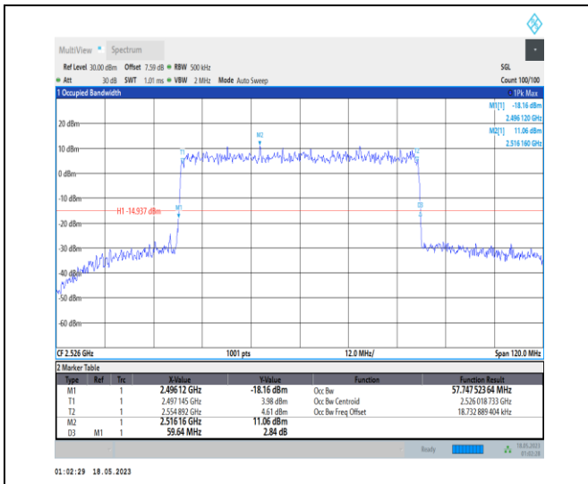
1-N41-PC1-30-60-L-9-CP-256QAM-Outer_Full-162 @ 0-Ant0-57.748-59.640-≤60-PASS
