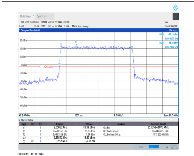
1-N41-PC1-30-40-H-5-DFT-256QAM-Outer_Full-100 @ 0-Ant0-35.736-37.520-≤40-PASS
