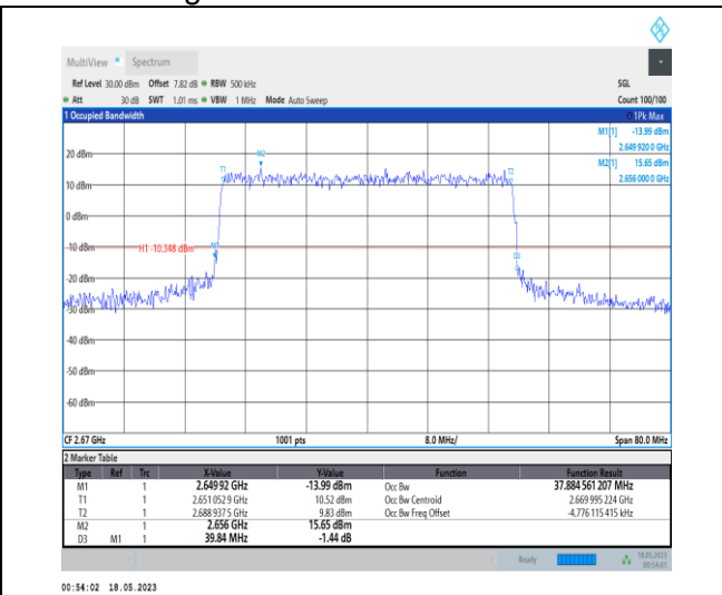
1-N41-PC1-30-40-H-6-CP-QPSK-Outer_Full-106 @ 0-Ant0-37.885-39.840-≤40-PASS
