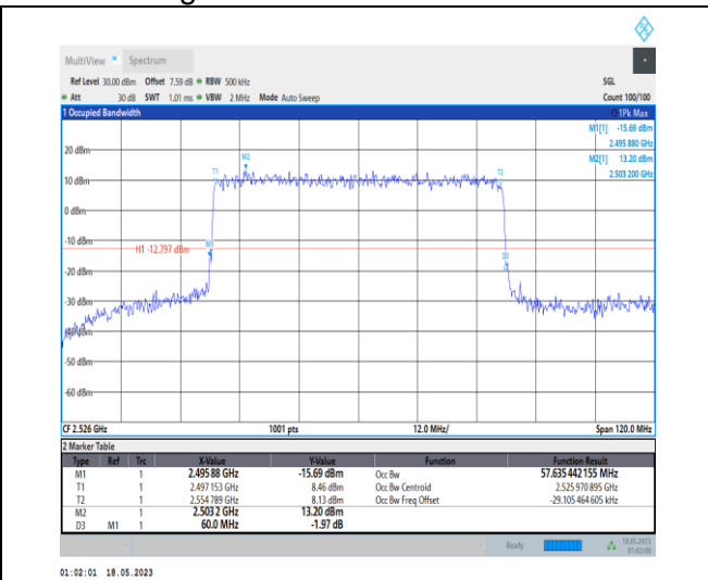
1-N41-PC1-30-60-L-6-CP-QPSK-Outer_Full-162 @ 0-Ant0-57.635-60.000-≤60-PASS
