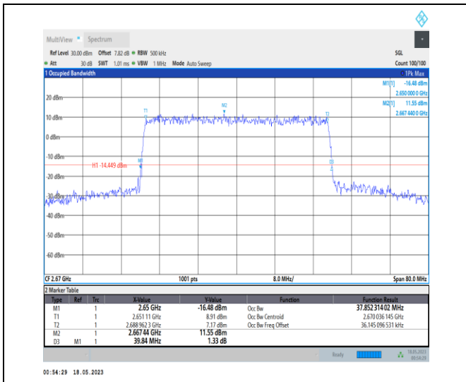
1-N41-PC1-30-40-H-9-CP-256QAM-Outer_Full-106 @ 0-Ant0-37.852-39.840-≤40-PASS
