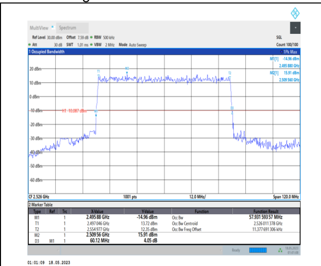
1-N41-PC1-30-60-L-2-DFT-PI2BPSK-Outer_Full-162 @0-Ant0-57.932-60.120-≤60-PASS
