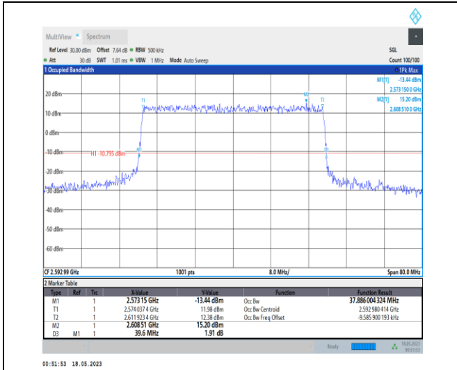
1-N41-PC1-30-40-M-6-CP-QPSK-Outer_Full-106@0 -Ant0-37.886-39.600-≤40-PASS
