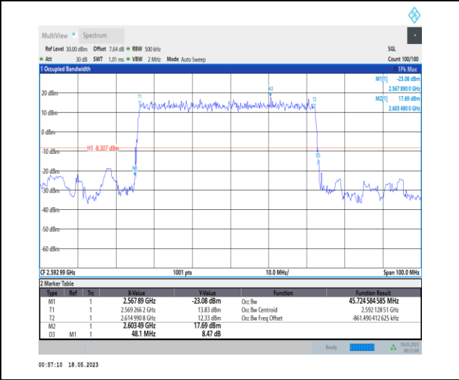
1-N41-PC1-30-50-M-2-DFT-PI2BPSK-Outer_Full-12 8@0-Ant0-45.725-48.100-≤50-PASS
