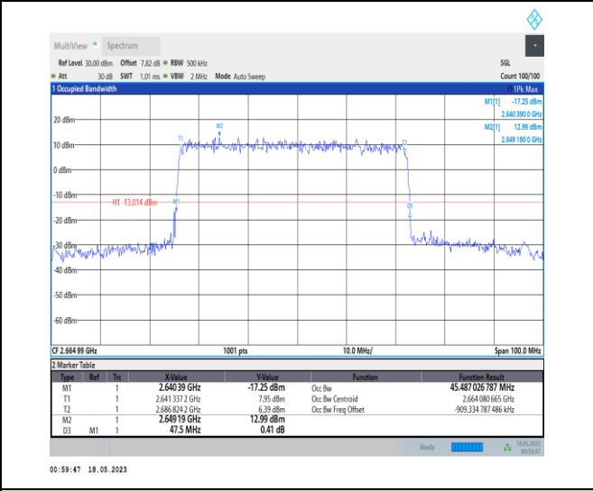
1-N41-PC1-30-50-H-5-DFT-256QAM-Outer_Full-128 @0-Ant0-45.487-47.500-≤50-PASS
