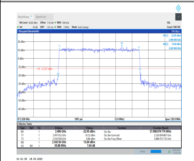
1-N41-PC1-30-60-L-4-DFT-64QAM-Outer_Full-162 @0-Ant0-57.906-59.880-≤60-PASS
