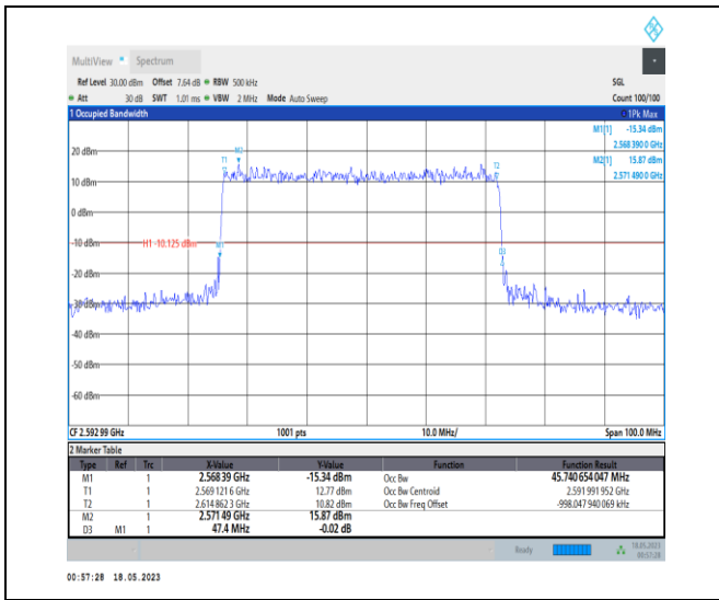
1-N41-PC1-30-50-M-3-DFT-16QAM-Outer_Full-128 @ 0-Ant0-45.741-47.400-≤50-PASS
