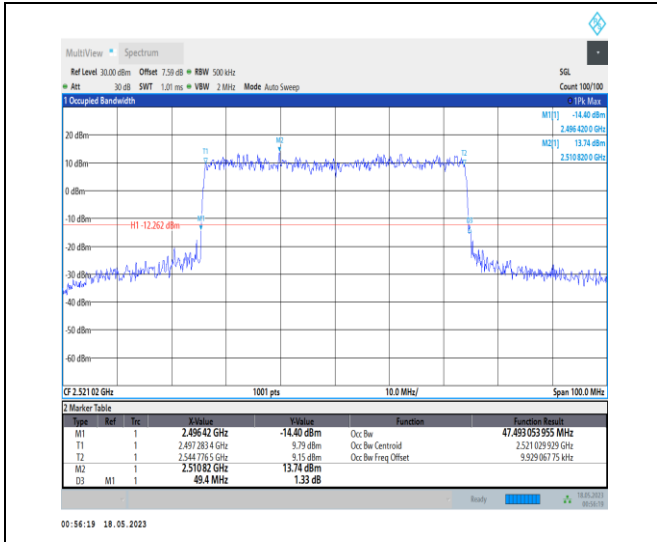
1-N41-PC1-30-50-L-8-CP-64QAM-Outer_Full-133@ 0-Ant0-47.493-49.400-≤50-PASS
