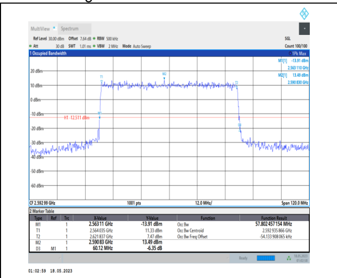
1-N41-PC1-30-60-M-1-DFT-QPSK-Outer_Full-162 @ 0-Ant0-57.802-60.120-≤60-PASS
