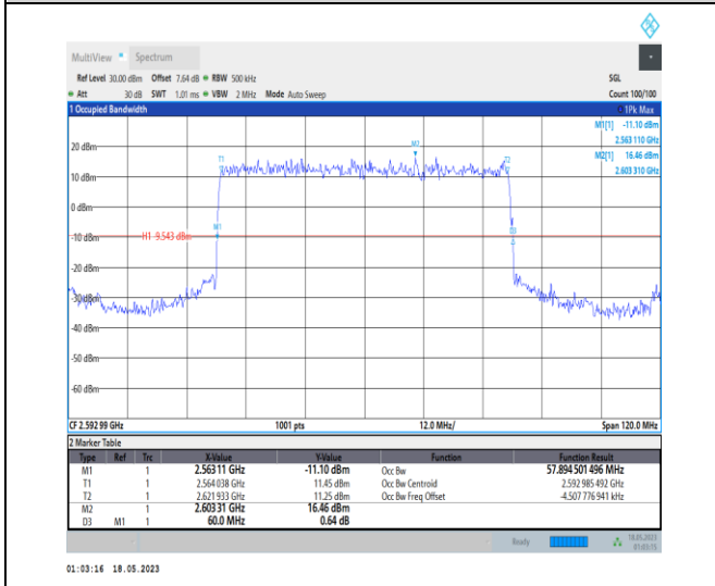
1-N41-PC1-30-60-M-2-DFT-PI2BPSK-Outer_Full-162 @ 0-Ant0-57.895-60.000-≤60-PASS
