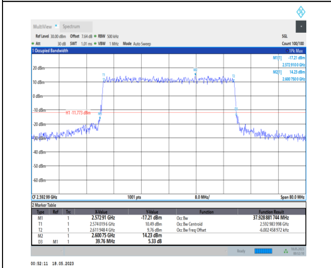
1-N41-PC1-30-40-M-8-CP-64QAM-Outer_Full-106@0 0-Ant0-37.929-39.760-≤40-PASS
