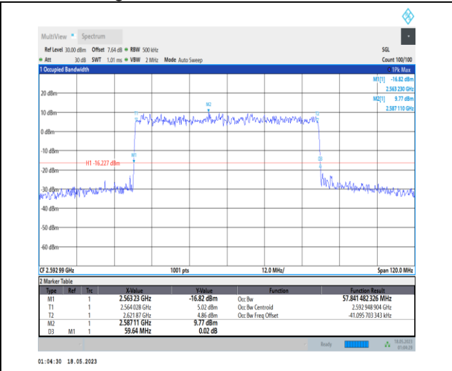
1-N41-PC1-30-60-M-9-CP-256QAM-Outer_Full-162 @0-Ant0-57.841-59.640-≤60-PASS
