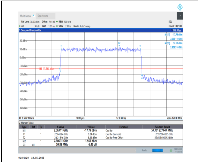
1-N41-PC1-30-60-M-8-CP-64QAM-Outer_Full-162@ 0-Ant0-57.761-59.880-≤60-PASS
