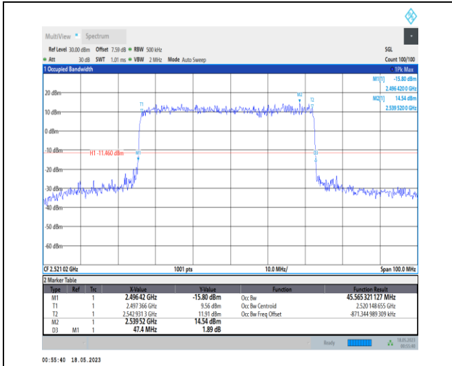
1-N41-PC1-30-50-L-4-DFT-64QAM-Outer_Full-128 @ 0-Ant0-45.565-47.400-≤50-PASS
