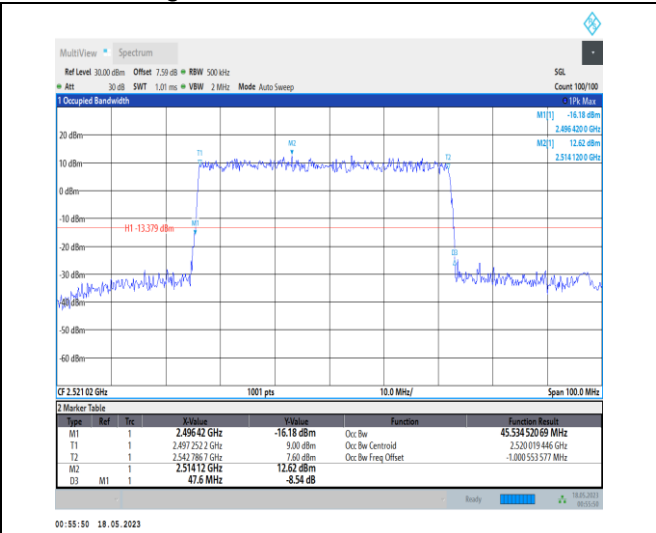
1-N41-PC1-30-50-L-5-DFT-256QAM-Outer_Full-128 @ 0-Ant0-45.535-47.600-≤50-PASS
