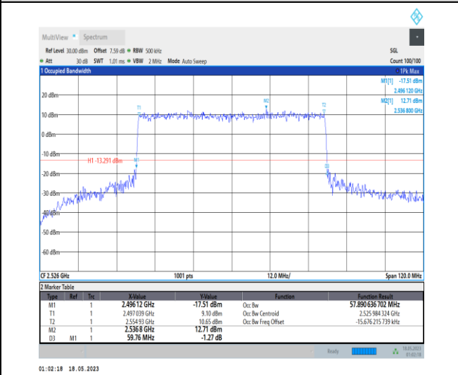
1-N41-PC1-30-60-L-8-CP-64QAM-Outer_Full-162 @ 0-Ant0-57.891-59.760-≤60-PASS
