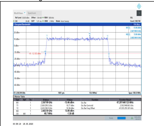
1-N41-PC1-30-50-M-8-CP-64QAM-Outer_Full-133@ 0-Ant0-47.298-49.700-≤50-PASS
