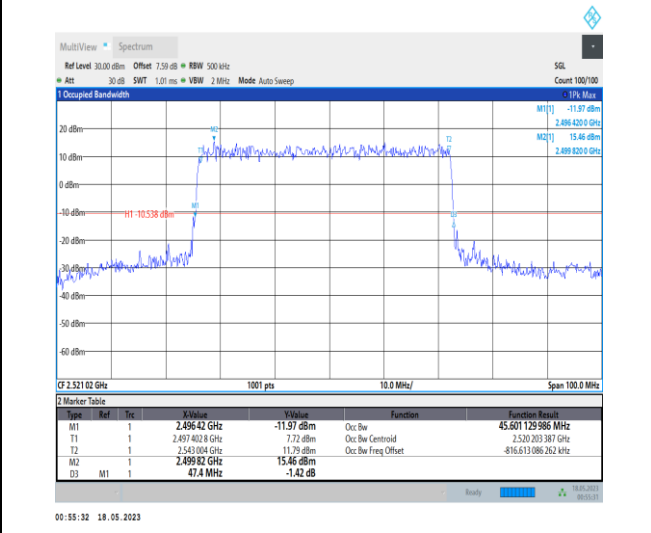
1-N41-PC1-30-50-L-3-DFT-16QAM-Outer_Full-128 @ 0-Ant0-45.601-47.400-≤50-PASS
