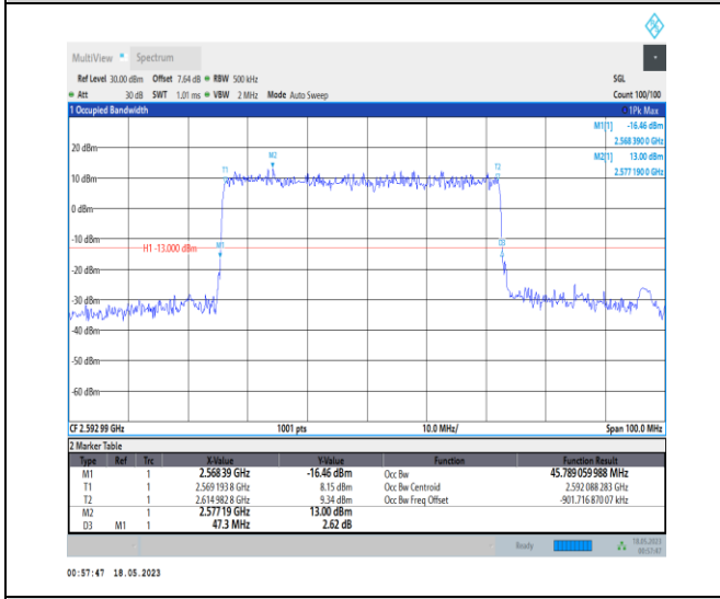
1-N41-PC1-30-50-M-5-DFT-256QAM-Outer_Full-128 @ 0-Ant0-45.789-47.300-≤50-PASS
