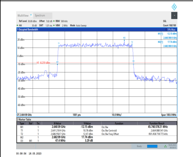
1-N41-PC1-30-50-H-1-DFT-QPSK-Outer_Full-128@ 0-Ant0-45.74-47.400-≤50-PASS
