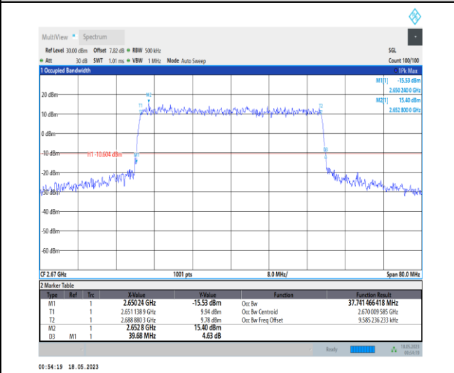
1-N41-PC1-30-40-H-8-CP-64QAM-Outer_Full-106 @ 0-Ant0-37.741-39.680-≤40-PASS
