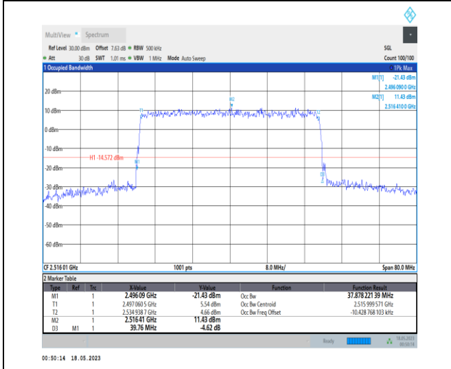
1-N41-PC1-30-40-L-9-CP-256QAM-Outer_Full-106 @0-Ant0-37.878-39.760-≤40-PASS
