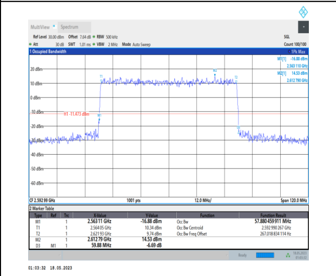
1-N41-PC1-30-60-M-3-DFT-16QAM-Outer_Full-162 @ 0-Ant0-57.88-59.880-≤60-PASS
