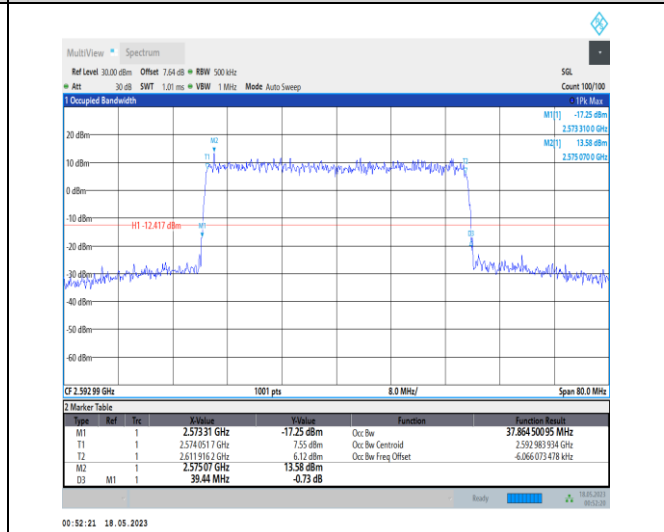
1-N41-PC1-30-40-M-9-CP-256QAM-Outer_Full-106@0 @0-Ant0-37.865-39.440-≤40-PASS
