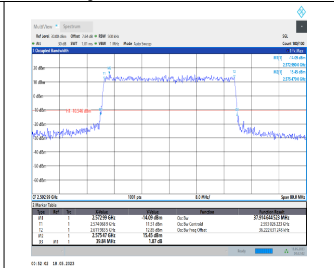
1-N41-PC1-30-40-M-7-CP-16QAM-Outer_Full-106@0 0-Ant0-37.915-39.840-≤40-PASS
