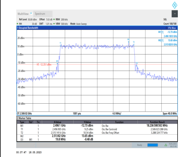
1-N41-PC1-30-20-L-8-CP-64QAM-Outer_Full-51 @0-Ant0-18.237-19.800-≤20-PASS
