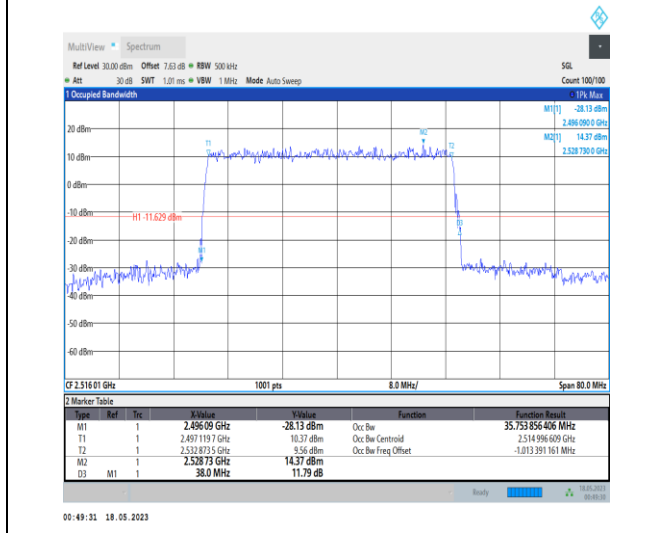
1-N41-PC1-30-40-L-5-DFT-256QAM-Outer_Full-100 @ 0-Ant0-35.754-38.000-≤40-PASS
