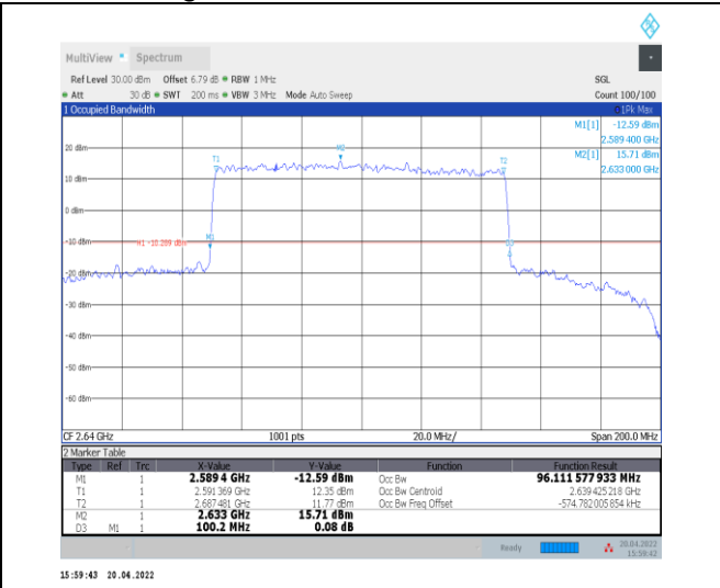
1-N41--30-100-H-4-DFT-64QAM-Outer_Full-270@0-Ant0-96.112-100.200-<=100-PASS
