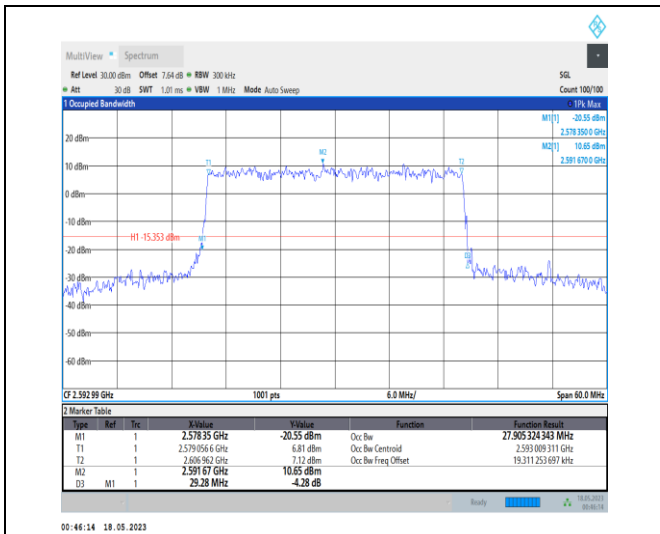
1-N41-PC1-30-30-M-9-CP-256QAM-Outer_Full-78@ 0-Ant0-27.905-29.280-≤30-PASS
