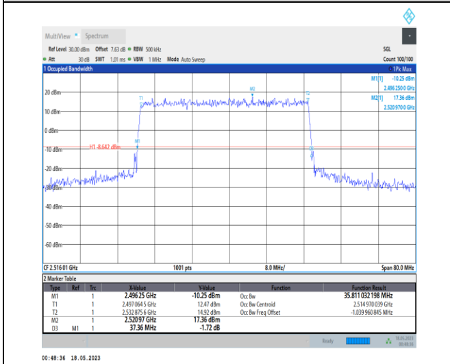
1-N41-PC1-30-40-L-1-DFT-QPSK-Outer_Full-100@0 -Ant0-35.811-37.360-<=40-PASS
