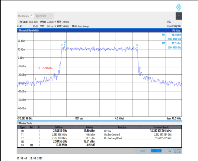
1-N41-PC1-30-20-M-7-CP-16QAM-Outer_Full-51@0- Ant0-18.283-19.360-≤20-PASS
