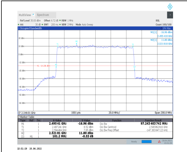
1-N41--30-100-L-9-CP-256QAM-Outer_Full-273@0-Ant0-97.243-101.200-<=100-PASS
