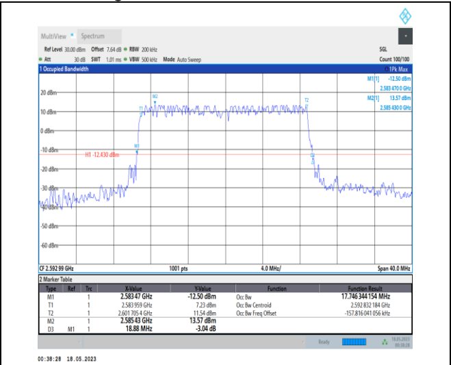
1-N41-PC1-30-20-M-1-DFT-QPSK-Outer_Full-50@0-Ant0-17.746-18.880-≤20-PASS
