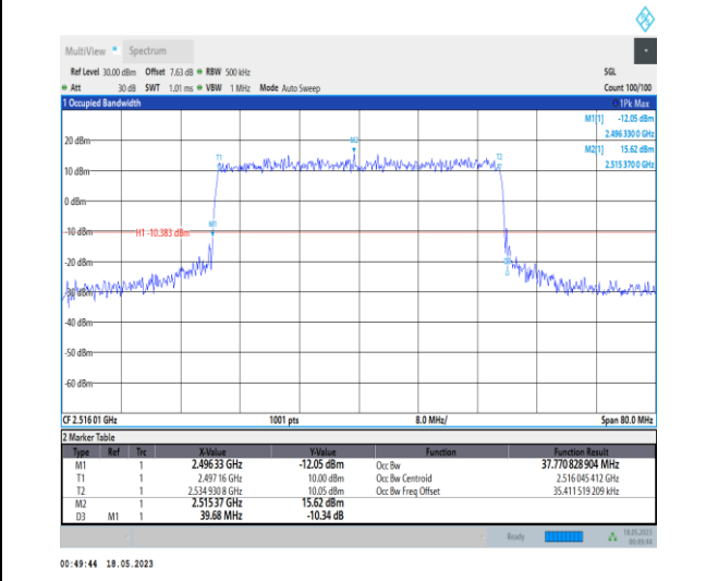
1-N41-PC1-30-40-L-6-CP-QPSK-Outer_Full-106 @ 0-Ant0-37.771-39.680-≤40-PASS
