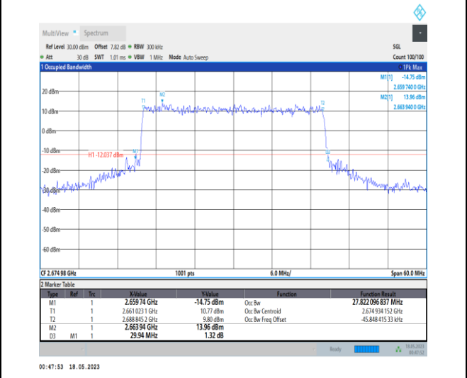
1-N41-PC1-30-30-H-7-CP-16QAM-Outer_Full-78@0 -Ant0-27.822-29.940-≤30-PASS
