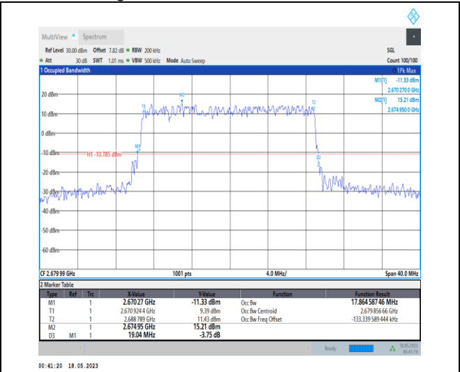
1-N41-PC1-30-20-H-4-DFT-64QAM-Outer_Full-50@ 0-Ant0-17.865-19.040-≤20-PASS
