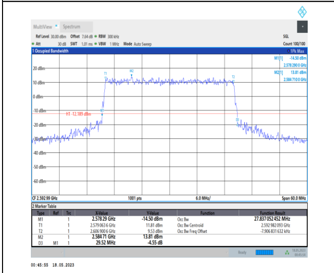
1-N41-PC1-30-30-M-7-CP-16QAM-Outer_Full-78 @ 0-Ant0-27.837-29.520-≤30-PASS
