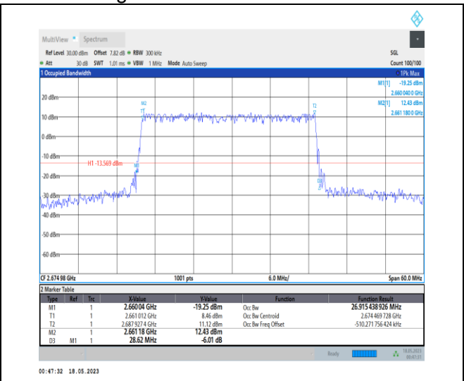
1-N41-PC1-30-30-H-5-DFT-256QAM-Outer_Full-75 @0-Ant0-26.915-28.620-≤30-PASS
