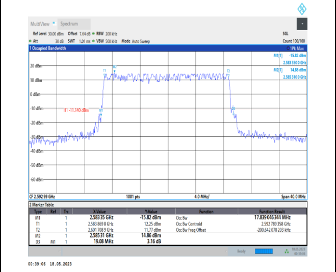
1-N41-PC1-30-20-M-3-DFT-16QAM-Outer_Full-50@0-Ant0-17.839-19.080-≤20-PASS
