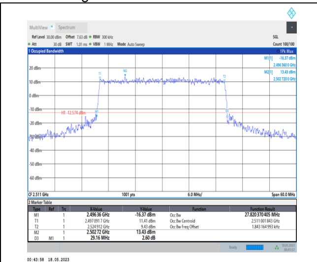
1-N41-PC1-30-30-L-7-CP-16QAM-Outer_Full-78@0-Ant0-27.82-29.160-≤30-PASS
