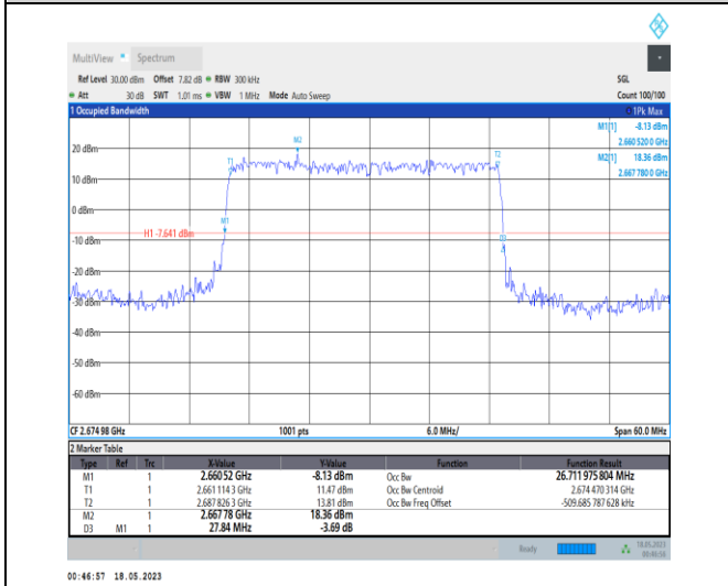
1-N41-PC1-30-30-H-2-DFT-PI2BPSK-Outer_Full-75@ 0-Ant0-26.712-27.840-≤30-PASS
