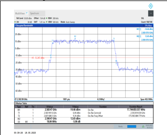
1-N41-PC1-30-20-M-5-DFT-256QAM-Outer_Full-50@ 0-Ant0-17.745-18.840-≤20-PASS
