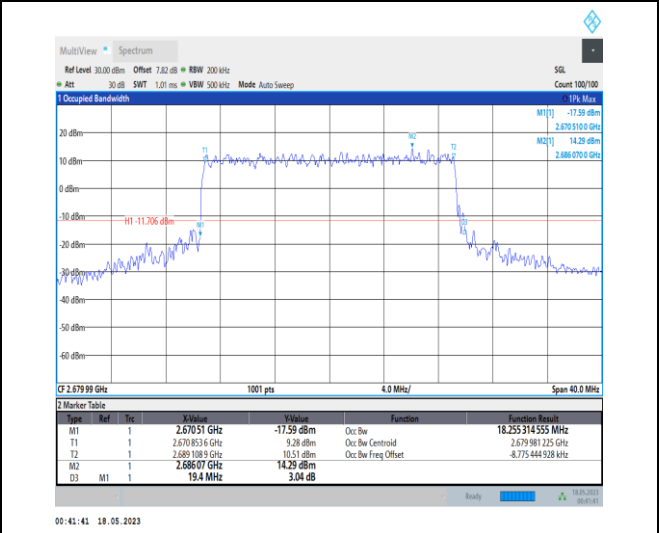
1-N41-PC1-30-20-H-6-CP-QPSK-Outer_Full-51@0- Ant0-18.255-19.400-≤20-PASS
