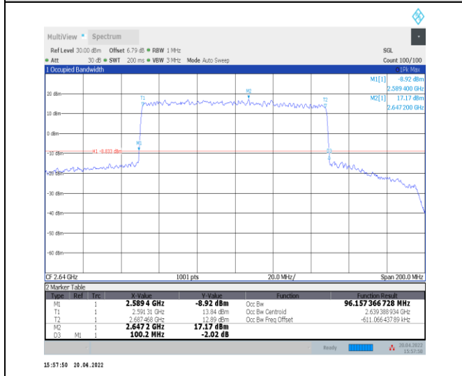
1-N41--30-100-H-1-DFT-QPSK-Outer_Full-270@0-A nt0-96.157-100.200-≤100-PASS
