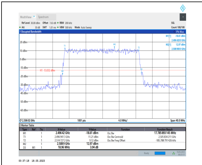
1-N41-PC1-30-20-L-5-DFT-256QAM-Outer_Full-50 @0-Ant0-17.786-18.960-≤20-PASS
