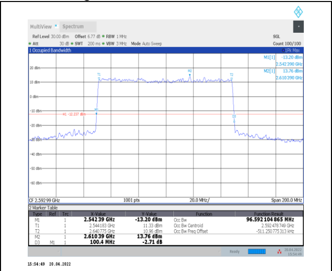
1-N41--30-100-M-5-DFT-256QAM-Outer_Full-270@0-Ant0-96.592-100.400-≤100-PASS
