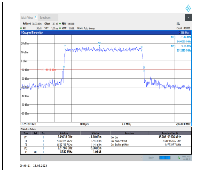
1-N41-PC1-30-40-L-3-DFT-16QAM-Outer_Full-100 @ 0-Ant0-35.708-37.520-≤40-PASS
