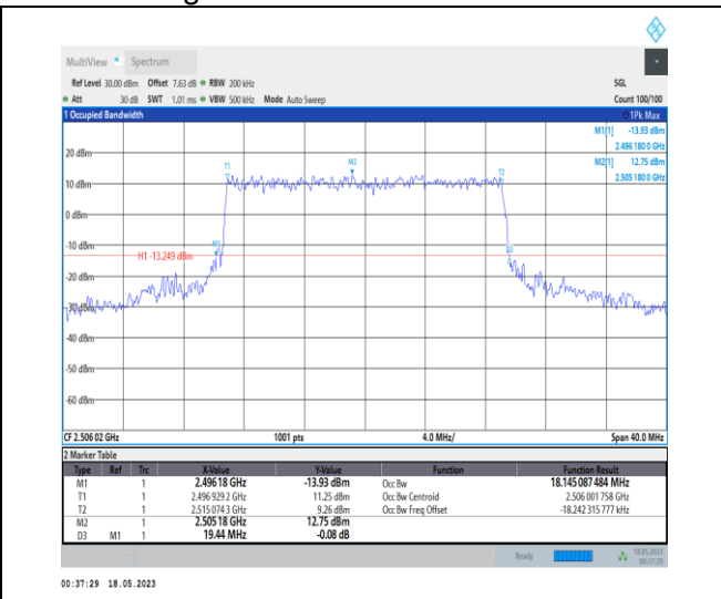
1-N41-PC1-30-20-L-6-CP-QPSK-Outer_Full-51 @0-Ant0-18.145-19.440-≤20-PASS
