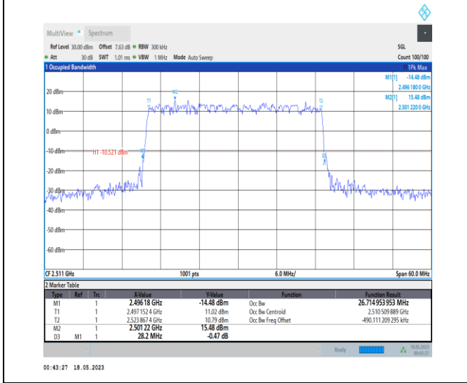
1-N41-PC1-30-30-L-4-DFT-64QAM-Outer_Full-75 @ 0-Ant0-26.715-28.200-≤30-PASS
