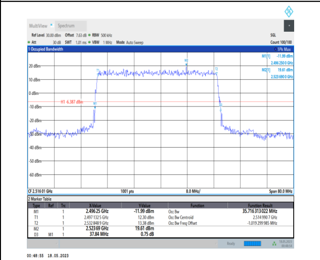
1-N41-PC1-30-40-L-2-DFT-PI2BPSK-Outer_Full-100@0 -Ant0-35.716-37.840-<=40-PASS
