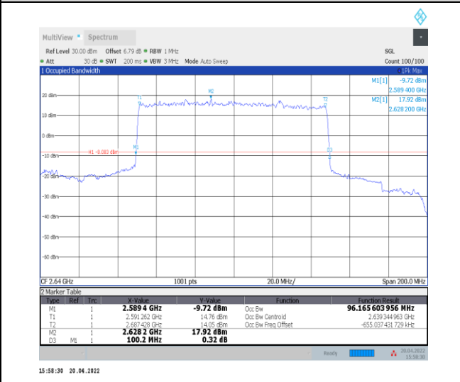
1-N41--30-100-H-2-DFT-Pl2BPSK-Outer_Full-270@ 0-Ant0-96.166-100.200-≤100-PASS
