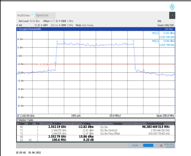
1-N41--30-100-M-3-DFT-16QAM-Outer_Full-270@0-Ant0-96.383-100.600-<=100-PASS
