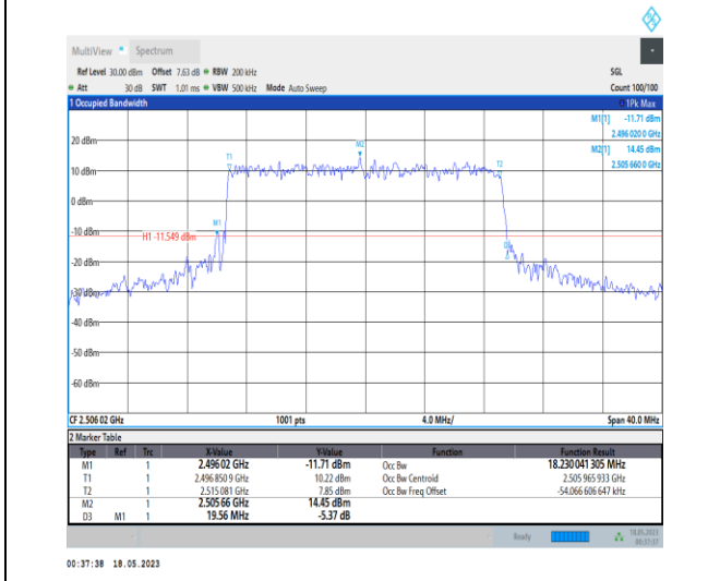
1-N41-PC1-30-20-L-7-CP-16QAM-Outer_Full-51 @0-Ant0-18.23-19.560-≤20-PASS
