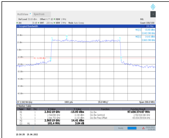
1-N41--30-100-M-8-CP-64QAM-Outer_Full-273@0-A nt0-97.656-101.400-≤100-PASS
