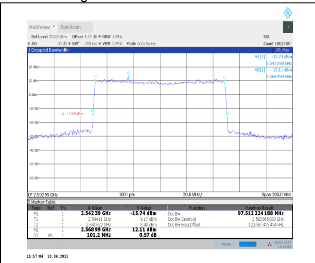
1-N41--30-100-M-9-CP-256QAM-Outer_Full-273@0- Ant0-97.512-101.200-≤100-PASS
