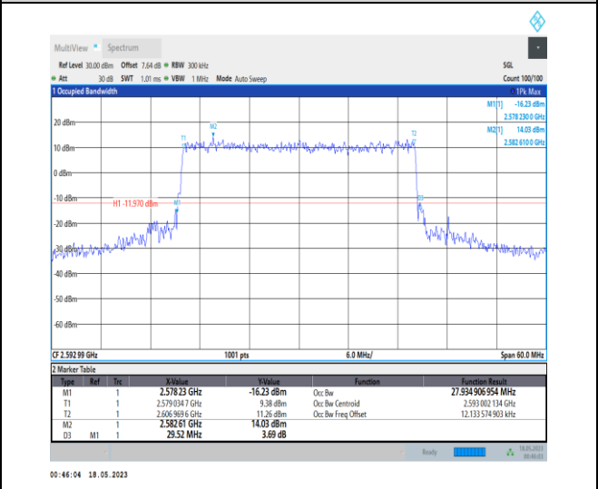
1-N41-PC1-30-30-M-8-CP-64QAM-Outer_Full-78 @ 0-Ant0-27.935-29.520-≤30-PASS
