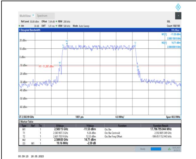
1-N41-PC1-30-20-M-4-DFT-64QAM-Outer_Full-50@ 0-Ant0-17.797-19.160-≤20-PASS
