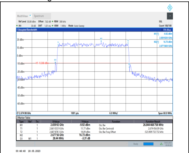
1-N41-PC1-30-30-H-1-DFT-QPSK-Outer_Full-75@0- Ant0-26.844-28.440-≤30-PASS
