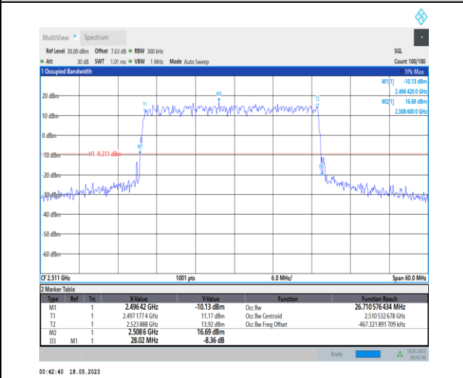
1-N41-PC1-30-30-L-1-DFT-QPSK-Outer_Full-75@0- Ant0-26.711-28.020-≤30-PASS
