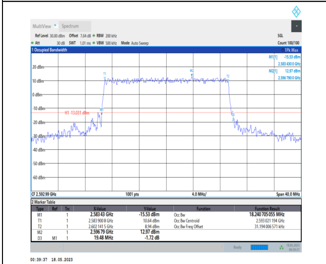
1-N41-PC1-30-20-M-6-CP-QPSK-Outer_Full-51@0- Ant0-18.241-19.480-≤20-PASS
