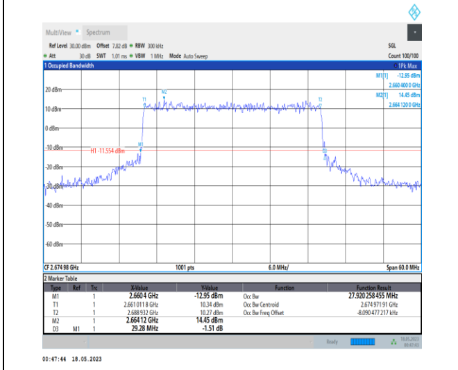
1-N41-PC1-30-30-H-6-CP-QPSK-Outer_Full-78@0- Ant0-27.92-29.280-≤30-PASS
