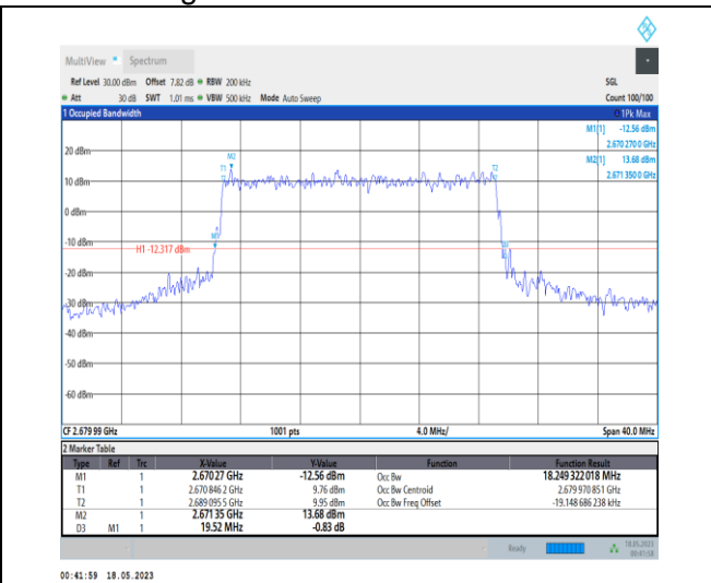
1-N41-PC1-30-20-H-8-CP-64QAM-Outer_Full-51@0 -Ant0-18.249-19.520-≤20-PASS
