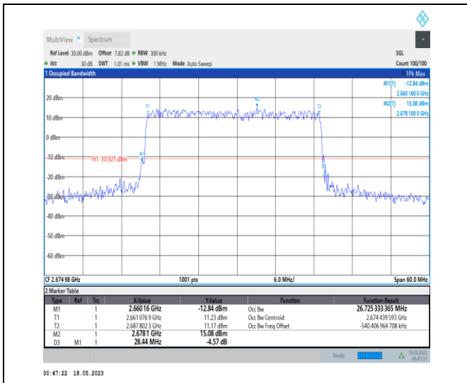
1-N41-PC1-30-30-H-4-DFT-64QAM-Outer_Full-75@ 0-Ant0-26.725-28.440-≤30-PASS
