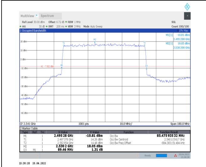
1-N41--30-90-L-2-DFT-PI2BPSK-Outer_Full-240@0-Ant 0-85.476-89.460-≤90-PASS
