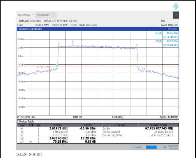
1-N41--30-70-H-7-CP-16QAM-Outer_Full-189@0-Ant t0-67.436-70.280-≤70-PASS
