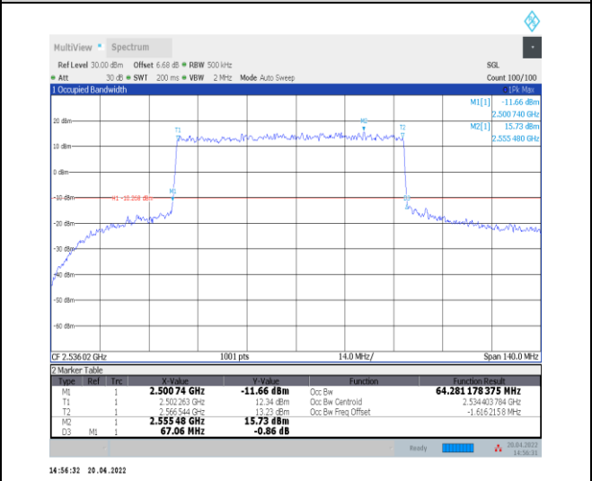
1-N41--30-70-L-1-DFT-QPSK-Outer_Full-180@0-Ant 0-64.281-67.060-≤70-PASS
