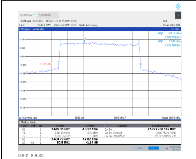
1-N41--30-80-H-3-DFT-16QAM-Outer_Full-216@0-A nt0-77.227-80.800-<math>\leq 80</math>-PASS
