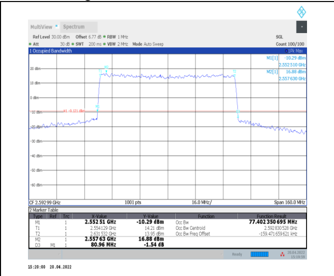
1-N41--30-80-M-3-DFT-16QAM-Outer_Full-216@0-Ant0-77.402-80.960-≤80-PASS
