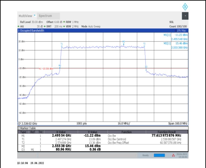
1-N41--30-80-L-6-CP-QPSK-Outer_Full-217@0-Ant 0-77.614-80.960-<80-PASS
