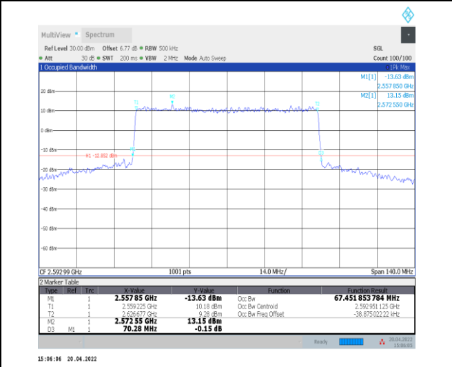
1-N41--30-70-M-8-CP-64QAM-Outer_Full-189@0-Ant0-67.452-70.280-<=70-PASS
