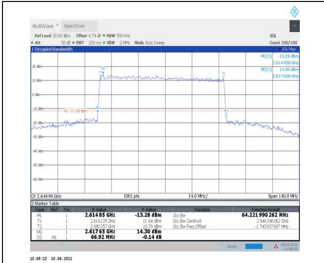
1-N41--30-70-H-4-DFT-64QAM-Outer_Full-180@0-A nt0-64.222-66.920-≤70-PASS
