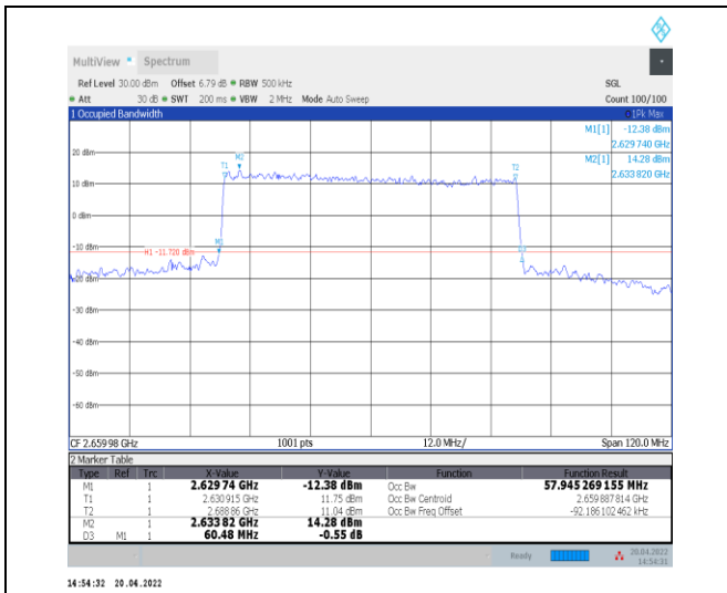
1-N41--30-60-H-7-CP-16QAM-Outer_Full-162@0-An t0-57.945-60.480-≤60-PASS
