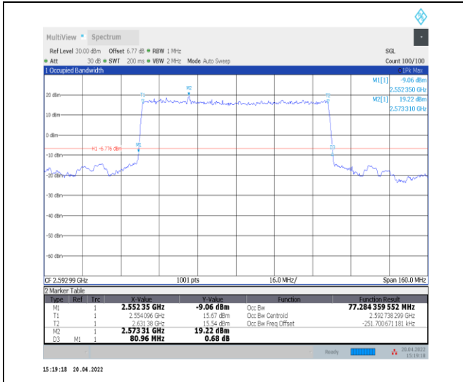
1-N41--30-80-M-2-DFT-PI2BPSK-Outer_Full-216@0-Ant0-77.284-80.960-≤80-PASS
