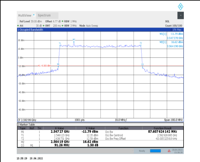
1-N41--30-90-M-6-CP-QPSK-Outer_Full-245@0-Ant 0-87.608-91.260-≤90-PASS
