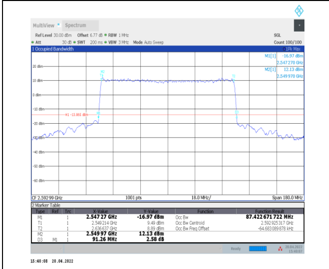
1-N41--30-90-M-9-CP-256QAM-Outer_Full-245@0-A nt0-87.423-91.260-<=90-PASS
