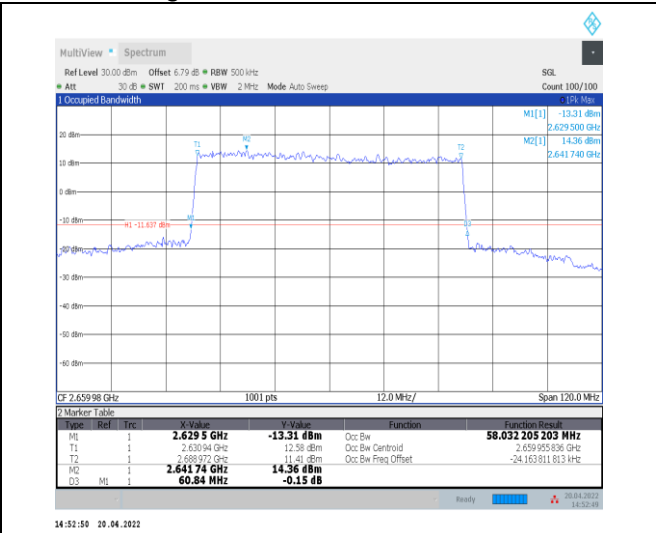
1-N41--30-60-H-4-DFT-64QAM-Outer_Full-162@0-A nt0-58.032-60.840-<math>\leq 60</math>-PASS
