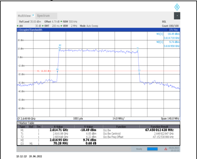
1-N41--30-70-H-9-CP-256QAM-Outer_Full-189@0-Ant0-67.45-70.280-≤70-PASS
