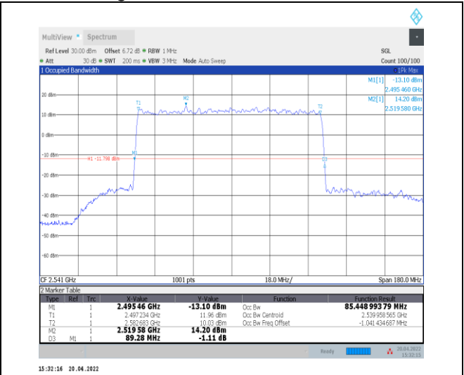
1-N41--30-90-L-5-DFT-256QAM-Outer_Full-240@0-A Ant0-85.449-89.280-≤90-PASS
