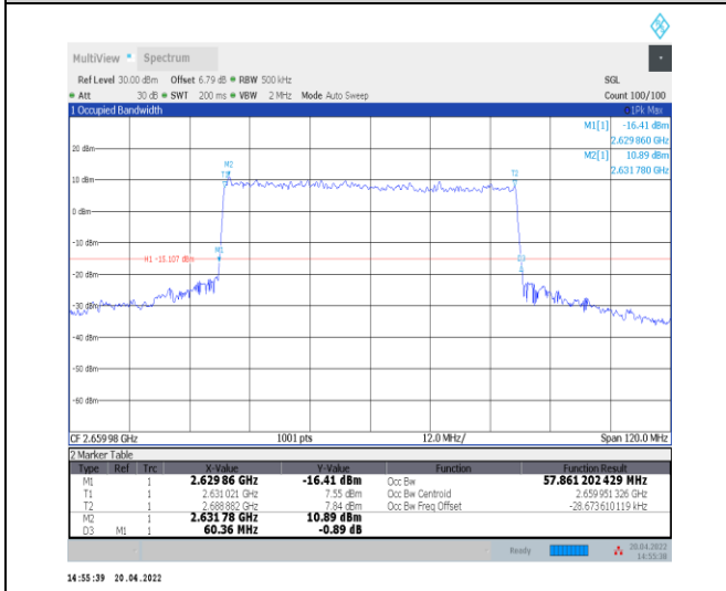
1-N41--30-60-H-9-CP-256QAM-Outer_Full-162@0-A nt0-57.861-60.360-≤60-PASS
