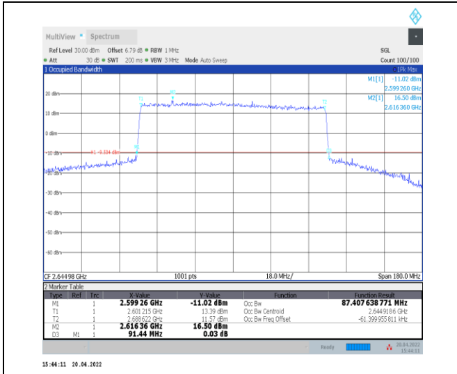
1-N41--30-90-H-6-CP-QPSK-Outer_Full-245@0-Ant 0-87.408-91.440-≤90-PASS
