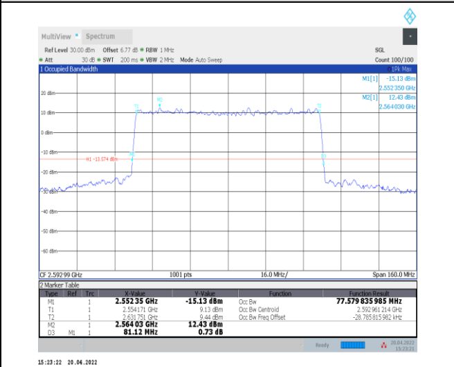
1-N41--30-80-M-9-CP-256QAM-Outer_Full-217@0-Ant Ant0-77.58-81.120-<80-PASS
