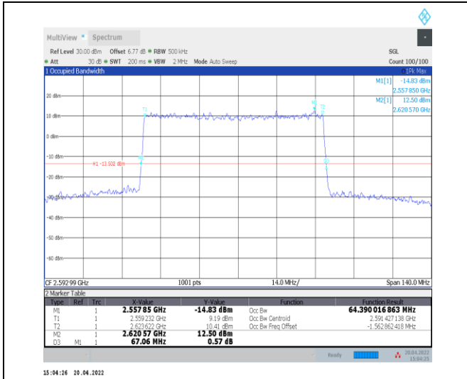
1-N41--30-70-M-5-DFT-256QAM-Outer_Full-180@0-Ant0-64.39-67.060-<=70-PASS
