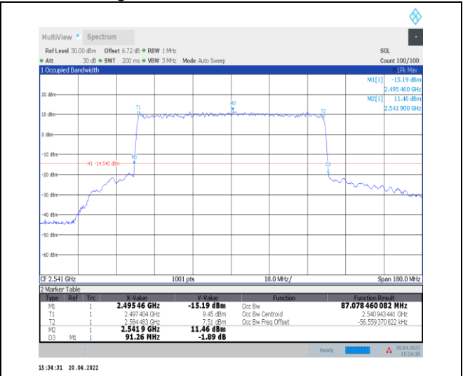
1-N41--30-90-L-9-CP-256QAM-Outer_Full-245@0-Ant 0-87.078-91.260-≤90-PASS
