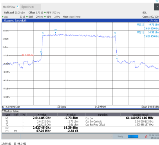
1-N41--30-70-H-2-DFT-PI2BPSK-Outer_Full-180@0-A Ant0-64.141-67.060-≤70-PASS
