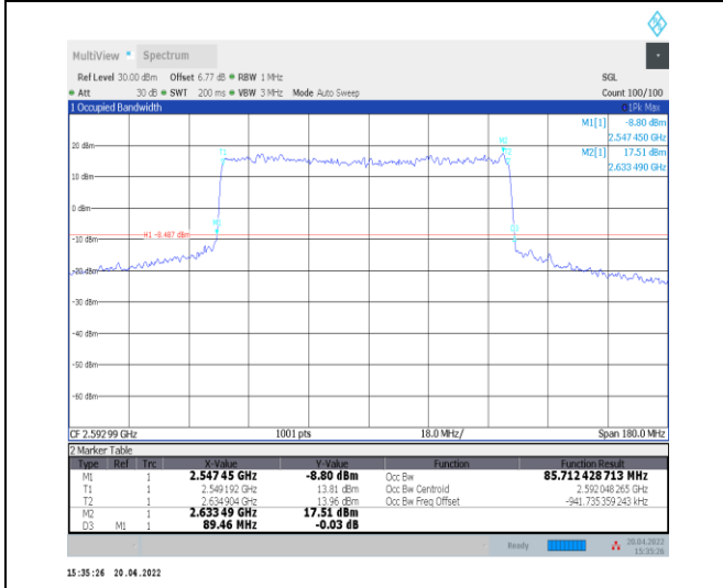
1-N41--30-90-M-1-DFT-QPSK-Outer_Full-240@0-Ant 0-85.712-89.460-≤90-PASS
