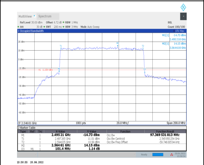
1-N41--30-100-L-8-CP-64QAM-Outer_Full-273@0-A nt0-97.37-101.400-≤100-PASS
