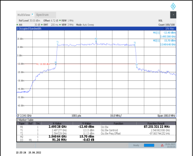
1-N41--30-90-L-7-CP-16QAM-Outer_Full-245@0-Ant0 t0-87.251-91.260-≤90-PASS
