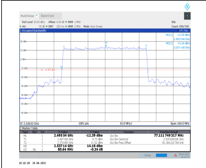
1-N41--30-80-L-5-DFT-256QAM-Outer_Full-216@0-A Ant0-77.112-80.640-<80-PASS
