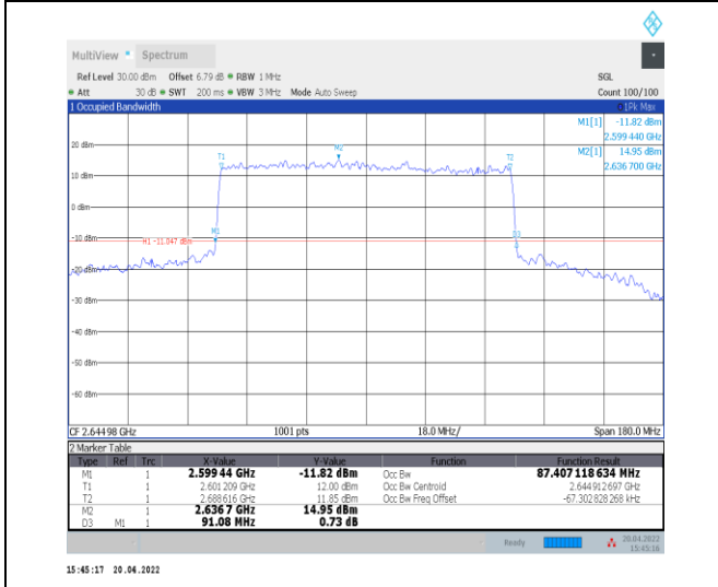
1-N41--30-90-H-8-CP-64QAM-Outer_Full-245@0-An t0-87.407-91.080-≤90-PASS
