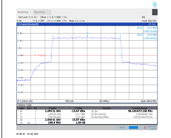
1-N41--30-100-L-3-DFT-16QAM-Outer_Full-270@0-Ant0-96.106-100.400-<=100-PASS
