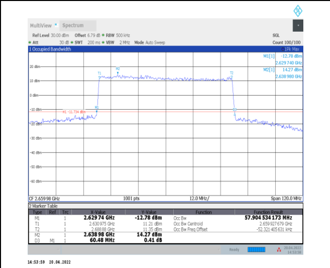
1-N41--30-60-H-6-CP-QPSK-Outer_Full-162@0-Ant 0-57.905-60.480-<math>\leq 60</math>-PASS
