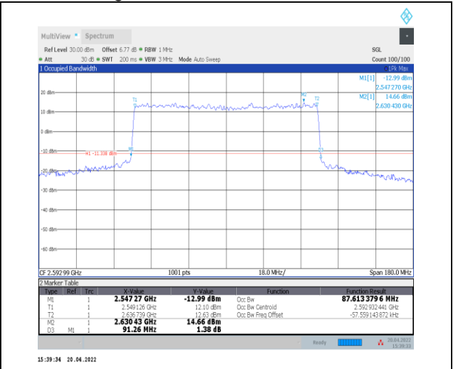
1-N41--30-90-M-8-CP-64QAM-Outer_Full-245@0-A nt0-87.613-91.260-<=90-PASS
