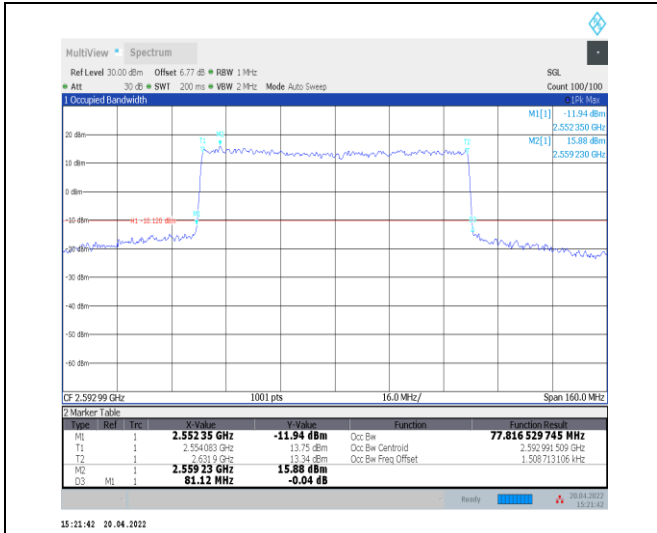
1-N41--30-80-M-6-CP-QPSK-Outer_Full-217@0-Ant 0-77.817-81.120-<80-PASS
