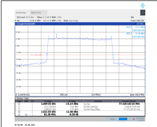
1-N41--30-80-H-9-CP-256QAM-Outer_Full-217@0-A nt0-77.428-81.280-≤80-PASS
