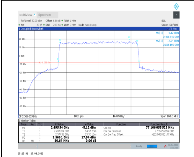
1-N41--30-80-L-1-DFT-QPSK-Outer_Full-216@0-Ant0-77.106-80.640-≤80-PASS
