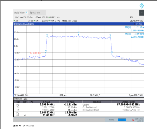
1-N41--30-90-H-7-CP-16QAM-Outer_Full-245@0-An t0-87.387-91.080-≤90-PASS
