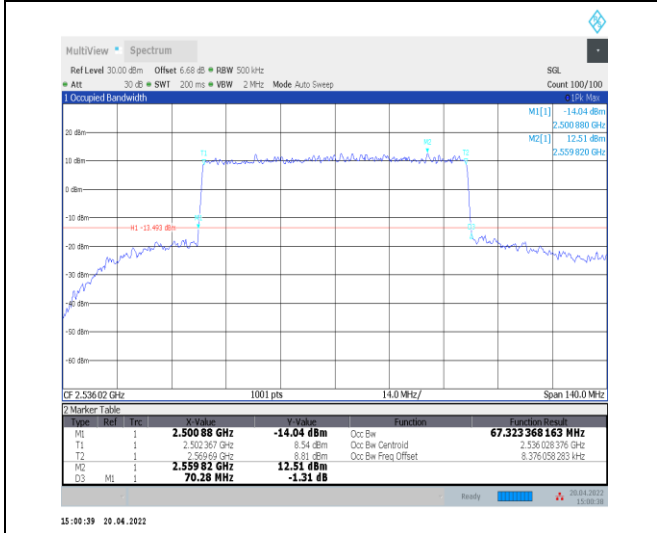
1-N41--30-70-L-8-CP-64QAM-Outer_Full-189@0-Ant0 0-67.323-70.280-≤70-PASS
