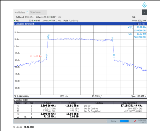
1-N41--30-90-H-9-CP-256QAM-Outer_Full-245@0-A nt0-87.188-91.260-≤90-PASS
