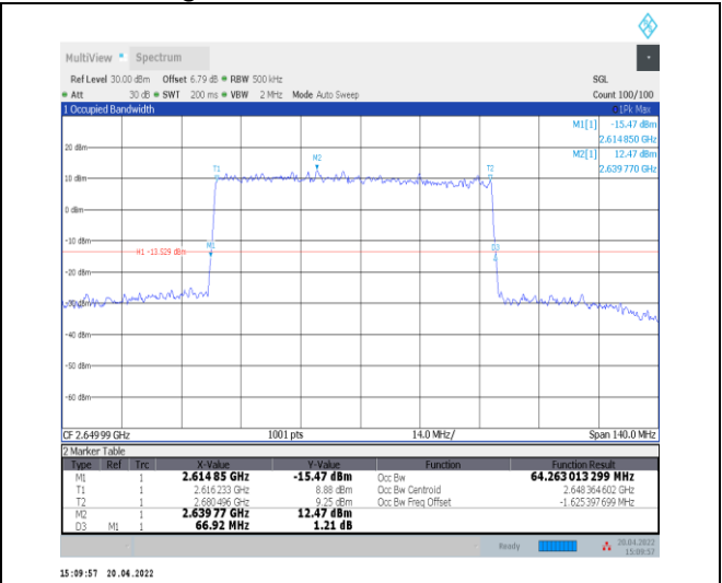
1-N41--30-70-H-5-DFT-256QAM-Outer_Full-180@0-A Ant0-64.263-66.920-≤70-PASS
