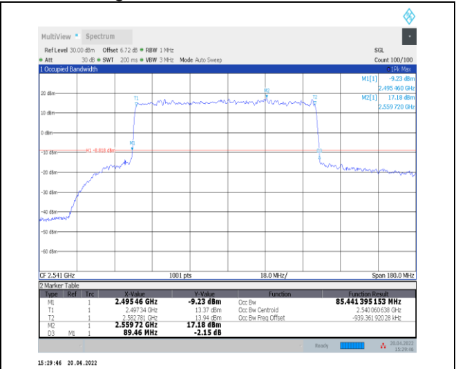
1-N41--30-90-L-1-DFT-QPSK-Outer_Full-240@0-Ant 0-85.441-89.460-≤90-PASS
