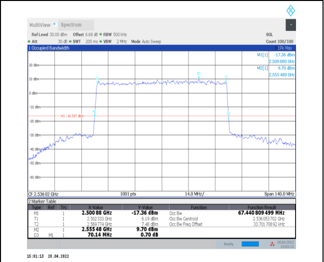
1-N41--30-70-L-9-CP-256QAM-Outer_Full-189@0-Ant0 -67.441-70.140-≤70-PASS
