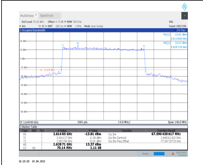
1-N41--30-70-H-6-CP-QPSK-Outer_Full-189@0-Ant 0-67.59-70.140-≤70-PASS
