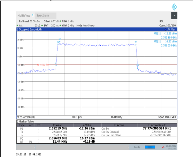
1-N41--30-80-M-7-CP-16QAM-Outer_Full-217@0-Ant nt0-77.774-81.440-<80-PASS
