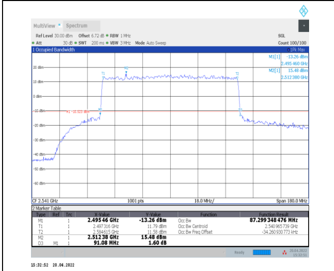
1-N41--30-90-L-6-CP-QPSK-Outer_Full-245@0-Ant0 -87.299-91.080-≤90-PASS
