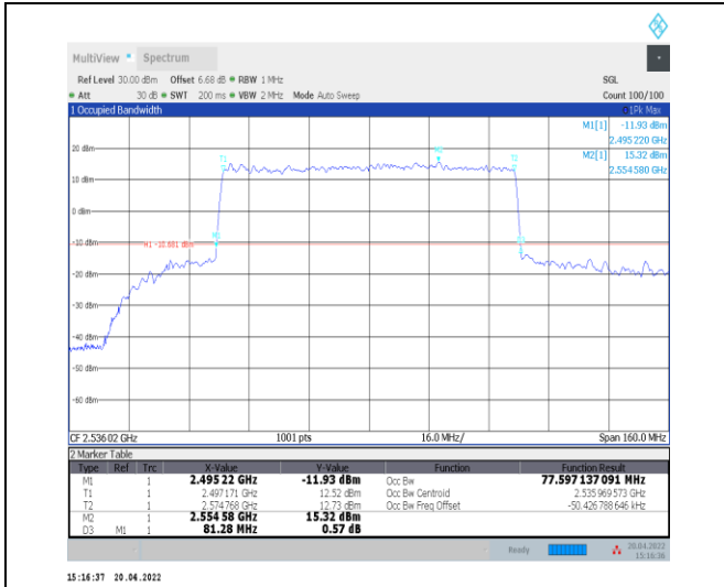
1-N41--30-80-L-7-CP-16QAM-Outer_Full-217@0-Ant 0-77.597-81.280-≤80-PASS
