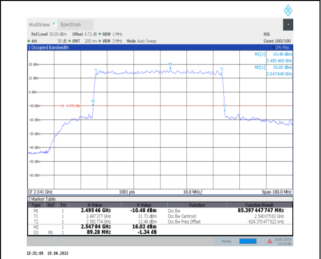
1-N41--30-90-L-3-DFT-16QAM-Outer_Full-240@0-A nt0-85.397-89.280-≤90-PASS
