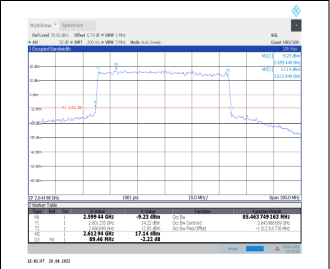
1-N41--30-90-H-1-DFT-QPSK-Outer_Full-240@0-An t0-85.464-89.460-<=90-PASS
