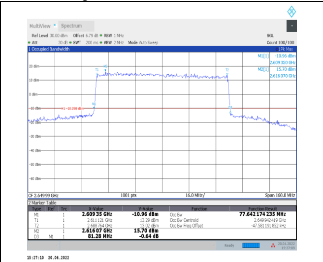
1-N41--30-80-H-6-CP-QPSK-Outer_Full-217@0-Ant0-77.642-81.280-<=80-PASS
