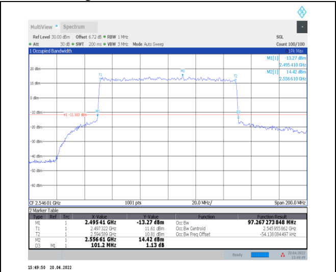
1-N41--30-100-L-6-CP-QPSK-Outer_Full-273@0-An t0-97.267-101.200-≤100-PASS
