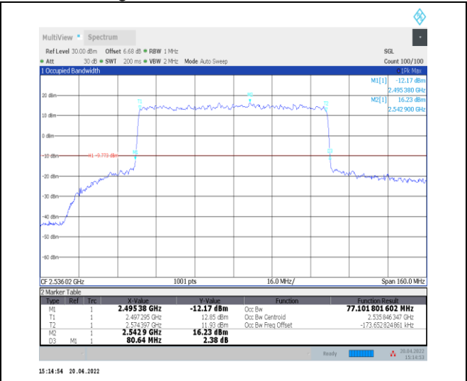
1-N41--30-80-L-4-DFT-64QAM-Outer_Full-216@0-A nt0-77.102-80.640-<80-PASS
