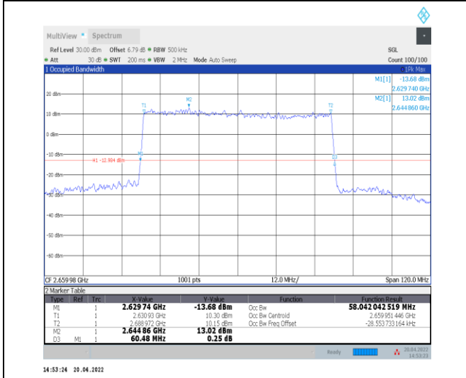
1-N41--30-60-H-5-DFT-256QAM-Outer_Full-162@0-A Ant0-58.042-60.480-<math>\leq 60</math>-PASS
