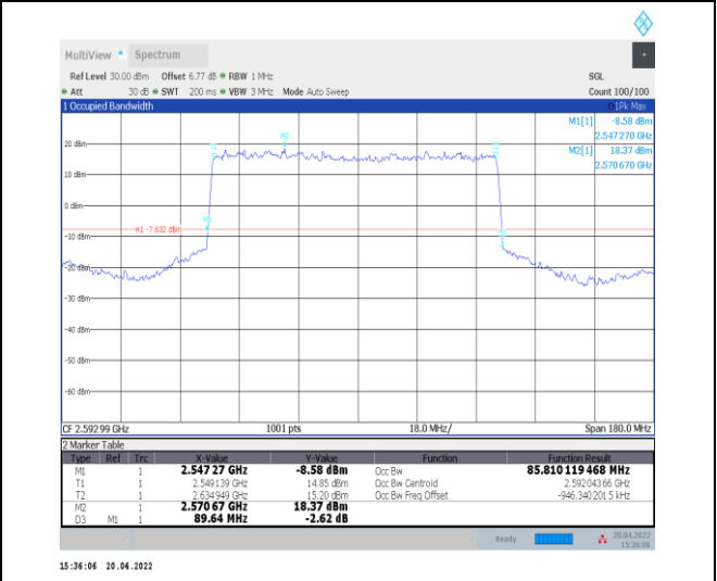
1-N41--30-90-M-2-DFT-PI2BPSK-Outer_Full-240@0-Ant 0-85.81-89.640-≤90-PASS
