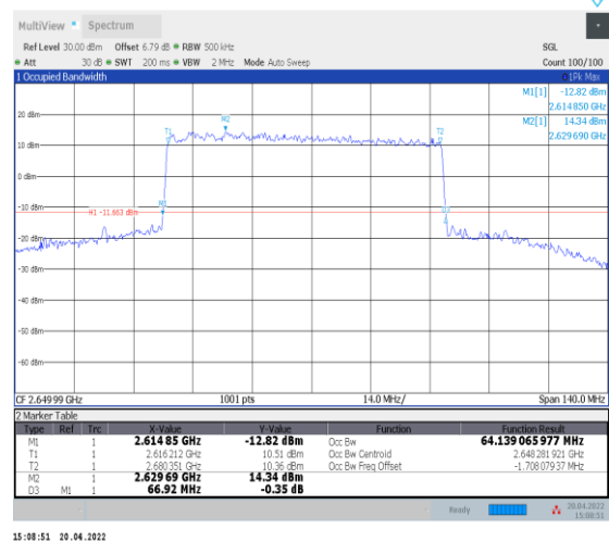
1-N41--30-70-H-3-DFT-16QAM-Outer_Full-180@0-A nt0-64.139-66.920-≤70-PASS
