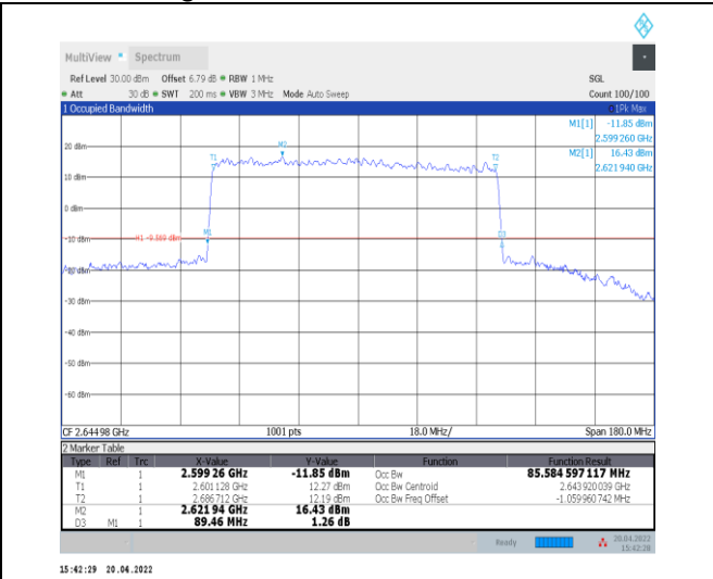
1-N41--30-90-H-3-DFT-16QAM-Outer_Full-240@0-A nt0-85.585-89.460-≤90-PASS
