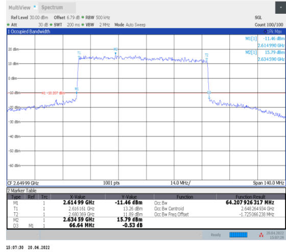
1-N41--30-70-H-1-DFT-QPSK-Outer_Full-180@0-An t0-64.208-66.640-≤70-PASS
