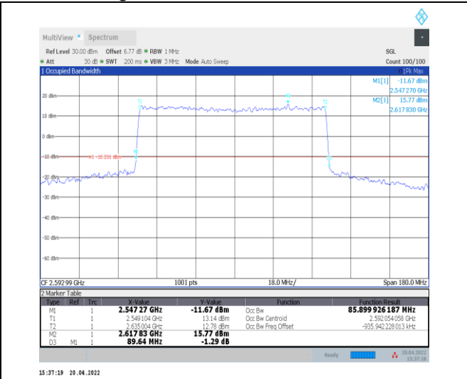
1-N41--30-90-M-4-DFT-64QAM-Outer_Full-240@0-A Ant0-85.9-89.640-≤90-PASS
