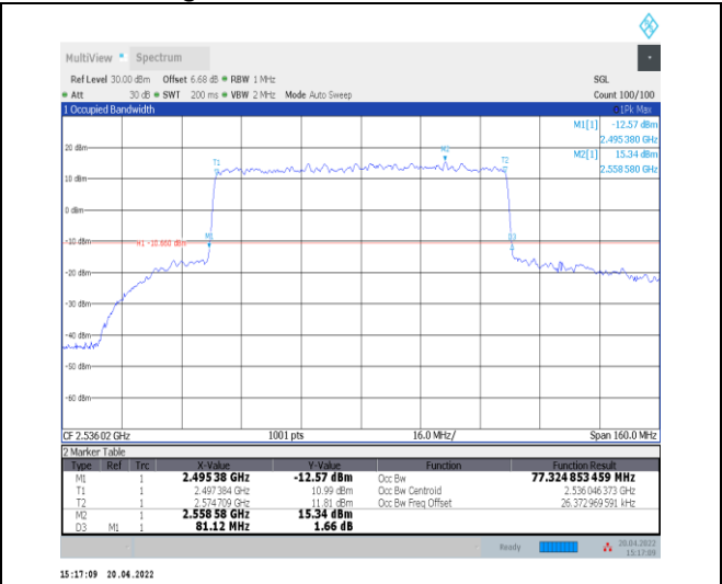
1-N41--30-80-L-8-CP-64QAM-Outer_Full-217@0-An t0-77.325-81.120-≤80-PASS
