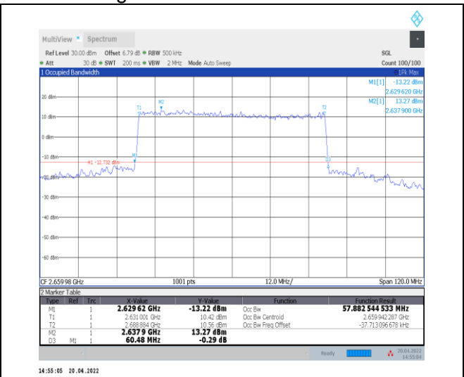
1-N41--30-60-H-8-CP-64QAM-Outer_Full-162@0-An t0-57.883-60.480-≤60-PASS
