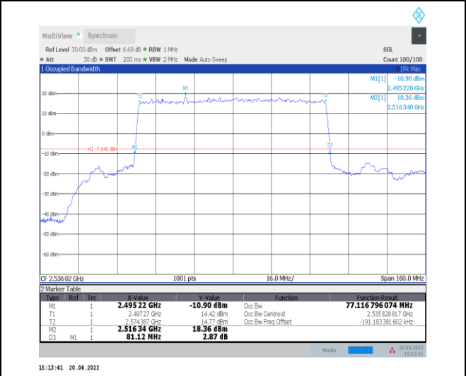
1-N41--30-80-L-2-DFT-PI2BPSK-Outer_Full-216@0-Ant0-77.117-81.120-≤80-PASS
