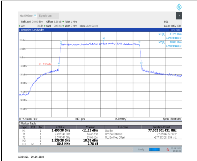
1-N41--30-80-L-3-DFT-16QAM-Outer_Full-216@0-A nt0-77.002-80.800-<80-PASS
