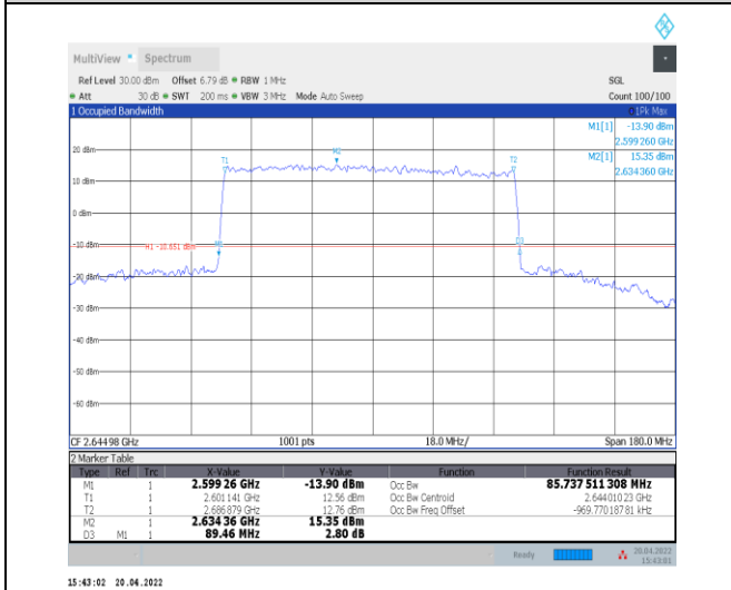
1-N41--30-90-H-4-DFT-64QAM-Outer_Full-240@0-A nt0-85.738-89.460-≤90-PASS
