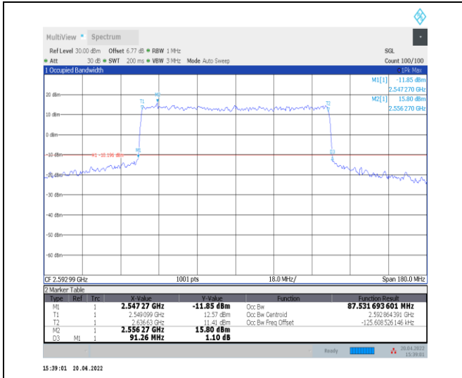
1-N41--30-90-M-7-CP-16QAM-Outer_Full-245@0-An t0-87.532-91.260-<=90-PASS
