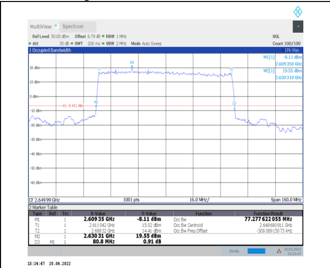
1-N41--30-80-H-2-DFT-PI2BPSK-Outer_Full-216@0-Ant0-77.278-80.800-<math>\leq 80</math>-PASS
