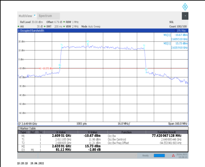
1-N41--30-80-H-8-CP-64QAM-Outer_Full-217@0-Ant0-77.42-81.120-<=80-PASS
