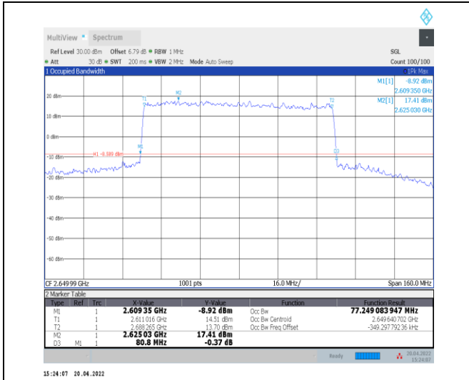
1-N41--30-80-H-1-DFT-QPSK-Outer_Full-216@0-An t0-77.249-80.800-<math>\leq 80</math>-PASS
