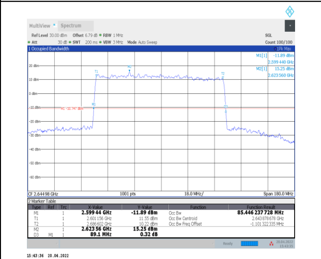
1-N41--30-90-H-5-DFT-256QAM-Outer_Full-240@0-A Ant0-85.446-89.100-≤90-PASS
