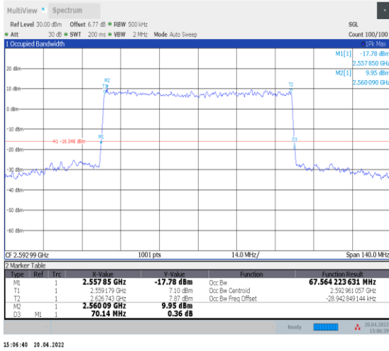
1-N41--30-70-M-9-CP-256QAM-Outer_Full-189@0-A nt0-67.564-70.140-≤70-PASS
