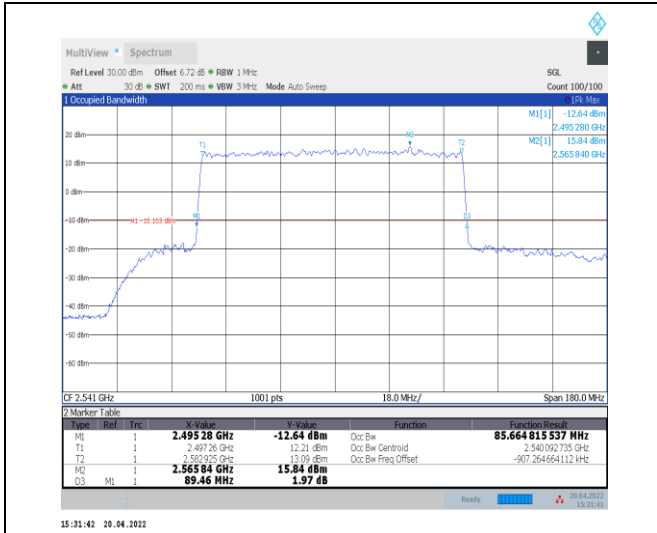
1-N41--30-90-L-4-DFT-64QAM-Outer_Full-240@0-A nt0-85.665-89.460-≤90-PASS
