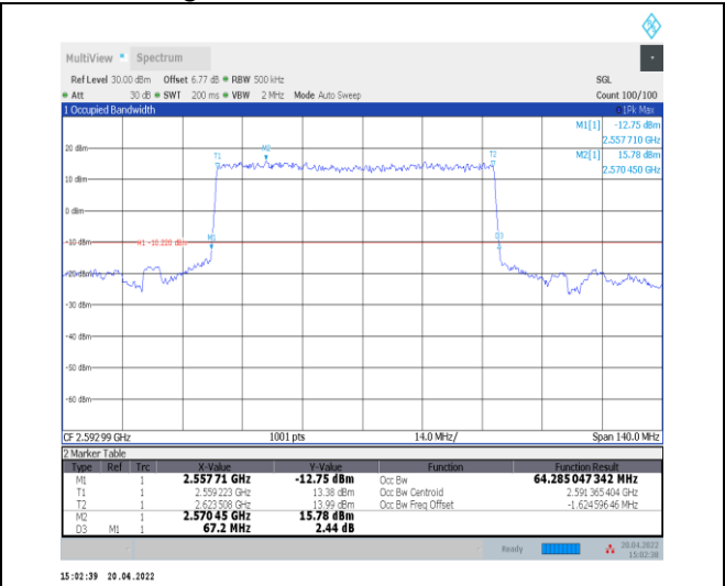
1-N41--30-70-M-2-DFT-PI2BPSK-Outer_Full-180@0-Ant0-64.285-67.200-≤70-PASS
