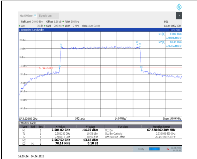
1-N41--30-70-L-6-CP-QPSK-Outer_Full-189@0-Ant0 -67.529-70.140-≤70-PASS
