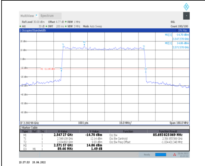
1-N41--30-90-M-5-DFT-256QAM-Outer_Full-240@0-A Ant0-85.694-89.460-≤90-PASS
