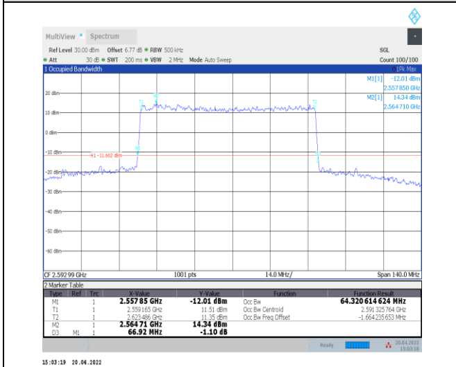
1-N41--30-70-M-3-DFT-16QAM-Outer_Full-180@0-Ant0-64.321-66.920-≤70-PASS
