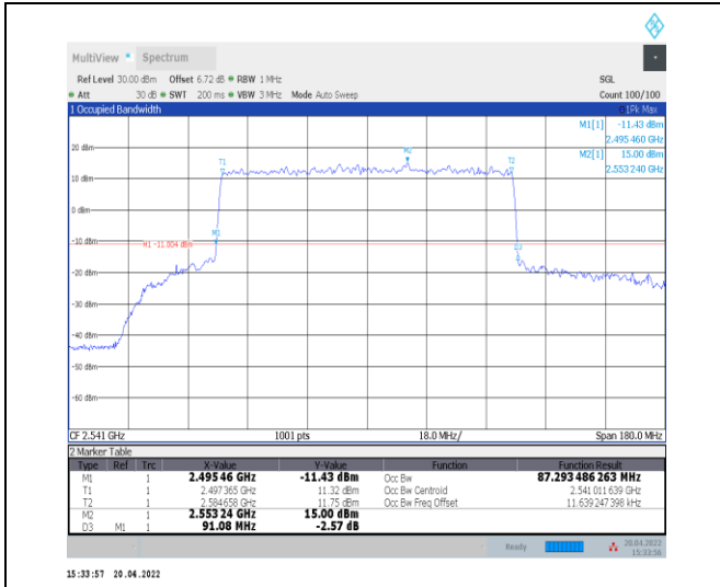
1-N41--30-90-L-8-CP-64QAM-Outer_Full-245@0-Ant 0-87.293-91.080-≤90-PASS
