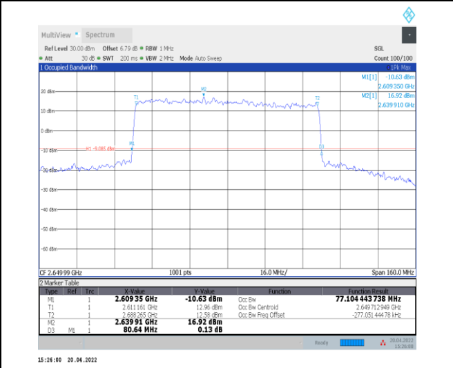
1-N41--30-80-H-4-DFT-64QAM-Outer_Full-216@0-A nt0-77.104-80.640-<math>\leq 80</math>-PASS
