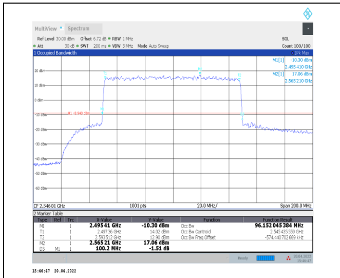
1-N41--30-100-L-1-DFT-QPSK-Outer_Full-270@0-A nt0-96.152-100.200-<=100-PASS
