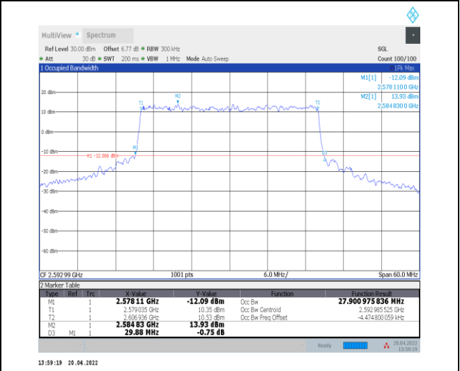
1-N41--30-30-M-8-CP-64QAM-Outer_Full-78@0-Ant 0-27.901-29.880-≤30-PASS
