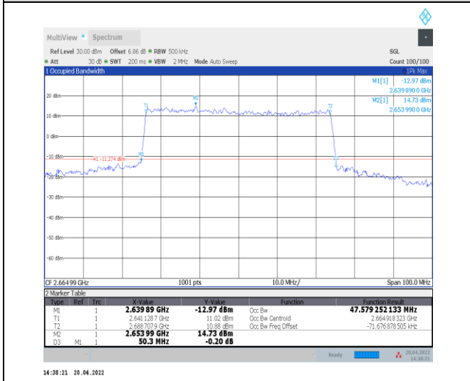
1-N41--30-50-H-8-CP-64QAM-Outer_Full-133@0-Ant 0-47.579-50.300-≤50-PASS
