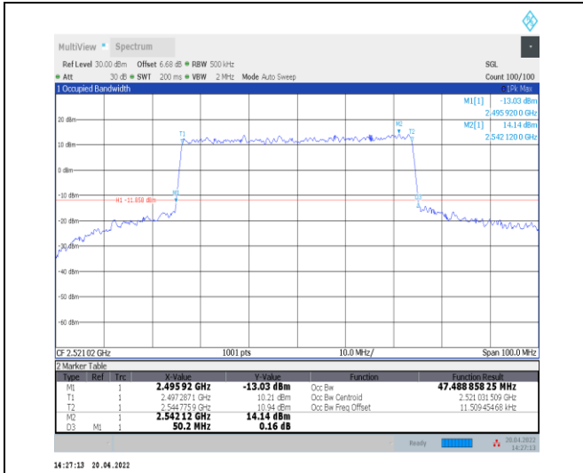
1-N41--30-50-L-8-CP-64QAM-Outer_Full-133@0-Ant 0-47.489-50.200-≤50-PASS
