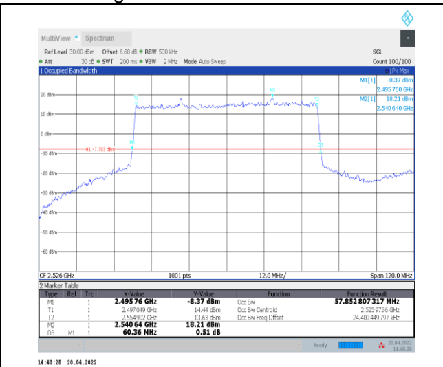
1-N41--30-60-L-2-DFT-PI2BPSK-Outer_Full-162@0-Ant0-57.853-60.360-≤60-PASS
