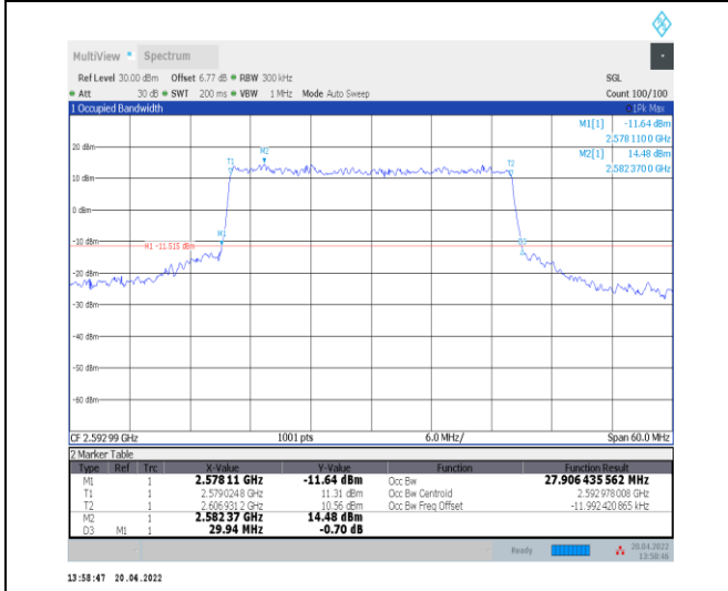
1-N41--30-30-M-7-CP-16QAM-Outer_Full-78@0-Ant 0-27.906-29.940-≤30-PASS
