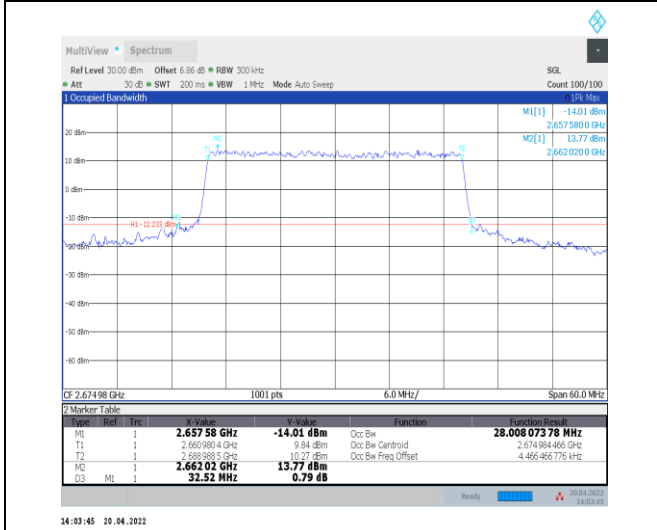
1-N41--30-30-H-6-CP-QPSK-Outer_Full-78@0-Ant0 28.008-32.520-<30-PASS
