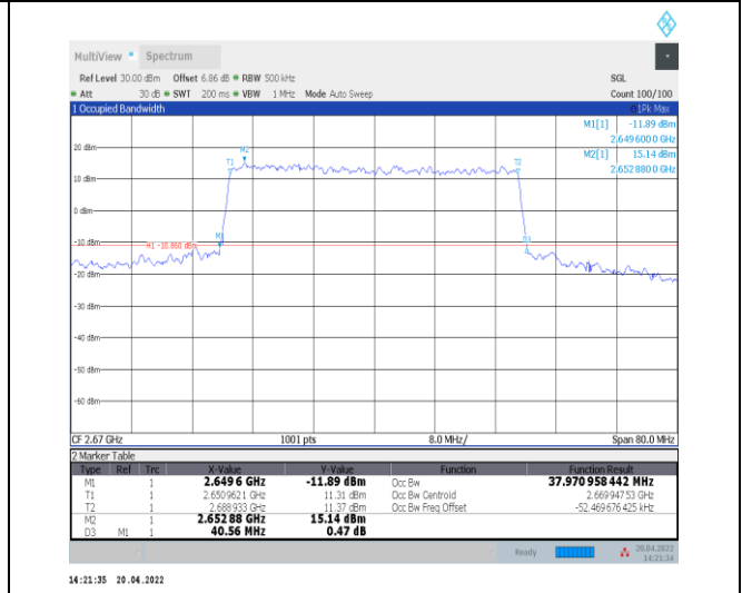
1-N41--30-40-H-8-CP-64QAM-Outer_Full-106@0-Ant0-37.971-40.560-<math>\leq 40</math>-PASS
