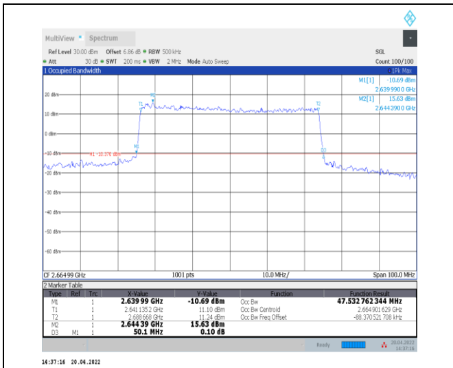
1-N41--30-50-H-6-CP-QPSK-Outer_Full-133@0-Ant 0-47.533-50.100-≤50-PASS
