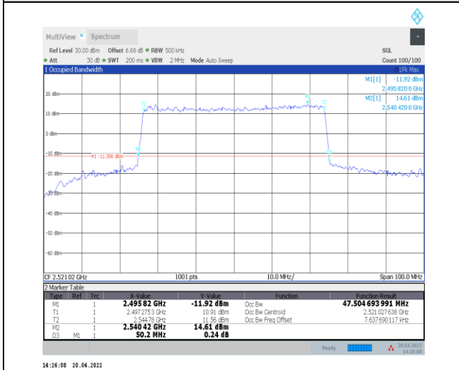
1-N41--30-50-L-6-CP-QPSK-Outer_Full-133@0-Ant0 -47.505-50.200-≤50-PASS
