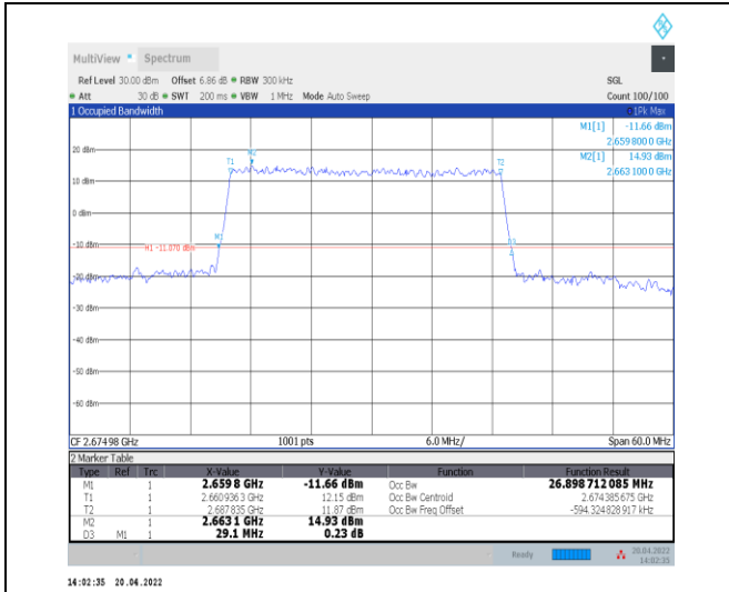
1-N41--30-30-H-4-DFT-64QAM-Outer_Full-75@0-Ant t0-26.899-29.100-<30-PASS
