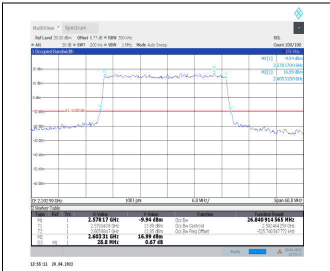
1-N41--30-30-M-1-DFT-QPSK-Outer_Full-75@0-Ant 0-26.841-28.800-≤30-PASS
