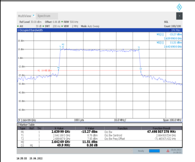
1-N41--30-50-H-9-CP-256QAM-Outer_Full-133@0-Ant 0-47.499-49.900-≤50-PASS
