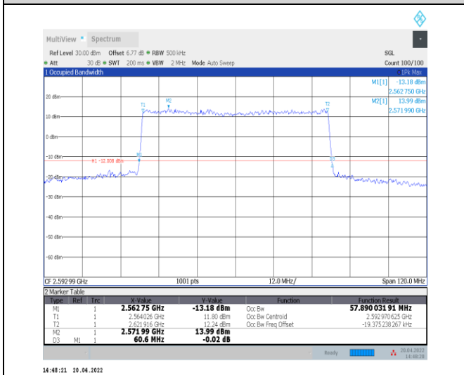
1-N41--30-60-M-6-CP-QPSK-Outer_Full-162@0-Ant 0-57.89-60.600-≤60-PASS
