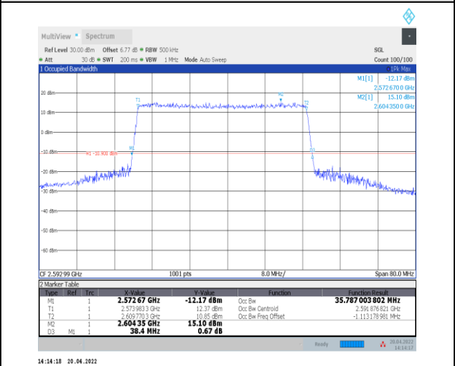
1-N41--30-40-M-5-DFT-256QAM-Outer_Full-100@0-Ant0-35.787-38.400-≤40-PASS
