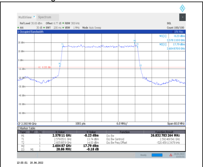
1-N41--30-30-M-2-DFT-PI2BPSK-Outer_Full-75@0-Ant 0-26.833-28.860-≤30-PASS
