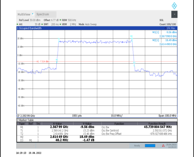
1-N41--30-50-M-2-DFT-PI2BPSK-Outer_Full-128@0 -Ant0-45.74-48.200-≤50-PASS
