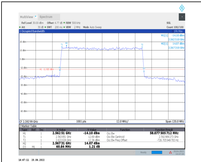
1-N41--30-60-M-4-DFT-64QAM-Outer_Full-162@0-A nt0-58.078-60.840-≤60-PASS
