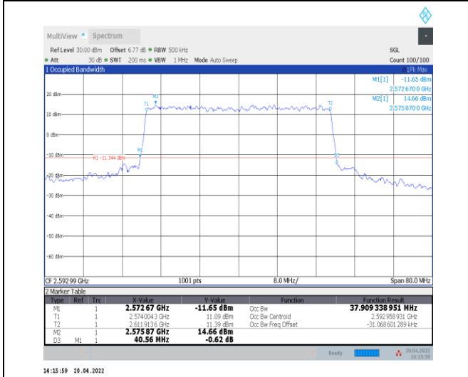
1-N41--30-40-M-8-CP-64QAM-Outer_Full-106@0-Ant t0-37.909-40.560-≤40-PASS
