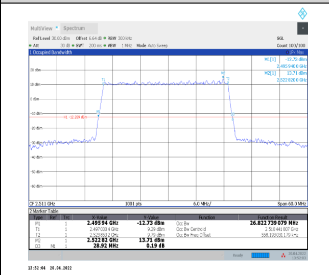
1-N41--30-30-L-5-DFT-256QAM-Outer_Full-75@0-A nt0-26.823-28.920-≤30-PASS
