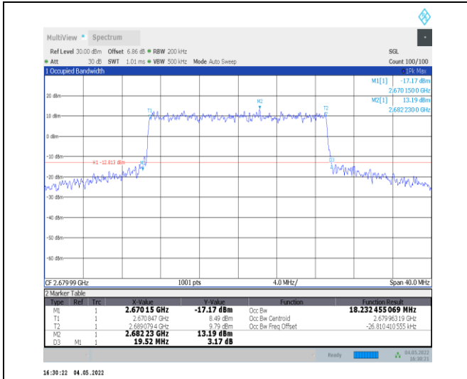
1-N41--30-20-H-7-CP-16QAM-Outer_Full-51@0-Ant 0-18.232-19.520-≤20-PASS
