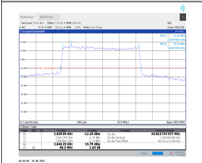
1-N41--30-50-H-4-DFT-64QAM-Outer_Full-128@0-A nt0-45.816-48.300-≤50-PASS
