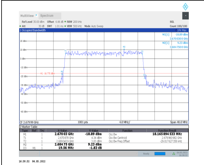
1-N41--30-20-H-9-CP-256QAM-Outer_Full-51@0-Ant t0-18.166-19.560-≤20-PASS
