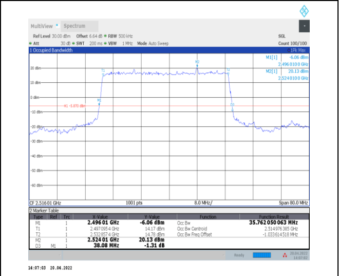
1-N41--30-40-L-2-DFT-PI2BPSK-Outer_Full-100@0- Ant0-35.762-38.080-<math>\leq</math>40-PASS
