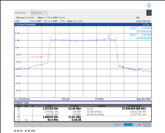
1-N41--30-40-M-9-CP-256QAM-Outer_Full-106@0-Ant Ant0-37.941-40.400-≤40-PASS
