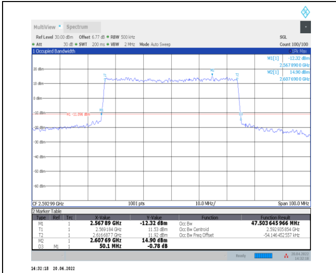
1-N41--30-50-M-7-CP-16QAM-Outer_Full-133@0-An t0-47.504-50.100-<=50-PASS
