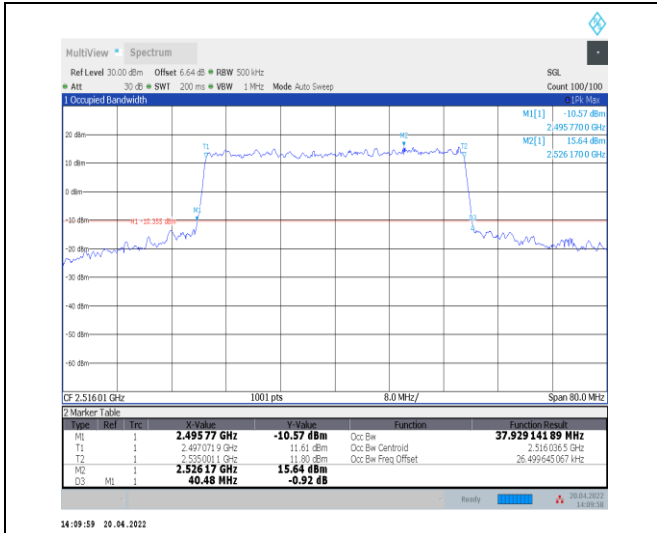
1-N41--30-40-L-7-CP-16QAM-Outer_Full-106@0-Ant 0-37.929-40.480-≤40-PASS
