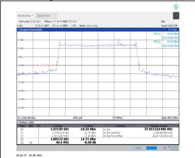
1-N41--30-40-M-7-CP-16QAM-Outer_Full-106@0-Ant nt0-37.913-40.400-≤40-PASS
