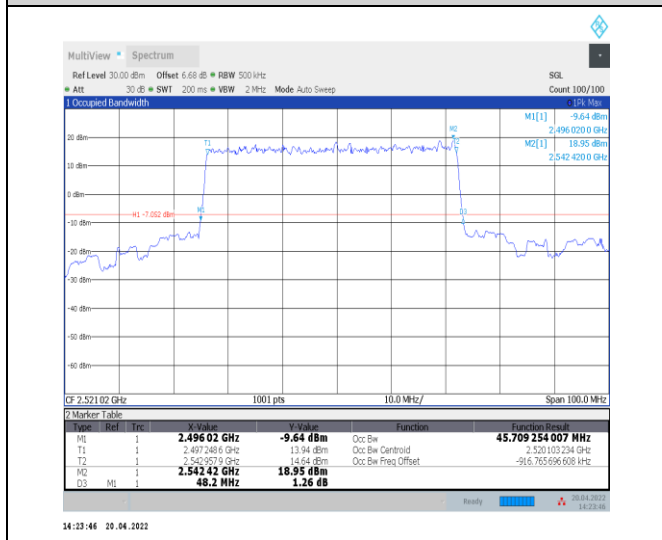
1-N41--30-50-L-2-DFT-PI2BPSK-Outer_Full-128@0-A Ant0-45.709-48.200-≤50-PASS
