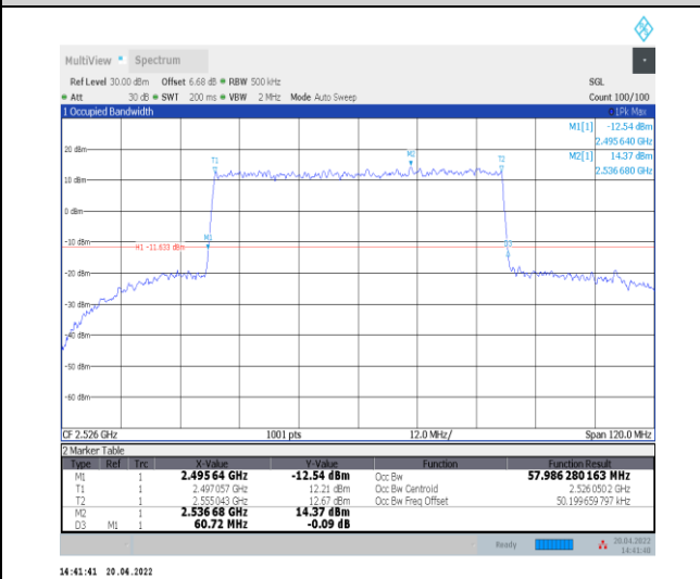
1-N41--30-60-L-4-DFT-64QAM-Outer_Full-162@0-A nt0-57.986-60.720-≤60-PASS
