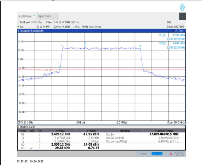
1-N41--30-30-L-7-CP-16QAM-Outer_Full-78@0-Ant0-27.896-29.880-≤30-PASS
