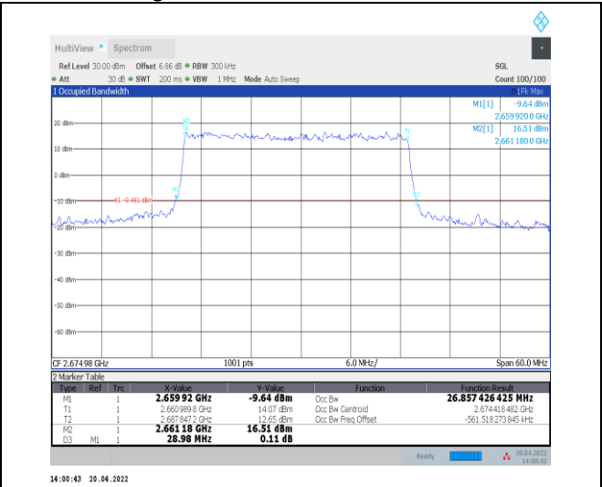
1-N41--30-30-H-1-DFT-QPSK-Outer_Full-75@0-Ant 0-26.857-28.980-<=30-PASS
