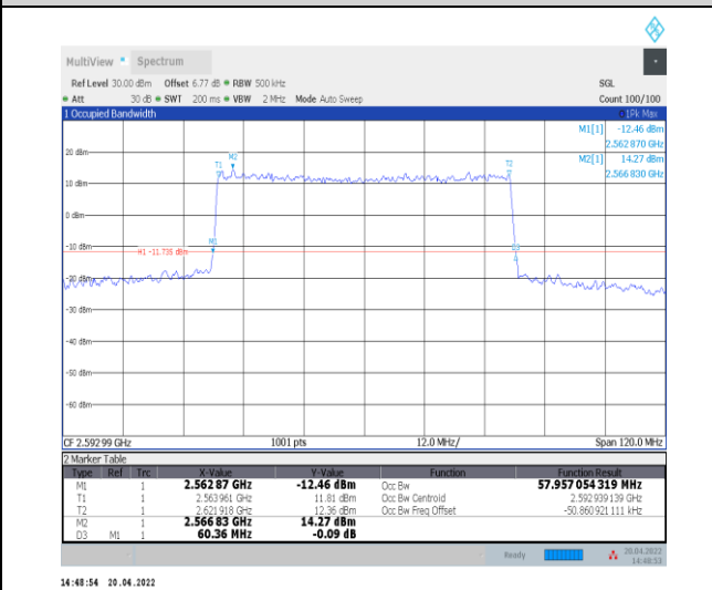
1-N41--30-60-M-7-CP-16QAM-Outer_Full-162@0-A nt0-57.957-60.360-≤60-PASS
