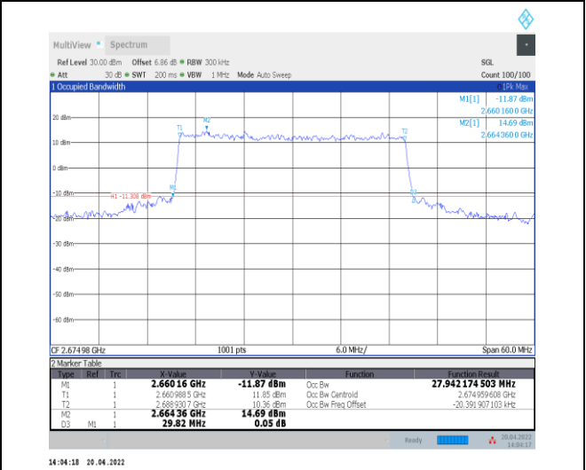
1-N41--30-30-H-7-CP-16QAM-Outer_Full-78@0-Ant 0-27.942-29.820-<30-PASS
