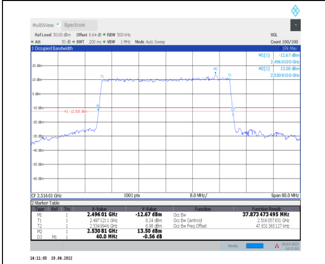
1-N41--30-40-L-9-CP-256QAM-Outer_Full-106@0-A nt0-37.873-40.000-≤40-PASS
