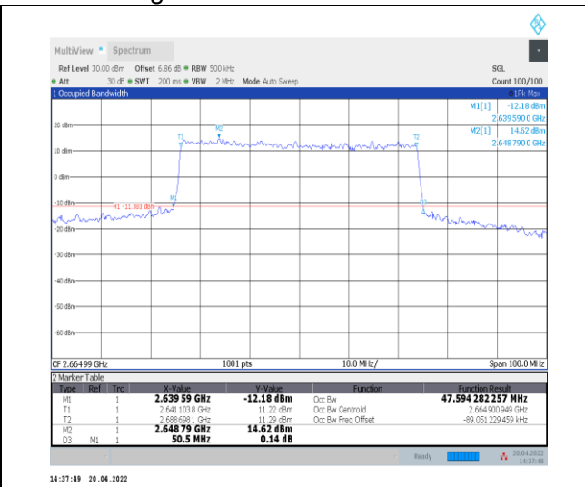
1-N41--30-50-H-7-CP-16QAM-Outer_Full-133@0-Ant 0-47.594-50.500-≤50-PASS
