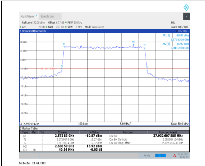
1-N41--30-40-M-6-CP-QPSK-Outer_Full-106@0-Ant 0-37.933-40.240-≤40-PASS
