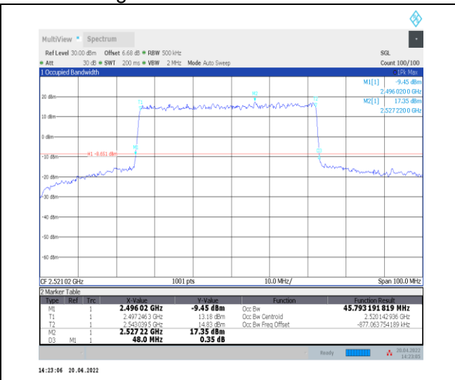
1-N41--30-50-L-1-DFT-QPSK-Outer_Full-128@0-Ant 0-45.793-48.000-≤50-PASS
