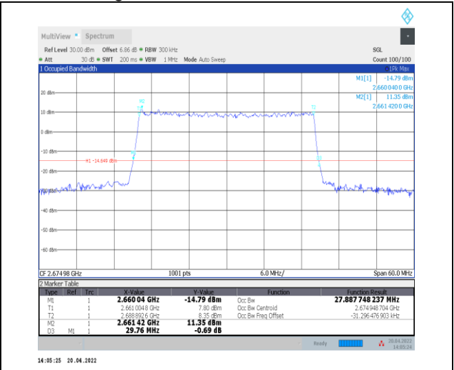
1-N41--30-30-H-9-CP-256QAM-Outer_Full-78@0-An t0-27.888-29.760-<math>\leq</math>30-PASS
