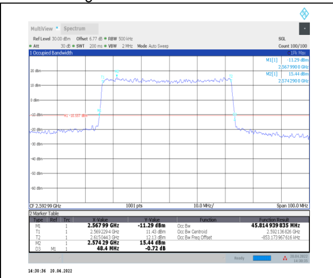
1-N41--30-50-M-4-DFT-64QAM-Outer_Full-128@0-A Ant0-45.815-48.400-≤50-PASS
