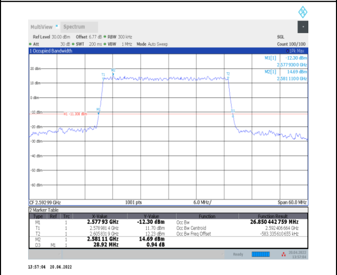
1-N41--30-30-M-4-DFT-64QAM-Outer_Full-75@0-Ant 0-26.85-28.920-≤30-PASS
