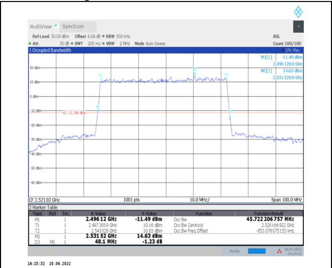
1-N41--30-50-L-5-DFT-256QAM-Outer_Full-128@0-A Ant0-45.722-48.100-≤50-PASS
