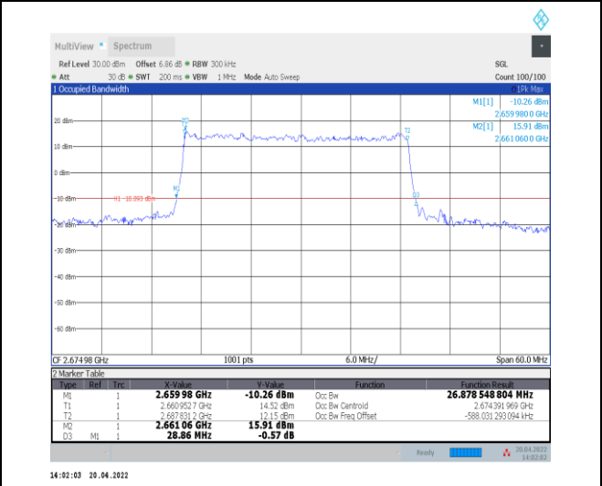
1-N41--30-30-H-3-DFT-16QAM-Outer_Full-75@0-An t0-26.879-28.860-<=30-PASS
