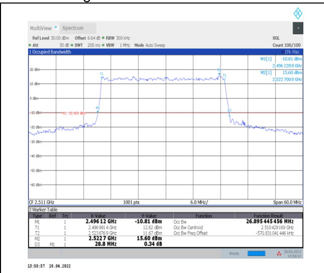
1-N41--30-30-L-3-DFT-16QAM-Outer_Full-75@0-An t0-26.895-28.800-≤30-PASS
