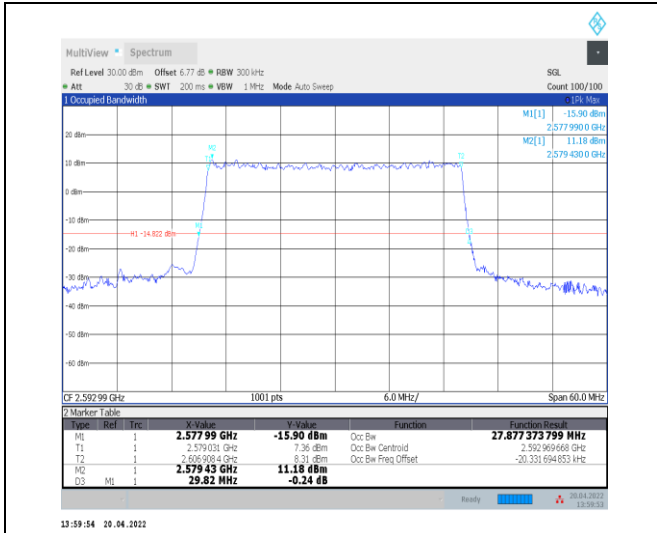
1-N41--30-30-M-9-CP-256QAM-Outer_Full-78@0-An t0-27.877-29.820-<=30-PASS
