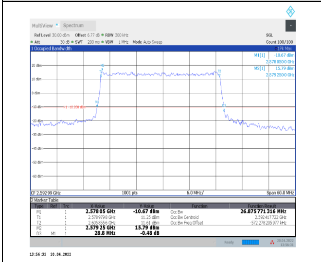
1-N41--30-30-M-3-DFT-16QAM-Outer_Full-75@0-Ant 0-26.876-28.800-≤30-PASS
