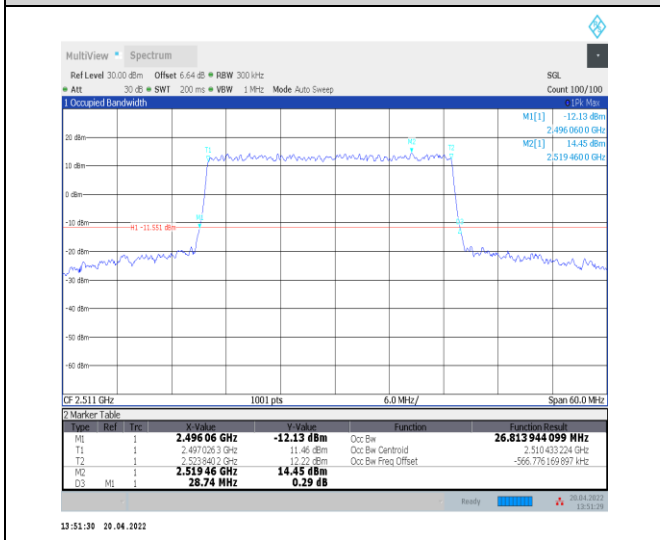
1-N41--30-30-L-4-DFT-64QAM-Outer_Full-75@0-Ant 0-26.814-28.740-≤30-PASS
