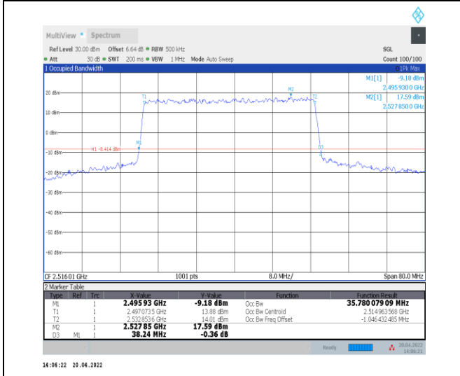
1-N41--30-40-L-1-DFT-QPSK-Outer_Full-100@0-Ant 0-35.78-38.240-<math>\leq</math>40-PASS
