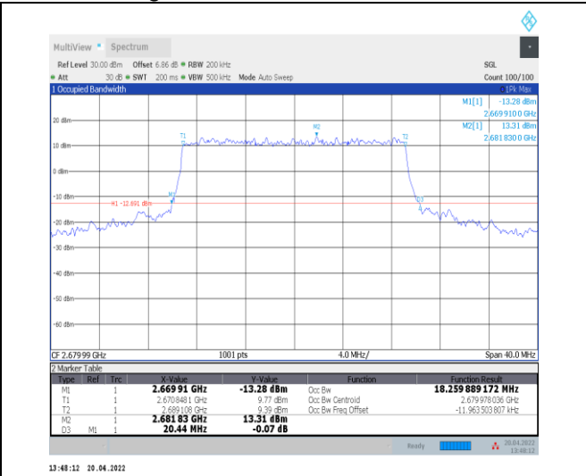
1-N41--30-20-H-8-CP-64QAM-Outer_Full-51@0-Ant 0-18.26-20.440-≤20-PASS
