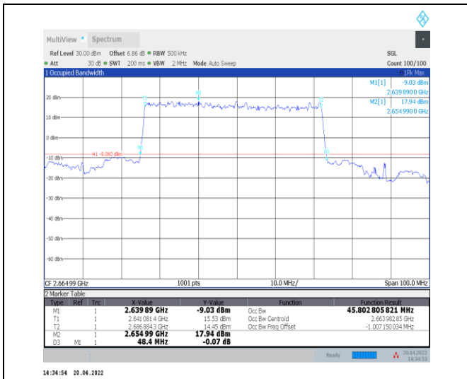
1-N41--30-50-H-2-DFT-PI2BPSK-Outer_Full-128@0-A Ant0-45.803-48.400-≤50-PASS
