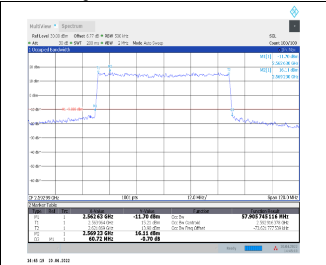
1-N41--30-60-M-1-DFT-QPSK-Outer_Full-162@0-An t0-57.906-60.720-≤60-PASS
