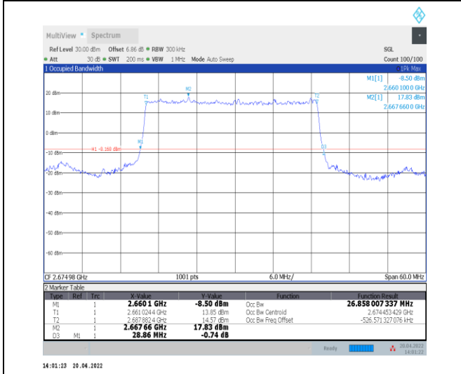
1-N41--30-30-H-2-DFT-PI2BPSK-Outer_Full-75@0-Ant0-26.858-28.860-<=30-PASS
