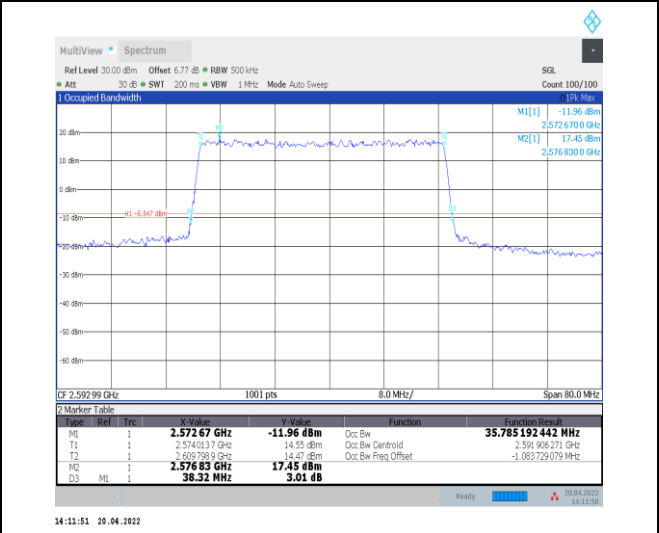
1-N41--30-40-M-1-DFT-QPSK-Outer_Full-100@0-An t0-35.785-38.320-≤40-PASS
