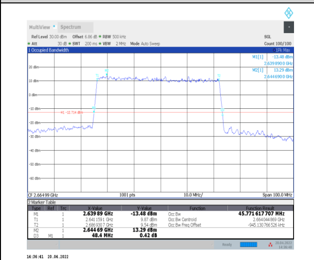
1-N41--30-50-H-5-DFT-256QAM-Outer_Full-128@0-A Ant0-45.772-48.400-≤50-PASS
