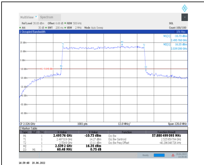
1-N41--30-60-L-1-DFT-QPSK-Outer_Full-162@0-Ant 0-57.88-60.480-≤60-PASS
