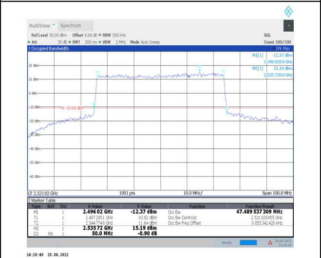
1-N41--30-50-L-7-CP-16QAM-Outer_Full-133@0-Ant0 t0-47.49-50.000-≤50-PASS
