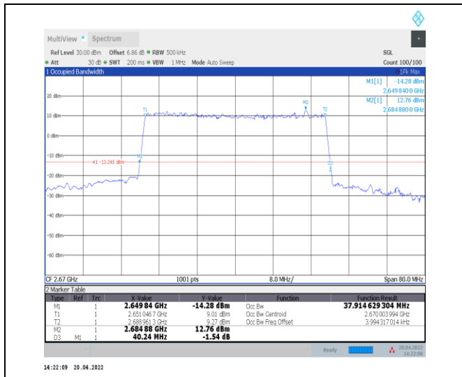
1-N41--30-40-H-9-CP-256QAM-Outer_Full-106@0-A nt0-37.915-40.240-≤40-PASS
