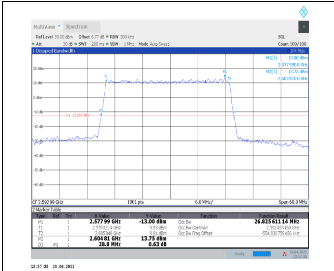
1-N41--30-30-M-5-DFT-256QAM-Outer_Full-75@0-A nt0-26.826-28.800-≤30-PASS
