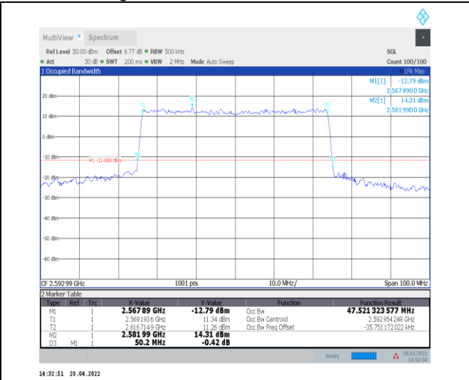
1-N41--30-50-M-8-CP-64QAM-Outer_Full-133@0-A nt0-47.521-50.200-<=50-PASS
