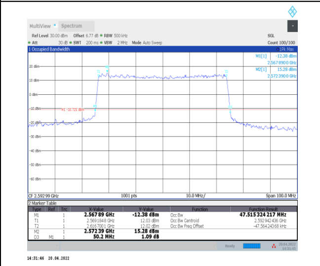
1-N41--30-50-M-6-CP-QPSK-Outer_Full-133@0-Ant 0-47.515-50.200-≤50-PASS
