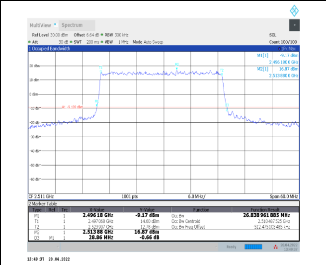
1-N41--30-30-L-1-DFT-QPSK-Outer_Full-75@0-Ant0 -26.839-28.860-≤30-PASS
