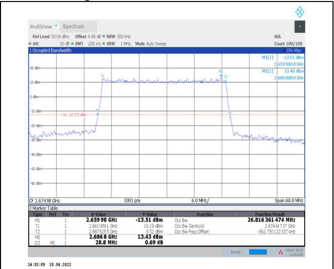
1-N41--30-30-H-5-DFT-256QAM-Outer_Full-75@0-Ant nt0-26.816-28.800-<30-PASS
