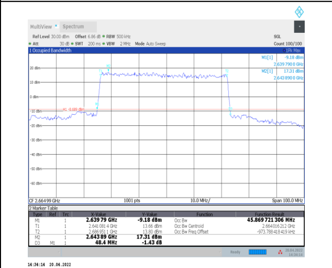
1-N41--30-50-H-1-DFT-QPSK-Outer_Full-128@0-An t0-45.87-48.400-<=50-PASS
