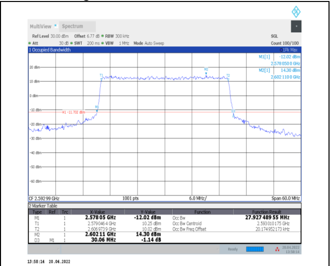
1-N41--30-30-M-6-CP-QPSK-Outer_Full-78@0-Ant0 -27.927-30.060-≤30-PASS
