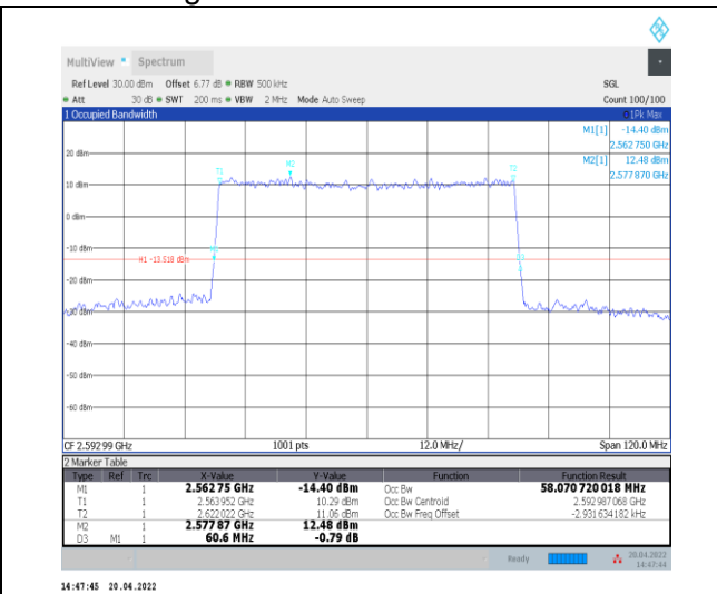
1-N41--30-60-M-5-DFT-256QAM-Outer_Full-162@0-A Ant0-58.071-60.600-≤60-PASS
