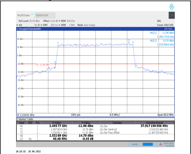
1-N41--30-40-L-8-CP-64QAM-Outer_Full-106@0-An t0-37.917-40.480-≤40-PASS
